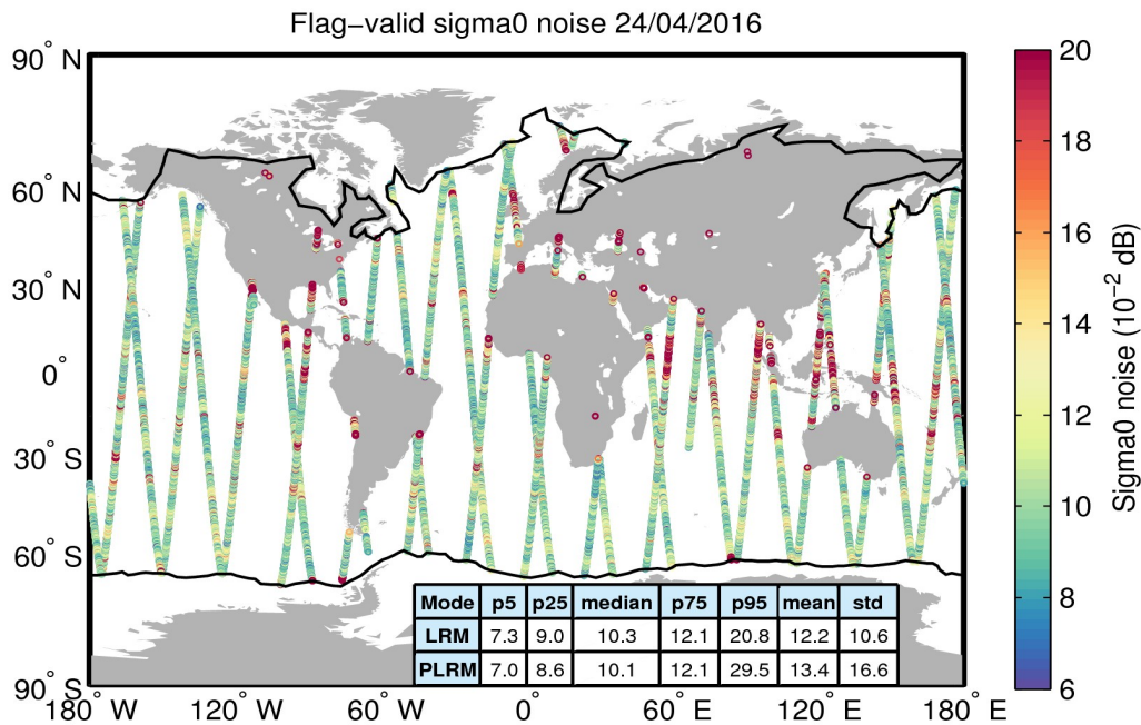
Figure 26. Geographical distribution of flag-valid 20-Hz sigma0 measurement noise over oceans and lakes for 24/04/2016. The statistical values shown in the table refer to the sigma0 noise and are calculated separately for LRM and PLRM regions. Measurements taken over polar polygons have been excluded from the computation of the statistical values. The black lines mark the outer limit of the Arctic and Antarctic polar polygons.
