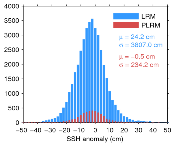
Figure 7. Histogram of flag-valid SSH anomaly over oceans and lakes for LRM (blue) and PLRM (red) for 24/04/2016. The mean ( \mu ) and standard deviation ( \sigma ) are also shown. Note that values outside [-50 50] cm are excluded from the histogram for the sake of readability but not from the computation of \mu and \sigma .
