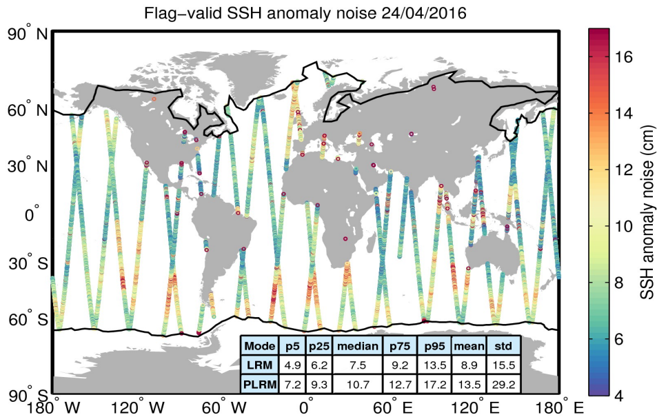
Figure 8. Geographical distribution of flag-valid 20-Hz SSH anomaly measurement noise over oceans and lakes for 24/04/2016. The statistical values shown in the table refer to the SSH anomaly noise and are calculated separately for LRM and PLRM regions. Measurements taken over polar polygons have been excluded from the computation of the statistical values. The black lines mark the outer limit of the Arctic and Antarctic polar polygons.
