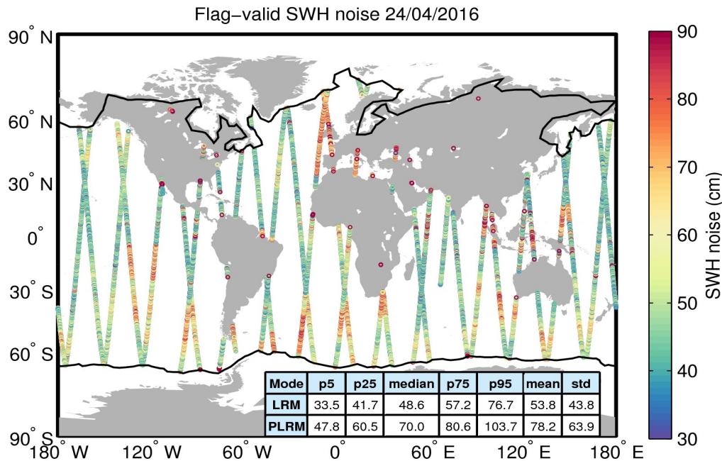
Figure 18. Geographical distribution of flag-valid 20-Hz SWH measurement noise over oceans and lakes for 24/04/2016. The statistical values shown in the table refer to the SWH noise and are calculated separately for LRM and PLRM regions. Measurements taken over polar polygons have been excluded from the computation of the statistical values. The black lines mark the outer limit of the Arctic and Antarctic polar polygons.
