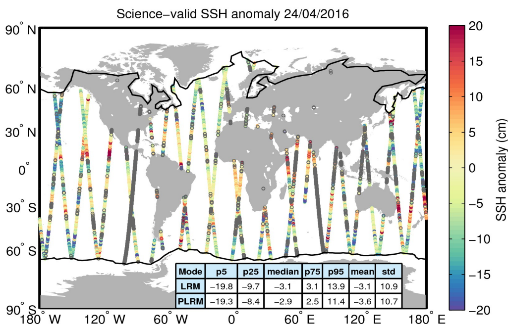
Figure 10. Geographical distribution of science-valid SSH anomaly data over oceans and lakes for 24/04/2016. The statistical values shown in the table refer to the SSH anomaly in cm and are calculated separately for LRM and PLRM regions. The black lines mark the outer limit of the Arctic and Antarctic polar polygons. Gray circles denote records that have been rejected based on the editing criteria described in Table 2.
