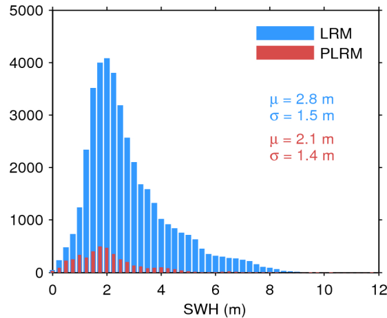
Figure 17. Histogram of flag-valid SWH over oceans and lakes for LRM (blue) and PLRM (red) for 24/04/2016. The mean ( \mu ) and standard deviation ( \sigma ) are also shown. Note that values larger than 12 m are excluded from the histogram for the sake of readability but not from the computation of \mu and \sigma .
