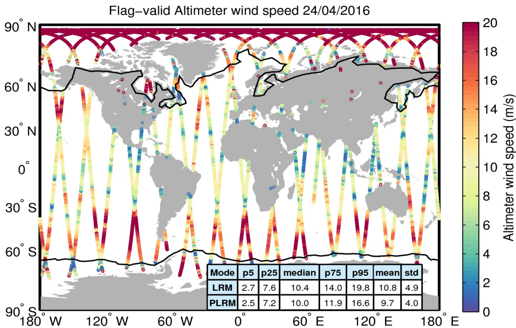
Figure 31. Geographical distribution of flag-valid wind data over oceans and lakes for 24/04/2016. The statistical values shown in the table refer to the wind in m/s and are calculated separately for LRM and PLRM regions. Measurements taken over polar polygons have been excluded from the computation of the statistical values. The black lines mark the outer limit of the Arctic and Antarctic polar polygons.
