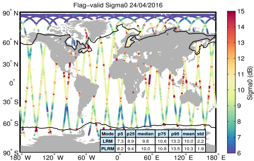
Figure 23. Geographical distribution of flag-valid sigma0 data over oceans and lakes for 24/04/2016. The statistical values shown in the table refer to the sigma0 in dB and are calculated separately for LRM and PLRM regions. Measurements taken over polar polygons have been excluded from the computation of the statistical values. The black lines mark the outer limit of the Arctic and Antarctic polar polygons.
