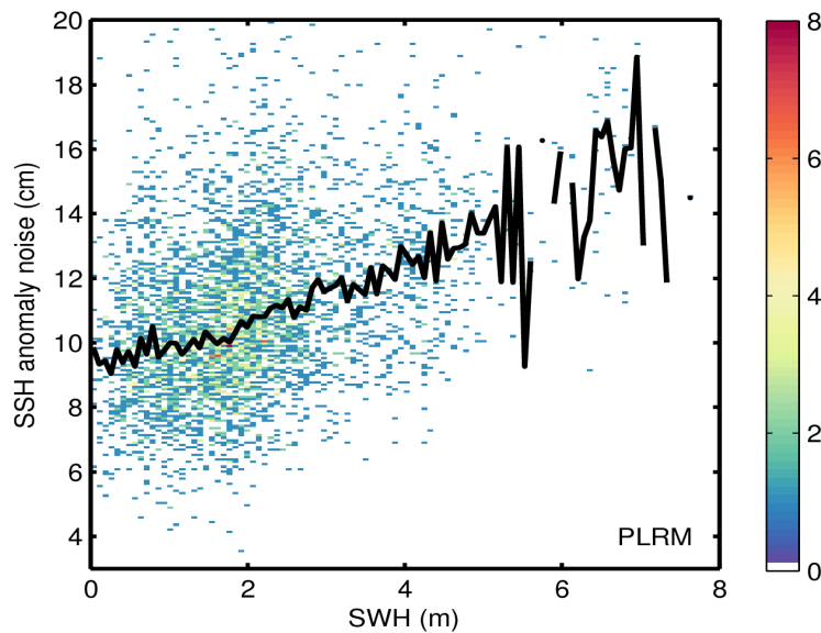
Figure 9. 2D histogram showing flag-valid SSH anomaly noise as a function of SWH for LRM (top) and PLRM (bottom) for 24/04/2016. The black line denotes the median SSH anomaly noise as a function of SWH.
