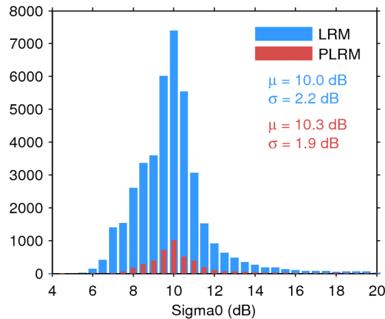
Figure 25. Histogram of flag-valid sigma0 over oceans and lakes for LRM (blue) and PLRM (red) for 24/04/2016. The mean ( \mu ) and standard deviation ( \sigma ) are also shown. Note that values outside [4 20] dB are excluded from the histogram for the sake of readability but not from the computation of \mu and \sigma .
