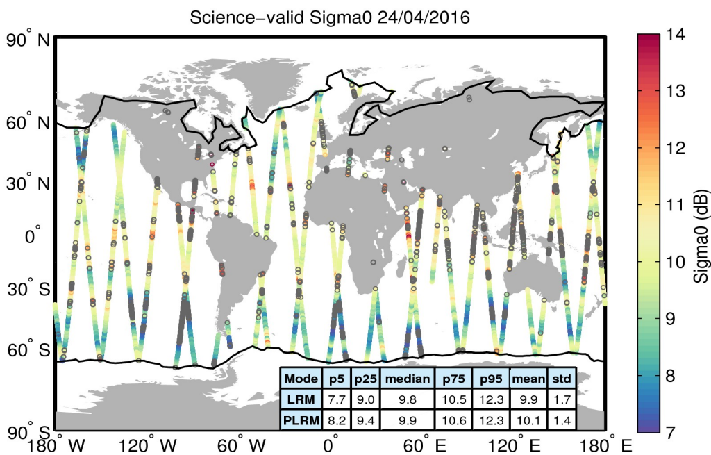
Figure 27. Geographical distribution of science-valid sigma0 data over oceans and lakes for 24/04/2016. The statistical values shown in the table refer to the sigma0 in dB and are calculated separately for LRM and PLRM regions. The black lines mark the outer limit of the Arctic and Antarctic polar polygons. Gray circles denote records that have been rejected based on the editing criteria described in Table 4.
