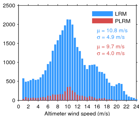
Figure 33. Histogram of flag-valid wind over oceans and lakes for LRM (blue) and PLRM (red) for 24/04/2016. The mean ( \mu ) and standard deviation ( \sigma ) are also shown. Note that values larger than 24 m/s are excluded from the histogram for the sake of readability but not from the computation of \mu and \sigma .
