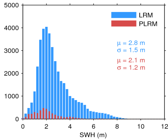
Figure 20. Histogram of science-valid SWH over oceans and lakes for LRM (blue) and PLRM (red) for 24/04/2016. The mean ( \mu ) and standard deviation ( \sigma ) are also shown. Note that values larger than 12 m are excluded from the histogram for the sake of readability but not from the computation of \mu and \sigma .
