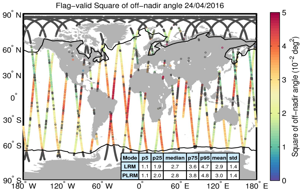
Figure 37. Geographical distribution of flag-valid mispointing data over oceans and lakes for 24/04/2016. The statistical values shown in the table refer to the mispointing in 10^{-2} \text{ deg}^2 and are calculated separately for LRM and PLRM regions. Measurements taken over polar polygons have been excluded from the computation of the statistical values. The black lines mark the outer limit of the Arctic and Antarctic polar polygons. Gray circles denote negative values.
