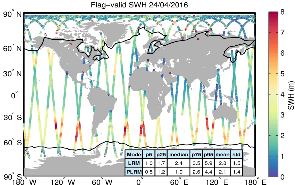
Figure 15. Geographical distribution of flag-valid SWH data over oceans and lakes for 24/04/2016. The statistical values shown in the table refer to the SWH in m and are calculated separately for LRM and PLRM regions. Measurements taken over polar polygons have been excluded from the computation of the statistical values. The black lines mark the outer limit of the Arctic and Antarctic polar polygons.
