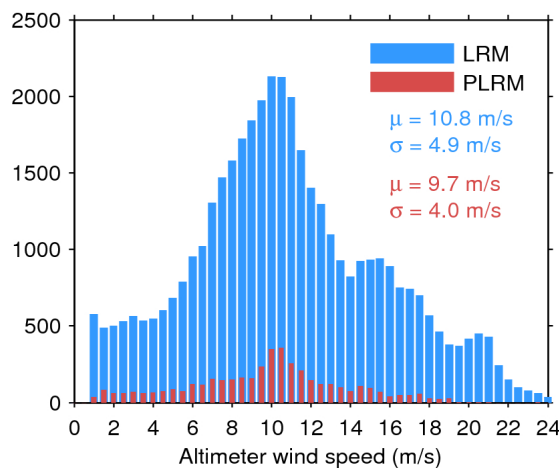
Figure 35. Histogram of science-valid wind over oceans and lakes for LRM (blue) and PLRM (red) for 24/04/2016. The mean ( \mu ) and standard deviation ( \sigma ) are also shown. Note that values larger than 24 m/s are excluded from the histogram for the sake of readability but not from the computation of \mu and \sigma .
