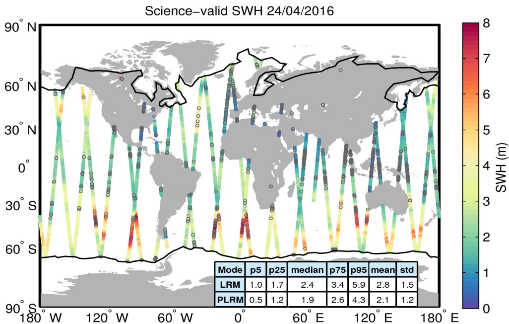
Figure 19. Geographical distribution of science-valid SWH data over oceans and lakes for 24/04/2016. The statistical values shown in the table refer to the SWH in m and are calculated separately for LRM and PLRM regions. The black lines mark the outer limit of the Arctic and Antarctic polar polygons. Gray circles denote records that have been rejected based on the editing criteria described in Table 3.
