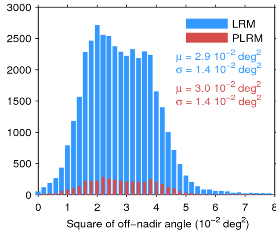
Figure 39. Histogram of flag-valid mispointing over oceans and lakes for LRM (blue) and PLRM (red) for 24/04/2016. Only positive values have been considered. The mean ( \mu ) and standard deviation ( \sigma ) are also shown. Note that values larger than 8 \cdot 10^{-2} \text{ deg}^2 are excluded from the histogram for the sake of readability but not from the computation of \mu and \sigma .
