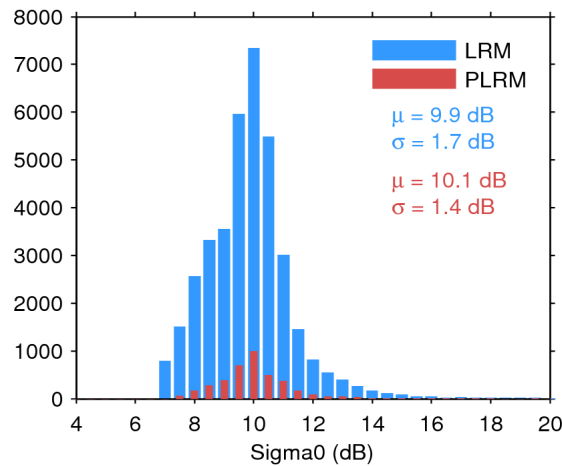
Figure 28. Histogram of science-valid sigma0 over oceans and lakes for LRM (blue) and PLRM (red) for 24/04/2016. The mean ( \mu ) and standard deviation ( \sigma ) are also shown. Note that values outside [4 20] dB are excluded from the histogram for the sake of readability but not from the computation of \mu and \sigma .
