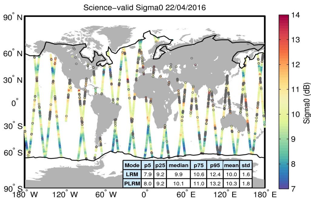
Figure 27. Geographical distribution of science-valid sigma0 data over oceans and lakes for 22/04/2016. The statistical values shown in the table refer to the sigma0 in dB and are calculated separately for LRM and PLRM regions. The black lines mark the outer limit of the Arctic and Antarctic polar polygons. Gray circles denote records that have been rejected based on the editing criteria described in Table 4.
