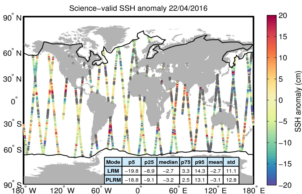
Figure 10. Geographical distribution of science-valid SSH anomaly data over oceans and lakes for 22/04/2016. The statistical values shown in the table refer to the SSH anomaly in cm and are calculated separately for LRM and PLRM regions. The black lines mark the outer limit of the Arctic and Antarctic polar polygons. Gray circles denote records that have been rejected based on the editing criteria described in Table 2.
