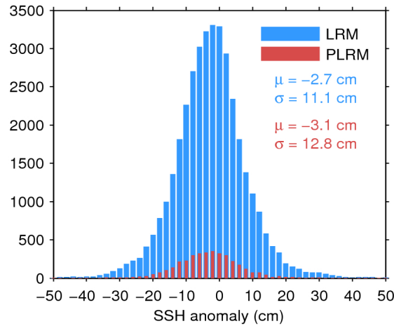
Figure 11. Histogram of science-valid SSH anomaly over oceans and lakes for LRM (blue) and PLRM (red) for 22/04/2016. The mean ( \mu ) and standard deviation ( \sigma ) are also shown. Note that values outside [-50 50] cm are excluded from the histogram for the sake of readability but not from the computation of \mu and \sigma .
