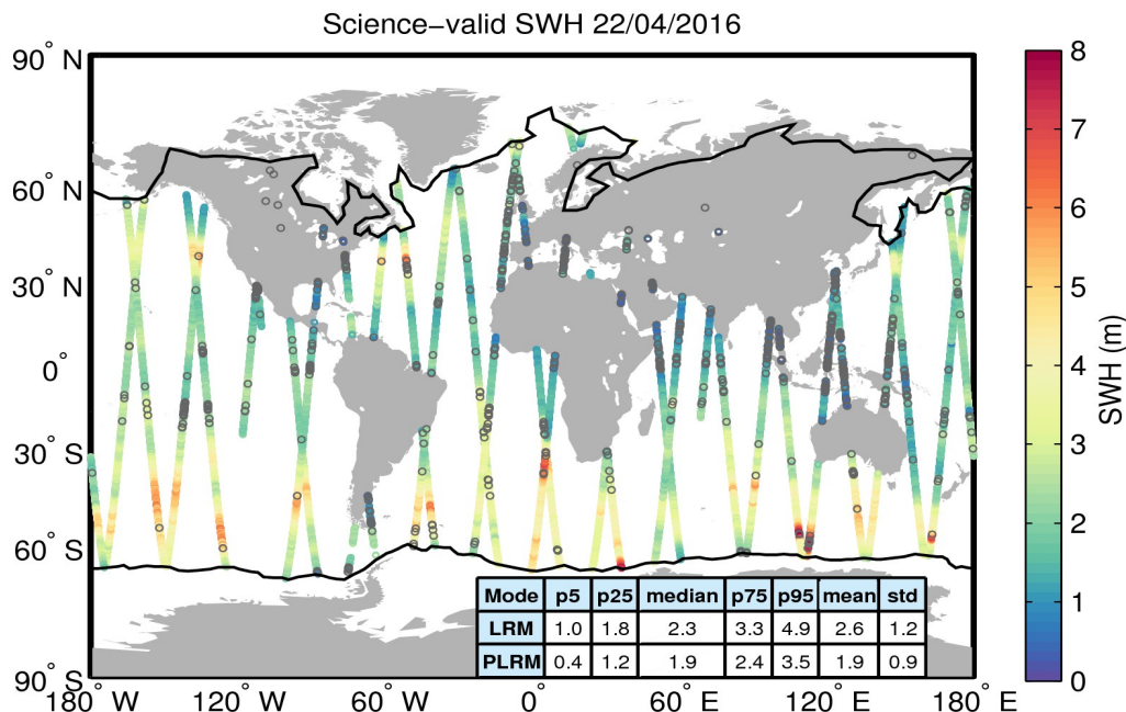
Figure 19. Geographical distribution of science-valid SWH data over oceans and lakes for 22/04/2016. The statistical values shown in the table refer to the SWH in m and are calculated separately for LRM and PLRM regions. The black lines mark the outer limit of the Arctic and Antarctic polar polygons. Gray circles denote records that have been rejected based on the editing criteria described in Table 3.
