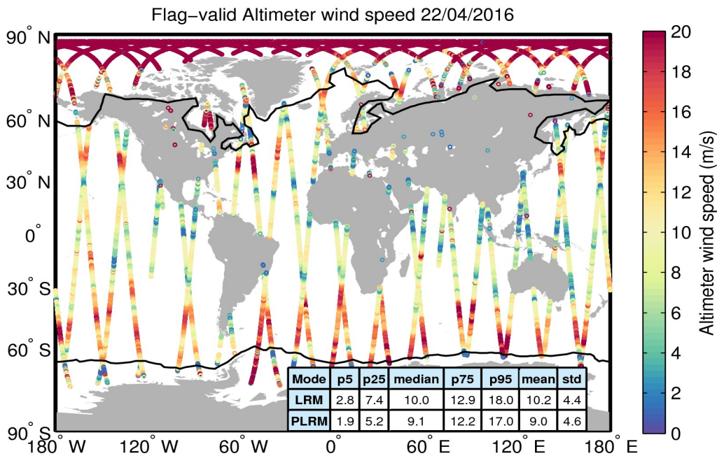
Figure 31. Geographical distribution of flag-valid wind data over oceans and lakes for 22/04/2016. The statistical values shown in the table refer to the wind in m/s and are calculated separately for LRM and PLRM regions. Measurements taken over polar polygons have been excluded from the computation of the statistical values. The black lines mark the outer limit of the Arctic and Antarctic polar polygons.
