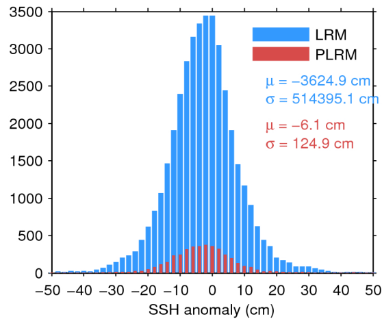
Figure 7. Histogram of flag-valid SSH anomaly over oceans and lakes for LRM (blue) and PLRM (red) for 22/04/2016. The mean ( \mu ) and standard deviation ( \sigma ) are also shown. Note that values outside [-50 50] cm are excluded from the histogram for the sake of readability but not from the computation of \mu and \sigma .
