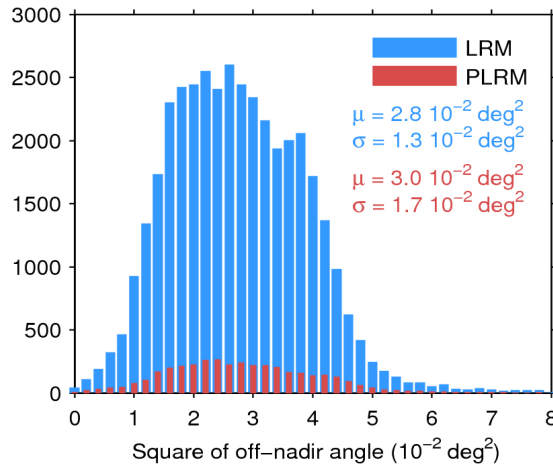
Figure 39. Histogram of flag-valid mispointing over oceans and lakes for LRM (blue) and PLRM (red) for 22/04/2016. Only positive values have been considered. The mean ( \mu ) and standard deviation ( \sigma ) are also shown. Note that values larger than 8 \cdot 10^{-2} \text{ deg}^2 are excluded from the histogram for the sake of readability but not from the computation of \mu and \sigma .
