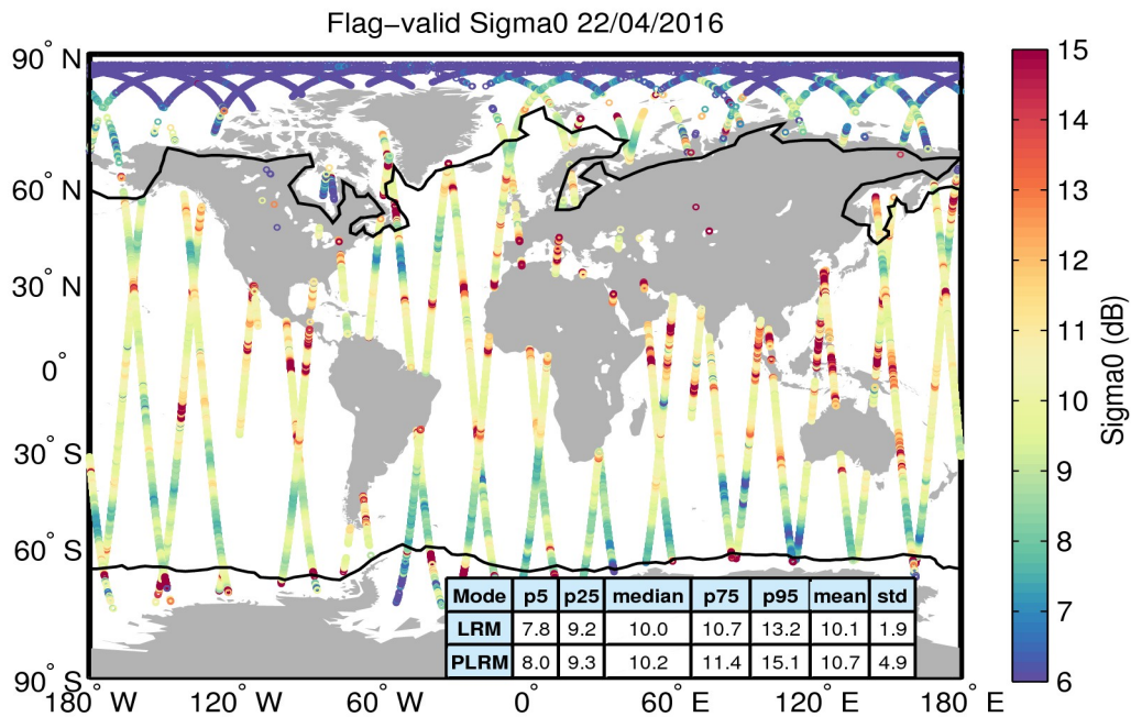
Figure 23. Geographical distribution of flag-valid sigma0 data over oceans and lakes for 22/04/2016. The statistical values shown in the table refer to the sigma0 in dB and are calculated separately for LRM and PLRM regions. Measurements taken over polar polygons have been excluded from the computation of the statistical values. The black lines mark the outer limit of the Arctic and Antarctic polar polygons.
