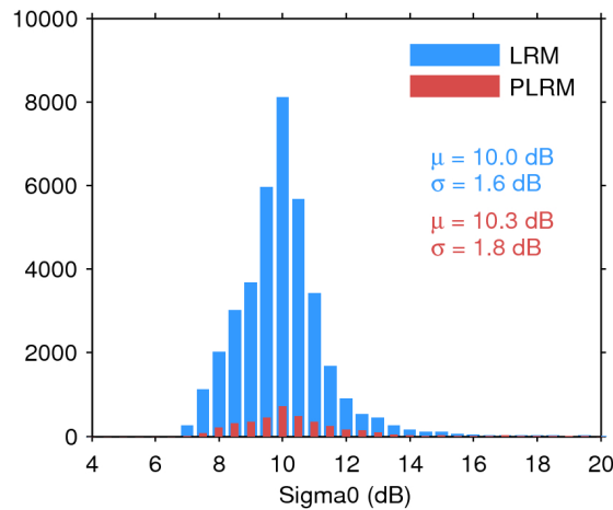
Figure 28. Histogram of science-valid sigma0 over oceans and lakes for LRM (blue) and PLRM (red) for 22/04/2016. The mean ( \mu ) and standard deviation ( \sigma ) are also shown. Note that values outside [4 20] dB are excluded from the histogram for the sake of readability but not from the computation of \mu and \sigma .
