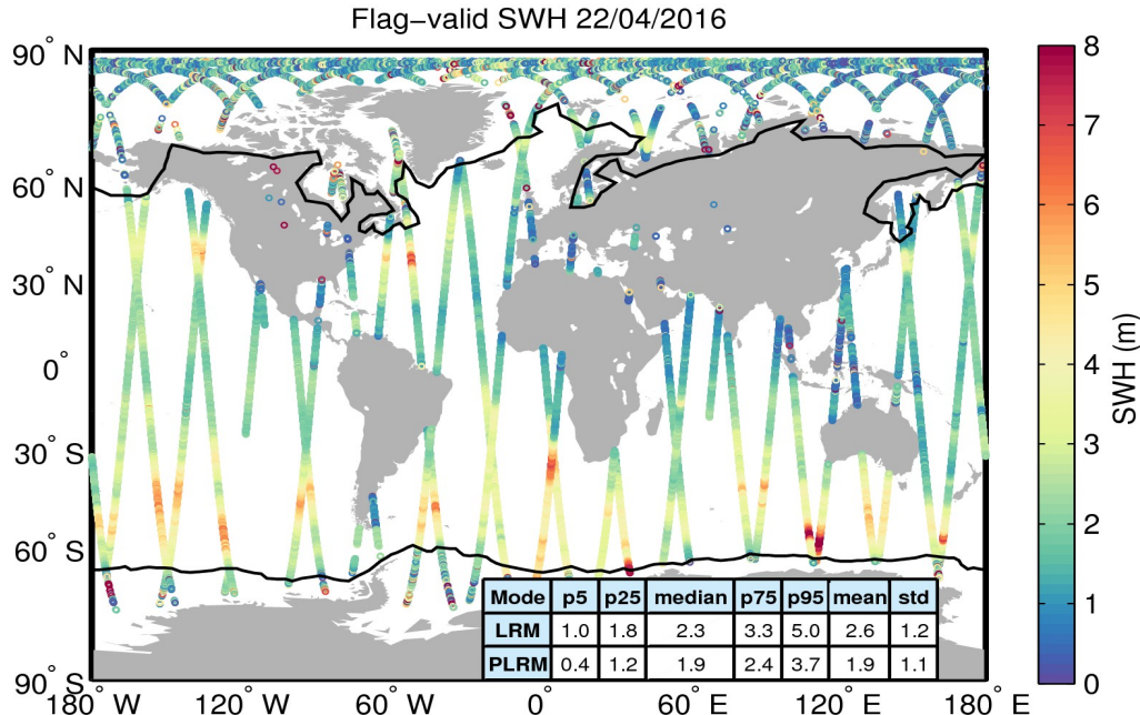
Figure 15. Geographical distribution of flag-valid SWH data over oceans and lakes for 22/04/2016. The statistical values shown in the table refer to the SWH in m and are calculated separately for LRM and PLRM regions. Measurements taken over polar polygons have been excluded from the computation of the statistical values. The black lines mark the outer limit of the Arctic and Antarctic polar polygons.
