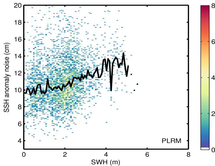
Figure 9. 2D histogram showing flag-valid SSH anomaly noise as a function of SWH for LRM (top) and PLRM (bottom) for 22/04/2016. The black line denotes the median SSH anomaly noise as a function of SWH.
