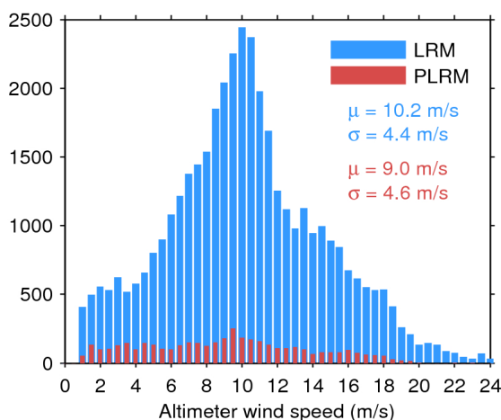
Figure 33. Histogram of flag-valid wind over oceans and lakes for LRM (blue) and PLRM (red) for 22/04/2016. The mean ( \mu ) and standard deviation ( \sigma ) are also shown. Note that values larger than 24 m/s are excluded from the histogram for the sake of readability but not from the computation of \mu and \sigma .
