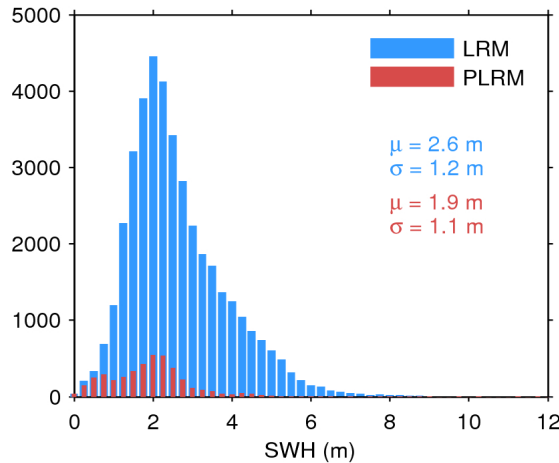
Figure 17. Histogram of flag-valid SWH over oceans and lakes for LRM (blue) and PLRM (red) for 22/04/2016. The mean ( \mu ) and standard deviation ( \sigma ) are also shown. Note that values larger than 12 m are excluded from the histogram for the sake of readability but not from the computation of \mu and \sigma .
