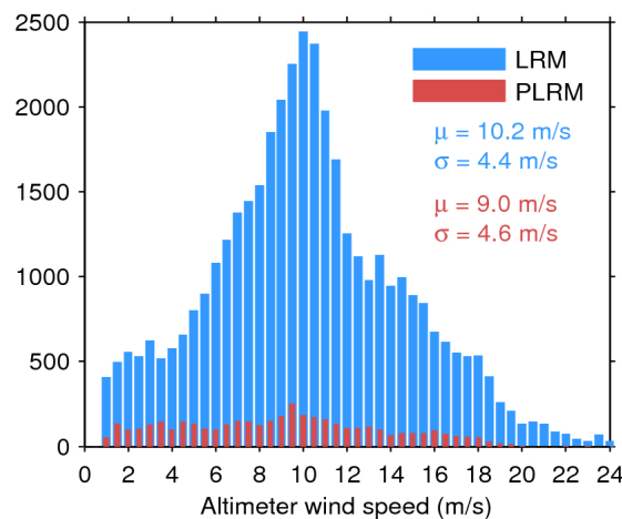
Figure 35. Histogram of science-valid wind over oceans and lakes for LRM (blue) and PLRM (red) for 22/04/2016. The mean ( \mu ) and standard deviation ( \sigma ) are also shown. Note that values larger than 24 m/s are excluded from the histogram for the sake of readability but not from the computation of \mu and \sigma .
