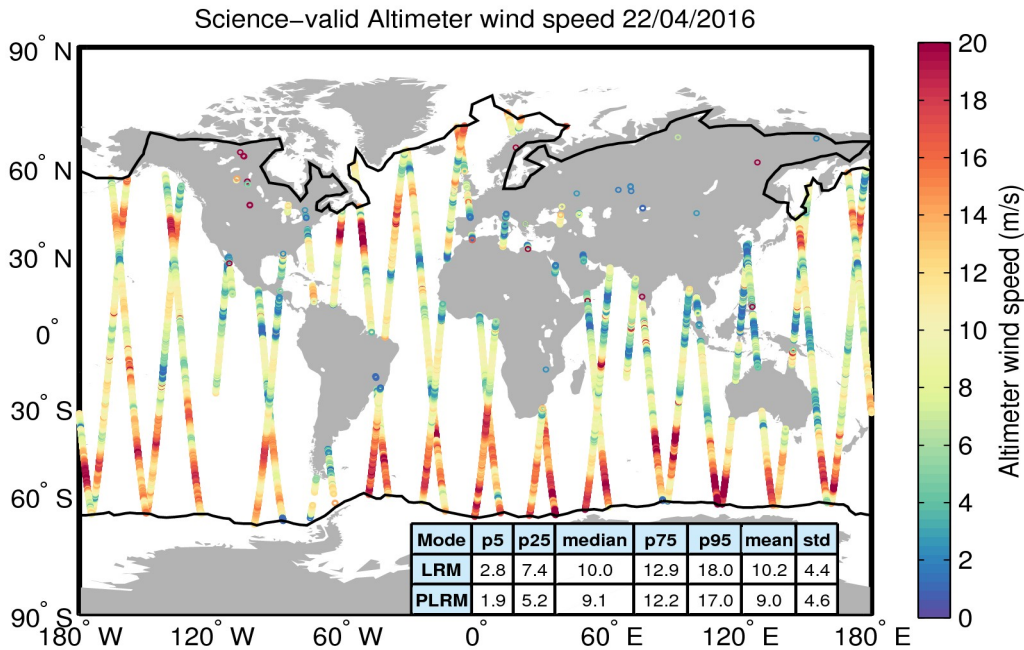
Figure 34. Geographical distribution of science-valid wind data over oceans and lakes for 22/04/2016. The statistical values shown in the table refer to the wind in m/s and are calculated separately for LRM and PLRM regions. The black lines mark the outer limit of the Arctic and Antarctic polar polygons. Gray circles denote records that have been rejected based on the editing criteria described in Table 5.
