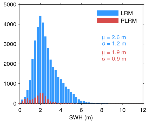
Figure 20. Histogram of science-valid SWH over oceans and lakes for LRM (blue) and PLRM (red) for 22/04/2016. The mean ( \mu ) and standard deviation ( \sigma ) are also shown. Note that values larger than 12 m are excluded from the histogram for the sake of readability but not from the computation of \mu and \sigma .
