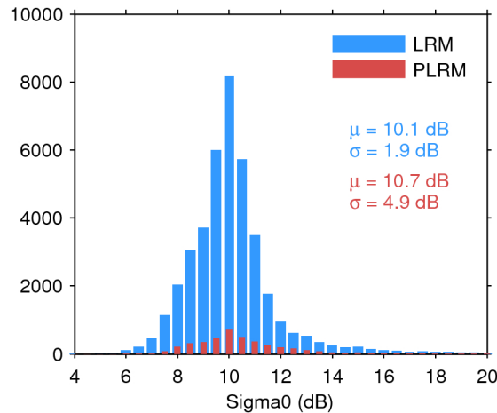
Figure 25. Histogram of flag-valid sigma0 over oceans and lakes for LRM (blue) and PLRM (red) for 22/04/2016. The mean ( \mu ) and standard deviation ( \sigma ) are also shown. Note that values outside [4 20] dB are excluded from the histogram for the sake of readability but not from the computation of \mu and \sigma .
