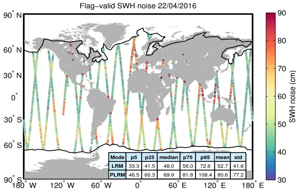
Figure 18. Geographical distribution of flag-valid 20-Hz SWH measurement noise over oceans and lakes for 22/04/2016. The statistical values shown in the table refer to the SWH noise and are calculated separately for LRM and PLRM regions. Measurements taken over polar polygons have been excluded from the computation of the statistical values. The black lines mark the outer limit of the Arctic and Antarctic polar polygons.
