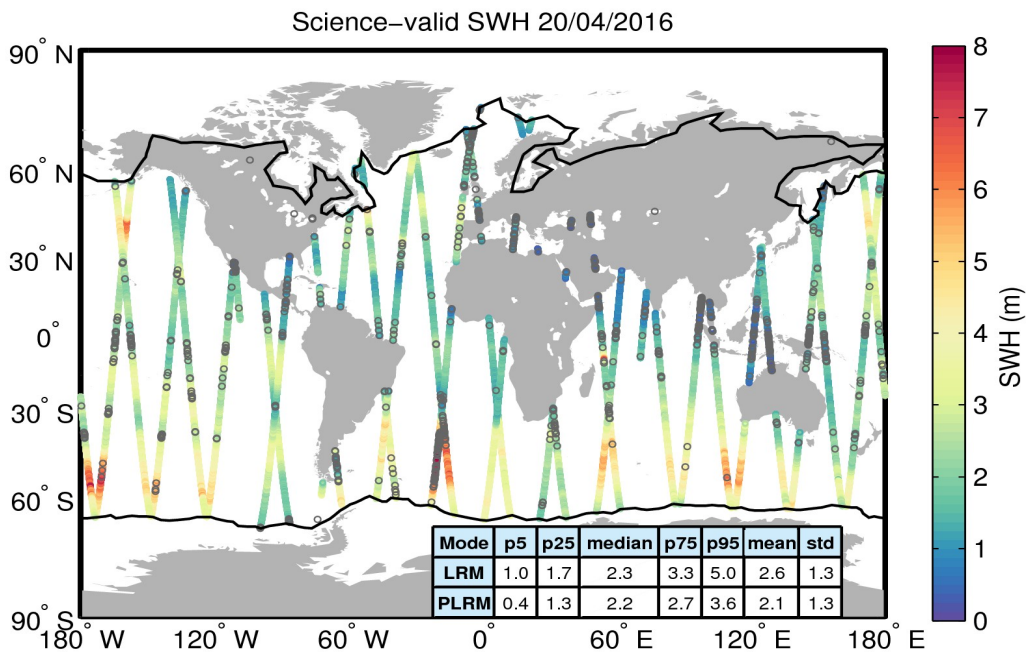
Figure 19. Geographical distribution of science-valid SWH data over oceans and lakes for 20/04/2016. The statistical values shown in the table refer to the SWH in m and are calculated separately for LRM and PLRM regions. The black lines mark the outer limit of the Arctic and Antarctic polar polygons. Gray circles denote records that have been rejected based on the editing criteria described in Table 3.
