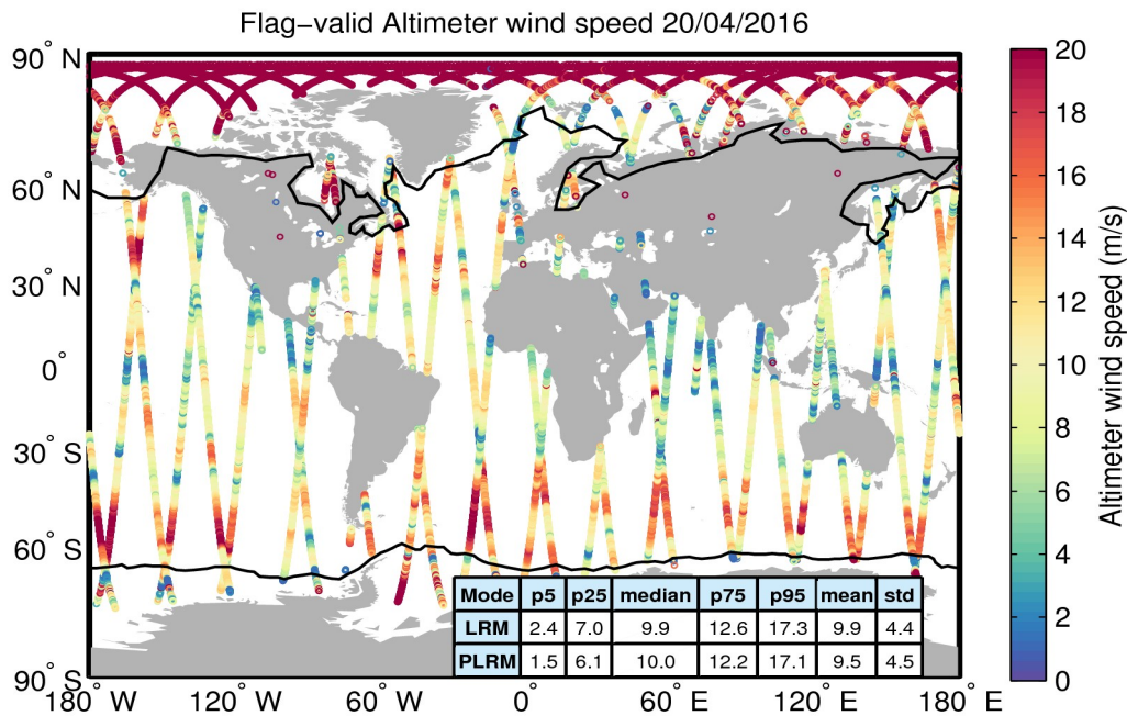
Figure 31. Geographical distribution of flag-valid wind data over oceans and lakes for 20/04/2016. The statistical values shown in the table refer to the wind in m/s and are calculated separately for LRM and PLRM regions. Measurements taken over polar polygons have been excluded from the computation of the statistical values. The black lines mark the outer limit of the Arctic and Antarctic polar polygons.
