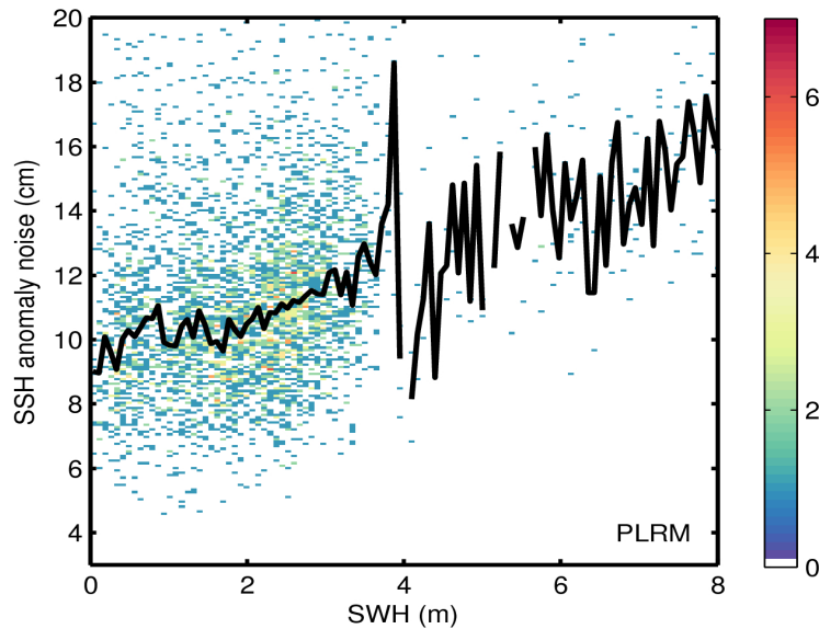
Figure 9. 2D histogram showing flag-valid SSH anomaly noise as a function of SWH for LRM (top) and PLRM (bottom) for 20/04/2016. The black line denotes the median SSH anomaly noise as a function of SWH.
