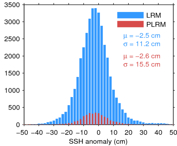
Figure 11. Histogram of science-valid SSH anomaly over oceans and lakes for LRM (blue) and PLRM (red) for 20/04/2016. The mean ( \mu ) and standard deviation ( \sigma ) are also shown. Note that values outside [-50 50] cm are excluded from the histogram for the sake of readability but not from the computation of \mu and \sigma .
