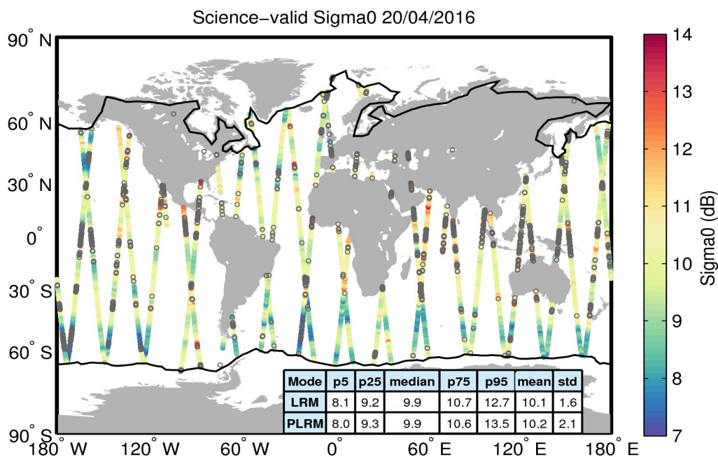
Figure 27. Geographical distribution of science-valid sigma0 data over oceans and lakes for 20/04/2016. The statistical values shown in the table refer to the sigma0 in dB and are calculated separately for LRM and PLRM regions. The black lines mark the outer limit of the Arctic and Antarctic polar polygons. Gray circles denote records that have been rejected based on the editing criteria described in Table 4.
