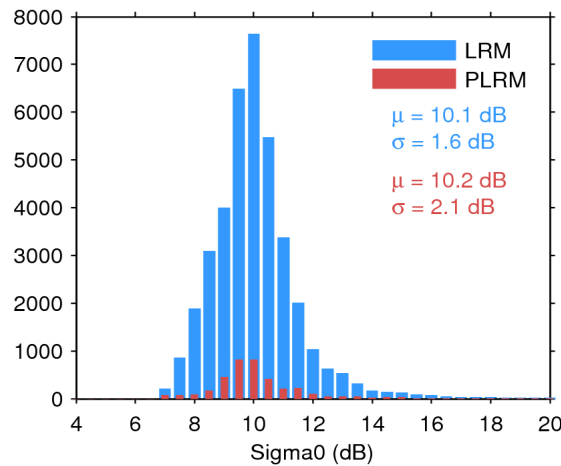
Figure 28. Histogram of science-valid sigma0 over oceans and lakes for LRM (blue) and PLRM (red) for 20/04/2016. The mean ( \mu ) and standard deviation ( \sigma ) are also shown. Note that values outside [4 20] dB are excluded from the histogram for the sake of readability but not from the computation of \mu and \sigma .
