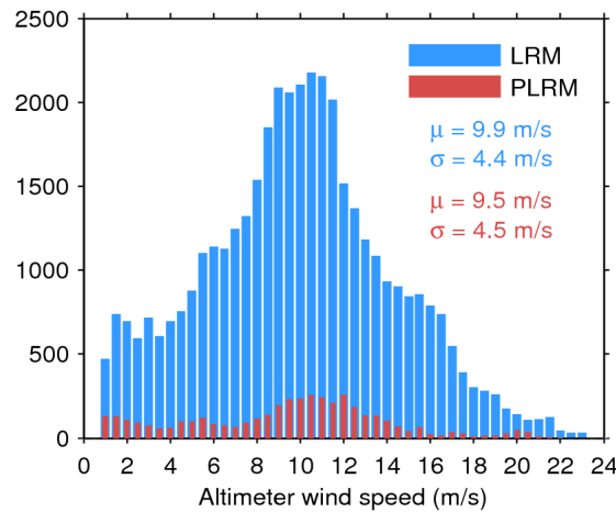
Figure 33. Histogram of flag-valid wind over oceans and lakes for LRM (blue) and PLRM (red) for 20/04/2016. The mean ( \mu ) and standard deviation ( \sigma ) are also shown. Note that values larger than 24 m/s are excluded from the histogram for the sake of readability but not from the computation of \mu and \sigma .
