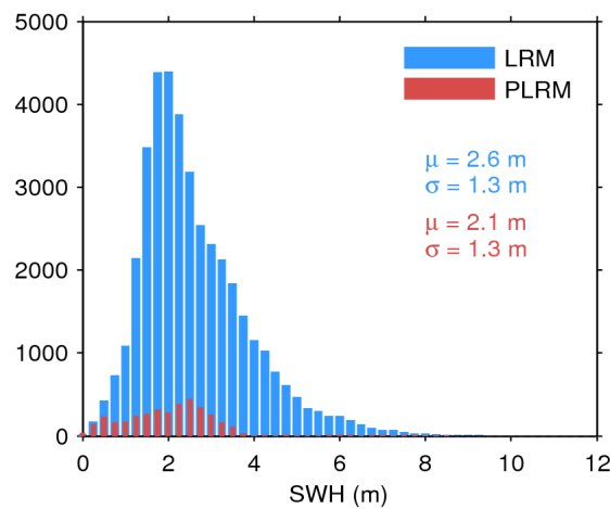
Figure 20. Histogram of science-valid SWH over oceans and lakes for LRM (blue) and PLRM (red) for 20/04/2016. The mean ( \mu ) and standard deviation ( \sigma ) are also shown. Note that values larger than 12 m are excluded from the histogram for the sake of readability but not from the computation of \mu and \sigma .
