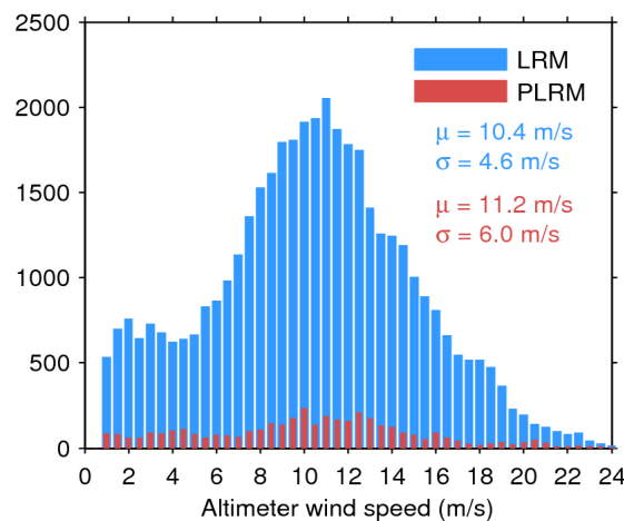
Figure 35. Histogram of science-valid wind over oceans and lakes for LRM (blue) and PLRM (red) for 18/04/2016. The mean ( \mu ) and standard deviation ( \sigma ) are also shown. Note that values larger than 24 m/s are excluded from the histogram for the sake of readability but not from the computation of \mu and \sigma .
