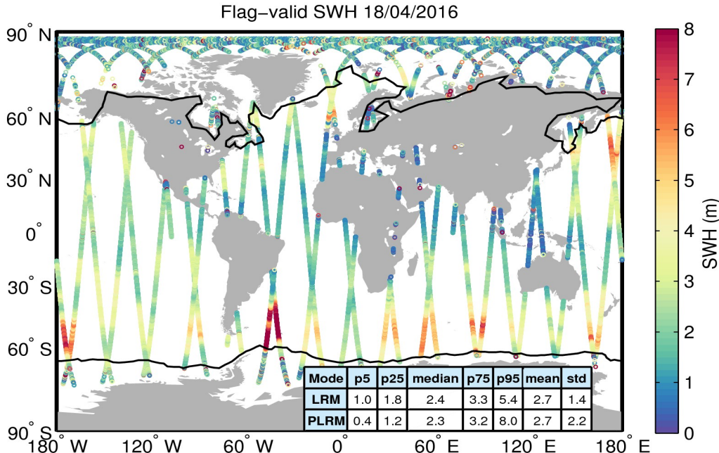
Figure 15. Geographical distribution of flag-valid SWH data over oceans and lakes for 18/04/2016. The statistical values shown in the table refer to the SWH in m and are calculated separately for LRM and PLRM regions. Measurements taken over polar polygons have been excluded from the computation of the statistical values. The black lines mark the outer limit of the Arctic and Antarctic polar polygons.
