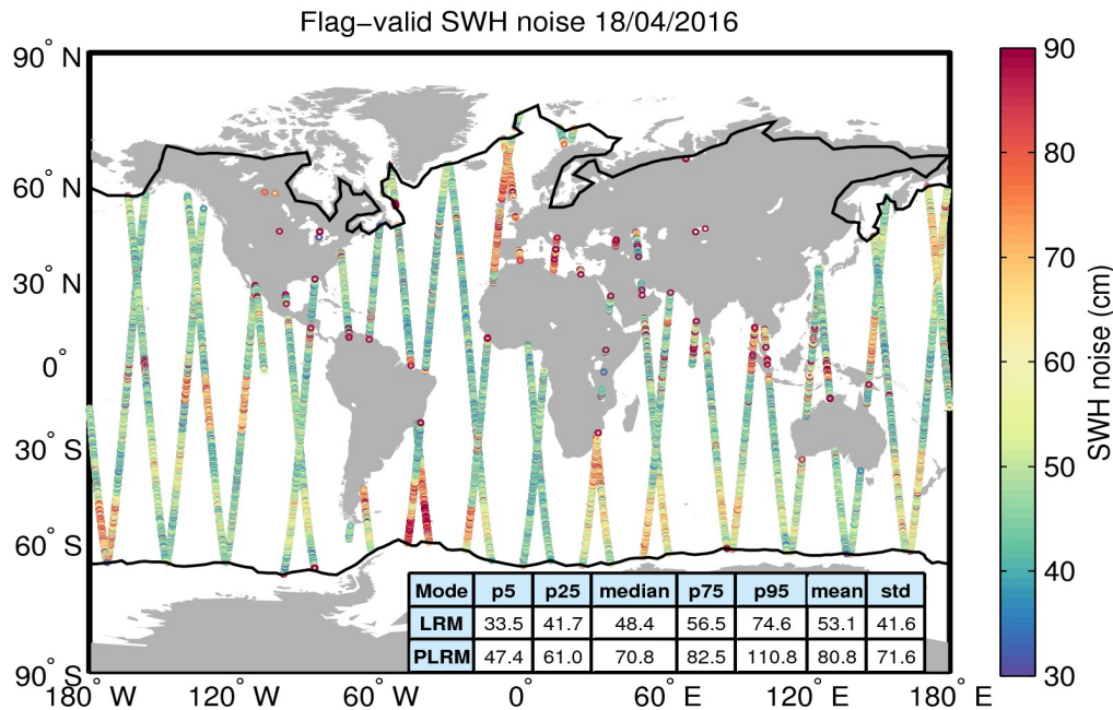
Figure 18. Geographical distribution of flag-valid 20-Hz SWH measurement noise over oceans and lakes for 18/04/2016. The statistical values shown in the table refer to the SWH noise and are calculated separately for LRM and PLRM regions. Measurements taken over polar polygons have been excluded from the computation of the statistical values. The black lines mark the outer limit of the Arctic and Antarctic polar polygons.
