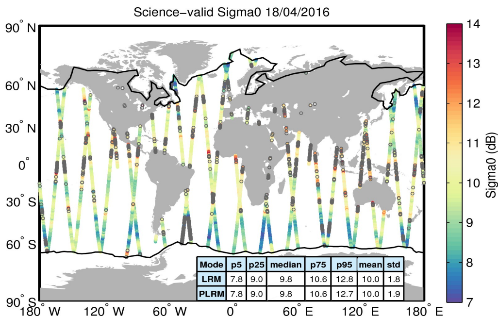
Figure 27. Geographical distribution of science-valid sigma0 data over oceans and lakes for 18/04/2016. The statistical values shown in the table refer to the sigma0 in dB and are calculated separately for LRM and PLRM regions. The black lines mark the outer limit of the Arctic and Antarctic polar polygons. Gray circles denote records that have been rejected based on the editing criteria described in Table 4.
