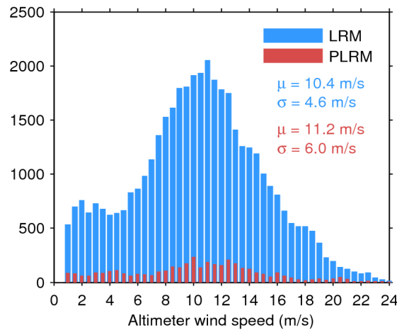
Figure 33. Histogram of flag-valid wind over oceans and lakes for LRM (blue) and PLRM (red) for 18/04/2016. The mean ( \mu ) and standard deviation ( \sigma ) are also shown. Note that values larger than 24 m/s are excluded from the histogram for the sake of readability but not from the computation of \mu and \sigma .
