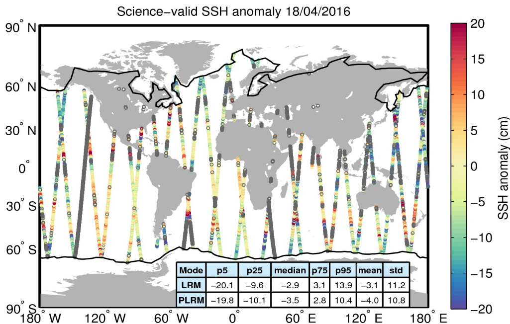
Figure 10. Geographical distribution of science-valid SSH anomaly data over oceans and lakes for 18/04/2016. The statistical values shown in the table refer to the SSH anomaly in cm and are calculated separately for LRM and PLRM regions. The black lines mark the outer limit of the Arctic and Antarctic polar polygons. Gray circles denote records that have been rejected based on the editing criteria described in Table 2.
