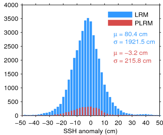
Figure 7. Histogram of flag-valid SSH anomaly over oceans and lakes for LRM (blue) and PLRM (red) for 18/04/2016. The mean ( \mu ) and standard deviation ( \sigma ) are also shown. Note that values outside [-50 50] cm are excluded from the histogram for the sake of readability but not from the computation of \mu and \sigma .
