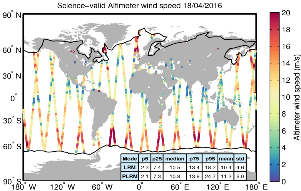
Figure 34. Geographical distribution of science-valid wind data over oceans and lakes for 18/04/2016. The statistical values shown in the table refer to the wind in m/s and are calculated separately for LRM and PLRM regions. The black lines mark the outer limit of the Arctic and Antarctic polar polygons. Gray circles denote records that have been rejected based on the editing criteria described in Table 5.
