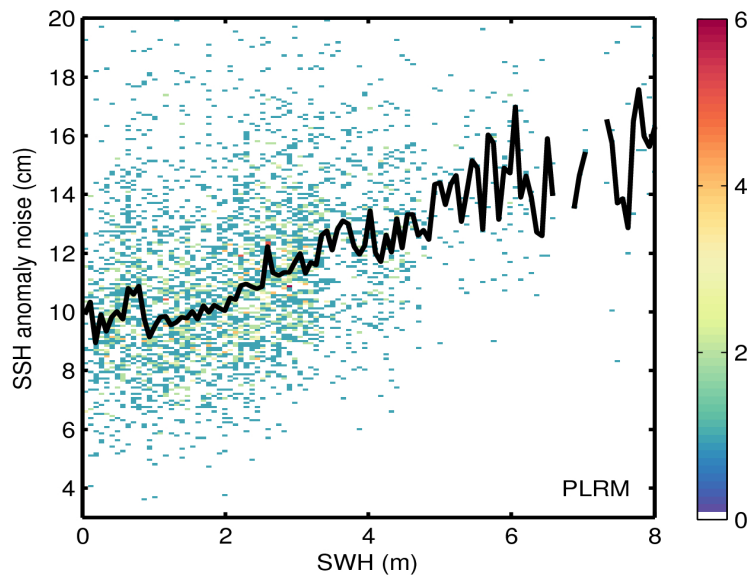
Figure 9. 2D histogram showing flag-valid SSH anomaly noise as a function of SWH for LRM (top) and PLRM (bottom) for 18/04/2016. The black line denotes the median SSH anomaly noise as a function of SWH.
