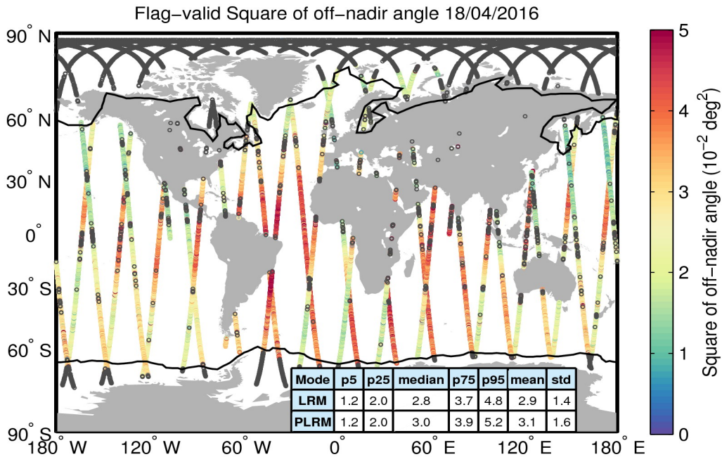
Figure 37. Geographical distribution of flag-valid mispointing data over oceans and lakes for 18/04/2016. The statistical values shown in the table refer to the mispointing in 10^{-2} deg 2 and are calculated separately for LRM and PLRM regions. Measurements taken over polar polygons have been excluded from the computation of the statistical values. The black lines mark the outer limit of the Arctic and Antarctic polar polygons. Gray circles denote negative values.
