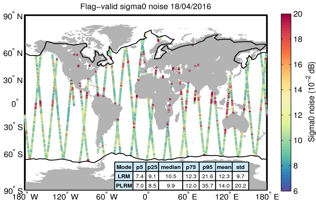
Figure 26. Geographical distribution of flag-valid 20-Hz sigma0 measurement noise over oceans and lakes for 18/04/2016. The statistical values shown in the table refer to the sigma0 noise and are calculated separately for LRM and PLRM regions. Measurements taken over polar polygons have been excluded from the computation of the statistical values. The black lines mark the outer limit of the Arctic and Antarctic polar polygons.
