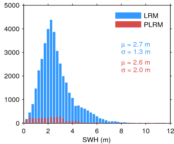
Figure 20. Histogram of science-valid SWH over oceans and lakes for LRM (blue) and PLRM (red) for 18/04/2016. The mean ( \mu ) and standard deviation ( \sigma ) are also shown. Note that values larger than 12 m are excluded from the histogram for the sake of readability but not from the computation of \mu and \sigma .
