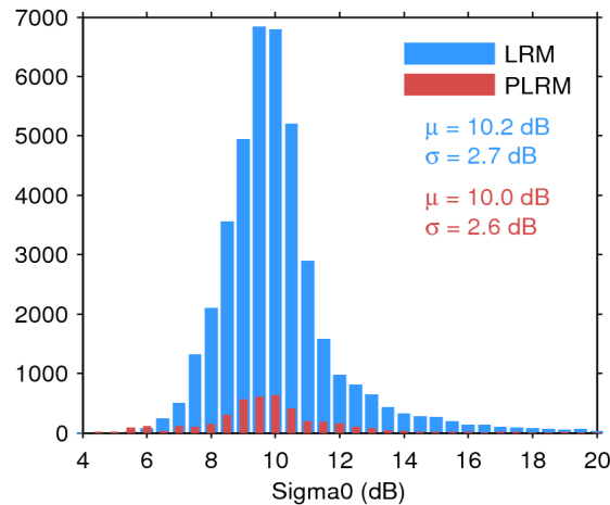
Figure 25. Histogram of flag-valid sigma0 over oceans and lakes for LRM (blue) and PLRM (red) for 18/04/2016. The mean ( \mu ) and standard deviation ( \sigma ) are also shown. Note that values outside [4 20] dB are excluded from the histogram for the sake of readability but not from the computation of \mu and \sigma .
