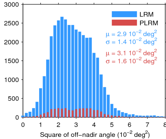
Figure 39. Histogram of flag-valid mispointing over oceans and lakes for LRM (blue) and PLRM (red) for 18/04/2016. Only positive values have been considered. The mean ( \mu ) and standard deviation ( \sigma ) are also shown. Note that values larger than 8 \cdot 10^{-2} \text{ deg}^2 are excluded from the histogram for the sake of readability but not from the computation of \mu and \sigma .
