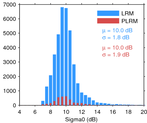
Figure 28. Histogram of science-valid sigma0 over oceans and lakes for LRM (blue) and PLRM (red) for 18/04/2016. The mean ( \mu ) and standard deviation ( \sigma ) are also shown. Note that values outside [4 20] dB are excluded from the histogram for the sake of readability but not from the computation of \mu and \sigma .
