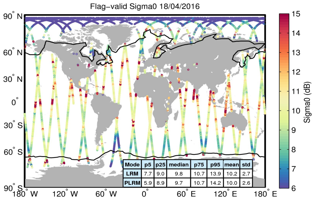
Figure 23. Geographical distribution of flag-valid sigma0 data over oceans and lakes for 18/04/2016. The statistical values shown in the table refer to the sigma0 in dB and are calculated separately for LRM and PLRM regions. Measurements taken over polar polygons have been excluded from the computation of the statistical values. The black lines mark the outer limit of the Arctic and Antarctic polar polygons.
