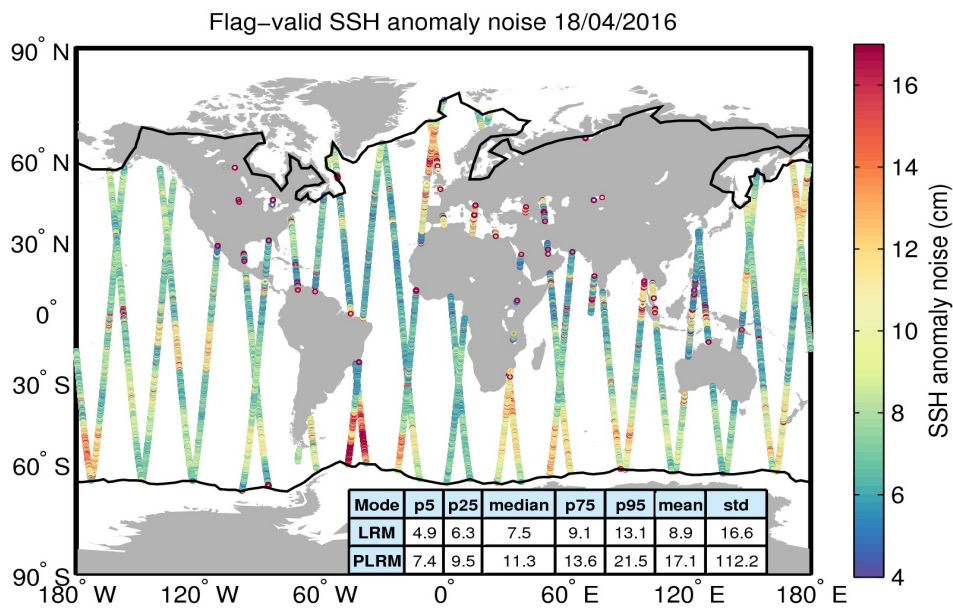
Figure 8. Geographical distribution of flag-valid 20-Hz SSH anomaly measurement noise over oceans and lakes for 18/04/2016. The statistical values shown in the table refer to the SSH anomaly noise and are calculated separately for LRM and PLRM regions. Measurements taken over polar polygons have been excluded from the computation of the statistical values. The black lines mark the outer limit of the Arctic and Antarctic polar polygons.
