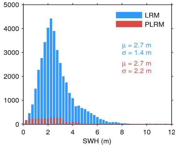
Figure 17. Histogram of flag-valid SWH over oceans and lakes for LRM (blue) and PLRM (red) for 18/04/2016. The mean ( \mu ) and standard deviation ( \sigma ) are also shown. Note that values larger than 12 m are excluded from the histogram for the sake of readability but not from the computation of \mu and \sigma .
