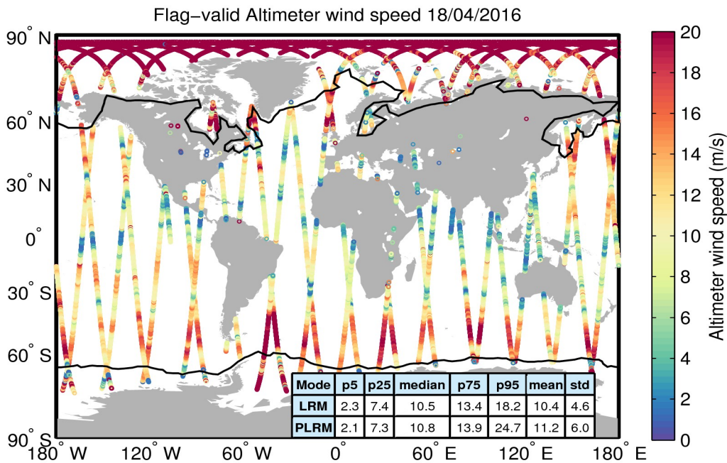
Figure 31. Geographical distribution of flag-valid wind data over oceans and lakes for 18/04/2016. The statistical values shown in the table refer to the wind in m/s and are calculated separately for LRM and PLRM regions. Measurements taken over polar polygons have been excluded from the computation of the statistical values. The black lines mark the outer limit of the Arctic and Antarctic polar polygons.
