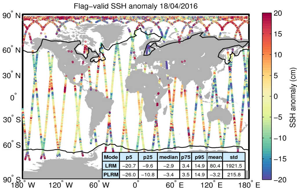
Figure 5. Geographical distribution of flag-valid 1-Hz SSH anomaly data over oceans and lakes for 18/04/2016. The statistical values shown in the table refer to the SSH anomaly in cm and are calculated separately for LRM and PLRM regions. Measurements taken over polar polygons have been excluded from the computation of the statistical values. The black lines mark the outer limit of the Arctic and Antarctic polar polygons.
