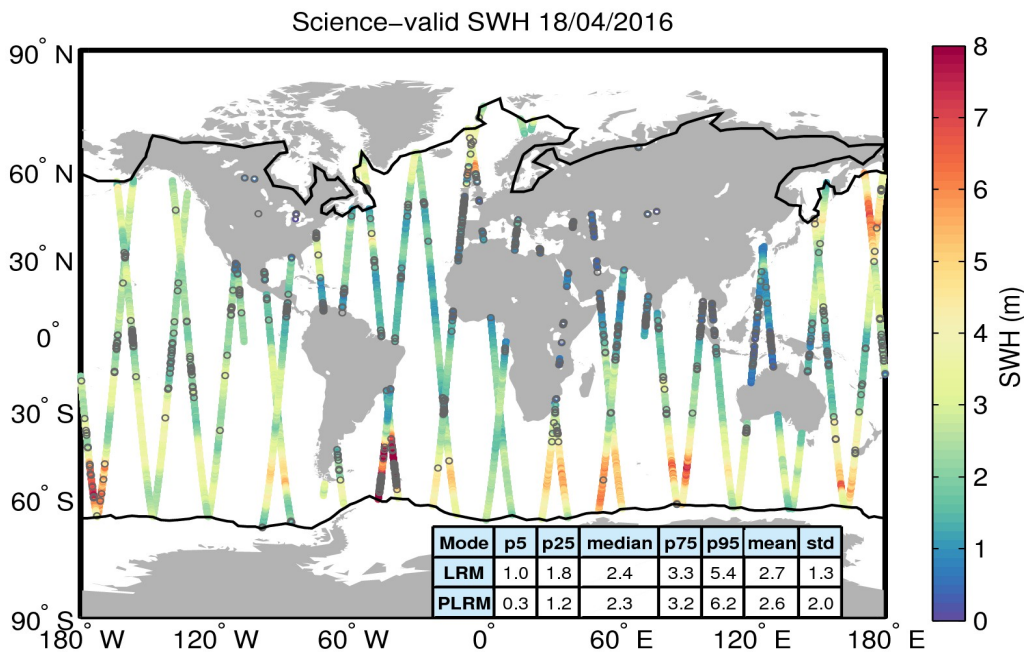
Figure 19. Geographical distribution of science-valid SWH data over oceans and lakes for 18/04/2016. The statistical values shown in the table refer to the SWH in m and are calculated separately for LRM and PLRM regions. The black lines mark the outer limit of the Arctic and Antarctic polar polygons. Gray circles denote records that have been rejected based on the editing criteria described in Table 3.
