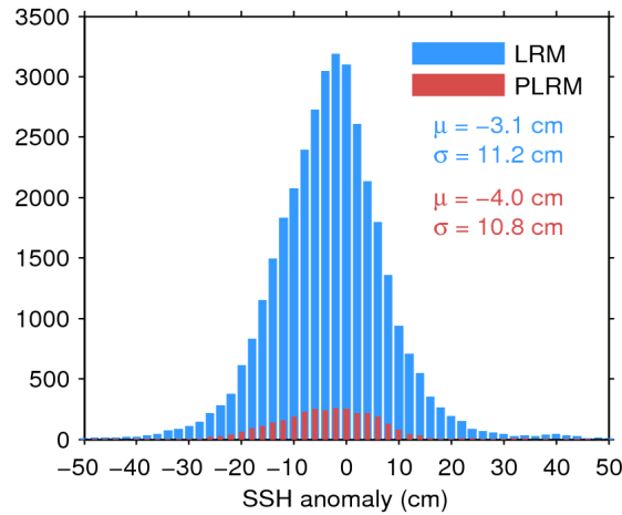
Figure 11. Histogram of science-valid SSH anomaly over oceans and lakes for LRM (blue) and PLRM (red) for 18/04/2016. The mean ( \mu ) and standard deviation ( \sigma ) are also shown. Note that values outside [-50 50] cm are excluded from the histogram for the sake of readability but not from the computation of \mu and \sigma .
