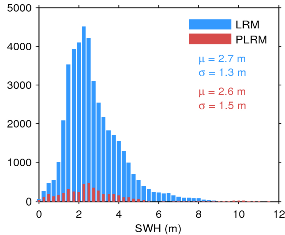
Figure 17. Histogram of flag-valid SWH over oceans and lakes for LRM (blue) and PLRM (red) for 17/04/2016. The mean ( \mu ) and standard deviation ( \sigma ) are also shown. Note that values larger than 12 m are excluded from the histogram for the sake of readability but not from the computation of \mu and \sigma .
