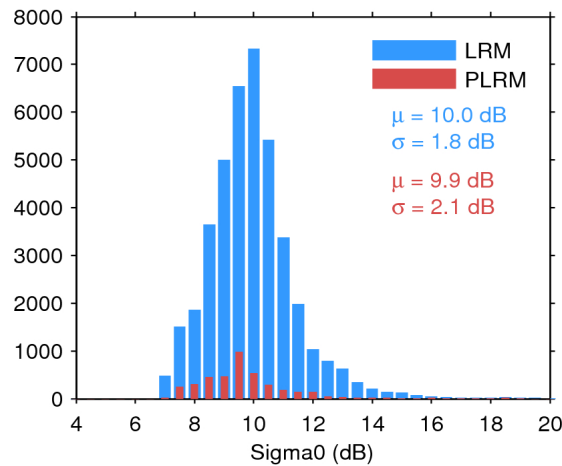
Figure 28. Histogram of science-valid sigma0 over oceans and lakes for LRM (blue) and PLRM (red) for 17/04/2016. The mean ( \mu ) and standard deviation ( \sigma ) are also shown. Note that values outside [4 20] dB are excluded from the histogram for the sake of readability but not from the computation of \mu and \sigma .
