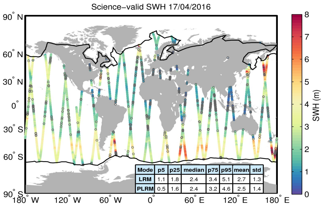
Figure 19. Geographical distribution of science-valid SWH data over oceans and lakes for 17/04/2016. The statistical values shown in the table refer to the SWH in m and are calculated separately for LRM and PLRM regions. The black lines mark the outer limit of the Arctic and Antarctic polar polygons. Gray circles denote records that have been rejected based on the editing criteria described in Table 3.
