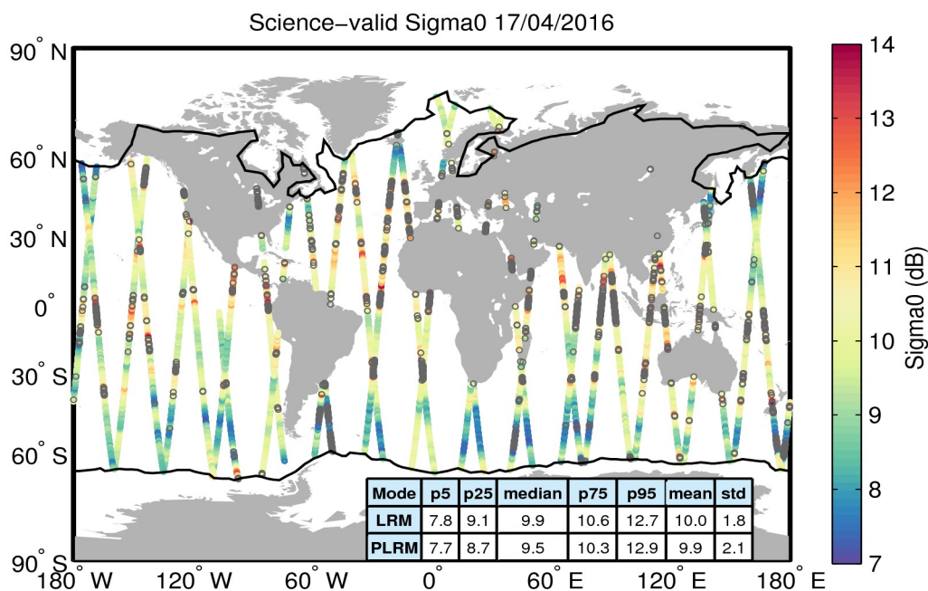
Figure 27. Geographical distribution of science-valid sigma0 data over oceans and lakes for 17/04/2016. The statistical values shown in the table refer to the sigma0 in dB and are calculated separately for LRM and PLRM regions. The black lines mark the outer limit of the Arctic and Antarctic polar polygons. Gray circles denote records that have been rejected based on the editing criteria described in Table 4.
