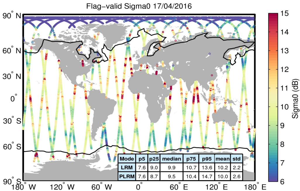
Figure 23. Geographical distribution of flag-valid sigma0 data over oceans and lakes for 17/04/2016. The statistical values shown in the table refer to the sigma0 in dB and are calculated separately for LRM and PLRM regions. Measurements taken over polar polygons have been excluded from the computation of the statistical values. The black lines mark the outer limit of the Arctic and Antarctic polar polygons.
