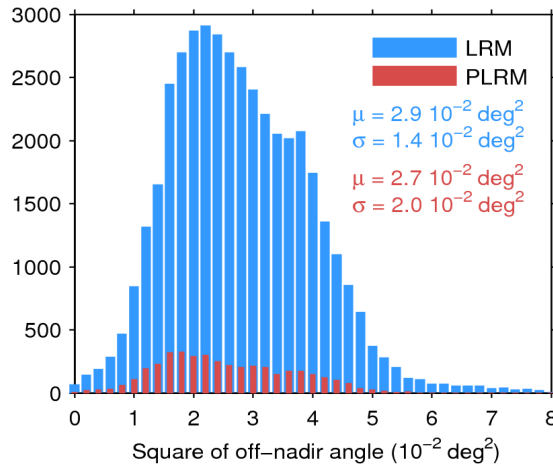
Figure 39. Histogram of flag-valid mispointing over oceans and lakes for LRM (blue) and PLRM (red) for 17/04/2016. Only positive values have been considered. The mean ( \mu ) and standard deviation ( \sigma ) are also shown. Note that values larger than 8 \cdot 10^{-2} \text{ deg}^2 are excluded from the histogram for the sake of readability but not from the computation of \mu and \sigma .
