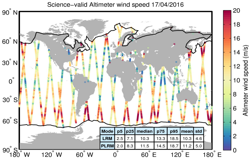
Figure 34. Geographical distribution of science-valid wind data over oceans and lakes for 17/04/2016. The statistical values shown in the table refer to the wind in m/s and are calculated separately for LRM and PLRM regions. The black lines mark the outer limit of the Arctic and Antarctic polar polygons. Gray circles denote records that have been rejected based on the editing criteria described in Table 5.
