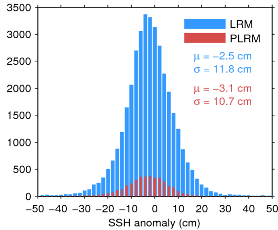
Figure 11. Histogram of science-valid SSH anomaly over oceans and lakes for LRM (blue) and PLRM (red) for 17/04/2016. The mean ( \mu ) and standard deviation ( \sigma ) are also shown. Note that values outside [-50 50] cm are excluded from the histogram for the sake of readability but not from the computation of \mu and \sigma .
