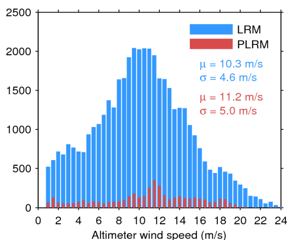
Figure 33. Histogram of flag-valid wind over oceans and lakes for LRM (blue) and PLRM (red) for 17/04/2016. The mean ( \mu ) and standard deviation ( \sigma ) are also shown. Note that values larger than 24 m/s are excluded from the histogram for the sake of readability but not from the computation of \mu and \sigma .
