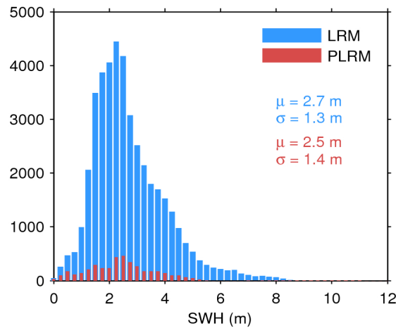
Figure 20. Histogram of science-valid SWH over oceans and lakes for LRM (blue) and PLRM (red) for 17/04/2016. The mean ( \mu ) and standard deviation ( \sigma ) are also shown. Note that values larger than 12 m are excluded from the histogram for the sake of readability but not from the computation of \mu and \sigma .
