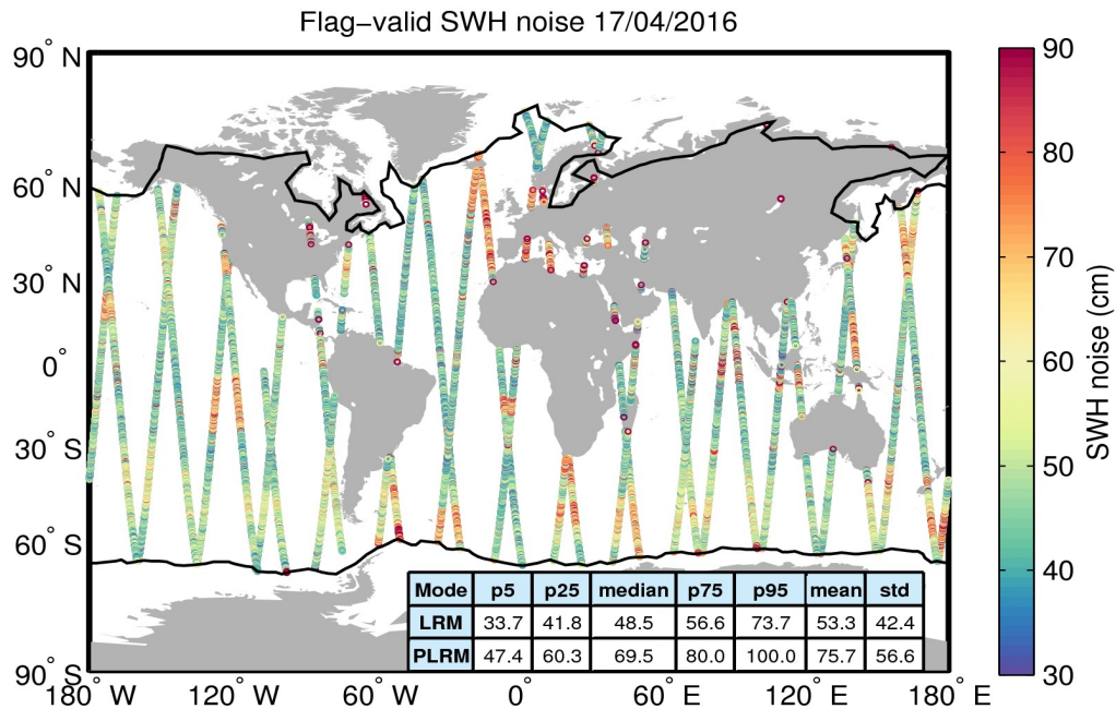
Figure 18. Geographical distribution of flag-valid 20-Hz SWH measurement noise over oceans and lakes for 17/04/2016. The statistical values shown in the table refer to the SWH noise and are calculated separately for LRM and PLRM regions. Measurements taken over polar polygons have been excluded from the computation of the statistical values. The black lines mark the outer limit of the Arctic and Antarctic polar polygons.
