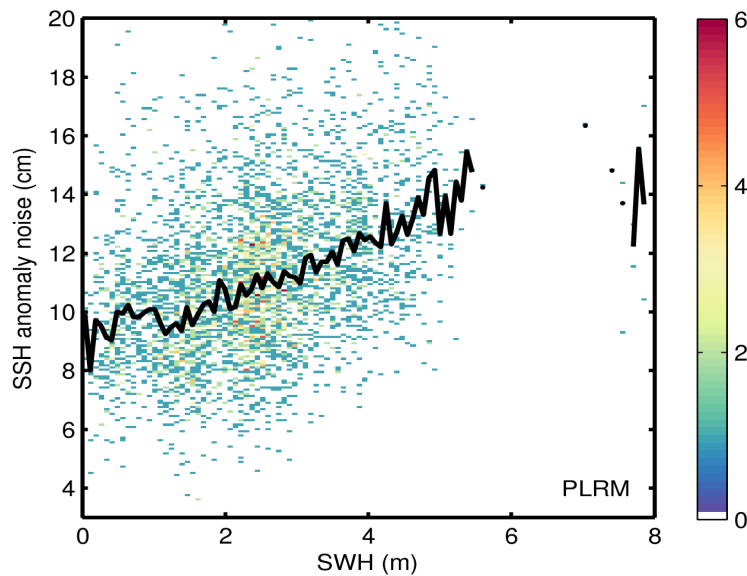
Figure 9. 2D histogram showing flag-valid SSH anomaly noise as a function of SWH for LRM (top) and PLRM (bottom) for 17/04/2016. The black line denotes the median SSH anomaly noise as a function of SWH.
