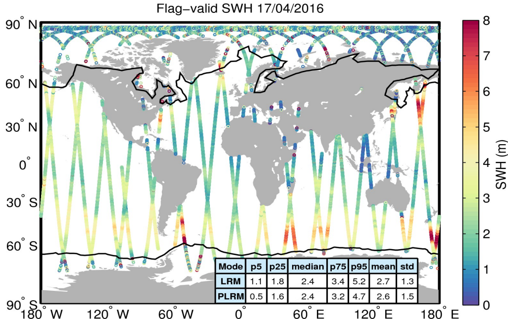
Figure 15. Geographical distribution of flag-valid SWH data over oceans and lakes for 17/04/2016. The statistical values shown in the table refer to the SWH in m and are calculated separately for LRM and PLRM regions. Measurements taken over polar polygons have been excluded from the computation of the statistical values. The black lines mark the outer limit of the Arctic and Antarctic polar polygons.
