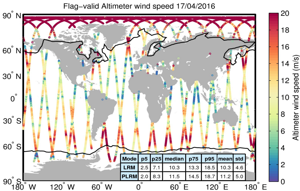
Figure 31. Geographical distribution of flag-valid wind data over oceans and lakes for 17/04/2016. The statistical values shown in the table refer to the wind in m/s and are calculated separately for LRM and PLRM regions. Measurements taken over polar polygons have been excluded from the computation of the statistical values. The black lines mark the outer limit of the Arctic and Antarctic polar polygons.
