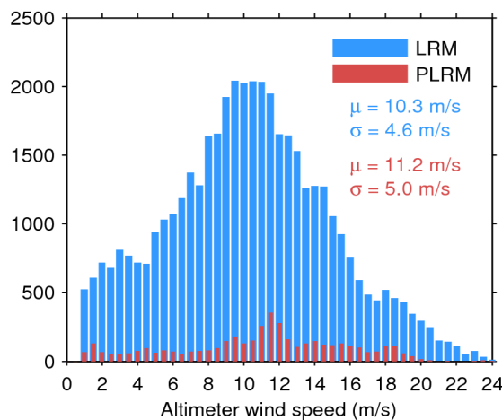
Figure 35. Histogram of science-valid wind over oceans and lakes for LRM (blue) and PLRM (red) for 17/04/2016. The mean ( \mu ) and standard deviation ( \sigma ) are also shown. Note that values larger than 24 m/s are excluded from the histogram for the sake of readability but not from the computation of \mu and \sigma .
