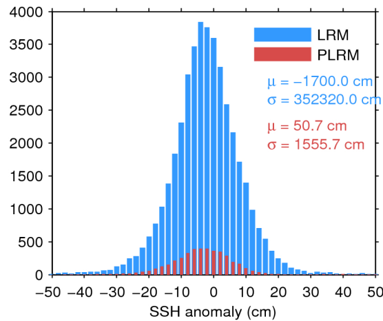
Figure 7. Histogram of flag-valid SSH anomaly over oceans and lakes for LRM (blue) and PLRM (red) for 17/04/2016. The mean ( \mu ) and standard deviation ( \sigma ) are also shown. Note that values outside [-50 50] cm are excluded from the histogram for the sake of readability but not from the computation of \mu and \sigma .
