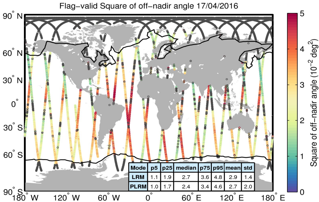
Figure 37. Geographical distribution of flag-valid mispointing data over oceans and lakes for 17/04/2016. The statistical values shown in the table refer to the mispointing in 10^{-2} deg 2 and are calculated separately for LRM and PLRM regions. Measurements taken over polar polygons have been excluded from the computation of the statistical values. The black lines mark the outer limit of the Arctic and Antarctic polar polygons. Gray circles denote negative values.
