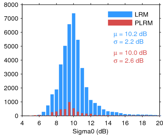
Figure 25. Histogram of flag-valid sigma0 over oceans and lakes for LRM (blue) and PLRM (red) for 17/04/2016. The mean ( \mu ) and standard deviation ( \sigma ) are also shown. Note that values outside [4 20] dB are excluded from the histogram for the sake of readability but not from the computation of \mu and \sigma .
