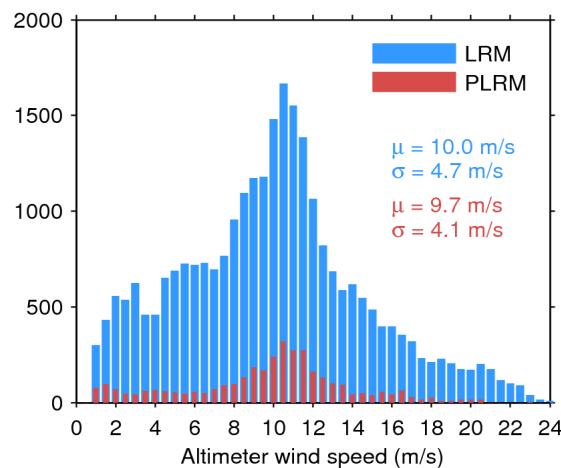
Figure 35. Histogram of science-valid wind over oceans and lakes for LRM (blue) and PLRM (red) for 09/04/2016. The mean ( \mu ) and standard deviation ( \sigma ) are also shown. Note that values larger than 24 m/s are excluded from the histogram for the sake of readability but not from the computation of \mu and \sigma .
