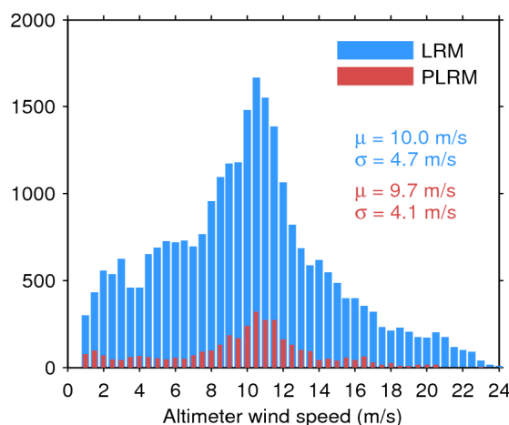
Figure 33. Histogram of flag-valid wind over oceans and lakes for LRM (blue) and PLRM (red) for 09/04/2016. The mean ( \mu ) and standard deviation ( \sigma ) are also shown. Note that values larger than 24 m/s are excluded from the histogram for the sake of readability but not from the computation of \mu and \sigma .
