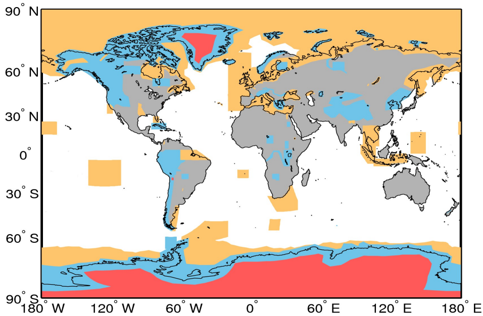
Figure A1. Extent of the regions defining the geographical mode mask for 09/04/2016. The regions where SAR, and SARIn are operated are denoted by the orange and blue polygons, respectively. LRM is operated over areas of the continental ice sheets (red polygons) and over oceans and land not covered by other modes.
