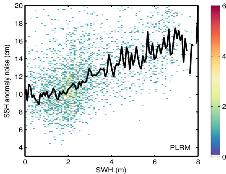
Figure 9. 2D histogram showing flag-valid SSH anomaly noise as a function of SWH for LRM (top) and PLRM (bottom) for 09/04/2016. The black line denotes the median SSH anomaly noise as a function of SWH.
