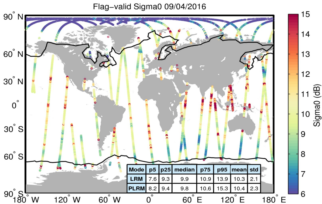
Figure 23. Geographical distribution of flag-valid sigma0 data over oceans and lakes for 09/04/2016. The statistical values shown in the table refer to the sigma0 in dB and are calculated separately for LRM and PLRM regions. Measurements taken over polar polygons have been excluded from the computation of the statistical values. The black lines mark the outer limit of the Arctic and Antarctic polar polygons.
