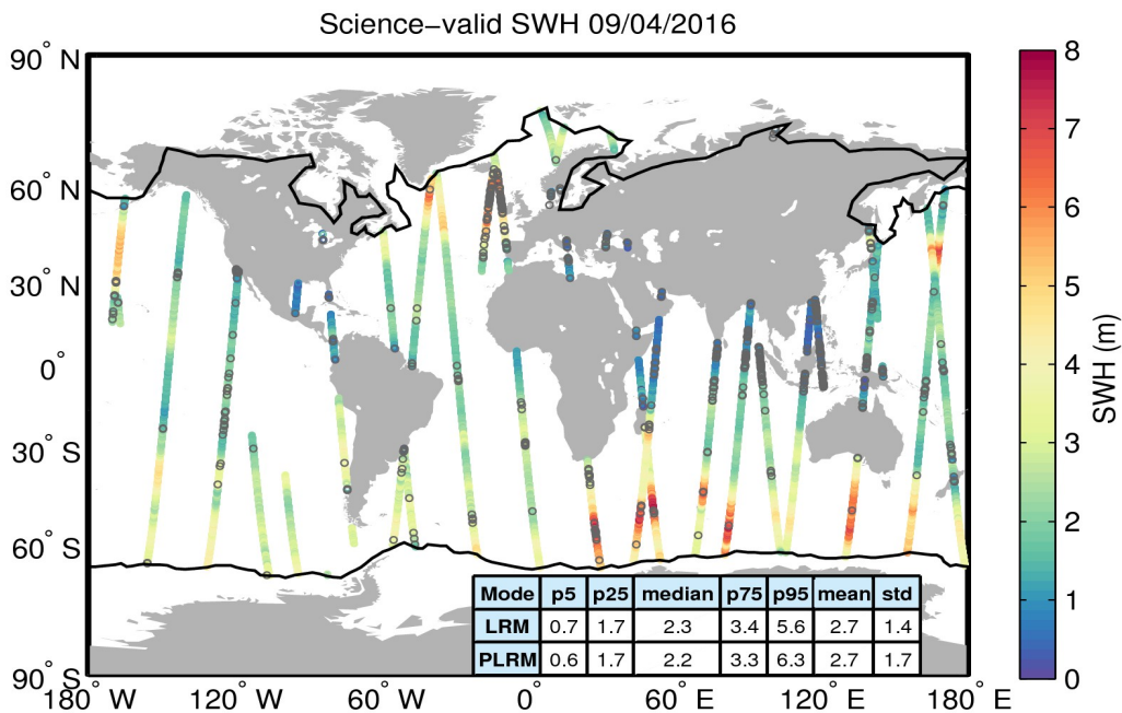
Figure 19. Geographical distribution of science-valid SWH data over oceans and lakes for 09/04/2016. The statistical values shown in the table refer to the SWH in m and are calculated separately for LRM and PLRM regions. The black lines mark the outer limit of the Arctic and Antarctic polar polygons. Gray circles denote records that have been rejected based on the editing criteria described in Table 3.
