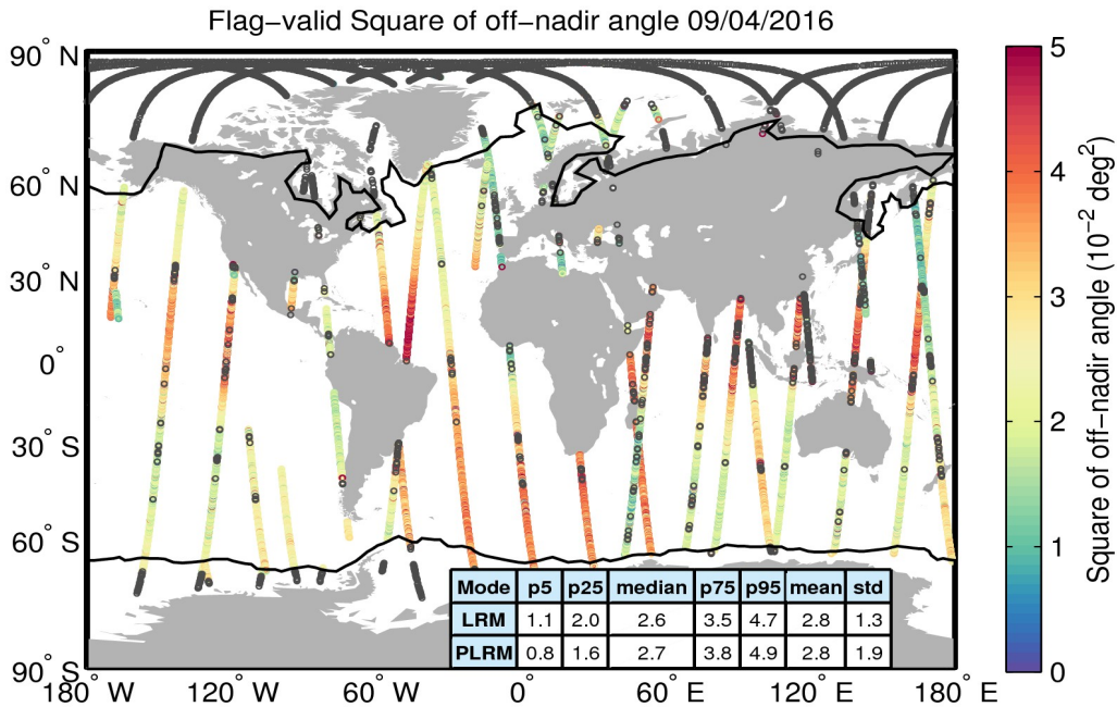
Figure 37. Geographical distribution of flag-valid mispointing data over oceans and lakes for 09/04/2016. The statistical values shown in the table refer to the mispointing in 10^{-2} deg 2 and are calculated separately for LRM and PLRM regions. Measurements taken over polar polygons have been excluded from the computation of the statistical values. The black lines mark the outer limit of the Arctic and Antarctic polar polygons. Gray circles denote negative values.
