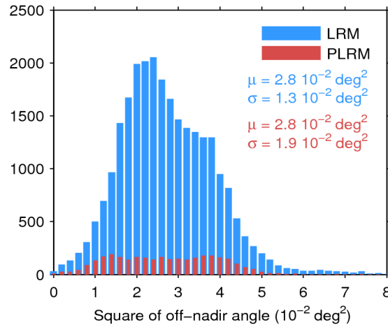
Figure 39. Histogram of flag-valid mispointing over oceans and lakes for LRM (blue) and PLRM (red) for 09/04/2016. Only positive values have been considered. The mean ( \mu ) and standard deviation ( \sigma ) are also shown. Note that values larger than 8 \cdot 10^{-2} \text{ deg}^2 are excluded from the histogram for the sake of readability but not from the computation of \mu and \sigma .
