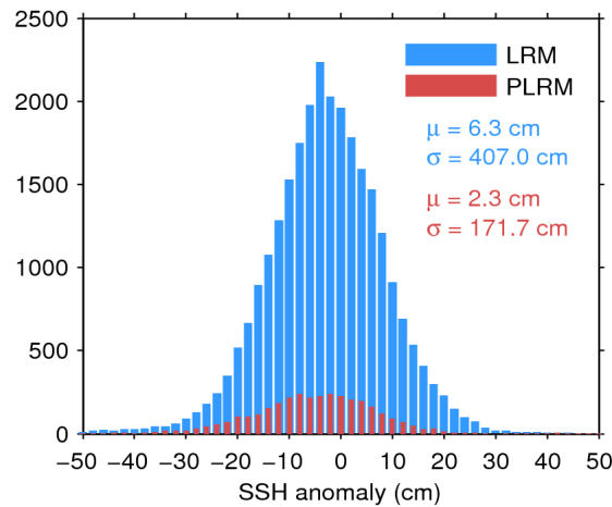
Figure 7. Histogram of flag-valid SSH anomaly over oceans and lakes for LRM (blue) and PLRM (red) for 09/04/2016. The mean ( \mu ) and standard deviation ( \sigma ) are also shown. Note that values outside [-50\ 50] cm are excluded from the histogram for the sake of readability but not from the computation of \mu and \sigma .
