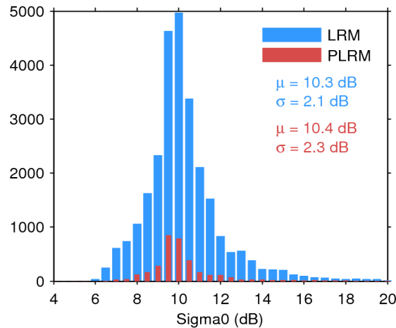
Figure 25. Histogram of flag-valid sigma0 over oceans and lakes for LRM (blue) and PLRM (red) for 09/04/2016. The mean ( \mu ) and standard deviation ( \sigma ) are also shown. Note that values outside [4 20] dB are excluded from the histogram for the sake of readability but not from the computation of \mu and \sigma .
