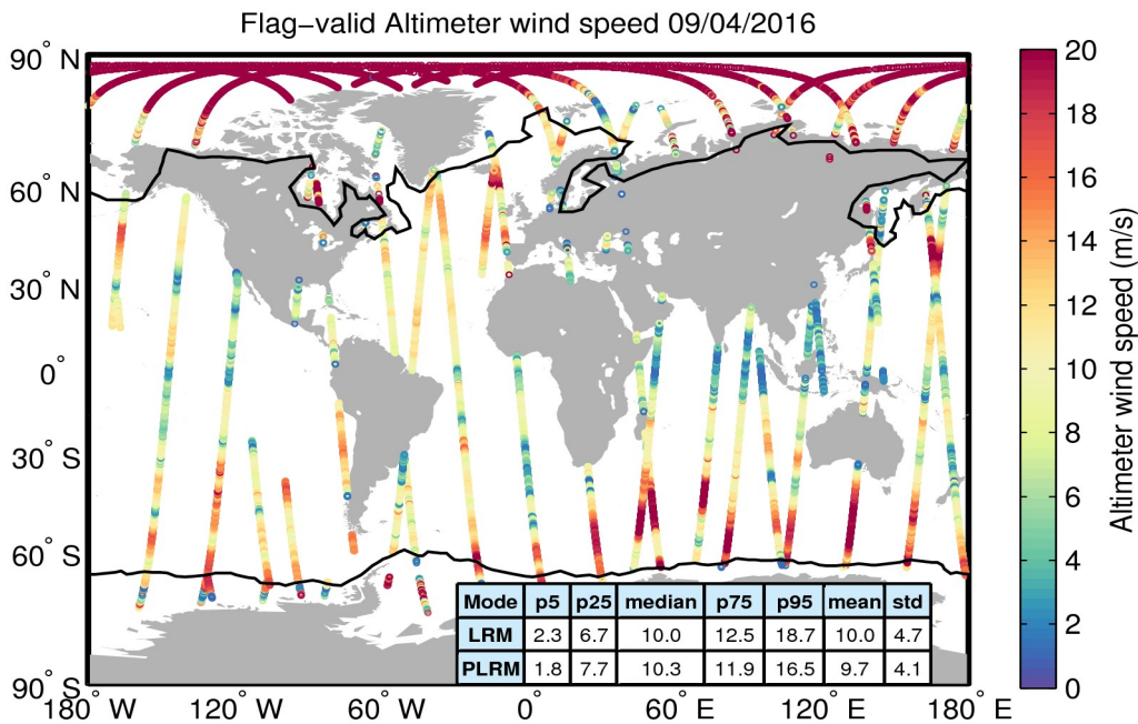
Figure 31. Geographical distribution of flag-valid wind data over oceans and lakes for 09/04/2016. The statistical values shown in the table refer to the wind in m/s and are calculated separately for LRM and PLRM regions. Measurements taken over polar polygons have been excluded from the computation of the statistical values. The black lines mark the outer limit of the Arctic and Antarctic polar polygons.
