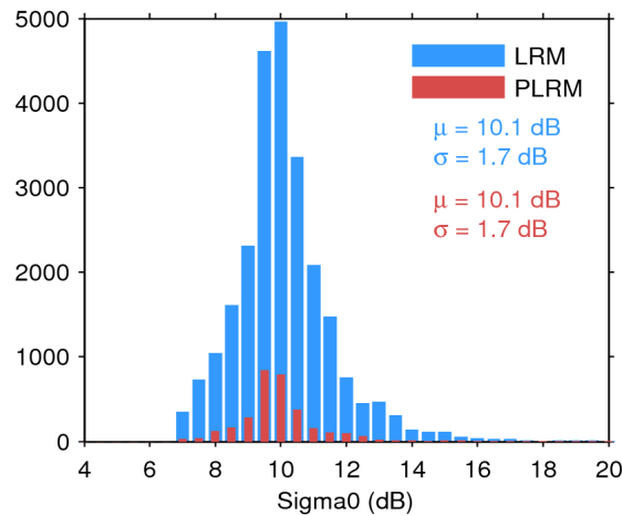
Figure 28. Histogram of science-valid sigma0 over oceans and lakes for LRM (blue) and PLRM (red) for 09/04/2016. The mean ( \mu ) and standard deviation ( \sigma ) are also shown. Note that values outside [4 20] dB are excluded from the histogram for the sake of readability but not from the computation of \mu and \sigma .
