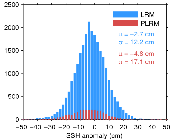
Figure 11. Histogram of science-valid SSH anomaly over oceans and lakes for LRM (blue) and PLRM (red) for 09/04/2016. The mean ( \mu ) and standard deviation ( \sigma ) are also shown. Note that values outside [-50 50] cm are excluded from the histogram for the sake of readability but not from the computation of \mu and \sigma .
