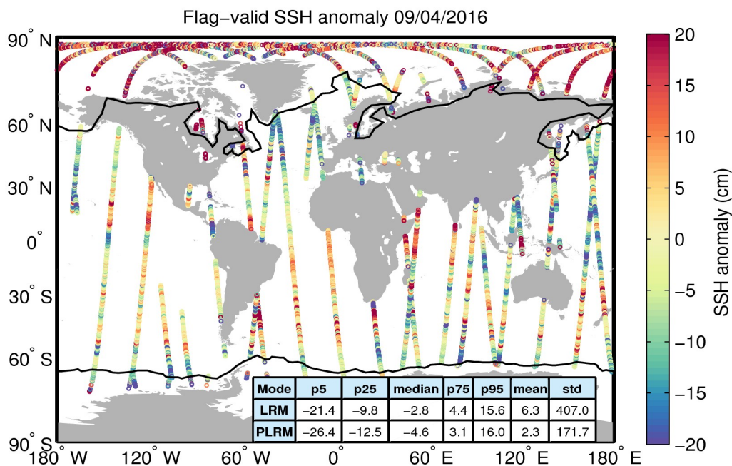
Figure 5. Geographical distribution of flag-valid 1-Hz SSH anomaly data over oceans and lakes for 09/04/2016. The statistical values shown in the table refer to the SSH anomaly in cm and are calculated separately for LRM and PLRM regions. Measurements taken over polar polygons have been excluded from the computation of the statistical values. The black lines mark the outer limit of the Arctic and Antarctic polar polygons.
