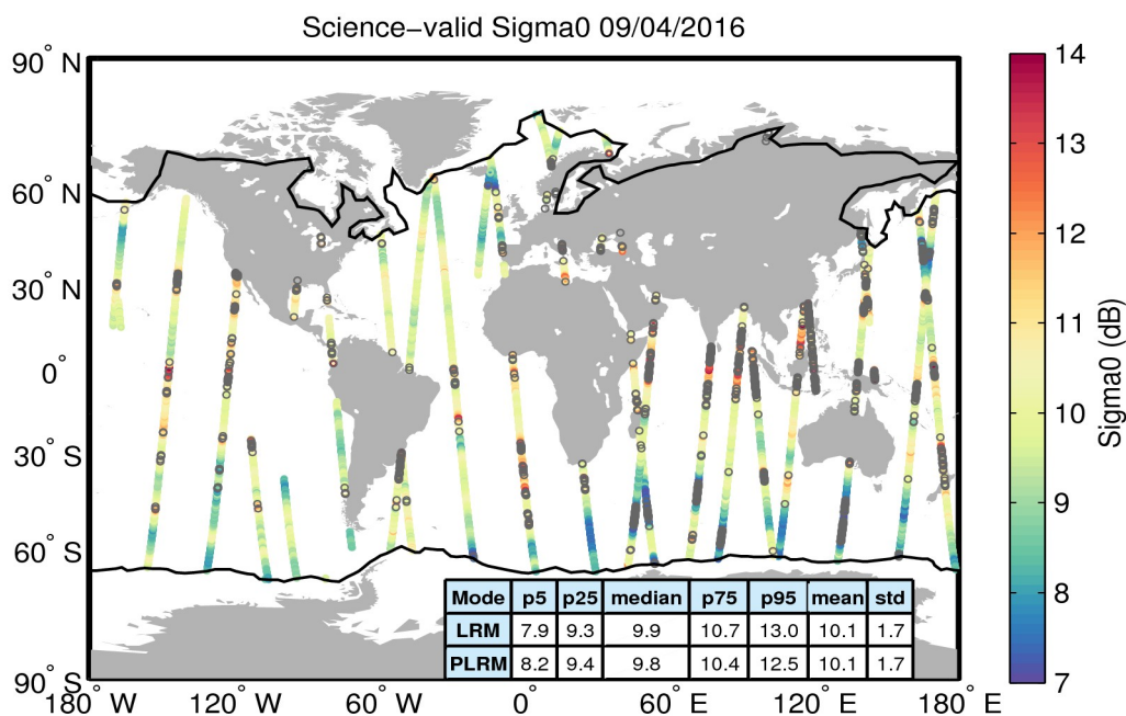
Figure 27. Geographical distribution of science-valid sigma0 data over oceans and lakes for 09/04/2016. The statistical values shown in the table refer to the sigma0 in dB and are calculated separately for LRM and PLRM regions. The black lines mark the outer limit of the Arctic and Antarctic polar polygons. Gray circles denote records that have been rejected based on the editing criteria described in Table 4.
