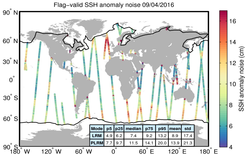
Figure 8. Geographical distribution of flag-valid 20-Hz SSH anomaly measurement noise over oceans and lakes for 09/04/2016. The statistical values shown in the table refer to the SSH anomaly noise and are calculated separately for LRM and PLRM regions. Measurements taken over polar polygons have been excluded from the computation of the statistical values. The black lines mark the outer limit of the Arctic and Antarctic polar polygons.
