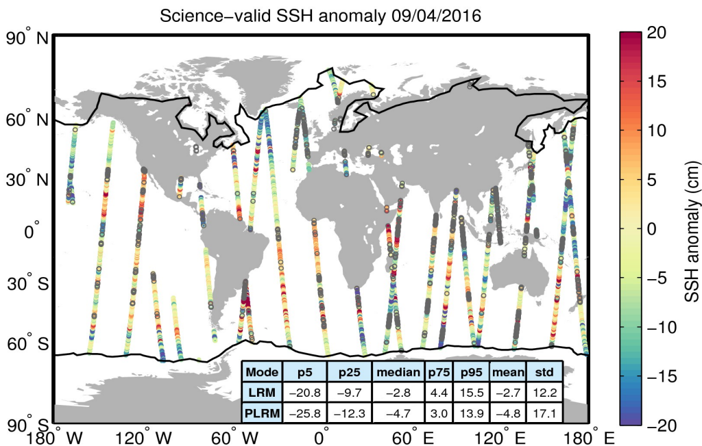
Figure 10. Geographical distribution of science-valid SSH anomaly data over oceans and lakes for 09/04/2016. The statistical values shown in the table refer to the SSH anomaly in cm and are calculated separately for LRM and PLRM regions. The black lines mark the outer limit of the Arctic and Antarctic polar polygons. Gray circles denote records that have been rejected based on the editing criteria described in Table 2.
