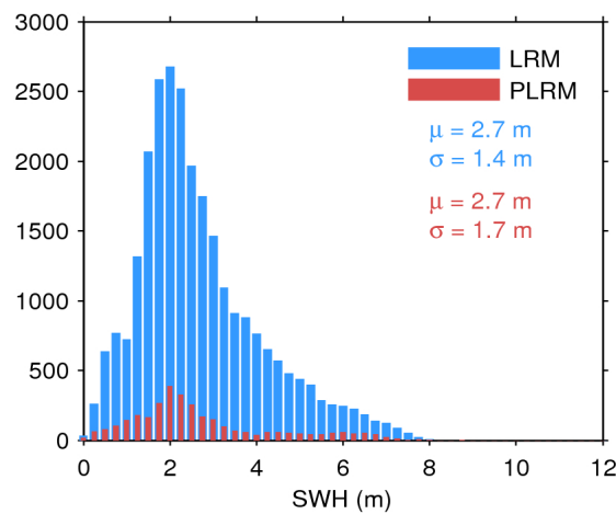
Figure 20. Histogram of science-valid SWH over oceans and lakes for LRM (blue) and PLRM (red) for 09/04/2016. The mean ( \mu ) and standard deviation ( \sigma ) are also shown. Note that values larger than 12 m are excluded from the histogram for the sake of readability but not from the computation of \mu and \sigma .
