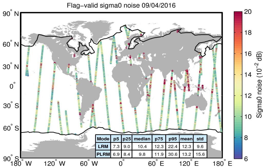
Figure 26. Geographical distribution of flag-valid 20-Hz sigma0 measurement noise over oceans and lakes for 09/04/2016. The statistical values shown in the table refer to the sigma0 noise and are calculated separately for LRM and PLRM regions. Measurements taken over polar polygons have been excluded from the computation of the statistical values. The black lines mark the outer limit of the Arctic and Antarctic polar polygons.
