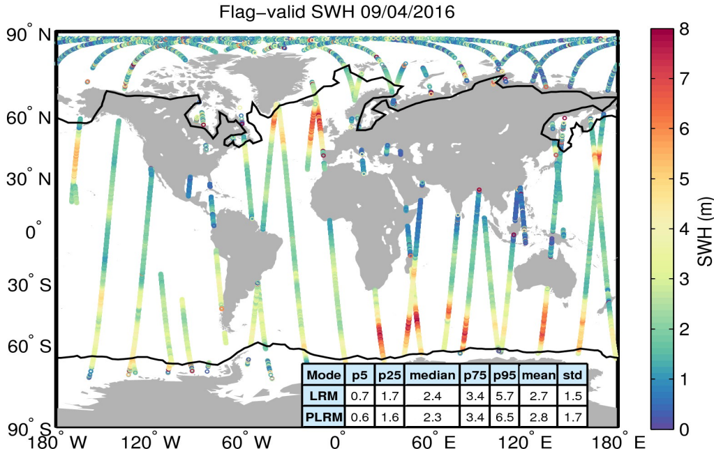
Figure 15. Geographical distribution of flag-valid SWH data over oceans and lakes for 09/04/2016. The statistical values shown in the table refer to the SWH in m and are calculated separately for LRM and PLRM regions. Measurements taken over polar polygons have been excluded from the computation of the statistical values. The black lines mark the outer limit of the Arctic and Antarctic polar polygons.
