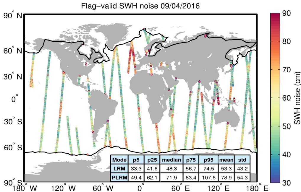
Figure 18. Geographical distribution of flag-valid 20-Hz SWH measurement noise over oceans and lakes for 09/04/2016. The statistical values shown in the table refer to the SWH noise and are calculated separately for LRM and PLRM regions. Measurements taken over polar polygons have been excluded from the computation of the statistical values. The black lines mark the outer limit of the Arctic and Antarctic polar polygons.
