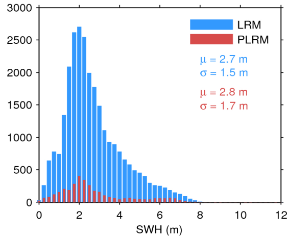
Figure 17. Histogram of flag-valid SWH over oceans and lakes for LRM (blue) and PLRM (red) for 09/04/2016. The mean ( \mu ) and standard deviation ( \sigma ) are also shown. Note that values larger than 12 m are excluded from the histogram for the sake of readability but not from the computation of \mu and \sigma .
