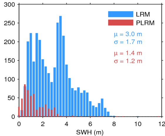
Figure 17. Histogram of flag-valid SWH over oceans and lakes for LRM (blue) and PLRM (red) for 08/04/2016. The mean ( \mu ) and standard deviation ( \sigma ) are also shown. Note that values larger than 12 m are excluded from the histogram for the sake of readability but not from the computation of \mu and \sigma .
