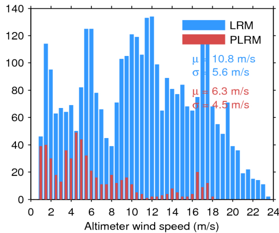
Figure 33. Histogram of flag-valid wind over oceans and lakes for LRM (blue) and PLRM (red) for 08/04/2016. The mean ( \mu ) and standard deviation ( \sigma ) are also shown. Note that values larger than 24 m/s are excluded from the histogram for the sake of readability but not from the computation of \mu and \sigma .
