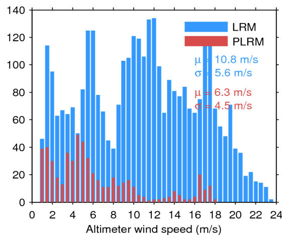
Figure 35. Histogram of science-valid wind over oceans and lakes for LRM (blue) and PLRM (red) for 08/04/2016. The mean ( \mu ) and standard deviation ( \sigma ) are also shown. Note that values larger than 24 m/s are excluded from the histogram for the sake of readability but not from the computation of \mu and \sigma .
