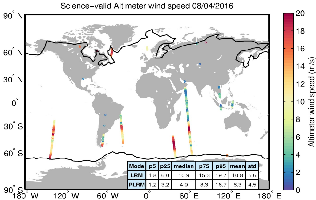
Figure 34. Geographical distribution of science-valid wind data over oceans and lakes for 08/04/2016. The statistical values shown in the table refer to the wind in m/s and are calculated separately for LRM and PLRM regions. The black lines mark the outer limit of the Arctic and Antarctic polar polygons. Gray circles denote records that have been rejected based on the editing criteria described in Table 5.
