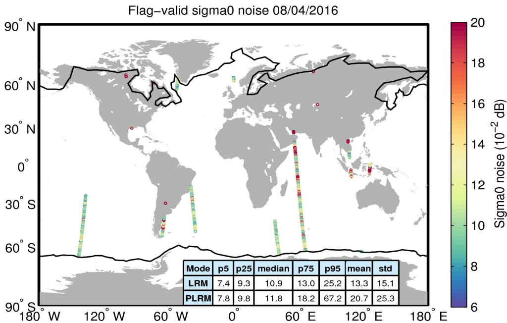
Figure 26. Geographical distribution of flag-valid 20-Hz sigma0 measurement noise over oceans and lakes for 08/04/2016. The statistical values shown in the table refer to the sigma0 noise and are calculated separately for LRM and PLRM regions. Measurements taken over polar polygons have been excluded from the computation of the statistical values. The black lines mark the outer limit of the Arctic and Antarctic polar polygons.
