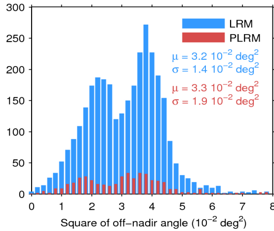
Figure 39. Histogram of flag-valid mispointing over oceans and lakes for LRM (blue) and PLRM (red) for 08/04/2016. Only positive values have been considered. The mean ( \mu ) and standard deviation ( \sigma ) are also shown. Note that values larger than 8 \cdot 10^{-2} \text{ deg}^2 are excluded from the histogram for the sake of readability but not from the computation of \mu and \sigma .
