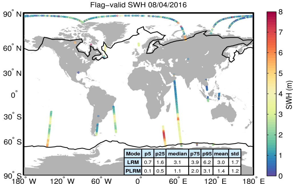
Figure 15. Geographical distribution of flag-valid SWH data over oceans and lakes for 08/04/2016. The statistical values shown in the table refer to the SWH in m and are calculated separately for LRM and PLRM regions. Measurements taken over polar polygons have been excluded from the computation of the statistical values. The black lines mark the outer limit of the Arctic and Antarctic polar polygons.
