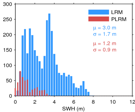
Figure 20. Histogram of science-valid SWH over oceans and lakes for LRM (blue) and PLRM (red) for 08/04/2016. The mean ( \mu ) and standard deviation ( \sigma ) are also shown. Note that values larger than 12 m are excluded from the histogram for the sake of readability but not from the computation of \mu and \sigma .
