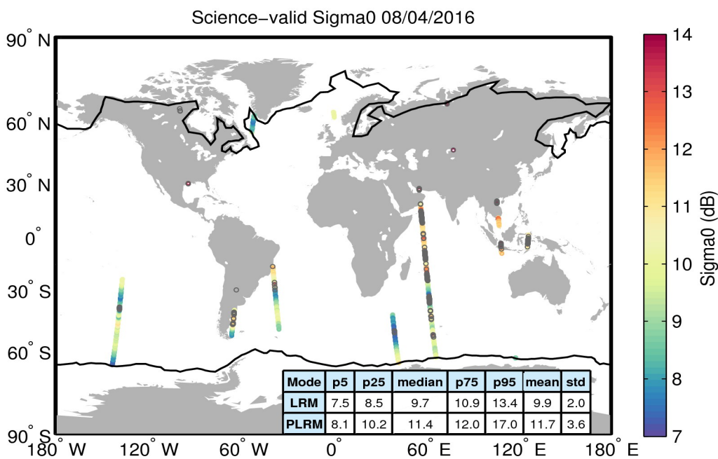
Figure 27. Geographical distribution of science-valid sigma0 data over oceans and lakes for 08/04/2016. The statistical values shown in the table refer to the sigma0 in dB and are calculated separately for LRM and PLRM regions. The black lines mark the outer limit of the Arctic and Antarctic polar polygons. Gray circles denote records that have been rejected based on the editing criteria described in Table 4.
