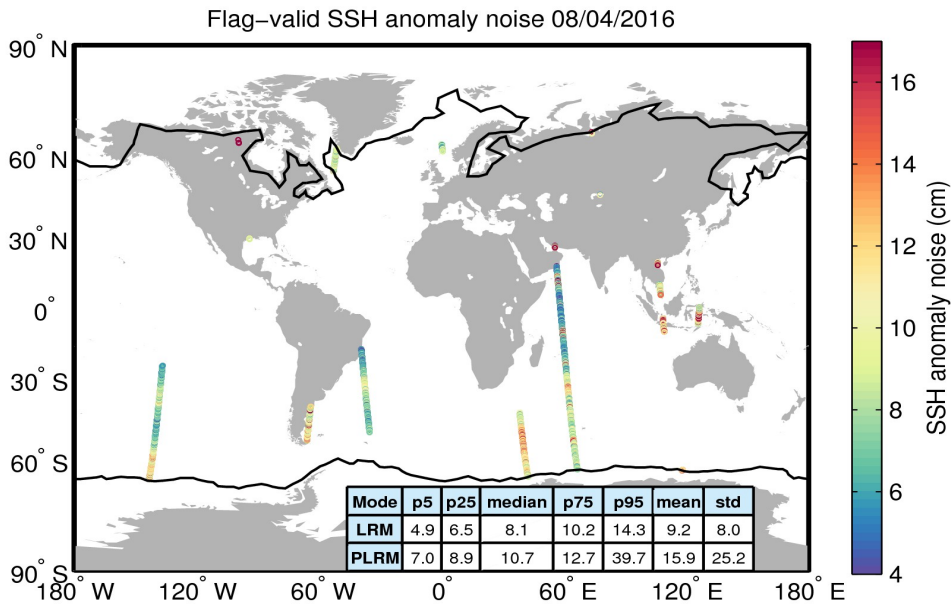
Figure 8. Geographical distribution of flag-valid 20-Hz SSH anomaly measurement noise over oceans and lakes for 08/04/2016. The statistical values shown in the table refer to the SSH anomaly noise and are calculated separately for LRM and PLRM regions. Measurements taken over polar polygons have been excluded from the computation of the statistical values. The black lines mark the outer limit of the Arctic and Antarctic polar polygons.
