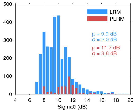
Figure 28. Histogram of science-valid sigma0 over oceans and lakes for LRM (blue) and PLRM (red) for 08/04/2016. The mean ( \mu ) and standard deviation ( \sigma ) are also shown. Note that values outside [4 20] dB are excluded from the histogram for the sake of readability but not from the computation of \mu and \sigma .
