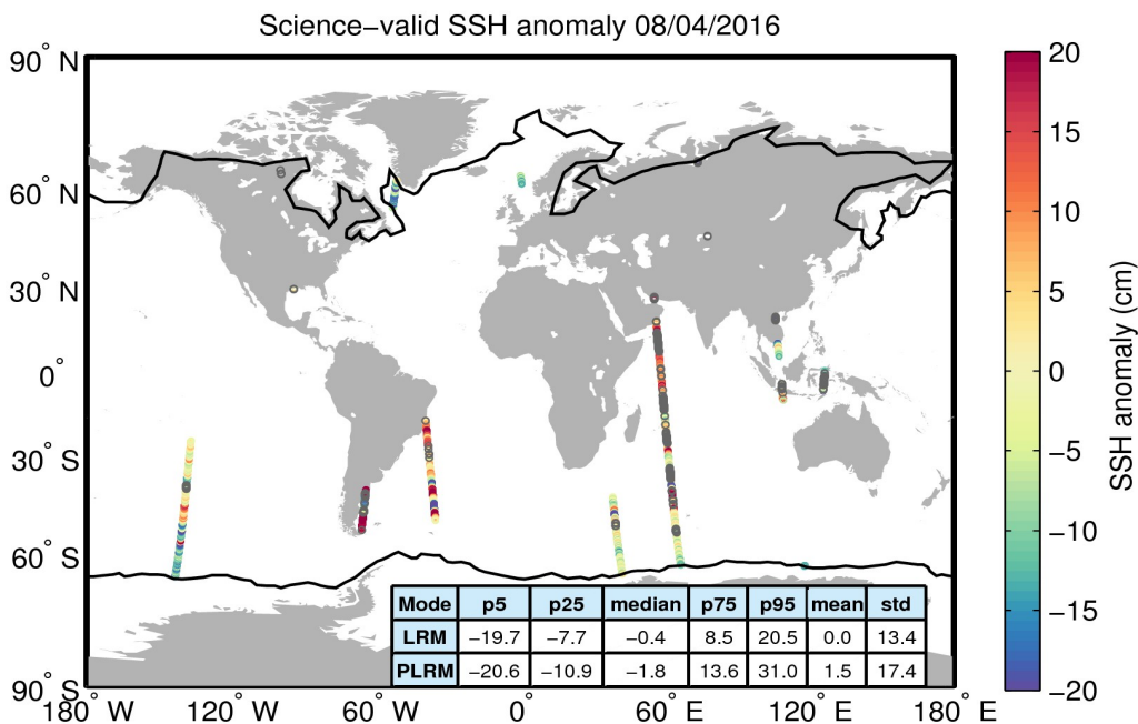
Figure 10. Geographical distribution of science-valid SSH anomaly data over oceans and lakes for 08/04/2016. The statistical values shown in the table refer to the SSH anomaly in cm and are calculated separately for LRM and PLRM regions. The black lines mark the outer limit of the Arctic and Antarctic polar polygons. Gray circles denote records that have been rejected based on the editing criteria described in Table 2.
