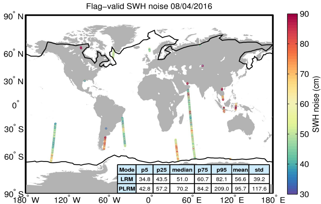
Figure 18. Geographical distribution of flag-valid 20-Hz SWH measurement noise over oceans and lakes for 08/04/2016. The statistical values shown in the table refer to the SWH noise and are calculated separately for LRM and PLRM regions. Measurements taken over polar polygons have been excluded from the computation of the statistical values. The black lines mark the outer limit of the Arctic and Antarctic polar polygons.
