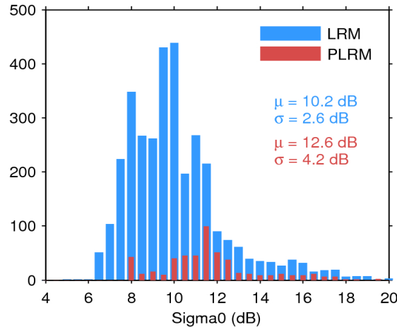
Figure 25. Histogram of flag-valid sigma0 over oceans and lakes for LRM (blue) and PLRM (red) for 08/04/2016. The mean ( \mu ) and standard deviation ( \sigma ) are also shown. Note that values outside [4 20] dB are excluded from the histogram for the sake of readability but not from the computation of \mu and \sigma .
