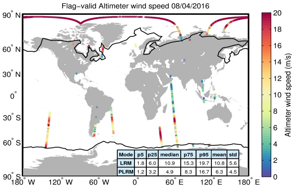
Figure 31. Geographical distribution of flag-valid wind data over oceans and lakes for 08/04/2016. The statistical values shown in the table refer to the wind in m/s and are calculated separately for LRM and PLRM regions. Measurements taken over polar polygons have been excluded from the computation of the statistical values. The black lines mark the outer limit of the Arctic and Antarctic polar polygons.
