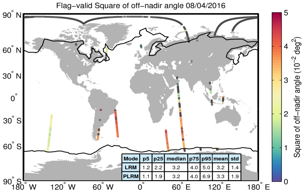
Figure 37. Geographical distribution of flag-valid mispointing data over oceans and lakes for 08/04/2016. The statistical values shown in the table refer to the mispointing in 10^{-2} deg 2 and are calculated separately for LRM and PLRM regions. Measurements taken over polar polygons have been excluded from the computation of the statistical values. The black lines mark the outer limit of the Arctic and Antarctic polar polygons. Gray circles denote negative values.
