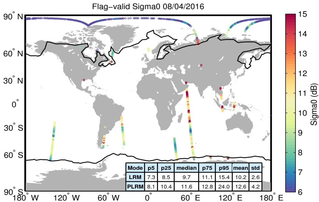
Figure 23. Geographical distribution of flag-valid sigma0 data over oceans and lakes for 08/04/2016. The statistical values shown in the table refer to the sigma0 in dB and are calculated separately for LRM and PLRM regions. Measurements taken over polar polygons have been excluded from the computation of the statistical values. The black lines mark the outer limit of the Arctic and Antarctic polar polygons.
