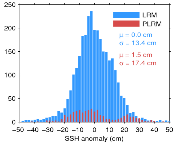
Figure 11. Histogram of science-valid SSH anomaly over oceans and lakes for LRM (blue) and PLRM (red) for 08/04/2016. The mean ( \mu ) and standard deviation ( \sigma ) are also shown. Note that values outside [-50\ 50] cm are excluded from the histogram for the sake of readability but not from the computation of \mu and \sigma .
