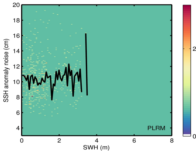
Figure 9. 2D histogram showing flag-valid SSH anomaly noise as a function of SWH for LRM (top) and PLRM (bottom) for 08/04/2016. The black line denotes the median SSH anomaly noise as a function of SWH.
