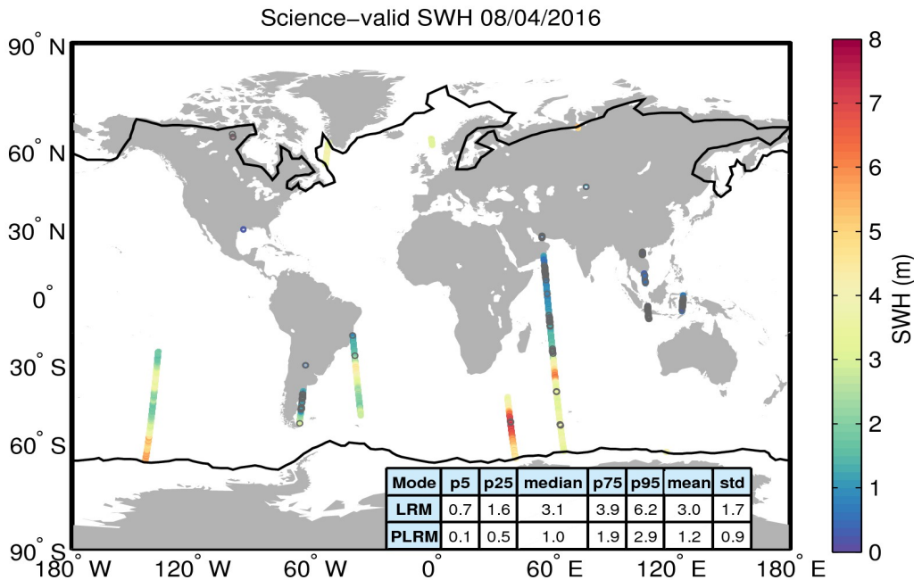
Figure 19. Geographical distribution of science-valid SWH data over oceans and lakes for 08/04/2016. The statistical values shown in the table refer to the SWH in m and are calculated separately for LRM and PLRM regions. The black lines mark the outer limit of the Arctic and Antarctic polar polygons. Gray circles denote records that have been rejected based on the editing criteria described in Table 3.
