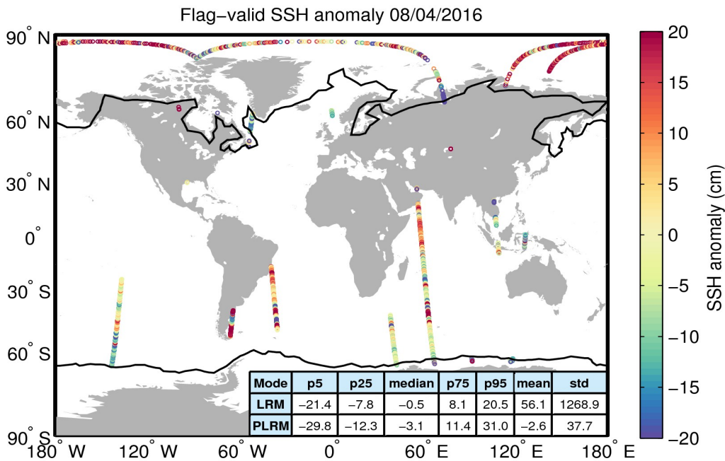
Figure 5. Geographical distribution of flag-valid 1-Hz SSH anomaly data over oceans and lakes for 08/04/2016. The statistical values shown in the table refer to the SSH anomaly in cm and are calculated separately for LRM and PLRM regions. Measurements taken over polar polygons have been excluded from the computation of the statistical values. The black lines mark the outer limit of the Arctic and Antarctic polar polygons.
