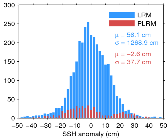
Figure 7. Histogram of flag-valid SSH anomaly over oceans and lakes for LRM (blue) and PLRM (red) for 08/04/2016. The mean ( \mu ) and standard deviation ( \sigma ) are also shown. Note that values outside [-50 \ 50] cm are excluded from the histogram for the sake of readability but not from the computation of \mu and \sigma .
