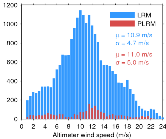
Figure 33. Histogram of flag-valid wind over oceans and lakes for LRM (blue) and PLRM (red) for 06/04/2016. The mean ( \mu ) and standard deviation ( \sigma ) are also shown. Note that values larger than 24 m/s are excluded from the histogram for the sake of readability but not from the computation of \mu and \sigma .
