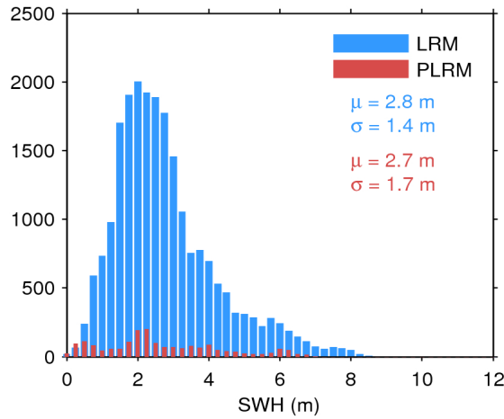
Figure 20. Histogram of science-valid SWH over oceans and lakes for LRM (blue) and PLRM (red) for 06/04/2016. The mean ( \mu ) and standard deviation ( \sigma ) are also shown. Note that values larger than 12 m are excluded from the histogram for the sake of readability but not from the computation of \mu and \sigma .
