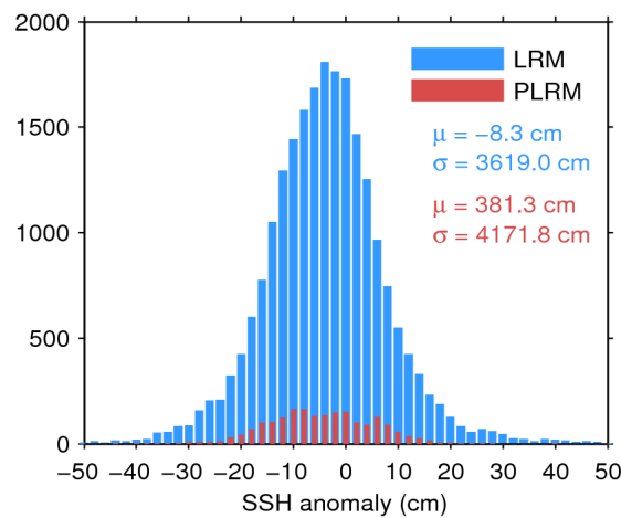
Figure 7. Histogram of flag-valid SSH anomaly over oceans and lakes for LRM (blue) and PLRM (red) for 06/04/2016. The mean ( \mu ) and standard deviation ( \sigma ) are also shown. Note that values outside [-50 50] cm are excluded from the histogram for the sake of readability but not from the computation of \mu and \sigma .
