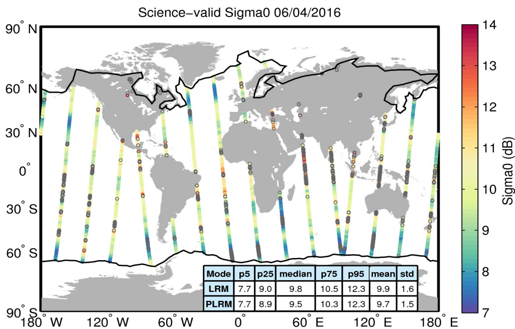
Figure 27. Geographical distribution of science-valid sigma0 data over oceans and lakes for 06/04/2016. The statistical values shown in the table refer to the sigma0 in dB and are calculated separately for LRM and PLRM regions. The black lines mark the outer limit of the Arctic and Antarctic polar polygons. Gray circles denote records that have been rejected based on the editing criteria described in Table 4.
