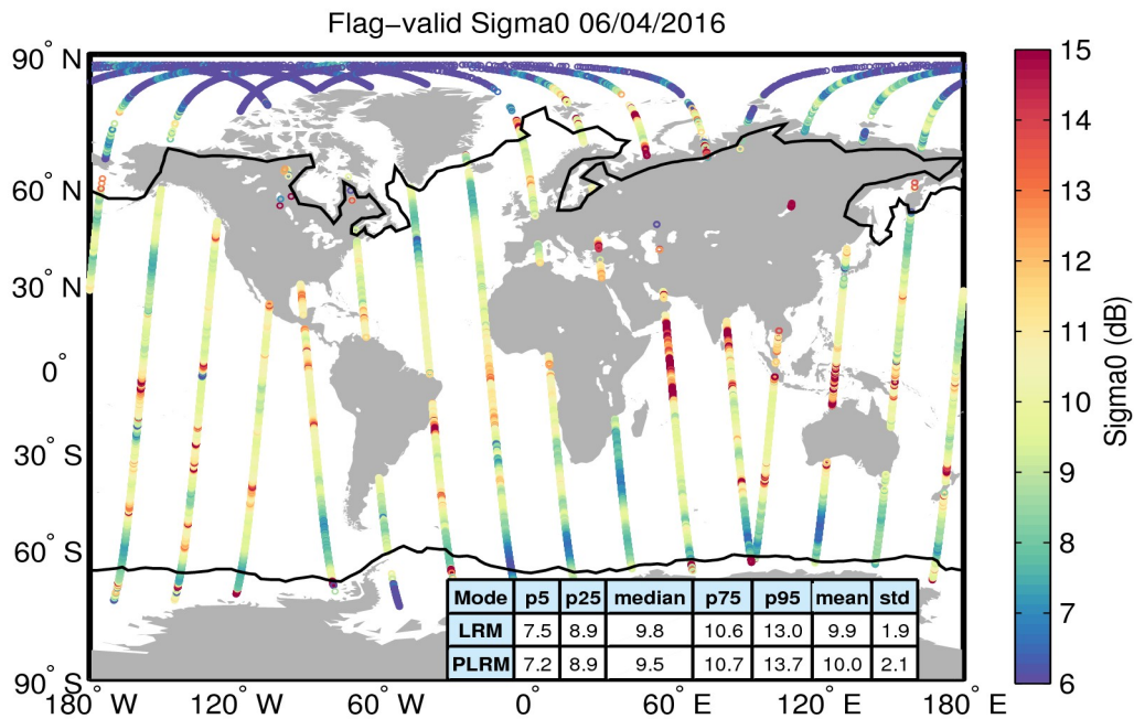
Figure 23. Geographical distribution of flag-valid sigma0 data over oceans and lakes for 06/04/2016. The statistical values shown in the table refer to the sigma0 in dB and are calculated separately for LRM and PLRM regions. Measurements taken over polar polygons have been excluded from the computation of the statistical values. The black lines mark the outer limit of the Arctic and Antarctic polar polygons.
