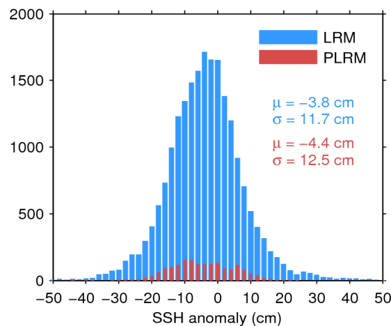
Figure 11. Histogram of science-valid SSH anomaly over oceans and lakes for LRM (blue) and PLRM (red) for 06/04/2016. The mean ( \mu ) and standard deviation ( \sigma ) are also shown. Note that values outside [-50 50] cm are excluded from the histogram for the sake of readability but not from the computation of \mu and \sigma .
