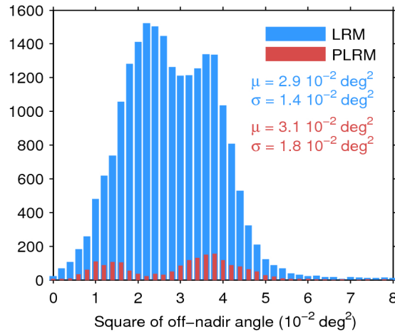
Figure 39. Histogram of flag-valid mispointing over oceans and lakes for LRM (blue) and PLRM (red) for 06/04/2016. Only positive values have been considered. The mean ( \mu ) and standard deviation ( \sigma ) are also shown. Note that values larger than 8 \cdot 10^{-2} \text{ deg}^2 are excluded from the histogram for the sake of readability but not from the computation of \mu and \sigma .
