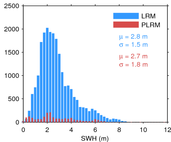
Figure 17. Histogram of flag-valid SWH over oceans and lakes for LRM (blue) and PLRM (red) for 06/04/2016. The mean ( \mu ) and standard deviation ( \sigma ) are also shown. Note that values larger than 12 m are excluded from the histogram for the sake of readability but not from the computation of \mu and \sigma .
