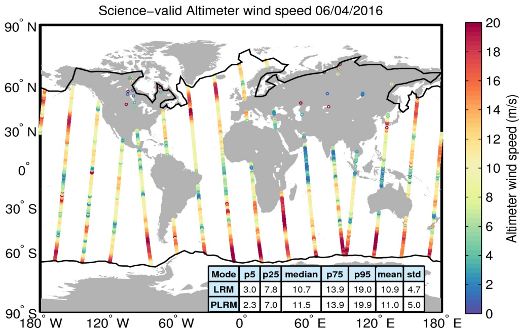
Figure 34. Geographical distribution of science-valid wind data over oceans and lakes for 06/04/2016. The statistical values shown in the table refer to the wind in m/s and are calculated separately for LRM and PLRM regions. The black lines mark the outer limit of the Arctic and Antarctic polar polygons. Gray circles denote records that have been rejected based on the editing criteria described in Table 5.
