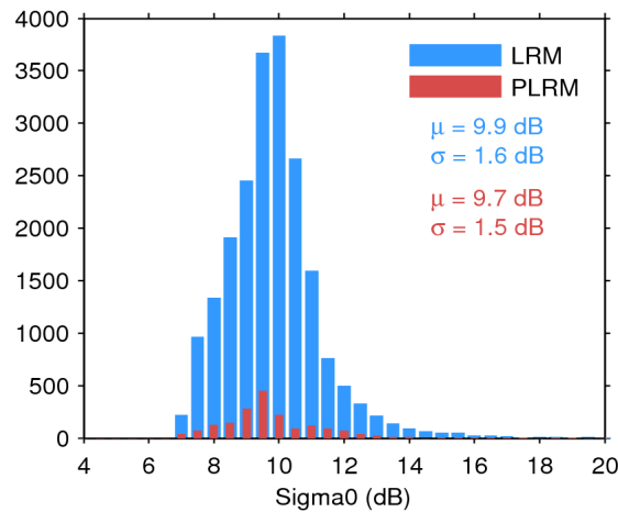
Figure 28. Histogram of science-valid sigma0 over oceans and lakes for LRM (blue) and PLRM (red) for 06/04/2016. The mean ( \mu ) and standard deviation ( \sigma ) are also shown. Note that values outside [4 20] dB are excluded from the histogram for the sake of readability but not from the computation of \mu and \sigma .
