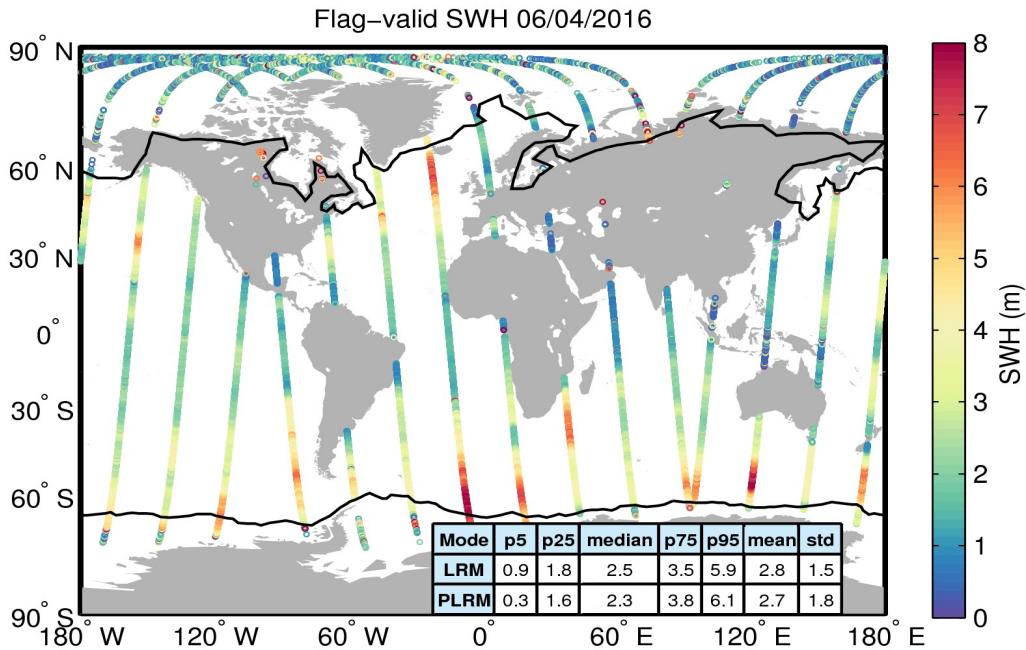
Figure 15. Geographical distribution of flag-valid SWH data over oceans and lakes for 06/04/2016. The statistical values shown in the table refer to the SWH in m and are calculated separately for LRM and PLRM regions. Measurements taken over polar polygons have been excluded from the computation of the statistical values. The black lines mark the outer limit of the Arctic and Antarctic polar polygons.
