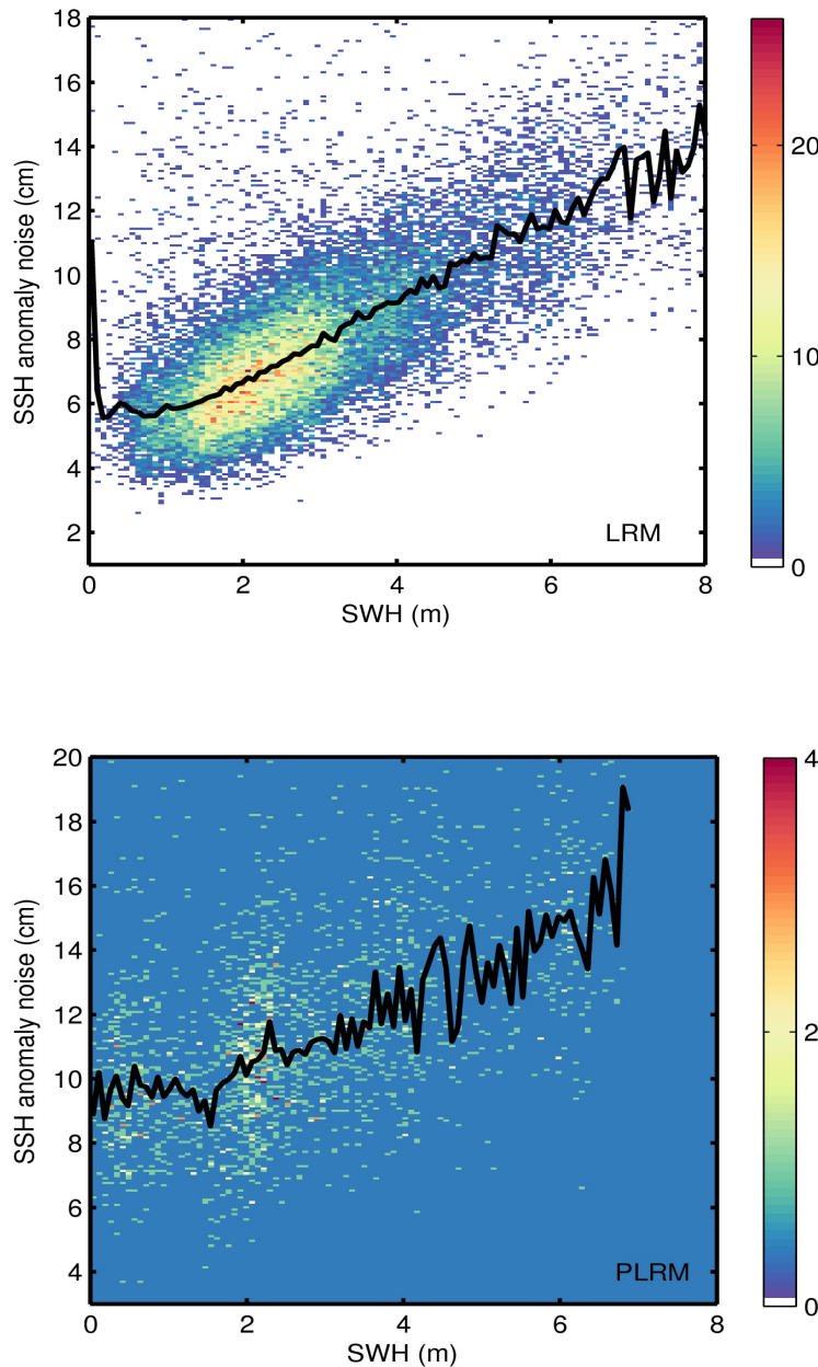
Figure 9. 2D histogram showing flag-valid SSH anomaly noise as a function of SWH for LRM (top) and PLRM (bottom) for 06/04/2016. The black line denotes the median SSH anomaly noise as a function of SWH.
