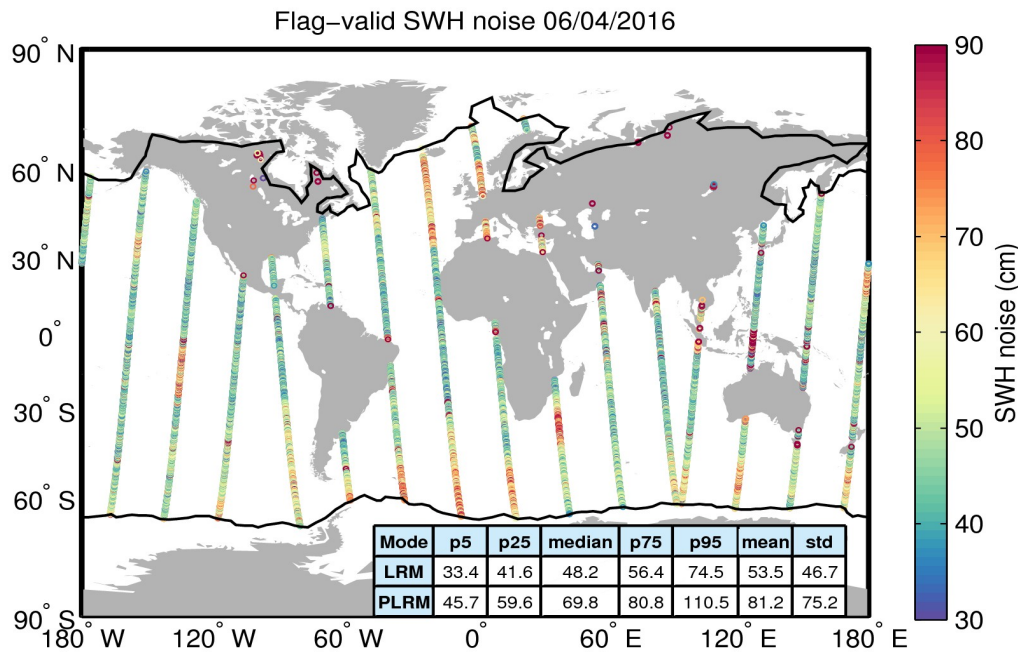
Figure 18. Geographical distribution of flag-valid 20-Hz SWH measurement noise over oceans and lakes for 06/04/2016. The statistical values shown in the table refer to the SWH noise and are calculated separately for LRM and PLRM regions. Measurements taken over polar polygons have been excluded from the computation of the statistical values. The black lines mark the outer limit of the Arctic and Antarctic polar polygons.
