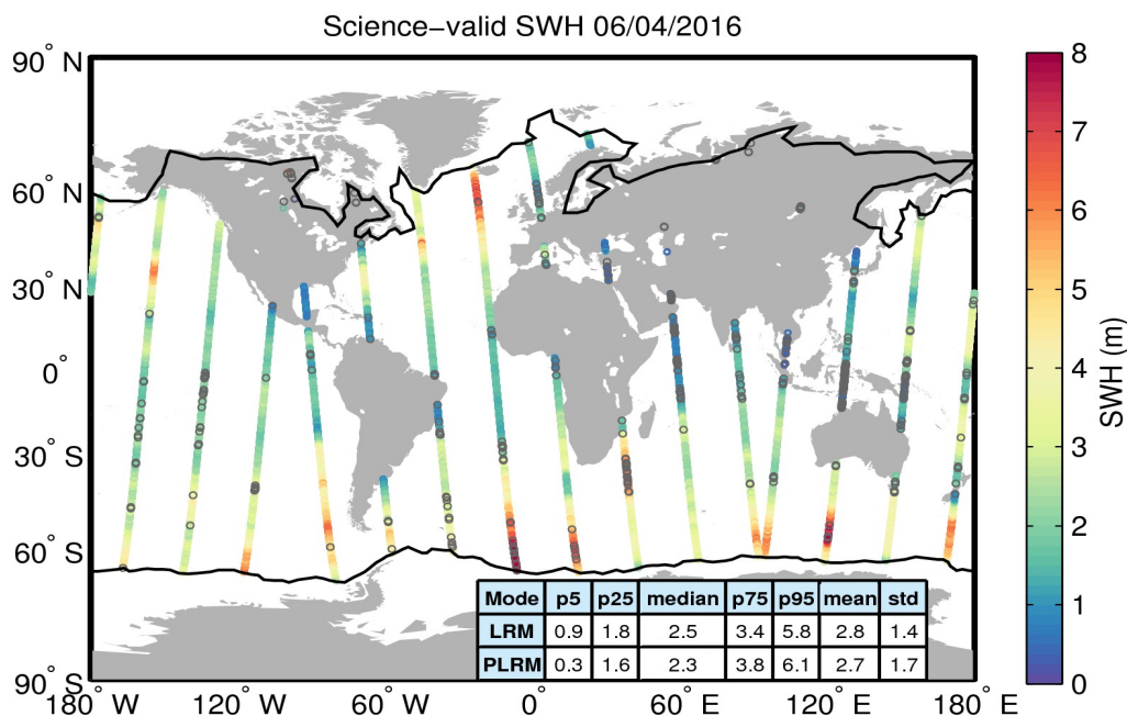
Figure 19. Geographical distribution of science-valid SWH data over oceans and lakes for 06/04/2016. The statistical values shown in the table refer to the SWH in m and are calculated separately for LRM and PLRM regions. The black lines mark the outer limit of the Arctic and Antarctic polar polygons. Gray circles denote records that have been rejected based on the editing criteria described in Table 3.
