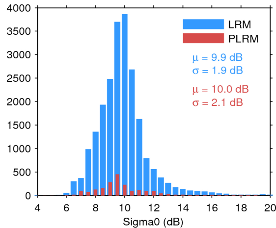
Figure 25. Histogram of flag-valid sigma0 over oceans and lakes for LRM (blue) and PLRM (red) for 06/04/2016. The mean ( \mu ) and standard deviation ( \sigma ) are also shown. Note that values outside [4 20] dB are excluded from the histogram for the sake of readability but not from the computation of \mu and \sigma .
