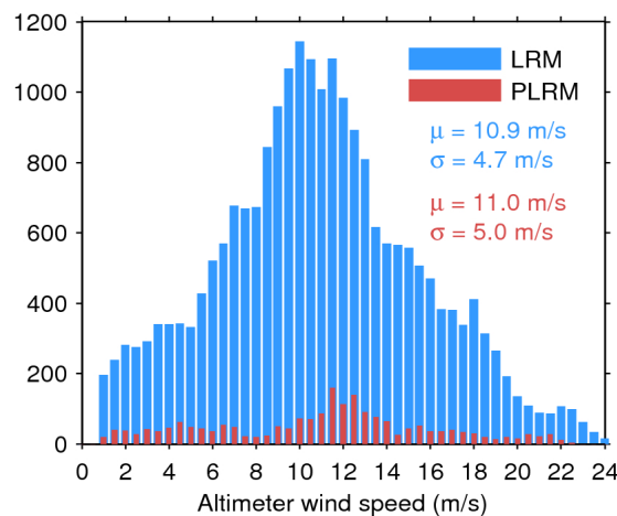
Figure 35. Histogram of science-valid wind over oceans and lakes for LRM (blue) and PLRM (red) for 06/04/2016. The mean ( \mu ) and standard deviation ( \sigma ) are also shown. Note that values larger than 24 m/s are excluded from the histogram for the sake of readability but not from the computation of \mu and \sigma .
