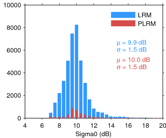
Figure 28. Histogram of science-valid sigma0 over oceans and lakes for LRM (blue) and PLRM (red) for 04/04/2016. The mean ( \mu ) and standard deviation ( \sigma ) are also shown. Note that values outside [4 20] dB are excluded from the histogram for the sake of readability but not from the computation of \mu and \sigma .
