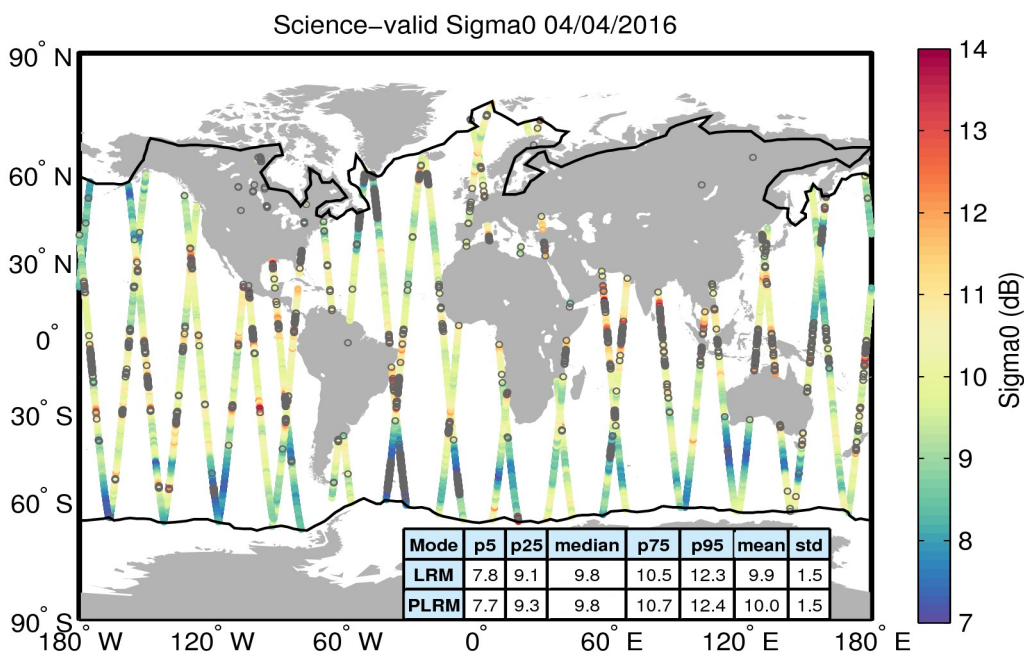
Figure 27. Geographical distribution of science-valid sigma0 data over oceans and lakes for 04/04/2016. The statistical values shown in the table refer to the sigma0 in dB and are calculated separately for LRM and PLRM regions. The black lines mark the outer limit of the Arctic and Antarctic polar polygons. Gray circles denote records that have been rejected based on the editing criteria described in Table 4.
