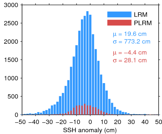
Figure 7. Histogram of flag-valid SSH anomaly over oceans and lakes for LRM (blue) and PLRM (red) for 04/04/2016. The mean ( \mu ) and standard deviation ( \sigma ) are also shown. Note that values outside [-50\ 50] cm are excluded from the histogram for the sake of readability but not from the computation of \mu and \sigma .
