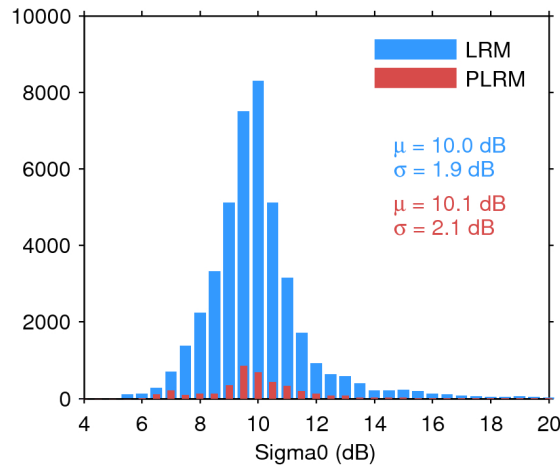
Figure 25. Histogram of flag-valid sigma0 over oceans and lakes for LRM (blue) and PLRM (red) for 04/04/2016. The mean ( \mu ) and standard deviation ( \sigma ) are also shown. Note that values outside [4 20] dB are excluded from the histogram for the sake of readability but not from the computation of \mu and \sigma .
