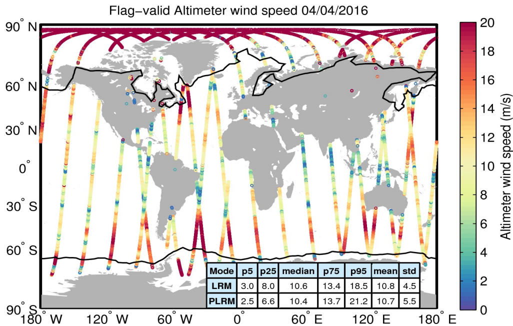
Figure 31. Geographical distribution of flag-valid wind data over oceans and lakes for 04/04/2016. The statistical values shown in the table refer to the wind in m/s and are calculated separately for LRM and PLRM regions. Measurements taken over polar polygons have been excluded from the computation of the statistical values. The black lines mark the outer limit of the Arctic and Antarctic polar polygons.
