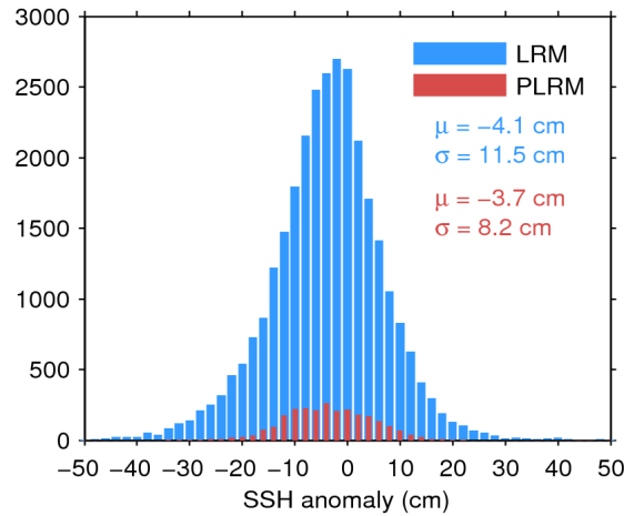
Figure 11. Histogram of science-valid SSH anomaly over oceans and lakes for LRM (blue) and PLRM (red) for 04/04/2016. The mean ( \mu ) and standard deviation ( \sigma ) are also shown. Note that values outside [-50 50] cm are excluded from the histogram for the sake of readability but not from the computation of \mu and \sigma .
