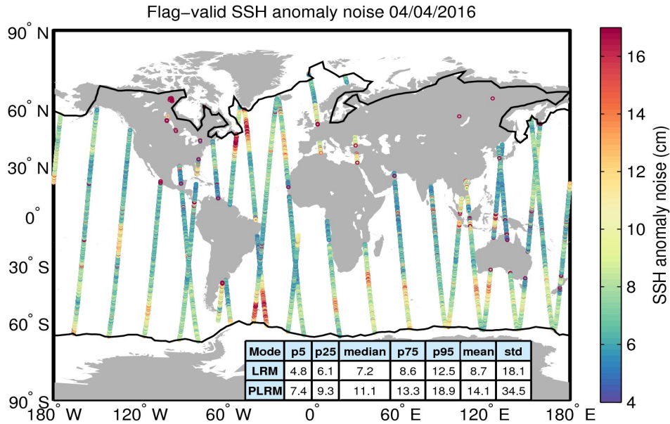
Figure 8. Geographical distribution of flag-valid 20-Hz SSH anomaly measurement noise over oceans and lakes for 04/04/2016. The statistical values shown in the table refer to the SSH anomaly noise and are calculated separately for LRM and PLRM regions. Measurements taken over polar polygons have been excluded from the computation of the statistical values. The black lines mark the outer limit of the Arctic and Antarctic polar polygons.
