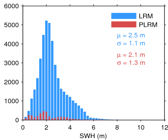
Figure 20. Histogram of science-valid SWH over oceans and lakes for LRM (blue) and PLRM (red) for 02/04/2016. The mean ( \mu ) and standard deviation ( \sigma ) are also shown. Note that values larger than 12 m are excluded from the histogram for the sake of readability but not from the computation of \mu and \sigma .
