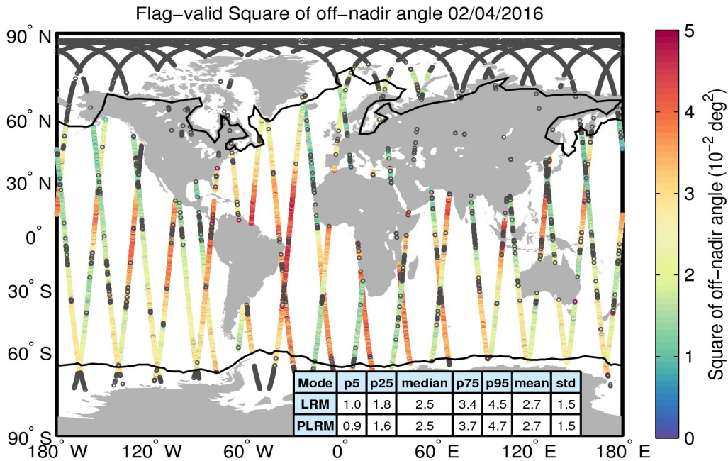
Figure 37. Geographical distribution of flag-valid mispointing data over oceans and lakes for 02/04/2016. The statistical values shown in the table refer to the mispointing in 10^{-2} deg 2 and are calculated separately for LRM and PLRM regions. Measurements taken over polar polygons have been excluded from the computation of the statistical values. The black lines mark the outer limit of the Arctic and Antarctic polar polygons. Gray circles denote negative values.
