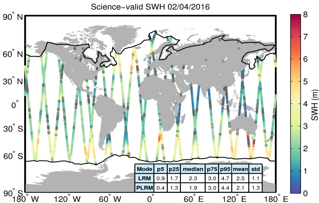
Figure 19. Geographical distribution of science-valid SWH data over oceans and lakes for 02/04/2016. The statistical values shown in the table refer to the SWH in m and are calculated separately for LRM and PLRM regions. The black lines mark the outer limit of the Arctic and Antarctic polar polygons. Gray circles denote records that have been rejected based on the editing criteria described in Table 3.
