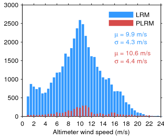
Figure 33. Histogram of flag-valid wind over oceans and lakes for LRM (blue) and PLRM (red) for 02/04/2016. The mean ( \mu ) and standard deviation ( \sigma ) are also shown. Note that values larger than 24 m/s are excluded from the histogram for the sake of readability but not from the computation of \mu and \sigma .
