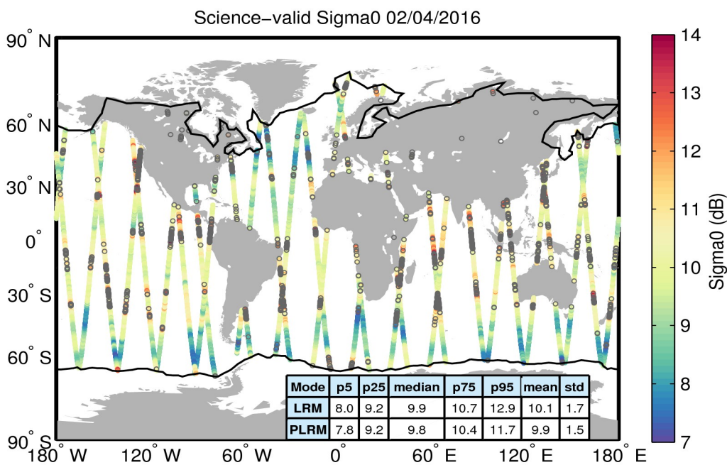
Figure 27. Geographical distribution of science-valid sigma0 data over oceans and lakes for 02/04/2016. The statistical values shown in the table refer to the sigma0 in dB and are calculated separately for LRM and PLRM regions. The black lines mark the outer limit of the Arctic and Antarctic polar polygons. Gray circles denote records that have been rejected based on the editing criteria described in Table 4.
