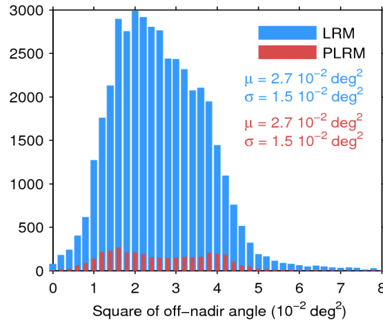
Figure 39. Histogram of flag-valid mispointing over oceans and lakes for LRM (blue) and PLRM (red) for 02/04/2016. Only positive values have been considered. The mean ( \mu ) and standard deviation ( \sigma ) are also shown. Note that values larger than 8 \cdot 10^{-2} \text{ deg}^2 are excluded from the histogram for the sake of readability but not from the computation of \mu and \sigma .
