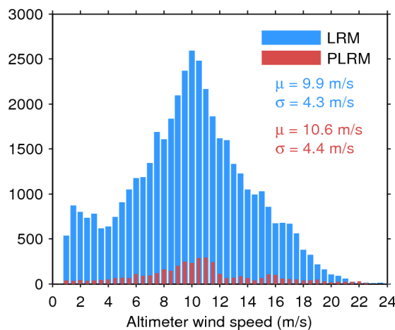
Figure 35. Histogram of science-valid wind over oceans and lakes for LRM (blue) and PLRM (red) for 02/04/2016. The mean ( \mu ) and standard deviation ( \sigma ) are also shown. Note that values larger than 24 m/s are excluded from the histogram for the sake of readability but not from the computation of \mu and \sigma .
