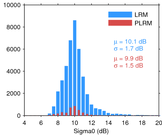
Figure 28. Histogram of science-valid sigma0 over oceans and lakes for LRM (blue) and PLRM (red) for 02/04/2016. The mean ( \mu ) and standard deviation ( \sigma ) are also shown. Note that values outside [4 20] dB are excluded from the histogram for the sake of readability but not from the computation of \mu and \sigma .
