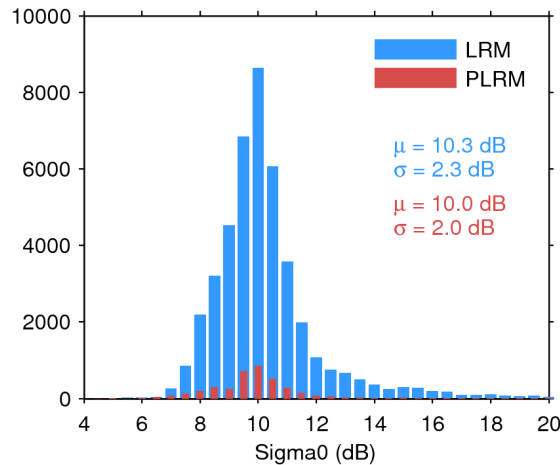
Figure 25. Histogram of flag-valid sigma0 over oceans and lakes for LRM (blue) and PLRM (red) for 02/04/2016. The mean ( \mu ) and standard deviation ( \sigma ) are also shown. Note that values outside [4 20] dB are excluded from the histogram for the sake of readability but not from the computation of \mu and \sigma .
