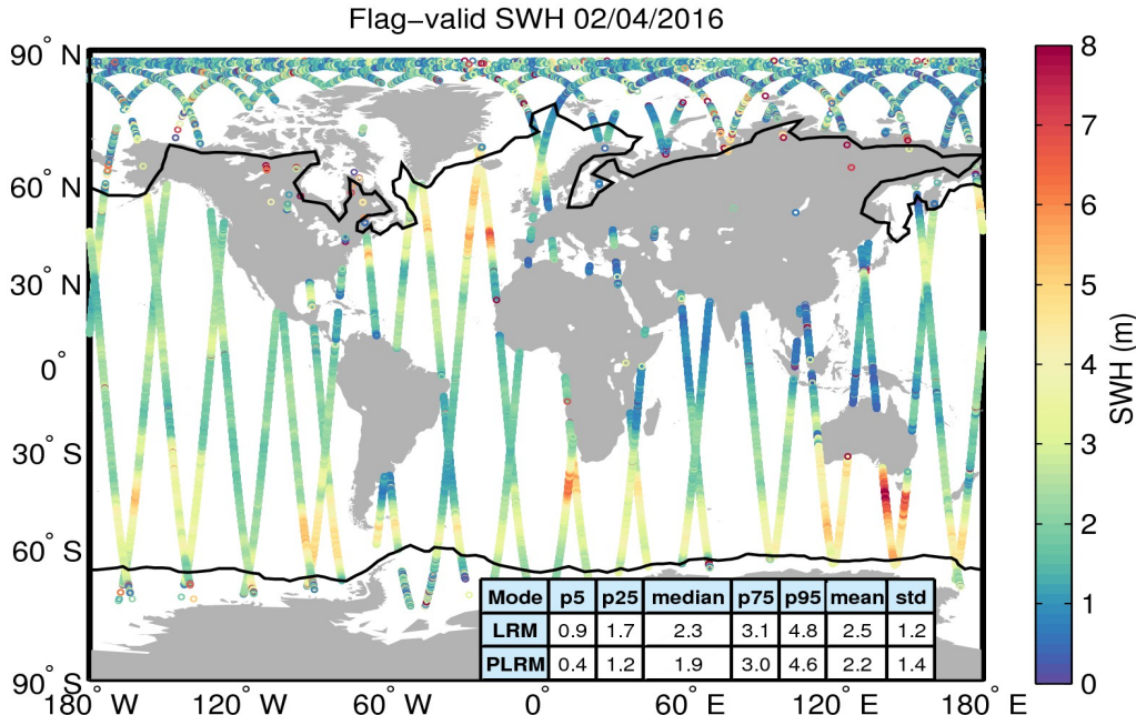
Figure 15. Geographical distribution of flag-valid SWH data over oceans and lakes for 02/04/2016. The statistical values shown in the table refer to the SWH in m and are calculated separately for LRM and PLRM regions. Measurements taken over polar polygons have been excluded from the computation of the statistical values. The black lines mark the outer limit of the Arctic and Antarctic polar polygons.
