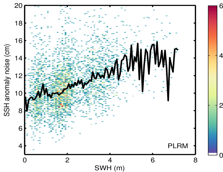
Figure 9. 2D histogram showing flag-valid SSH anomaly noise as a function of SWH for LRM (top) and PLRM (bottom) for 02/04/2016. The black line denotes the median SSH anomaly noise as a function of SWH.
