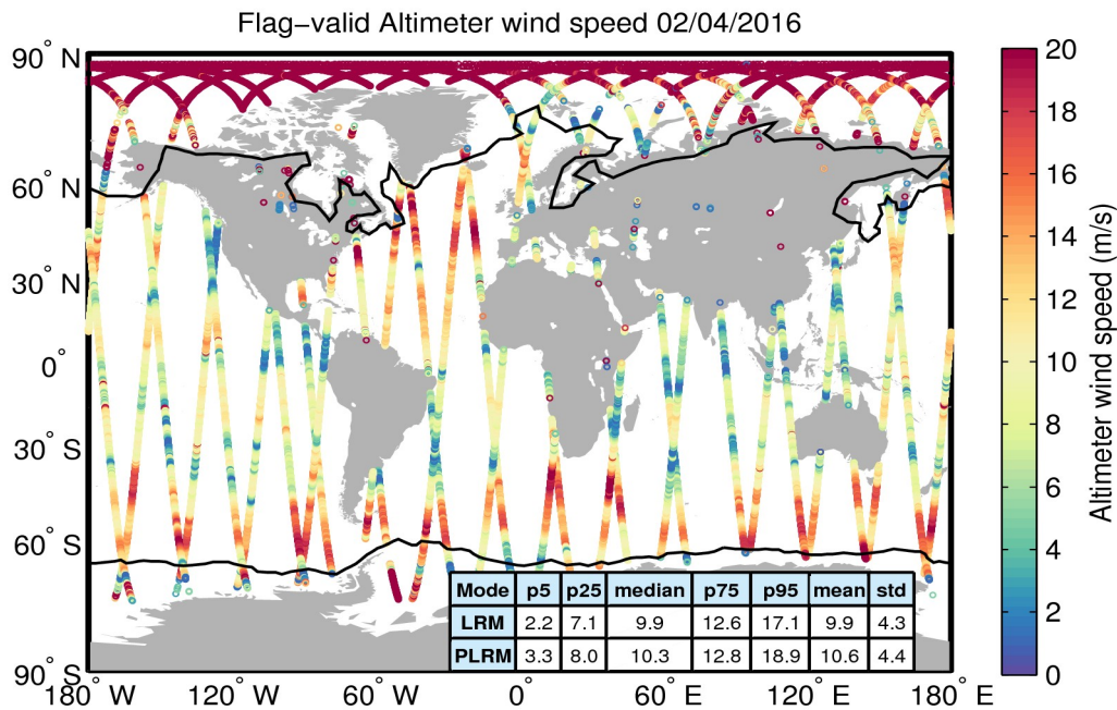
Figure 31. Geographical distribution of flag-valid wind data over oceans and lakes for 02/04/2016. The statistical values shown in the table refer to the wind in m/s and are calculated separately for LRM and PLRM regions. Measurements taken over polar polygons have been excluded from the computation of the statistical values. The black lines mark the outer limit of the Arctic and Antarctic polar polygons.
