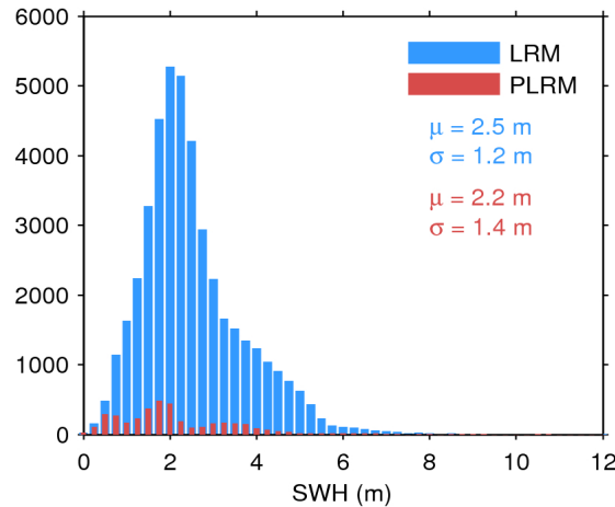
Figure 17. Histogram of flag-valid SWH over oceans and lakes for LRM (blue) and PLRM (red) for 02/04/2016. The mean ( \mu ) and standard deviation ( \sigma ) are also shown. Note that values larger than 12 m are excluded from the histogram for the sake of readability but not from the computation of \mu and \sigma .
