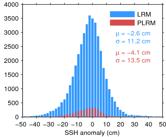
Figure 11. Histogram of science-valid SSH anomaly over oceans and lakes for LRM (blue) and PLRM (red) for 02/04/2016. The mean ( \mu ) and standard deviation ( \sigma ) are also shown. Note that values outside [-50 50] cm are excluded from the histogram for the sake of readability but not from the computation of \mu and \sigma .
