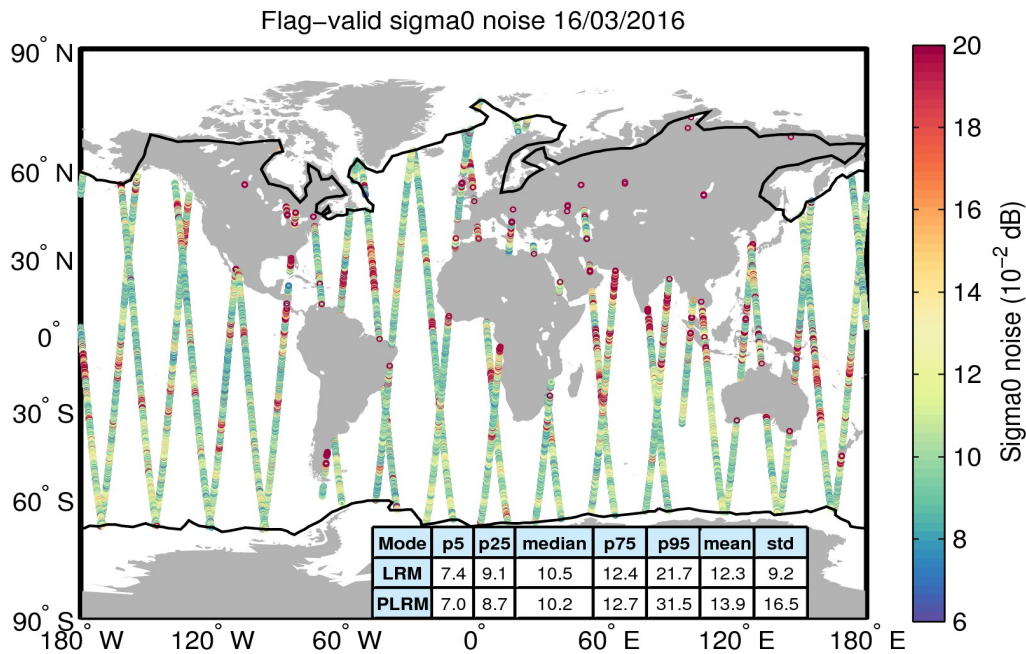
Figure 26. Geographical distribution of flag-valid 20-Hz sigma0 measurement noise over oceans and lakes for 16/03/2016. The statistical values shown in the table refer to the sigma0 noise and are calculated separately for LRM and PLRM regions. Measurements taken over polar polygons have been excluded from the computation of the statistical values. The black lines mark the outer limit of the Arctic and Antarctic polar polygons.
