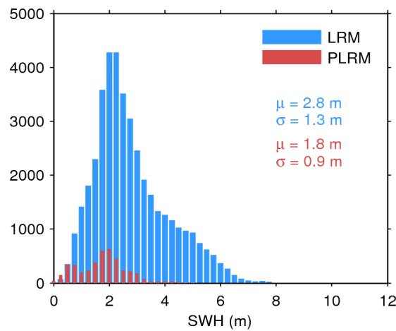
Figure 20. Histogram of science-valid SWH over oceans and lakes for LRM (blue) and PLRM (red) for 16/03/2016. The mean ( \mu ) and standard deviation ( \sigma ) are also shown. Note that values larger than 12 m are excluded from the histogram for the sake of readability but not from the computation of \mu and \sigma .
