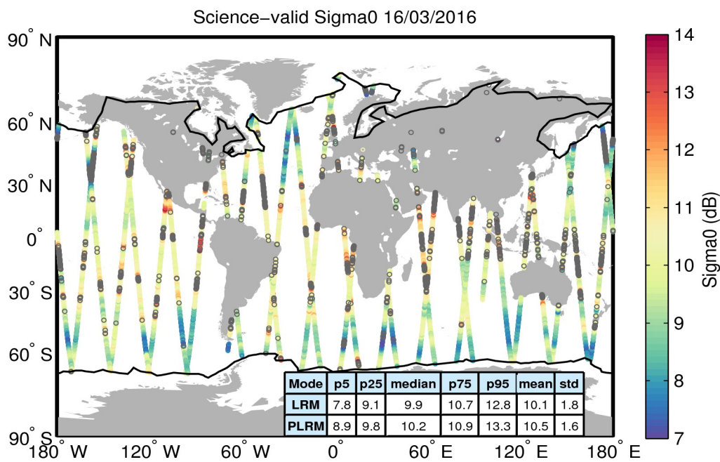
Figure 27. Geographical distribution of science-valid sigma0 data over oceans and lakes for 16/03/2016. The statistical values shown in the table refer to the sigma0 in dB and are calculated separately for LRM and PLRM regions. The black lines mark the outer limit of the Arctic and Antarctic polar polygons. Gray circles denote records that have been rejected based on the editing criteria described in Table 4.
