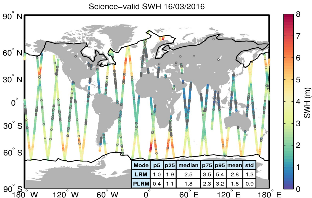
Figure 19. Geographical distribution of science-valid SWH data over oceans and lakes for 16/03/2016. The statistical values shown in the table refer to the SWH in m and are calculated separately for LRM and PLRM regions. The black lines mark the outer limit of the Arctic and Antarctic polar polygons. Gray circles denote records that have been rejected based on the editing criteria described in Table 3.
