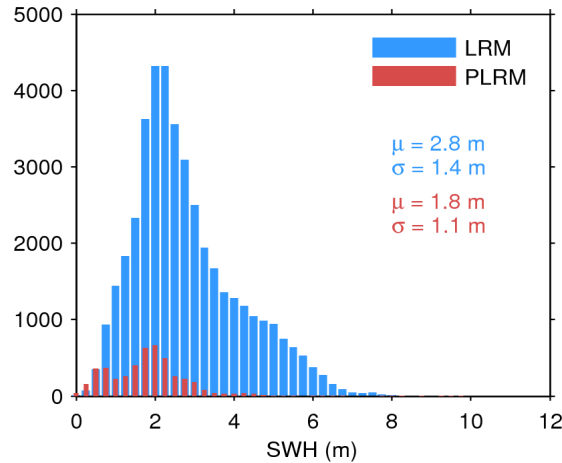
Figure 17. Histogram of flag-valid SWH over oceans and lakes for LRM (blue) and PLRM (red) for 16/03/2016. The mean ( \mu ) and standard deviation ( \sigma ) are also shown. Note that values larger than 12 m are excluded from the histogram for the sake of readability but not from the computation of \mu and \sigma .
