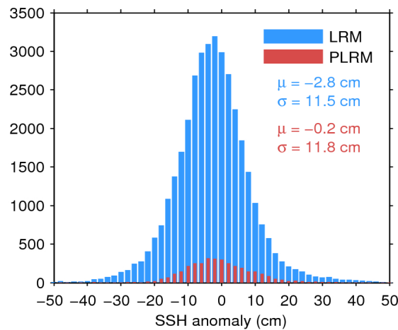
Figure 11. Histogram of science-valid SSH anomaly over oceans and lakes for LRM (blue) and PLRM (red) for 16/03/2016. The mean ( \mu ) and standard deviation ( \sigma ) are also shown. Note that values outside [-50 50] cm are excluded from the histogram for the sake of readability but not from the computation of \mu and \sigma .
