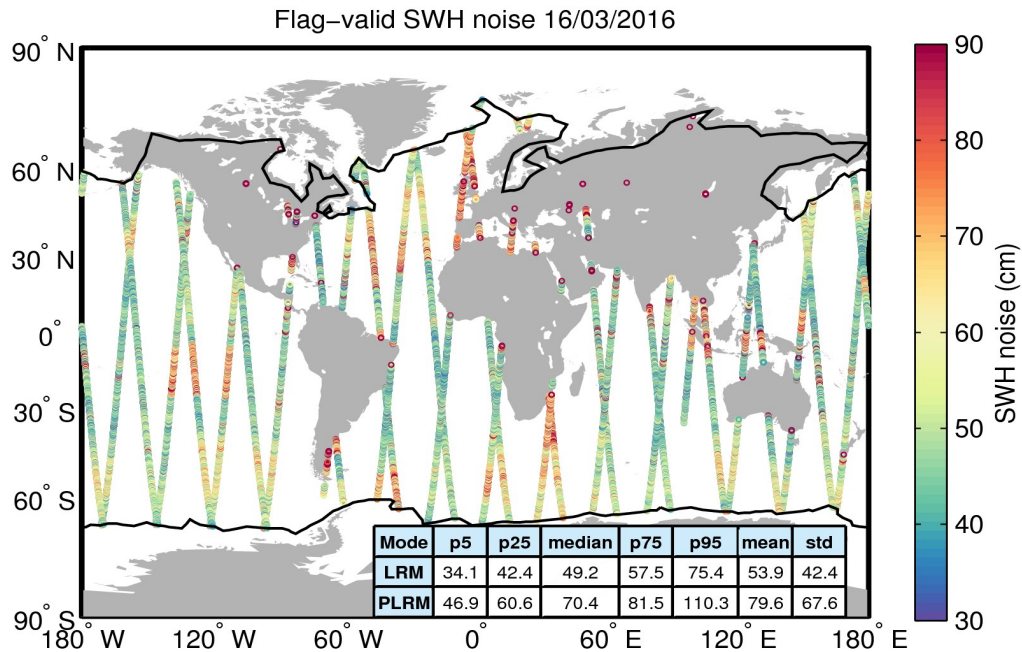
Figure 18. Geographical distribution of flag-valid 20-Hz SWH measurement noise over oceans and lakes for 16/03/2016. The statistical values shown in the table refer to the SWH noise and are calculated separately for LRM and PLRM regions. Measurements taken over polar polygons have been excluded from the computation of the statistical values. The black lines mark the outer limit of the Arctic and Antarctic polar polygons.
