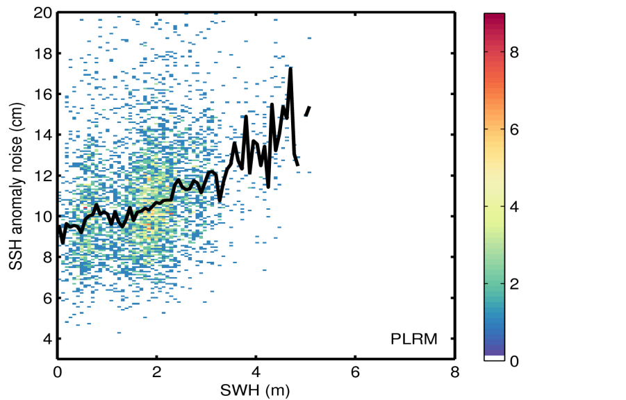
Figure 9. 2D histogram showing flag-valid SSH anomaly noise as a function of SWH for LRM (top) and PLRM (bottom) for 16/03/2016. The black line denotes the median SSH anomaly noise as a function of SWH.
