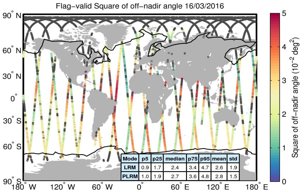
Figure 37. Geographical distribution of flag-valid mispointing data over oceans and lakes for 16/03/2016. The statistical values shown in the table refer to the mispointing in 10^{-2} deg 2 and are calculated separately for LRM and PLRM regions. Measurements taken over polar polygons have been excluded from the computation of the statistical values. The black lines mark the outer limit of the Arctic and Antarctic polar polygons. Gray circles denote negative values.
