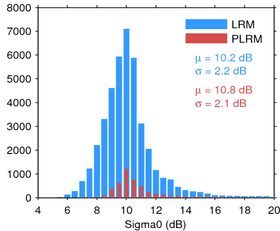
Figure 25. Histogram of flag-valid sigma0 over oceans and lakes for LRM (blue) and PLRM (red) for 16/03/2016. The mean ( \mu ) and standard deviation ( \sigma ) are also shown. Note that values outside [4 20] dB are excluded from the histogram for the sake of readability but not from the computation of \mu and \sigma .
