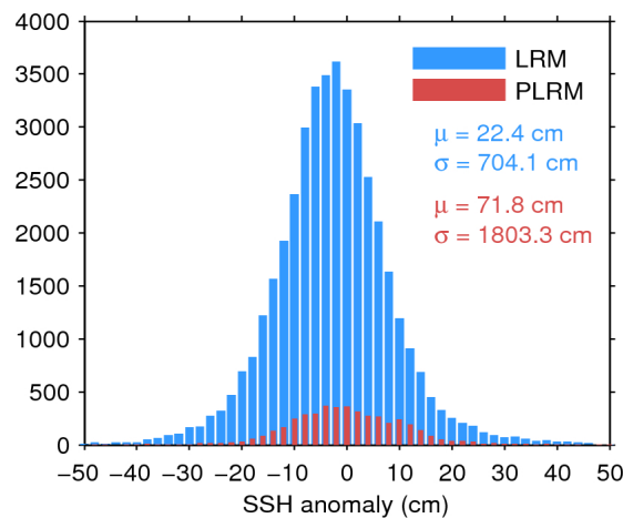
Figure 7. Histogram of flag-valid SSH anomaly over oceans and lakes for LRM (blue) and PLRM (red) for 16/03/2016. The mean ( \mu ) and standard deviation ( \sigma ) are also shown. Note that values outside [-50 50] cm are excluded from the histogram for the sake of readability but not from the computation of \mu and \sigma .
