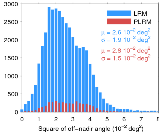
Figure 39. Histogram of flag-valid mispointing over oceans and lakes for LRM (blue) and PLRM (red) for 16/03/2016. Only positive values have been considered. The mean ( \mu ) and standard deviation ( \sigma ) are also shown. Note that values larger than 8 \cdot 10^{-2} \text{ deg}^2 are excluded from the histogram for the sake of readability but not from the computation of \mu and \sigma .
