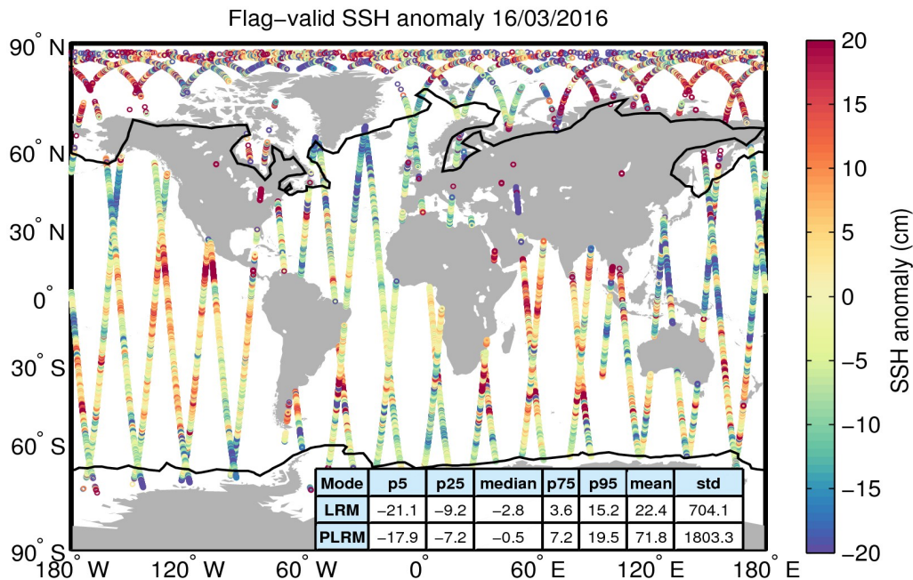
Figure 5. Geographical distribution of flag-valid 1-Hz SSH anomaly data over oceans and lakes for 16/03/2016. The statistical values shown in the table refer to the SSH anomaly in cm and are calculated separately for LRM and PLRM regions. Measurements taken over polar polygons have been excluded from the computation of the statistical values. The black lines mark the outer limit of the Arctic and Antarctic polar polygons.
