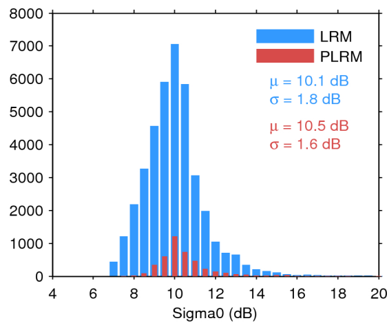
Figure 28. Histogram of science-valid sigma0 over oceans and lakes for LRM (blue) and PLRM (red) for 16/03/2016. The mean ( \mu ) and standard deviation ( \sigma ) are also shown. Note that values outside [4 20] dB are excluded from the histogram for the sake of readability but not from the computation of \mu and \sigma .
