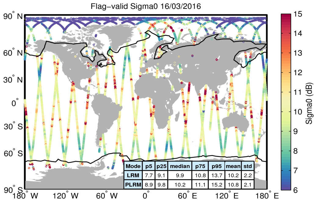
Figure 23. Geographical distribution of flag-valid sigma0 data over oceans and lakes for 16/03/2016. The statistical values shown in the table refer to the sigma0 in dB and are calculated separately for LRM and PLRM regions. Measurements taken over polar polygons have been excluded from the computation of the statistical values. The black lines mark the outer limit of the Arctic and Antarctic polar polygons.
