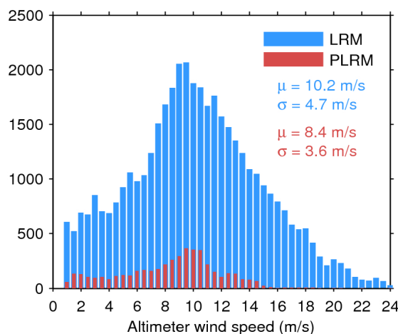
Figure 35. Histogram of science-valid wind over oceans and lakes for LRM (blue) and PLRM (red) for 16/03/2016. The mean ( \mu ) and standard deviation ( \sigma ) are also shown. Note that values larger than 24 m/s are excluded from the histogram for the sake of readability but not from the computation of \mu and \sigma .
