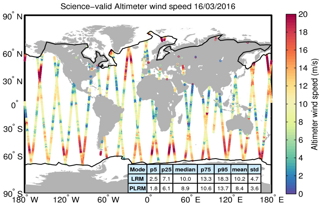
Figure 34. Geographical distribution of science-valid wind data over oceans and lakes for 16/03/2016. The statistical values shown in the table refer to the wind in m/s and are calculated separately for LRM and PLRM regions. The black lines mark the outer limit of the Arctic and Antarctic polar polygons. Gray circles denote records that have been rejected based on the editing criteria described in Table 5.
