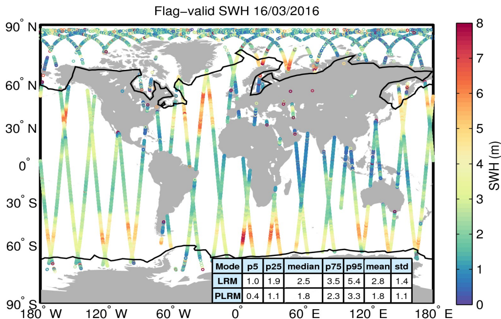
Figure 15. Geographical distribution of flag-valid SWH data over oceans and lakes for 16/03/2016. The statistical values shown in the table refer to the SWH in m and are calculated separately for LRM and PLRM regions. Measurements taken over polar polygons have been excluded from the computation of the statistical values. The black lines mark the outer limit of the Arctic and Antarctic polar polygons.
