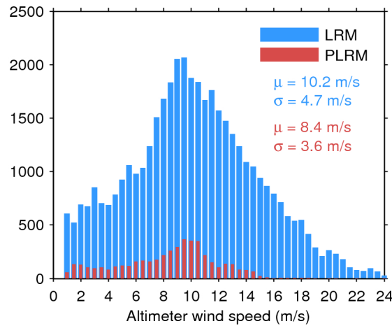
Figure 33. Histogram of flag-valid wind over oceans and lakes for LRM (blue) and PLRM (red) for 16/03/2016. The mean ( \mu ) and standard deviation ( \sigma ) are also shown. Note that values larger than 24 m/s are excluded from the histogram for the sake of readability but not from the computation of \mu and \sigma .
