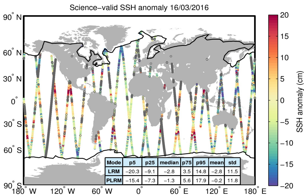
Figure 10. Geographical distribution of science-valid SSH anomaly data over oceans and lakes for 16/03/2016. The statistical values shown in the table refer to the SSH anomaly in cm and are calculated separately for LRM and PLRM regions. The black lines mark the outer limit of the Arctic and Antarctic polar polygons. Gray circles denote records that have been rejected based on the editing criteria described in Table 2.
