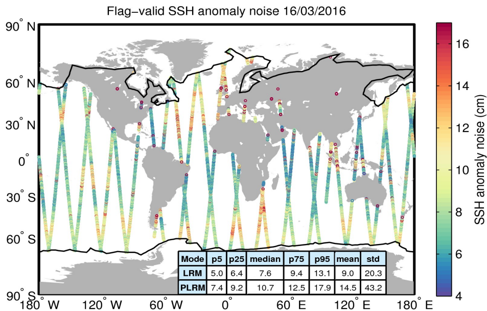
Figure 8. Geographical distribution of flag-valid 20-Hz SSH anomaly measurement noise over oceans and lakes for 16/03/2016. The statistical values shown in the table refer to the SSH anomaly noise and are calculated separately for LRM and PLRM regions. Measurements taken over polar polygons have been excluded from the computation of the statistical values. The black lines mark the outer limit of the Arctic and Antarctic polar polygons.
