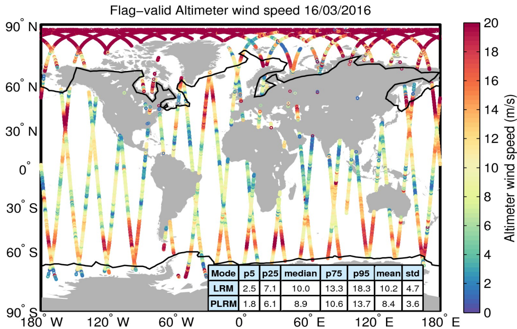
Figure 31. Geographical distribution of flag-valid wind data over oceans and lakes for 16/03/2016. The statistical values shown in the table refer to the wind in m/s and are calculated separately for LRM and PLRM regions. Measurements taken over polar polygons have been excluded from the computation of the statistical values. The black lines mark the outer limit of the Arctic and Antarctic polar polygons.
