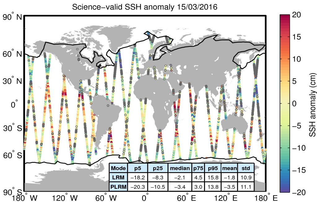
Figure 10. Geographical distribution of science-valid SSH anomaly data over oceans and lakes for 15/03/2016. The statistical values shown in the table refer to the SSH anomaly in cm and are calculated separately for LRM and PLRM regions. The black lines mark the outer limit of the Arctic and Antarctic polar polygons. Gray circles denote records that have been rejected based on the editing criteria described in Table 2.
