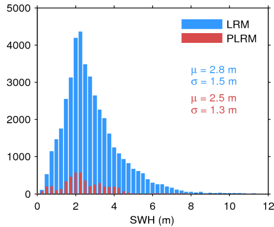
Figure 20. Histogram of science-valid SWH over oceans and lakes for LRM (blue) and PLRM (red) for 15/03/2016. The mean ( \mu ) and standard deviation ( \sigma ) are also shown. Note that values larger than 12 m are excluded from the histogram for the sake of readability but not from the computation of \mu and \sigma .
