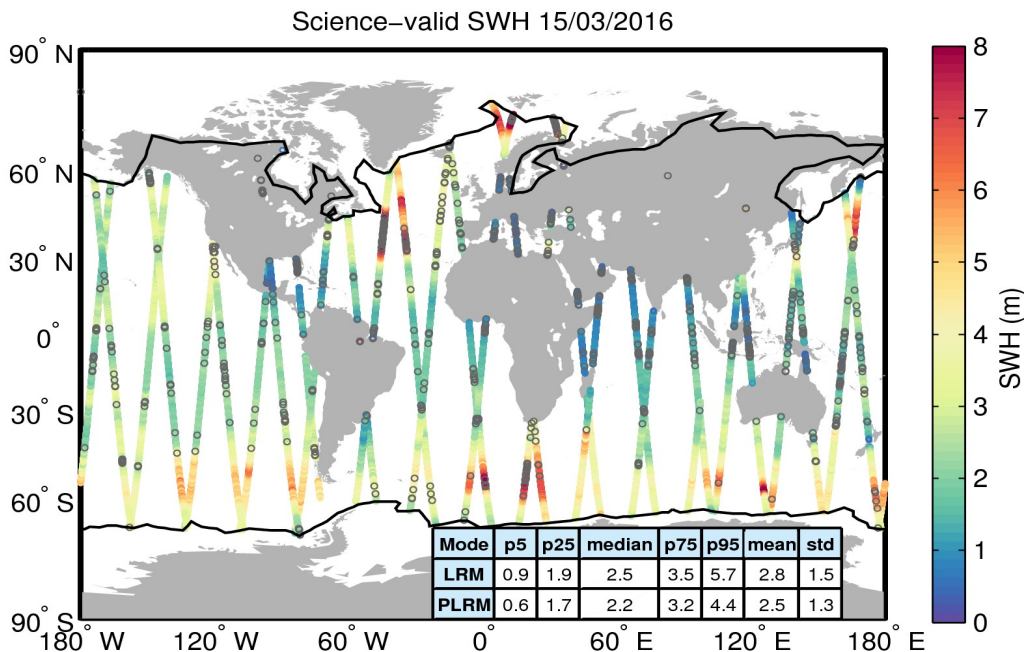
Figure 19. Geographical distribution of science-valid SWH data over oceans and lakes for 15/03/2016. The statistical values shown in the table refer to the SWH in m and are calculated separately for LRM and PLRM regions. The black lines mark the outer limit of the Arctic and Antarctic polar polygons. Gray circles denote records that have been rejected based on the editing criteria described in Table 3.
