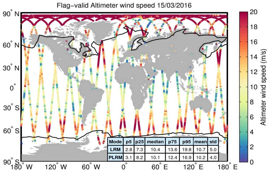
Figure 31. Geographical distribution of flag-valid wind data over oceans and lakes for 15/03/2016. The statistical values shown in the table refer to the wind in m/s and are calculated separately for LRM and PLRM regions. Measurements taken over polar polygons have been excluded from the computation of the statistical values. The black lines mark the outer limit of the Arctic and Antarctic polar polygons.
