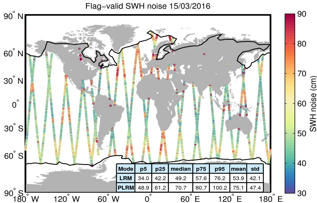
Figure 18. Geographical distribution of flag-valid 20-Hz SWH measurement noise over oceans and lakes for 15/03/2016. The statistical values shown in the table refer to the SWH noise and are calculated separately for LRM and PLRM regions. Measurements taken over polar polygons have been excluded from the computation of the statistical values. The black lines mark the outer limit of the Arctic and Antarctic polar polygons.
