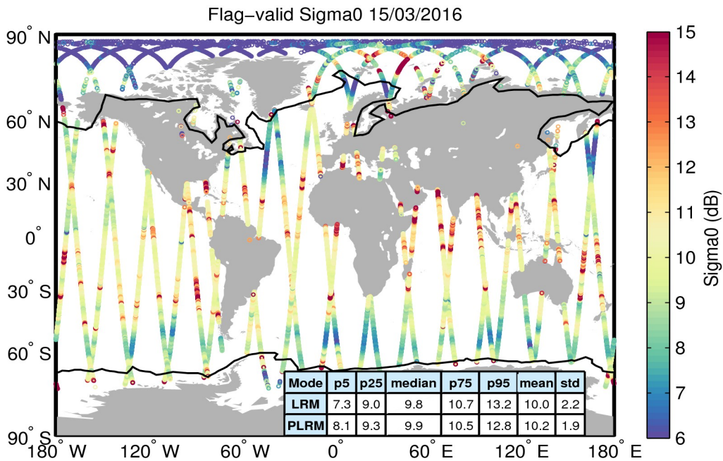
Figure 23. Geographical distribution of flag-valid sigma0 data over oceans and lakes for 15/03/2016. The statistical values shown in the table refer to the sigma0 in dB and are calculated separately for LRM and PLRM regions. Measurements taken over polar polygons have been excluded from the computation of the statistical values. The black lines mark the outer limit of the Arctic and Antarctic polar polygons.
