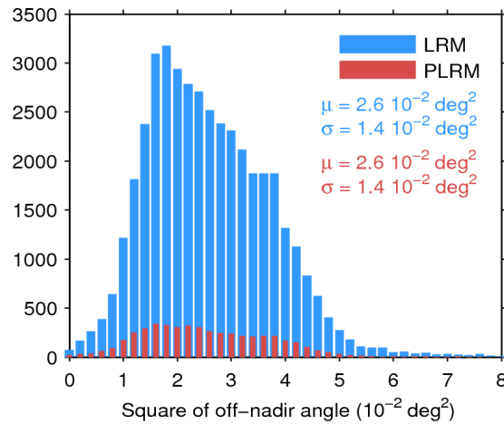
Figure 39. Histogram of flag-valid mispointing over oceans and lakes for LRM (blue) and PLRM (red) for 15/03/2016. Only positive values have been considered. The mean ( \mu ) and standard deviation ( \sigma ) are also shown. Note that values larger than 8 \cdot 10^{-2} \text{ deg}^2 are excluded from the histogram for the sake of readability but not from the computation of \mu and \sigma .
