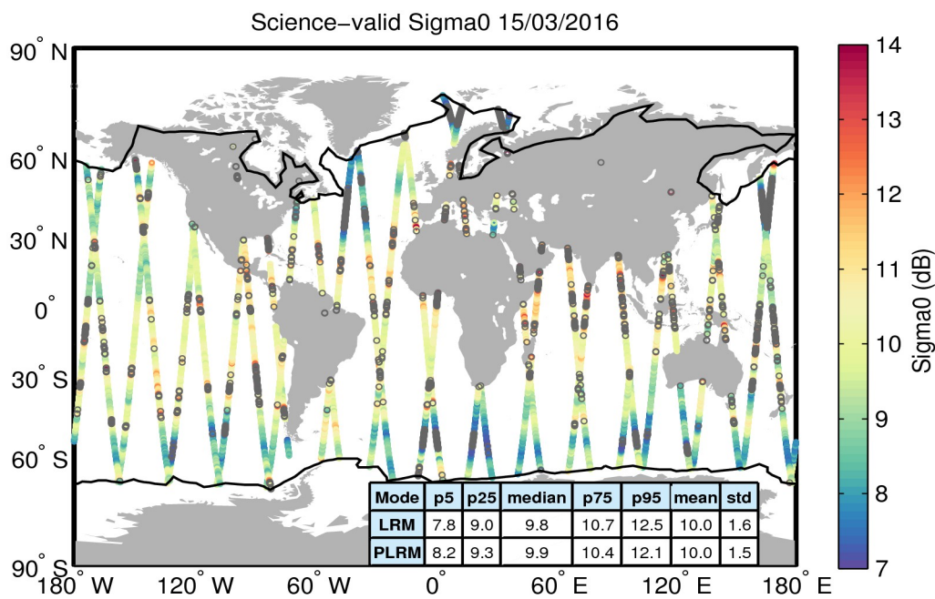
Figure 27. Geographical distribution of science-valid sigma0 data over oceans and lakes for 15/03/2016. The statistical values shown in the table refer to the sigma0 in dB and are calculated separately for LRM and PLRM regions. The black lines mark the outer limit of the Arctic and Antarctic polar polygons. Gray circles denote records that have been rejected based on the editing criteria described in Table 4.
