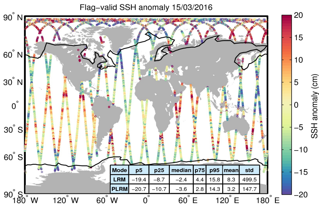
Figure 5. Geographical distribution of flag-valid 1-Hz SSH anomaly data over oceans and lakes for 15/03/2016. The statistical values shown in the table refer to the SSH anomaly in cm and are calculated separately for LRM and PLRM regions. Measurements taken over polar polygons have been excluded from the computation of the statistical values. The black lines mark the outer limit of the Arctic and Antarctic polar polygons.
