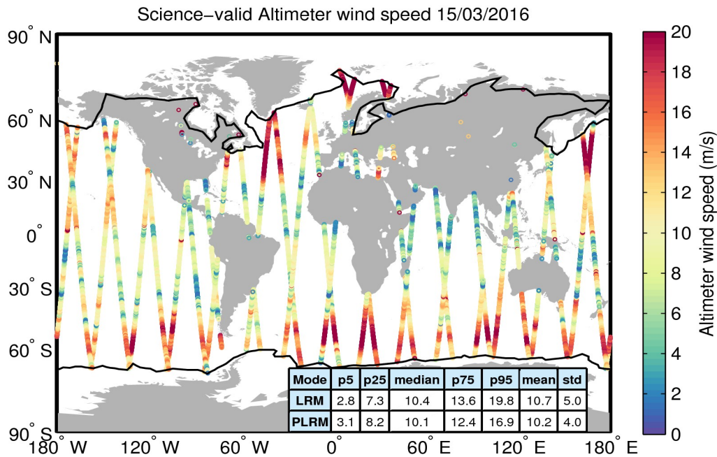
Figure 34. Geographical distribution of science-valid wind data over oceans and lakes for 15/03/2016. The statistical values shown in the table refer to the wind in m/s and are calculated separately for LRM and PLRM regions. The black lines mark the outer limit of the Arctic and Antarctic polar polygons. Gray circles denote records that have been rejected based on the editing criteria described in Table 5.
