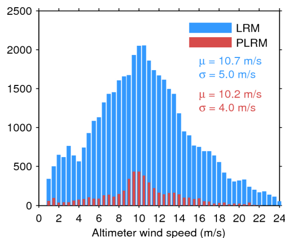
Figure 35. Histogram of science-valid wind over oceans and lakes for LRM (blue) and PLRM (red) for 15/03/2016. The mean ( \mu ) and standard deviation ( \sigma ) are also shown. Note that values larger than 24 m/s are excluded from the histogram for the sake of readability but not from the computation of \mu and \sigma .
