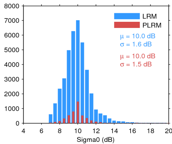
Figure 28. Histogram of science-valid sigma0 over oceans and lakes for LRM (blue) and PLRM (red) for 15/03/2016. The mean ( \mu ) and standard deviation ( \sigma ) are also shown. Note that values outside [4 20] dB are excluded from the histogram for the sake of readability but not from the computation of \mu and \sigma .
