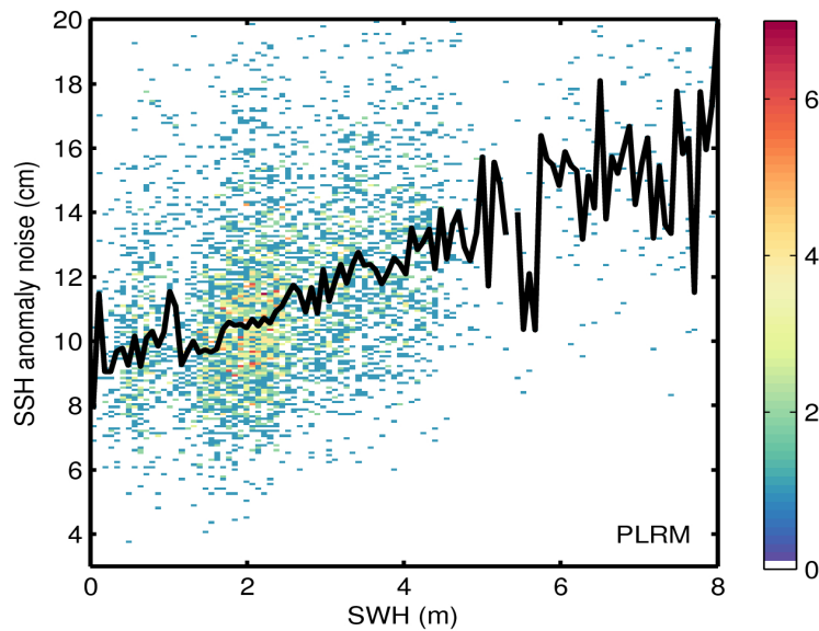
Figure 9. 2D histogram showing flag-valid SSH anomaly noise as a function of SWH for LRM (top) and PLRM (bottom) for 15/03/2016. The black line denotes the median SSH anomaly noise as a function of SWH.
