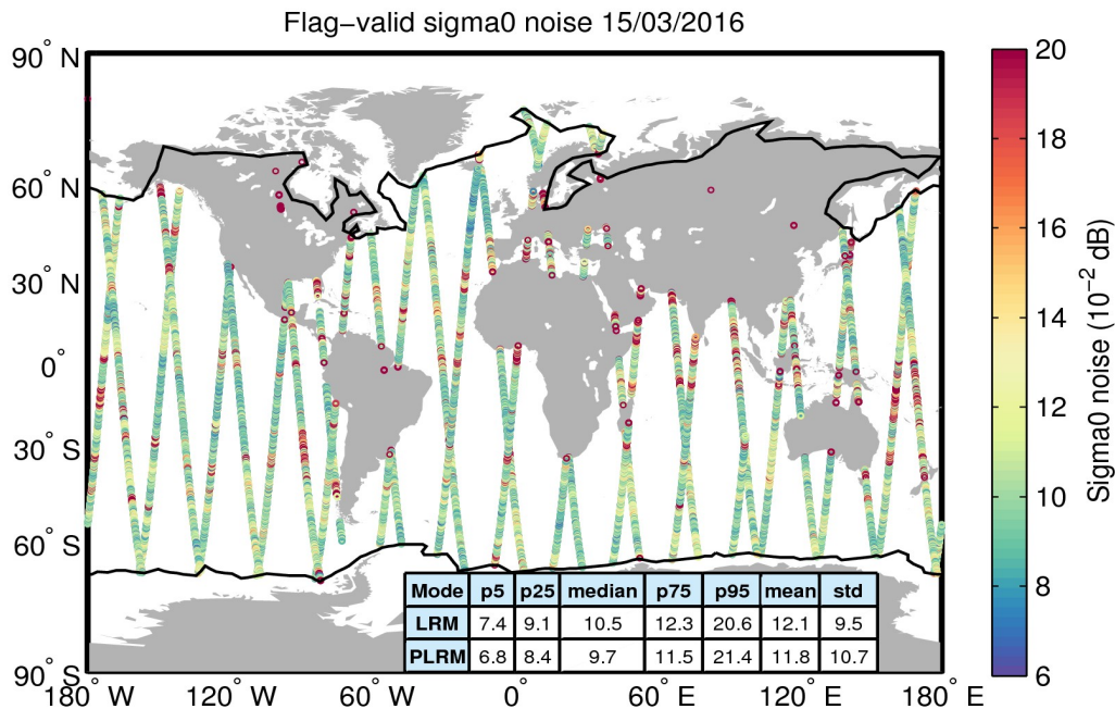
Figure 26. Geographical distribution of flag-valid 20-Hz sigma0 measurement noise over oceans and lakes for 15/03/2016. The statistical values shown in the table refer to the sigma0 noise and are calculated separately for LRM and PLRM regions. Measurements taken over polar polygons have been excluded from the computation of the statistical values. The black lines mark the outer limit of the Arctic and Antarctic polar polygons.
