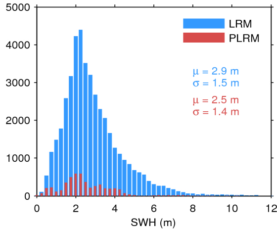
Figure 17. Histogram of flag-valid SWH over oceans and lakes for LRM (blue) and PLRM (red) for 15/03/2016. The mean ( \mu ) and standard deviation ( \sigma ) are also shown. Note that values larger than 12 m are excluded from the histogram for the sake of readability but not from the computation of \mu and \sigma .
