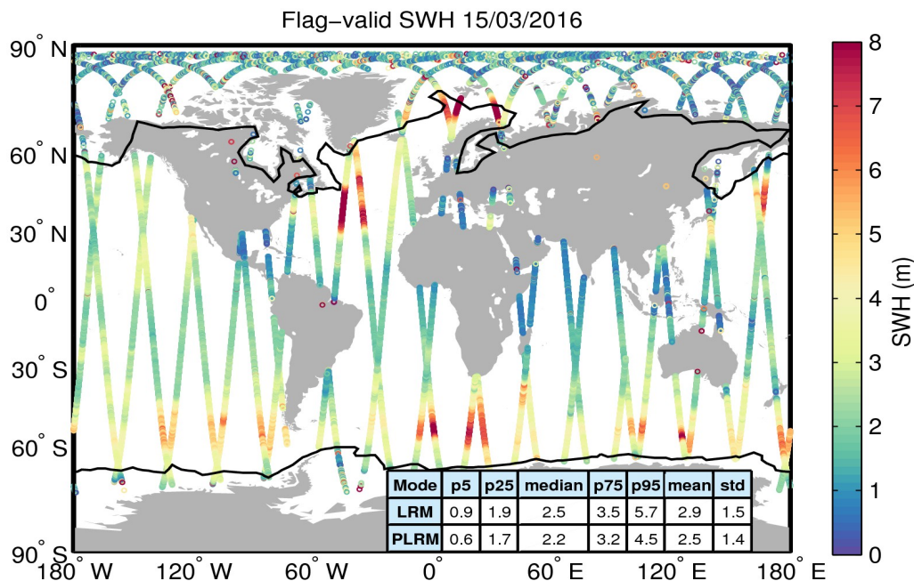
Figure 15. Geographical distribution of flag-valid SWH data over oceans and lakes for 15/03/2016. The statistical values shown in the table refer to the SWH in m and are calculated separately for LRM and PLRM regions. Measurements taken over polar polygons have been excluded from the computation of the statistical values. The black lines mark the outer limit of the Arctic and Antarctic polar polygons.
