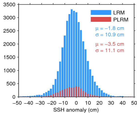
Figure 11. Histogram of science-valid SSH anomaly over oceans and lakes for LRM (blue) and PLRM (red) for 15/03/2016. The mean ( \mu ) and standard deviation ( \sigma ) are also shown. Note that values outside [-50 50] cm are excluded from the histogram for the sake of readability but not from the computation of \mu and \sigma .
