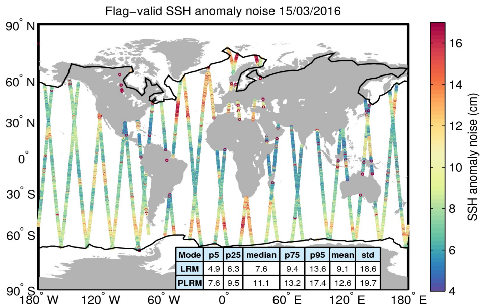
Figure 8. Geographical distribution of flag-valid 20-Hz SSH anomaly measurement noise over oceans and lakes for 15/03/2016. The statistical values shown in the table refer to the SSH anomaly noise and are calculated separately for LRM and PLRM regions. Measurements taken over polar polygons have been excluded from the computation of the statistical values. The black lines mark the outer limit of the Arctic and Antarctic polar polygons.
