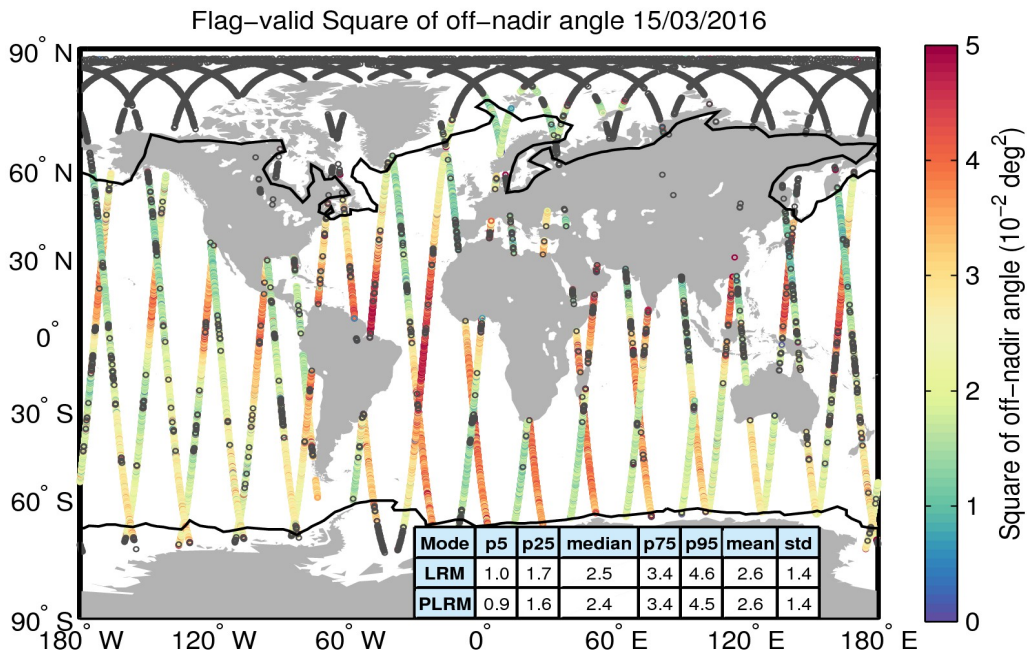
Figure 37. Geographical distribution of flag-valid mispointing data over oceans and lakes for 15/03/2016. The statistical values shown in the table refer to the mispointing in 10^{-2} deg 2 and are calculated separately for LRM and PLRM regions. Measurements taken over polar polygons have been excluded from the computation of the statistical values. The black lines mark the outer limit of the Arctic and Antarctic polar polygons. Gray circles denote negative values.
