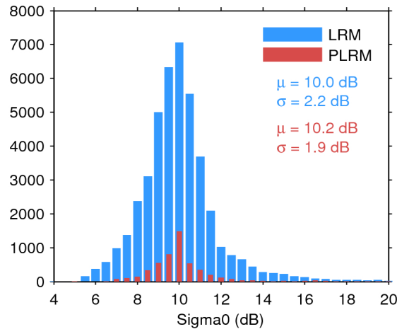
Figure 25. Histogram of flag-valid sigma0 over oceans and lakes for LRM (blue) and PLRM (red) for 15/03/2016. The mean ( \mu ) and standard deviation ( \sigma ) are also shown. Note that values outside [4 20] dB are excluded from the histogram for the sake of readability but not from the computation of \mu and \sigma .
