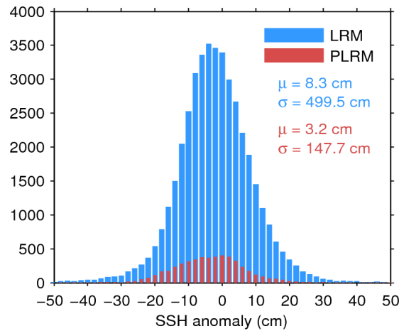
Figure 7. Histogram of flag-valid SSH anomaly over oceans and lakes for LRM (blue) and PLRM (red) for 15/03/2016. The mean ( \mu ) and standard deviation ( \sigma ) are also shown. Note that values outside [-50\ 50] cm are excluded from the histogram for the sake of readability but not from the computation of \mu and \sigma .
