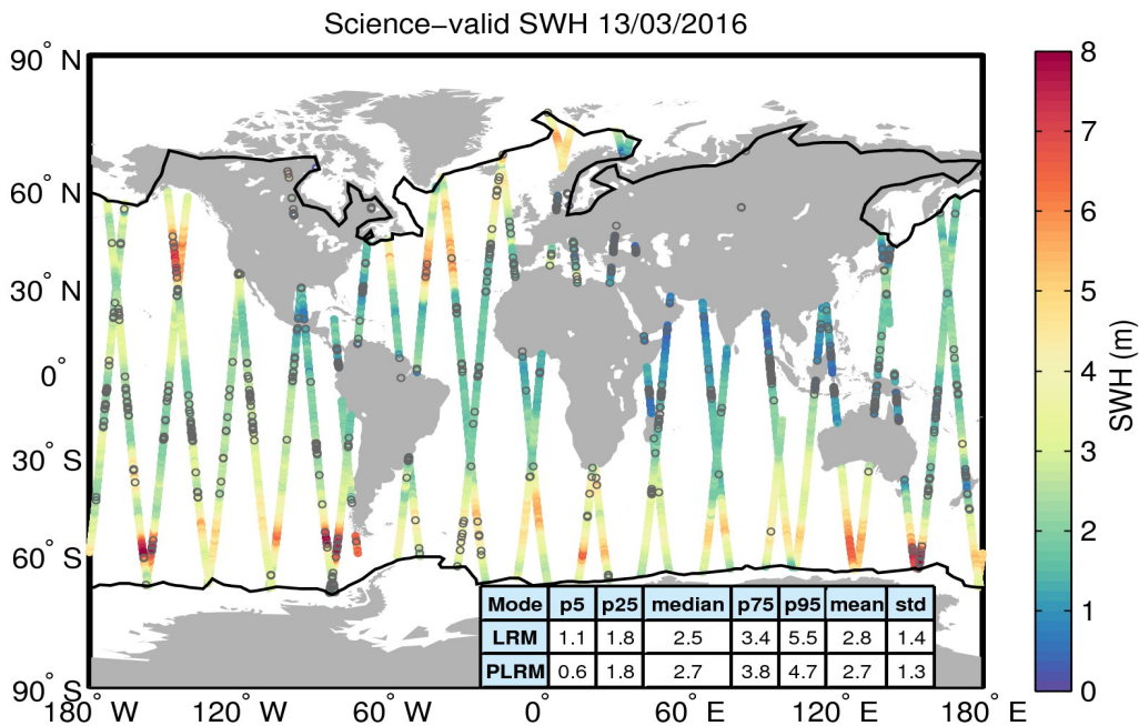
Figure 19. Geographical distribution of science-valid SWH data over oceans and lakes for 13/03/2016. The statistical values shown in the table refer to the SWH in m and are calculated separately for LRM and PLRM regions. The black lines mark the outer limit of the Arctic and Antarctic polar polygons. Gray circles denote records that have been rejected based on the editing criteria described in Table 3.
