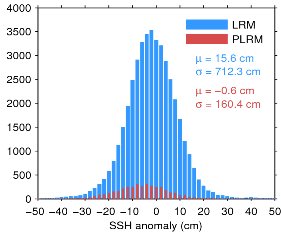
Figure 7. Histogram of flag-valid SSH anomaly over oceans and lakes for LRM (blue) and PLRM (red) for 13/03/2016. The mean ( \mu ) and standard deviation ( \sigma ) are also shown. Note that values outside [-50\ 50] cm are excluded from the histogram for the sake of readability but not from the computation of \mu and \sigma .
