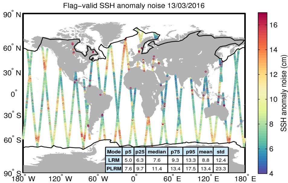
Figure 8. Geographical distribution of flag-valid 20-Hz SSH anomaly measurement noise over oceans and lakes for 13/03/2016. The statistical values shown in the table refer to the SSH anomaly noise and are calculated separately for LRM and PLRM regions. Measurements taken over polar polygons have been excluded from the computation of the statistical values. The black lines mark the outer limit of the Arctic and Antarctic polar polygons.
