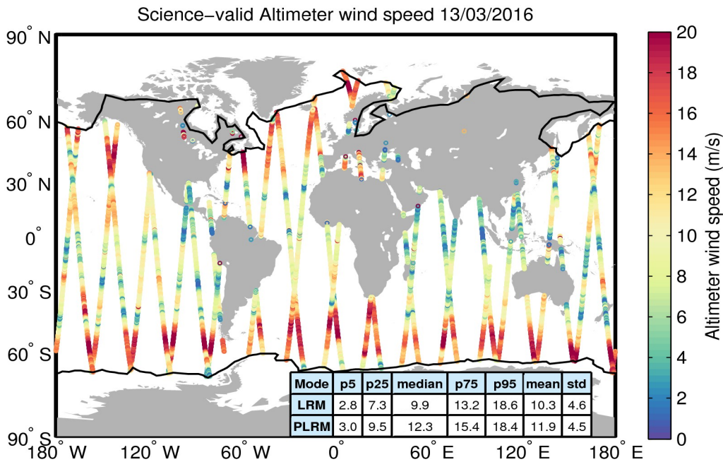
Figure 34. Geographical distribution of science-valid wind data over oceans and lakes for 13/03/2016. The statistical values shown in the table refer to the wind in m/s and are calculated separately for LRM and PLRM regions. The black lines mark the outer limit of the Arctic and Antarctic polar polygons. Gray circles denote records that have been rejected based on the editing criteria described in Table 5.
