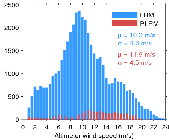
Figure 33. Histogram of flag-valid wind over oceans and lakes for LRM (blue) and PLRM (red) for 13/03/2016. The mean ( \mu ) and standard deviation ( \sigma ) are also shown. Note that values larger than 24 m/s are excluded from the histogram for the sake of readability but not from the computation of \mu and \sigma .
