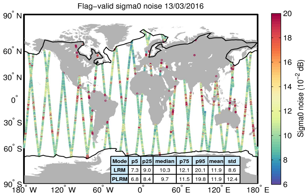
Figure 26. Geographical distribution of flag-valid 20-Hz sigma0 measurement noise over oceans and lakes for 13/03/2016. The statistical values shown in the table refer to the sigma0 noise and are calculated separately for LRM and PLRM regions. Measurements taken over polar polygons have been excluded from the computation of the statistical values. The black lines mark the outer limit of the Arctic and Antarctic polar polygons.
