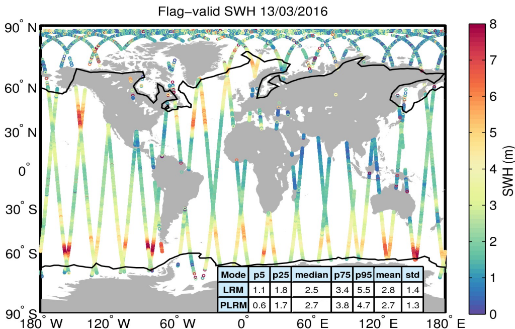
Figure 15. Geographical distribution of flag-valid SWH data over oceans and lakes for 13/03/2016. The statistical values shown in the table refer to the SWH in m and are calculated separately for LRM and PLRM regions. Measurements taken over polar polygons have been excluded from the computation of the statistical values. The black lines mark the outer limit of the Arctic and Antarctic polar polygons.
