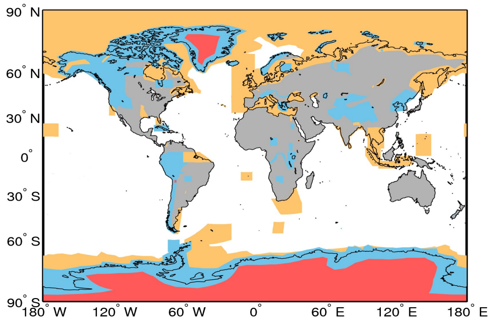
Figure A1. Extent of the regions defining the geographical mode mask for 13/03/2016. The regions where SAR, and SARIn are operated are denoted by the orange and blue polygons, respectively. LRM is operated over areas of the continental ice sheets (red polygons) and over oceans and land not covered by other modes.
