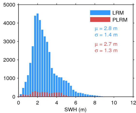
Figure 20. Histogram of science-valid SWH over oceans and lakes for LRM (blue) and PLRM (red) for 13/03/2016. The mean ( \mu ) and standard deviation ( \sigma ) are also shown. Note that values larger than 12 m are excluded from the histogram for the sake of readability but not from the computation of \mu and \sigma .
