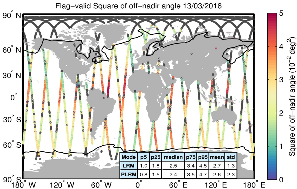
Figure 37. Geographical distribution of flag-valid mispointing data over oceans and lakes for 13/03/2016. The statistical values shown in the table refer to the mispointing in 10^{-2} deg 2 and are calculated separately for LRM and PLRM regions. Measurements taken over polar polygons have been excluded from the computation of the statistical values. The black lines mark the outer limit of the Arctic and Antarctic polar polygons. Gray circles denote negative values.
