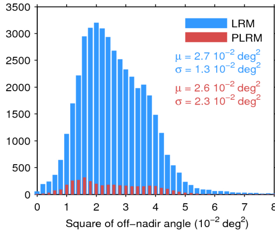
Figure 39. Histogram of flag-valid mispointing over oceans and lakes for LRM (blue) and PLRM (red) for 13/03/2016. Only positive values have been considered. The mean ( \mu ) and standard deviation ( \sigma ) are also shown. Note that values larger than 8 \cdot 10^{-2} \text{ deg}^2 are excluded from the histogram for the sake of readability but not from the computation of \mu and \sigma .
