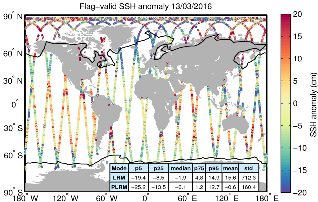
Figure 5. Geographical distribution of flag-valid 1-Hz SSH anomaly data over oceans and lakes for 13/03/2016. The statistical values shown in the table refer to the SSH anomaly in cm and are calculated separately for LRM and PLRM regions. Measurements taken over polar polygons have been excluded from the computation of the statistical values. The black lines mark the outer limit of the Arctic and Antarctic polar polygons.
