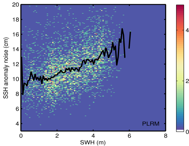
Figure 9. 2D histogram showing flag-valid SSH anomaly noise as a function of SWH for LRM (top) and PLRM (bottom) for 13/03/2016. The black line denotes the median SSH anomaly noise as a function of SWH.
