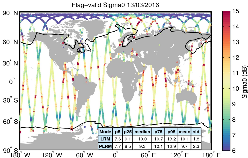
Figure 23. Geographical distribution of flag-valid sigma0 data over oceans and lakes for 13/03/2016. The statistical values shown in the table refer to the sigma0 in dB and are calculated separately for LRM and PLRM regions. Measurements taken over polar polygons have been excluded from the computation of the statistical values. The black lines mark the outer limit of the Arctic and Antarctic polar polygons.
