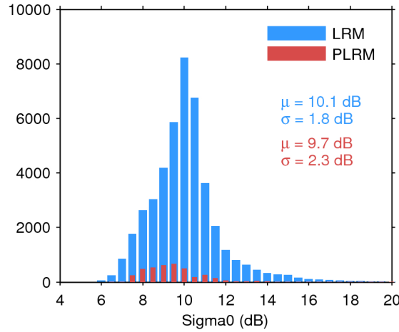
Figure 25. Histogram of flag-valid sigma0 over oceans and lakes for LRM (blue) and PLRM (red) for 13/03/2016. The mean ( \mu ) and standard deviation ( \sigma ) are also shown. Note that values outside [4 20] dB are excluded from the histogram for the sake of readability but not from the computation of \mu and \sigma .
