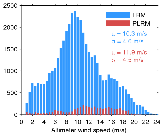
Figure 35. Histogram of science-valid wind over oceans and lakes for LRM (blue) and PLRM (red) for 13/03/2016. The mean ( \mu ) and standard deviation ( \sigma ) are also shown. Note that values larger than 24 m/s are excluded from the histogram for the sake of readability but not from the computation of \mu and \sigma .
