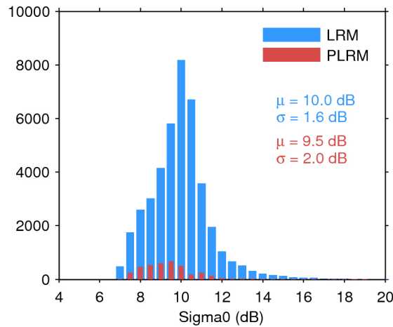
Figure 28. Histogram of science-valid sigma0 over oceans and lakes for LRM (blue) and PLRM (red) for 13/03/2016. The mean ( \mu ) and standard deviation ( \sigma ) are also shown. Note that values outside [4 20] dB are excluded from the histogram for the sake of readability but not from the computation of \mu and \sigma .
