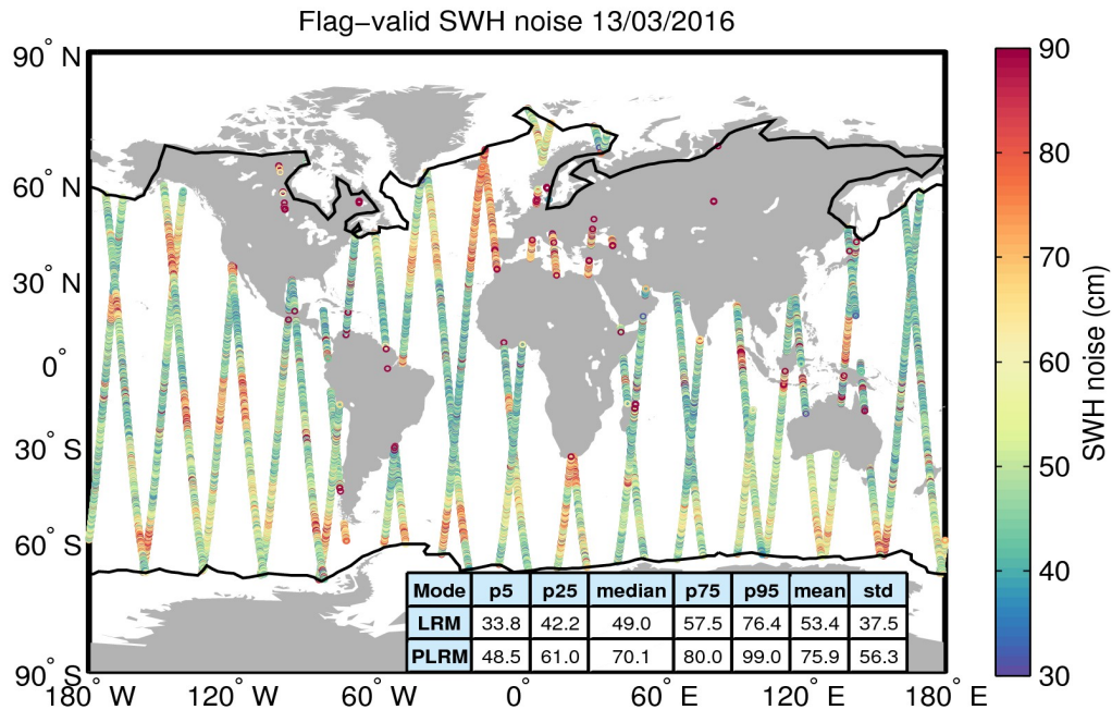
Figure 18. Geographical distribution of flag-valid 20-Hz SWH measurement noise over oceans and lakes for 13/03/2016. The statistical values shown in the table refer to the SWH noise and are calculated separately for LRM and PLRM regions. Measurements taken over polar polygons have been excluded from the computation of the statistical values. The black lines mark the outer limit of the Arctic and Antarctic polar polygons.
