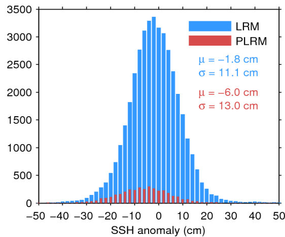
Figure 11. Histogram of science-valid SSH anomaly over oceans and lakes for LRM (blue) and PLRM (red) for 13/03/2016. The mean ( \mu ) and standard deviation ( \sigma ) are also shown. Note that values outside [-50 50] cm are excluded from the histogram for the sake of readability but not from the computation of \mu and \sigma .
