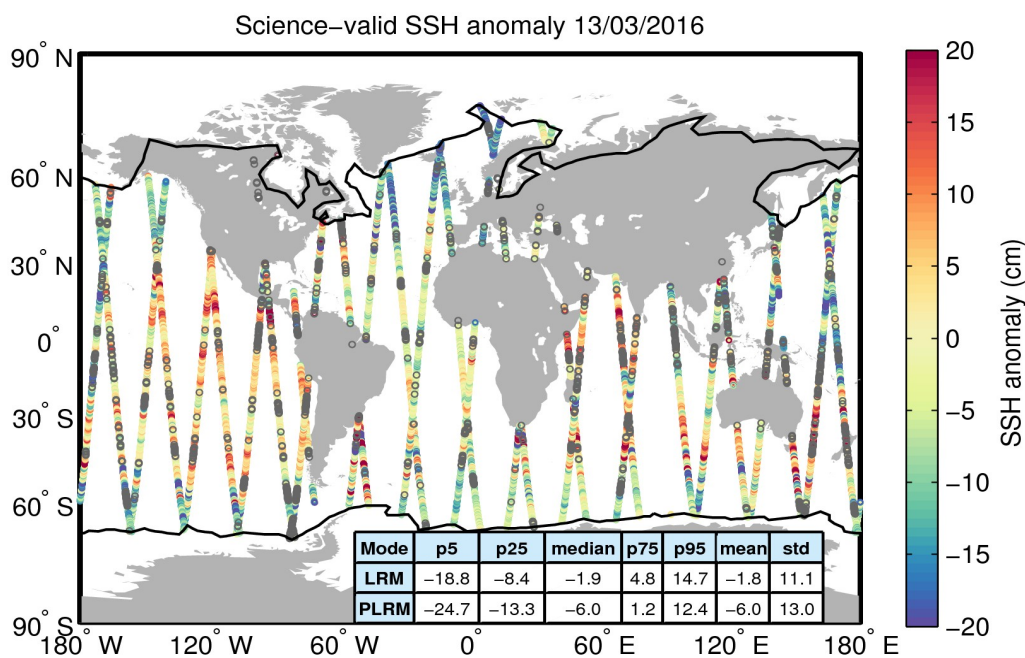
Figure 10. Geographical distribution of science-valid SSH anomaly data over oceans and lakes for 13/03/2016. The statistical values shown in the table refer to the SSH anomaly in cm and are calculated separately for LRM and PLRM regions. The black lines mark the outer limit of the Arctic and Antarctic polar polygons. Gray circles denote records that have been rejected based on the editing criteria described in Table 2.
