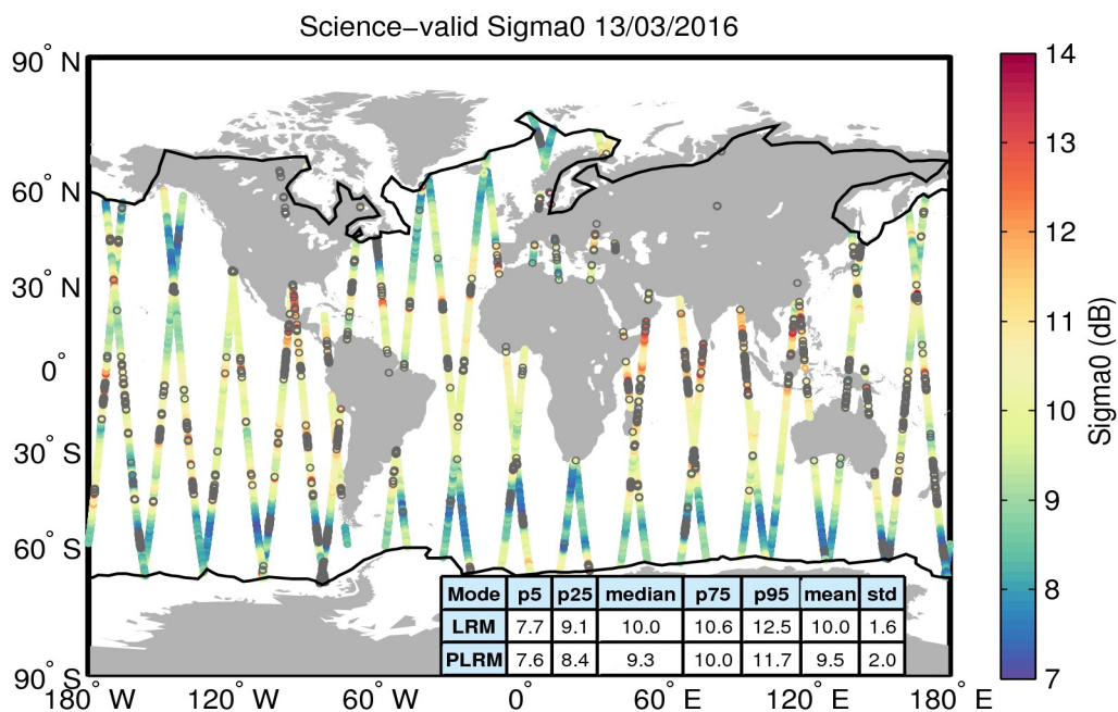
Figure 27. Geographical distribution of science-valid sigma0 data over oceans and lakes for 13/03/2016. The statistical values shown in the table refer to the sigma0 in dB and are calculated separately for LRM and PLRM regions. The black lines mark the outer limit of the Arctic and Antarctic polar polygons. Gray circles denote records that have been rejected based on the editing criteria described in Table 4.
