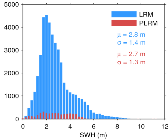
Figure 17. Histogram of flag-valid SWH over oceans and lakes for LRM (blue) and PLRM (red) for 13/03/2016. The mean ( \mu ) and standard deviation ( \sigma ) are also shown. Note that values larger than 12 m are excluded from the histogram for the sake of readability but not from the computation of \mu and \sigma .
