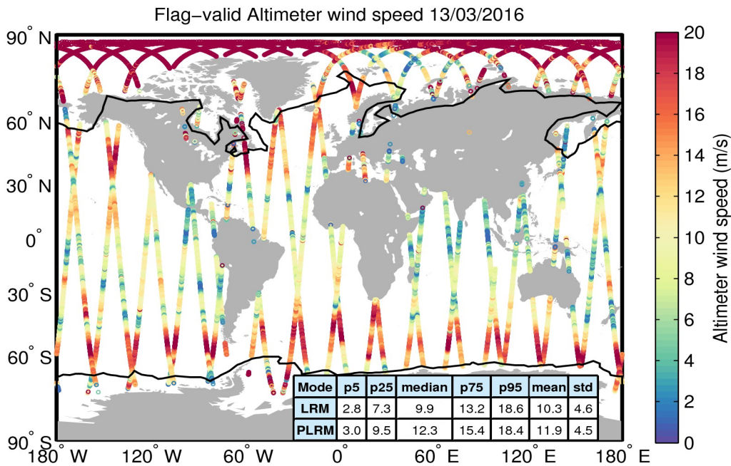
Figure 31. Geographical distribution of flag-valid wind data over oceans and lakes for 13/03/2016. The statistical values shown in the table refer to the wind in m/s and are calculated separately for LRM and PLRM regions. Measurements taken over polar polygons have been excluded from the computation of the statistical values. The black lines mark the outer limit of the Arctic and Antarctic polar polygons.
