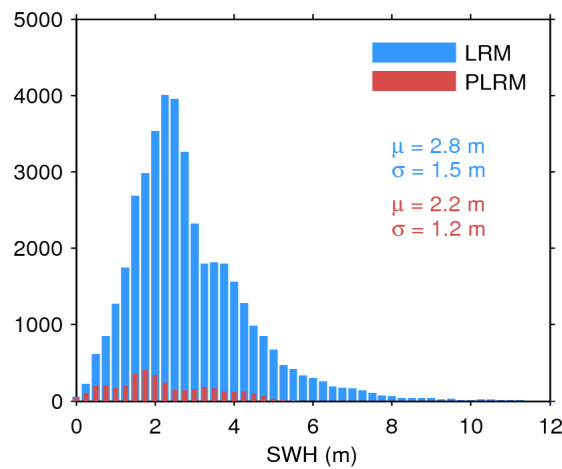
Figure 20. Histogram of science-valid SWH over oceans and lakes for LRM (blue) and PLRM (red) for 01/03/2016. The mean ( \mu ) and standard deviation ( \sigma ) are also shown. Note that values larger than 12 m are excluded from the histogram for the sake of readability but not from the computation of \mu and \sigma .
