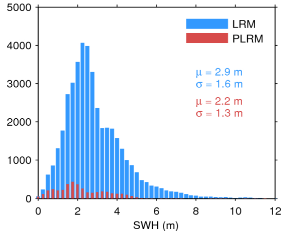
Figure 17. Histogram of flag-valid SWH over oceans and lakes for LRM (blue) and PLRM (red) for 01/03/2016. The mean ( \mu ) and standard deviation ( \sigma ) are also shown. Note that values larger than 12 m are excluded from the histogram for the sake of readability but not from the computation of \mu and \sigma .
