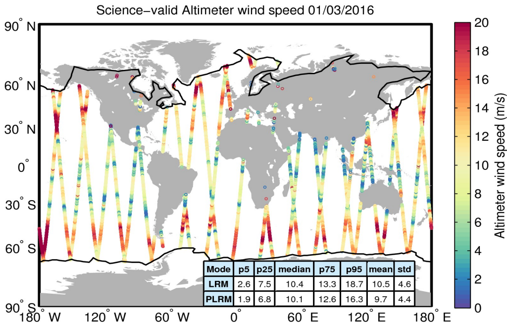
Figure 34. Geographical distribution of science-valid wind data over oceans and lakes for 01/03/2016. The statistical values shown in the table refer to the wind in m/s and are calculated separately for LRM and PLRM regions. The black lines mark the outer limit of the Arctic and Antarctic polar polygons. Gray circles denote records that have been rejected based on the editing criteria described in Table 5.
