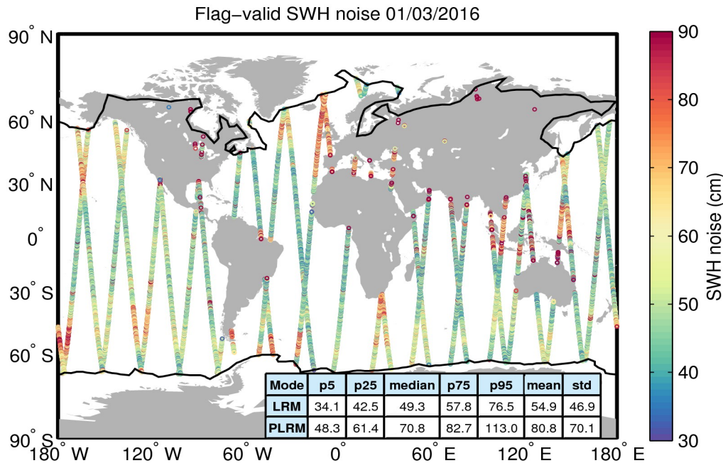
Figure 18. Geographical distribution of flag-valid 20-Hz SWH measurement noise over oceans and lakes for 01/03/2016. The statistical values shown in the table refer to the SWH noise and are calculated separately for LRM and PLRM regions. Measurements taken over polar polygons have been excluded from the computation of the statistical values. The black lines mark the outer limit of the Arctic and Antarctic polar polygons.
