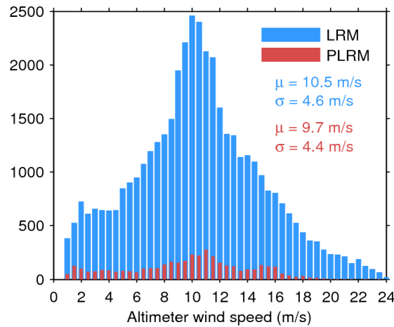
Figure 33. Histogram of flag-valid wind over oceans and lakes for LRM (blue) and PLRM (red) for 01/03/2016. The mean ( \mu ) and standard deviation ( \sigma ) are also shown. Note that values larger than 24 m/s are excluded from the histogram for the sake of readability but not from the computation of \mu and \sigma .
