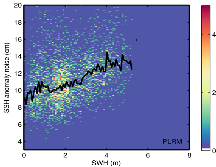
Figure 9. 2D histogram showing flag-valid SSH anomaly noise as a function of SWH for LRM (top) and PLRM (bottom) for 01/03/2016. The black line denotes the median SSH anomaly noise as a function of SWH.
