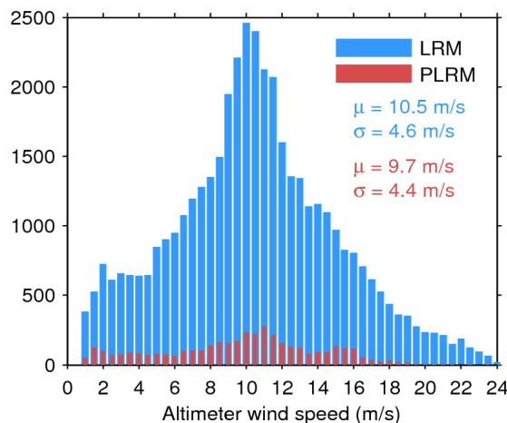
Figure 35. Histogram of science-valid wind over oceans and lakes for LRM (blue) and PLRM (red) for 01/03/2016. The mean ( \mu ) and standard deviation ( \sigma ) are also shown. Note that values larger than 24 m/s are excluded from the histogram for the sake of readability but not from the computation of \mu and \sigma .
