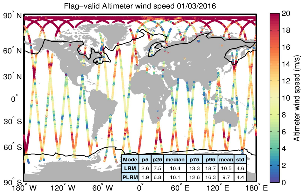
Figure 31. Geographical distribution of flag-valid wind data over oceans and lakes for 01/03/2016. The statistical values shown in the table refer to the wind in m/s and are calculated separately for LRM and PLRM regions. Measurements taken over polar polygons have been excluded from the computation of the statistical values. The black lines mark the outer limit of the Arctic and Antarctic polar polygons.
