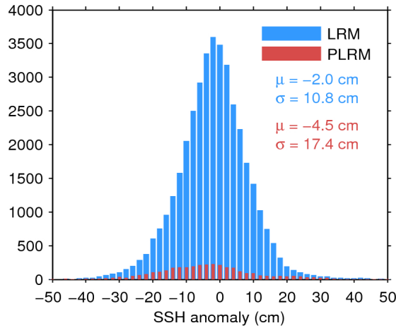
Figure 11. Histogram of science-valid SSH anomaly over oceans and lakes for LRM (blue) and PLRM (red) for 01/03/2016. The mean ( \mu ) and standard deviation ( \sigma ) are also shown. Note that values outside [-50\ 50] cm are excluded from the histogram for the sake of readability but not from the computation of \mu and \sigma .
