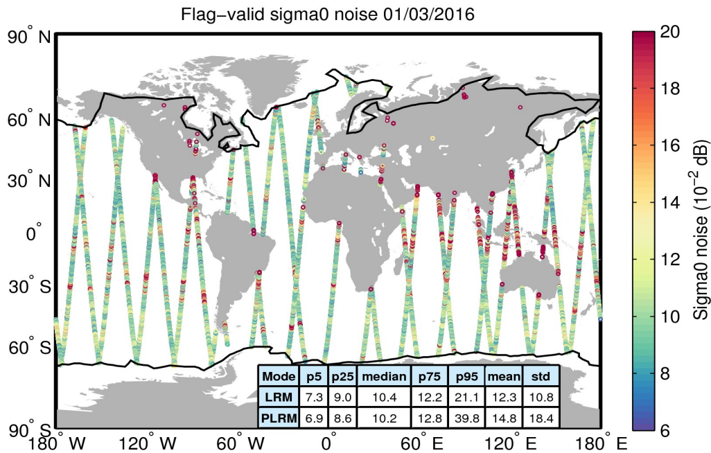
Figure 26. Geographical distribution of flag-valid 20-Hz sigma0 measurement noise over oceans and lakes for 01/03/2016. The statistical values shown in the table refer to the sigma0 noise and are calculated separately for LRM and PLRM regions. Measurements taken over polar polygons have been excluded from the computation of the statistical values. The black lines mark the outer limit of the Arctic and Antarctic polar polygons.
