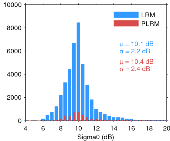
Figure 25. Histogram of flag-valid sigma0 over oceans and lakes for LRM (blue) and PLRM (red) for 01/03/2016. The mean ( \mu ) and standard deviation ( \sigma ) are also shown. Note that values outside [4 20] dB are excluded from the histogram for the sake of readability but not from the computation of \mu and \sigma .
