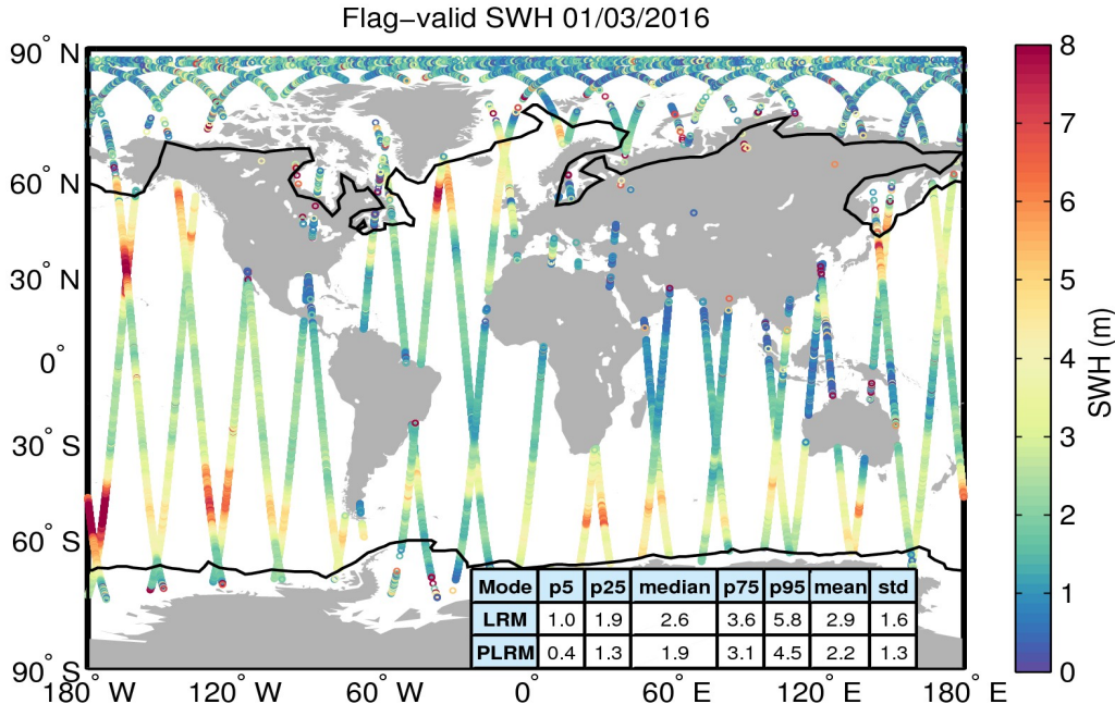
Figure 15. Geographical distribution of flag-valid SWH data over oceans and lakes for 01/03/2016. The statistical values shown in the table refer to the SWH in m and are calculated separately for LRM and PLRM regions. Measurements taken over polar polygons have been excluded from the computation of the statistical values. The black lines mark the outer limit of the Arctic and Antarctic polar polygons.
