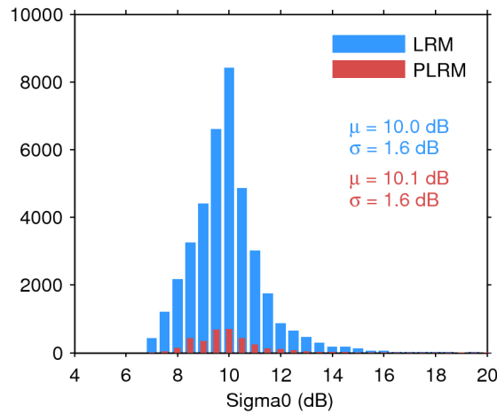
Figure 28. Histogram of science-valid sigma0 over oceans and lakes for LRM (blue) and PLRM (red) for 01/03/2016. The mean ( \mu ) and standard deviation ( \sigma ) are also shown. Note that values outside [4 20] dB are excluded from the histogram for the sake of readability but not from the computation of \mu and \sigma .
