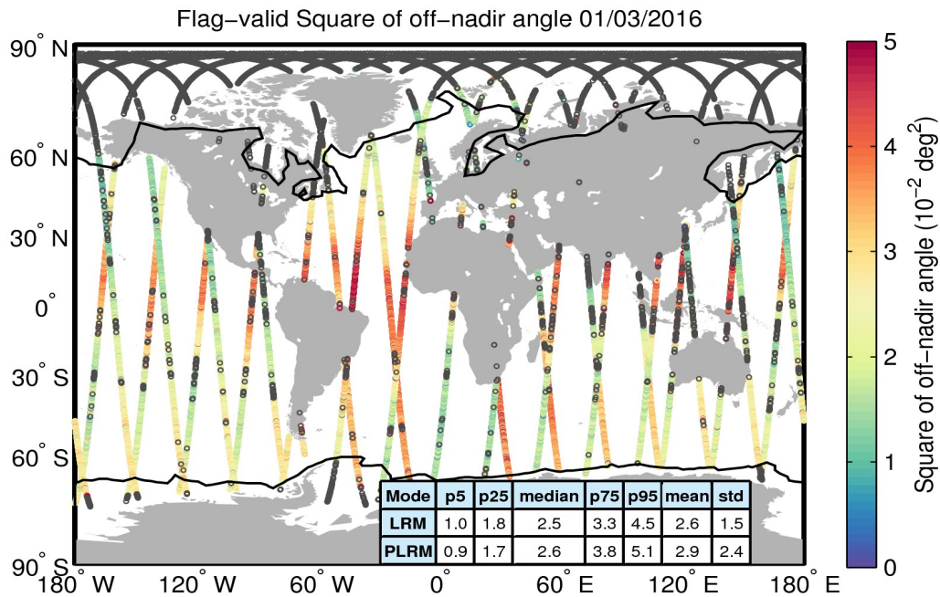
Figure 37. Geographical distribution of flag-valid mispointing data over oceans and lakes for 01/03/2016. The statistical values shown in the table refer to the mispointing in 10^{-2} deg 2 and are calculated separately for LRM and PLRM regions. Measurements taken over polar polygons have been excluded from the computation of the statistical values. The black lines mark the outer limit of the Arctic and Antarctic polar polygons. Gray circles denote negative values.
