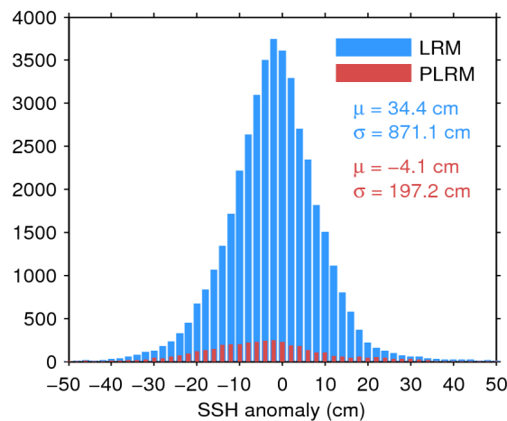
Figure 7. Histogram of flag-valid SSH anomaly over oceans and lakes for LRM (blue) and PLRM (red) for 01/03/2016. The mean ( \mu ) and standard deviation ( \sigma ) are also shown. Note that values outside [-50\ 50] cm are excluded from the histogram for the sake of readability but not from the computation of \mu and \sigma .
