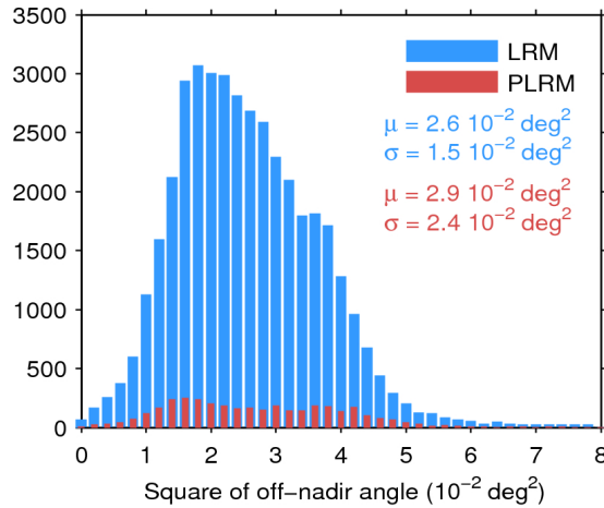
Figure 39. Histogram of flag-valid mispointing over oceans and lakes for LRM (blue) and PLRM (red) for 01/03/2016. Only positive values have been considered. The mean ( \mu ) and standard deviation ( \sigma ) are also shown. Note that values larger than 8 \cdot 10^{-2} \text{ deg}^2 are excluded from the histogram for the sake of readability but not from the computation of \mu and \sigma .
