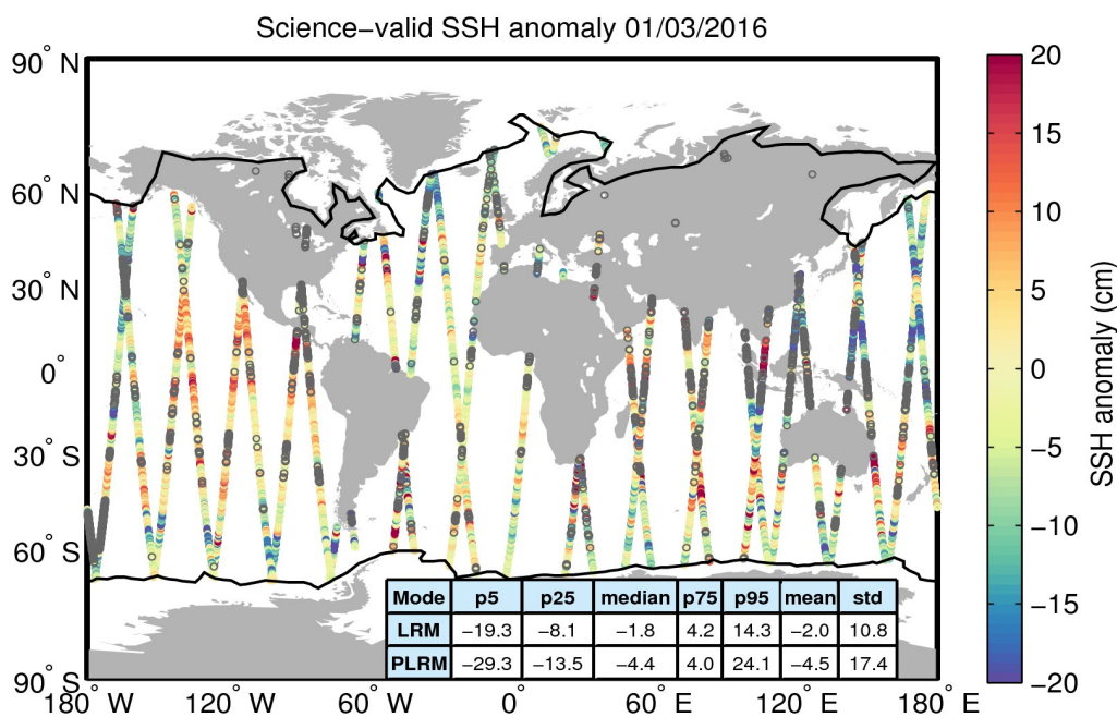
Figure 10. Geographical distribution of science-valid SSH anomaly data over oceans and lakes for 01/03/2016. The statistical values shown in the table refer to the SSH anomaly in cm and are calculated separately for LRM and PLRM regions. The black lines mark the outer limit of the Arctic and Antarctic polar polygons. Gray circles denote records that have been rejected based on the editing criteria described in Table 2.
