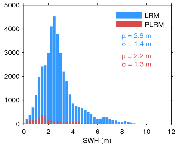
Figure 20. Histogram of science-valid SWH over oceans and lakes for LRM (blue) and PLRM (red) for 29/02/2016. The mean ( \mu ) and standard deviation ( \sigma ) are also shown. Note that values larger than 12 m are excluded from the histogram for the sake of readability but not from the computation of \mu and \sigma .
