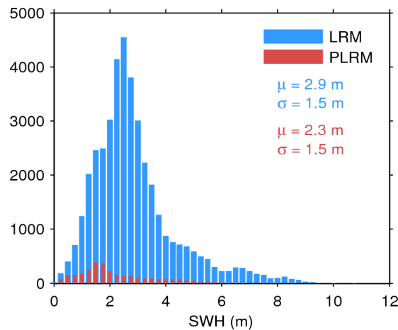
Figure 17. Histogram of flag-valid SWH over oceans and lakes for LRM (blue) and PLRM (red) for 29/02/2016. The mean ( \mu ) and standard deviation ( \sigma ) are also shown. Note that values larger than 12 m are excluded from the histogram for the sake of readability but not from the computation of \mu and \sigma .
