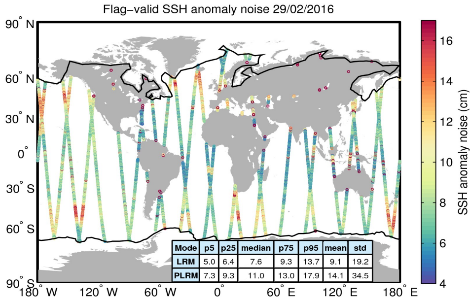
Figure 8. Geographical distribution of flag-valid 20-Hz SSH anomaly measurement noise over oceans and lakes for 29/02/2016. The statistical values shown in the table refer to the SSH anomaly noise and are calculated separately for LRM and PLRM regions. Measurements taken over polar polygons have been excluded from the computation of the statistical values. The black lines mark the outer limit of the Arctic and Antarctic polar polygons.
