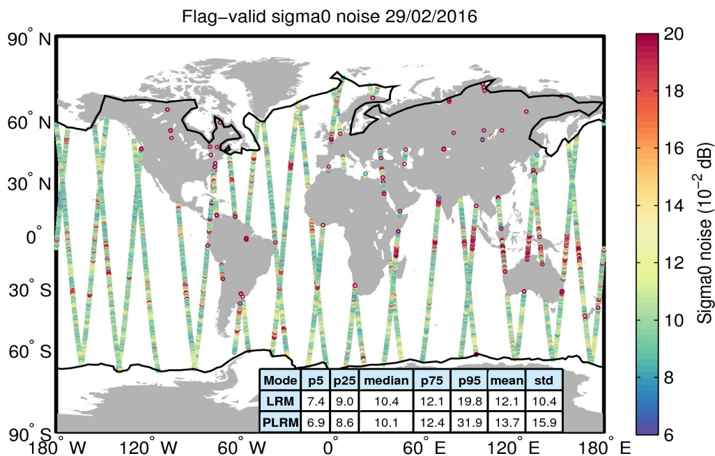
Figure 26. Geographical distribution of flag-valid 20-Hz sigma0 measurement noise over oceans and lakes for 29/02/2016. The statistical values shown in the table refer to the sigma0 noise and are calculated separately for LRM and PLRM regions. Measurements taken over polar polygons have been excluded from the computation of the statistical values. The black lines mark the outer limit of the Arctic and Antarctic polar polygons.
