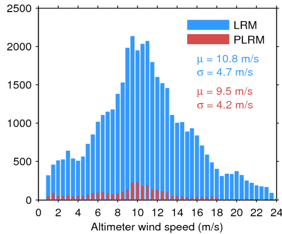
Figure 33. Histogram of flag-valid wind over oceans and lakes for LRM (blue) and PLRM (red) for 29/02/2016. The mean ( \mu ) and standard deviation ( \sigma ) are also shown. Note that values larger than 24 m/s are excluded from the histogram for the sake of readability but not from the computation of \mu and \sigma .
