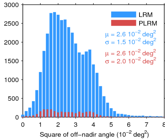
Figure 39. Histogram of flag-valid mispointing over oceans and lakes for LRM (blue) and PLRM (red) for 29/02/2016. Only positive values have been considered. The mean ( \mu ) and standard deviation ( \sigma ) are also shown. Note that values larger than 8 \cdot 10^{-2} \text{ deg}^2 are excluded from the histogram for the sake of readability but not from the computation of \mu and \sigma .
