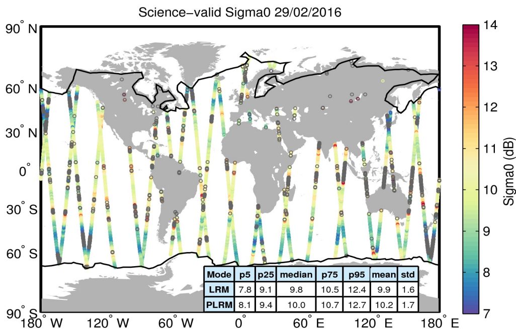
Figure 27. Geographical distribution of science-valid sigma0 data over oceans and lakes for 29/02/2016. The statistical values shown in the table refer to the sigma0 in dB and are calculated separately for LRM and PLRM regions. The black lines mark the outer limit of the Arctic and Antarctic polar polygons. Gray circles denote records that have been rejected based on the editing criteria described in Table 4.
