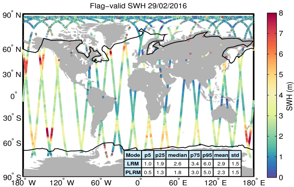
Figure 15. Geographical distribution of flag-valid SWH data over oceans and lakes for 29/02/2016. The statistical values shown in the table refer to the SWH in m and are calculated separately for LRM and PLRM regions. Measurements taken over polar polygons have been excluded from the computation of the statistical values. The black lines mark the outer limit of the Arctic and Antarctic polar polygons.
