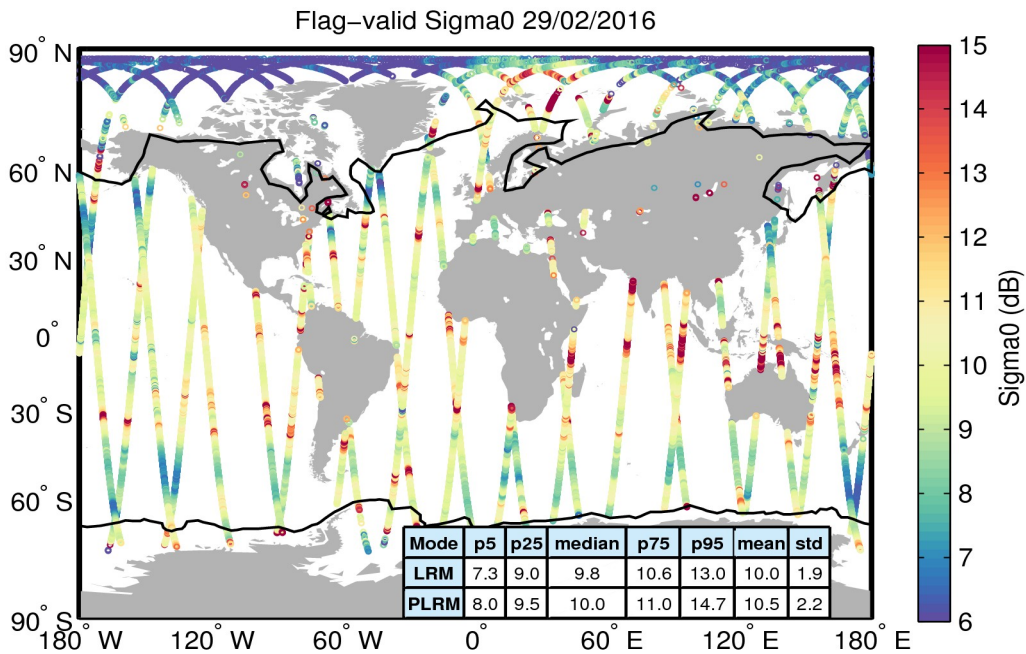
Figure 23. Geographical distribution of flag-valid sigma0 data over oceans and lakes for 29/02/2016. The statistical values shown in the table refer to the sigma0 in dB and are calculated separately for LRM and PLRM regions. Measurements taken over polar polygons have been excluded from the computation of the statistical values. The black lines mark the outer limit of the Arctic and Antarctic polar polygons.
