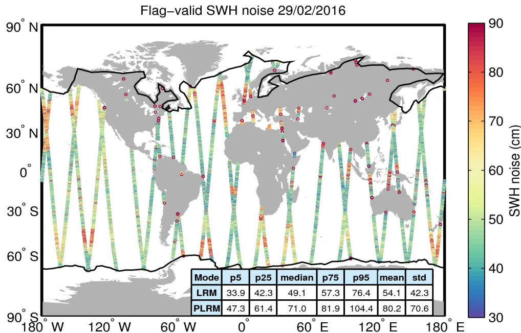
Figure 18. Geographical distribution of flag-valid 20-Hz SWH measurement noise over oceans and lakes for 29/02/2016. The statistical values shown in the table refer to the SWH noise and are calculated separately for LRM and PLRM regions. Measurements taken over polar polygons have been excluded from the computation of the statistical values. The black lines mark the outer limit of the Arctic and Antarctic polar polygons.
