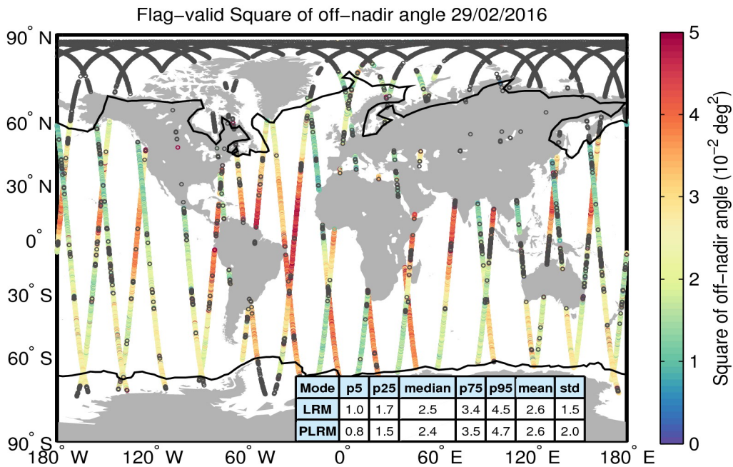
Figure 37. Geographical distribution of flag-valid mispointing data over oceans and lakes for 29/02/2016. The statistical values shown in the table refer to the mispointing in 10^{-2} deg 2 and are calculated separately for LRM and PLRM regions. Measurements taken over polar polygons have been excluded from the computation of the statistical values. The black lines mark the outer limit of the Arctic and Antarctic polar polygons. Gray circles denote negative values.
