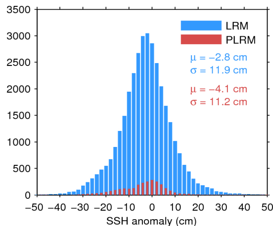
Figure 11. Histogram of science-valid SSH anomaly over oceans and lakes for LRM (blue) and PLRM (red) for 29/02/2016. The mean ( \mu ) and standard deviation ( \sigma ) are also shown. Note that values outside [-50 50] cm are excluded from the histogram for the sake of readability but not from the computation of \mu and \sigma .
