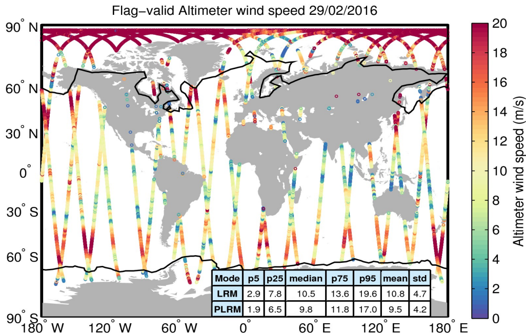
Figure 31. Geographical distribution of flag-valid wind data over oceans and lakes for 29/02/2016. The statistical values shown in the table refer to the wind in m/s and are calculated separately for LRM and PLRM regions. Measurements taken over polar polygons have been excluded from the computation of the statistical values. The black lines mark the outer limit of the Arctic and Antarctic polar polygons.
