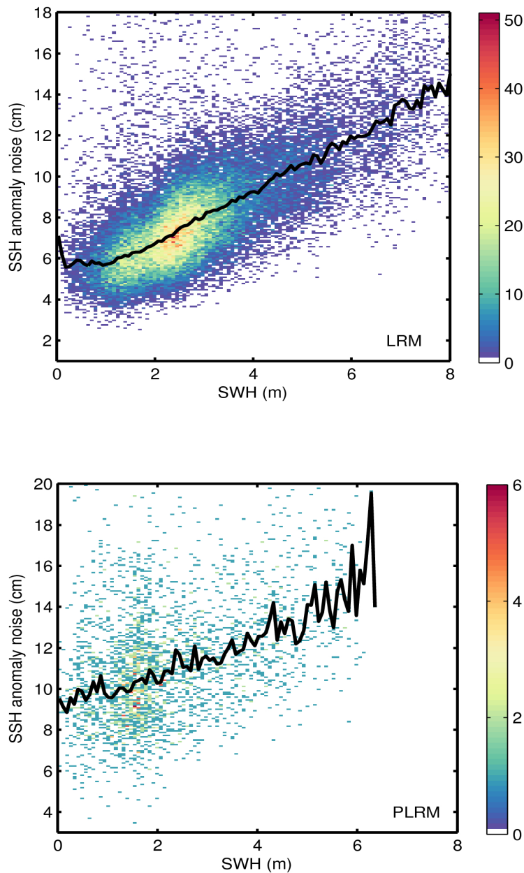
Figure 9. 2D histogram showing flag-valid SSH anomaly noise as a function of SWH for LRM (top) and PLRM (bottom) for 29/02/2016. The black line denotes the median SSH anomaly noise as a function of SWH.
