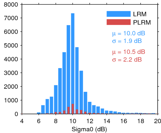
Figure 25. Histogram of flag-valid sigma0 over oceans and lakes for LRM (blue) and PLRM (red) for 29/02/2016. The mean ( \mu ) and standard deviation ( \sigma ) are also shown. Note that values outside [4 20] dB are excluded from the histogram for the sake of readability but not from the computation of \mu and \sigma .
