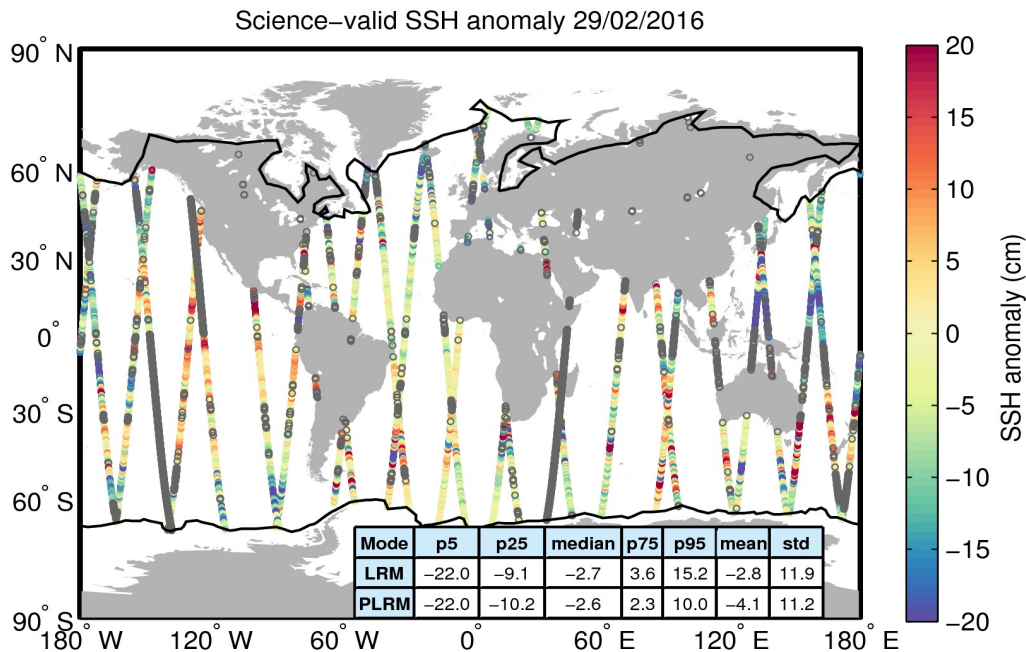
Figure 10. Geographical distribution of science-valid SSH anomaly data over oceans and lakes for 29/02/2016. The statistical values shown in the table refer to the SSH anomaly in cm and are calculated separately for LRM and PLRM regions. The black lines mark the outer limit of the Arctic and Antarctic polar polygons. Gray circles denote records that have been rejected based on the editing criteria described in Table 2.
