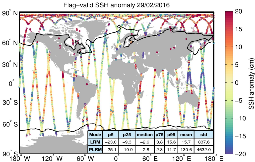
Figure 5. Geographical distribution of flag-valid 1-Hz SSH anomaly data over oceans and lakes for 29/02/2016. The statistical values shown in the table refer to the SSH anomaly in cm and are calculated separately for LRM and PLRM regions. Measurements taken over polar polygons have been excluded from the computation of the statistical values. The black lines mark the outer limit of the Arctic and Antarctic polar polygons.
