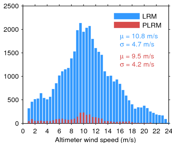
Figure 35. Histogram of science-valid wind over oceans and lakes for LRM (blue) and PLRM (red) for 29/02/2016. The mean ( \mu ) and standard deviation ( \sigma ) are also shown. Note that values larger than 24 m/s are excluded from the histogram for the sake of readability but not from the computation of \mu and \sigma .
