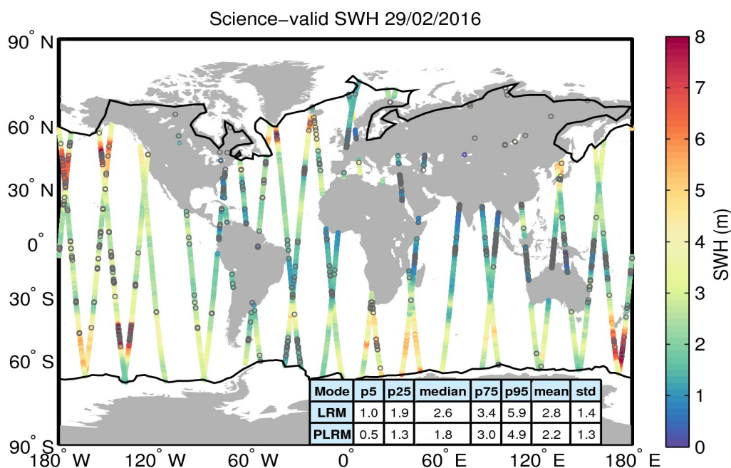
Figure 19. Geographical distribution of science-valid SWH data over oceans and lakes for 29/02/2016. The statistical values shown in the table refer to the SWH in m and are calculated separately for LRM and PLRM regions. The black lines mark the outer limit of the Arctic and Antarctic polar polygons. Gray circles denote records that have been rejected based on the editing criteria described in Table 3.
