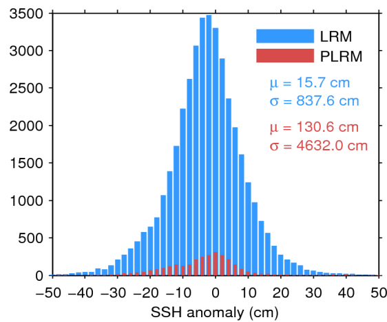
Figure 7. Histogram of flag-valid SSH anomaly over oceans and lakes for LRM (blue) and PLRM (red) for 29/02/2016. The mean ( \mu ) and standard deviation ( \sigma ) are also shown. Note that values outside [-50 50] cm are excluded from the histogram for the sake of readability but not from the computation of \mu and \sigma .
