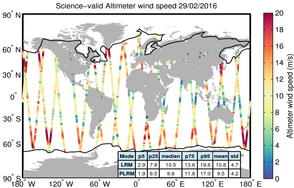
Figure 34. Geographical distribution of science-valid wind data over oceans and lakes for 29/02/2016. The statistical values shown in the table refer to the wind in m/s and are calculated separately for LRM and PLRM regions. The black lines mark the outer limit of the Arctic and Antarctic polar polygons. Gray circles denote records that have been rejected based on the editing criteria described in Table 5.
