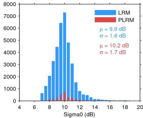
Figure 28. Histogram of science-valid sigma0 over oceans and lakes for LRM (blue) and PLRM (red) for 29/02/2016. The mean ( \mu ) and standard deviation ( \sigma ) are also shown. Note that values outside [4 20] dB are excluded from the histogram for the sake of readability but not from the computation of \mu and \sigma .
