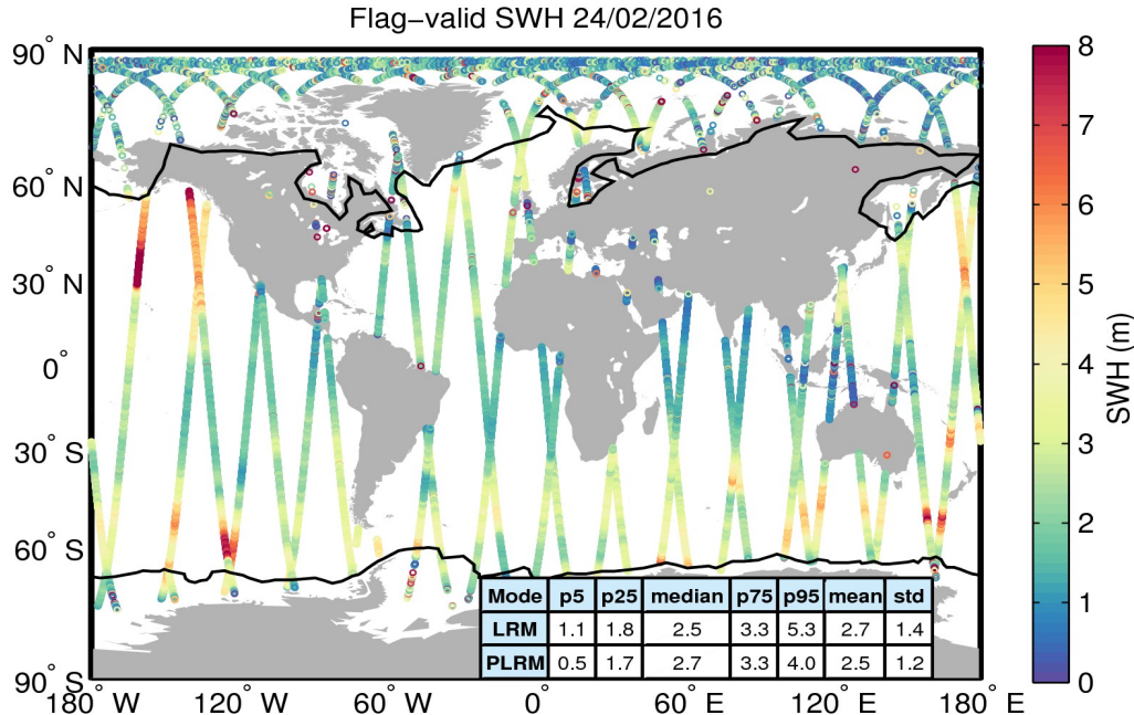
Figure 15. Geographical distribution of flag-valid SWH data over oceans and lakes for 24/02/2016. The statistical values shown in the table refer to the SWH in m and are calculated separately for LRM and PLRM regions. Measurements taken over polar polygons have been excluded from the computation of the statistical values. The black lines mark the outer limit of the Arctic and Antarctic polar polygons.
