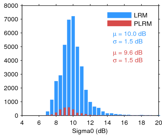
Figure 28. Histogram of science-valid sigma0 over oceans and lakes for LRM (blue) and PLRM (red) for 24/02/2016. The mean ( \mu ) and standard deviation ( \sigma ) are also shown. Note that values outside [4 20] dB are excluded from the histogram for the sake of readability but not from the computation of \mu and \sigma .
