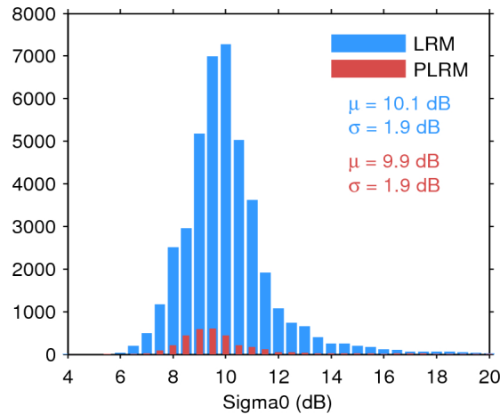
Figure 25. Histogram of flag-valid sigma0 over oceans and lakes for LRM (blue) and PLRM (red) for 24/02/2016. The mean ( \mu ) and standard deviation ( \sigma ) are also shown. Note that values outside [4 20] dB are excluded from the histogram for the sake of readability but not from the computation of \mu and \sigma .
