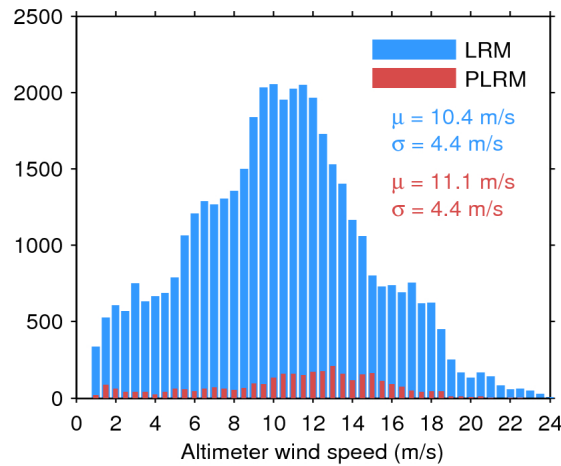
Figure 33. Histogram of flag-valid wind over oceans and lakes for LRM (blue) and PLRM (red) for 24/02/2016. The mean ( \mu ) and standard deviation ( \sigma ) are also shown. Note that values larger than 24 m/s are excluded from the histogram for the sake of readability but not from the computation of \mu and \sigma .
