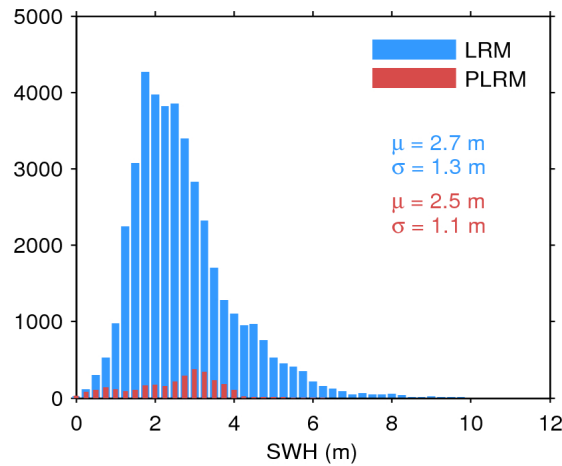
Figure 20. Histogram of science-valid SWH over oceans and lakes for LRM (blue) and PLRM (red) for 24/02/2016. The mean ( \mu ) and standard deviation ( \sigma ) are also shown. Note that values larger than 12 m are excluded from the histogram for the sake of readability but not from the computation of \mu and \sigma .
