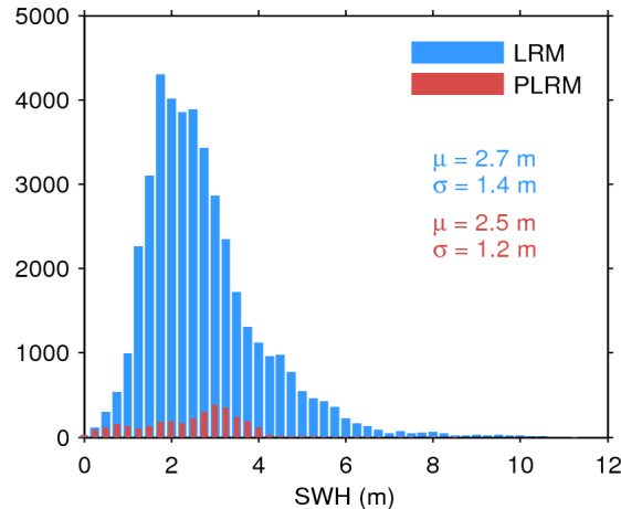
Figure 17. Histogram of flag-valid SWH over oceans and lakes for LRM (blue) and PLRM (red) for 24/02/2016. The mean ( \mu ) and standard deviation ( \sigma ) are also shown. Note that values larger than 12 m are excluded from the histogram for the sake of readability but not from the computation of \mu and \sigma .
