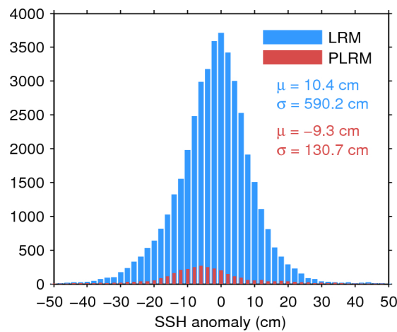
Figure 7. Histogram of flag-valid SSH anomaly over oceans and lakes for LRM (blue) and PLRM (red) for 24/02/2016. The mean ( \mu ) and standard deviation ( \sigma ) are also shown. Note that values outside [-50\ 50] cm are excluded from the histogram for the sake of readability but not from the computation of \mu and \sigma .
