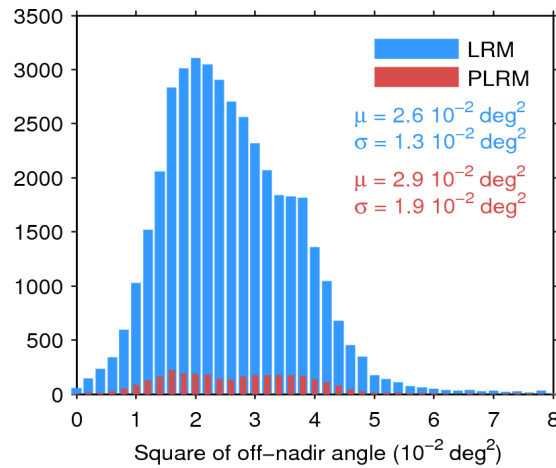
Figure 39. Histogram of flag-valid mispointing over oceans and lakes for LRM (blue) and PLRM (red) for 24/02/2016. Only positive values have been considered. The mean ( \mu ) and standard deviation ( \sigma ) are also shown. Note that values larger than 8 \cdot 10^{-2} \text{ deg}^2 are excluded from the histogram for the sake of readability but not from the computation of \mu and \sigma .
