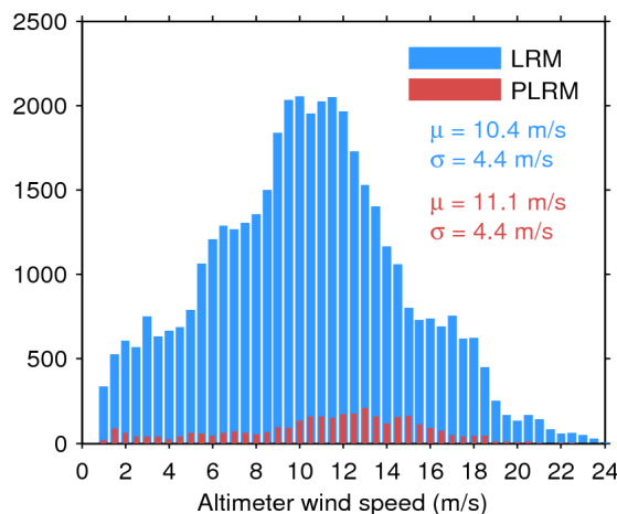
Figure 35. Histogram of science-valid wind over oceans and lakes for LRM (blue) and PLRM (red) for 24/02/2016. The mean ( \mu ) and standard deviation ( \sigma ) are also shown. Note that values larger than 24 m/s are excluded from the histogram for the sake of readability but not from the computation of \mu and \sigma .
