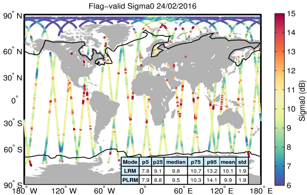
Figure 23. Geographical distribution of flag-valid sigma0 data over oceans and lakes for 24/02/2016. The statistical values shown in the table refer to the sigma0 in dB and are calculated separately for LRM and PLRM regions. Measurements taken over polar polygons have been excluded from the computation of the statistical values. The black lines mark the outer limit of the Arctic and Antarctic polar polygons.
