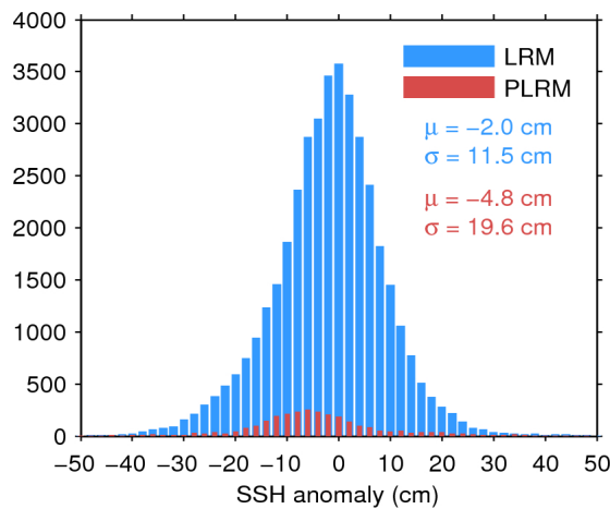
Figure 11. Histogram of science-valid SSH anomaly over oceans and lakes for LRM (blue) and PLRM (red) for 24/02/2016. The mean ( \mu ) and standard deviation ( \sigma ) are also shown. Note that values outside [-50 50] cm are excluded from the histogram for the sake of readability but not from the computation of \mu and \sigma .
