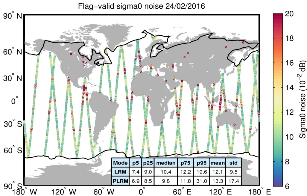
Figure 26. Geographical distribution of flag-valid 20-Hz sigma0 measurement noise over oceans and lakes for 24/02/2016. The statistical values shown in the table refer to the sigma0 noise and are calculated separately for LRM and PLRM regions. Measurements taken over polar polygons have been excluded from the computation of the statistical values. The black lines mark the outer limit of the Arctic and Antarctic polar polygons.
