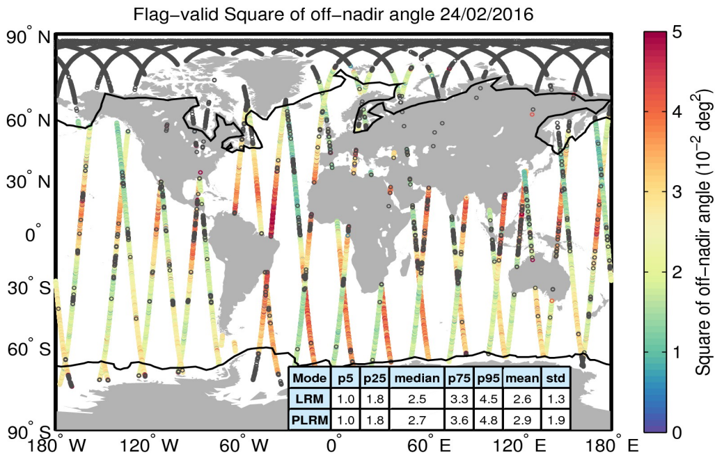
Figure 37. Geographical distribution of flag-valid mispointing data over oceans and lakes for 24/02/2016. The statistical values shown in the table refer to the mispointing in 10^{-2} deg 2 and are calculated separately for LRM and PLRM regions. Measurements taken over polar polygons have been excluded from the computation of the statistical values. The black lines mark the outer limit of the Arctic and Antarctic polar polygons. Gray circles denote negative values.
