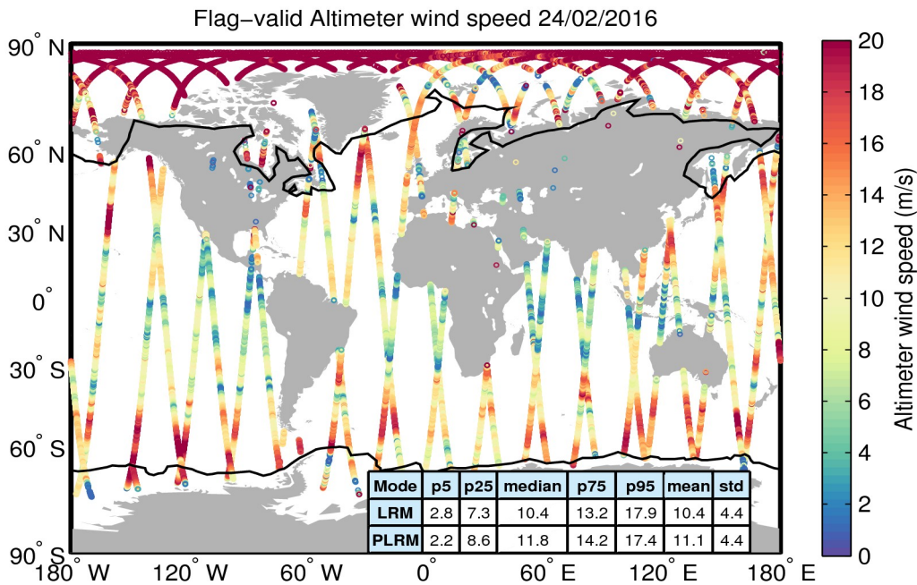
Figure 31. Geographical distribution of flag-valid wind data over oceans and lakes for 24/02/2016. The statistical values shown in the table refer to the wind in m/s and are calculated separately for LRM and PLRM regions. Measurements taken over polar polygons have been excluded from the computation of the statistical values. The black lines mark the outer limit of the Arctic and Antarctic polar polygons.
