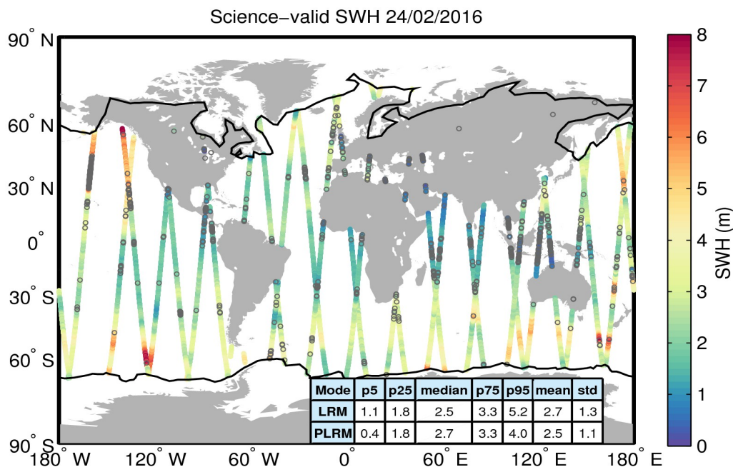
Figure 19. Geographical distribution of science-valid SWH data over oceans and lakes for 24/02/2016. The statistical values shown in the table refer to the SWH in m and are calculated separately for LRM and PLRM regions. The black lines mark the outer limit of the Arctic and Antarctic polar polygons. Gray circles denote records that have been rejected based on the editing criteria described in Table 3.
