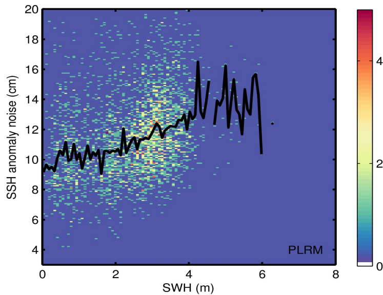
Figure 9. 2D histogram showing flag-valid SSH anomaly noise as a function of SWH for LRM (top) and PLRM (bottom) for 24/02/2016. The black line denotes the median SSH anomaly noise as a function of SWH.
