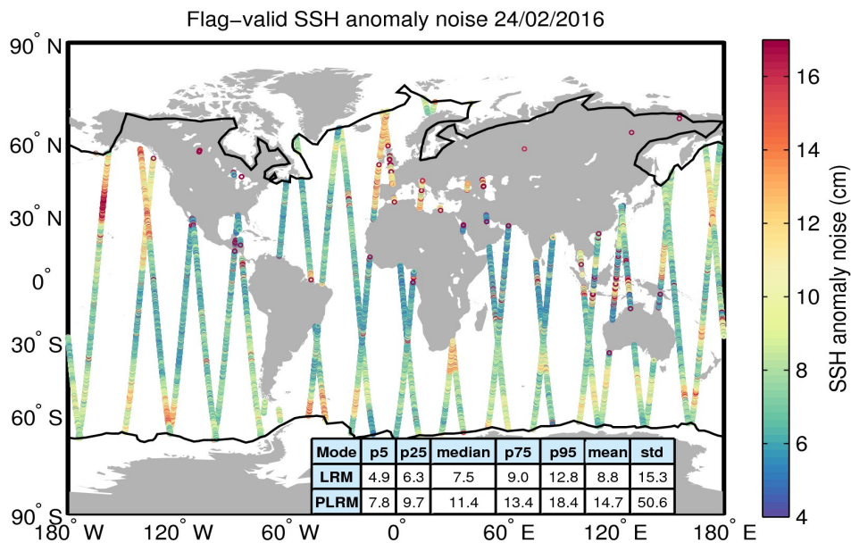
Figure 8. Geographical distribution of flag-valid 20-Hz SSH anomaly measurement noise over oceans and lakes for 24/02/2016. The statistical values shown in the table refer to the SSH anomaly noise and are calculated separately for LRM and PLRM regions. Measurements taken over polar polygons have been excluded from the computation of the statistical values. The black lines mark the outer limit of the Arctic and Antarctic polar polygons.
