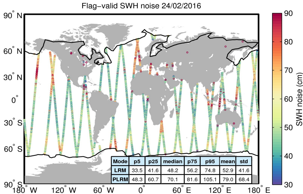
Figure 18. Geographical distribution of flag-valid 20-Hz SWH measurement noise over oceans and lakes for 24/02/2016. The statistical values shown in the table refer to the SWH noise and are calculated separately for LRM and PLRM regions. Measurements taken over polar polygons have been excluded from the computation of the statistical values. The black lines mark the outer limit of the Arctic and Antarctic polar polygons.
