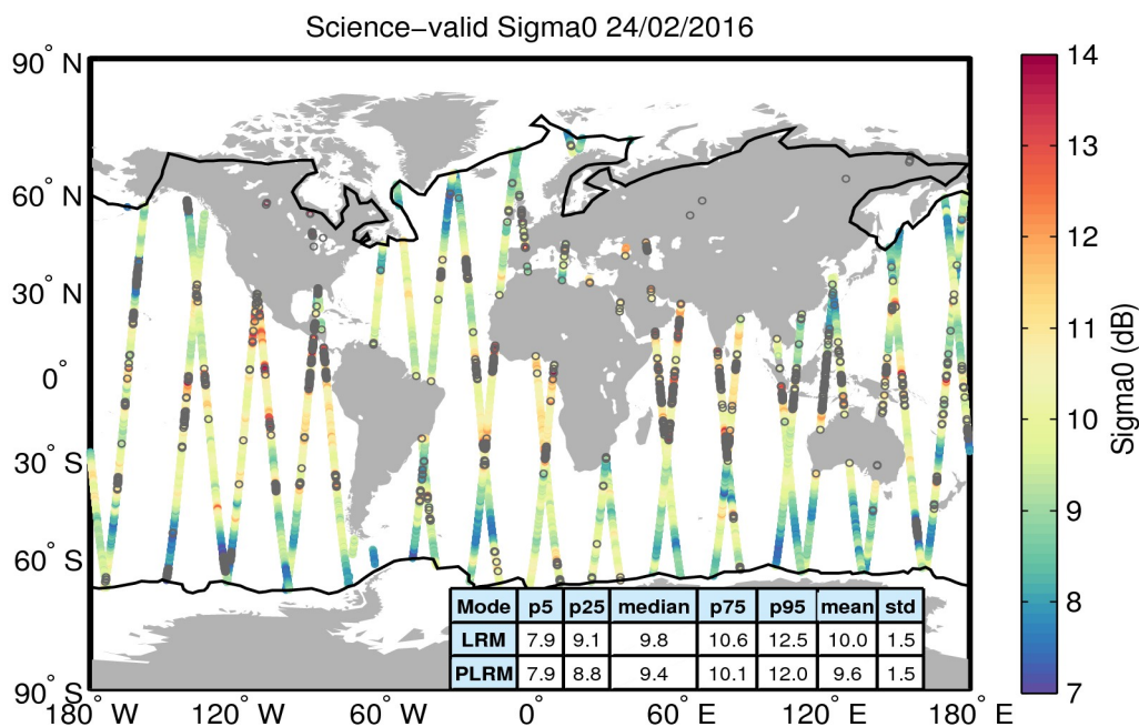
Figure 27. Geographical distribution of science-valid sigma0 data over oceans and lakes for 24/02/2016. The statistical values shown in the table refer to the sigma0 in dB and are calculated separately for LRM and PLRM regions. The black lines mark the outer limit of the Arctic and Antarctic polar polygons. Gray circles denote records that have been rejected based on the editing criteria described in Table 4.
