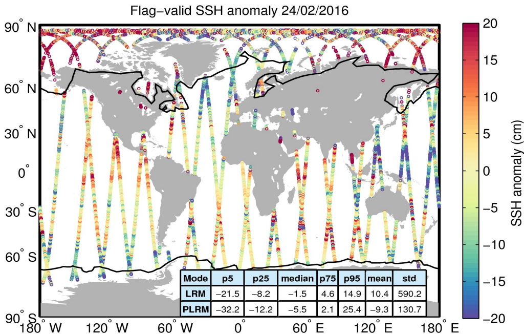
Figure 5. Geographical distribution of flag-valid 1-Hz SSH anomaly data over oceans and lakes for 24/02/2016. The statistical values shown in the table refer to the SSH anomaly in cm and are calculated separately for LRM and PLRM regions. Measurements taken over polar polygons have been excluded from the computation of the statistical values. The black lines mark the outer limit of the Arctic and Antarctic polar polygons.
