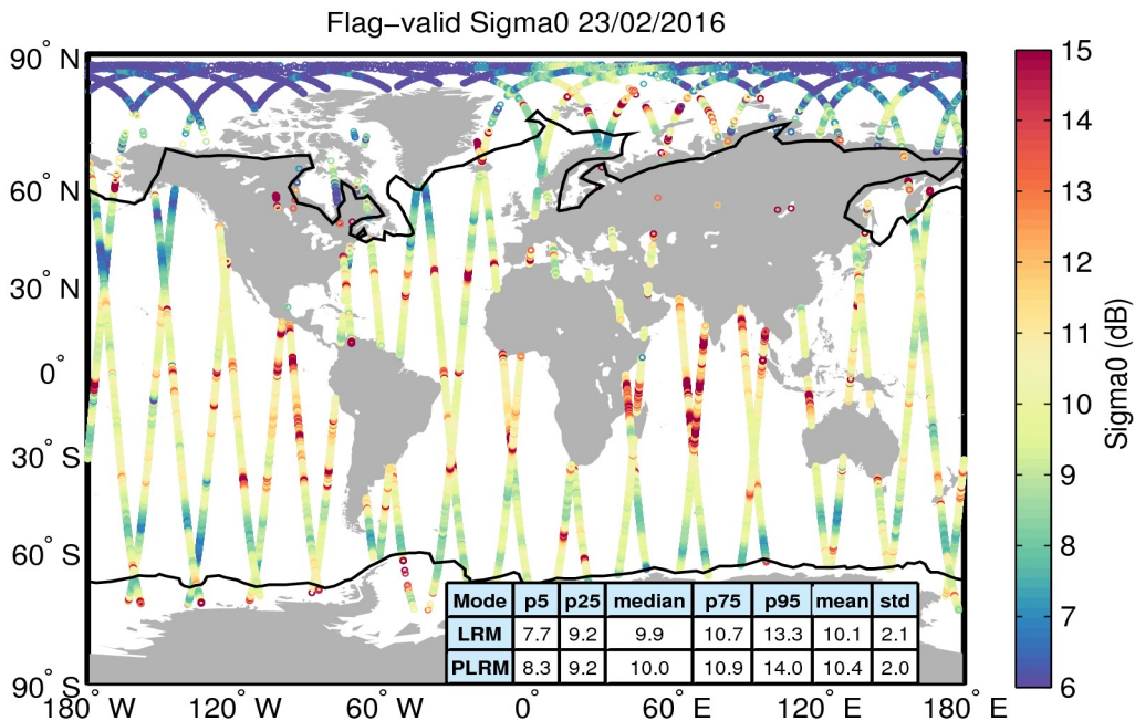
Figure 23. Geographical distribution of flag-valid sigma0 data over oceans and lakes for 23/02/2016. The statistical values shown in the table refer to the sigma0 in dB and are calculated separately for LRM and PLRM regions. Measurements taken over polar polygons have been excluded from the computation of the statistical values. The black lines mark the outer limit of the Arctic and Antarctic polar polygons.
