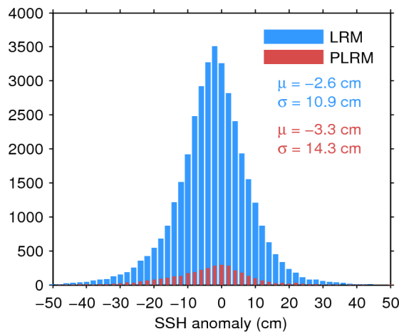
Figure 11. Histogram of science-valid SSH anomaly over oceans and lakes for LRM (blue) and PLRM (red) for 23/02/2016. The mean ( \mu ) and standard deviation ( \sigma ) are also shown. Note that values outside [-50 50] cm are excluded from the histogram for the sake of readability but not from the computation of \mu and \sigma .
