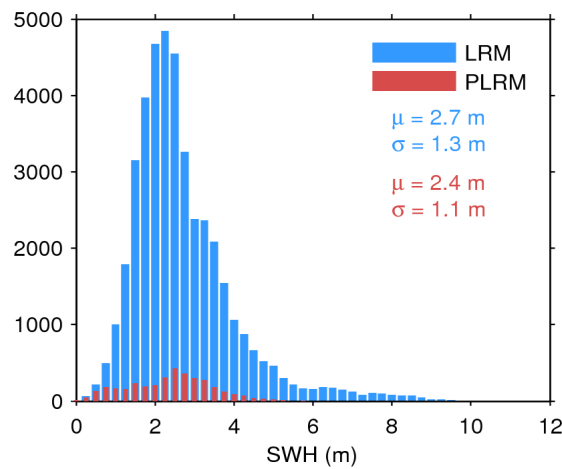
Figure 20. Histogram of science-valid SWH over oceans and lakes for LRM (blue) and PLRM (red) for 23/02/2016. The mean ( \mu ) and standard deviation ( \sigma ) are also shown. Note that values larger than 12 m are excluded from the histogram for the sake of readability but not from the computation of \mu and \sigma .
