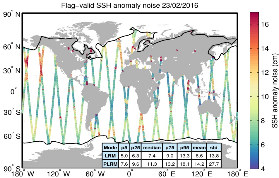
Figure 8. Geographical distribution of flag-valid 20-Hz SSH anomaly measurement noise over oceans and lakes for 23/02/2016. The statistical values shown in the table refer to the SSH anomaly noise and are calculated separately for LRM and PLRM regions. Measurements taken over polar polygons have been excluded from the computation of the statistical values. The black lines mark the outer limit of the Arctic and Antarctic polar polygons.
