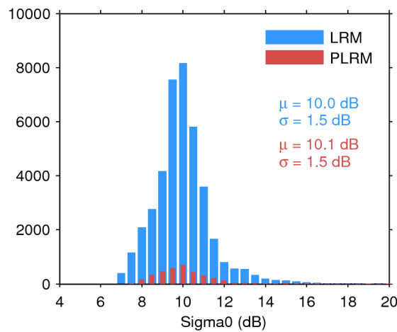
Figure 28. Histogram of science-valid sigma0 over oceans and lakes for LRM (blue) and PLRM (red) for 23/02/2016. The mean ( \mu ) and standard deviation ( \sigma ) are also shown. Note that values outside [4 20] dB are excluded from the histogram for the sake of readability but not from the computation of \mu and \sigma .
