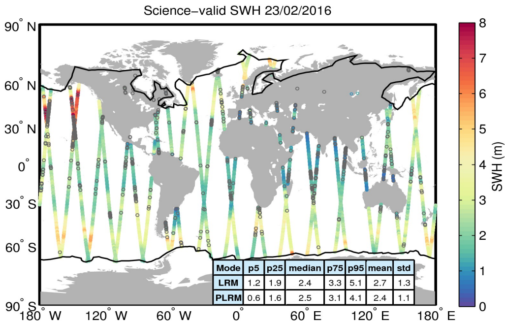
Figure 19. Geographical distribution of science-valid SWH data over oceans and lakes for 23/02/2016. The statistical values shown in the table refer to the SWH in m and are calculated separately for LRM and PLRM regions. The black lines mark the outer limit of the Arctic and Antarctic polar polygons. Gray circles denote records that have been rejected based on the editing criteria described in Table 3.
