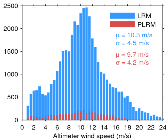
Figure 35. Histogram of science-valid wind over oceans and lakes for LRM (blue) and PLRM (red) for 23/02/2016. The mean ( \mu ) and standard deviation ( \sigma ) are also shown. Note that values larger than 24 m/s are excluded from the histogram for the sake of readability but not from the computation of \mu and \sigma .
