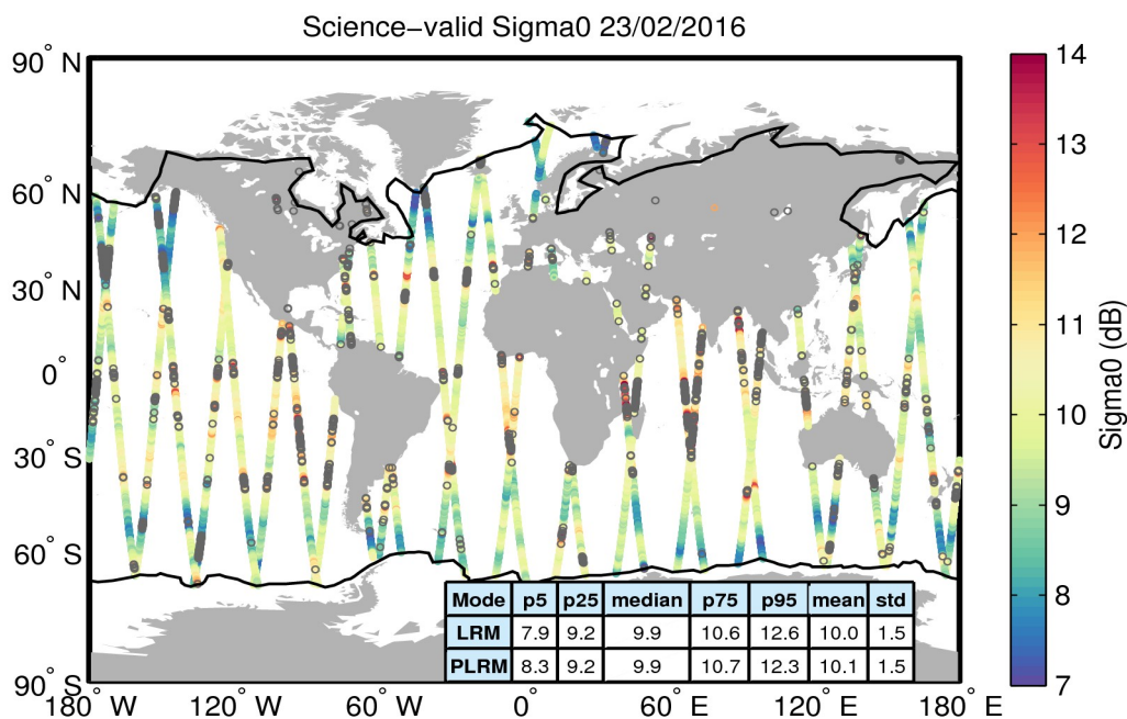
Figure 27. Geographical distribution of science-valid sigma0 data over oceans and lakes for 23/02/2016. The statistical values shown in the table refer to the sigma0 in dB and are calculated separately for LRM and PLRM regions. The black lines mark the outer limit of the Arctic and Antarctic polar polygons. Gray circles denote records that have been rejected based on the editing criteria described in Table 4.
