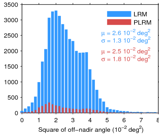
Figure 39. Histogram of flag-valid mispointing over oceans and lakes for LRM (blue) and PLRM (red) for 23/02/2016. Only positive values have been considered. The mean ( \mu ) and standard deviation ( \sigma ) are also shown. Note that values larger than 8 \cdot 10^{-2} \text{ deg}^2 are excluded from the histogram for the sake of readability but not from the computation of \mu and \sigma .
