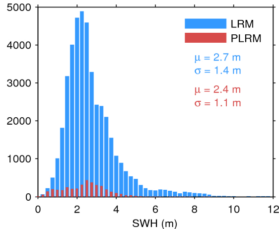
Figure 17. Histogram of flag-valid SWH over oceans and lakes for LRM (blue) and PLRM (red) for 23/02/2016. The mean ( \mu ) and standard deviation ( \sigma ) are also shown. Note that values larger than 12 m are excluded from the histogram for the sake of readability but not from the computation of \mu and \sigma .
