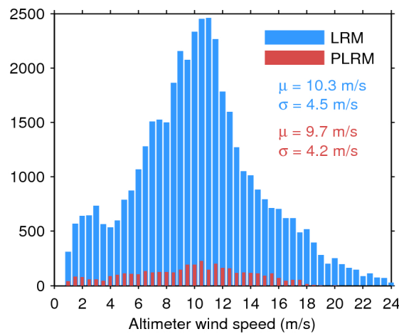
Figure 33. Histogram of flag-valid wind over oceans and lakes for LRM (blue) and PLRM (red) for 23/02/2016. The mean ( \mu ) and standard deviation ( \sigma ) are also shown. Note that values larger than 24 m/s are excluded from the histogram for the sake of readability but not from the computation of \mu and \sigma .
