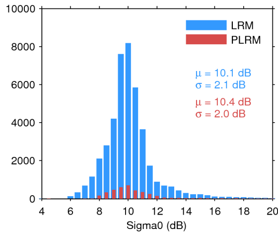
Figure 25. Histogram of flag-valid sigma0 over oceans and lakes for LRM (blue) and PLRM (red) for 23/02/2016. The mean ( \mu ) and standard deviation ( \sigma ) are also shown. Note that values outside [4 20] dB are excluded from the histogram for the sake of readability but not from the computation of \mu and \sigma .
