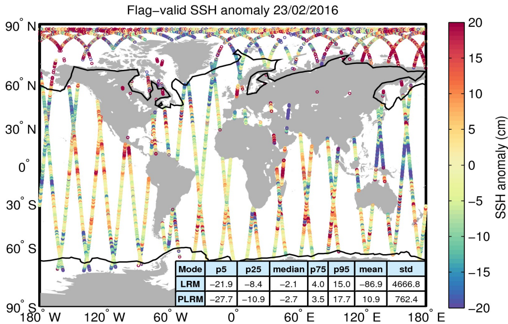
Figure 5. Geographical distribution of flag-valid 1-Hz SSH anomaly data over oceans and lakes for 23/02/2016. The statistical values shown in the table refer to the SSH anomaly in cm and are calculated separately for LRM and PLRM regions. Measurements taken over polar polygons have been excluded from the computation of the statistical values. The black lines mark the outer limit of the Arctic and Antarctic polar polygons.
