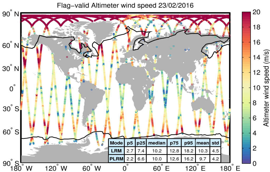
Figure 31. Geographical distribution of flag-valid wind data over oceans and lakes for 23/02/2016. The statistical values shown in the table refer to the wind in m/s and are calculated separately for LRM and PLRM regions. Measurements taken over polar polygons have been excluded from the computation of the statistical values. The black lines mark the outer limit of the Arctic and Antarctic polar polygons.
