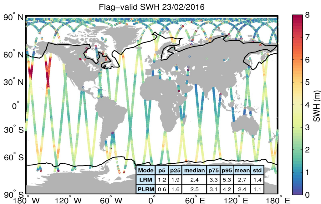
Figure 15. Geographical distribution of flag-valid SWH data over oceans and lakes for 23/02/2016. The statistical values shown in the table refer to the SWH in m and are calculated separately for LRM and PLRM regions. Measurements taken over polar polygons have been excluded from the computation of the statistical values. The black lines mark the outer limit of the Arctic and Antarctic polar polygons.
