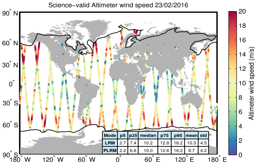
Figure 34. Geographical distribution of science-valid wind data over oceans and lakes for 23/02/2016. The statistical values shown in the table refer to the wind in m/s and are calculated separately for LRM and PLRM regions. The black lines mark the outer limit of the Arctic and Antarctic polar polygons. Gray circles denote records that have been rejected based on the editing criteria described in Table 5.
