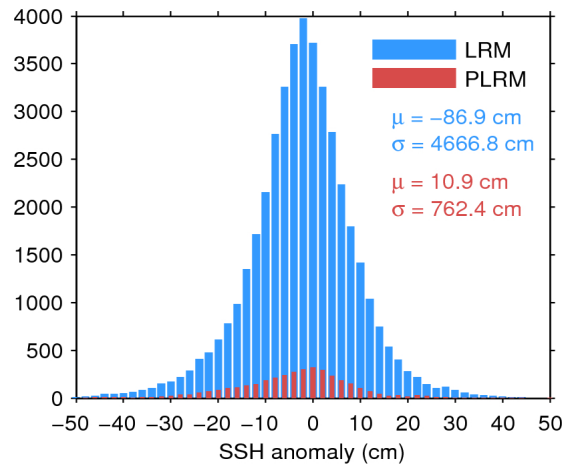
Figure 7. Histogram of flag-valid SSH anomaly over oceans and lakes for LRM (blue) and PLRM (red) for 23/02/2016. The mean ( \mu ) and standard deviation ( \sigma ) are also shown. Note that values outside [-50 50] cm are excluded from the histogram for the sake of readability but not from the computation of \mu and \sigma .
