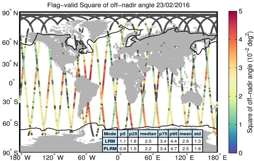
Figure 37. Geographical distribution of flag-valid mispointing data over oceans and lakes for 23/02/2016. The statistical values shown in the table refer to the mispointing in 10^{-2} deg 2 and are calculated separately for LRM and PLRM regions. Measurements taken over polar polygons have been excluded from the computation of the statistical values. The black lines mark the outer limit of the Arctic and Antarctic polar polygons. Gray circles denote negative values.
