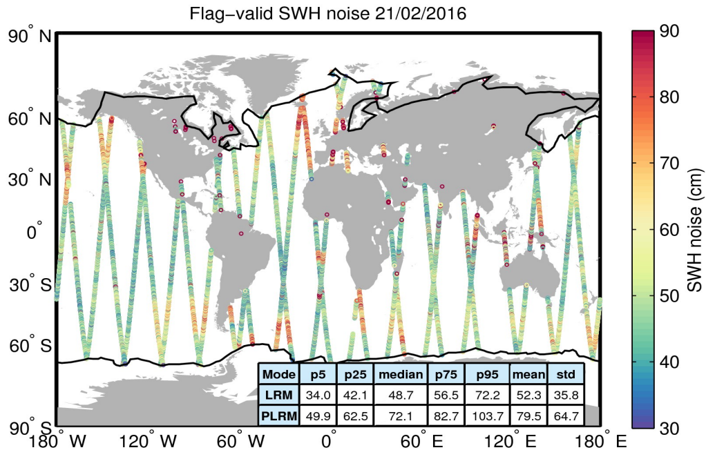
Figure 18. Geographical distribution of flag-valid 20-Hz SWH measurement noise over oceans and lakes for 21/02/2016. The statistical values shown in the table refer to the SWH noise and are calculated separately for LRM and PLRM regions. Measurements taken over polar polygons have been excluded from the computation of the statistical values. The black lines mark the outer limit of the Arctic and Antarctic polar polygons.
