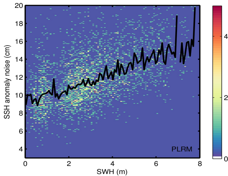
Figure 9. 2D histogram showing flag-valid SSH anomaly noise as a function of SWH for LRM (top) and PLRM (bottom) for 21/02/2016. The black line denotes the median SSH anomaly noise as a function of SWH.
