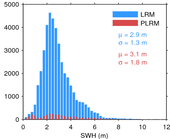
Figure 17. Histogram of flag-valid SWH over oceans and lakes for LRM (blue) and PLRM (red) for 21/02/2016. The mean ( \mu ) and standard deviation ( \sigma ) are also shown. Note that values larger than 12 m are excluded from the histogram for the sake of readability but not from the computation of \mu and \sigma .
