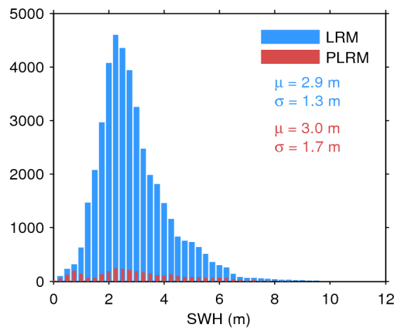
Figure 20. Histogram of science-valid SWH over oceans and lakes for LRM (blue) and PLRM (red) for 21/02/2016. The mean ( \mu ) and standard deviation ( \sigma ) are also shown. Note that values larger than 12 m are excluded from the histogram for the sake of readability but not from the computation of \mu and \sigma .
