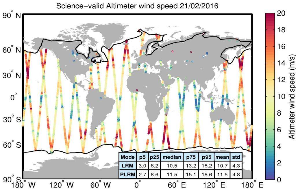
Figure 34. Geographical distribution of science-valid wind data over oceans and lakes for 21/02/2016. The statistical values shown in the table refer to the wind in m/s and are calculated separately for LRM and PLRM regions. The black lines mark the outer limit of the Arctic and Antarctic polar polygons. Gray circles denote records that have been rejected based on the editing criteria described in Table 5.
