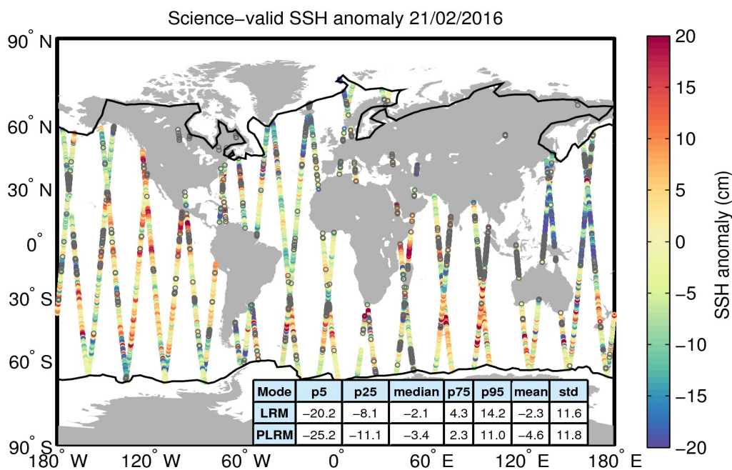
Figure 10. Geographical distribution of science-valid SSH anomaly data over oceans and lakes for 21/02/2016. The statistical values shown in the table refer to the SSH anomaly in cm and are calculated separately for LRM and PLRM regions. The black lines mark the outer limit of the Arctic and Antarctic polar polygons. Gray circles denote records that have been rejected based on the editing criteria described in Table 2.
