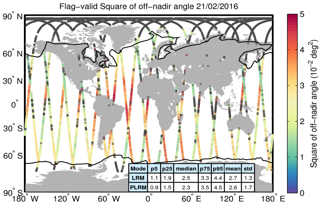
Figure 37. Geographical distribution of flag-valid mispointing data over oceans and lakes for 21/02/2016. The statistical values shown in the table refer to the mispointing in 10^{-2} deg 2 and are calculated separately for LRM and PLRM regions. Measurements taken over polar polygons have been excluded from the computation of the statistical values. The black lines mark the outer limit of the Arctic and Antarctic polar polygons. Gray circles denote negative values.
