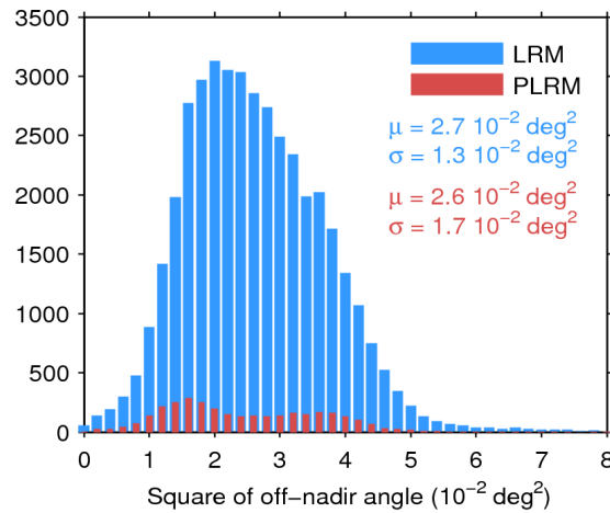
Figure 39. Histogram of flag-valid mispointing over oceans and lakes for LRM (blue) and PLRM (red) for 21/02/2016. Only positive values have been considered. The mean ( \mu ) and standard deviation ( \sigma ) are also shown. Note that values larger than 8 \cdot 10^{-2} \text{ deg}^2 are excluded from the histogram for the sake of readability but not from the computation of \mu and \sigma .
