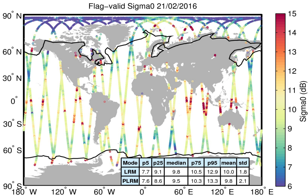
Figure 23. Geographical distribution of flag-valid sigma0 data over oceans and lakes for 21/02/2016. The statistical values shown in the table refer to the sigma0 in dB and are calculated separately for LRM and PLRM regions. Measurements taken over polar polygons have been excluded from the computation of the statistical values. The black lines mark the outer limit of the Arctic and Antarctic polar polygons.
