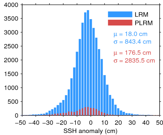
Figure 7. Histogram of flag-valid SSH anomaly over oceans and lakes for LRM (blue) and PLRM (red) for 21/02/2016. The mean ( \mu ) and standard deviation ( \sigma ) are also shown. Note that values outside [-50 50] cm are excluded from the histogram for the sake of readability but not from the computation of \mu and \sigma .
