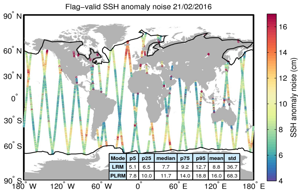
Figure 8. Geographical distribution of flag-valid 20-Hz SSH anomaly measurement noise over oceans and lakes for 21/02/2016. The statistical values shown in the table refer to the SSH anomaly noise and are calculated separately for LRM and PLRM regions. Measurements taken over polar polygons have been excluded from the computation of the statistical values. The black lines mark the outer limit of the Arctic and Antarctic polar polygons.
