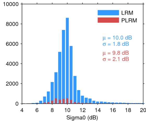
Figure 25. Histogram of flag-valid sigma0 over oceans and lakes for LRM (blue) and PLRM (red) for 21/02/2016. The mean ( \mu ) and standard deviation ( \sigma ) are also shown. Note that values outside [4 20] dB are excluded from the histogram for the sake of readability but not from the computation of \mu and \sigma .
