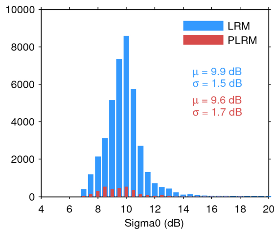
Figure 28. Histogram of science-valid sigma0 over oceans and lakes for LRM (blue) and PLRM (red) for 21/02/2016. The mean ( \mu ) and standard deviation ( \sigma ) are also shown. Note that values outside [4 20] dB are excluded from the histogram for the sake of readability but not from the computation of \mu and \sigma .
