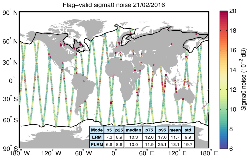
Figure 26. Geographical distribution of flag-valid 20-Hz sigma0 measurement noise over oceans and lakes for 21/02/2016. The statistical values shown in the table refer to the sigma0 noise and are calculated separately for LRM and PLRM regions. Measurements taken over polar polygons have been excluded from the computation of the statistical values. The black lines mark the outer limit of the Arctic and Antarctic polar polygons.
