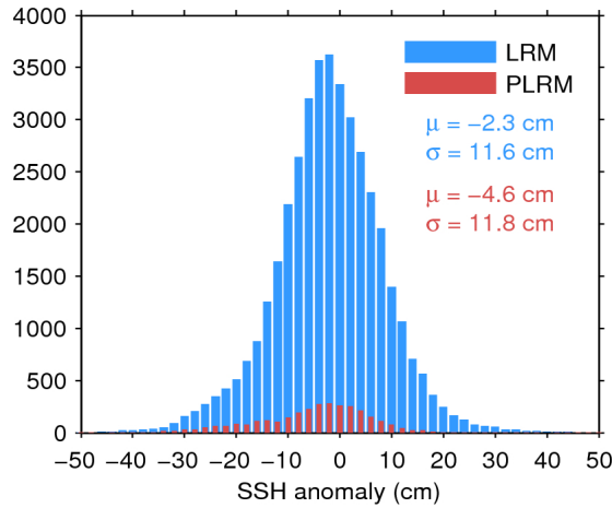
Figure 11. Histogram of science-valid SSH anomaly over oceans and lakes for LRM (blue) and PLRM (red) for 21/02/2016. The mean ( \mu ) and standard deviation ( \sigma ) are also shown. Note that values outside [-50 50] cm are excluded from the histogram for the sake of readability but not from the computation of \mu and \sigma .
