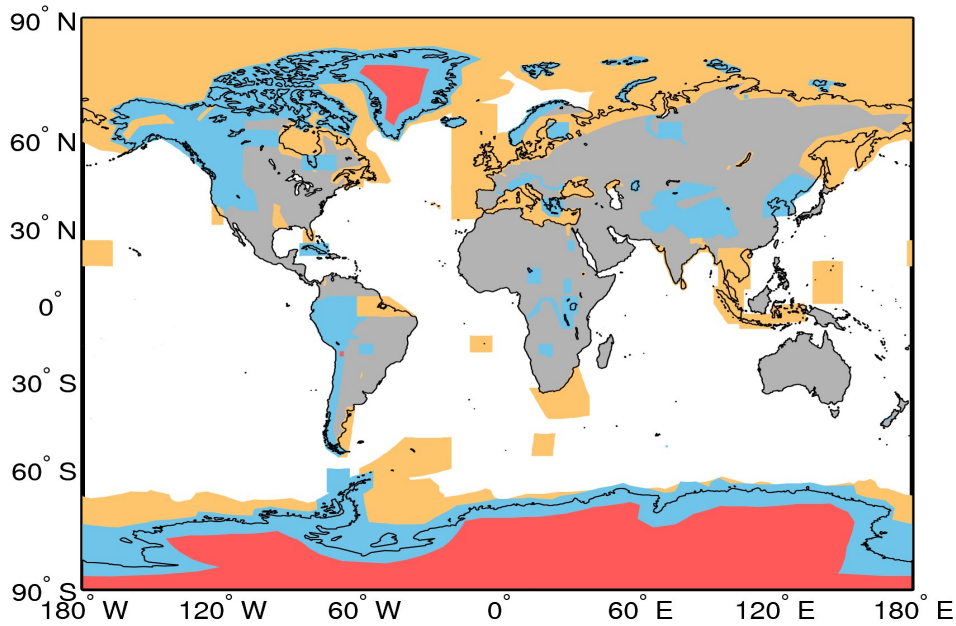
Figure A1. Extent of the regions defining the geographical mode mask for 21/02/2016. The regions where SAR, and SARIn are operated are denoted by the orange and blue polygons, respectively. LRM is operated over areas of the continental ice sheets (red polygons) and over oceans and land not covered by other modes.
