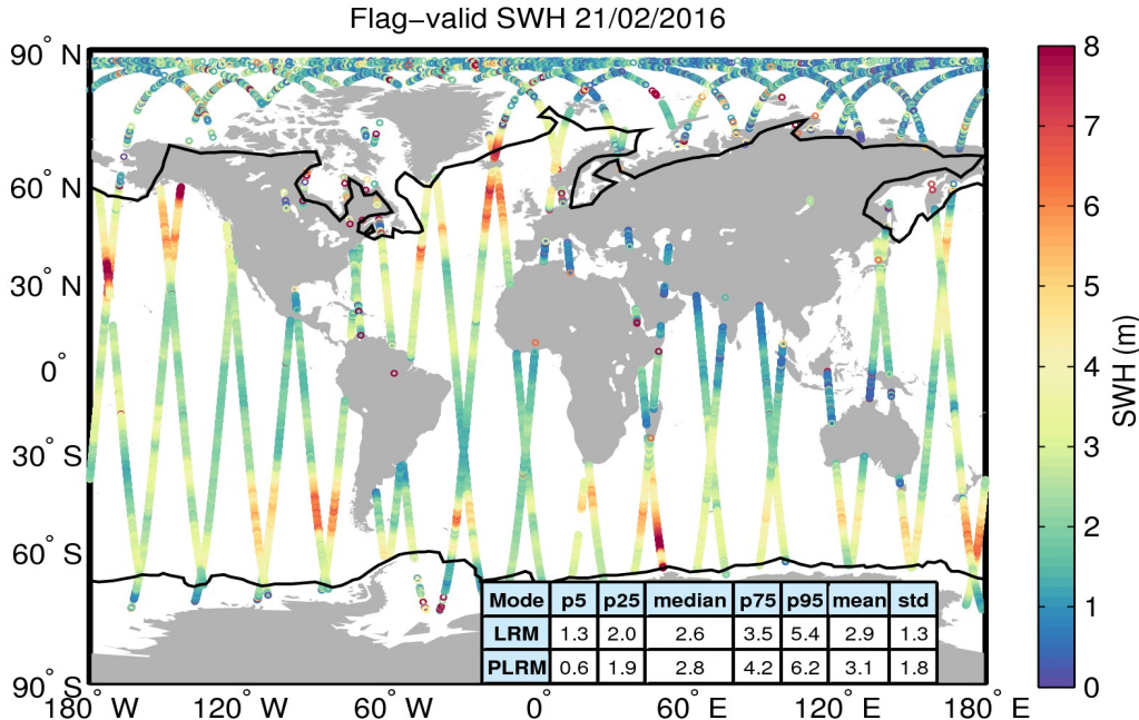
Figure 15. Geographical distribution of flag-valid SWH data over oceans and lakes for 21/02/2016. The statistical values shown in the table refer to the SWH in m and are calculated separately for LRM and PLRM regions. Measurements taken over polar polygons have been excluded from the computation of the statistical values. The black lines mark the outer limit of the Arctic and Antarctic polar polygons.
