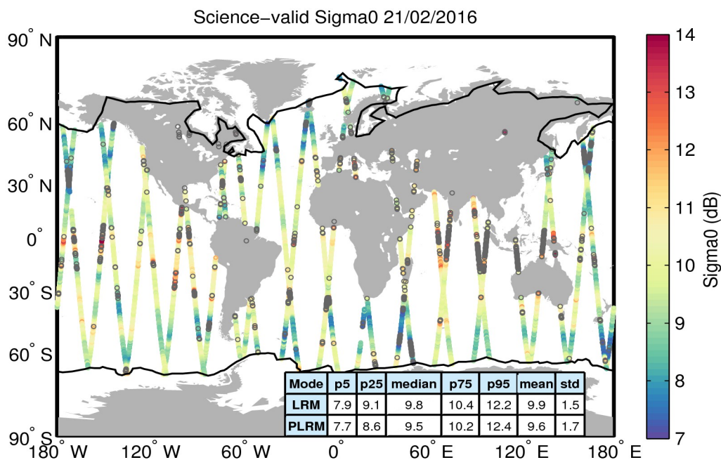
Figure 27. Geographical distribution of science-valid sigma0 data over oceans and lakes for 21/02/2016. The statistical values shown in the table refer to the sigma0 in dB and are calculated separately for LRM and PLRM regions. The black lines mark the outer limit of the Arctic and Antarctic polar polygons. Gray circles denote records that have been rejected based on the editing criteria described in Table 4.
