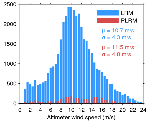
Figure 33. Histogram of flag-valid wind over oceans and lakes for LRM (blue) and PLRM (red) for 21/02/2016. The mean ( \mu ) and standard deviation ( \sigma ) are also shown. Note that values larger than 24 m/s are excluded from the histogram for the sake of readability but not from the computation of \mu and \sigma .
