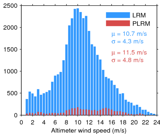
Figure 35. Histogram of science-valid wind over oceans and lakes for LRM (blue) and PLRM (red) for 21/02/2016. The mean ( \mu ) and standard deviation ( \sigma ) are also shown. Note that values larger than 24 m/s are excluded from the histogram for the sake of readability but not from the computation of \mu and \sigma .
