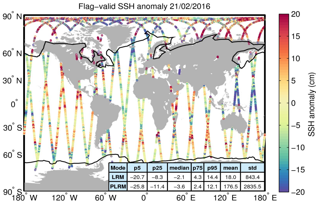
Figure 5. Geographical distribution of flag-valid 1-Hz SSH anomaly data over oceans and lakes for 21/02/2016. The statistical values shown in the table refer to the SSH anomaly in cm and are calculated separately for LRM and PLRM regions. Measurements taken over polar polygons have been excluded from the computation of the statistical values. The black lines mark the outer limit of the Arctic and Antarctic polar polygons.
