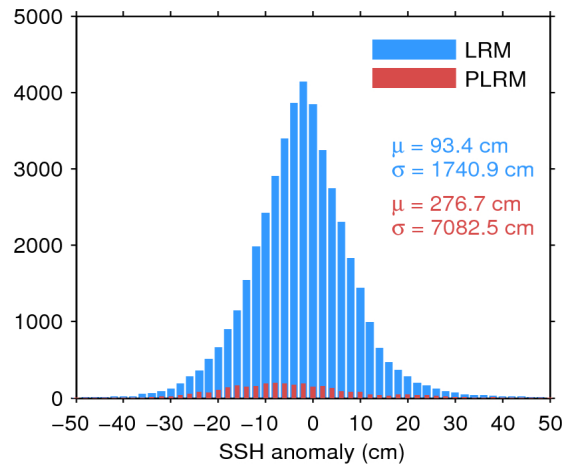
Figure 7. Histogram of flag-valid SSH anomaly over oceans and lakes for LRM (blue) and PLRM (red) for 20/02/2016. The mean ( \mu ) and standard deviation ( \sigma ) are also shown. Note that values outside [-50 50] cm are excluded from the histogram for the sake of readability but not from the computation of \mu and \sigma .
