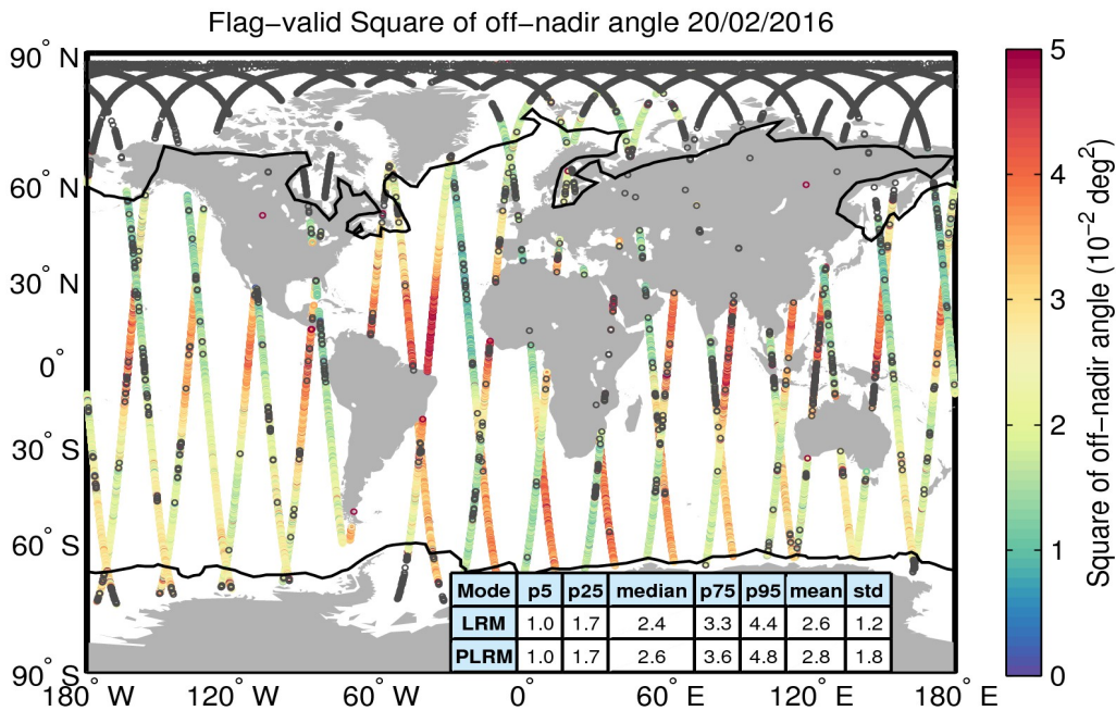
Figure 37. Geographical distribution of flag-valid mispointing data over oceans and lakes for 20/02/2016. The statistical values shown in the table refer to the mispointing in 10^{-2} deg 2 and are calculated separately for LRM and PLRM regions. Measurements taken over polar polygons have been excluded from the computation of the statistical values. The black lines mark the outer limit of the Arctic and Antarctic polar polygons. Gray circles denote negative values.
