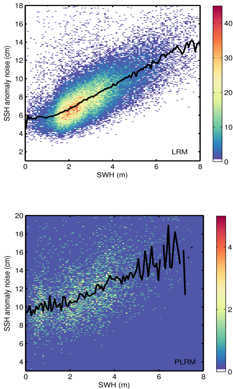
Figure 9. 2D histogram showing flag-valid SSH anomaly noise as a function of SWH for LRM (top) and PLRM (bottom) for 20/02/2016. The black line denotes the median SSH anomaly noise as a function of SWH.
