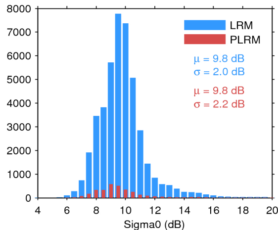
Figure 25. Histogram of flag-valid sigma0 over oceans and lakes for LRM (blue) and PLRM (red) for 20/02/2016. The mean ( \mu ) and standard deviation ( \sigma ) are also shown. Note that values outside [4 20] dB are excluded from the histogram for the sake of readability but not from the computation of \mu and \sigma .
