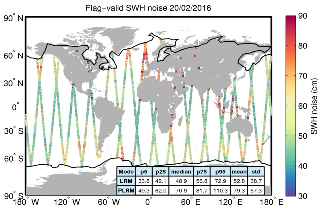
Figure 18. Geographical distribution of flag-valid 20-Hz SWH measurement noise over oceans and lakes for 20/02/2016. The statistical values shown in the table refer to the SWH noise and are calculated separately for LRM and PLRM regions. Measurements taken over polar polygons have been excluded from the computation of the statistical values. The black lines mark the outer limit of the Arctic and Antarctic polar polygons.
