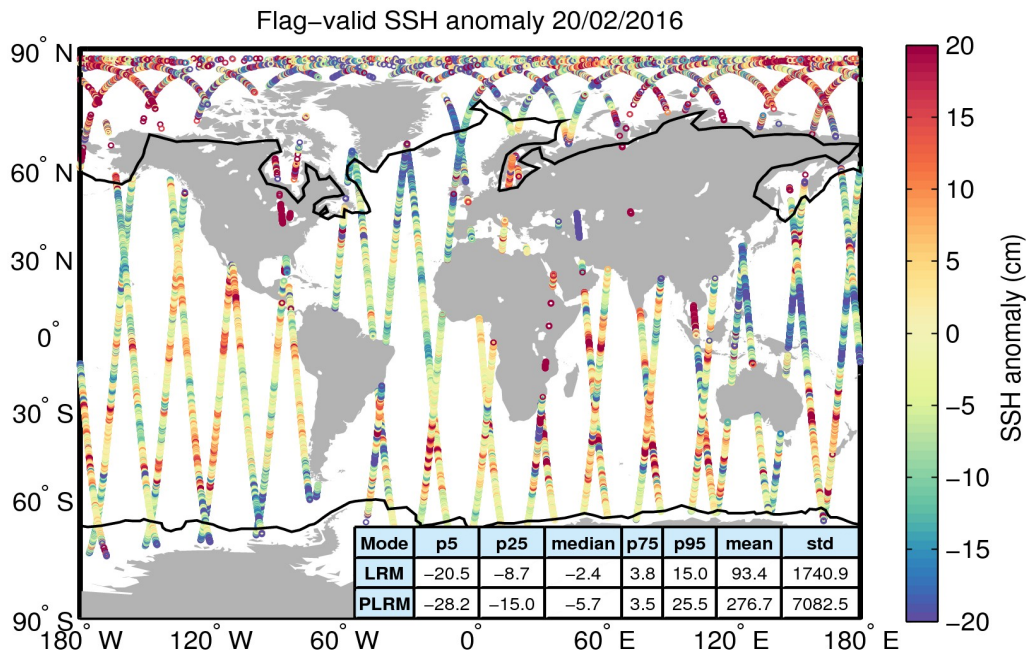
Figure 5. Geographical distribution of flag-valid 1-Hz SSH anomaly data over oceans and lakes for 20/02/2016. The statistical values shown in the table refer to the SSH anomaly in cm and are calculated separately for LRM and PLRM regions. Measurements taken over polar polygons have been excluded from the computation of the statistical values. The black lines mark the outer limit of the Arctic and Antarctic polar polygons.
