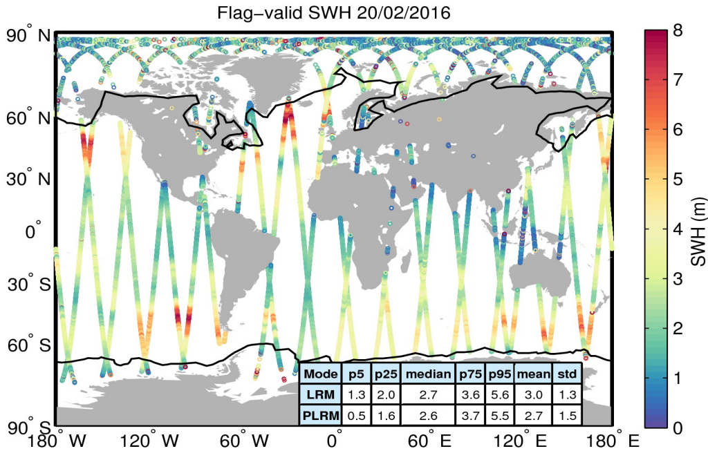
Figure 15. Geographical distribution of flag-valid SWH data over oceans and lakes for 20/02/2016. The statistical values shown in the table refer to the SWH in m and are calculated separately for LRM and PLRM regions. Measurements taken over polar polygons have been excluded from the computation of the statistical values. The black lines mark the outer limit of the Arctic and Antarctic polar polygons.
