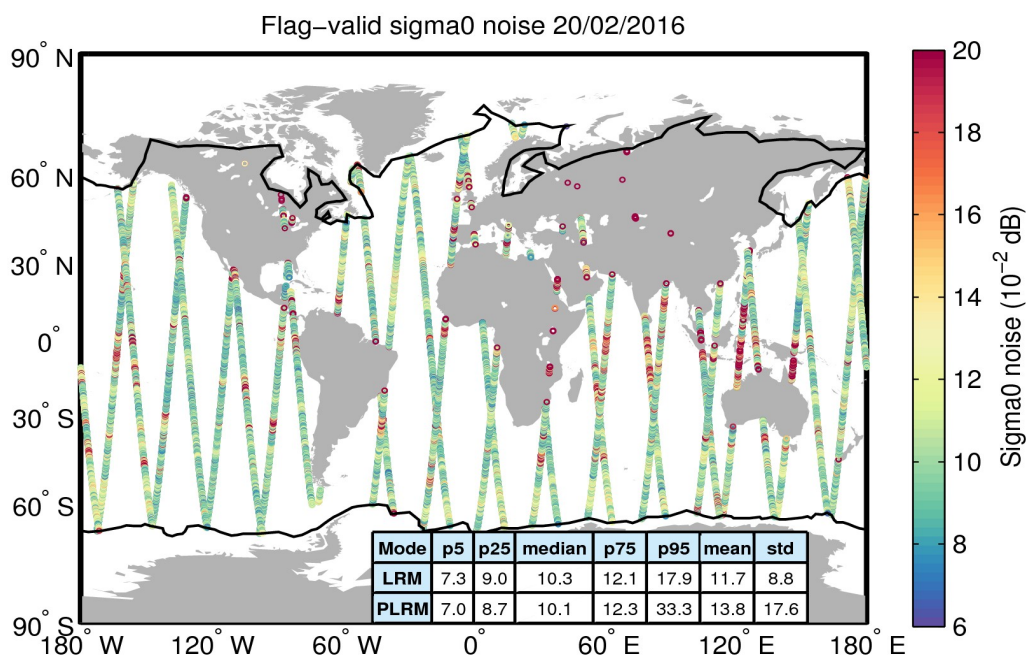
Figure 26. Geographical distribution of flag-valid 20-Hz sigma0 measurement noise over oceans and lakes for 20/02/2016. The statistical values shown in the table refer to the sigma0 noise and are calculated separately for LRM and PLRM regions. Measurements taken over polar polygons have been excluded from the computation of the statistical values. The black lines mark the outer limit of the Arctic and Antarctic polar polygons.
