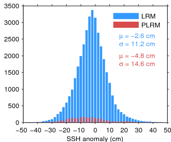
Figure 11. Histogram of science-valid SSH anomaly over oceans and lakes for LRM (blue) and PLRM (red) for 20/02/2016. The mean ( \mu ) and standard deviation ( \sigma ) are also shown. Note that values outside [-50 50] cm are excluded from the histogram for the sake of readability but not from the computation of \mu and \sigma .
