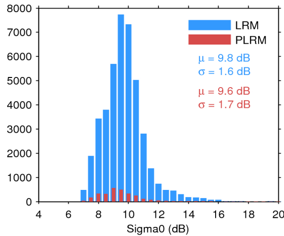
Figure 28. Histogram of science-valid sigma0 over oceans and lakes for LRM (blue) and PLRM (red) for 20/02/2016. The mean ( \mu ) and standard deviation ( \sigma ) are also shown. Note that values outside [4 20] dB are excluded from the histogram for the sake of readability but not from the computation of \mu and \sigma .
