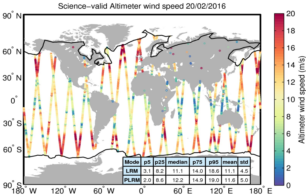
Figure 34. Geographical distribution of science-valid wind data over oceans and lakes for 20/02/2016. The statistical values shown in the table refer to the wind in m/s and are calculated separately for LRM and PLRM regions. The black lines mark the outer limit of the Arctic and Antarctic polar polygons. Gray circles denote records that have been rejected based on the editing criteria described in Table 5.
