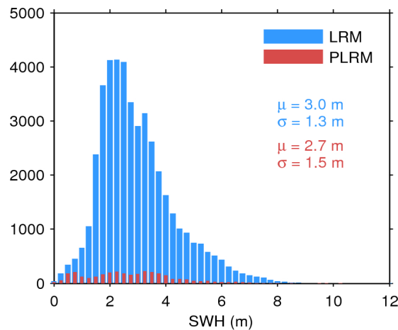
Figure 17. Histogram of flag-valid SWH over oceans and lakes for LRM (blue) and PLRM (red) for 20/02/2016. The mean ( \mu ) and standard deviation ( \sigma ) are also shown. Note that values larger than 12 m are excluded from the histogram for the sake of readability but not from the computation of \mu and \sigma .
