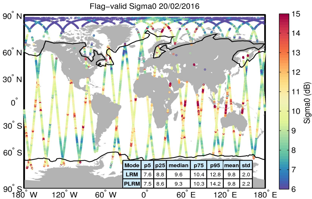
Figure 23. Geographical distribution of flag-valid sigma0 data over oceans and lakes for 20/02/2016. The statistical values shown in the table refer to the sigma0 in dB and are calculated separately for LRM and PLRM regions. Measurements taken over polar polygons have been excluded from the computation of the statistical values. The black lines mark the outer limit of the Arctic and Antarctic polar polygons.
