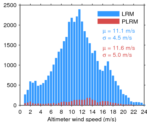
Figure 35. Histogram of science-valid wind over oceans and lakes for LRM (blue) and PLRM (red) for 20/02/2016. The mean ( \mu ) and standard deviation ( \sigma ) are also shown. Note that values larger than 24 m/s are excluded from the histogram for the sake of readability but not from the computation of \mu and \sigma .
