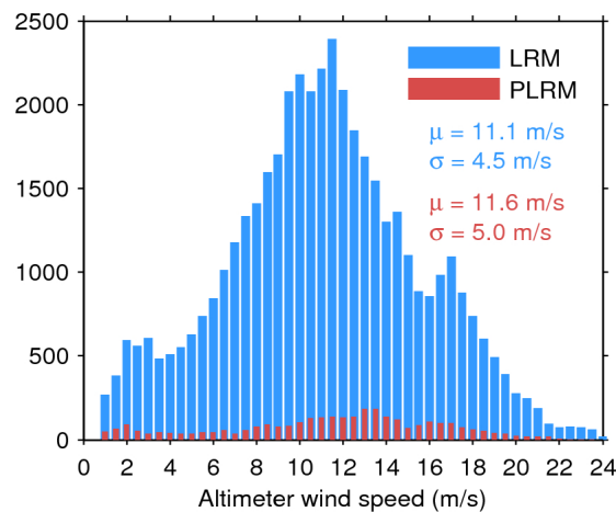
Figure 33. Histogram of flag-valid wind over oceans and lakes for LRM (blue) and PLRM (red) for 20/02/2016. The mean ( \mu ) and standard deviation ( \sigma ) are also shown. Note that values larger than 24 m/s are excluded from the histogram for the sake of readability but not from the computation of \mu and \sigma .
