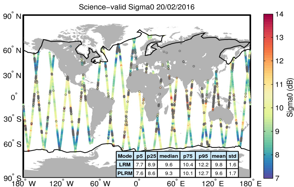
Figure 27. Geographical distribution of science-valid sigma0 data over oceans and lakes for 20/02/2016. The statistical values shown in the table refer to the sigma0 in dB and are calculated separately for LRM and PLRM regions. The black lines mark the outer limit of the Arctic and Antarctic polar polygons. Gray circles denote records that have been rejected based on the editing criteria described in Table 4.
