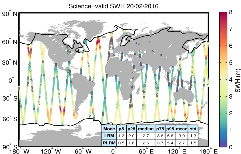
Figure 19. Geographical distribution of science-valid SWH data over oceans and lakes for 20/02/2016. The statistical values shown in the table refer to the SWH in m and are calculated separately for LRM and PLRM regions. The black lines mark the outer limit of the Arctic and Antarctic polar polygons. Gray circles denote records that have been rejected based on the editing criteria described in Table 3.
