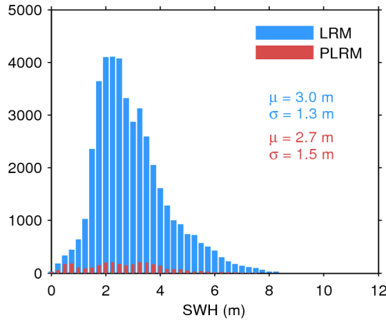
Figure 20. Histogram of science-valid SWH over oceans and lakes for LRM (blue) and PLRM (red) for 20/02/2016. The mean ( \mu ) and standard deviation ( \sigma ) are also shown. Note that values larger than 12 m are excluded from the histogram for the sake of readability but not from the computation of \mu and \sigma .
