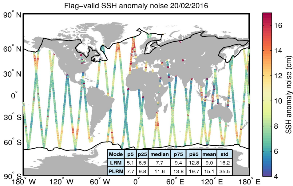
Figure 8. Geographical distribution of flag-valid 20-Hz SSH anomaly measurement noise over oceans and lakes for 20/02/2016. The statistical values shown in the table refer to the SSH anomaly noise and are calculated separately for LRM and PLRM regions. Measurements taken over polar polygons have been excluded from the computation of the statistical values. The black lines mark the outer limit of the Arctic and Antarctic polar polygons.
