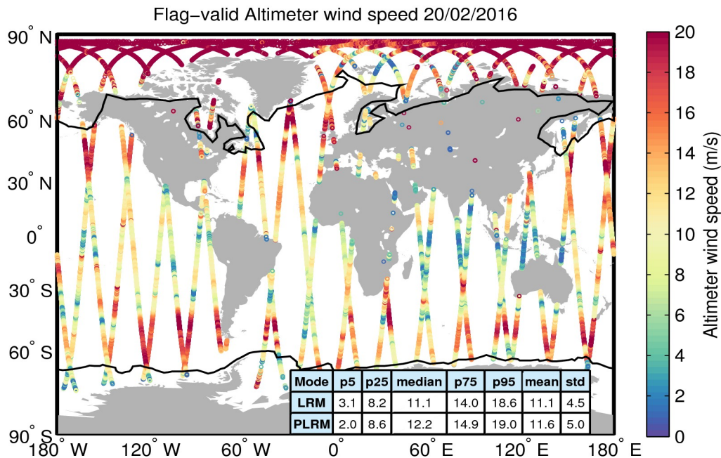
Figure 31. Geographical distribution of flag-valid wind data over oceans and lakes for 20/02/2016. The statistical values shown in the table refer to the wind in m/s and are calculated separately for LRM and PLRM regions. Measurements taken over polar polygons have been excluded from the computation of the statistical values. The black lines mark the outer limit of the Arctic and Antarctic polar polygons.
