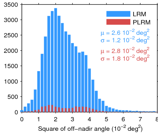
Figure 39. Histogram of flag-valid mispointing over oceans and lakes for LRM (blue) and PLRM (red) for 20/02/2016. Only positive values have been considered. The mean ( \mu ) and standard deviation ( \sigma ) are also shown. Note that values larger than 8 \cdot 10^{-2} \text{ deg}^2 are excluded from the histogram for the sake of readability but not from the computation of \mu and \sigma .
