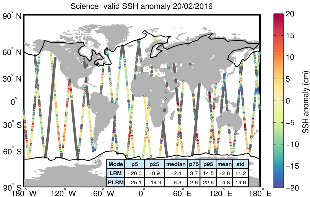
Figure 10. Geographical distribution of science-valid SSH anomaly data over oceans and lakes for 20/02/2016. The statistical values shown in the table refer to the SSH anomaly in cm and are calculated separately for LRM and PLRM regions. The black lines mark the outer limit of the Arctic and Antarctic polar polygons. Gray circles denote records that have been rejected based on the editing criteria described in Table 2.
