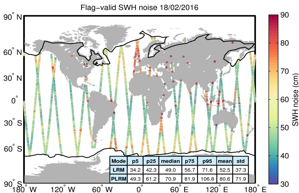
Figure 18. Geographical distribution of flag-valid 20-Hz SWH measurement noise over oceans and lakes for 18/02/2016. The statistical values shown in the table refer to the SWH noise and are calculated separately for LRM and PLRM regions. Measurements taken over polar polygons have been excluded from the computation of the statistical values. The black lines mark the outer limit of the Arctic and Antarctic polar polygons.
