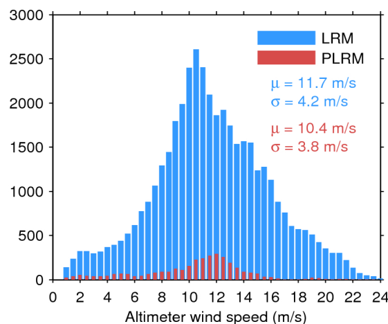
Figure 35. Histogram of science-valid wind over oceans and lakes for LRM (blue) and PLRM (red) for 18/02/2016. The mean ( \mu ) and standard deviation ( \sigma ) are also shown. Note that values larger than 24 m/s are excluded from the histogram for the sake of readability but not from the computation of \mu and \sigma .
