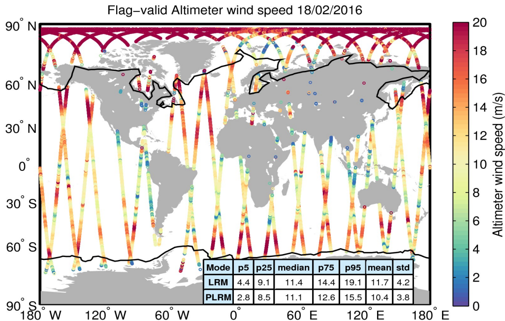
Figure 31. Geographical distribution of flag-valid wind data over oceans and lakes for 18/02/2016. The statistical values shown in the table refer to the wind in m/s and are calculated separately for LRM and PLRM regions. Measurements taken over polar polygons have been excluded from the computation of the statistical values. The black lines mark the outer limit of the Arctic and Antarctic polar polygons.
