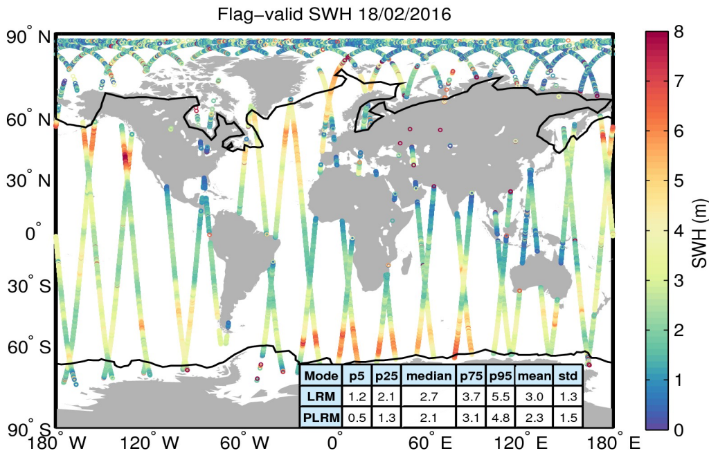
Figure 15. Geographical distribution of flag-valid SWH data over oceans and lakes for 18/02/2016. The statistical values shown in the table refer to the SWH in m and are calculated separately for LRM and PLRM regions. Measurements taken over polar polygons have been excluded from the computation of the statistical values. The black lines mark the outer limit of the Arctic and Antarctic polar polygons.
