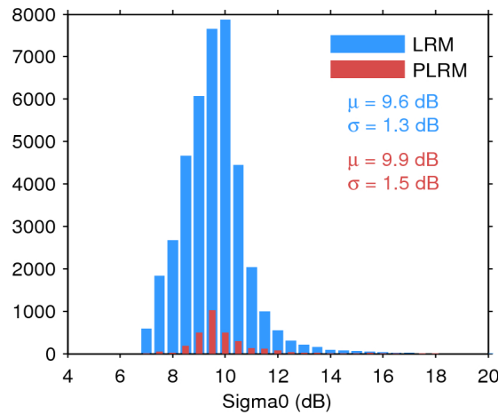
Figure 28. Histogram of science-valid sigma0 over oceans and lakes for LRM (blue) and PLRM (red) for 18/02/2016. The mean ( \mu ) and standard deviation ( \sigma ) are also shown. Note that values outside [4 20] dB are excluded from the histogram for the sake of readability but not from the computation of \mu and \sigma .
