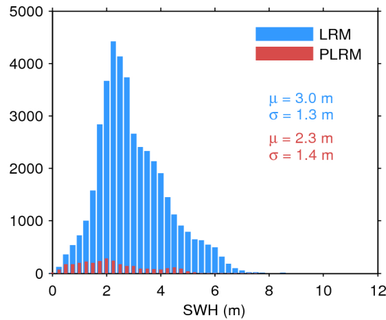
Figure 20. Histogram of science-valid SWH over oceans and lakes for LRM (blue) and PLRM (red) for 18/02/2016. The mean ( \mu ) and standard deviation ( \sigma ) are also shown. Note that values larger than 12 m are excluded from the histogram for the sake of readability but not from the computation of \mu and \sigma .
