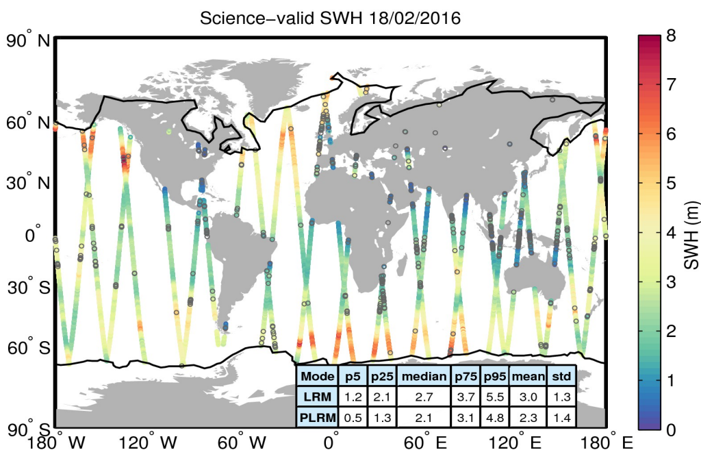
Figure 19. Geographical distribution of science-valid SWH data over oceans and lakes for 18/02/2016. The statistical values shown in the table refer to the SWH in m and are calculated separately for LRM and PLRM regions. The black lines mark the outer limit of the Arctic and Antarctic polar polygons. Gray circles denote records that have been rejected based on the editing criteria described in Table 3.
