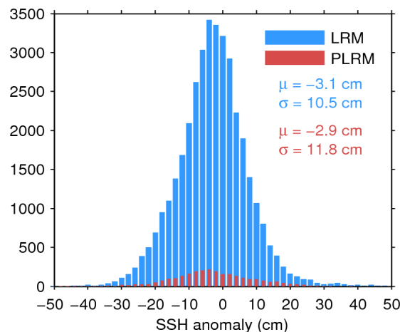
Figure 11. Histogram of science-valid SSH anomaly over oceans and lakes for LRM (blue) and PLRM (red) for 18/02/2016. The mean ( \mu ) and standard deviation ( \sigma ) are also shown. Note that values outside [-50 50] cm are excluded from the histogram for the sake of readability but not from the computation of \mu and \sigma .
