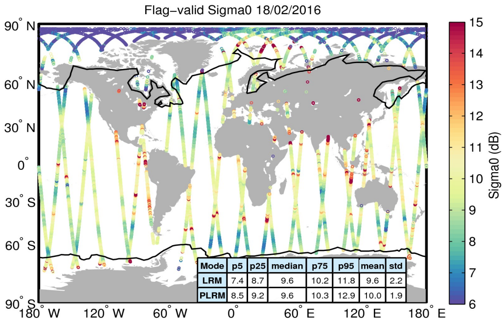
Figure 23. Geographical distribution of flag-valid sigma0 data over oceans and lakes for 18/02/2016. The statistical values shown in the table refer to the sigma0 in dB and are calculated separately for LRM and PLRM regions. Measurements taken over polar polygons have been excluded from the computation of the statistical values. The black lines mark the outer limit of the Arctic and Antarctic polar polygons.
