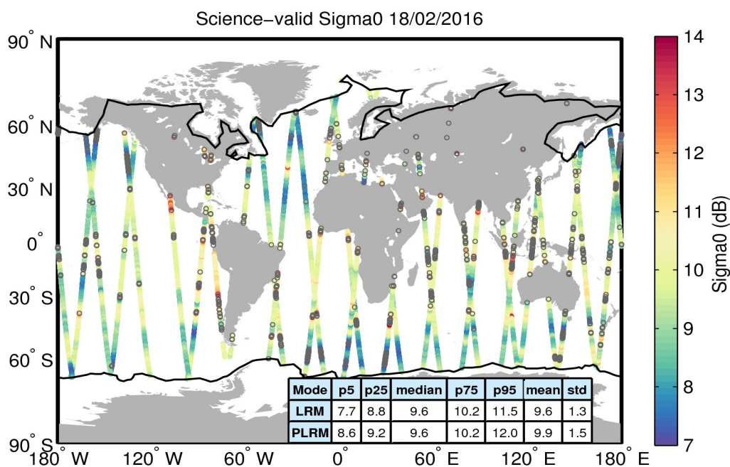
Figure 27. Geographical distribution of science-valid sigma0 data over oceans and lakes for 18/02/2016. The statistical values shown in the table refer to the sigma0 in dB and are calculated separately for LRM and PLRM regions. The black lines mark the outer limit of the Arctic and Antarctic polar polygons. Gray circles denote records that have been rejected based on the editing criteria described in Table 4.
