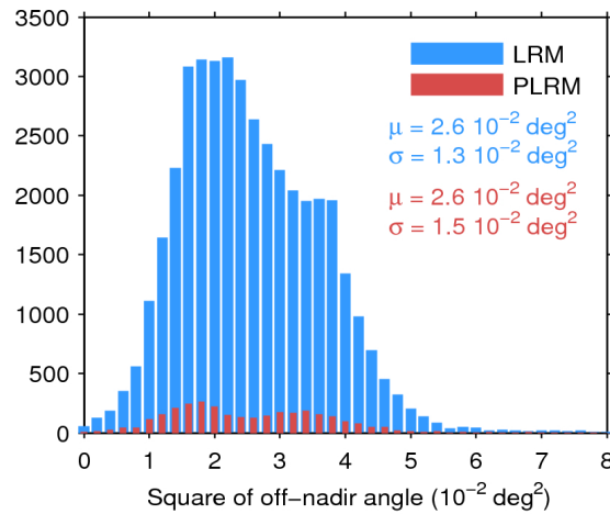
Figure 39. Histogram of flag-valid mispointing over oceans and lakes for LRM (blue) and PLRM (red) for 18/02/2016. Only positive values have been considered. The mean ( \mu ) and standard deviation ( \sigma ) are also shown. Note that values larger than 8 \cdot 10^{-2} \text{ deg}^2 are excluded from the histogram for the sake of readability but not from the computation of \mu and \sigma .
