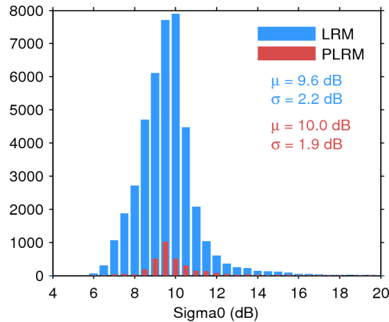
Figure 25. Histogram of flag-valid sigma0 over oceans and lakes for LRM (blue) and PLRM (red) for 18/02/2016. The mean ( \mu ) and standard deviation ( \sigma ) are also shown. Note that values outside [4 20] dB are excluded from the histogram for the sake of readability but not from the computation of \mu and \sigma .
