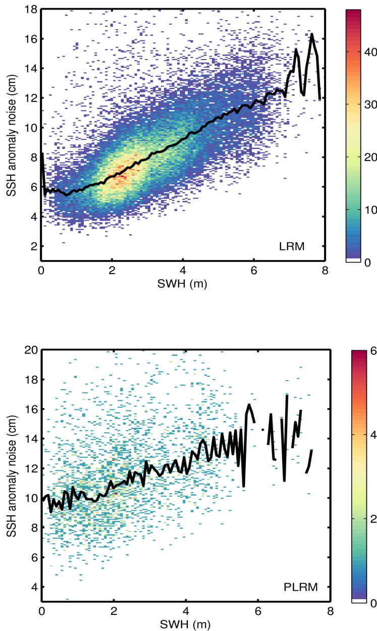
Figure 9. 2D histogram showing flag-valid SSH anomaly noise as a function of SWH for LRM (top) and PLRM (bottom) for 18/02/2016. The black line denotes the median SSH anomaly noise as a function of SWH.
