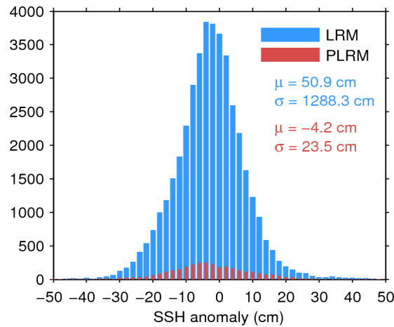
Figure 7. Histogram of flag-valid SSH anomaly over oceans and lakes for LRM (blue) and PLRM (red) for 18/02/2016. The mean ( \mu ) and standard deviation ( \sigma ) are also shown. Note that values outside [-50 50] cm are excluded from the histogram for the sake of readability but not from the computation of \mu and \sigma .
