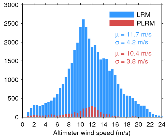
Figure 33. Histogram of flag-valid wind over oceans and lakes for LRM (blue) and PLRM (red) for 18/02/2016. The mean ( \mu ) and standard deviation ( \sigma ) are also shown. Note that values larger than 24 m/s are excluded from the histogram for the sake of readability but not from the computation of \mu and \sigma .
