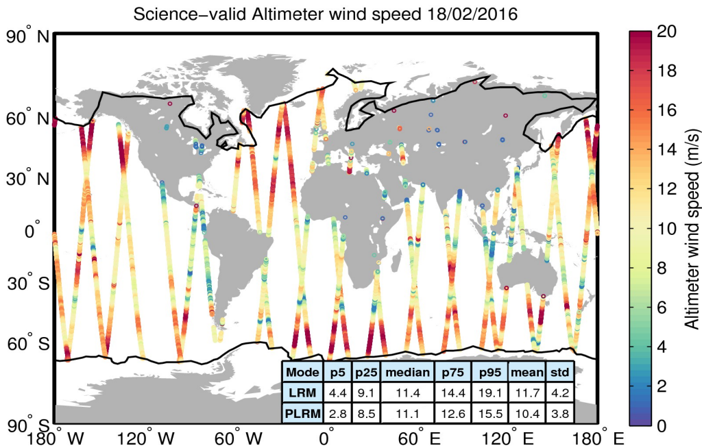
Figure 34. Geographical distribution of science-valid wind data over oceans and lakes for 18/02/2016. The statistical values shown in the table refer to the wind in m/s and are calculated separately for LRM and PLRM regions. The black lines mark the outer limit of the Arctic and Antarctic polar polygons. Gray circles denote records that have been rejected based on the editing criteria described in Table 5.
