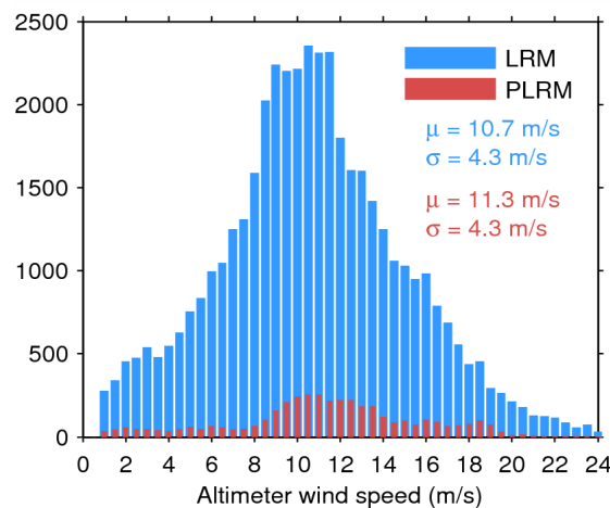
Figure 35. Histogram of science-valid wind over oceans and lakes for LRM (blue) and PLRM (red) for 09/02/2016. The mean ( \mu ) and standard deviation ( \sigma ) are also shown. Note that values larger than 24 m/s are excluded from the histogram for the sake of readability but not from the computation of \mu and \sigma .
