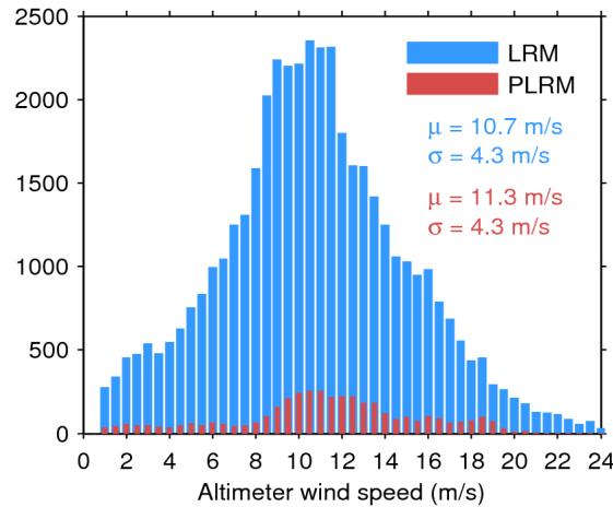
Figure 33. Histogram of flag-valid wind over oceans and lakes for LRM (blue) and PLRM (red) for 09/02/2016. The mean ( \mu ) and standard deviation ( \sigma ) are also shown. Note that values larger than 24 m/s are excluded from the histogram for the sake of readability but not from the computation of \mu and \sigma .
