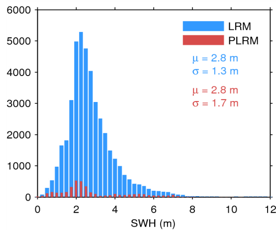
Figure 20. Histogram of science-valid SWH over oceans and lakes for LRM (blue) and PLRM (red) for 09/02/2016. The mean ( \mu ) and standard deviation ( \sigma ) are also shown. Note that values larger than 12 m are excluded from the histogram for the sake of readability but not from the computation of \mu and \sigma .
