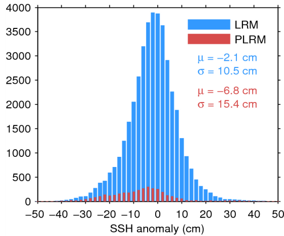
Figure 11. Histogram of science-valid SSH anomaly over oceans and lakes for LRM (blue) and PLRM (red) for 09/02/2016. The mean ( \mu ) and standard deviation ( \sigma ) are also shown. Note that values outside [-50\ 50] cm are excluded from the histogram for the sake of readability but not from the computation of \mu and \sigma .
