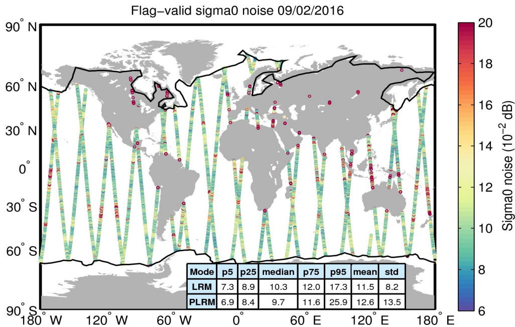
Figure 26. Geographical distribution of flag-valid 20-Hz sigma0 measurement noise over oceans and lakes for 09/02/2016. The statistical values shown in the table refer to the sigma0 noise and are calculated separately for LRM and PLRM regions. Measurements taken over polar polygons have been excluded from the computation of the statistical values. The black lines mark the outer limit of the Arctic and Antarctic polar polygons.
