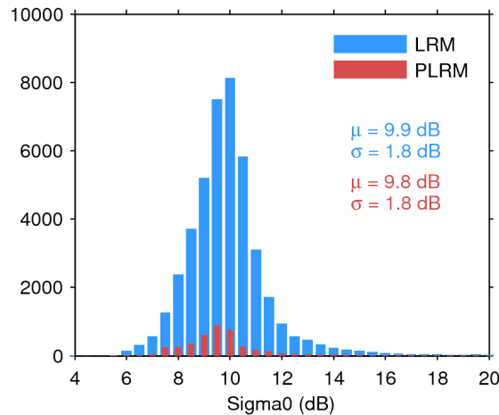
Figure 25. Histogram of flag-valid sigma0 over oceans and lakes for LRM (blue) and PLRM (red) for 09/02/2016. The mean ( \mu ) and standard deviation ( \sigma ) are also shown. Note that values outside [4 20] dB are excluded from the histogram for the sake of readability but not from the computation of \mu and \sigma .
