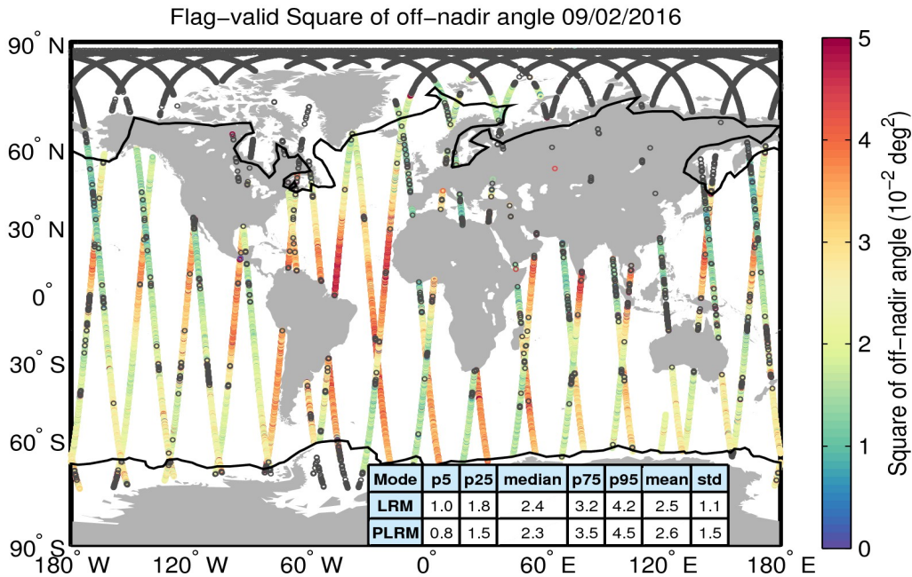
Figure 37. Geographical distribution of flag-valid mispointing data over oceans and lakes for 09/02/2016. The statistical values shown in the table refer to the mispointing in 10^{-2} deg 2 and are calculated separately for LRM and PLRM regions. Measurements taken over polar polygons have been excluded from the computation of the statistical values. The black lines mark the outer limit of the Arctic and Antarctic polar polygons. Gray circles denote negative values.
