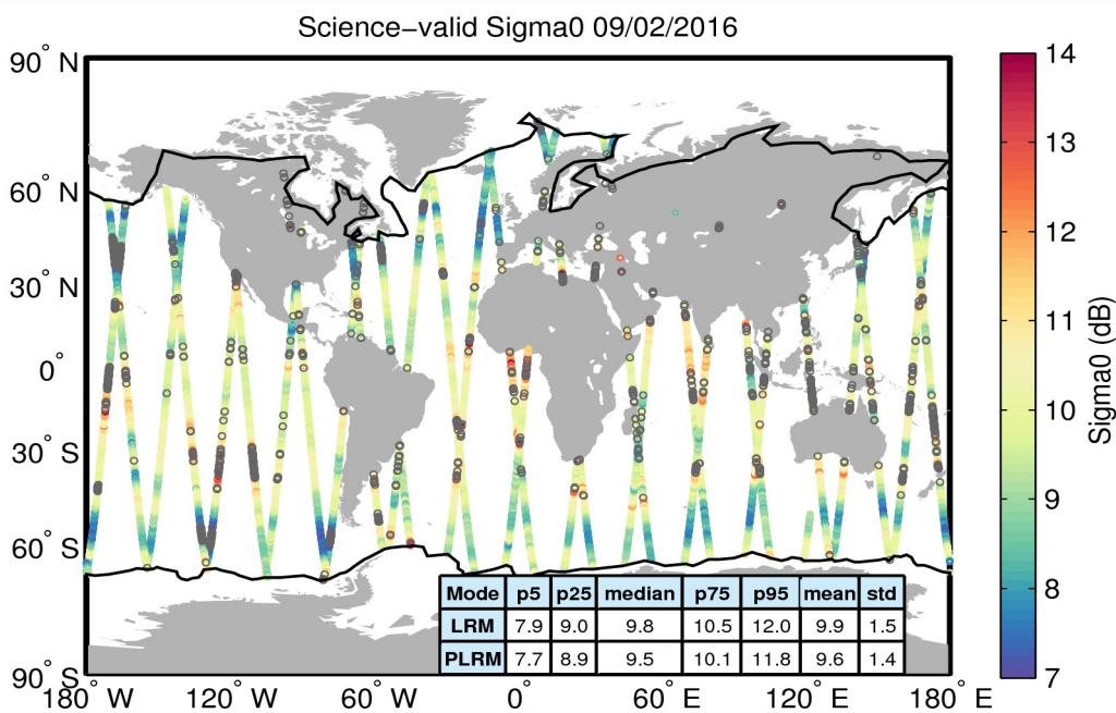
Figure 27. Geographical distribution of science-valid sigma0 data over oceans and lakes for 09/02/2016. The statistical values shown in the table refer to the sigma0 in dB and are calculated separately for LRM and PLRM regions. The black lines mark the outer limit of the Arctic and Antarctic polar polygons. Gray circles denote records that have been rejected based on the editing criteria described in Table 4.
