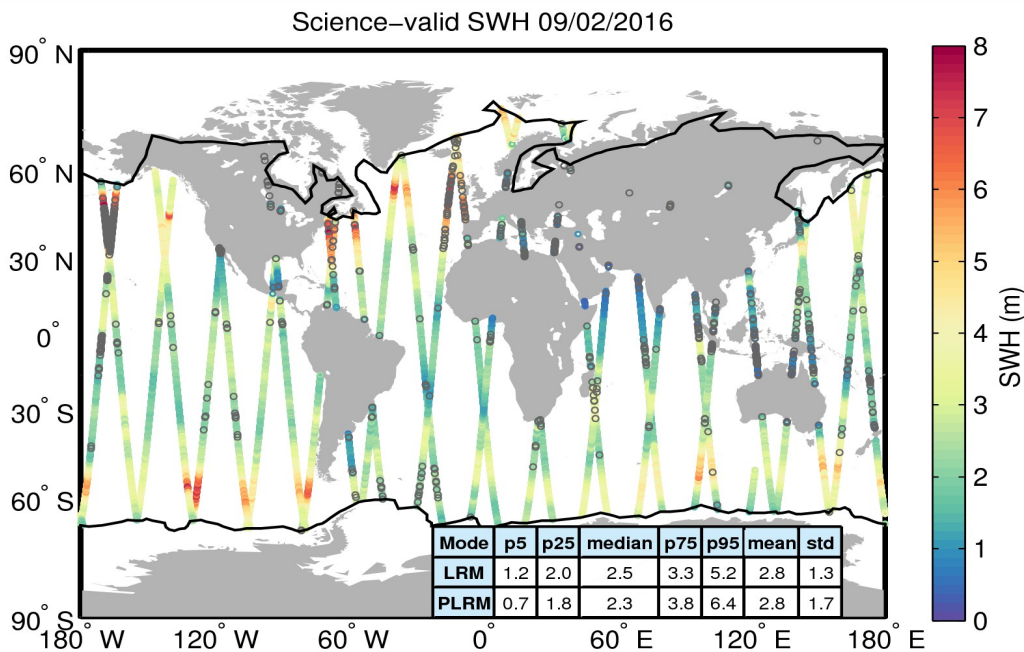
Figure 19. Geographical distribution of science-valid SWH data over oceans and lakes for 09/02/2016. The statistical values shown in the table refer to the SWH in m and are calculated separately for LRM and PLRM regions. The black lines mark the outer limit of the Arctic and Antarctic polar polygons. Gray circles denote records that have been rejected based on the editing criteria described in Table 3.
