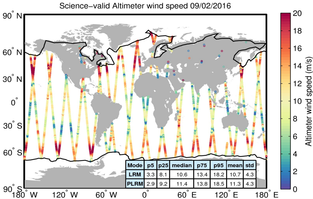
Figure 34. Geographical distribution of science-valid wind data over oceans and lakes for 09/02/2016. The statistical values shown in the table refer to the wind in m/s and are calculated separately for LRM and PLRM regions. The black lines mark the outer limit of the Arctic and Antarctic polar polygons. Gray circles denote records that have been rejected based on the editing criteria described in Table 5.
