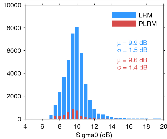
Figure 28. Histogram of science-valid sigma0 over oceans and lakes for LRM (blue) and PLRM (red) for 09/02/2016. The mean ( \mu ) and standard deviation ( \sigma ) are also shown. Note that values outside [4 20] dB are excluded from the histogram for the sake of readability but not from the computation of \mu and \sigma .
