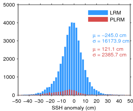
Figure 7. Histogram of flag-valid SSH anomaly over oceans and lakes for LRM (blue) and PLRM (red) for 09/02/2016. The mean ( \mu ) and standard deviation ( \sigma ) are also shown. Note that values outside [-50\ 50] cm are excluded from the histogram for the sake of readability but not from the computation of \mu and \sigma .
