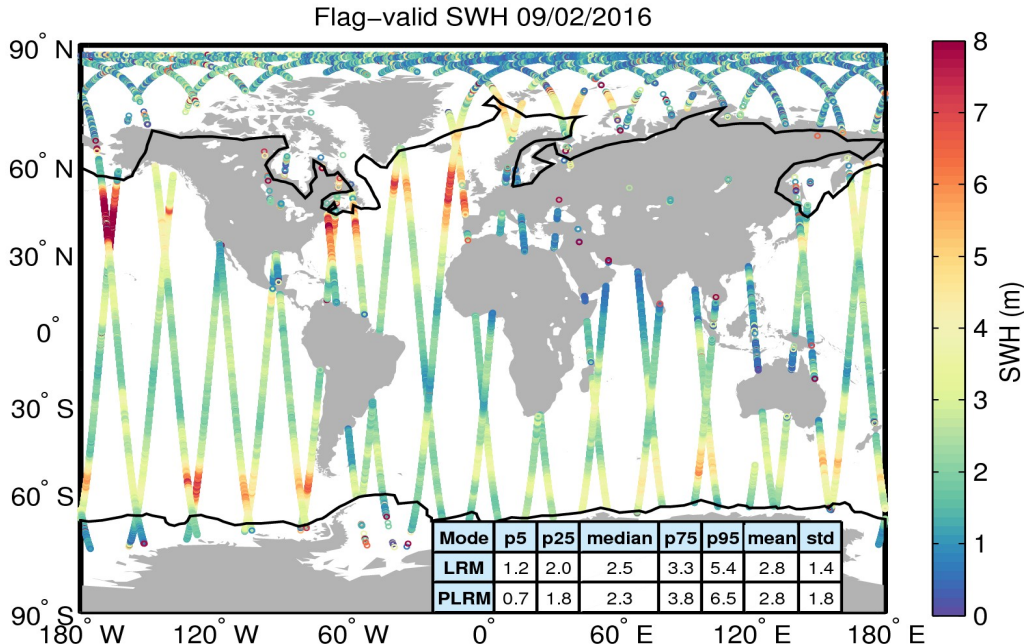
Figure 15. Geographical distribution of flag-valid SWH data over oceans and lakes for 09/02/2016. The statistical values shown in the table refer to the SWH in m and are calculated separately for LRM and PLRM regions. Measurements taken over polar polygons have been excluded from the computation of the statistical values. The black lines mark the outer limit of the Arctic and Antarctic polar polygons.
