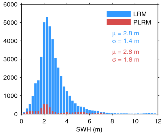
Figure 17. Histogram of flag-valid SWH over oceans and lakes for LRM (blue) and PLRM (red) for 09/02/2016. The mean ( \mu ) and standard deviation ( \sigma ) are also shown. Note that values larger than 12 m are excluded from the histogram for the sake of readability but not from the computation of \mu and \sigma .
