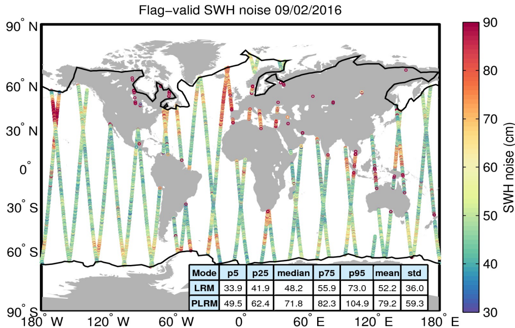
Figure 18. Geographical distribution of flag-valid 20-Hz SWH measurement noise over oceans and lakes for 09/02/2016. The statistical values shown in the table refer to the SWH noise and are calculated separately for LRM and PLRM regions. Measurements taken over polar polygons have been excluded from the computation of the statistical values. The black lines mark the outer limit of the Arctic and Antarctic polar polygons.
