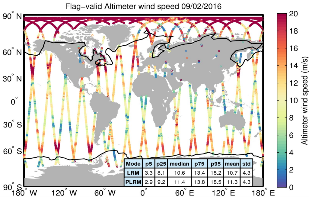
Figure 31. Geographical distribution of flag-valid wind data over oceans and lakes for 09/02/2016. The statistical values shown in the table refer to the wind in m/s and are calculated separately for LRM and PLRM regions. Measurements taken over polar polygons have been excluded from the computation of the statistical values. The black lines mark the outer limit of the Arctic and Antarctic polar polygons.
