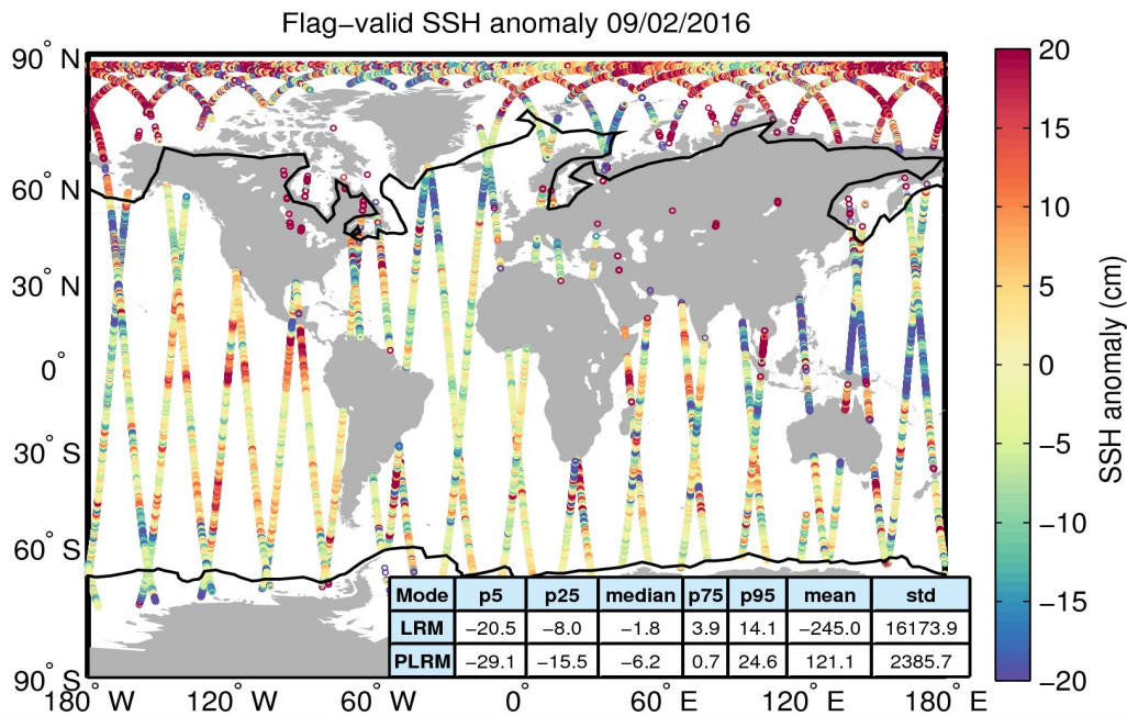
Figure 5. Geographical distribution of flag-valid 1-Hz SSH anomaly data over oceans and lakes for 09/02/2016. The statistical values shown in the table refer to the SSH anomaly in cm and are calculated separately for LRM and PLRM regions. Measurements taken over polar polygons have been excluded from the computation of the statistical values. The black lines mark the outer limit of the Arctic and Antarctic polar polygons.
