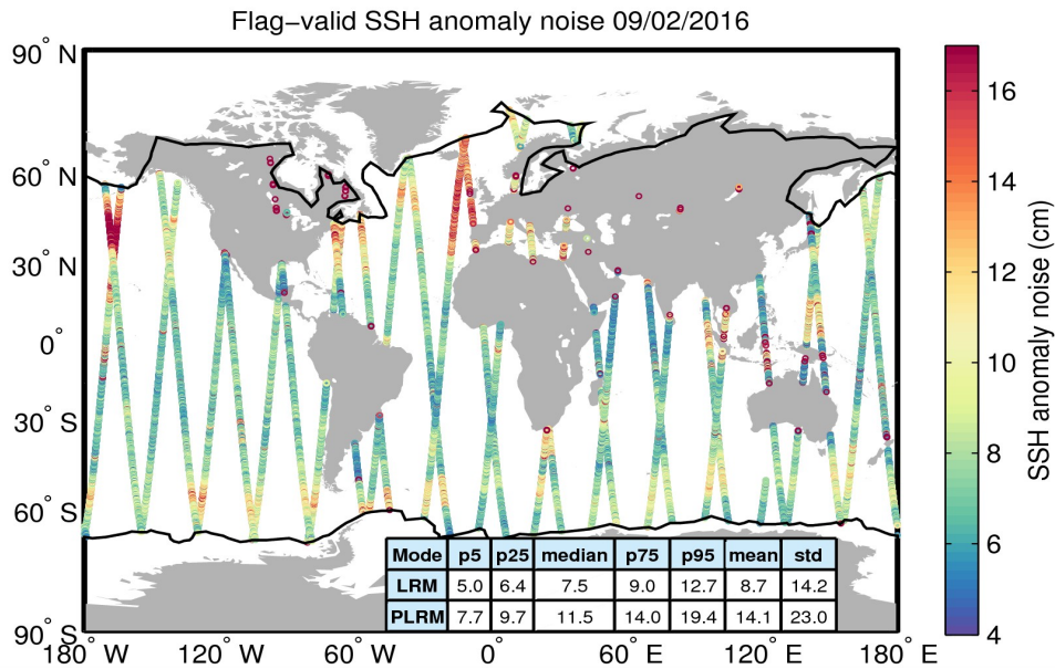
Figure 8. Geographical distribution of flag-valid 20-Hz SSH anomaly measurement noise over oceans and lakes for 09/02/2016. The statistical values shown in the table refer to the SSH anomaly noise and are calculated separately for LRM and PLRM regions. Measurements taken over polar polygons have been excluded from the computation of the statistical values. The black lines mark the outer limit of the Arctic and Antarctic polar polygons.
