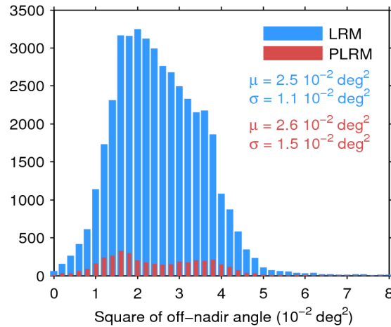
Figure 39. Histogram of flag-valid mispointing over oceans and lakes for LRM (blue) and PLRM (red) for 09/02/2016. Only positive values have been considered. The mean ( \mu ) and standard deviation ( \sigma ) are also shown. Note that values larger than 8 \cdot 10^{-2} \text{ deg}^2 are excluded from the histogram for the sake of readability but not from the computation of \mu and \sigma .
