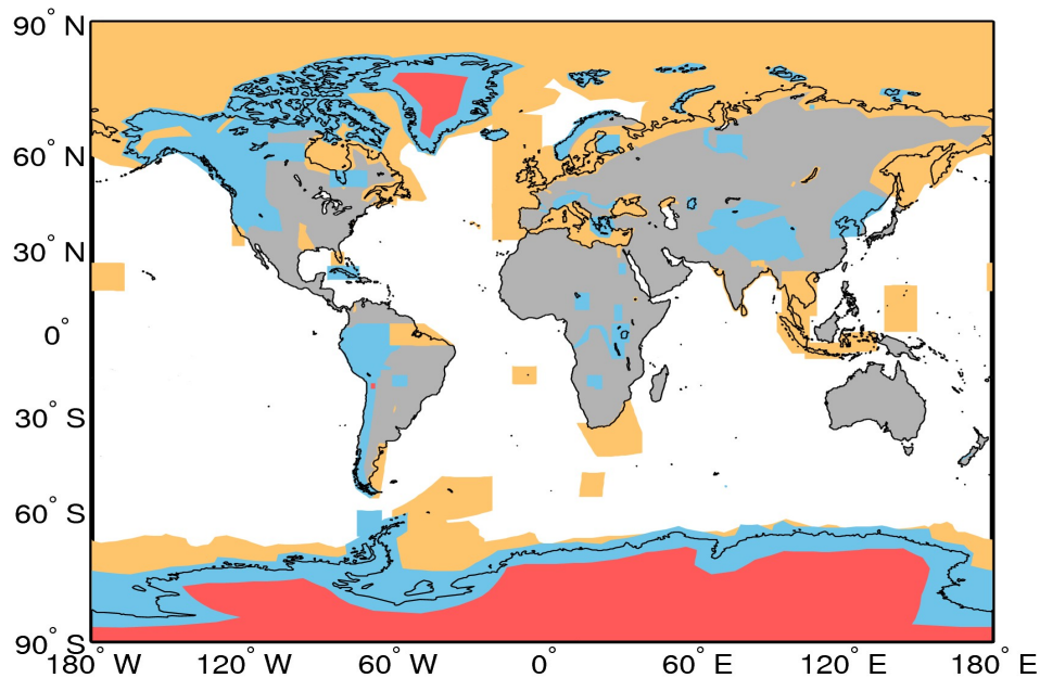
Figure A1. Extent of the regions defining the geographical mode mask for 09/02/2016. The regions where SAR, and SARIn are operated are denoted by the orange and blue polygons, respectively. LRM is operated over areas of the continental ice sheets (red polygons) and over oceans and land not covered by other modes.
