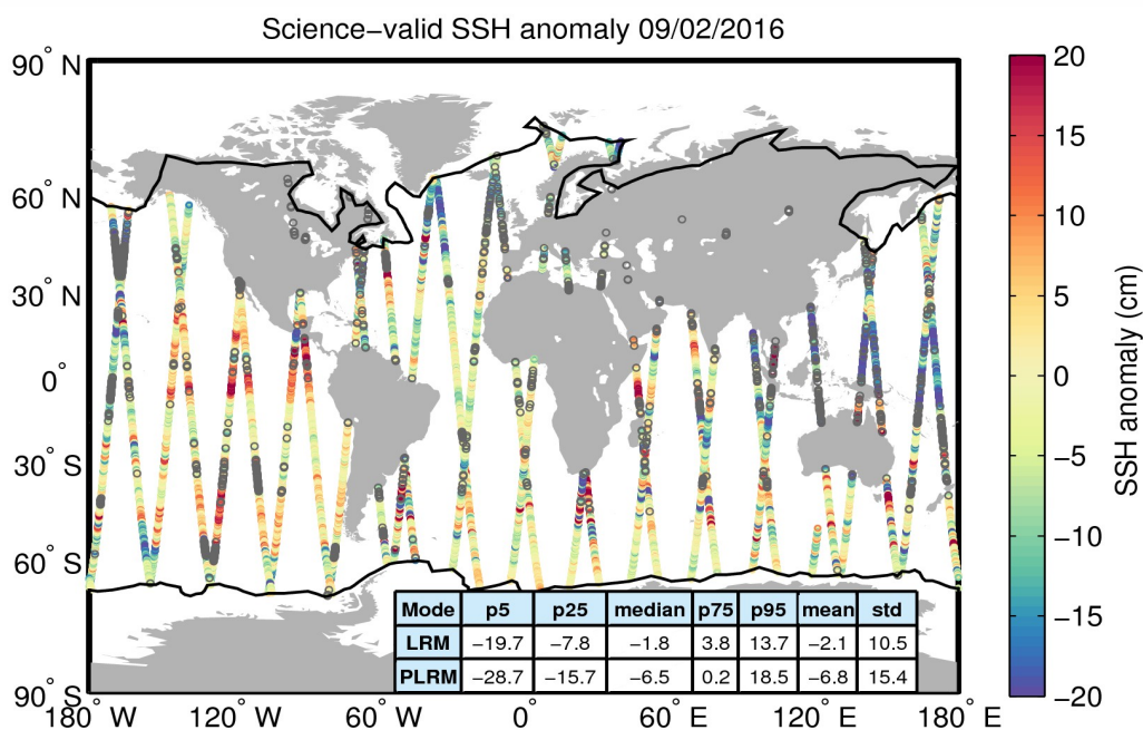
Figure 10. Geographical distribution of science-valid SSH anomaly data over oceans and lakes for 09/02/2016. The statistical values shown in the table refer to the SSH anomaly in cm and are calculated separately for LRM and PLRM regions. The black lines mark the outer limit of the Arctic and Antarctic polar polygons. Gray circles denote records that have been rejected based on the editing criteria described in Table 2.
