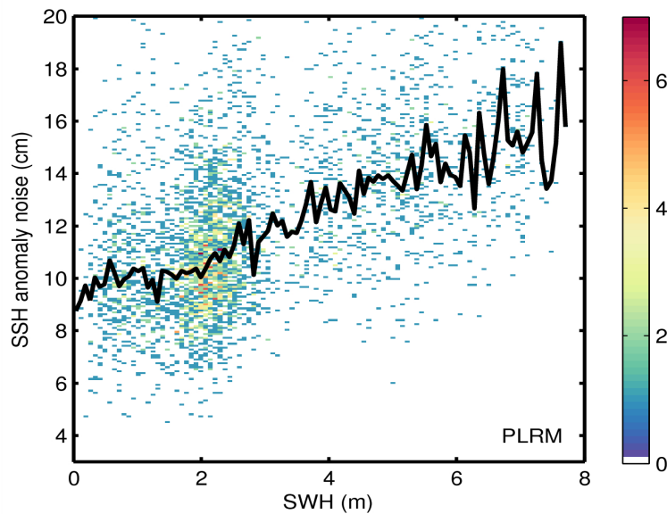
Figure 9. 2D histogram showing flag-valid SSH anomaly noise as a function of SWH for LRM (top) and PLRM (bottom) for 09/02/2016. The black line denotes the median SSH anomaly noise as a function of SWH.
