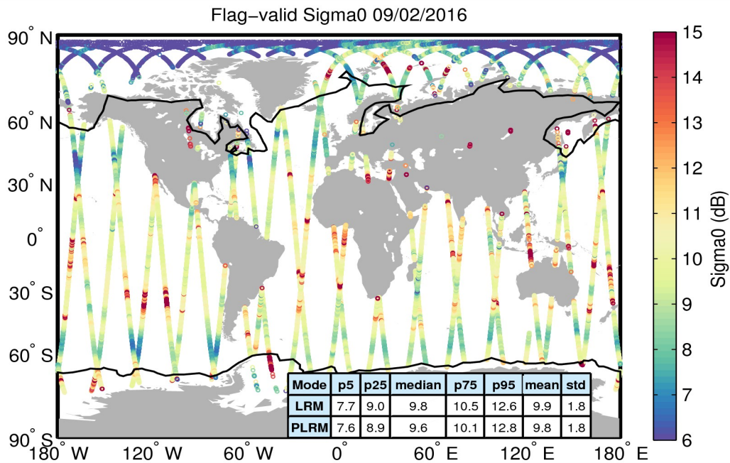
Figure 23. Geographical distribution of flag-valid sigma0 data over oceans and lakes for 09/02/2016. The statistical values shown in the table refer to the sigma0 in dB and are calculated separately for LRM and PLRM regions. Measurements taken over polar polygons have been excluded from the computation of the statistical values. The black lines mark the outer limit of the Arctic and Antarctic polar polygons.
