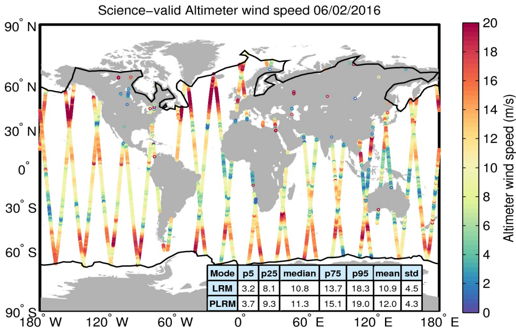
Figure 34. Geographical distribution of science-valid wind data over oceans and lakes for 06/02/2016. The statistical values shown in the table refer to the wind in m/s and are calculated separately for LRM and PLRM regions. The black lines mark the outer limit of the Arctic and Antarctic polar polygons. Gray circles denote records that have been rejected based on the editing criteria described in Table 5.
