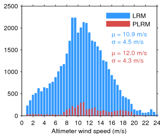
Figure 35. Histogram of science-valid wind over oceans and lakes for LRM (blue) and PLRM (red) for 06/02/2016. The mean ( \mu ) and standard deviation ( \sigma ) are also shown. Note that values larger than 24 m/s are excluded from the histogram for the sake of readability but not from the computation of \mu and \sigma .
