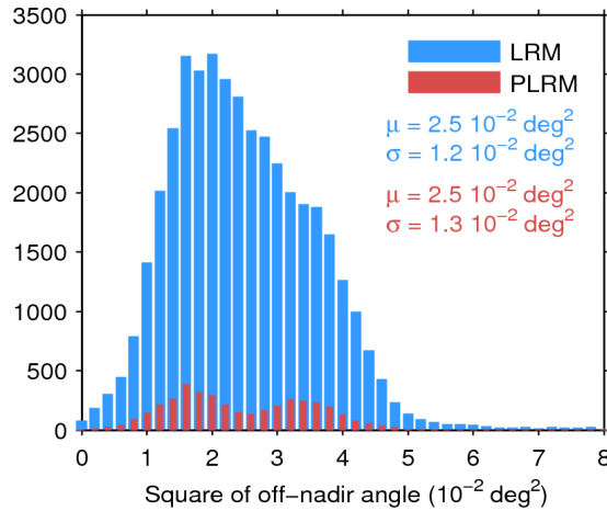
Figure 39. Histogram of flag-valid mispointing over oceans and lakes for LRM (blue) and PLRM (red) for 06/02/2016. Only positive values have been considered. The mean ( \mu ) and standard deviation ( \sigma ) are also shown. Note that values larger than 8 \cdot 10^{-2} \text{ deg}^2 are excluded from the histogram for the sake of readability but not from the computation of \mu and \sigma .
