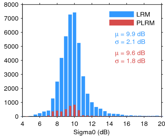
Figure 25. Histogram of flag-valid sigma0 over oceans and lakes for LRM (blue) and PLRM (red) for 06/02/2016. The mean ( \mu ) and standard deviation ( \sigma ) are also shown. Note that values outside [4 20] dB are excluded from the histogram for the sake of readability but not from the computation of \mu and \sigma .
