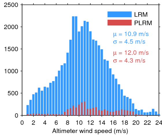
Figure 33. Histogram of flag-valid wind over oceans and lakes for LRM (blue) and PLRM (red) for 06/02/2016. The mean ( \mu ) and standard deviation ( \sigma ) are also shown. Note that values larger than 24 m/s are excluded from the histogram for the sake of readability but not from the computation of \mu and \sigma .
