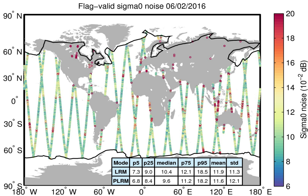
Figure 26. Geographical distribution of flag-valid 20-Hz sigma0 measurement noise over oceans and lakes for 06/02/2016. The statistical values shown in the table refer to the sigma0 noise and are calculated separately for LRM and PLRM regions. Measurements taken over polar polygons have been excluded from the computation of the statistical values. The black lines mark the outer limit of the Arctic and Antarctic polar polygons.
