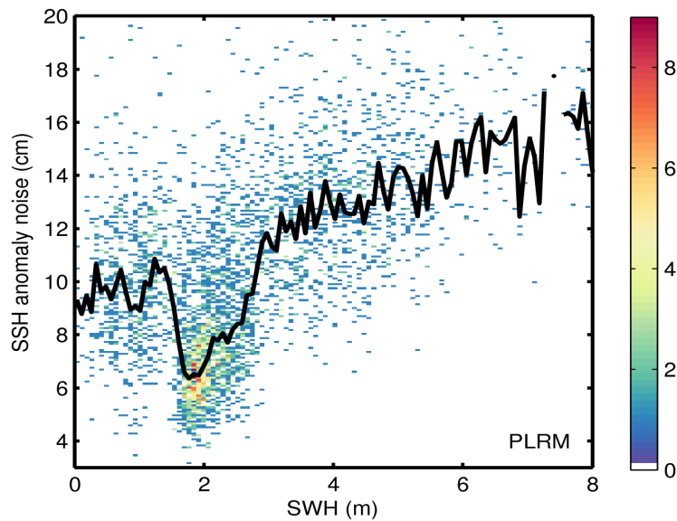
Figure 9. 2D histogram showing flag-valid SSH anomaly noise as a function of SWH for LRM (top) and PLRM (bottom) for 06/02/2016. The black line denotes the median SSH anomaly noise as a function of SWH.
