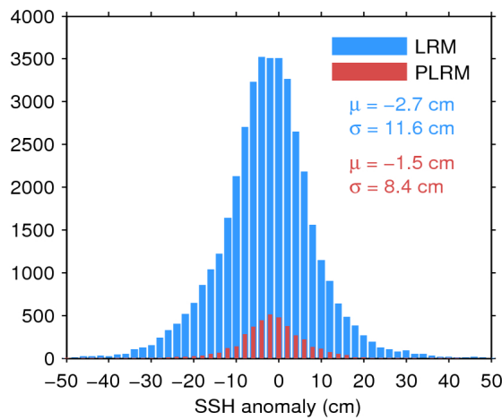
Figure 11. Histogram of science-valid SSH anomaly over oceans and lakes for LRM (blue) and PLRM (red) for 06/02/2016. The mean ( \mu ) and standard deviation ( \sigma ) are also shown. Note that values outside [-50 50] cm are excluded from the histogram for the sake of readability but not from the computation of \mu and \sigma .
