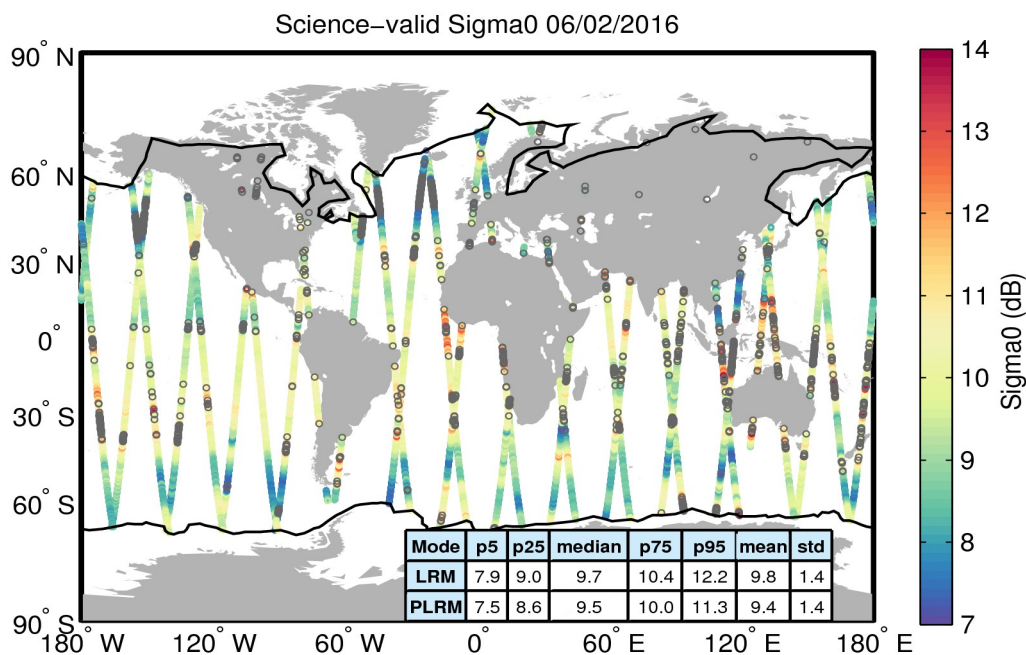
Figure 27. Geographical distribution of science-valid sigma0 data over oceans and lakes for 06/02/2016. The statistical values shown in the table refer to the sigma0 in dB and are calculated separately for LRM and PLRM regions. The black lines mark the outer limit of the Arctic and Antarctic polar polygons. Gray circles denote records that have been rejected based on the editing criteria described in Table 4.
