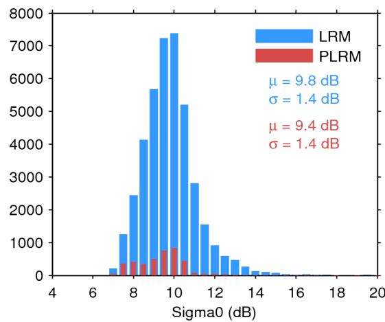
Figure 28. Histogram of science-valid sigma0 over oceans and lakes for LRM (blue) and PLRM (red) for 06/02/2016. The mean ( \mu ) and standard deviation ( \sigma ) are also shown. Note that values outside [4 20] dB are excluded from the histogram for the sake of readability but not from the computation of \mu and \sigma .
