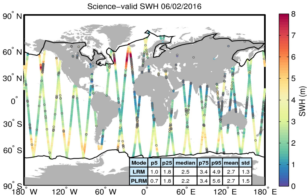
Figure 19. Geographical distribution of science-valid SWH data over oceans and lakes for 06/02/2016. The statistical values shown in the table refer to the SWH in m and are calculated separately for LRM and PLRM regions. The black lines mark the outer limit of the Arctic and Antarctic polar polygons. Gray circles denote records that have been rejected based on the editing criteria described in Table 3.
