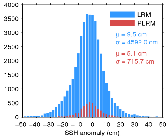
Figure 7. Histogram of flag-valid SSH anomaly over oceans and lakes for LRM (blue) and PLRM (red) for 06/02/2016. The mean ( \mu ) and standard deviation ( \sigma ) are also shown. Note that values outside [-50 50] cm are excluded from the histogram for the sake of readability but not from the computation of \mu and \sigma .
