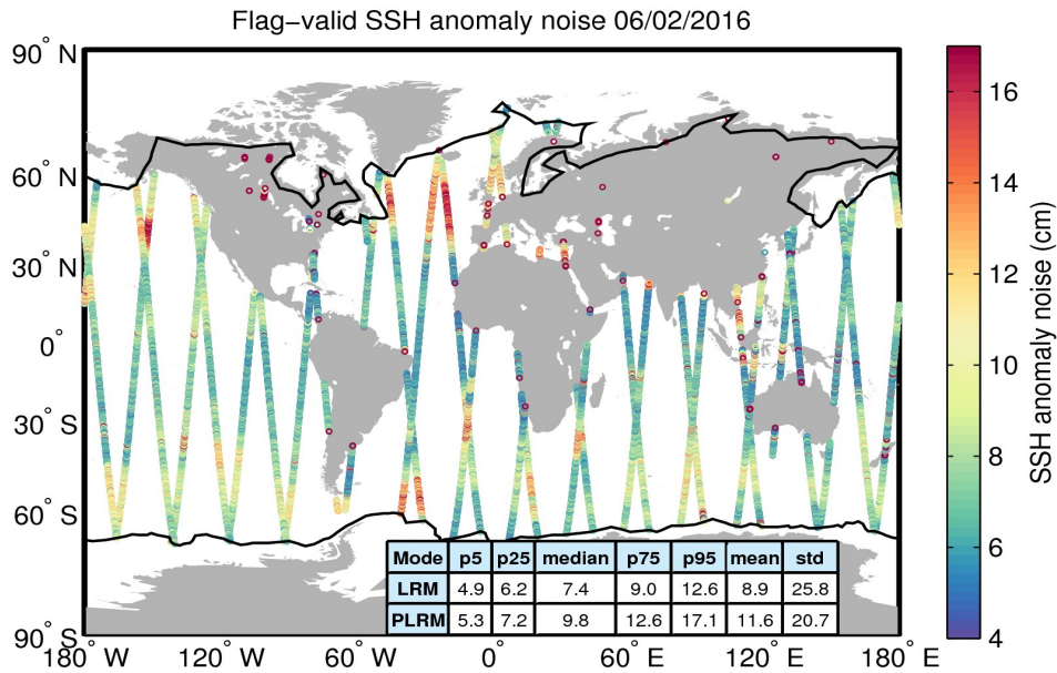
Figure 8. Geographical distribution of flag-valid 20-Hz SSH anomaly measurement noise over oceans and lakes for 06/02/2016. The statistical values shown in the table refer to the SSH anomaly noise and are calculated separately for LRM and PLRM regions. Measurements taken over polar polygons have been excluded from the computation of the statistical values. The black lines mark the outer limit of the Arctic and Antarctic polar polygons.
