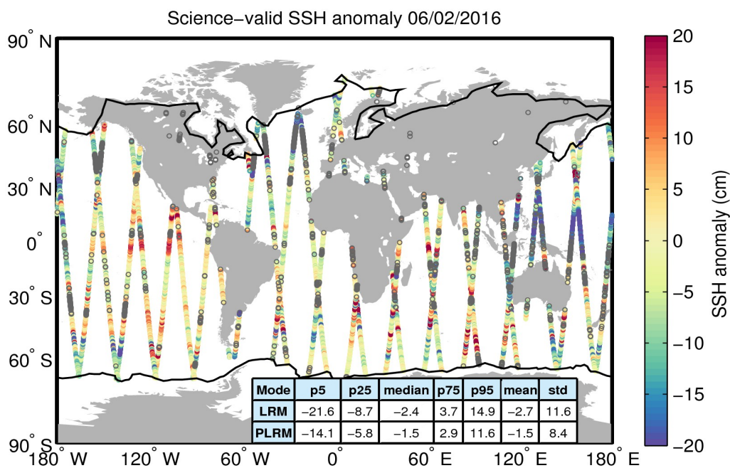
Figure 10. Geographical distribution of science-valid SSH anomaly data over oceans and lakes for 06/02/2016. The statistical values shown in the table refer to the SSH anomaly in cm and are calculated separately for LRM and PLRM regions. The black lines mark the outer limit of the Arctic and Antarctic polar polygons. Gray circles denote records that have been rejected based on the editing criteria described in Table 2.
