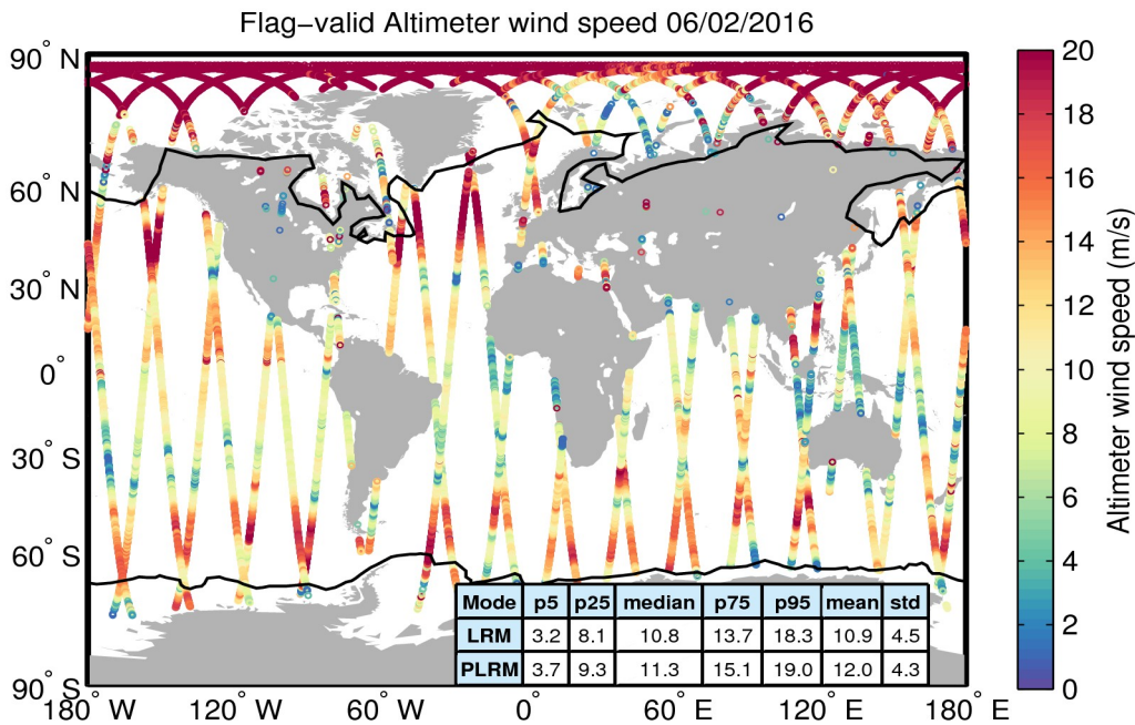
Figure 31. Geographical distribution of flag-valid wind data over oceans and lakes for 06/02/2016. The statistical values shown in the table refer to the wind in m/s and are calculated separately for LRM and PLRM regions. Measurements taken over polar polygons have been excluded from the computation of the statistical values. The black lines mark the outer limit of the Arctic and Antarctic polar polygons.
