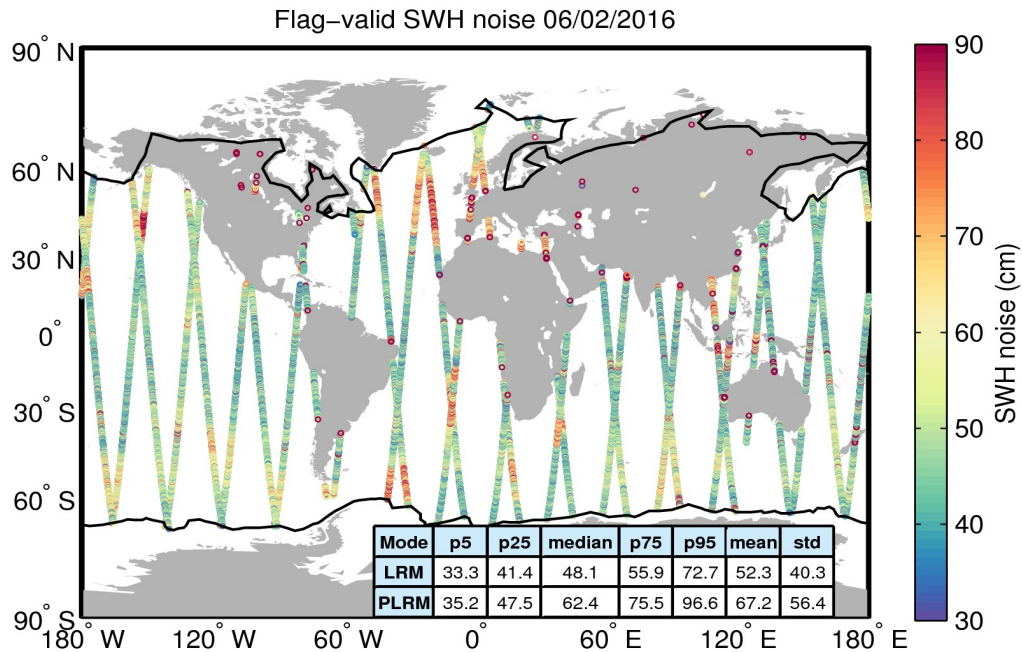
Figure 18. Geographical distribution of flag-valid 20-Hz SWH measurement noise over oceans and lakes for 06/02/2016. The statistical values shown in the table refer to the SWH noise and are calculated separately for LRM and PLRM regions. Measurements taken over polar polygons have been excluded from the computation of the statistical values. The black lines mark the outer limit of the Arctic and Antarctic polar polygons.
