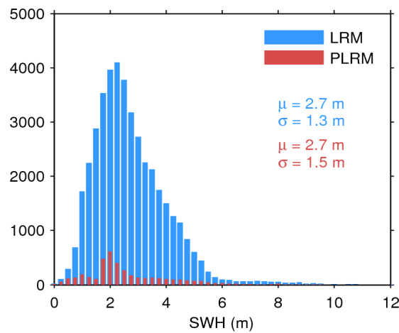
Figure 20. Histogram of science-valid SWH over oceans and lakes for LRM (blue) and PLRM (red) for 06/02/2016. The mean ( \mu ) and standard deviation ( \sigma ) are also shown. Note that values larger than 12 m are excluded from the histogram for the sake of readability but not from the computation of \mu and \sigma .
