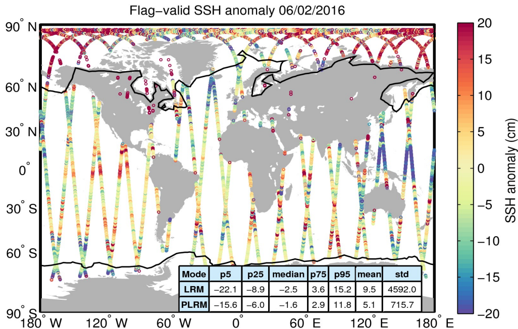
Figure 5. Geographical distribution of flag-valid 1-Hz SSH anomaly data over oceans and lakes for 06/02/2016. The statistical values shown in the table refer to the SSH anomaly in cm and are calculated separately for LRM and PLRM regions. Measurements taken over polar polygons have been excluded from the computation of the statistical values. The black lines mark the outer limit of the Arctic and Antarctic polar polygons.
