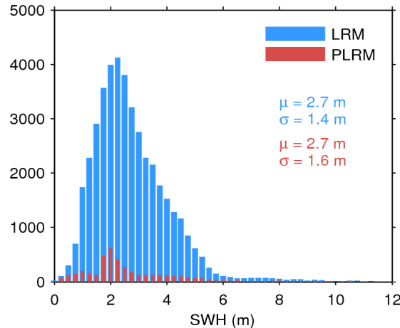
Figure 17. Histogram of flag-valid SWH over oceans and lakes for LRM (blue) and PLRM (red) for 06/02/2016. The mean ( \mu ) and standard deviation ( \sigma ) are also shown. Note that values larger than 12 m are excluded from the histogram for the sake of readability but not from the computation of \mu and \sigma .
