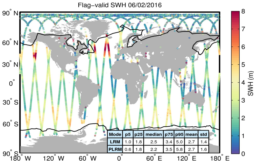
Figure 15. Geographical distribution of flag-valid SWH data over oceans and lakes for 06/02/2016. The statistical values shown in the table refer to the SWH in m and are calculated separately for LRM and PLRM regions. Measurements taken over polar polygons have been excluded from the computation of the statistical values. The black lines mark the outer limit of the Arctic and Antarctic polar polygons.
