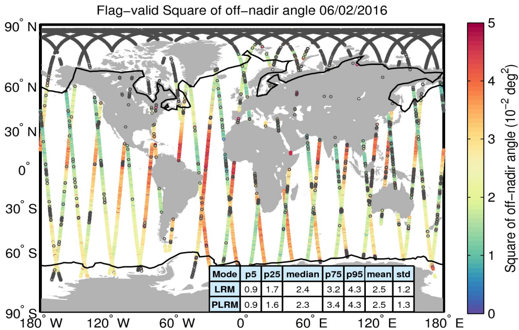
Figure 37. Geographical distribution of flag-valid mispointing data over oceans and lakes for 06/02/2016. The statistical values shown in the table refer to the mispointing in 10^{-2} deg 2 and are calculated separately for LRM and PLRM regions. Measurements taken over polar polygons have been excluded from the computation of the statistical values. The black lines mark the outer limit of the Arctic and Antarctic polar polygons. Gray circles denote negative values.
