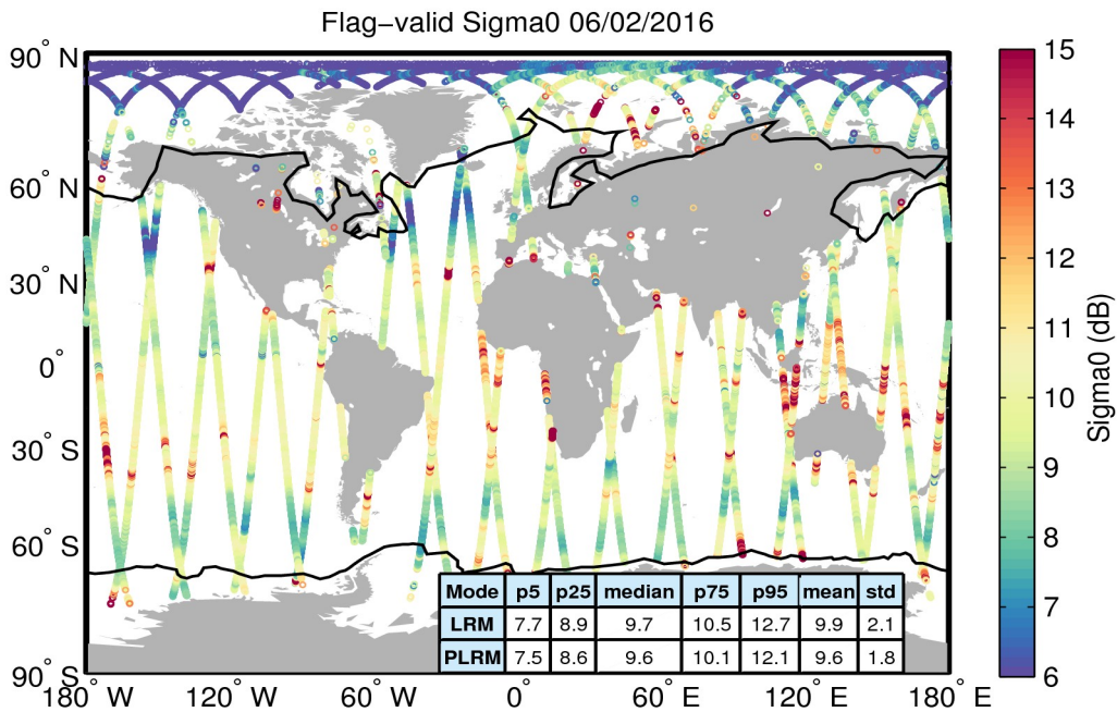
Figure 23. Geographical distribution of flag-valid sigma0 data over oceans and lakes for 06/02/2016. The statistical values shown in the table refer to the sigma0 in dB and are calculated separately for LRM and PLRM regions. Measurements taken over polar polygons have been excluded from the computation of the statistical values. The black lines mark the outer limit of the Arctic and Antarctic polar polygons.
