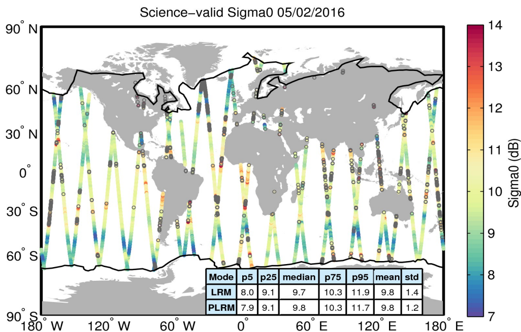
Figure 27. Geographical distribution of science-valid sigma0 data over oceans and lakes for 05/02/2016. The statistical values shown in the table refer to the sigma0 in dB and are calculated separately for LRM and PLRM regions. The black lines mark the outer limit of the Arctic and Antarctic polar polygons. Gray circles denote records that have been rejected based on the editing criteria described in Table 4.
