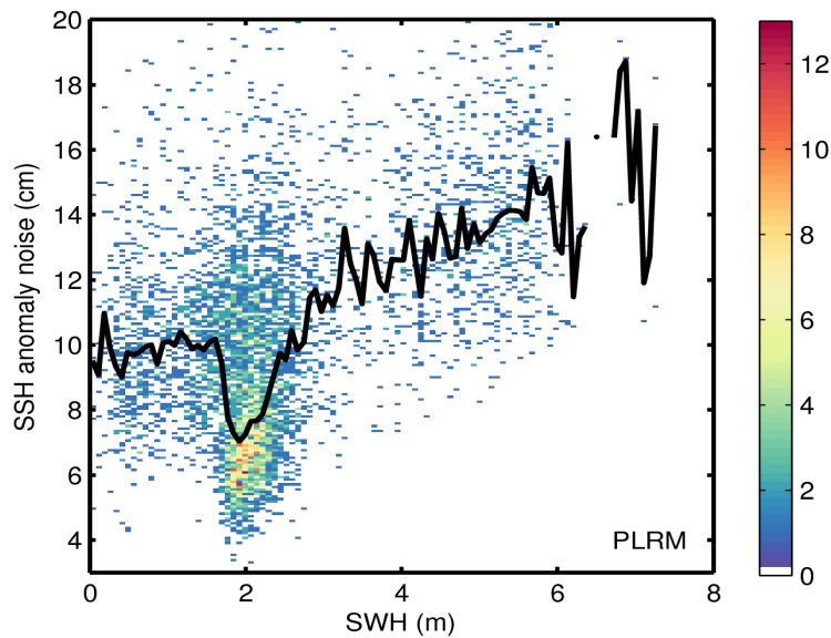
Figure 9. 2D histogram showing flag-valid SSH anomaly noise as a function of SWH for LRM (top) and PLRM (bottom) for 05/02/2016. The black line denotes the median SSH anomaly noise as a function of SWH.
