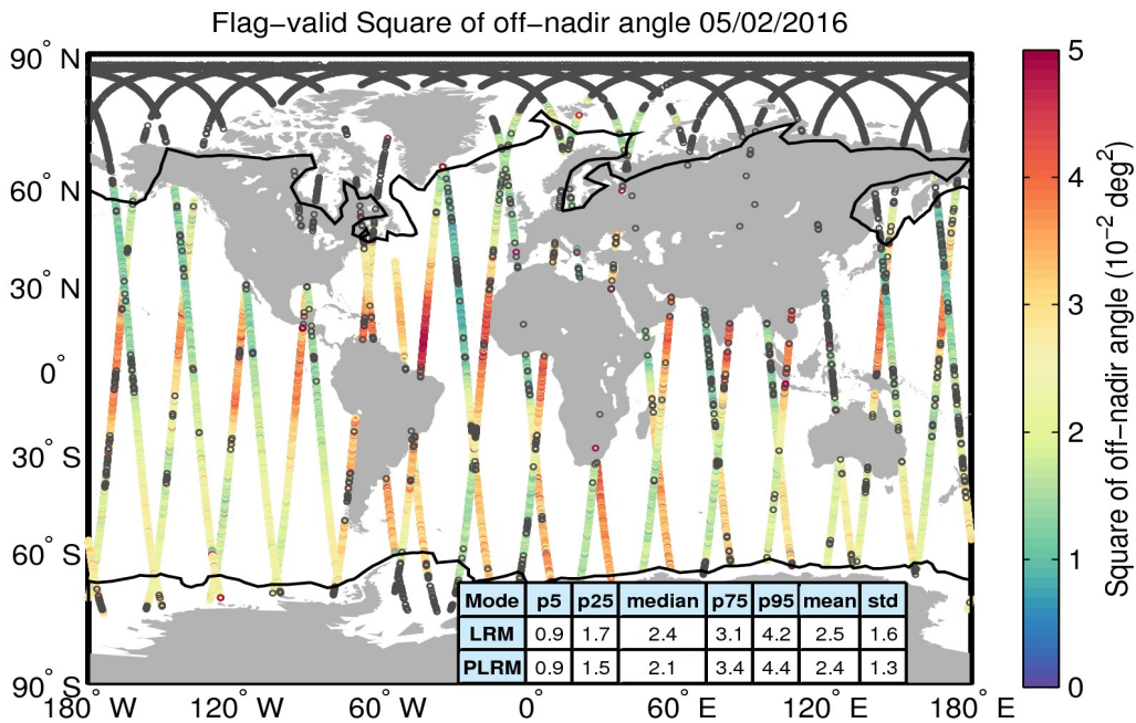
Figure 37. Geographical distribution of flag-valid mispointing data over oceans and lakes for 05/02/2016. The statistical values shown in the table refer to the mispointing in 10^{-2} deg 2 and are calculated separately for LRM and PLRM regions. Measurements taken over polar polygons have been excluded from the computation of the statistical values. The black lines mark the outer limit of the Arctic and Antarctic polar polygons. Gray circles denote negative values.
