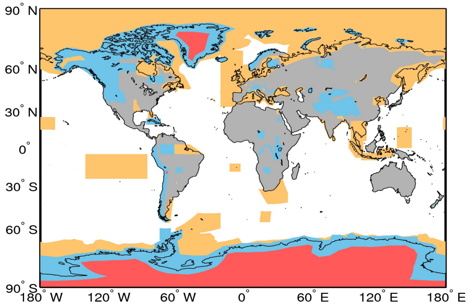
Figure A1. Extent of the regions defining the geographical mode mask for 05/02/2016. The regions where SAR, and SARIn are operated are denoted by the orange and blue polygons, respectively. LRM is operated over areas of the continental ice sheets (red polygons) and over oceans and land not covered by other modes.
