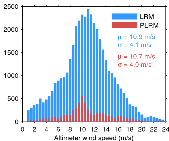
Figure 33. Histogram of flag-valid wind over oceans and lakes for LRM (blue) and PLRM (red) for 05/02/2016. The mean ( \mu ) and standard deviation ( \sigma ) are also shown. Note that values larger than 24 m/s are excluded from the histogram for the sake of readability but not from the computation of \mu and \sigma .
