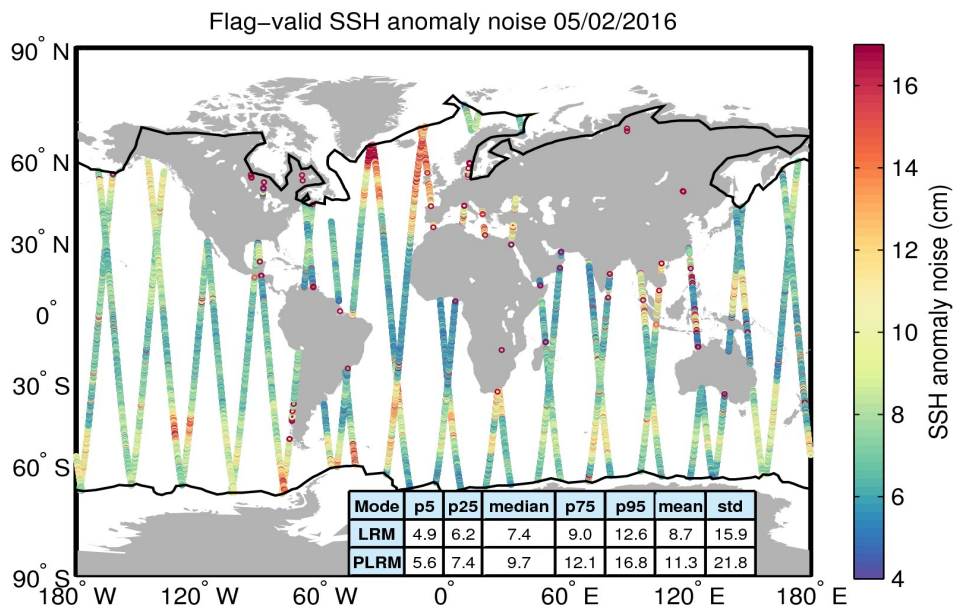
Figure 8. Geographical distribution of flag-valid 20-Hz SSH anomaly measurement noise over oceans and lakes for 05/02/2016. The statistical values shown in the table refer to the SSH anomaly noise and are calculated separately for LRM and PLRM regions. Measurements taken over polar polygons have been excluded from the computation of the statistical values. The black lines mark the outer limit of the Arctic and Antarctic polar polygons.
