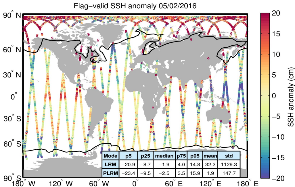
Figure 5. Geographical distribution of flag-valid 1-Hz SSH anomaly data over oceans and lakes for 05/02/2016. The statistical values shown in the table refer to the SSH anomaly in cm and are calculated separately for LRM and PLRM regions. Measurements taken over polar polygons have been excluded from the computation of the statistical values. The black lines mark the outer limit of the Arctic and Antarctic polar polygons.
