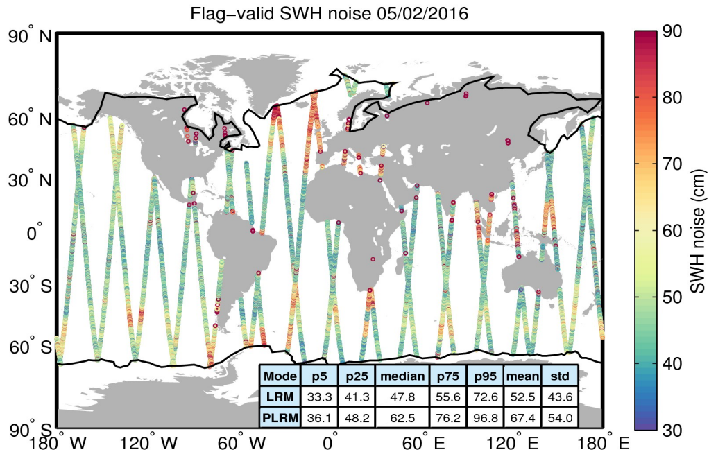
Figure 18. Geographical distribution of flag-valid 20-Hz SWH measurement noise over oceans and lakes for 05/02/2016. The statistical values shown in the table refer to the SWH noise and are calculated separately for LRM and PLRM regions. Measurements taken over polar polygons have been excluded from the computation of the statistical values. The black lines mark the outer limit of the Arctic and Antarctic polar polygons.
