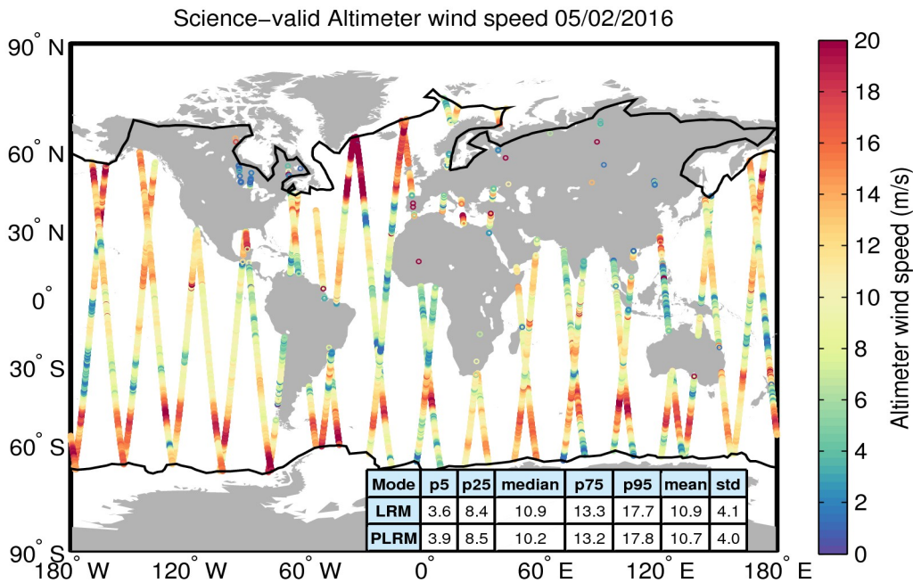
Figure 34. Geographical distribution of science-valid wind data over oceans and lakes for 05/02/2016. The statistical values shown in the table refer to the wind in m/s and are calculated separately for LRM and PLRM regions. The black lines mark the outer limit of the Arctic and Antarctic polar polygons. Gray circles denote records that have been rejected based on the editing criteria described in Table 5.
