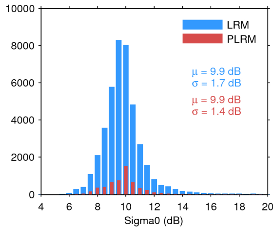
Figure 25. Histogram of flag-valid sigma0 over oceans and lakes for LRM (blue) and PLRM (red) for 05/02/2016. The mean ( \mu ) and standard deviation ( \sigma ) are also shown. Note that values outside [4 20] dB are excluded from the histogram for the sake of readability but not from the computation of \mu and \sigma .
