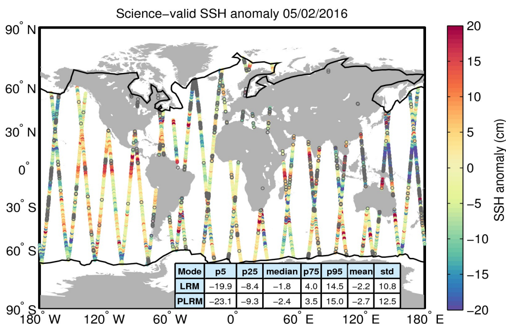
Figure 10. Geographical distribution of science-valid SSH anomaly data over oceans and lakes for 05/02/2016. The statistical values shown in the table refer to the SSH anomaly in cm and are calculated separately for LRM and PLRM regions. The black lines mark the outer limit of the Arctic and Antarctic polar polygons. Gray circles denote records that have been rejected based on the editing criteria described in Table 2.
