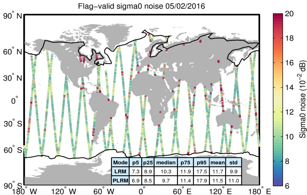
Figure 26. Geographical distribution of flag-valid 20-Hz sigma0 measurement noise over oceans and lakes for 05/02/2016. The statistical values shown in the table refer to the sigma0 noise and are calculated separately for LRM and PLRM regions. Measurements taken over polar polygons have been excluded from the computation of the statistical values. The black lines mark the outer limit of the Arctic and Antarctic polar polygons.
