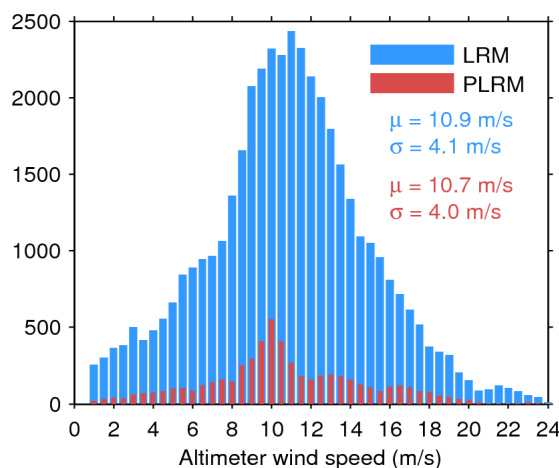
Figure 35. Histogram of science-valid wind over oceans and lakes for LRM (blue) and PLRM (red) for 05/02/2016. The mean ( \mu ) and standard deviation ( \sigma ) are also shown. Note that values larger than 24 m/s are excluded from the histogram for the sake of readability but not from the computation of \mu and \sigma .
