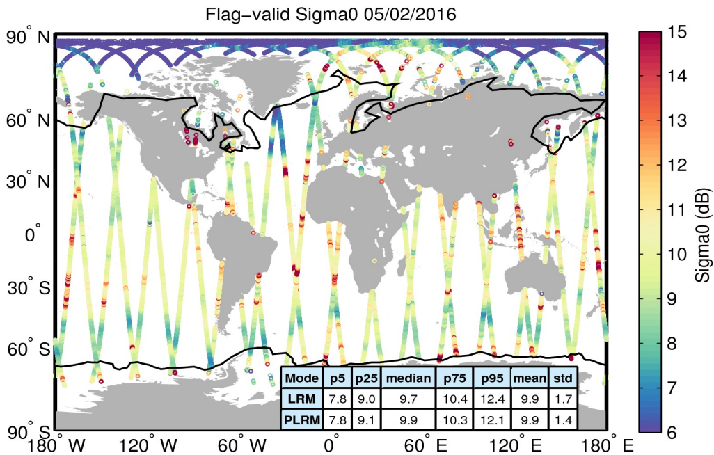
Figure 23. Geographical distribution of flag-valid sigma0 data over oceans and lakes for 05/02/2016. The statistical values shown in the table refer to the sigma0 in dB and are calculated separately for LRM and PLRM regions. Measurements taken over polar polygons have been excluded from the computation of the statistical values. The black lines mark the outer limit of the Arctic and Antarctic polar polygons.
