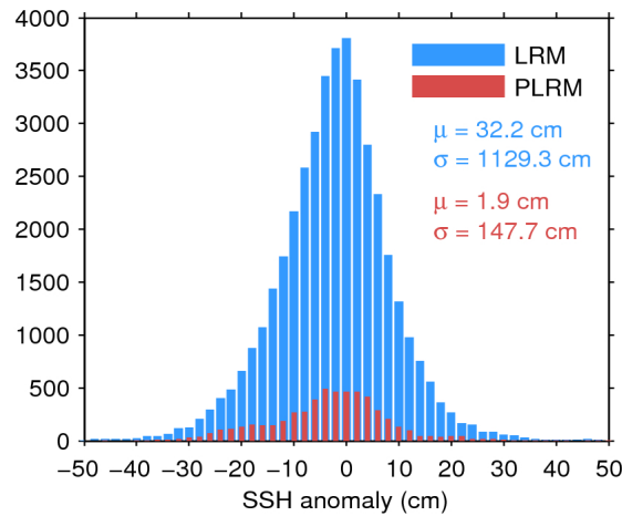
Figure 7. Histogram of flag-valid SSH anomaly over oceans and lakes for LRM (blue) and PLRM (red) for 05/02/2016. The mean ( \mu ) and standard deviation ( \sigma ) are also shown. Note that values outside [-50 50] cm are excluded from the histogram for the sake of readability but not from the computation of \mu and \sigma .
