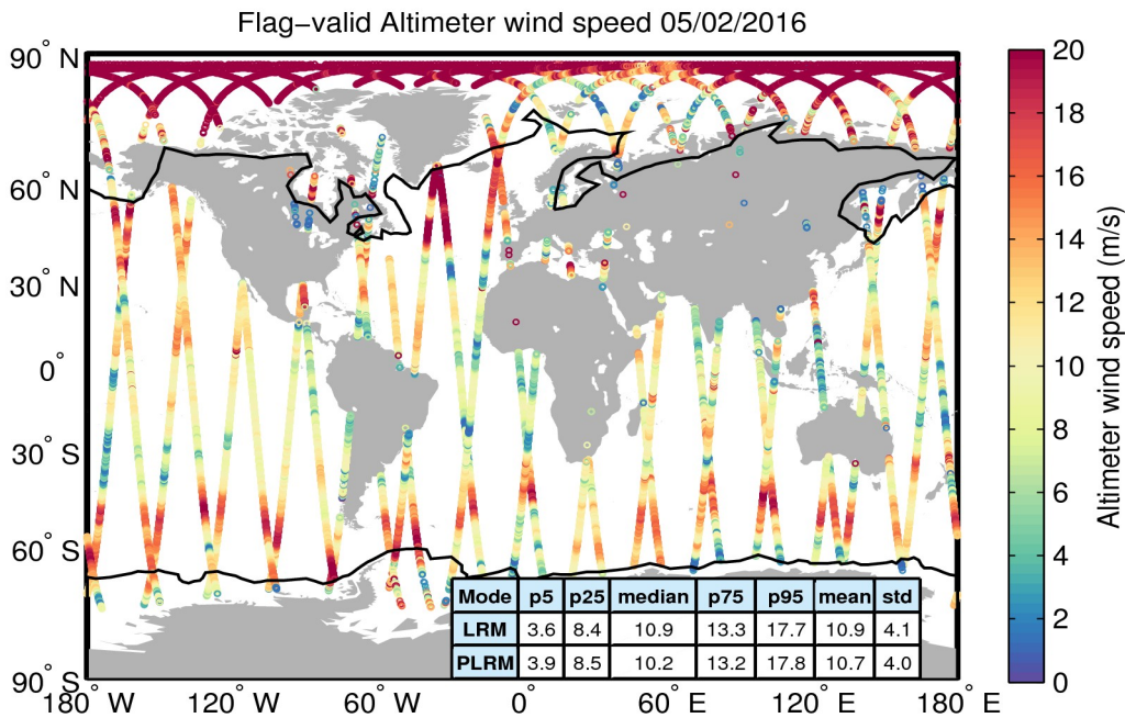
Figure 31. Geographical distribution of flag-valid wind data over oceans and lakes for 05/02/2016. The statistical values shown in the table refer to the wind in m/s and are calculated separately for LRM and PLRM regions. Measurements taken over polar polygons have been excluded from the computation of the statistical values. The black lines mark the outer limit of the Arctic and Antarctic polar polygons.
