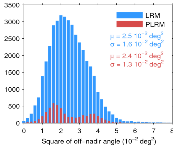
Figure 39. Histogram of flag-valid mispointing over oceans and lakes for LRM (blue) and PLRM (red) for 05/02/2016. Only positive values have been considered. The mean ( \mu ) and standard deviation ( \sigma ) are also shown. Note that values larger than 8 \cdot 10^{-2} \text{ deg}^2 are excluded from the histogram for the sake of readability but not from the computation of \mu and \sigma .
