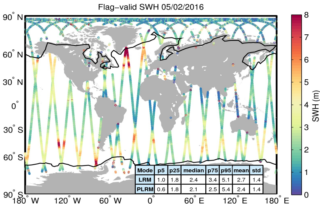
Figure 15. Geographical distribution of flag-valid SWH data over oceans and lakes for 05/02/2016. The statistical values shown in the table refer to the SWH in m and are calculated separately for LRM and PLRM regions. Measurements taken over polar polygons have been excluded from the computation of the statistical values. The black lines mark the outer limit of the Arctic and Antarctic polar polygons.
