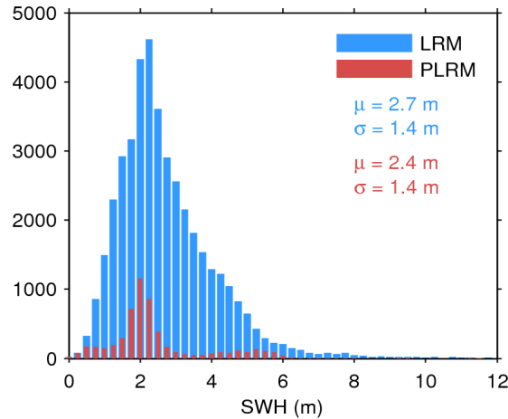
Figure 17. Histogram of flag-valid SWH over oceans and lakes for LRM (blue) and PLRM (red) for 05/02/2016. The mean ( \mu ) and standard deviation ( \sigma ) are also shown. Note that values larger than 12 m are excluded from the histogram for the sake of readability but not from the computation of \mu and \sigma .
