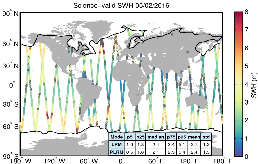
Figure 19. Geographical distribution of science-valid SWH data over oceans and lakes for 05/02/2016. The statistical values shown in the table refer to the SWH in m and are calculated separately for LRM and PLRM regions. The black lines mark the outer limit of the Arctic and Antarctic polar polygons. Gray circles denote records that have been rejected based on the editing criteria described in Table 3.
