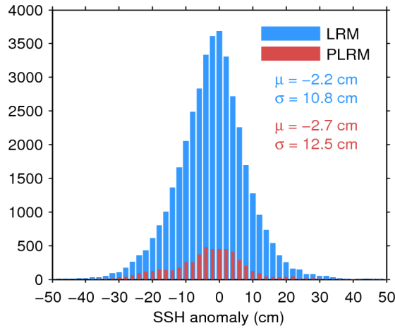
Figure 11. Histogram of science-valid SSH anomaly over oceans and lakes for LRM (blue) and PLRM (red) for 05/02/2016. The mean ( \mu ) and standard deviation ( \sigma ) are also shown. Note that values outside [-50 50] cm are excluded from the histogram for the sake of readability but not from the computation of \mu and \sigma .
