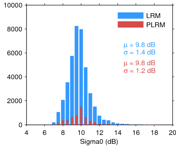
Figure 28. Histogram of science-valid sigma0 over oceans and lakes for LRM (blue) and PLRM (red) for 05/02/2016. The mean ( \mu ) and standard deviation ( \sigma ) are also shown. Note that values outside [4 20] dB are excluded from the histogram for the sake of readability but not from the computation of \mu and \sigma .
