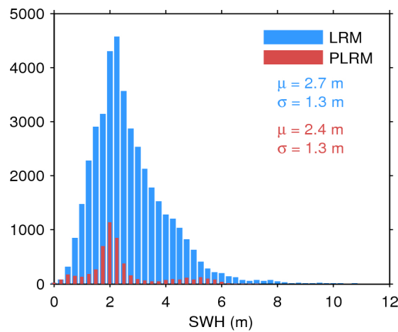
Figure 20. Histogram of science-valid SWH over oceans and lakes for LRM (blue) and PLRM (red) for 05/02/2016. The mean ( \mu ) and standard deviation ( \sigma ) are also shown. Note that values larger than 12 m are excluded from the histogram for the sake of readability but not from the computation of \mu and \sigma .
