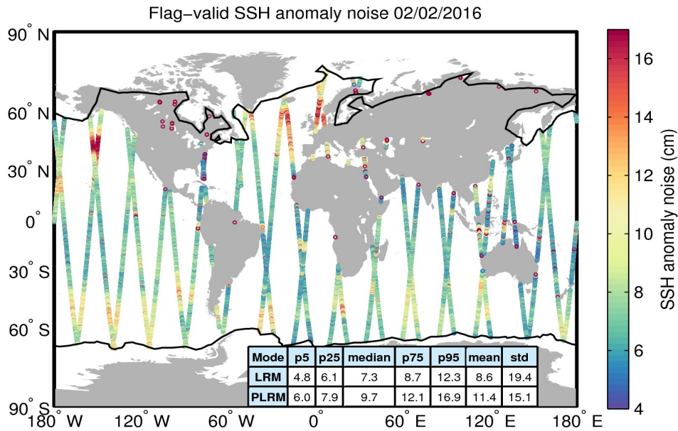
Figure 8. Geographical distribution of flag-valid 20-Hz SSH anomaly measurement noise over oceans and lakes for 02/02/2016. The statistical values shown in the table refer to the SSH anomaly noise and are calculated separately for LRM and PLRM regions. Measurements taken over polar polygons have been excluded from the computation of the statistical values. The black lines mark the outer limit of the Arctic and Antarctic polar polygons.
