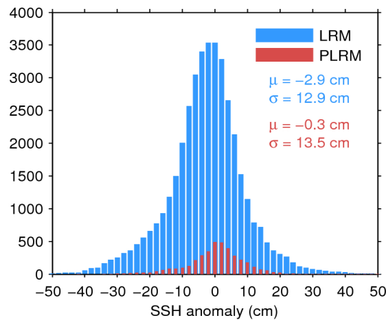
Figure 11. Histogram of science-valid SSH anomaly over oceans and lakes for LRM (blue) and PLRM (red) for 02/02/2016. The mean ( \mu ) and standard deviation ( \sigma ) are also shown. Note that values outside [-50 50] cm are excluded from the histogram for the sake of readability but not from the computation of \mu and \sigma .
