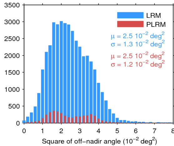
Figure 39. Histogram of flag-valid mispointing over oceans and lakes for LRM (blue) and PLRM (red) for 02/02/2016. Only positive values have been considered. The mean ( \mu ) and standard deviation ( \sigma ) are also shown. Note that values larger than 8 \cdot 10^{-2} \text{ deg}^2 are excluded from the histogram for the sake of readability but not from the computation of \mu and \sigma .
