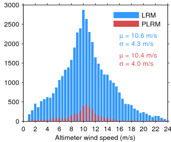
Figure 33. Histogram of flag-valid wind over oceans and lakes for LRM (blue) and PLRM (red) for 02/02/2016. The mean ( \mu ) and standard deviation ( \sigma ) are also shown. Note that values larger than 24 m/s are excluded from the histogram for the sake of readability but not from the computation of \mu and \sigma .
