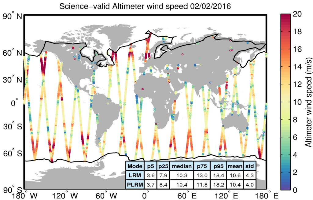
Figure 34. Geographical distribution of science-valid wind data over oceans and lakes for 02/02/2016. The statistical values shown in the table refer to the wind in m/s and are calculated separately for LRM and PLRM regions. The black lines mark the outer limit of the Arctic and Antarctic polar polygons. Gray circles denote records that have been rejected based on the editing criteria described in Table 5.
