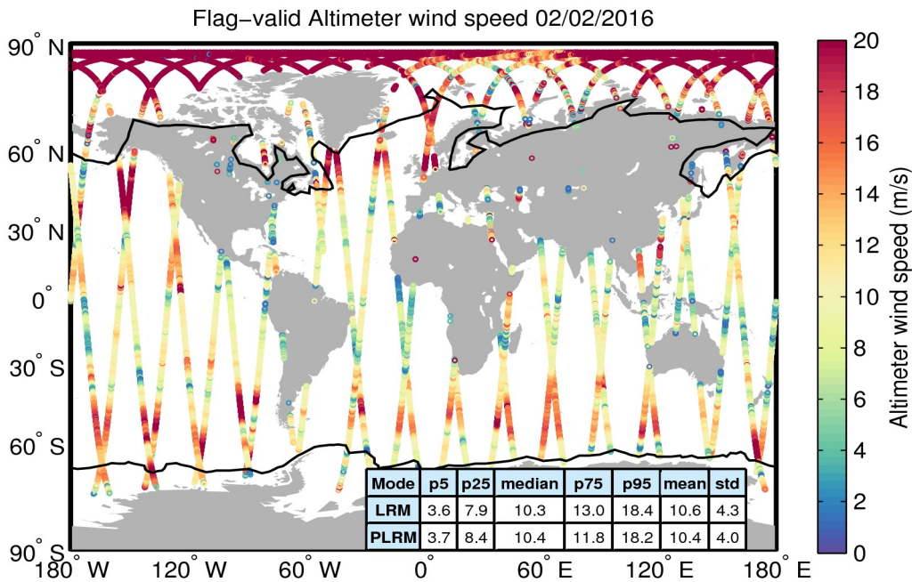
Figure 31. Geographical distribution of flag-valid wind data over oceans and lakes for 02/02/2016. The statistical values shown in the table refer to the wind in m/s and are calculated separately for LRM and PLRM regions. Measurements taken over polar polygons have been excluded from the computation of the statistical values. The black lines mark the outer limit of the Arctic and Antarctic polar polygons.
