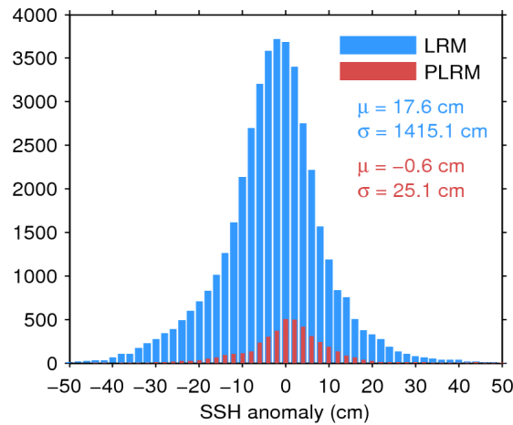
Figure 7. Histogram of flag-valid SSH anomaly over oceans and lakes for LRM (blue) and PLRM (red) for 02/02/2016. The mean ( \mu ) and standard deviation ( \sigma ) are also shown. Note that values outside [-50\ 50] cm are excluded from the histogram for the sake of readability but not from the computation of \mu and \sigma .
