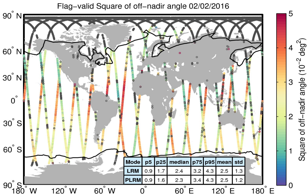
Figure 37. Geographical distribution of flag-valid mispointing data over oceans and lakes for 02/02/2016. The statistical values shown in the table refer to the mispointing in 10^{-2} deg 2 and are calculated separately for LRM and PLRM regions. Measurements taken over polar polygons have been excluded from the computation of the statistical values. The black lines mark the outer limit of the Arctic and Antarctic polar polygons. Gray circles denote negative values.
