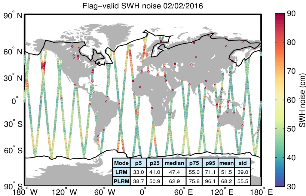
Figure 18. Geographical distribution of flag-valid 20-Hz SWH measurement noise over oceans and lakes for 02/02/2016. The statistical values shown in the table refer to the SWH noise and are calculated separately for LRM and PLRM regions. Measurements taken over polar polygons have been excluded from the computation of the statistical values. The black lines mark the outer limit of the Arctic and Antarctic polar polygons.
