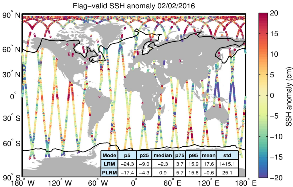
Figure 5. Geographical distribution of flag-valid 1-Hz SSH anomaly data over oceans and lakes for 02/02/2016. The statistical values shown in the table refer to the SSH anomaly in cm and are calculated separately for LRM and PLRM regions. Measurements taken over polar polygons have been excluded from the computation of the statistical values. The black lines mark the outer limit of the Arctic and Antarctic polar polygons.
