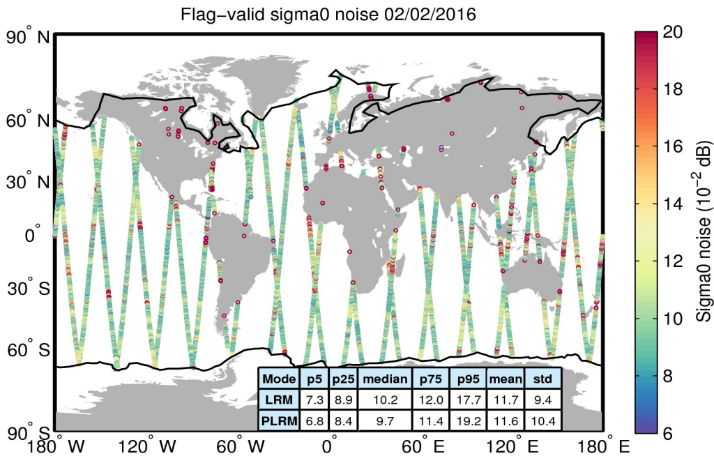
Figure 26. Geographical distribution of flag-valid 20-Hz sigma0 measurement noise over oceans and lakes for 02/02/2016. The statistical values shown in the table refer to the sigma0 noise and are calculated separately for LRM and PLRM regions. Measurements taken over polar polygons have been excluded from the computation of the statistical values. The black lines mark the outer limit of the Arctic and Antarctic polar polygons.
