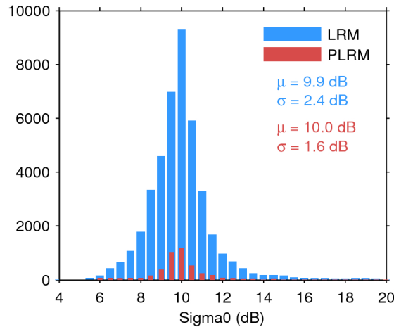
Figure 25. Histogram of flag-valid sigma0 over oceans and lakes for LRM (blue) and PLRM (red) for 02/02/2016. The mean ( \mu ) and standard deviation ( \sigma ) are also shown. Note that values outside [4 20] dB are excluded from the histogram for the sake of readability but not from the computation of \mu and \sigma .
