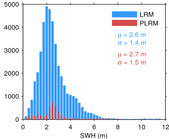
Figure 17. Histogram of flag-valid SWH over oceans and lakes for LRM (blue) and PLRM (red) for 02/02/2016. The mean ( \mu ) and standard deviation ( \sigma ) are also shown. Note that values larger than 12 m are excluded from the histogram for the sake of readability but not from the computation of \mu and \sigma .
