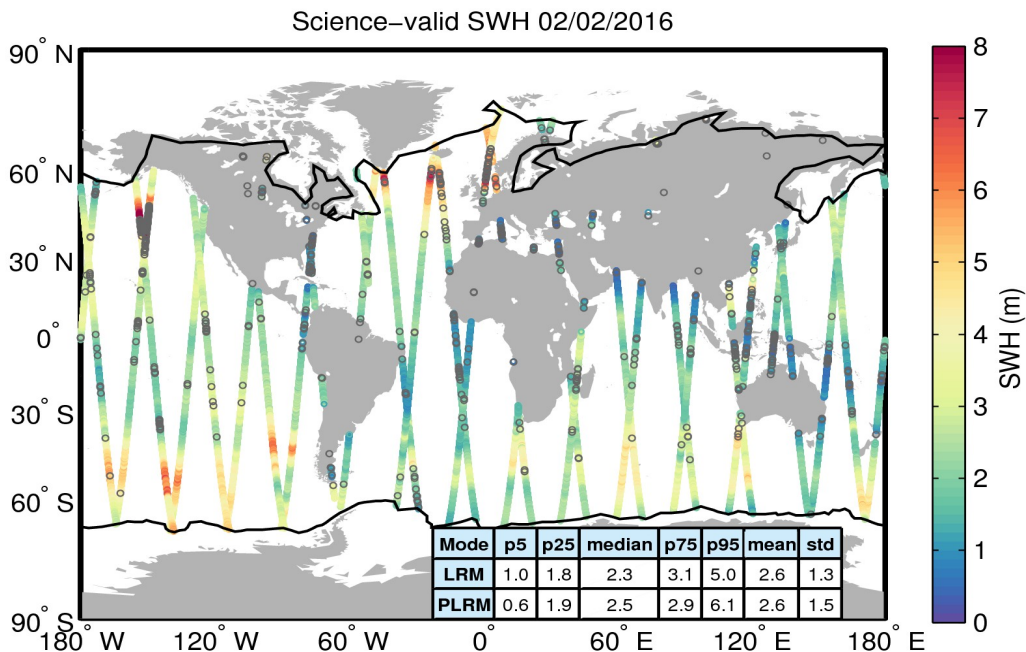
Figure 19. Geographical distribution of science-valid SWH data over oceans and lakes for 02/02/2016. The statistical values shown in the table refer to the SWH in m and are calculated separately for LRM and PLRM regions. The black lines mark the outer limit of the Arctic and Antarctic polar polygons. Gray circles denote records that have been rejected based on the editing criteria described in Table 3.
