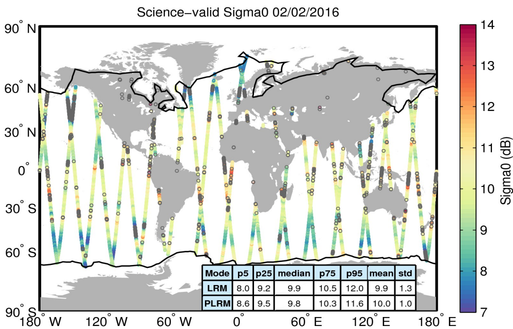
Figure 27. Geographical distribution of science-valid sigma0 data over oceans and lakes for 02/02/2016. The statistical values shown in the table refer to the sigma0 in dB and are calculated separately for LRM and PLRM regions. The black lines mark the outer limit of the Arctic and Antarctic polar polygons. Gray circles denote records that have been rejected based on the editing criteria described in Table 4.
