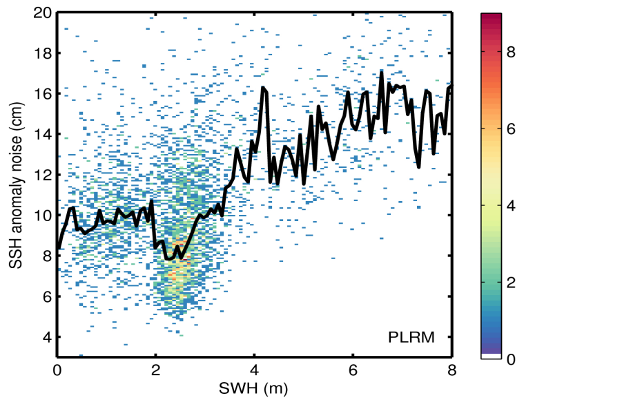
Figure 9. 2D histogram showing flag-valid SSH anomaly noise as a function of SWH for LRM (top) and PLRM (bottom) for 02/02/2016. The black line denotes the median SSH anomaly noise as a function of SWH.
