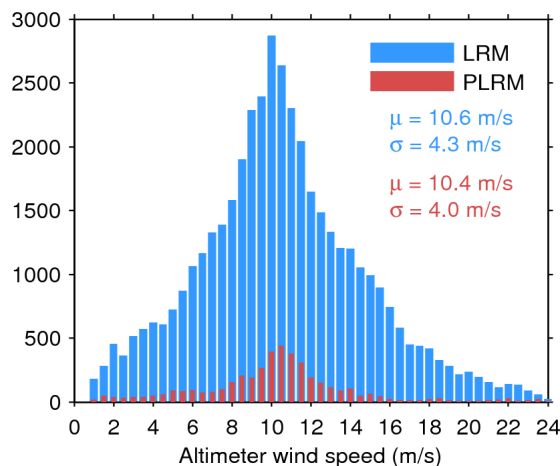
Figure 35. Histogram of science-valid wind over oceans and lakes for LRM (blue) and PLRM (red) for 02/02/2016. The mean ( \mu ) and standard deviation ( \sigma ) are also shown. Note that values larger than 24 m/s are excluded from the histogram for the sake of readability but not from the computation of \mu and \sigma .
