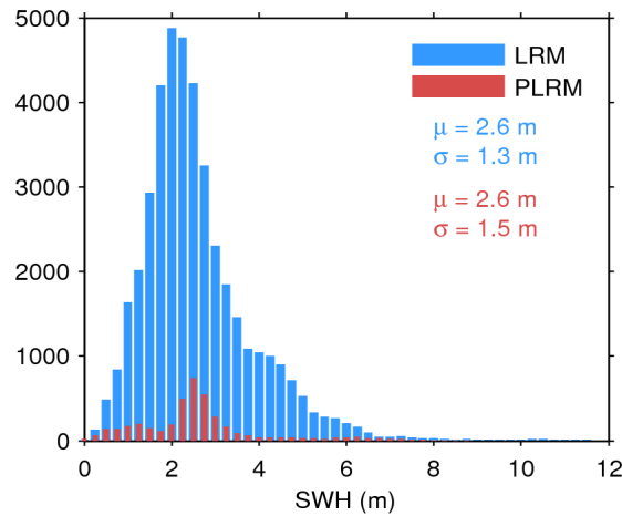
Figure 20. Histogram of science-valid SWH over oceans and lakes for LRM (blue) and PLRM (red) for 02/02/2016. The mean ( \mu ) and standard deviation ( \sigma ) are also shown. Note that values larger than 12 m are excluded from the histogram for the sake of readability but not from the computation of \mu and \sigma .
