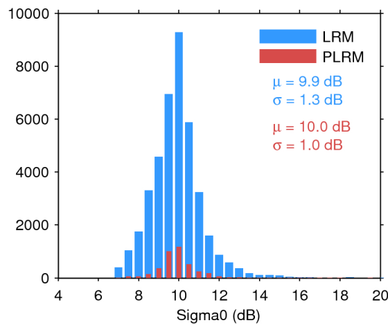
Figure 28. Histogram of science-valid sigma0 over oceans and lakes for LRM (blue) and PLRM (red) for 02/02/2016. The mean ( \mu ) and standard deviation ( \sigma ) are also shown. Note that values outside [4 20] dB are excluded from the histogram for the sake of readability but not from the computation of \mu and \sigma .
