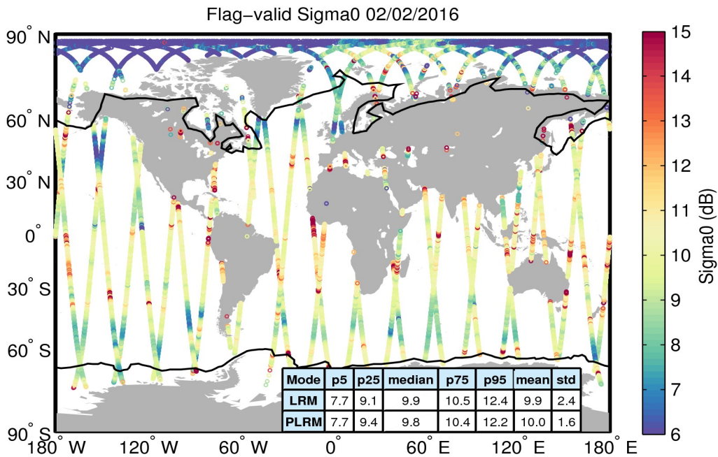
Figure 23. Geographical distribution of flag-valid sigma0 data over oceans and lakes for 02/02/2016. The statistical values shown in the table refer to the sigma0 in dB and are calculated separately for LRM and PLRM regions. Measurements taken over polar polygons have been excluded from the computation of the statistical values. The black lines mark the outer limit of the Arctic and Antarctic polar polygons.
