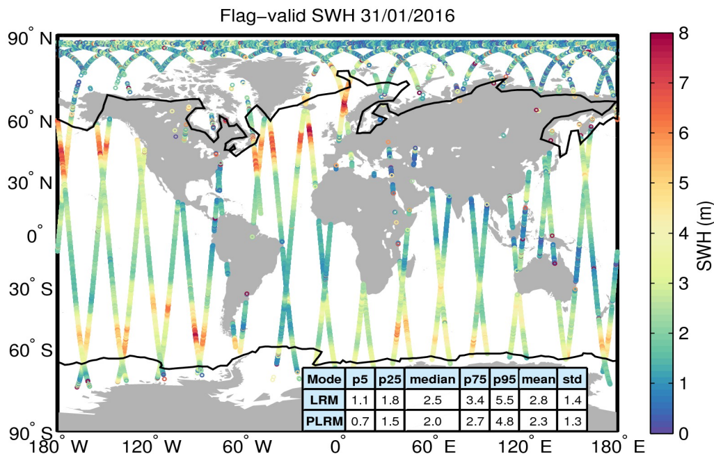
Figure 15. Geographical distribution of flag-valid SWH data over oceans and lakes for 31/01/2016. The statistical values shown in the table refer to the SWH in m and are calculated separately for LRM and PLRM regions. Measurements taken over polar polygons have been excluded from the computation of the statistical values. The black lines mark the outer limit of the Arctic and Antarctic polar polygons.
