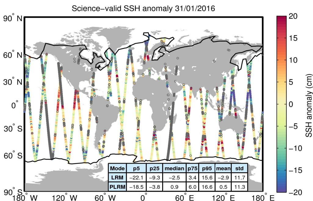
Figure 10. Geographical distribution of science-valid SSH anomaly data over oceans and lakes for 31/01/2016. The statistical values shown in the table refer to the SSH anomaly in cm and are calculated separately for LRM and PLRM regions. The black lines mark the outer limit of the Arctic and Antarctic polar polygons. Gray circles denote records that have been rejected based on the editing criteria described in Table 2.
