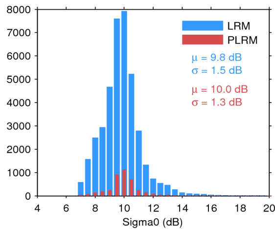
Figure 28. Histogram of science-valid sigma0 over oceans and lakes for LRM (blue) and PLRM (red) for 31/01/2016. The mean ( \mu ) and standard deviation ( \sigma ) are also shown. Note that values outside [4 20] dB are excluded from the histogram for the sake of readability but not from the computation of \mu and \sigma .
