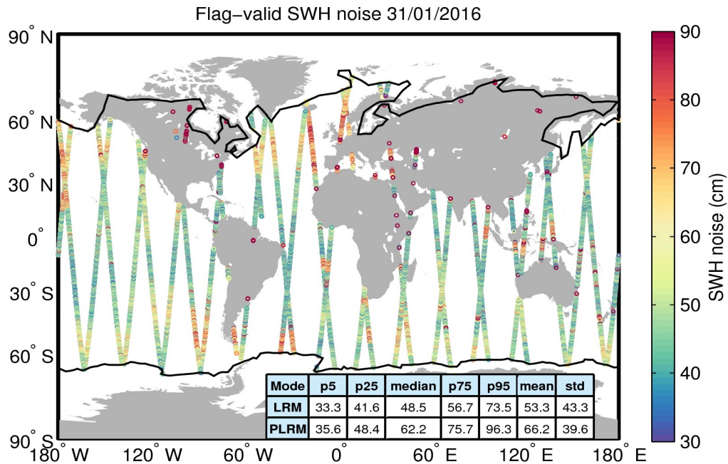
Figure 18. Geographical distribution of flag-valid 20-Hz SWH measurement noise over oceans and lakes for 31/01/2016. The statistical values shown in the table refer to the SWH noise and are calculated separately for LRM and PLRM regions. Measurements taken over polar polygons have been excluded from the computation of the statistical values. The black lines mark the outer limit of the Arctic and Antarctic polar polygons.
