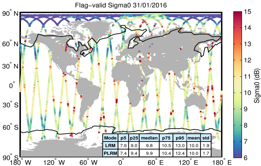
Figure 23. Geographical distribution of flag-valid sigma0 data over oceans and lakes for 31/01/2016. The statistical values shown in the table refer to the sigma0 in dB and are calculated separately for LRM and PLRM regions. Measurements taken over polar polygons have been excluded from the computation of the statistical values. The black lines mark the outer limit of the Arctic and Antarctic polar polygons.
