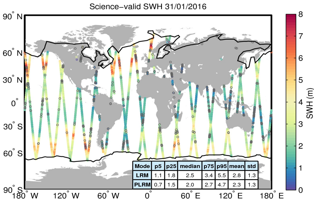
Figure 19. Geographical distribution of science-valid SWH data over oceans and lakes for 31/01/2016. The statistical values shown in the table refer to the SWH in m and are calculated separately for LRM and PLRM regions. The black lines mark the outer limit of the Arctic and Antarctic polar polygons. Gray circles denote records that have been rejected based on the editing criteria described in Table 3.
