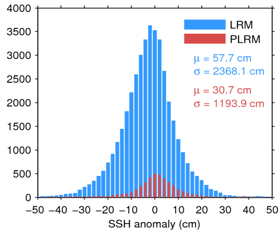
Figure 7. Histogram of flag-valid SSH anomaly over oceans and lakes for LRM (blue) and PLRM (red) for 31/01/2016. The mean ( \mu ) and standard deviation ( \sigma ) are also shown. Note that values outside [-50\ 50] cm are excluded from the histogram for the sake of readability but not from the computation of \mu and \sigma .
