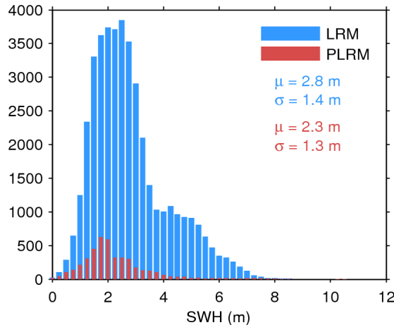
Figure 17. Histogram of flag-valid SWH over oceans and lakes for LRM (blue) and PLRM (red) for 31/01/2016. The mean ( \mu ) and standard deviation ( \sigma ) are also shown. Note that values larger than 12 m are excluded from the histogram for the sake of readability but not from the computation of \mu and \sigma .
