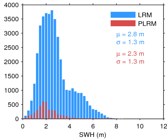
Figure 20. Histogram of science-valid SWH over oceans and lakes for LRM (blue) and PLRM (red) for 31/01/2016. The mean ( \mu ) and standard deviation ( \sigma ) are also shown. Note that values larger than 12 m are excluded from the histogram for the sake of readability but not from the computation of \mu and \sigma .
