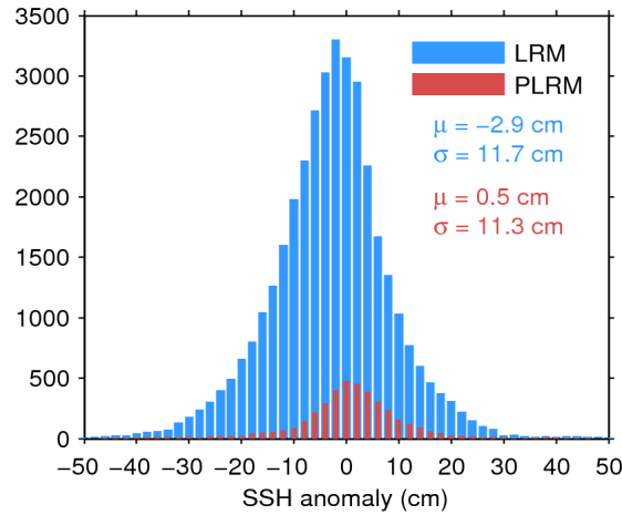
Figure 11. Histogram of science-valid SSH anomaly over oceans and lakes for LRM (blue) and PLRM (red) for 31/01/2016. The mean ( \mu ) and standard deviation ( \sigma ) are also shown. Note that values outside [-50\ 50] cm are excluded from the histogram for the sake of readability but not from the computation of \mu and \sigma .
