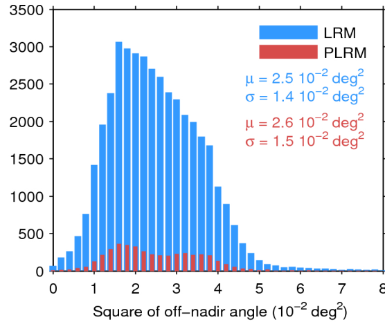
Figure 39. Histogram of flag-valid mispointing over oceans and lakes for LRM (blue) and PLRM (red) for 31/01/2016. Only positive values have been considered. The mean ( \mu ) and standard deviation ( \sigma ) are also shown. Note that values larger than 8 \cdot 10^{-2} \text{ deg}^2 are excluded from the histogram for the sake of readability but not from the computation of \mu and \sigma .
