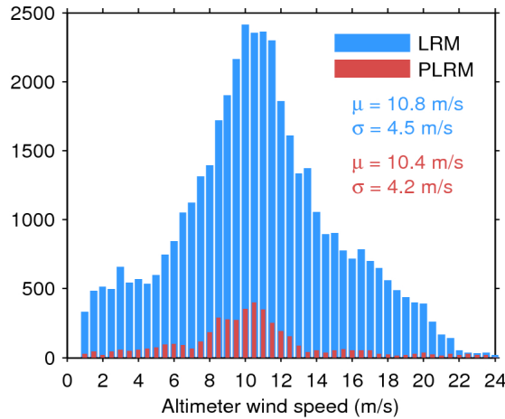
Figure 33. Histogram of flag-valid wind over oceans and lakes for LRM (blue) and PLRM (red) for 31/01/2016. The mean ( \mu ) and standard deviation ( \sigma ) are also shown. Note that values larger than 24 m/s are excluded from the histogram for the sake of readability but not from the computation of \mu and \sigma .
