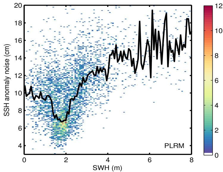
Figure 9. 2D histogram showing flag-valid SSH anomaly noise as a function of SWH for LRM (top) and PLRM (bottom) for 31/01/2016. The black line denotes the median SSH anomaly noise as a function of SWH.
