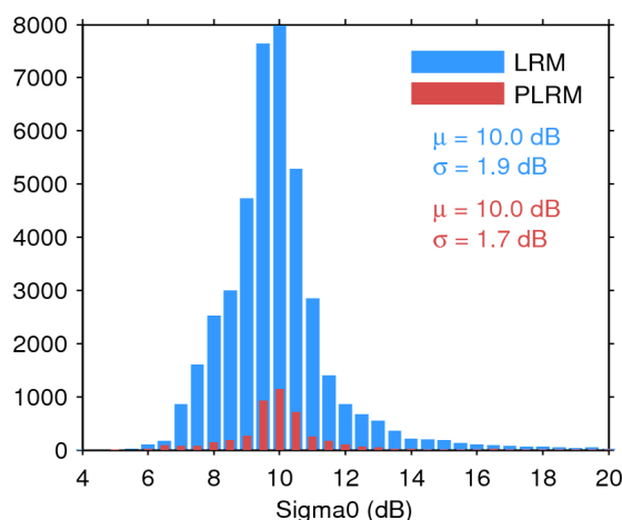
Figure 25. Histogram of flag-valid sigma0 over oceans and lakes for LRM (blue) and PLRM (red) for 31/01/2016. The mean ( \mu ) and standard deviation ( \sigma ) are also shown. Note that values outside [4 20] dB are excluded from the histogram for the sake of readability but not from the computation of \mu and \sigma .
