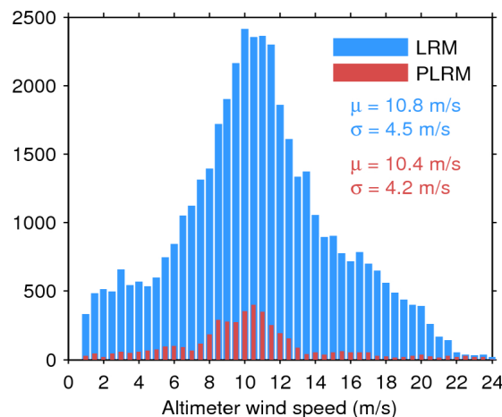
Figure 35. Histogram of science-valid wind over oceans and lakes for LRM (blue) and PLRM (red) for 31/01/2016. The mean ( \mu ) and standard deviation ( \sigma ) are also shown. Note that values larger than 24 m/s are excluded from the histogram for the sake of readability but not from the computation of \mu and \sigma .
