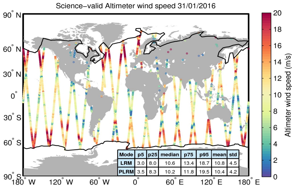
Figure 34. Geographical distribution of science-valid wind data over oceans and lakes for 31/01/2016. The statistical values shown in the table refer to the wind in m/s and are calculated separately for LRM and PLRM regions. The black lines mark the outer limit of the Arctic and Antarctic polar polygons. Gray circles denote records that have been rejected based on the editing criteria described in Table 5.
