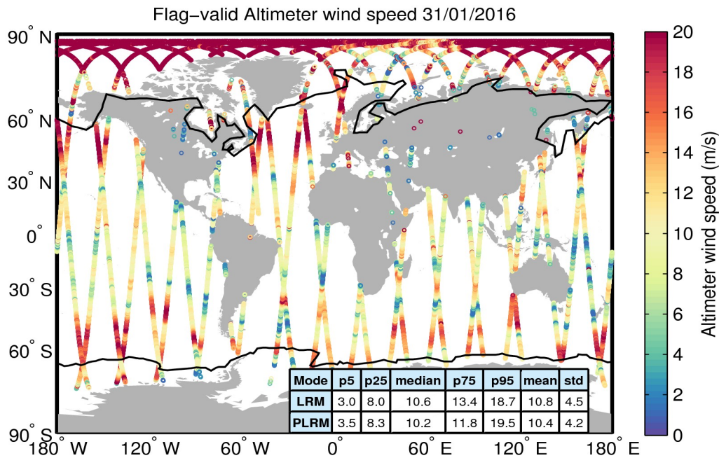
Figure 31. Geographical distribution of flag-valid wind data over oceans and lakes for 31/01/2016. The statistical values shown in the table refer to the wind in m/s and are calculated separately for LRM and PLRM regions. Measurements taken over polar polygons have been excluded from the computation of the statistical values. The black lines mark the outer limit of the Arctic and Antarctic polar polygons.
