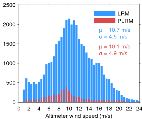
Figure 35. Histogram of science-valid wind over oceans and lakes for LRM (blue) and PLRM (red) for 29/01/2016. The mean ( \mu ) and standard deviation ( \sigma ) are also shown. Note that values larger than 24 m/s are excluded from the histogram for the sake of readability but not from the computation of \mu and \sigma .
