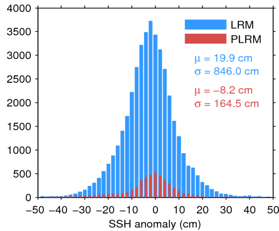
Figure 7. Histogram of flag-valid SSH anomaly over oceans and lakes for LRM (blue) and PLRM (red) for 29/01/2016. The mean ( \mu ) and standard deviation ( \sigma ) are also shown. Note that values outside [-50\ 50] cm are excluded from the histogram for the sake of readability but not from the computation of \mu and \sigma .
