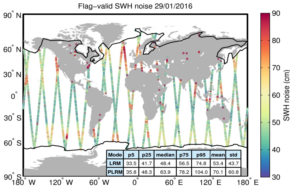
Figure 18. Geographical distribution of flag-valid 20-Hz SWH measurement noise over oceans and lakes for 29/01/2016. The statistical values shown in the table refer to the SWH noise and are calculated separately for LRM and PLRM regions. Measurements taken over polar polygons have been excluded from the computation of the statistical values. The black lines mark the outer limit of the Arctic and Antarctic polar polygons.
