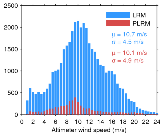
Figure 33. Histogram of flag-valid wind over oceans and lakes for LRM (blue) and PLRM (red) for 29/01/2016. The mean ( \mu ) and standard deviation ( \sigma ) are also shown. Note that values larger than 24 m/s are excluded from the histogram for the sake of readability but not from the computation of \mu and \sigma .
