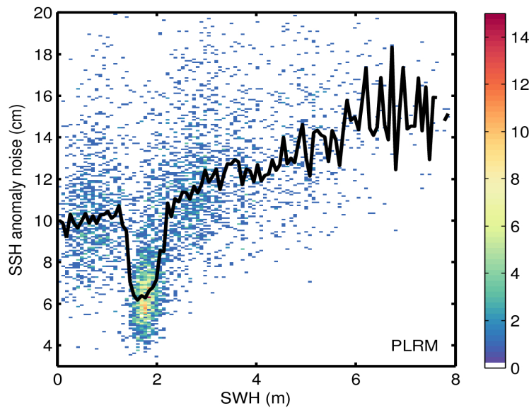
Figure 9. 2D histogram showing flag-valid SSH anomaly noise as a function of SWH for LRM (top) and PLRM (bottom) for 29/01/2016. The black line denotes the median SSH anomaly noise as a function of SWH.
