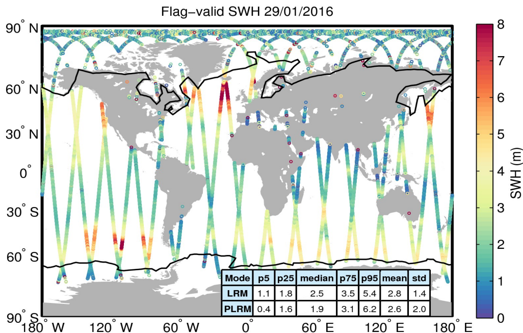
Figure 15. Geographical distribution of flag-valid SWH data over oceans and lakes for 29/01/2016. The statistical values shown in the table refer to the SWH in m and are calculated separately for LRM and PLRM regions. Measurements taken over polar polygons have been excluded from the computation of the statistical values. The black lines mark the outer limit of the Arctic and Antarctic polar polygons.
