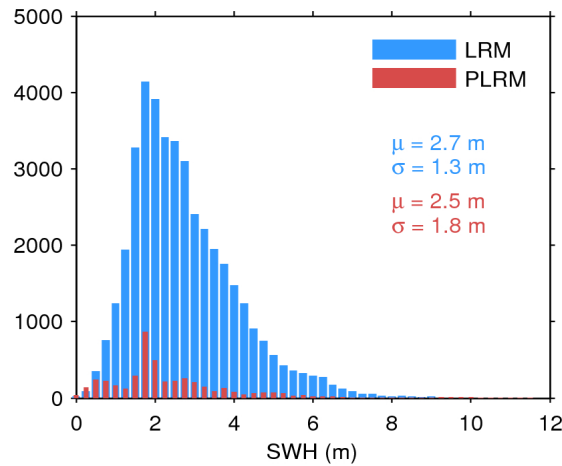
Figure 20. Histogram of science-valid SWH over oceans and lakes for LRM (blue) and PLRM (red) for 29/01/2016. The mean ( \mu ) and standard deviation ( \sigma ) are also shown. Note that values larger than 12 m are excluded from the histogram for the sake of readability but not from the computation of \mu and \sigma .
