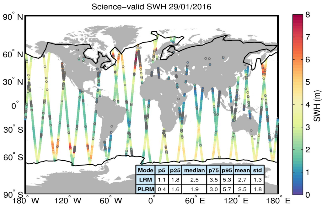
Figure 19. Geographical distribution of science-valid SWH data over oceans and lakes for 29/01/2016. The statistical values shown in the table refer to the SWH in m and are calculated separately for LRM and PLRM regions. The black lines mark the outer limit of the Arctic and Antarctic polar polygons. Gray circles denote records that have been rejected based on the editing criteria described in Table 3.
