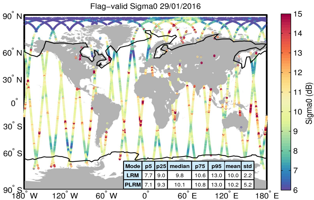
Figure 23. Geographical distribution of flag-valid sigma0 data over oceans and lakes for 29/01/2016. The statistical values shown in the table refer to the sigma0 in dB and are calculated separately for LRM and PLRM regions. Measurements taken over polar polygons have been excluded from the computation of the statistical values. The black lines mark the outer limit of the Arctic and Antarctic polar polygons.
