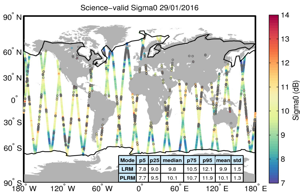
Figure 27. Geographical distribution of science-valid sigma0 data over oceans and lakes for 29/01/2016. The statistical values shown in the table refer to the sigma0 in dB and are calculated separately for LRM and PLRM regions. The black lines mark the outer limit of the Arctic and Antarctic polar polygons. Gray circles denote records that have been rejected based on the editing criteria described in Table 4.
