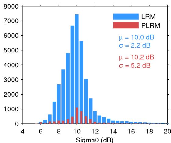
Figure 25. Histogram of flag-valid sigma0 over oceans and lakes for LRM (blue) and PLRM (red) for 29/01/2016. The mean ( \mu ) and standard deviation ( \sigma ) are also shown. Note that values outside [4 20] dB are excluded from the histogram for the sake of readability but not from the computation of \mu and \sigma .
