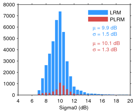
Figure 28. Histogram of science-valid sigma0 over oceans and lakes for LRM (blue) and PLRM (red) for 29/01/2016. The mean ( \mu ) and standard deviation ( \sigma ) are also shown. Note that values outside [4 20] dB are excluded from the histogram for the sake of readability but not from the computation of \mu and \sigma .
