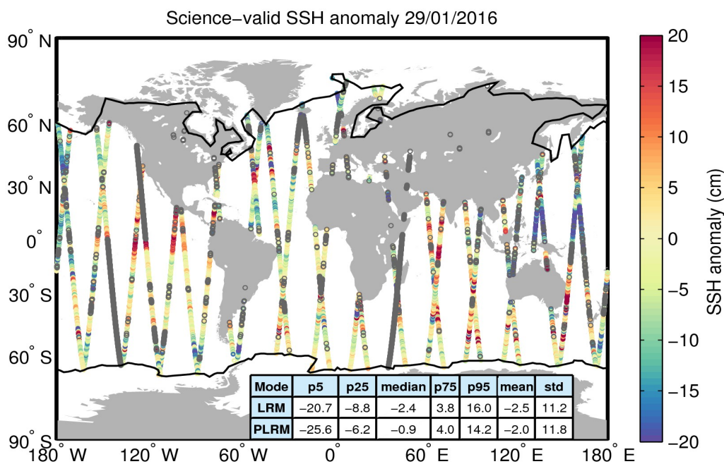
Figure 10. Geographical distribution of science-valid SSH anomaly data over oceans and lakes for 29/01/2016. The statistical values shown in the table refer to the SSH anomaly in cm and are calculated separately for LRM and PLRM regions. The black lines mark the outer limit of the Arctic and Antarctic polar polygons. Gray circles denote records that have been rejected based on the editing criteria described in Table 2.
