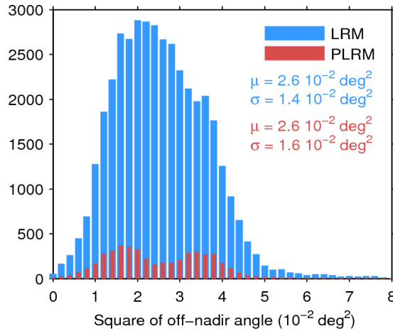
Figure 39. Histogram of flag-valid mispointing over oceans and lakes for LRM (blue) and PLRM (red) for 29/01/2016. Only positive values have been considered. The mean ( \mu ) and standard deviation ( \sigma ) are also shown. Note that values larger than 8 \cdot 10^{-2} \text{ deg}^2 are excluded from the histogram for the sake of readability but not from the computation of \mu and \sigma .
