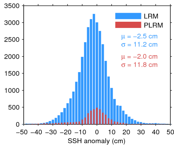
Figure 11. Histogram of science-valid SSH anomaly over oceans and lakes for LRM (blue) and PLRM (red) for 29/01/2016. The mean ( \mu ) and standard deviation ( \sigma ) are also shown. Note that values outside [-50 50] cm are excluded from the histogram for the sake of readability but not from the computation of \mu and \sigma .
