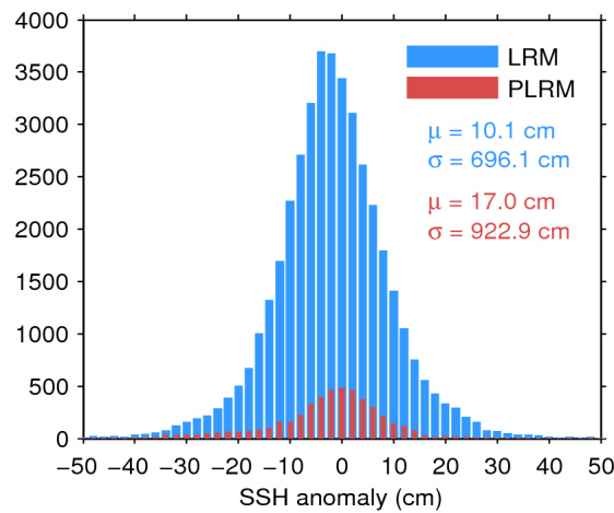
Figure 7. Histogram of flag-valid SSH anomaly over oceans and lakes for LRM (blue) and PLRM (red) for 25/01/2016. The mean ( \mu ) and standard deviation ( \sigma ) are also shown. Note that values outside [-50\ 50] cm are excluded from the histogram for the sake of readability but not from the computation of \mu and \sigma .
