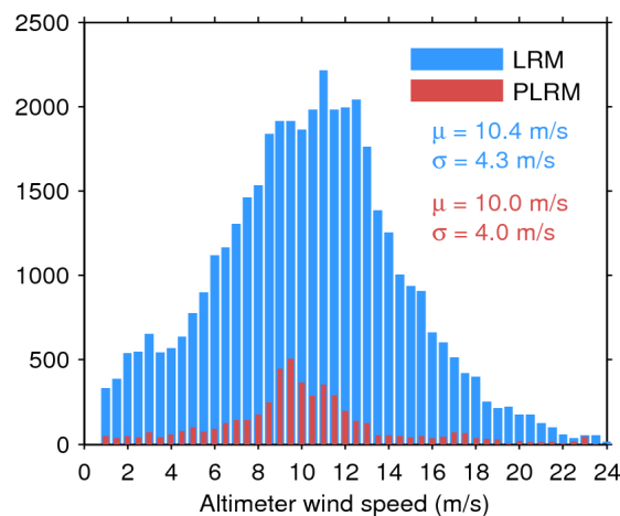
Figure 35. Histogram of science-valid wind over oceans and lakes for LRM (blue) and PLRM (red) for 25/01/2016. The mean ( \mu ) and standard deviation ( \sigma ) are also shown. Note that values larger than 24 m/s are excluded from the histogram for the sake of readability but not from the computation of \mu and \sigma .
