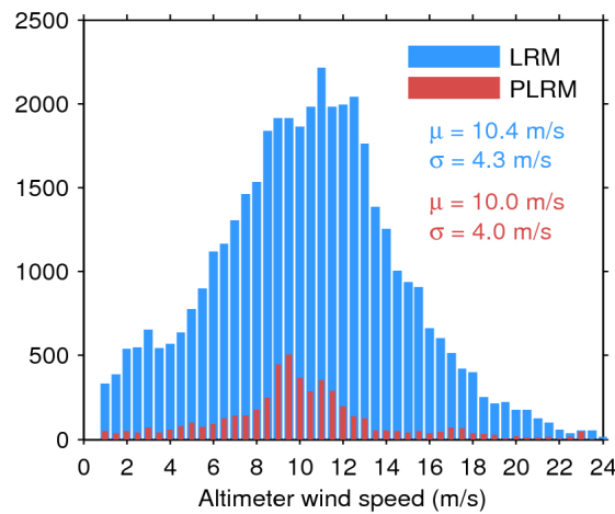
Figure 33. Histogram of flag-valid wind over oceans and lakes for LRM (blue) and PLRM (red) for 25/01/2016. The mean ( \mu ) and standard deviation ( \sigma ) are also shown. Note that values larger than 24 m/s are excluded from the histogram for the sake of readability but not from the computation of \mu and \sigma .
