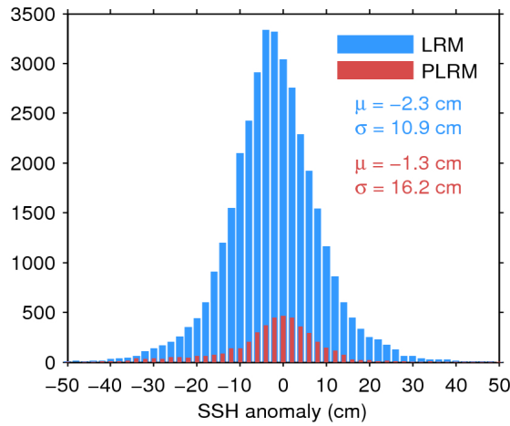
Figure 11. Histogram of science-valid SSH anomaly over oceans and lakes for LRM (blue) and PLRM (red) for 25/01/2016. The mean ( \mu ) and standard deviation ( \sigma ) are also shown. Note that values outside [-50\ 50] cm are excluded from the histogram for the sake of readability but not from the computation of \mu and \sigma .
