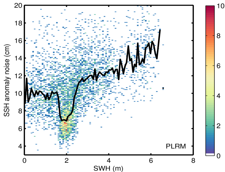
Figure 9. 2D histogram showing flag-valid SSH anomaly noise as a function of SWH for LRM (top) and PLRM (bottom) for 25/01/2016. The black line denotes the median SSH anomaly noise as a function of SWH.
