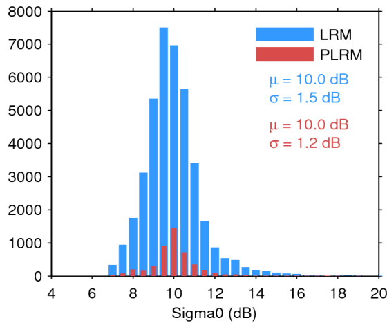
Figure 28. Histogram of science-valid sigma0 over oceans and lakes for LRM (blue) and PLRM (red) for 25/01/2016. The mean ( \mu ) and standard deviation ( \sigma ) are also shown. Note that values outside [4 20] dB are excluded from the histogram for the sake of readability but not from the computation of \mu and \sigma .
