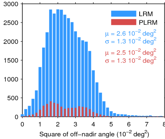
Figure 39. Histogram of flag-valid mispointing over oceans and lakes for LRM (blue) and PLRM (red) for 25/01/2016. Only positive values have been considered. The mean ( \mu ) and standard deviation ( \sigma ) are also shown. Note that values larger than 8 \times 10^{-2} \text{ deg}^2 are excluded from the histogram for the sake of readability but not from the computation of \mu and \sigma .
