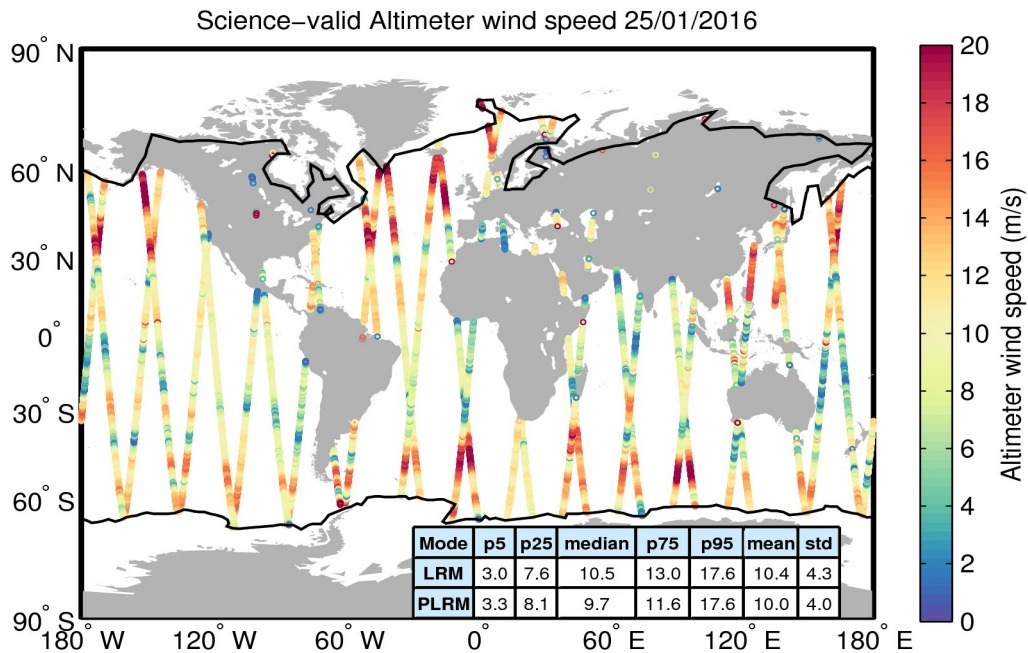
Figure 34. Geographical distribution of science-valid wind data over oceans and lakes for 25/01/2016. The statistical values shown in the table refer to the wind in m/s and are calculated separately for LRM and PLRM regions. The black lines mark the outer limit of the Arctic and Antarctic polar polygons. Gray circles denote records that have been rejected based on the editing criteria described in Table 5.
