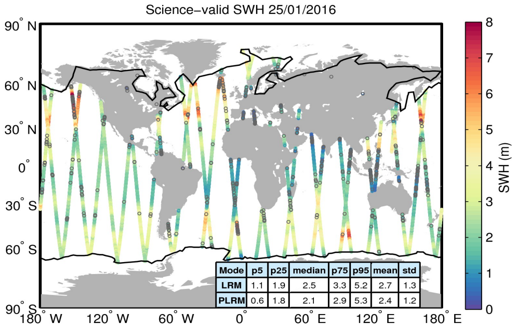
Figure 19. Geographical distribution of science-valid SWH data over oceans and lakes for 25/01/2016. The statistical values shown in the table refer to the SWH in m and are calculated separately for LRM and PLRM regions. The black lines mark the outer limit of the Arctic and Antarctic polar polygons. Gray circles denote records that have been rejected based on the editing criteria described in Table 3.
