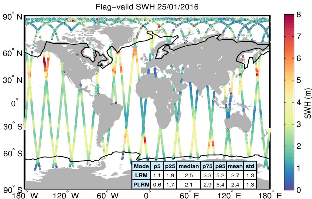
Figure 15. Geographical distribution of flag-valid SWH data over oceans and lakes for 25/01/2016. The statistical values shown in the table refer to the SWH in m and are calculated separately for LRM and PLRM regions. Measurements taken over polar polygons have been excluded from the computation of the statistical values. The black lines mark the outer limit of the Arctic and Antarctic polar polygons.
