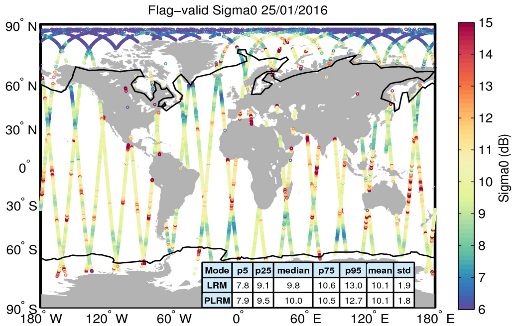
Figure 23. Geographical distribution of flag-valid sigma0 data over oceans and lakes for 25/01/2016. The statistical values shown in the table refer to the sigma0 in dB and are calculated separately for LRM and PLRM regions. Measurements taken over polar polygons have been excluded from the computation of the statistical values. The black lines mark the outer limit of the Arctic and Antarctic polar polygons.
