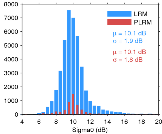
Figure 25. Histogram of flag-valid sigma0 over oceans and lakes for LRM (blue) and PLRM (red) for 25/01/2016. The mean ( \mu ) and standard deviation ( \sigma ) are also shown. Note that values outside [4 20] dB are excluded from the histogram for the sake of readability but not from the computation of \mu and \sigma .
