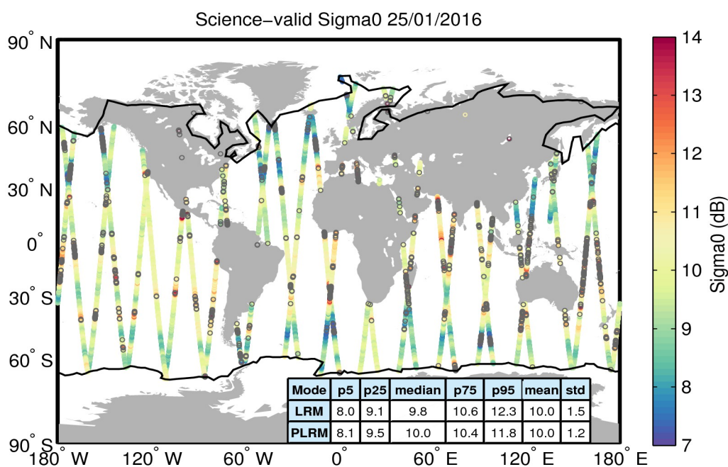
Figure 27. Geographical distribution of science-valid sigma0 data over oceans and lakes for 25/01/2016. The statistical values shown in the table refer to the sigma0 in dB and are calculated separately for LRM and PLRM regions. The black lines mark the outer limit of the Arctic and Antarctic polar polygons. Gray circles denote records that have been rejected based on the editing criteria described in Table 4.
