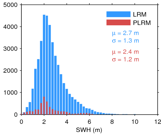
Figure 20. Histogram of science-valid SWH over oceans and lakes for LRM (blue) and PLRM (red) for 25/01/2016. The mean ( \mu ) and standard deviation ( \sigma ) are also shown. Note that values larger than 12 m are excluded from the histogram for the sake of readability but not from the computation of \mu and \sigma .
