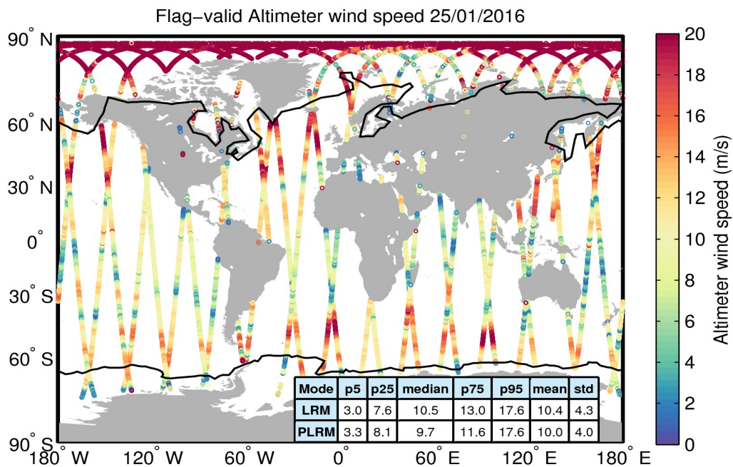
Figure 31. Geographical distribution of flag-valid wind data over oceans and lakes for 25/01/2016. The statistical values shown in the table refer to the wind in m/s and are calculated separately for LRM and PLRM regions. Measurements taken over polar polygons have been excluded from the computation of the statistical values. The black lines mark the outer limit of the Arctic and Antarctic polar polygons.
