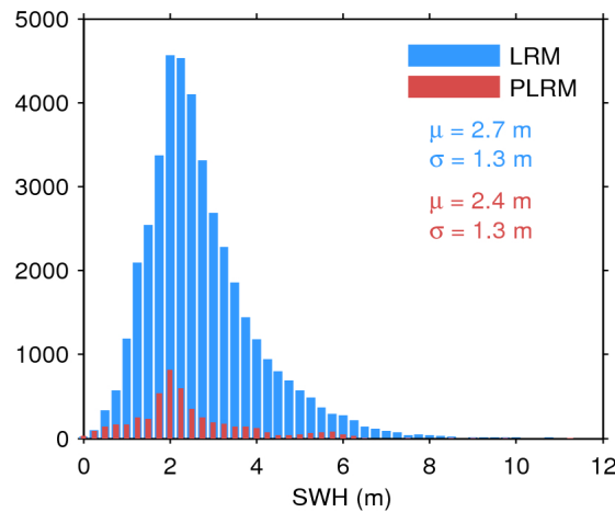
Figure 17. Histogram of flag-valid SWH over oceans and lakes for LRM (blue) and PLRM (red) for 25/01/2016. The mean ( \mu ) and standard deviation ( \sigma ) are also shown. Note that values larger than 12 m are excluded from the histogram for the sake of readability but not from the computation of \mu and \sigma .
