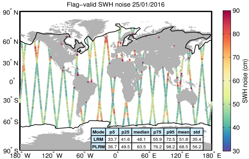
Figure 18. Geographical distribution of flag-valid 20-Hz SWH measurement noise over oceans and lakes for 25/01/2016. The statistical values shown in the table refer to the SWH noise and are calculated separately for LRM and PLRM regions. Measurements taken over polar polygons have been excluded from the computation of the statistical values. The black lines mark the outer limit of the Arctic and Antarctic polar polygons.
