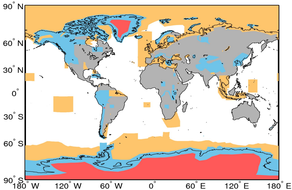
Figure A1. Extent of the regions defining the geographical mode mask for 25/01/2016. The regions where SAR, and SARIn are operated are denoted by the orange and blue polygons, respectively. LRM is operated over areas of the continental ice sheets (red polygons) and over oceans and land not covered by other modes.
