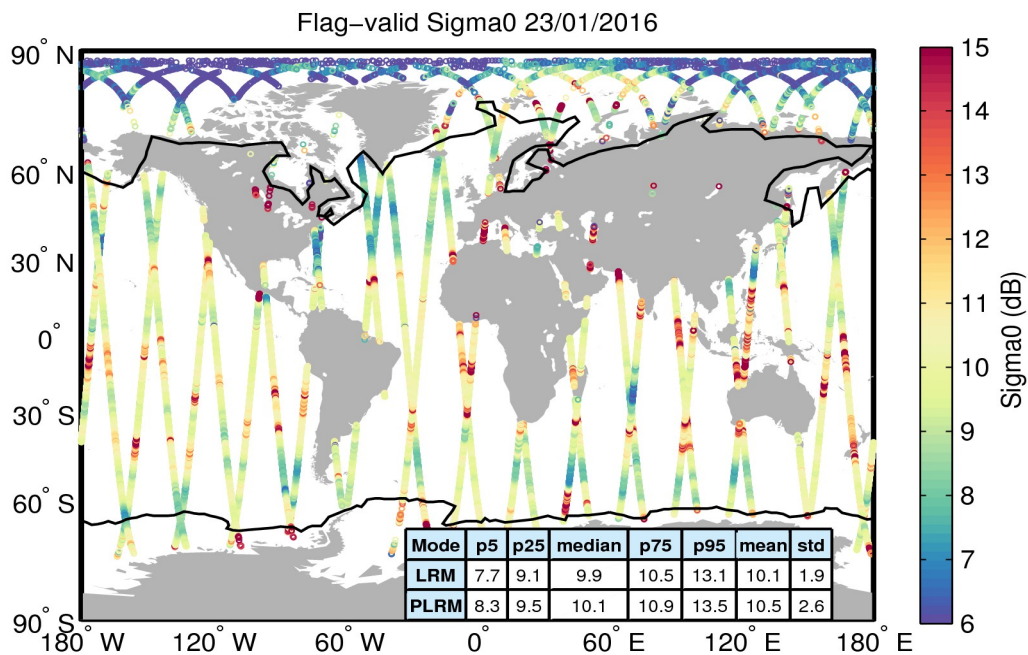
Figure 23. Geographical distribution of flag-valid sigma0 data over oceans and lakes for 23/01/2016. The statistical values shown in the table refer to the sigma0 in dB and are calculated separately for LRM and PLRM regions. Measurements taken over polar polygons have been excluded from the computation of the statistical values. The black lines mark the outer limit of the Arctic and Antarctic polar polygons.
