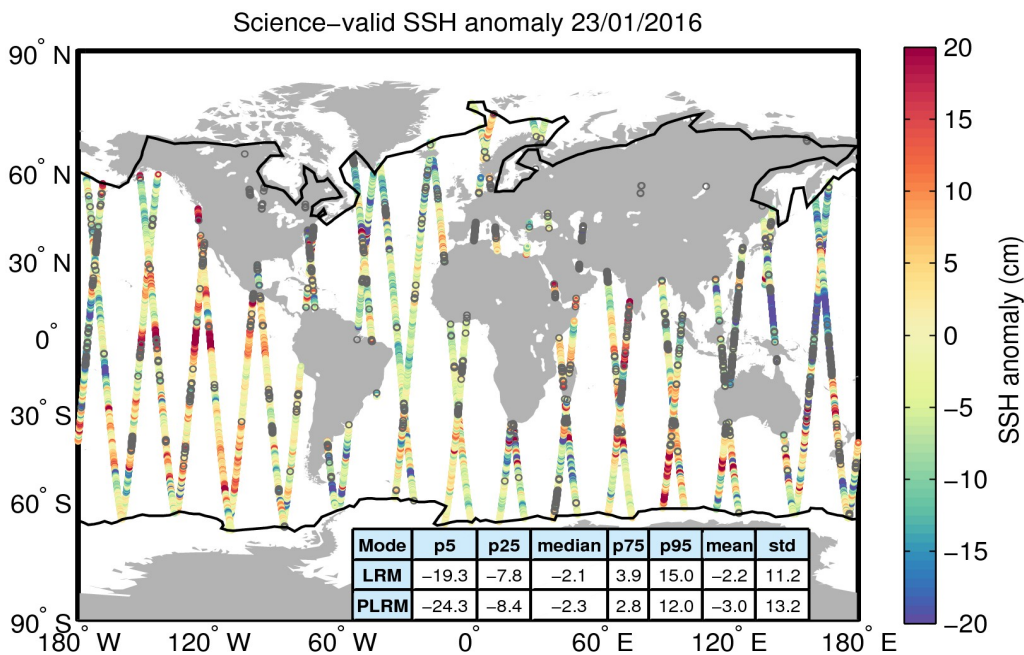
Figure 10. Geographical distribution of science-valid SSH anomaly data over oceans and lakes for 23/01/2016. The statistical values shown in the table refer to the SSH anomaly in cm and are calculated separately for LRM and PLRM regions. The black lines mark the outer limit of the Arctic and Antarctic polar polygons. Gray circles denote records that have been rejected based on the editing criteria described in Table 2.
