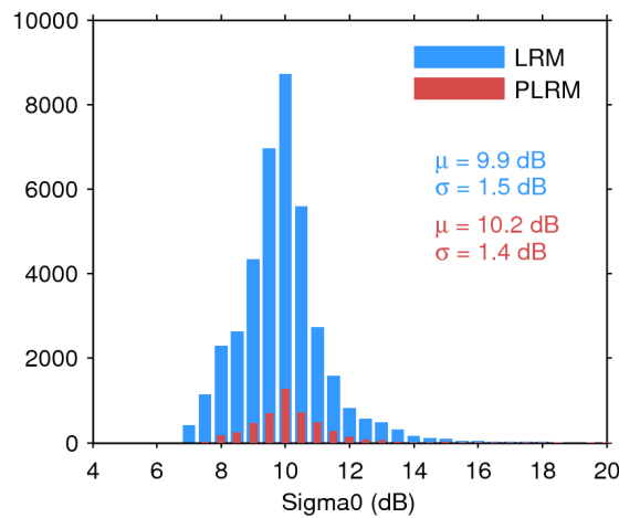
Figure 28. Histogram of science-valid sigma0 over oceans and lakes for LRM (blue) and PLRM (red) for 23/01/2016. The mean ( \mu ) and standard deviation ( \sigma ) are also shown. Note that values outside [4 20] dB are excluded from the histogram for the sake of readability but not from the computation of \mu and \sigma .
