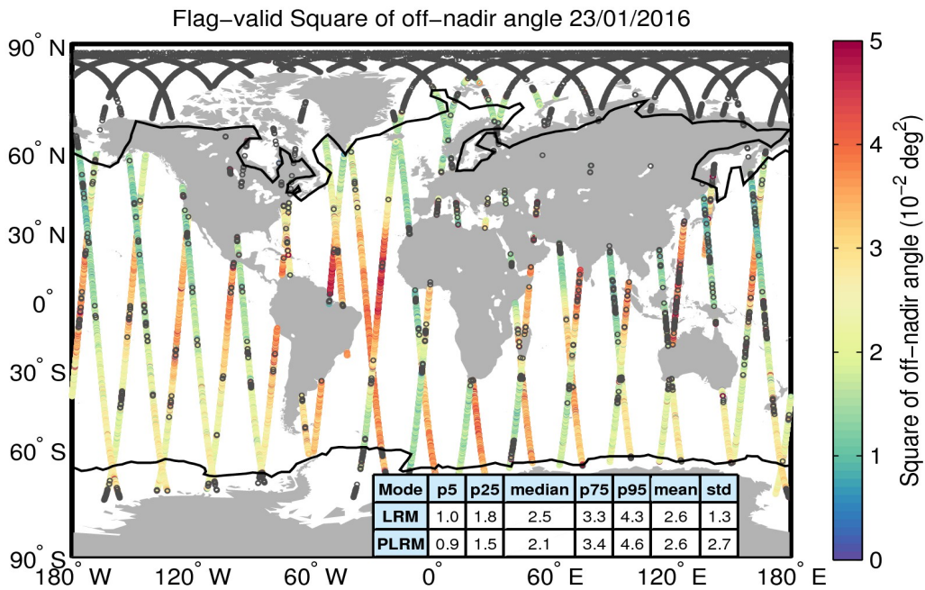
Figure 37. Geographical distribution of flag-valid mispointing data over oceans and lakes for 23/01/2016. The statistical values shown in the table refer to the mispointing in 10^{-2} deg 2 and are calculated separately for LRM and PLRM regions. Measurements taken over polar polygons have been excluded from the computation of the statistical values. The black lines mark the outer limit of the Arctic and Antarctic polar polygons. Gray circles denote negative values.
