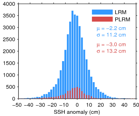
Figure 11. Histogram of science-valid SSH anomaly over oceans and lakes for LRM (blue) and PLRM (red) for 23/01/2016. The mean ( \mu ) and standard deviation ( \sigma ) are also shown. Note that values outside [-50 50] cm are excluded from the histogram for the sake of readability but not from the computation of \mu and \sigma .
