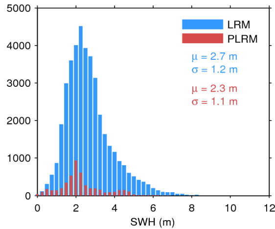
Figure 20. Histogram of science-valid SWH over oceans and lakes for LRM (blue) and PLRM (red) for 23/01/2016. The mean ( \mu ) and standard deviation ( \sigma ) are also shown. Note that values larger than 12 m are excluded from the histogram for the sake of readability but not from the computation of \mu and \sigma .
