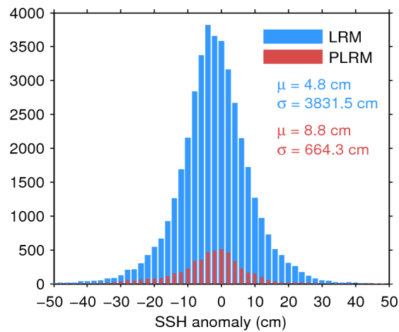
Figure 7. Histogram of flag-valid SSH anomaly over oceans and lakes for LRM (blue) and PLRM (red) for 23/01/2016. The mean ( \mu ) and standard deviation ( \sigma ) are also shown. Note that values outside [-50\ 50] cm are excluded from the histogram for the sake of readability but not from the computation of \mu and \sigma .
