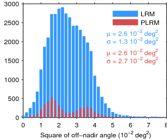
Figure 39. Histogram of flag-valid mispointing over oceans and lakes for LRM (blue) and PLRM (red) for 23/01/2016. Only positive values have been considered. The mean ( \mu ) and standard deviation ( \sigma ) are also shown. Note that values larger than 8 \cdot 10^{-2} \text{ deg}^2 are excluded from the histogram for the sake of readability but not from the computation of \mu and \sigma .
