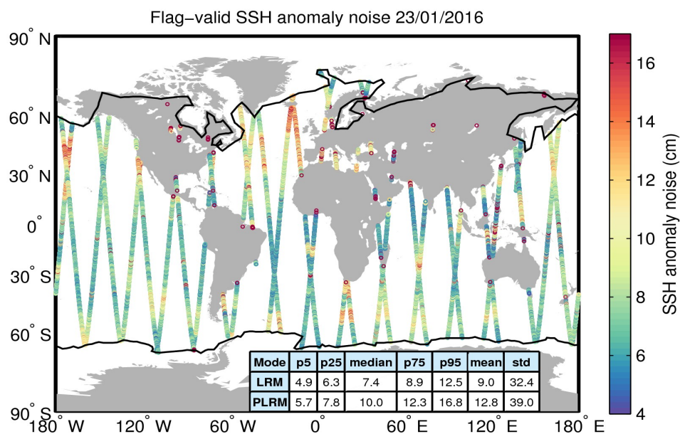
Figure 8. Geographical distribution of flag-valid 20-Hz SSH anomaly measurement noise over oceans and lakes for 23/01/2016. The statistical values shown in the table refer to the SSH anomaly noise and are calculated separately for LRM and PLRM regions. Measurements taken over polar polygons have been excluded from the computation of the statistical values. The black lines mark the outer limit of the Arctic and Antarctic polar polygons.
