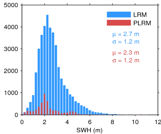
Figure 17. Histogram of flag-valid SWH over oceans and lakes for LRM (blue) and PLRM (red) for 23/01/2016. The mean ( \mu ) and standard deviation ( \sigma ) are also shown. Note that values larger than 12 m are excluded from the histogram for the sake of readability but not from the computation of \mu and \sigma .
