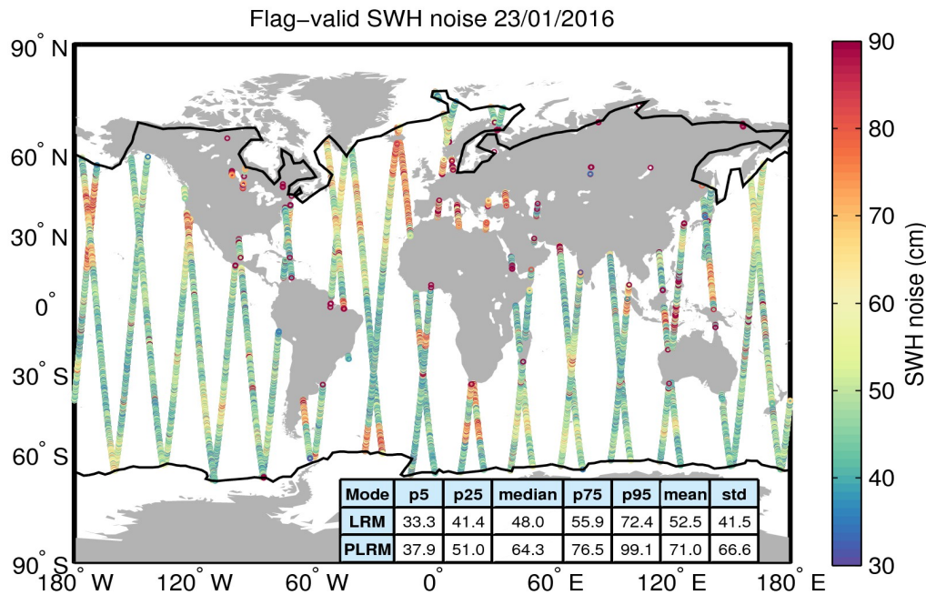
Figure 18. Geographical distribution of flag-valid 20-Hz SWH measurement noise over oceans and lakes for 23/01/2016. The statistical values shown in the table refer to the SWH noise and are calculated separately for LRM and PLRM regions. Measurements taken over polar polygons have been excluded from the computation of the statistical values. The black lines mark the outer limit of the Arctic and Antarctic polar polygons.
