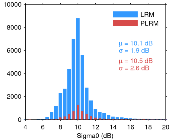
Figure 25. Histogram of flag-valid sigma0 over oceans and lakes for LRM (blue) and PLRM (red) for 23/01/2016. The mean ( \mu ) and standard deviation ( \sigma ) are also shown. Note that values outside [4 20] dB are excluded from the histogram for the sake of readability but not from the computation of \mu and \sigma .
