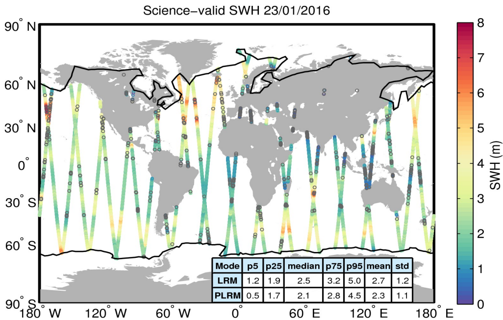
Figure 19. Geographical distribution of science-valid SWH data over oceans and lakes for 23/01/2016. The statistical values shown in the table refer to the SWH in m and are calculated separately for LRM and PLRM regions. The black lines mark the outer limit of the Arctic and Antarctic polar polygons. Gray circles denote records that have been rejected based on the editing criteria described in Table 3.
