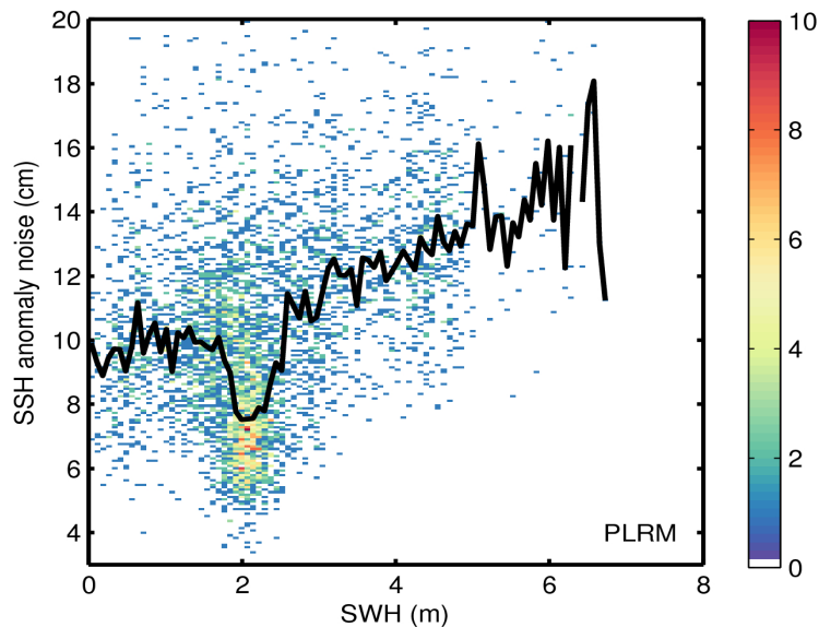
Figure 9. 2D histogram showing flag-valid SSH anomaly noise as a function of SWH for LRM (top) and PLRM (bottom) for 23/01/2016. The black line denotes the median SSH anomaly noise as a function of SWH.
