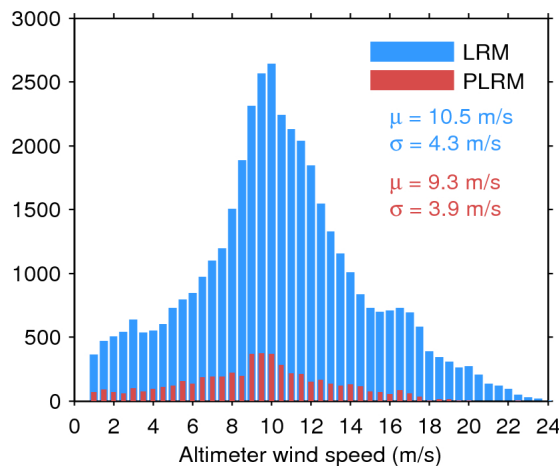
Figure 35. Histogram of science-valid wind over oceans and lakes for LRM (blue) and PLRM (red) for 23/01/2016. The mean ( \mu ) and standard deviation ( \sigma ) are also shown. Note that values larger than 24 m/s are excluded from the histogram for the sake of readability but not from the computation of \mu and \sigma .
