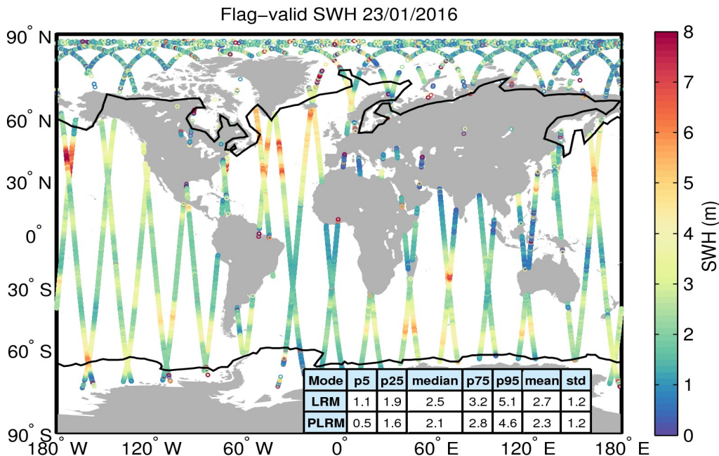
Figure 15. Geographical distribution of flag-valid SWH data over oceans and lakes for 23/01/2016. The statistical values shown in the table refer to the SWH in m and are calculated separately for LRM and PLRM regions. Measurements taken over polar polygons have been excluded from the computation of the statistical values. The black lines mark the outer limit of the Arctic and Antarctic polar polygons.
