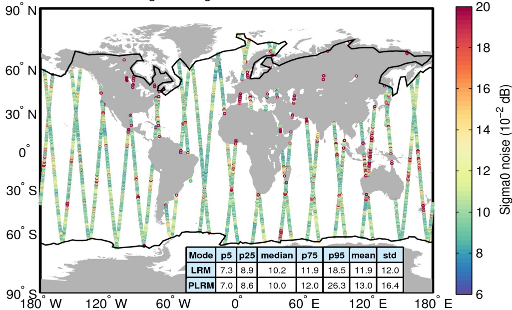
Flag-valid sigma0 noise 23/01/2016
