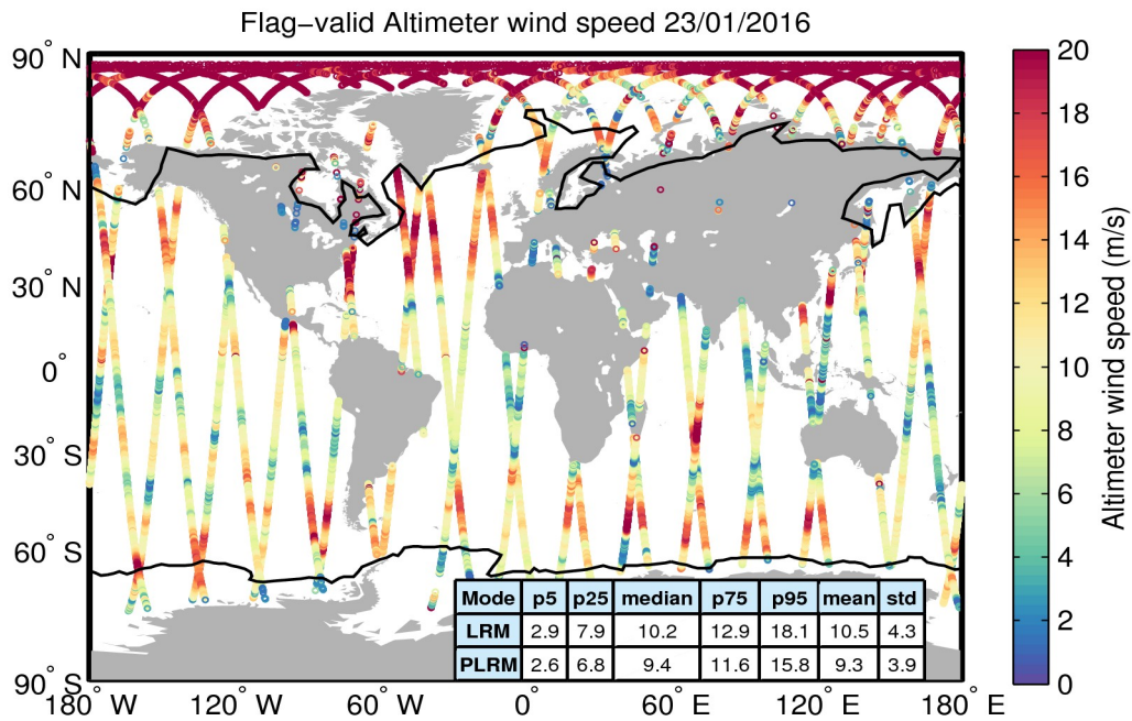
Figure 31. Geographical distribution of flag-valid wind data over oceans and lakes for 23/01/2016. The statistical values shown in the table refer to the wind in m/s and are calculated separately for LRM and PLRM regions. Measurements taken over polar polygons have been excluded from the computation of the statistical values. The black lines mark the outer limit of the Arctic and Antarctic polar polygons.
