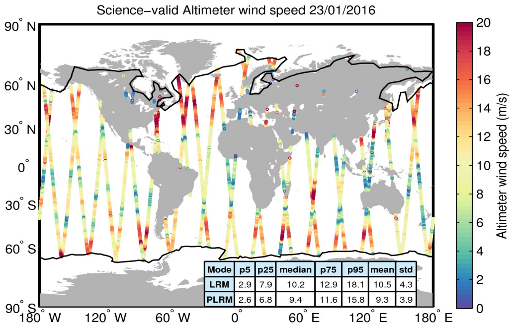
Figure 34. Geographical distribution of science-valid wind data over oceans and lakes for 23/01/2016. The statistical values shown in the table refer to the wind in m/s and are calculated separately for LRM and PLRM regions. The black lines mark the outer limit of the Arctic and Antarctic polar polygons. Gray circles denote records that have been rejected based on the editing criteria described in Table 5.
