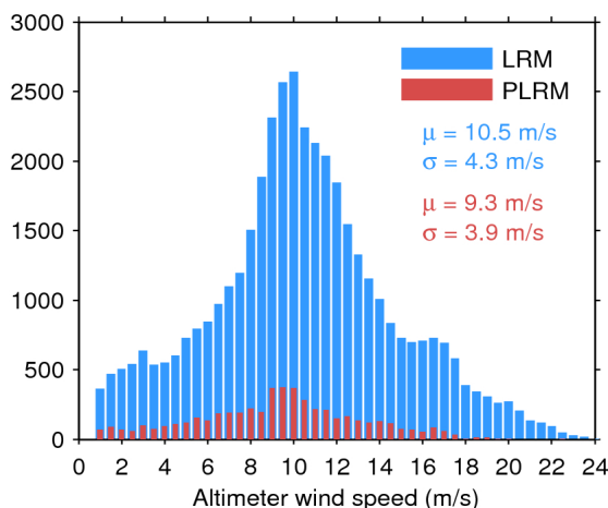
Figure 33. Histogram of flag-valid wind over oceans and lakes for LRM (blue) and PLRM (red) for 23/01/2016. The mean ( \mu ) and standard deviation ( \sigma ) are also shown. Note that values larger than 24 m/s are excluded from the histogram for the sake of readability but not from the computation of \mu and \sigma .
