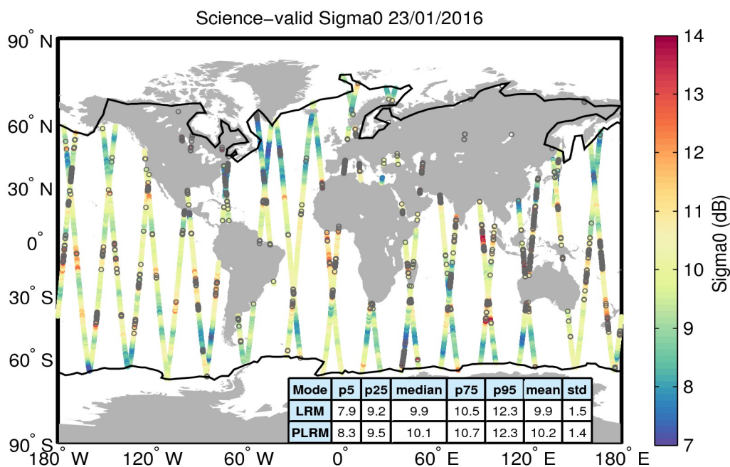
Figure 27. Geographical distribution of science-valid sigma0 data over oceans and lakes for 23/01/2016. The statistical values shown in the table refer to the sigma0 in dB and are calculated separately for LRM and PLRM regions. The black lines mark the outer limit of the Arctic and Antarctic polar polygons. Gray circles denote records that have been rejected based on the editing criteria described in Table 4.
