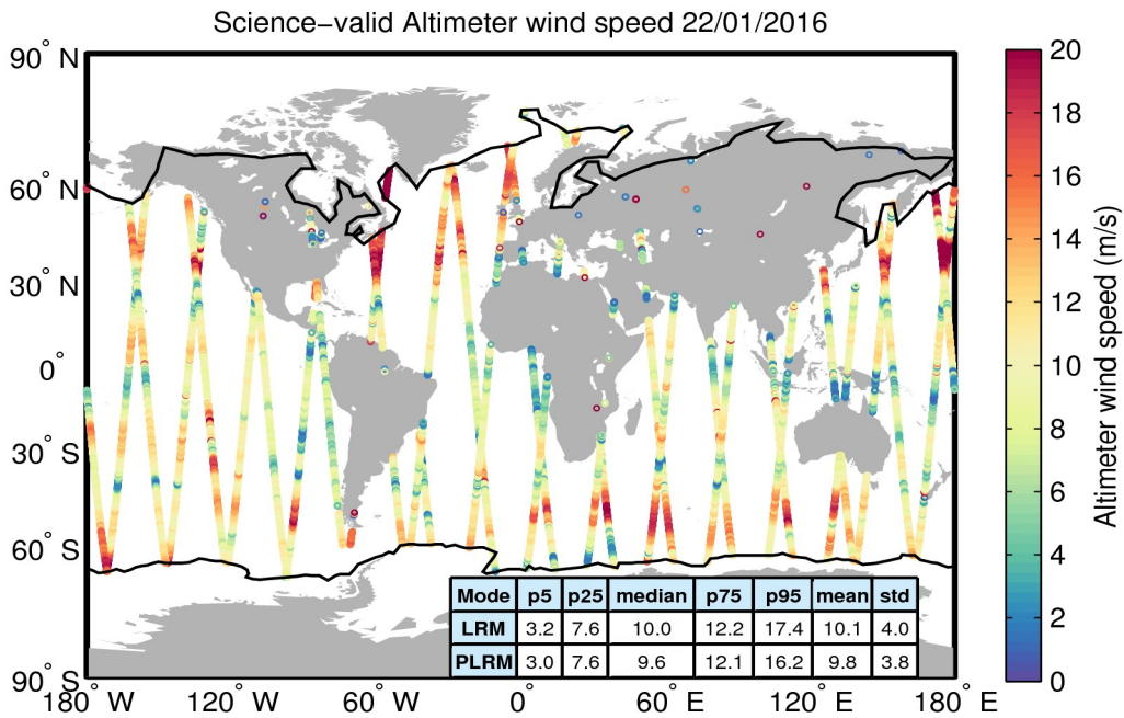
Figure 34. Geographical distribution of science-valid wind data over oceans and lakes for 22/01/2016. The statistical values shown in the table refer to the wind in m/s and are calculated separately for LRM and PLRM regions. The black lines mark the outer limit of the Arctic and Antarctic polar polygons. Gray circles denote records that have been rejected based on the editing criteria described in Table 5.
