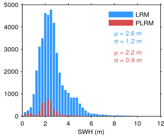
Figure 20. Histogram of science-valid SWH over oceans and lakes for LRM (blue) and PLRM (red) for 22/01/2016. The mean ( \mu ) and standard deviation ( \sigma ) are also shown. Note that values larger than 12 m are excluded from the histogram for the sake of readability but not from the computation of \mu and \sigma .
