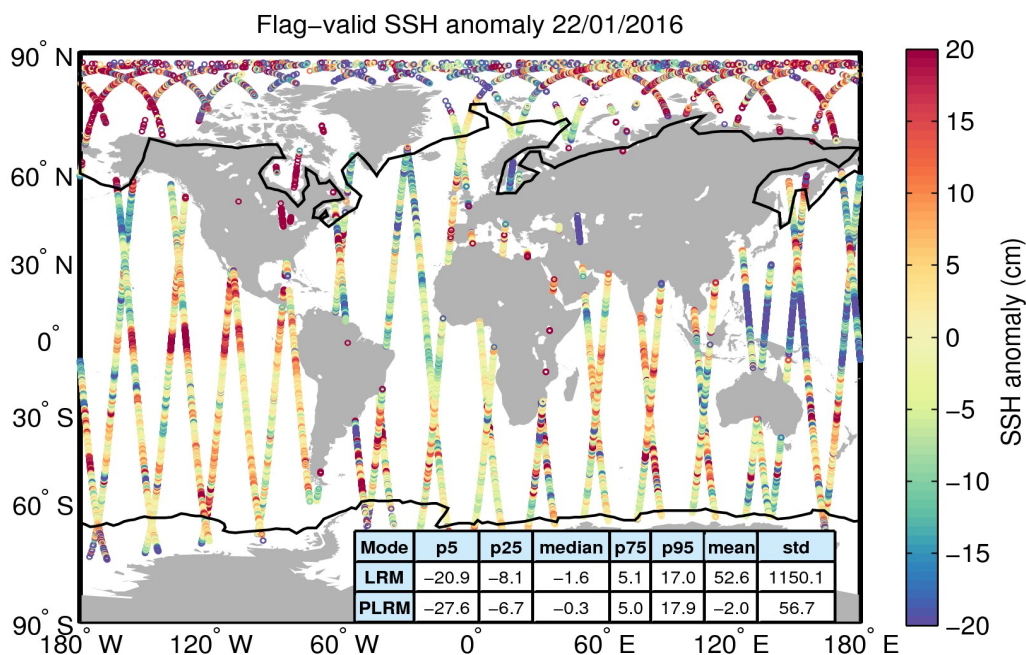
Figure 5. Geographical distribution of flag-valid 1-Hz SSH anomaly data over oceans and lakes for 22/01/2016. The statistical values shown in the table refer to the SSH anomaly in cm and are calculated separately for LRM and PLRM regions. Measurements taken over polar polygons have been excluded from the computation of the statistical values. The black lines mark the outer limit of the Arctic and Antarctic polar polygons.
