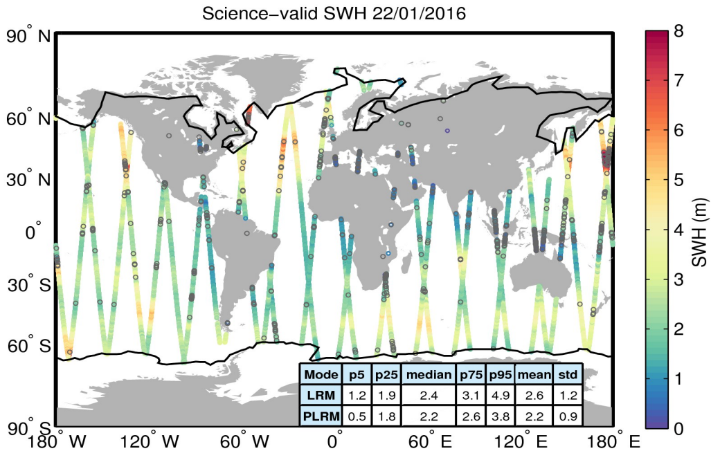
Figure 19. Geographical distribution of science-valid SWH data over oceans and lakes for 22/01/2016. The statistical values shown in the table refer to the SWH in m and are calculated separately for LRM and PLRM regions. The black lines mark the outer limit of the Arctic and Antarctic polar polygons. Gray circles denote records that have been rejected based on the editing criteria described in Table 3.
