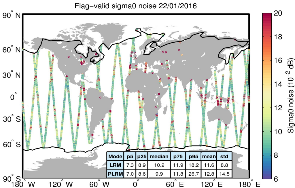
Figure 26. Geographical distribution of flag-valid 20-Hz sigma0 measurement noise over oceans and lakes for 22/01/2016. The statistical values shown in the table refer to the sigma0 noise and are calculated separately for LRM and PLRM regions. Measurements taken over polar polygons have been excluded from the computation of the statistical values. The black lines mark the outer limit of the Arctic and Antarctic polar polygons.
