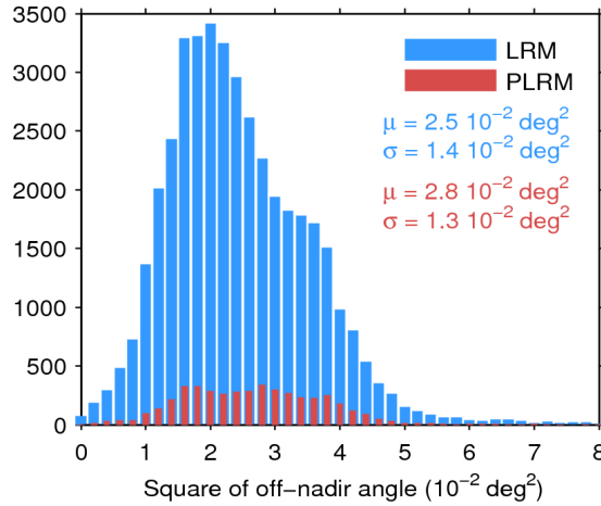
Figure 39. Histogram of flag-valid mispointing over oceans and lakes for LRM (blue) and PLRM (red) for 22/01/2016. Only positive values have been considered. The mean ( \mu ) and standard deviation ( \sigma ) are also shown. Note that values larger than 8 \cdot 10^{-2} \text{ deg}^2 are excluded from the histogram for the sake of readability but not from the computation of \mu and \sigma .
