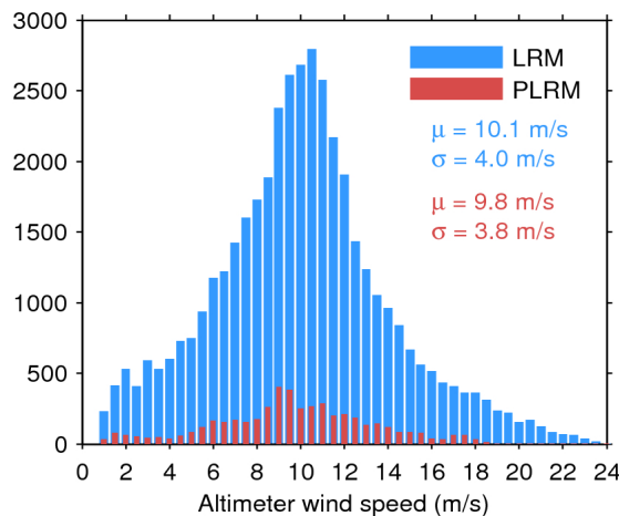
Figure 35. Histogram of science-valid wind over oceans and lakes for LRM (blue) and PLRM (red) for 22/01/2016. The mean ( \mu ) and standard deviation ( \sigma ) are also shown. Note that values larger than 24 m/s are excluded from the histogram for the sake of readability but not from the computation of \mu and \sigma .
