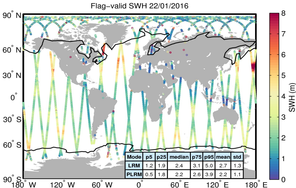
Figure 15. Geographical distribution of flag-valid SWH data over oceans and lakes for 22/01/2016. The statistical values shown in the table refer to the SWH in m and are calculated separately for LRM and PLRM regions. Measurements taken over polar polygons have been excluded from the computation of the statistical values. The black lines mark the outer limit of the Arctic and Antarctic polar polygons.
