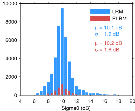
Figure 25. Histogram of flag-valid sigma0 over oceans and lakes for LRM (blue) and PLRM (red) for 22/01/2016. The mean ( \mu ) and standard deviation ( \sigma ) are also shown. Note that values outside [4 20] dB are excluded from the histogram for the sake of readability but not from the computation of \mu and \sigma .
