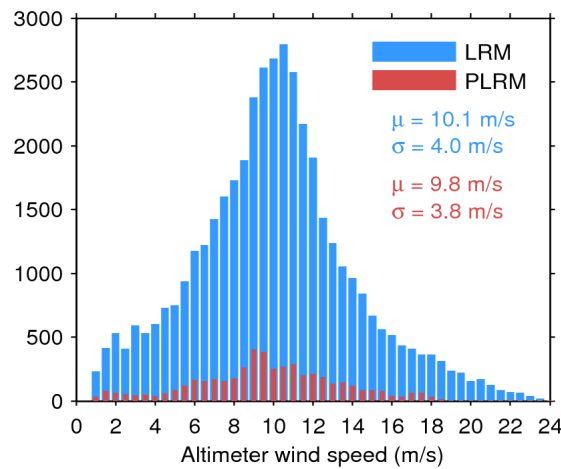
Figure 33. Histogram of flag-valid wind over oceans and lakes for LRM (blue) and PLRM (red) for 22/01/2016. The mean ( \mu ) and standard deviation ( \sigma ) are also shown. Note that values larger than 24 m/s are excluded from the histogram for the sake of readability but not from the computation of \mu and \sigma .
