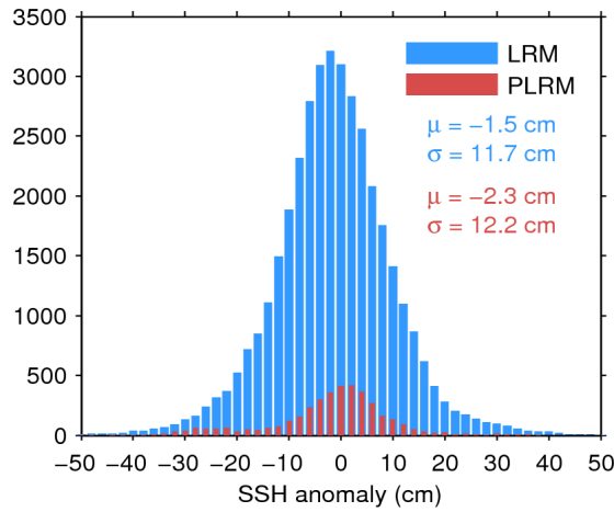
Figure 11. Histogram of science-valid SSH anomaly over oceans and lakes for LRM (blue) and PLRM (red) for 22/01/2016. The mean ( \mu ) and standard deviation ( \sigma ) are also shown. Note that values outside [-50\ 50] cm are excluded from the histogram for the sake of readability but not from the computation of \mu and \sigma .
