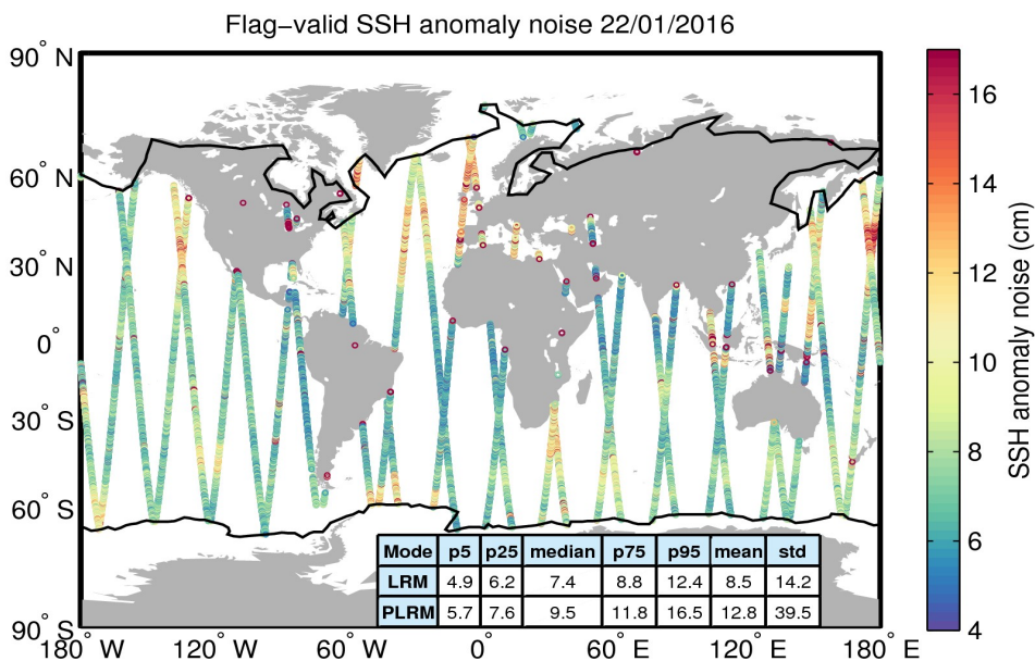
Figure 8. Geographical distribution of flag-valid 20-Hz SSH anomaly measurement noise over oceans and lakes for 22/01/2016. The statistical values shown in the table refer to the SSH anomaly noise and are calculated separately for LRM and PLRM regions. Measurements taken over polar polygons have been excluded from the computation of the statistical values. The black lines mark the outer limit of the Arctic and Antarctic polar polygons.
