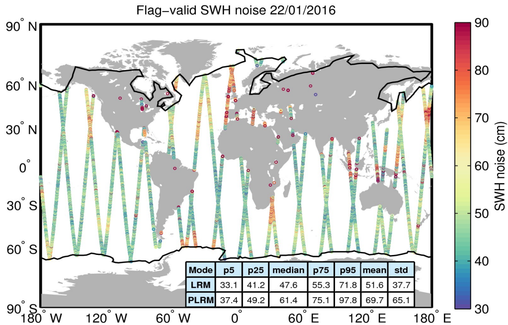
Figure 18. Geographical distribution of flag-valid 20-Hz SWH measurement noise over oceans and lakes for 22/01/2016. The statistical values shown in the table refer to the SWH noise and are calculated separately for LRM and PLRM regions. Measurements taken over polar polygons have been excluded from the computation of the statistical values. The black lines mark the outer limit of the Arctic and Antarctic polar polygons.
