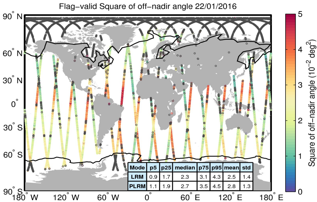
Figure 37. Geographical distribution of flag-valid mispointing data over oceans and lakes for 22/01/2016. The statistical values shown in the table refer to the mispointing in 10^{-2} deg 2 and are calculated separately for LRM and PLRM regions. Measurements taken over polar polygons have been excluded from the computation of the statistical values. The black lines mark the outer limit of the Arctic and Antarctic polar polygons. Gray circles denote negative values.
