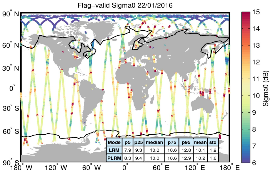
Figure 23. Geographical distribution of flag-valid sigma0 data over oceans and lakes for 22/01/2016. The statistical values shown in the table refer to the sigma0 in dB and are calculated separately for LRM and PLRM regions. Measurements taken over polar polygons have been excluded from the computation of the statistical values. The black lines mark the outer limit of the Arctic and Antarctic polar polygons.
