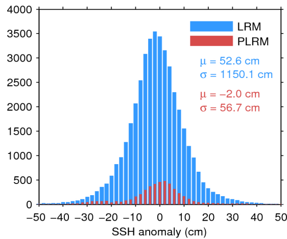
Figure 7. Histogram of flag-valid SSH anomaly over oceans and lakes for LRM (blue) and PLRM (red) for 22/01/2016. The mean ( \mu ) and standard deviation ( \sigma ) are also shown. Note that values outside [-50\ 50] cm are excluded from the histogram for the sake of readability but not from the computation of \mu and \sigma .
