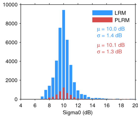
Figure 28. Histogram of science-valid sigma0 over oceans and lakes for LRM (blue) and PLRM (red) for 22/01/2016. The mean ( \mu ) and standard deviation ( \sigma ) are also shown. Note that values outside [4 20] dB are excluded from the histogram for the sake of readability but not from the computation of \mu and \sigma .
