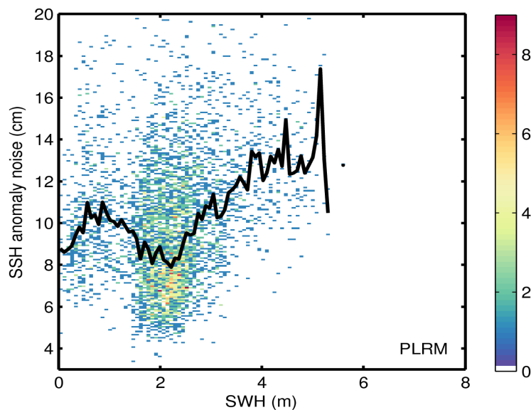
Figure 9. 2D histogram showing flag-valid SSH anomaly noise as a function of SWH for LRM (top) and PLRM (bottom) for 22/01/2016. The black line denotes the median SSH anomaly noise as a function of SWH.
