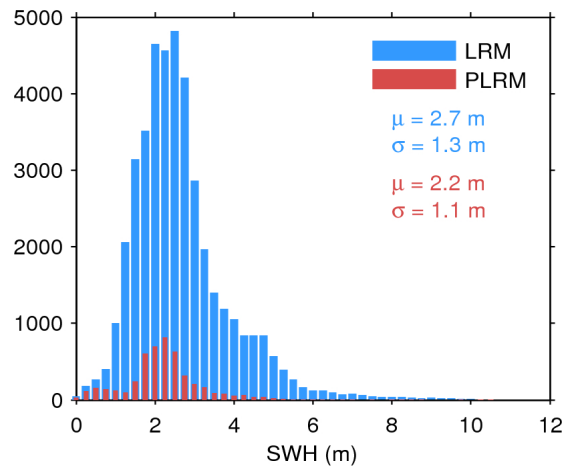
Figure 17. Histogram of flag-valid SWH over oceans and lakes for LRM (blue) and PLRM (red) for 22/01/2016. The mean ( \mu ) and standard deviation ( \sigma ) are also shown. Note that values larger than 12 m are excluded from the histogram for the sake of readability but not from the computation of \mu and \sigma .
