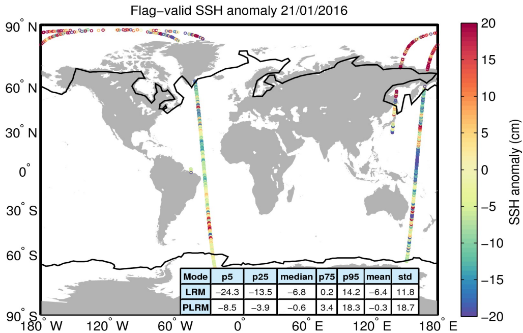
Figure 5. Geographical distribution of flag-valid 1-Hz SSH anomaly data over oceans and lakes for 21/01/2016. The statistical values shown in the table refer to the SSH anomaly in cm and are calculated separately for LRM and PLRM regions. Measurements taken over polar polygons have been excluded from the computation of the statistical values. The black lines mark the outer limit of the Arctic and Antarctic polar polygons.
