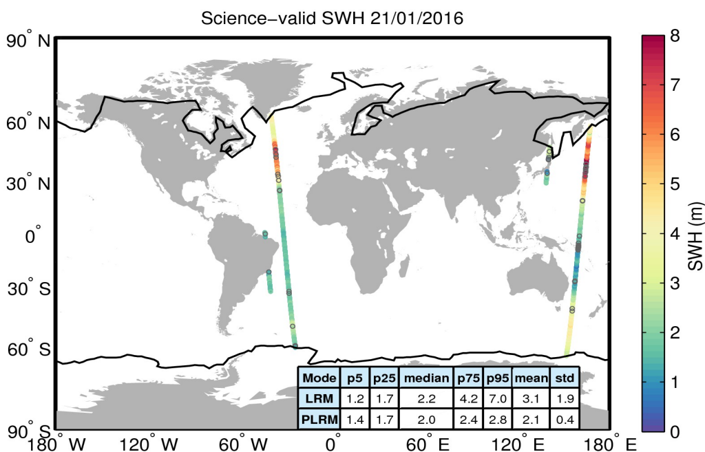
Figure 19. Geographical distribution of science-valid SWH data over oceans and lakes for 21/01/2016. The statistical values shown in the table refer to the SWH in m and are calculated separately for LRM and PLRM regions. The black lines mark the outer limit of the Arctic and Antarctic polar polygons. Gray circles denote records that have been rejected based on the editing criteria described in Table 3.
