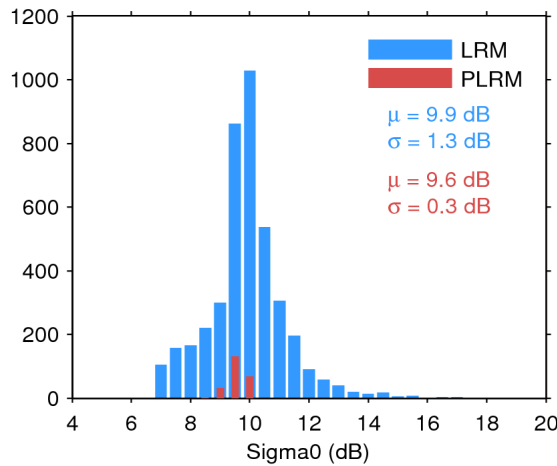
Figure 28. Histogram of science-valid sigma0 over oceans and lakes for LRM (blue) and PLRM (red) for 21/01/2016. The mean ( \mu ) and standard deviation ( \sigma ) are also shown. Note that values outside [4 20] dB are excluded from the histogram for the sake of readability but not from the computation of \mu and \sigma .
