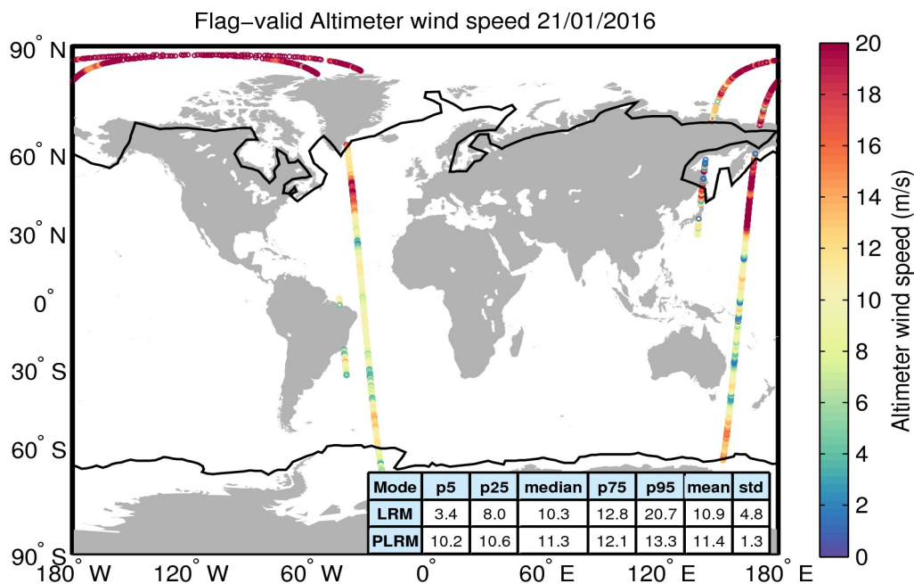
Figure 31. Geographical distribution of flag-valid wind data over oceans and lakes for 21/01/2016. The statistical values shown in the table refer to the wind in m/s and are calculated separately for LRM and PLRM regions. Measurements taken over polar polygons have been excluded from the computation of the statistical values. The black lines mark the outer limit of the Arctic and Antarctic polar polygons.
