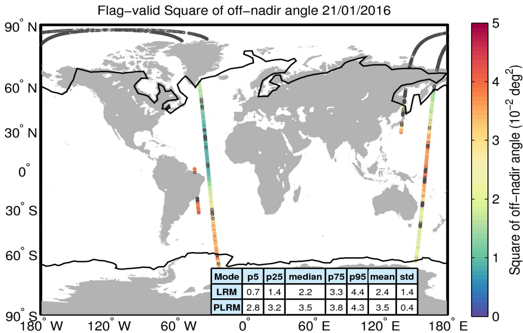
Figure 37. Geographical distribution of flag-valid mispointing data over oceans and lakes for 21/01/2016. The statistical values shown in the table refer to the mispointing in 10^{-2} deg 2 and are calculated separately for LRM and PLRM regions. Measurements taken over polar polygons have been excluded from the computation of the statistical values. The black lines mark the outer limit of the Arctic and Antarctic polar polygons. Gray circles denote negative values.
