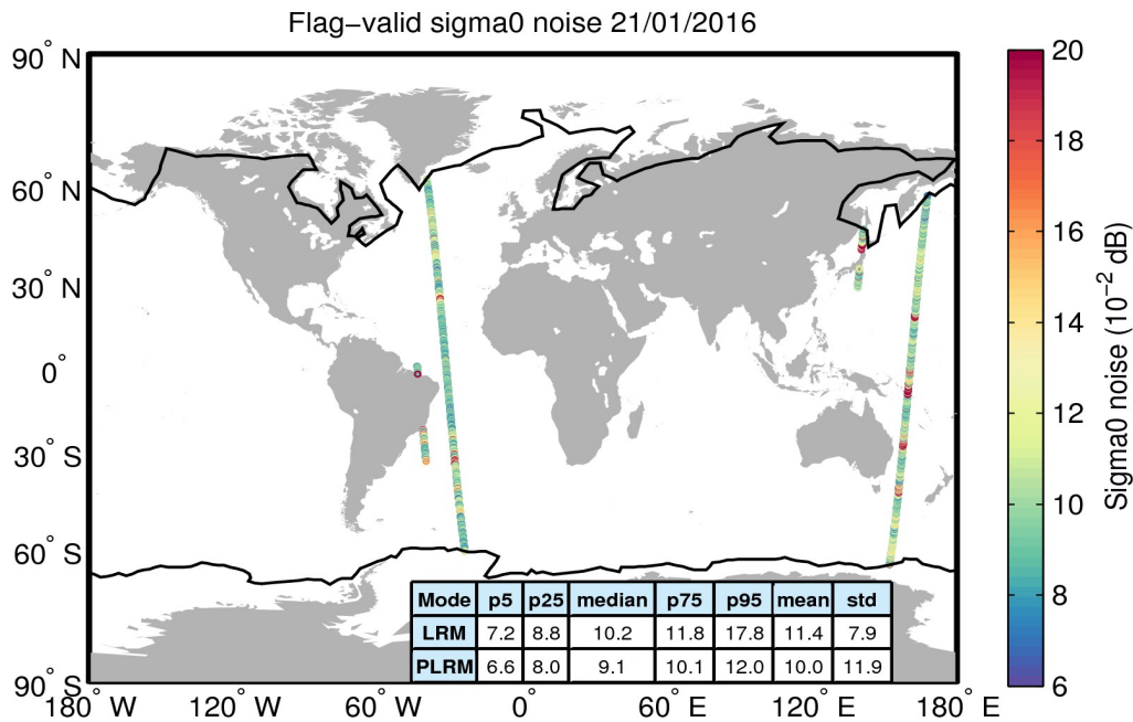
Figure 26. Geographical distribution of flag-valid 20-Hz sigma0 measurement noise over oceans and lakes for 21/01/2016. The statistical values shown in the table refer to the sigma0 noise and are calculated separately for LRM and PLRM regions. Measurements taken over polar polygons have been excluded from the computation of the statistical values. The black lines mark the outer limit of the Arctic and Antarctic polar polygons.
