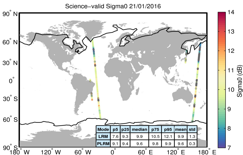
Figure 27. Geographical distribution of science-valid sigma0 data over oceans and lakes for 21/01/2016. The statistical values shown in the table refer to the sigma0 in dB and are calculated separately for LRM and PLRM regions. The black lines mark the outer limit of the Arctic and Antarctic polar polygons. Gray circles denote records that have been rejected based on the editing criteria described in Table 4.
