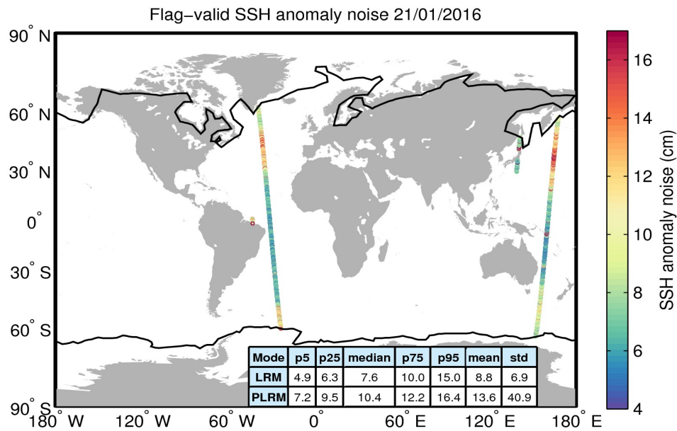
Figure 8. Geographical distribution of flag-valid 20-Hz SSH anomaly measurement noise over oceans and lakes for 21/01/2016. The statistical values shown in the table refer to the SSH anomaly noise and are calculated separately for LRM and PLRM regions. Measurements taken over polar polygons have been excluded from the computation of the statistical values. The black lines mark the outer limit of the Arctic and Antarctic polar polygons.
