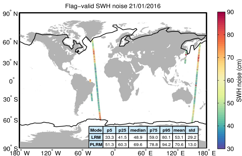
Figure 18. Geographical distribution of flag-valid 20-Hz SWH measurement noise over oceans and lakes for 21/01/2016. The statistical values shown in the table refer to the SWH noise and are calculated separately for LRM and PLRM regions. Measurements taken over polar polygons have been excluded from the computation of the statistical values. The black lines mark the outer limit of the Arctic and Antarctic polar polygons.
