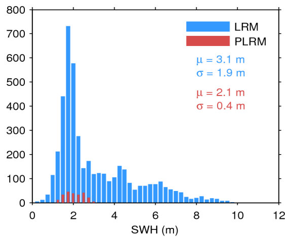
Figure 20. Histogram of science-valid SWH over oceans and lakes for LRM (blue) and PLRM (red) for 21/01/2016. The mean ( \mu ) and standard deviation ( \sigma ) are also shown. Note that values larger than 12 m are excluded from the histogram for the sake of readability but not from the computation of \mu and \sigma .
