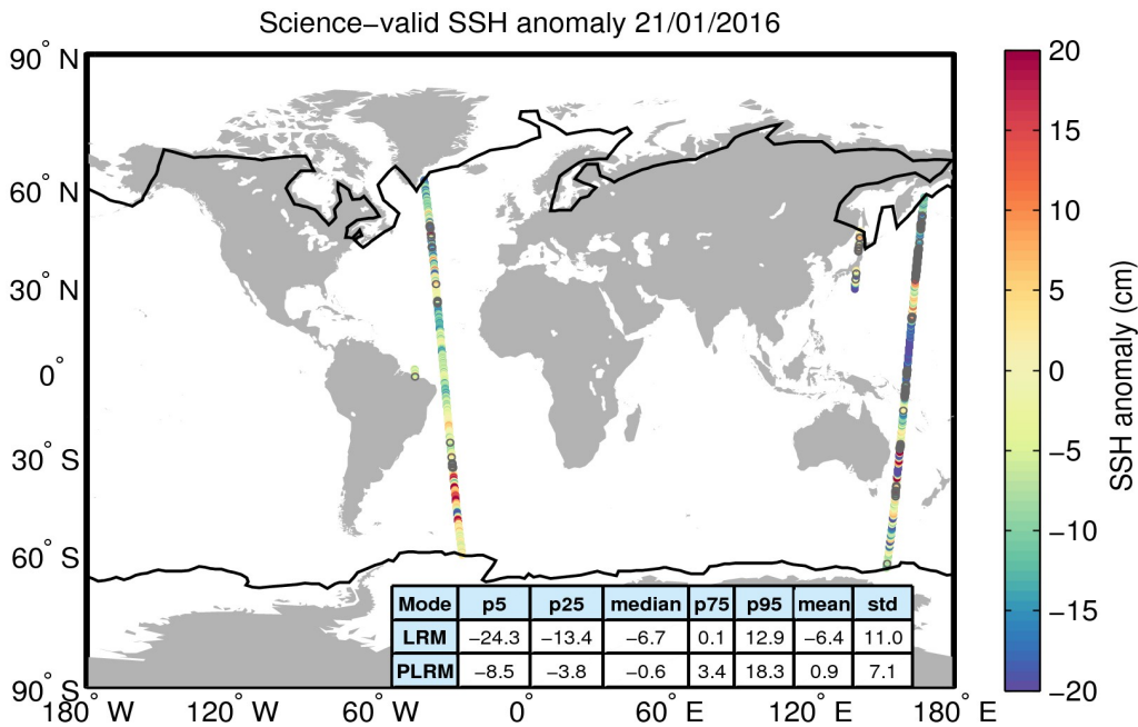
Figure 10. Geographical distribution of science-valid SSH anomaly data over oceans and lakes for 21/01/2016. The statistical values shown in the table refer to the SSH anomaly in cm and are calculated separately for LRM and PLRM regions. The black lines mark the outer limit of the Arctic and Antarctic polar polygons. Gray circles denote records that have been rejected based on the editing criteria described in Table 2.
