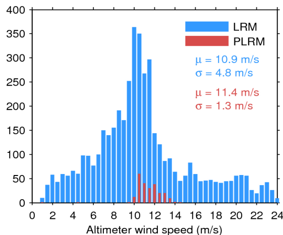
Figure 35. Histogram of science-valid wind over oceans and lakes for LRM (blue) and PLRM (red) for 21/01/2016. The mean ( \mu ) and standard deviation ( \sigma ) are also shown. Note that values larger than 24 m/s are excluded from the histogram for the sake of readability but not from the computation of \mu and \sigma .
