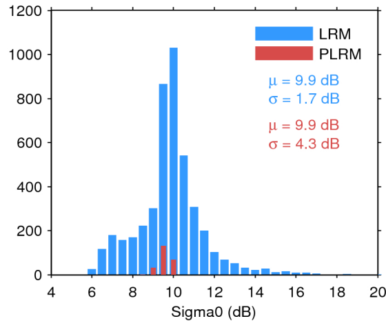
Figure 25. Histogram of flag-valid sigma0 over oceans and lakes for LRM (blue) and PLRM (red) for 21/01/2016. The mean ( \mu ) and standard deviation ( \sigma ) are also shown. Note that values outside [4 20] dB are excluded from the histogram for the sake of readability but not from the computation of \mu and \sigma .
