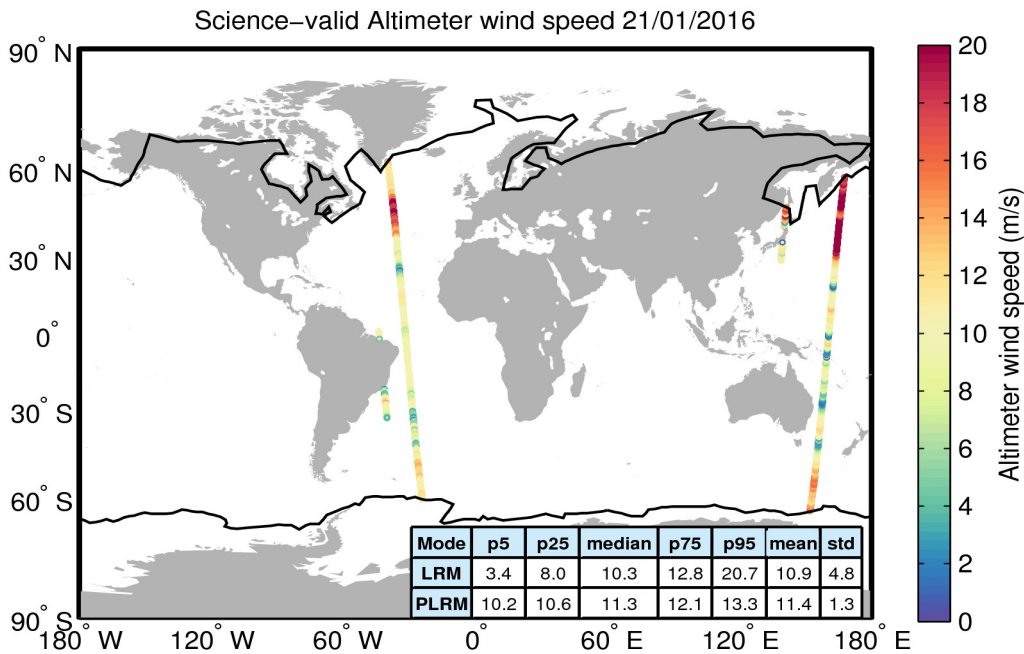
Figure 34. Geographical distribution of science-valid wind data over oceans and lakes for 21/01/2016. The statistical values shown in the table refer to the wind in m/s and are calculated separately for LRM and PLRM regions. The black lines mark the outer limit of the Arctic and Antarctic polar polygons. Gray circles denote records that have been rejected based on the editing criteria described in Table 5.
