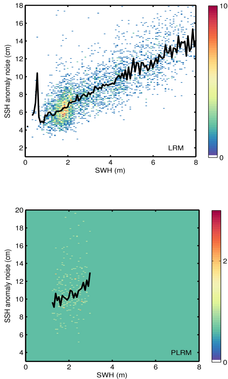
Figure 9. 2D histogram showing flag-valid SSH anomaly noise as a function of SWH for LRM (top) and PLRM (bottom) for 21/01/2016. The black line denotes the median SSH anomaly noise as a function of SWH.
