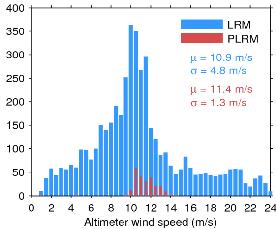
Figure 33. Histogram of flag-valid wind over oceans and lakes for LRM (blue) and PLRM (red) for 21/01/2016. The mean ( \mu ) and standard deviation ( \sigma ) are also shown. Note that values larger than 24 m/s are excluded from the histogram for the sake of readability but not from the computation of \mu and \sigma .
