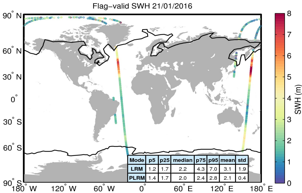
Figure 15. Geographical distribution of flag-valid SWH data over oceans and lakes for 21/01/2016. The statistical values shown in the table refer to the SWH in m and are calculated separately for LRM and PLRM regions. Measurements taken over polar polygons have been excluded from the computation of the statistical values. The black lines mark the outer limit of the Arctic and Antarctic polar polygons.
