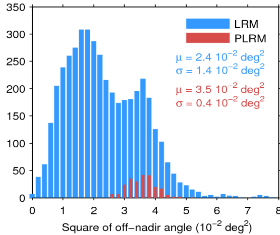
Figure 39. Histogram of flag-valid mispointing over oceans and lakes for LRM (blue) and PLRM (red) for 21/01/2016. Only positive values have been considered. The mean ( \mu ) and standard deviation ( \sigma ) are also shown. Note that values larger than 8 \cdot 10^{-2} \text{ deg}^2 are excluded from the histogram for the sake of readability but not from the computation of \mu and \sigma .
