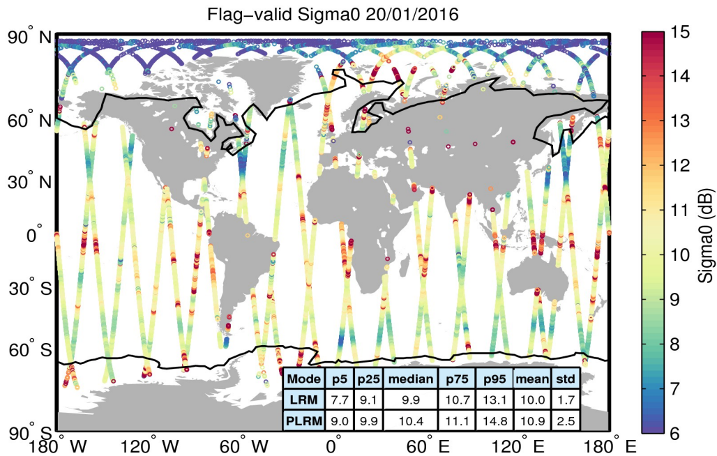
Figure 23. Geographical distribution of flag-valid sigma0 data over oceans and lakes for 20/01/2016. The statistical values shown in the table refer to the sigma0 in dB and are calculated separately for LRM and PLRM regions. Measurements taken over polar polygons have been excluded from the computation of the statistical values. The black lines mark the outer limit of the Arctic and Antarctic polar polygons.
