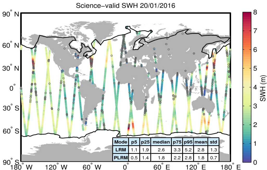
Figure 19. Geographical distribution of science-valid SWH data over oceans and lakes for 20/01/2016. The statistical values shown in the table refer to the SWH in m and are calculated separately for LRM and PLRM regions. The black lines mark the outer limit of the Arctic and Antarctic polar polygons. Gray circles denote records that have been rejected based on the editing criteria described in Table 3.
