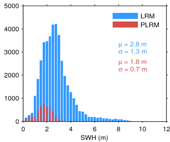
Figure 20. Histogram of science-valid SWH over oceans and lakes for LRM (blue) and PLRM (red) for 20/01/2016. The mean ( \mu ) and standard deviation ( \sigma ) are also shown. Note that values larger than 12 m are excluded from the histogram for the sake of readability but not from the computation of \mu and \sigma .
