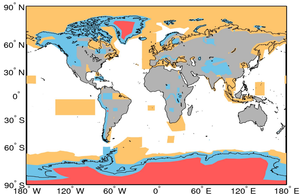
Figure A1. Extent of the regions defining the geographical mode mask for 20/01/2016. The regions where SAR, and SARIn are operated are denoted by the orange and blue polygons, respectively. LRM is operated over areas of the continental ice sheets (red polygons) and over oceans and land not covered by other modes.
