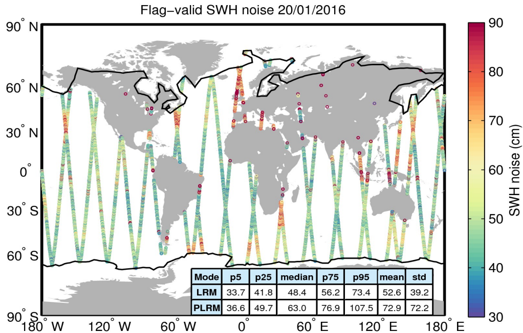
Figure 18. Geographical distribution of flag-valid 20-Hz SWH measurement noise over oceans and lakes for 20/01/2016. The statistical values shown in the table refer to the SWH noise and are calculated separately for LRM and PLRM regions. Measurements taken over polar polygons have been excluded from the computation of the statistical values. The black lines mark the outer limit of the Arctic and Antarctic polar polygons.
