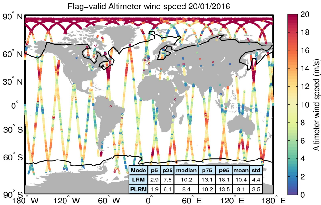
Figure 31. Geographical distribution of flag-valid wind data over oceans and lakes for 20/01/2016. The statistical values shown in the table refer to the wind in m/s and are calculated separately for LRM and PLRM regions. Measurements taken over polar polygons have been excluded from the computation of the statistical values. The black lines mark the outer limit of the Arctic and Antarctic polar polygons.
