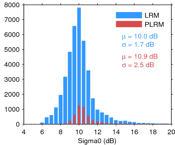
Figure 25. Histogram of flag-valid sigma0 over oceans and lakes for LRM (blue) and PLRM (red) for 20/01/2016. The mean ( \mu ) and standard deviation ( \sigma ) are also shown. Note that values outside [4 20] dB are excluded from the histogram for the sake of readability but not from the computation of \mu and \sigma .
