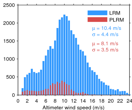
Figure 35. Histogram of science-valid wind over oceans and lakes for LRM (blue) and PLRM (red) for 20/01/2016. The mean ( \mu ) and standard deviation ( \sigma ) are also shown. Note that values larger than 24 m/s are excluded from the histogram for the sake of readability but not from the computation of \mu and \sigma .
