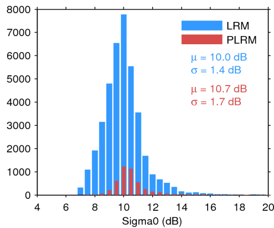
Figure 28. Histogram of science-valid sigma0 over oceans and lakes for LRM (blue) and PLRM (red) for 20/01/2016. The mean ( \mu ) and standard deviation ( \sigma ) are also shown. Note that values outside [4 20] dB are excluded from the histogram for the sake of readability but not from the computation of \mu and \sigma .
