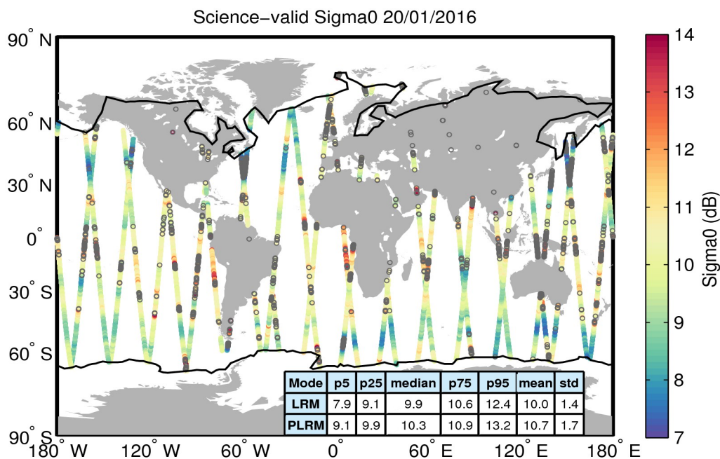
Figure 27. Geographical distribution of science-valid sigma0 data over oceans and lakes for 20/01/2016. The statistical values shown in the table refer to the sigma0 in dB and are calculated separately for LRM and PLRM regions. The black lines mark the outer limit of the Arctic and Antarctic polar polygons. Gray circles denote records that have been rejected based on the editing criteria described in Table 4.
