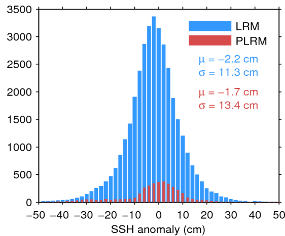
Figure 11. Histogram of science-valid SSH anomaly over oceans and lakes for LRM (blue) and PLRM (red) for 20/01/2016. The mean ( \mu ) and standard deviation ( \sigma ) are also shown. Note that values outside [-50 50] cm are excluded from the histogram for the sake of readability but not from the computation of \mu and \sigma .
