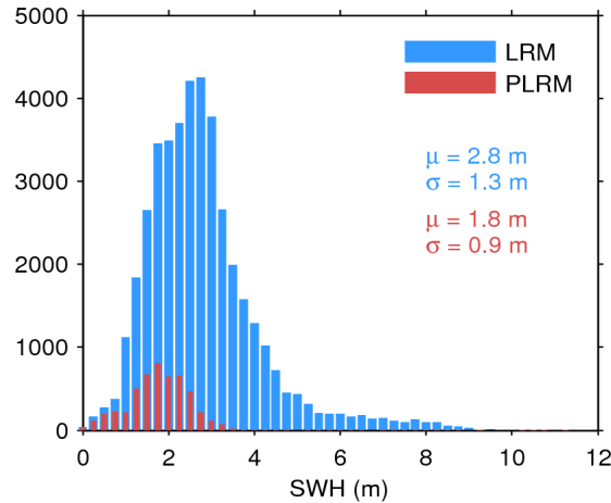
Figure 17. Histogram of flag-valid SWH over oceans and lakes for LRM (blue) and PLRM (red) for 20/01/2016. The mean ( \mu ) and standard deviation ( \sigma ) are also shown. Note that values larger than 12 m are excluded from the histogram for the sake of readability but not from the computation of \mu and \sigma .
