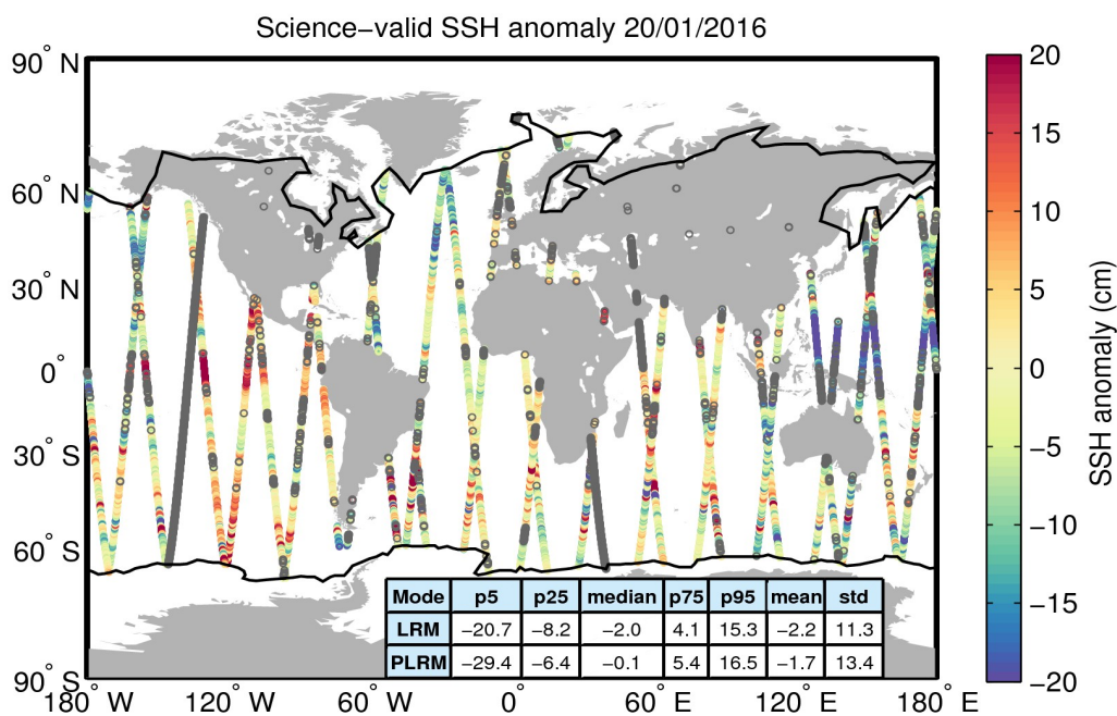
Figure 10. Geographical distribution of science-valid SSH anomaly data over oceans and lakes for 20/01/2016. The statistical values shown in the table refer to the SSH anomaly in cm and are calculated separately for LRM and PLRM regions. The black lines mark the outer limit of the Arctic and Antarctic polar polygons. Gray circles denote records that have been rejected based on the editing criteria described in Table 2.
