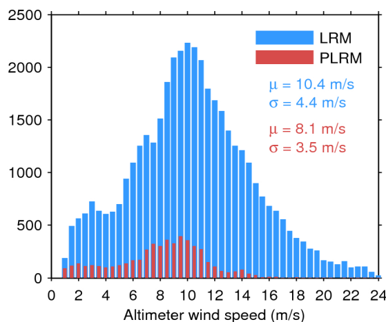
Figure 33. Histogram of flag-valid wind over oceans and lakes for LRM (blue) and PLRM (red) for 20/01/2016. The mean ( \mu ) and standard deviation ( \sigma ) are also shown. Note that values larger than 24 m/s are excluded from the histogram for the sake of readability but not from the computation of \mu and \sigma .
