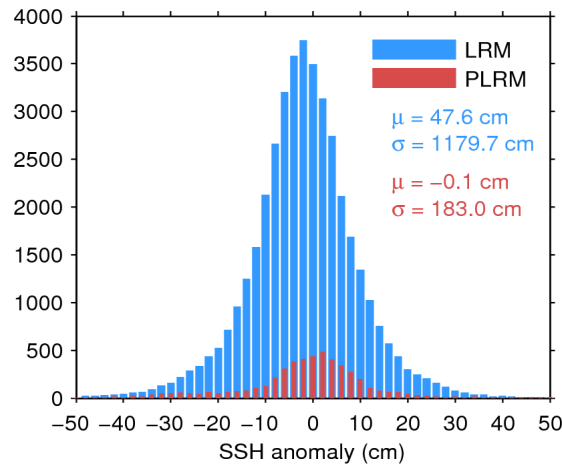
Figure 7. Histogram of flag-valid SSH anomaly over oceans and lakes for LRM (blue) and PLRM (red) for 20/01/2016. The mean ( \mu ) and standard deviation ( \sigma ) are also shown. Note that values outside [-50 50] cm are excluded from the histogram for the sake of readability but not from the computation of \mu and \sigma .
