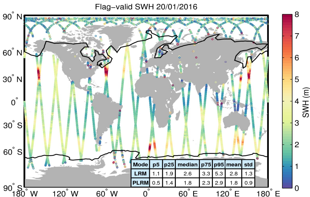
Figure 15. Geographical distribution of flag-valid SWH data over oceans and lakes for 20/01/2016. The statistical values shown in the table refer to the SWH in m and are calculated separately for LRM and PLRM regions. Measurements taken over polar polygons have been excluded from the computation of the statistical values. The black lines mark the outer limit of the Arctic and Antarctic polar polygons.
