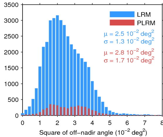
Figure 39. Histogram of flag-valid mispointing over oceans and lakes for LRM (blue) and PLRM (red) for 20/01/2016. Only positive values have been considered. The mean ( \mu ) and standard deviation ( \sigma ) are also shown. Note that values larger than 8 \cdot 10^{-2} \text{ deg}^2 are excluded from the histogram for the sake of readability but not from the computation of \mu and \sigma .
