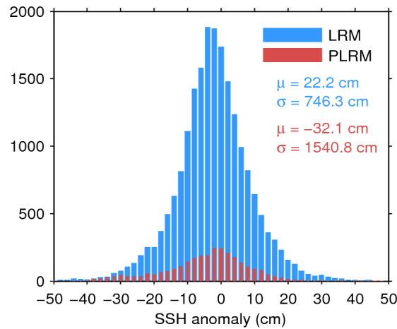
Figure 7. Histogram of flag-valid SSH anomaly over oceans and lakes for LRM (blue) and PLRM (red) for 19/01/2016. The mean ( \mu ) and standard deviation ( \sigma ) are also shown. Note that values outside [-50\ 50] cm are excluded from the histogram for the sake of readability but not from the computation of \mu and \sigma .
