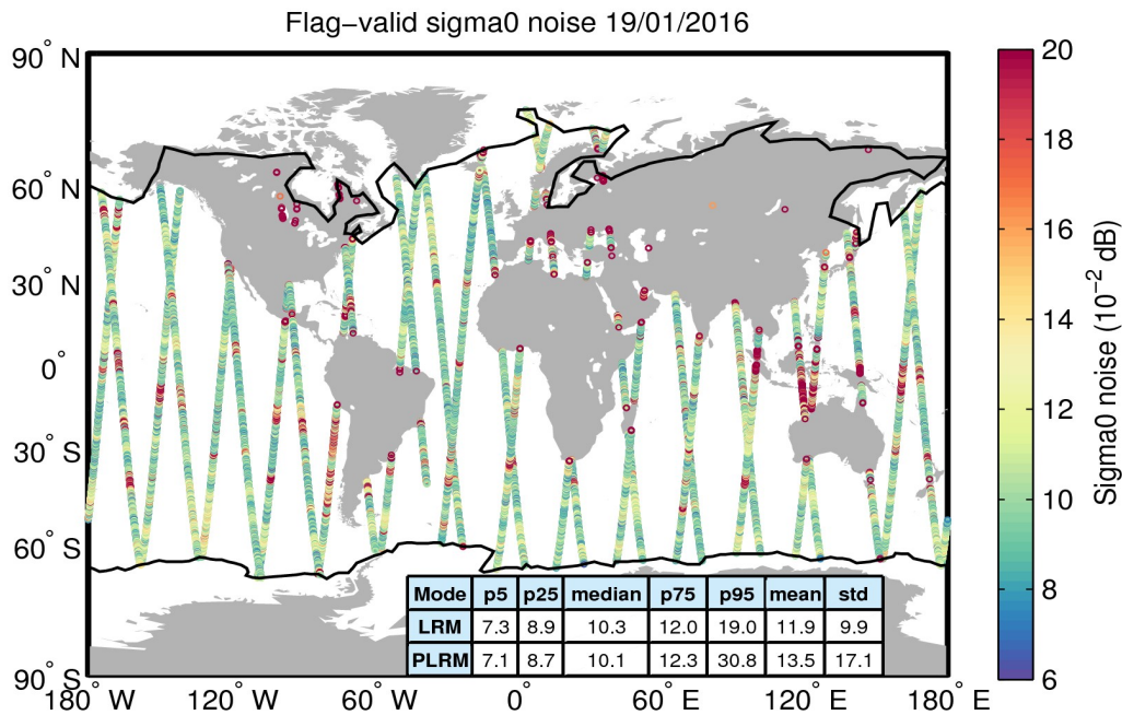
Figure 26. Geographical distribution of flag-valid 20-Hz sigma0 measurement noise over oceans and lakes for 19/01/2016. The statistical values shown in the table refer to the sigma0 noise and are calculated separately for LRM and PLRM regions. Measurements taken over polar polygons have been excluded from the computation of the statistical values. The black lines mark the outer limit of the Arctic and Antarctic polar polygons.
