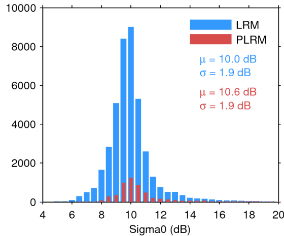
Figure 25. Histogram of flag-valid sigma0 over oceans and lakes for LRM (blue) and PLRM (red) for 19/01/2016. The mean ( \mu ) and standard deviation ( \sigma ) are also shown. Note that values outside [4 20] dB are excluded from the histogram for the sake of readability but not from the computation of \mu and \sigma .
