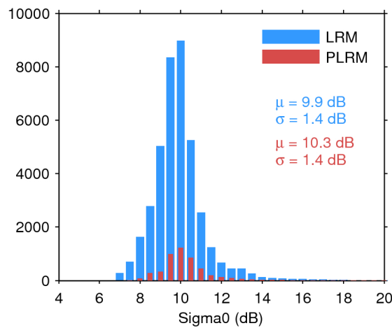
Figure 28. Histogram of science-valid sigma0 over oceans and lakes for LRM (blue) and PLRM (red) for 19/01/2016. The mean ( \mu ) and standard deviation ( \sigma ) are also shown. Note that values outside [4 20] dB are excluded from the histogram for the sake of readability but not from the computation of \mu and \sigma .
