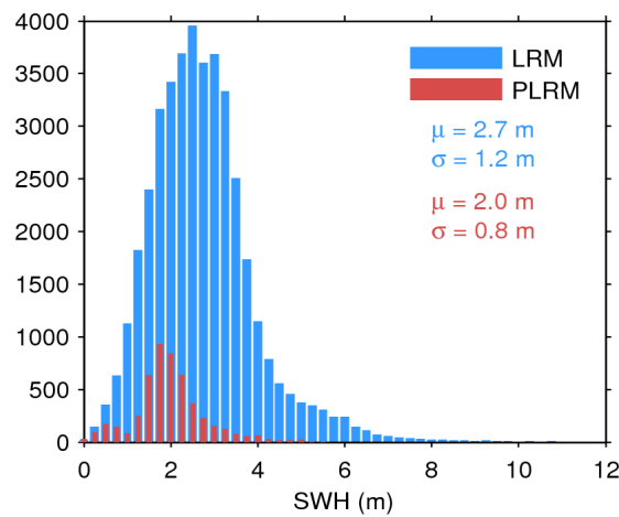
Figure 20. Histogram of science-valid SWH over oceans and lakes for LRM (blue) and PLRM (red) for 19/01/2016. The mean ( \mu ) and standard deviation ( \sigma ) are also shown. Note that values larger than 12 m are excluded from the histogram for the sake of readability but not from the computation of \mu and \sigma .
