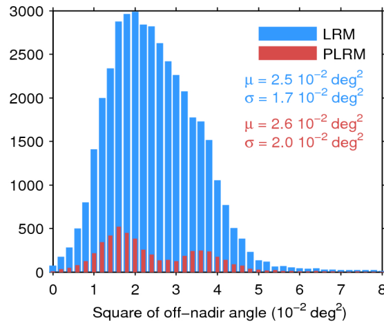
Figure 39. Histogram of flag-valid mispointing over oceans and lakes for LRM (blue) and PLRM (red) for 19/01/2016. Only positive values have been considered. The mean ( \mu ) and standard deviation ( \sigma ) are also shown. Note that values larger than 8 \cdot 10^{-2} \text{ deg}^2 are excluded from the histogram for the sake of readability but not from the computation of \mu and \sigma .
