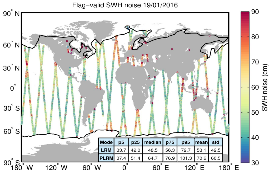
Figure 18. Geographical distribution of flag-valid 20-Hz SWH measurement noise over oceans and lakes for 19/01/2016. The statistical values shown in the table refer to the SWH noise and are calculated separately for LRM and PLRM regions. Measurements taken over polar polygons have been excluded from the computation of the statistical values. The black lines mark the outer limit of the Arctic and Antarctic polar polygons.
