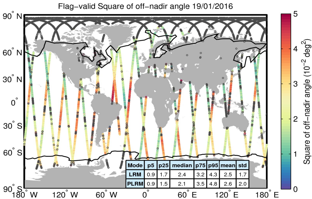
Figure 37. Geographical distribution of flag-valid mispointing data over oceans and lakes for 19/01/2016. The statistical values shown in the table refer to the mispointing in 10^{-2} deg 2 and are calculated separately for LRM and PLRM regions. Measurements taken over polar polygons have been excluded from the computation of the statistical values. The black lines mark the outer limit of the Arctic and Antarctic polar polygons. Gray circles denote negative values.
