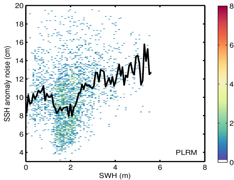
Figure 9. 2D histogram showing flag-valid SSH anomaly noise as a function of SWH for LRM (top) and PLRM (bottom) for 19/01/2016. The black line denotes the median SSH anomaly noise as a function of SWH.
