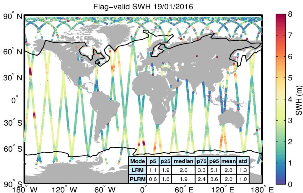
Figure 15. Geographical distribution of flag-valid SWH data over oceans and lakes for 19/01/2016. The statistical values shown in the table refer to the SWH in m and are calculated separately for LRM and PLRM regions. Measurements taken over polar polygons have been excluded from the computation of the statistical values. The black lines mark the outer limit of the Arctic and Antarctic polar polygons.
