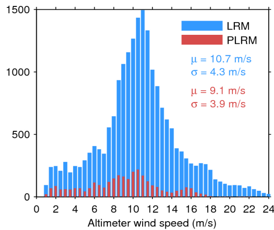
Figure 33. Histogram of flag-valid wind over oceans and lakes for LRM (blue) and PLRM (red) for 19/01/2016. The mean ( \mu ) and standard deviation ( \sigma ) are also shown. Note that values larger than 24 m/s are excluded from the histogram for the sake of readability but not from the computation of \mu and \sigma .
