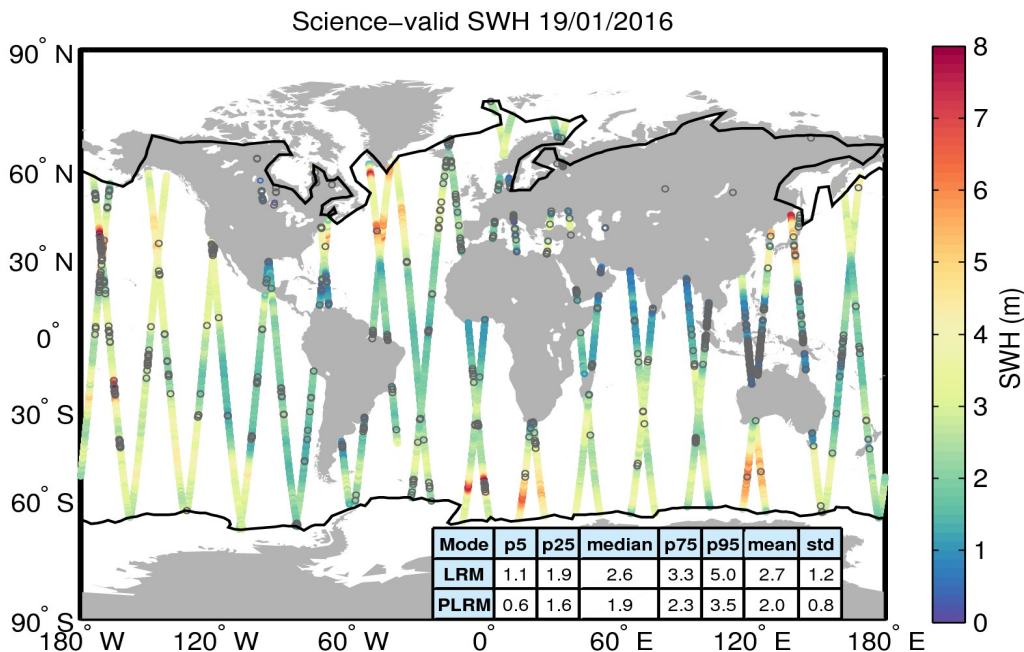
Figure 19. Geographical distribution of science-valid SWH data over oceans and lakes for 19/01/2016. The statistical values shown in the table refer to the SWH in m and are calculated separately for LRM and PLRM regions. The black lines mark the outer limit of the Arctic and Antarctic polar polygons. Gray circles denote records that have been rejected based on the editing criteria described in Table 3.
