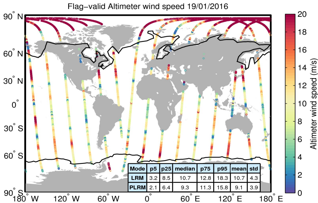
Figure 31. Geographical distribution of flag-valid wind data over oceans and lakes for 19/01/2016. The statistical values shown in the table refer to the wind in m/s and are calculated separately for LRM and PLRM regions. Measurements taken over polar polygons have been excluded from the computation of the statistical values. The black lines mark the outer limit of the Arctic and Antarctic polar polygons.
