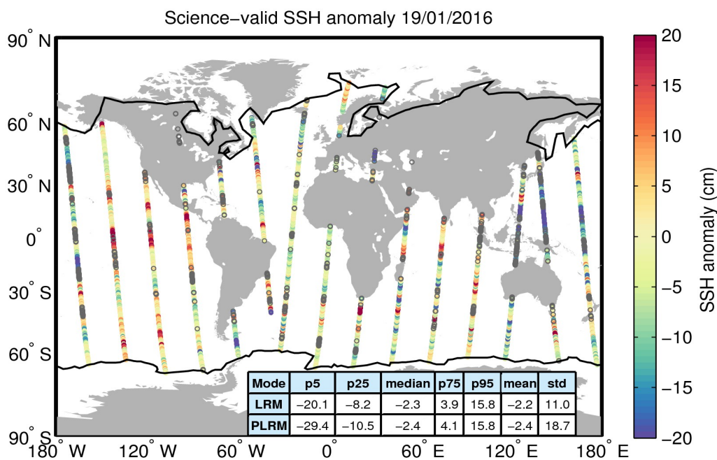
Figure 10. Geographical distribution of science-valid SSH anomaly data over oceans and lakes for 19/01/2016. The statistical values shown in the table refer to the SSH anomaly in cm and are calculated separately for LRM and PLRM regions. The black lines mark the outer limit of the Arctic and Antarctic polar polygons. Gray circles denote records that have been rejected based on the editing criteria described in Table 2.
