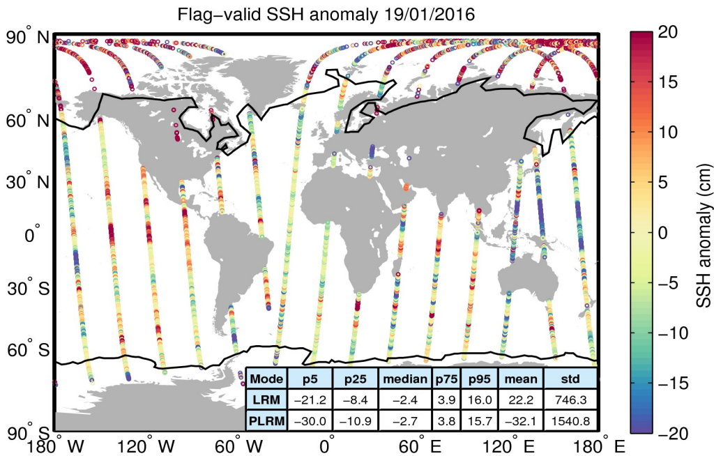
Figure 5. Geographical distribution of flag-valid 1-Hz SSH anomaly data over oceans and lakes for 19/01/2016. The statistical values shown in the table refer to the SSH anomaly in cm and are calculated separately for LRM and PLRM regions. Measurements taken over polar polygons have been excluded from the computation of the statistical values. The black lines mark the outer limit of the Arctic and Antarctic polar polygons.
