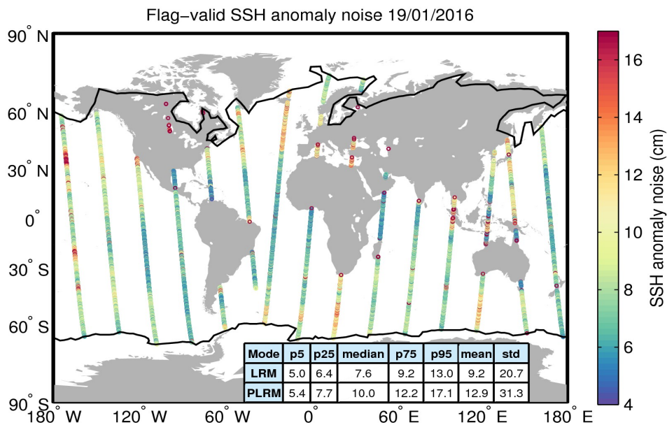
Figure 8. Geographical distribution of flag-valid 20-Hz SSH anomaly measurement noise over oceans and lakes for 19/01/2016. The statistical values shown in the table refer to the SSH anomaly noise and are calculated separately for LRM and PLRM regions. Measurements taken over polar polygons have been excluded from the computation of the statistical values. The black lines mark the outer limit of the Arctic and Antarctic polar polygons.
