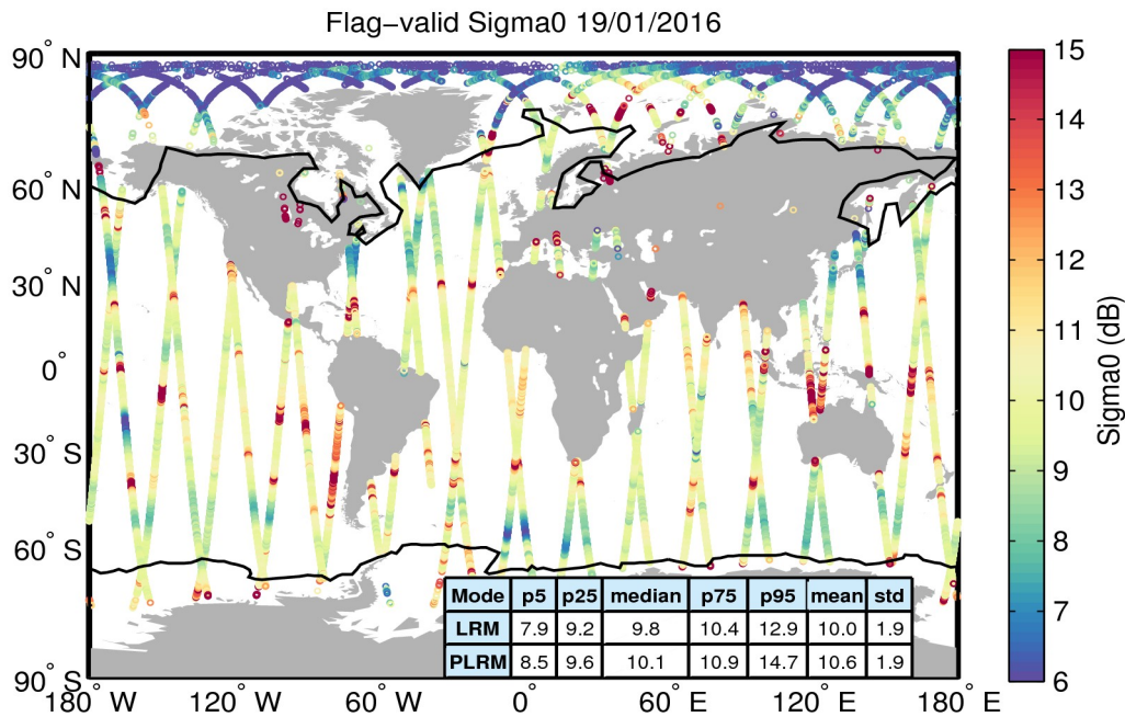
Figure 23. Geographical distribution of flag-valid sigma0 data over oceans and lakes for 19/01/2016. The statistical values shown in the table refer to the sigma0 in dB and are calculated separately for LRM and PLRM regions. Measurements taken over polar polygons have been excluded from the computation of the statistical values. The black lines mark the outer limit of the Arctic and Antarctic polar polygons.
