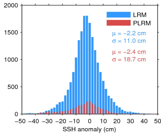
Figure 11. Histogram of science-valid SSH anomaly over oceans and lakes for LRM (blue) and PLRM (red) for 19/01/2016. The mean ( \mu ) and standard deviation ( \sigma ) are also shown. Note that values outside [-50\ 50] cm are excluded from the histogram for the sake of readability but not from the computation of \mu and \sigma .
