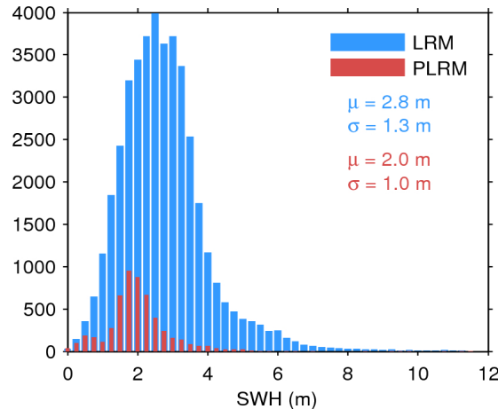
Figure 17. Histogram of flag-valid SWH over oceans and lakes for LRM (blue) and PLRM (red) for 19/01/2016. The mean ( \mu ) and standard deviation ( \sigma ) are also shown. Note that values larger than 12 m are excluded from the histogram for the sake of readability but not from the computation of \mu and \sigma .
