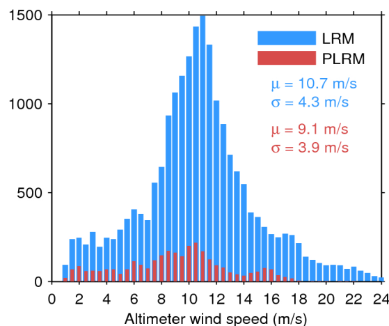
Figure 35. Histogram of science-valid wind over oceans and lakes for LRM (blue) and PLRM (red) for 19/01/2016. The mean ( \mu ) and standard deviation ( \sigma ) are also shown. Note that values larger than 24 m/s are excluded from the histogram for the sake of readability but not from the computation of \mu and \sigma .
