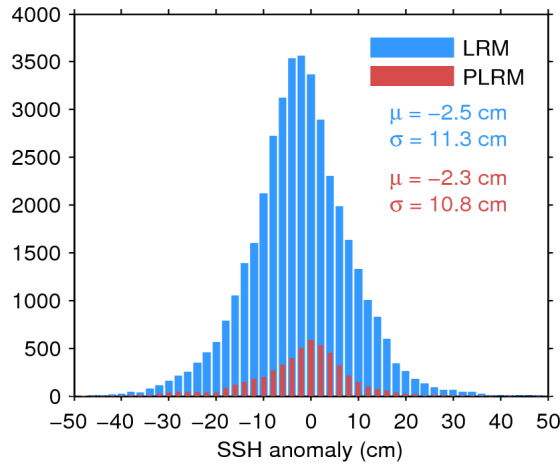
Figure 11. Histogram of science-valid SSH anomaly over oceans and lakes for LRM (blue) and PLRM (red) for 17/01/2016. The mean ( \mu ) and standard deviation ( \sigma ) are also shown. Note that values outside [-50 50] cm are excluded from the histogram for the sake of readability but not from the computation of \mu and \sigma .
