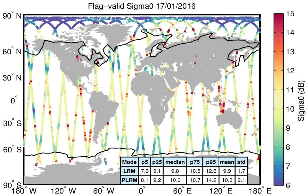
Figure 23. Geographical distribution of flag-valid sigma0 data over oceans and lakes for 17/01/2016. The statistical values shown in the table refer to the sigma0 in dB and are calculated separately for LRM and PLRM regions. Measurements taken over polar polygons have been excluded from the computation of the statistical values. The black lines mark the outer limit of the Arctic and Antarctic polar polygons.
