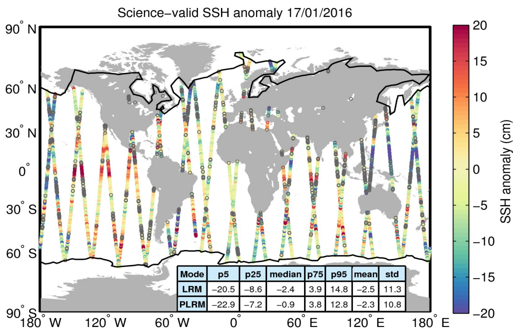
Figure 10. Geographical distribution of science-valid SSH anomaly data over oceans and lakes for 17/01/2016. The statistical values shown in the table refer to the SSH anomaly in cm and are calculated separately for LRM and PLRM regions. The black lines mark the outer limit of the Arctic and Antarctic polar polygons. Gray circles denote records that have been rejected based on the editing criteria described in Table 2.
