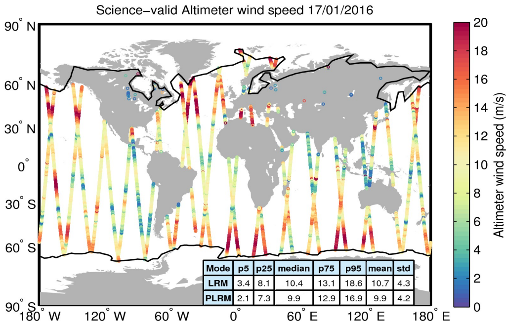
Figure 34. Geographical distribution of science-valid wind data over oceans and lakes for 17/01/2016. The statistical values shown in the table refer to the wind in m/s and are calculated separately for LRM and PLRM regions. The black lines mark the outer limit of the Arctic and Antarctic polar polygons. Gray circles denote records that have been rejected based on the editing criteria described in Table 5.
