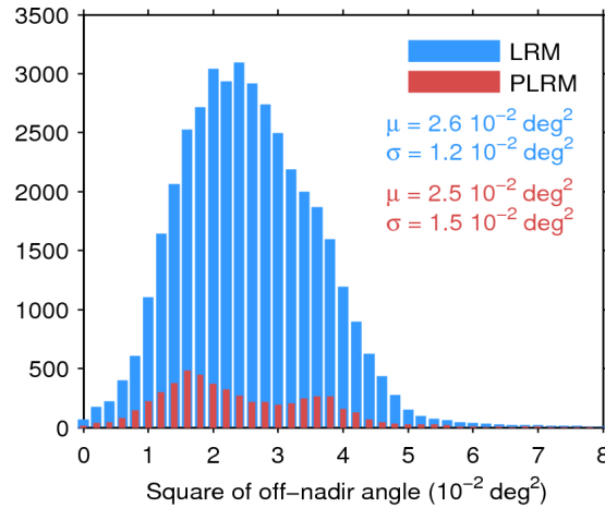
Figure 39. Histogram of flag-valid mispointing over oceans and lakes for LRM (blue) and PLRM (red) for 17/01/2016. Only positive values have been considered. The mean ( \mu ) and standard deviation ( \sigma ) are also shown. Note that values larger than 8 \cdot 10^{-2} \text{ deg}^2 are excluded from the histogram for the sake of readability but not from the computation of \mu and \sigma .
