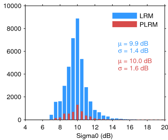
Figure 28. Histogram of science-valid sigma0 over oceans and lakes for LRM (blue) and PLRM (red) for 17/01/2016. The mean ( \mu ) and standard deviation ( \sigma ) are also shown. Note that values outside [4 20] dB are excluded from the histogram for the sake of readability but not from the computation of \mu and \sigma .
