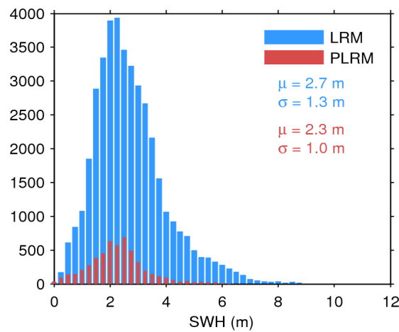
Figure 20. Histogram of science-valid SWH over oceans and lakes for LRM (blue) and PLRM (red) for 17/01/2016. The mean ( \mu ) and standard deviation ( \sigma ) are also shown. Note that values larger than 12 m are excluded from the histogram for the sake of readability but not from the computation of \mu and \sigma .
