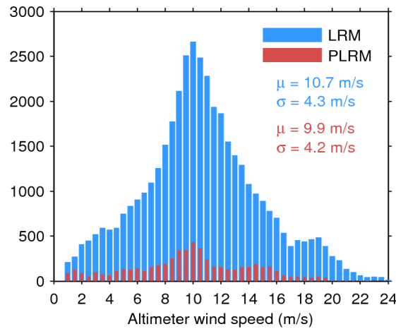
Figure 33. Histogram of flag-valid wind over oceans and lakes for LRM (blue) and PLRM (red) for 17/01/2016. The mean ( \mu ) and standard deviation ( \sigma ) are also shown. Note that values larger than 24 m/s are excluded from the histogram for the sake of readability but not from the computation of \mu and \sigma .
