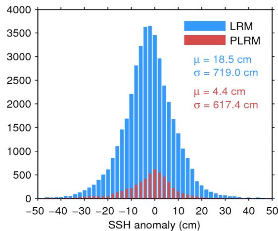
Figure 7. Histogram of flag-valid SSH anomaly over oceans and lakes for LRM (blue) and PLRM (red) for 17/01/2016. The mean ( \mu ) and standard deviation ( \sigma ) are also shown. Note that values outside [-50 50] cm are excluded from the histogram for the sake of readability but not from the computation of \mu and \sigma .
