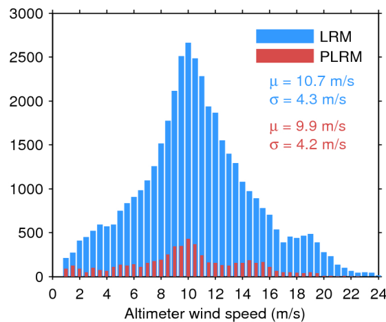
Figure 35. Histogram of science-valid wind over oceans and lakes for LRM (blue) and PLRM (red) for 17/01/2016. The mean ( \mu ) and standard deviation ( \sigma ) are also shown. Note that values larger than 24 m/s are excluded from the histogram for the sake of readability but not from the computation of \mu and \sigma .
