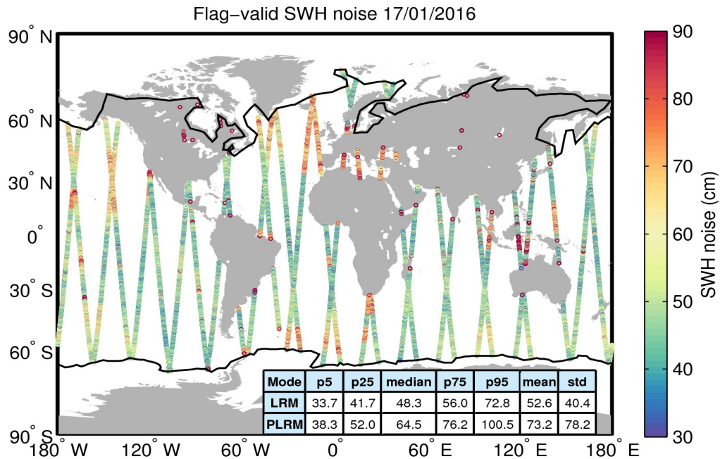
Figure 18. Geographical distribution of flag-valid 20-Hz SWH measurement noise over oceans and lakes for 17/01/2016. The statistical values shown in the table refer to the SWH noise and are calculated separately for LRM and PLRM regions. Measurements taken over polar polygons have been excluded from the computation of the statistical values. The black lines mark the outer limit of the Arctic and Antarctic polar polygons.
