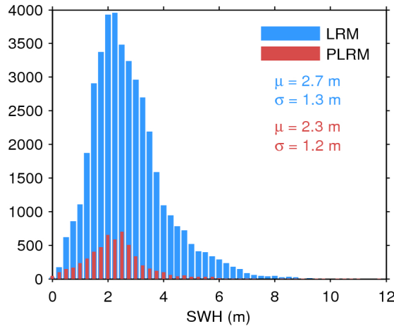
Figure 17. Histogram of flag-valid SWH over oceans and lakes for LRM (blue) and PLRM (red) for 17/01/2016. The mean ( \mu ) and standard deviation ( \sigma ) are also shown. Note that values larger than 12 m are excluded from the histogram for the sake of readability but not from the computation of \mu and \sigma .
