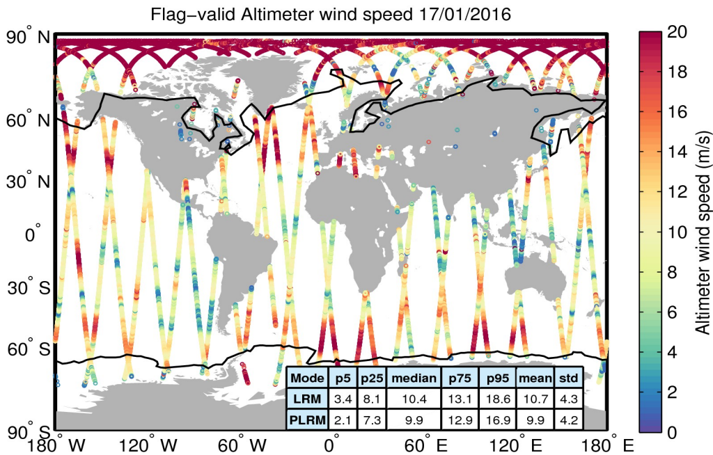
Figure 31. Geographical distribution of flag-valid wind data over oceans and lakes for 17/01/2016. The statistical values shown in the table refer to the wind in m/s and are calculated separately for LRM and PLRM regions. Measurements taken over polar polygons have been excluded from the computation of the statistical values. The black lines mark the outer limit of the Arctic and Antarctic polar polygons.
