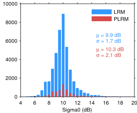
Figure 25. Histogram of flag-valid sigma0 over oceans and lakes for LRM (blue) and PLRM (red) for 17/01/2016. The mean ( \mu ) and standard deviation ( \sigma ) are also shown. Note that values outside [4 20] dB are excluded from the histogram for the sake of readability but not from the computation of \mu and \sigma .
