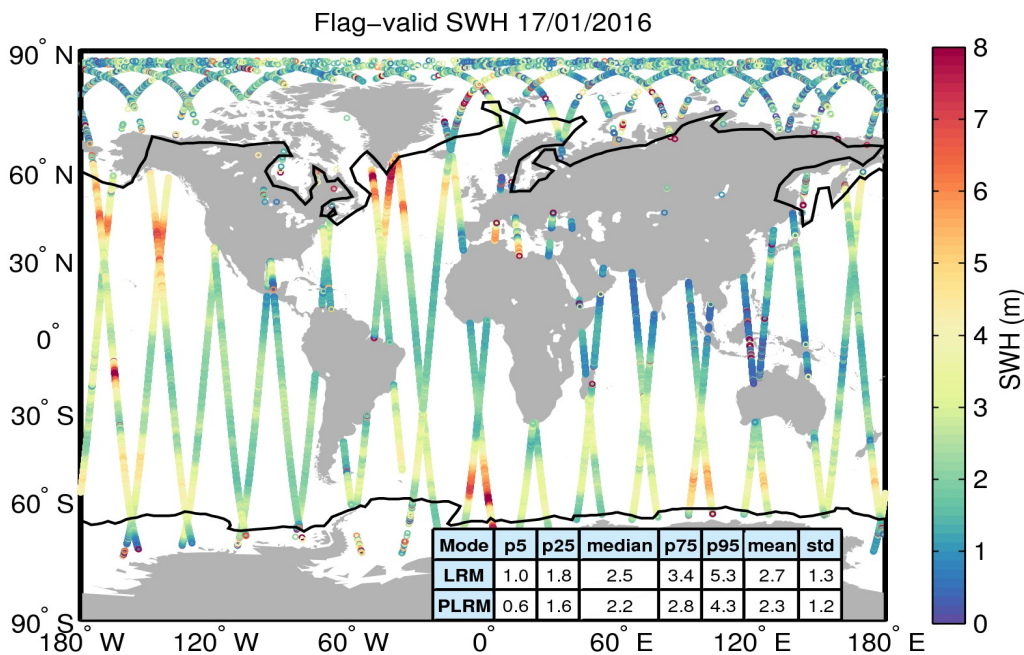
Figure 15. Geographical distribution of flag-valid SWH data over oceans and lakes for 17/01/2016. The statistical values shown in the table refer to the SWH in m and are calculated separately for LRM and PLRM regions. Measurements taken over polar polygons have been excluded from the computation of the statistical values. The black lines mark the outer limit of the Arctic and Antarctic polar polygons.
