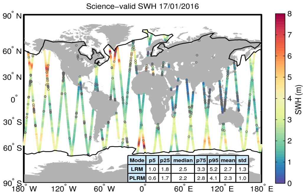
Figure 19. Geographical distribution of science-valid SWH data over oceans and lakes for 17/01/2016. The statistical values shown in the table refer to the SWH in m and are calculated separately for LRM and PLRM regions. The black lines mark the outer limit of the Arctic and Antarctic polar polygons. Gray circles denote records that have been rejected based on the editing criteria described in Table 3.
