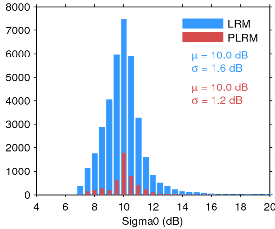
Figure 28. Histogram of science-valid sigma0 over oceans and lakes for LRM (blue) and PLRM (red) for 15/01/2016. The mean ( \mu ) and standard deviation ( \sigma ) are also shown. Note that values outside [4 20] dB are excluded from the histogram for the sake of readability but not from the computation of \mu and \sigma .
