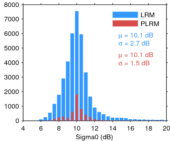
Figure 25. Histogram of flag-valid sigma0 over oceans and lakes for LRM (blue) and PLRM (red) for 15/01/2016. The mean ( \mu ) and standard deviation ( \sigma ) are also shown. Note that values outside [4 20] dB are excluded from the histogram for the sake of readability but not from the computation of \mu and \sigma .
