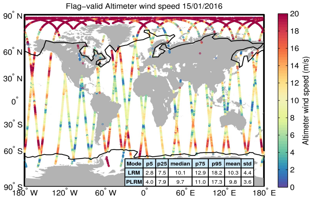
Figure 31. Geographical distribution of flag-valid wind data over oceans and lakes for 15/01/2016. The statistical values shown in the table refer to the wind in m/s and are calculated separately for LRM and PLRM regions. Measurements taken over polar polygons have been excluded from the computation of the statistical values. The black lines mark the outer limit of the Arctic and Antarctic polar polygons.
