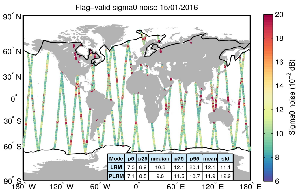
Figure 26. Geographical distribution of flag-valid 20-Hz sigma0 measurement noise over oceans and lakes for 15/01/2016. The statistical values shown in the table refer to the sigma0 noise and are calculated separately for LRM and PLRM regions. Measurements taken over polar polygons have been excluded from the computation of the statistical values. The black lines mark the outer limit of the Arctic and Antarctic polar polygons.
