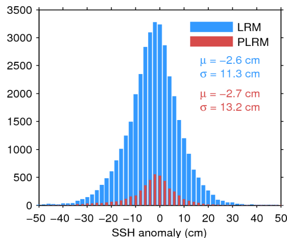
Figure 11. Histogram of science-valid SSH anomaly over oceans and lakes for LRM (blue) and PLRM (red) for 15/01/2016. The mean ( \mu ) and standard deviation ( \sigma ) are also shown. Note that values outside [-50 50] cm are excluded from the histogram for the sake of readability but not from the computation of \mu and \sigma .
