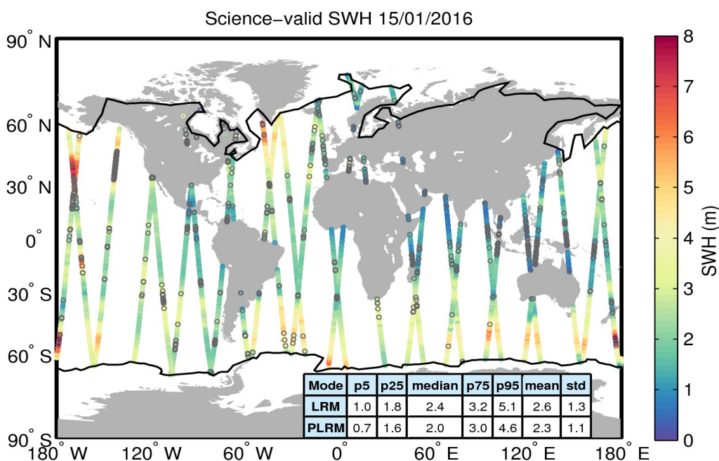
Figure 19. Geographical distribution of science-valid SWH data over oceans and lakes for 15/01/2016. The statistical values shown in the table refer to the SWH in m and are calculated separately for LRM and PLRM regions. The black lines mark the outer limit of the Arctic and Antarctic polar polygons. Gray circles denote records that have been rejected based on the editing criteria described in Table 3.
