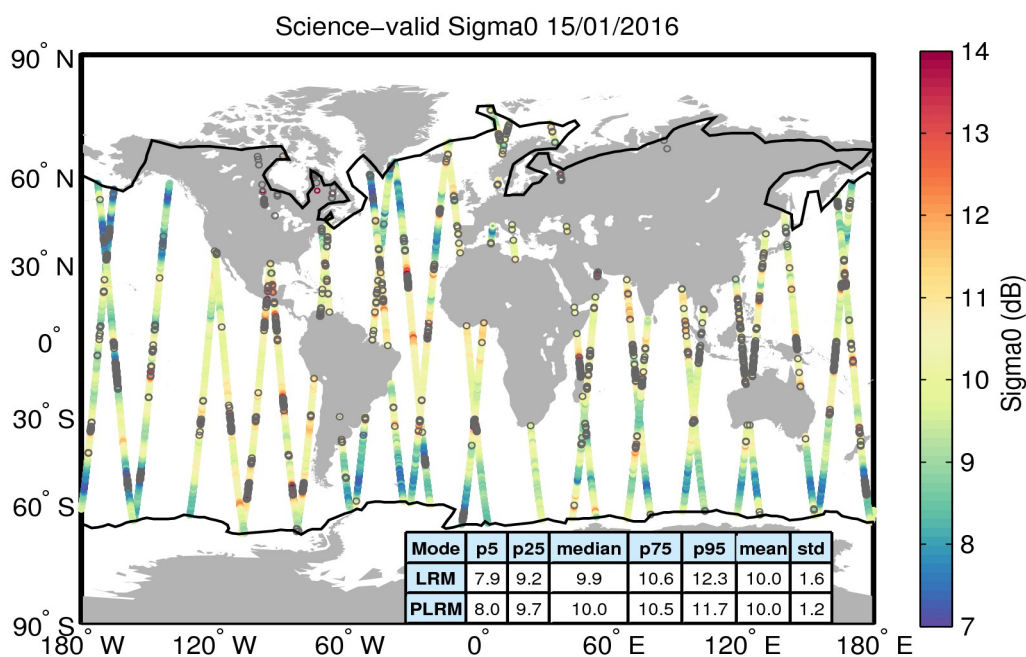
Figure 27. Geographical distribution of science-valid sigma0 data over oceans and lakes for 15/01/2016. The statistical values shown in the table refer to the sigma0 in dB and are calculated separately for LRM and PLRM regions. The black lines mark the outer limit of the Arctic and Antarctic polar polygons. Gray circles denote records that have been rejected based on the editing criteria described in Table 4.
