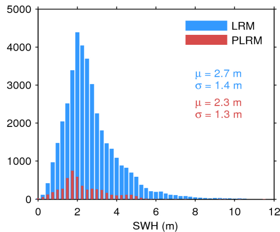
Figure 17. Histogram of flag-valid SWH over oceans and lakes for LRM (blue) and PLRM (red) for 15/01/2016. The mean ( \mu ) and standard deviation ( \sigma ) are also shown. Note that values larger than 12 m are excluded from the histogram for the sake of readability but not from the computation of \mu and \sigma .
