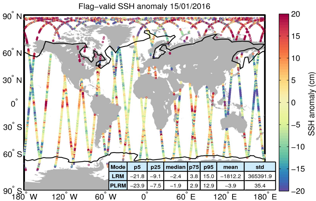
Figure 5. Geographical distribution of flag-valid 1-Hz SSH anomaly data over oceans and lakes for 15/01/2016. The statistical values shown in the table refer to the SSH anomaly in cm and are calculated separately for LRM and PLRM regions. Measurements taken over polar polygons have been excluded from the computation of the statistical values. The black lines mark the outer limit of the Arctic and Antarctic polar polygons.
