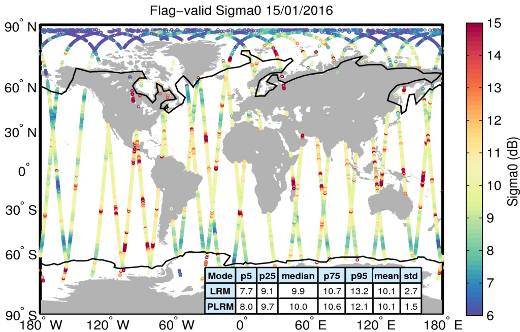
Figure 23. Geographical distribution of flag-valid sigma0 data over oceans and lakes for 15/01/2016. The statistical values shown in the table refer to the sigma0 in dB and are calculated separately for LRM and PLRM regions. Measurements taken over polar polygons have been excluded from the computation of the statistical values. The black lines mark the outer limit of the Arctic and Antarctic polar polygons.
