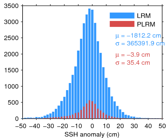
Figure 7. Histogram of flag-valid SSH anomaly over oceans and lakes for LRM (blue) and PLRM (red) for 15/01/2016. The mean ( \mu ) and standard deviation ( \sigma ) are also shown. Note that values outside [-50 \ 50] cm are excluded from the histogram for the sake of readability but not from the computation of \mu and \sigma .
