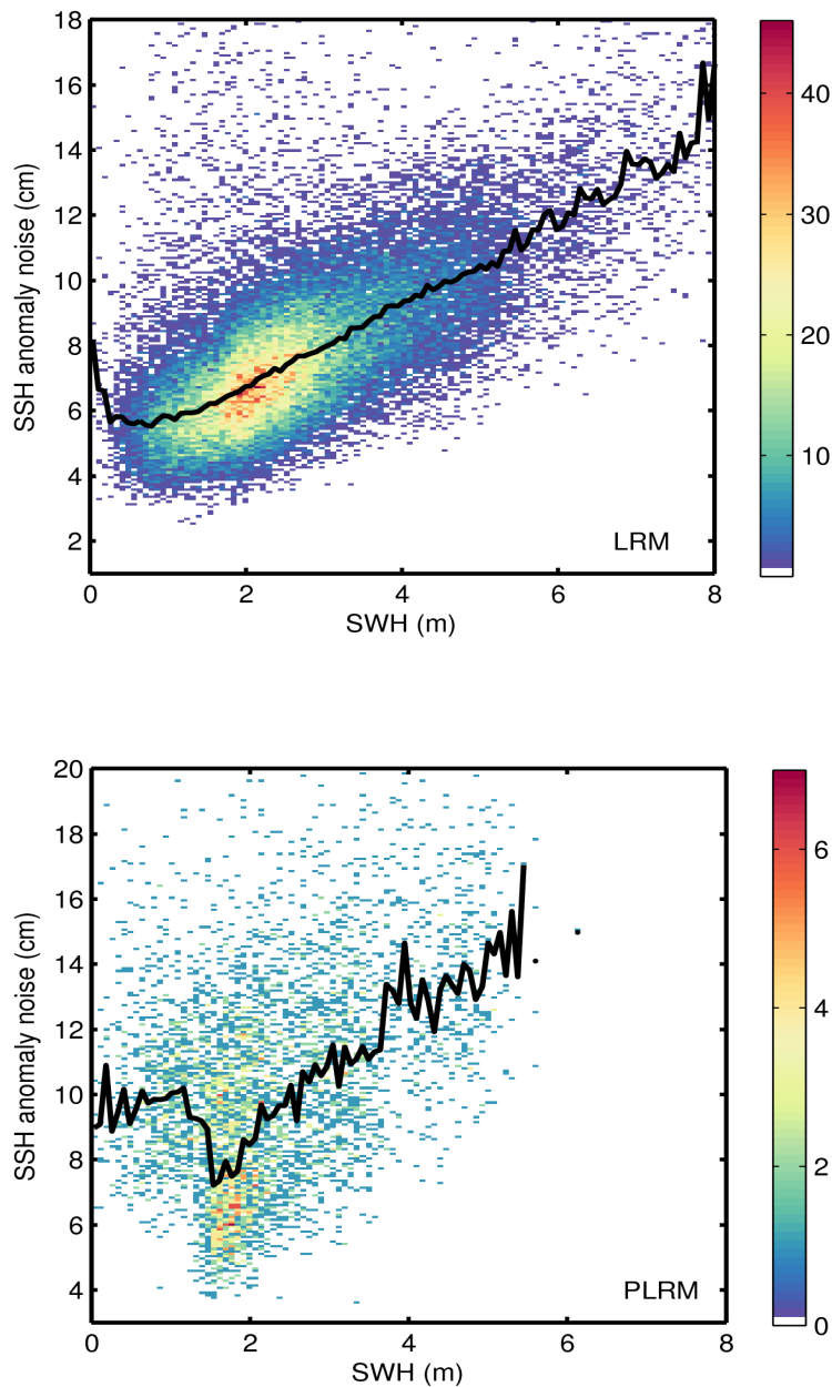
Figure 9. 2D histogram showing flag-valid SSH anomaly noise as a function of SWH for LRM (top) and PLRM (bottom) for 15/01/2016. The black line denotes the median SSH anomaly noise as a function of SWH.
