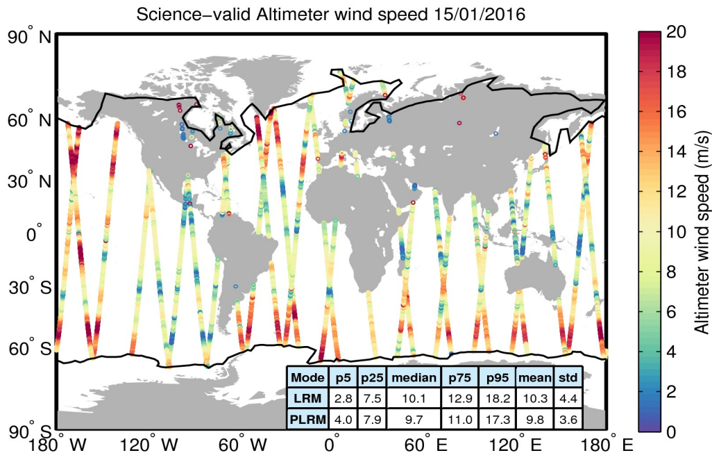
Figure 34. Geographical distribution of science-valid wind data over oceans and lakes for 15/01/2016. The statistical values shown in the table refer to the wind in m/s and are calculated separately for LRM and PLRM regions. The black lines mark the outer limit of the Arctic and Antarctic polar polygons. Gray circles denote records that have been rejected based on the editing criteria described in Table 5.
