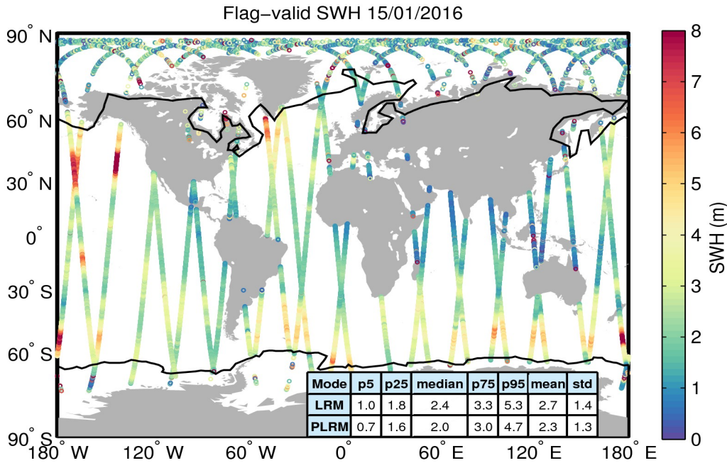
Figure 15. Geographical distribution of flag-valid SWH data over oceans and lakes for 15/01/2016. The statistical values shown in the table refer to the SWH in m and are calculated separately for LRM and PLRM regions. Measurements taken over polar polygons have been excluded from the computation of the statistical values. The black lines mark the outer limit of the Arctic and Antarctic polar polygons.
