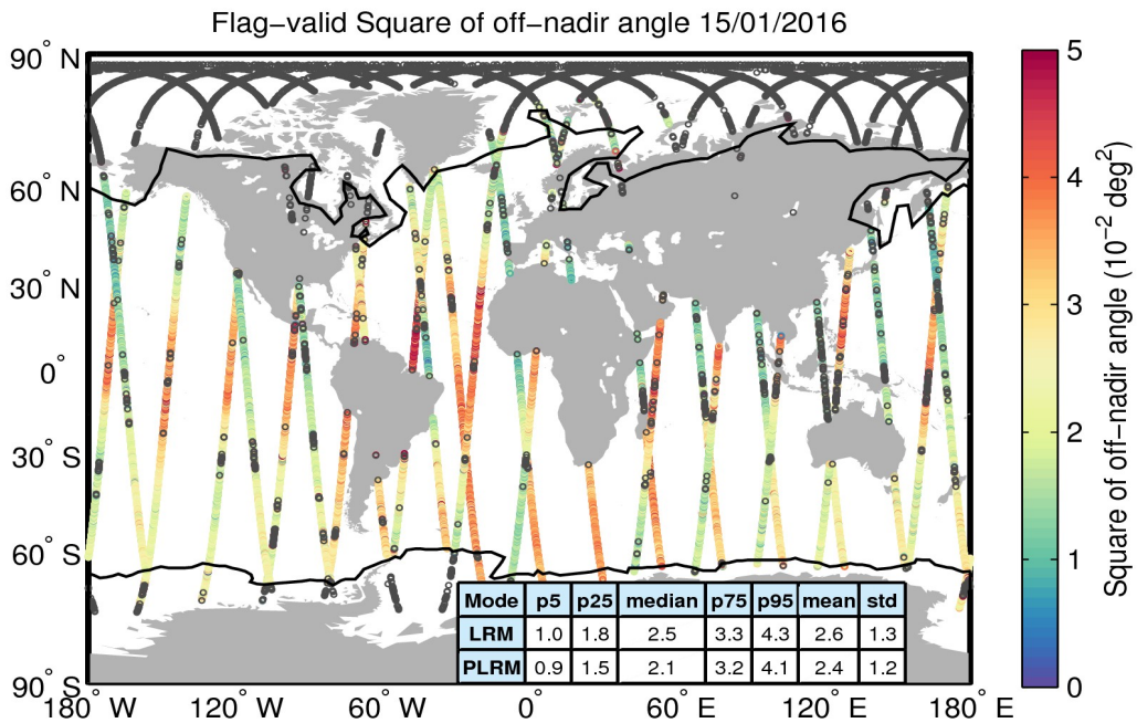
Figure 37. Geographical distribution of flag-valid mispointing data over oceans and lakes for 15/01/2016. The statistical values shown in the table refer to the mispointing in 10^{-2} deg 2 and are calculated separately for LRM and PLRM regions. Measurements taken over polar polygons have been excluded from the computation of the statistical values. The black lines mark the outer limit of the Arctic and Antarctic polar polygons. Gray circles denote negative values.
