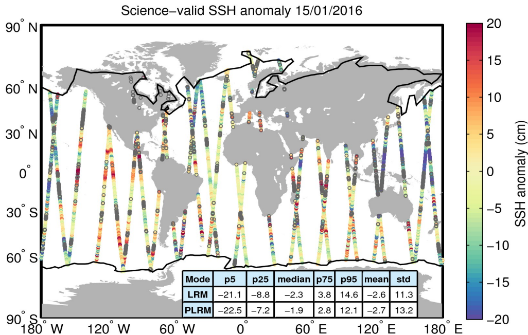
Figure 10. Geographical distribution of science-valid SSH anomaly data over oceans and lakes for 15/01/2016. The statistical values shown in the table refer to the SSH anomaly in cm and are calculated separately for LRM and PLRM regions. The black lines mark the outer limit of the Arctic and Antarctic polar polygons. Gray circles denote records that have been rejected based on the editing criteria described in Table 2.
