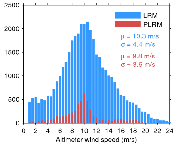
Figure 33. Histogram of flag-valid wind over oceans and lakes for LRM (blue) and PLRM (red) for 15/01/2016. The mean ( \mu ) and standard deviation ( \sigma ) are also shown. Note that values larger than 24 m/s are excluded from the histogram for the sake of readability but not from the computation of \mu and \sigma .
