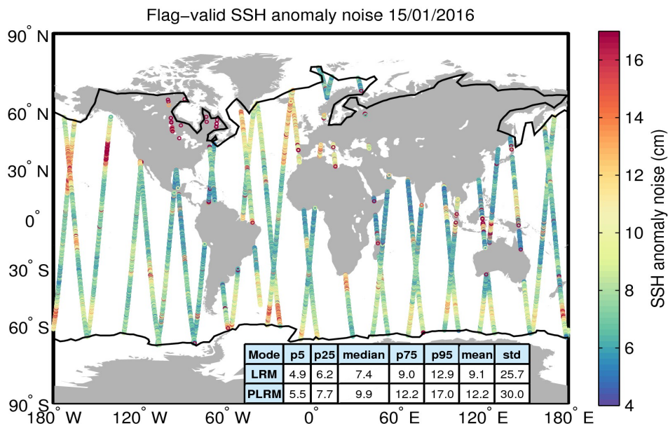
Figure 8. Geographical distribution of flag-valid 20-Hz SSH anomaly measurement noise over oceans and lakes for 15/01/2016. The statistical values shown in the table refer to the SSH anomaly noise and are calculated separately for LRM and PLRM regions. Measurements taken over polar polygons have been excluded from the computation of the statistical values. The black lines mark the outer limit of the Arctic and Antarctic polar polygons.
