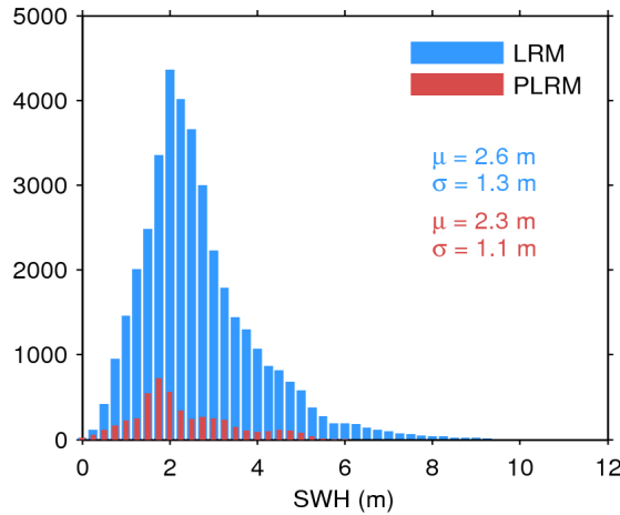
Figure 20. Histogram of science-valid SWH over oceans and lakes for LRM (blue) and PLRM (red) for 15/01/2016. The mean ( \mu ) and standard deviation ( \sigma ) are also shown. Note that values larger than 12 m are excluded from the histogram for the sake of readability but not from the computation of \mu and \sigma .
