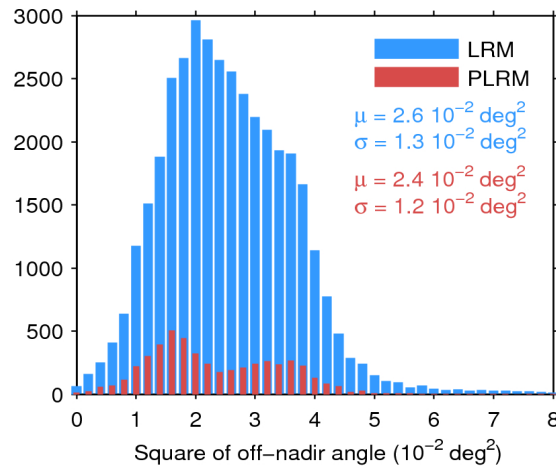
Figure 39. Histogram of flag-valid mispointing over oceans and lakes for LRM (blue) and PLRM (red) for 15/01/2016. Only positive values have been considered. The mean ( \mu ) and standard deviation ( \sigma ) are also shown. Note that values larger than 8 \cdot 10^{-2} \text{ deg}^2 are excluded from the histogram for the sake of readability but not from the computation of \mu and \sigma .
