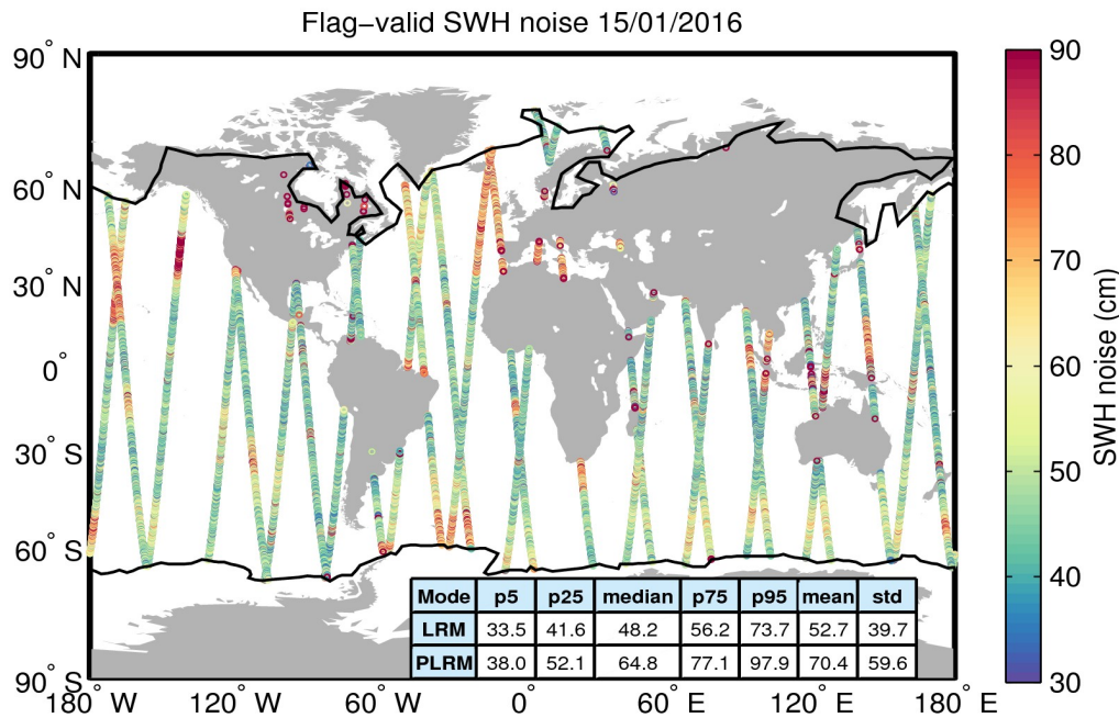
Figure 18. Geographical distribution of flag-valid 20-Hz SWH measurement noise over oceans and lakes for 15/01/2016. The statistical values shown in the table refer to the SWH noise and are calculated separately for LRM and PLRM regions. Measurements taken over polar polygons have been excluded from the computation of the statistical values. The black lines mark the outer limit of the Arctic and Antarctic polar polygons.
