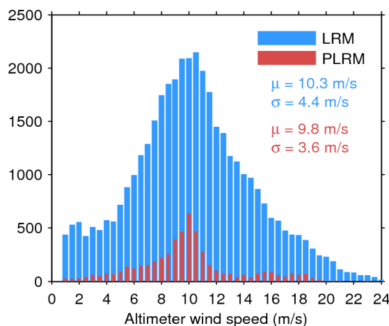
Figure 35. Histogram of science-valid wind over oceans and lakes for LRM (blue) and PLRM (red) for 15/01/2016. The mean ( \mu ) and standard deviation ( \sigma ) are also shown. Note that values larger than 24 m/s are excluded from the histogram for the sake of readability but not from the computation of \mu and \sigma .
