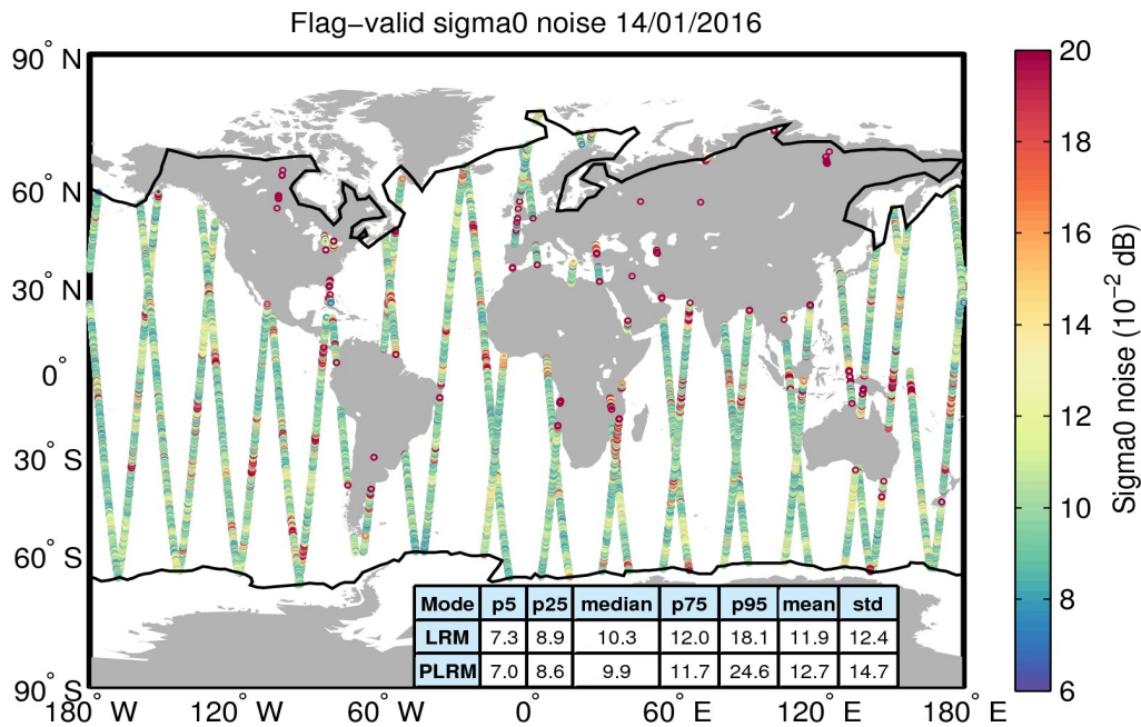
Figure 26. Geographical distribution of flag-valid 20-Hz sigma0 measurement noise over oceans and lakes for 14/01/2016. The statistical values shown in the table refer to the sigma0 noise and are calculated separately for LRM and PLRM regions. Measurements taken over polar polygons have been excluded from the computation of the statistical values. The black lines mark the outer limit of the Arctic and Antarctic polar polygons.
