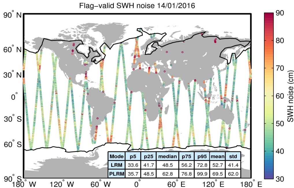
Figure 18. Geographical distribution of flag-valid 20-Hz SWH measurement noise over oceans and lakes for 14/01/2016. The statistical values shown in the table refer to the SWH noise and are calculated separately for LRM and PLRM regions. Measurements taken over polar polygons have been excluded from the computation of the statistical values. The black lines mark the outer limit of the Arctic and Antarctic polar polygons.
