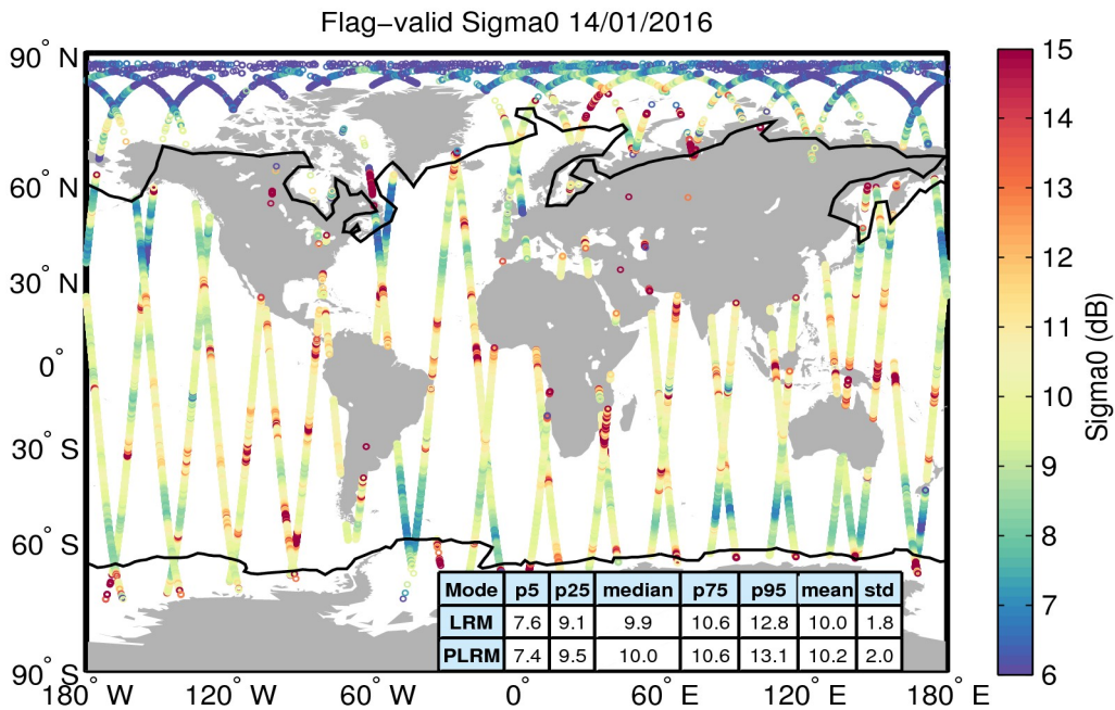
Figure 23. Geographical distribution of flag-valid sigma0 data over oceans and lakes for 14/01/2016. The statistical values shown in the table refer to the sigma0 in dB and are calculated separately for LRM and PLRM regions. Measurements taken over polar polygons have been excluded from the computation of the statistical values. The black lines mark the outer limit of the Arctic and Antarctic polar polygons.
