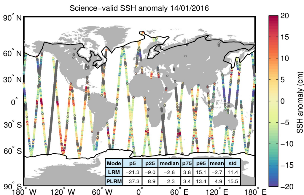
Figure 10. Geographical distribution of science-valid SSH anomaly data over oceans and lakes for 14/01/2016. The statistical values shown in the table refer to the SSH anomaly in cm and are calculated separately for LRM and PLRM regions. The black lines mark the outer limit of the Arctic and Antarctic polar polygons. Gray circles denote records that have been rejected based on the editing criteria described in Table 2.
