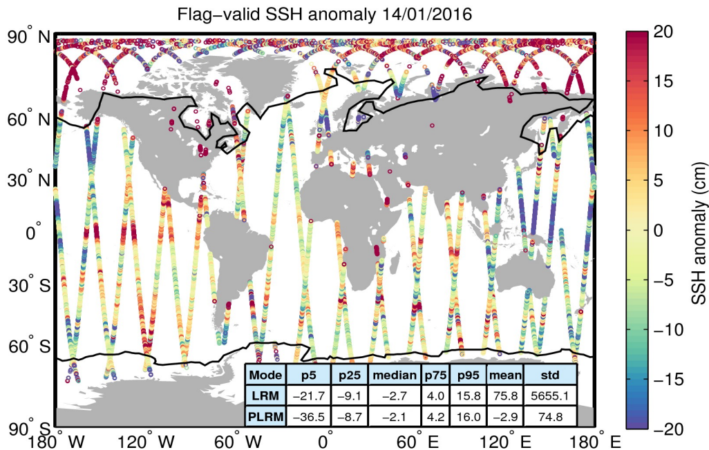
Figure 5. Geographical distribution of flag-valid 1-Hz SSH anomaly data over oceans and lakes for 14/01/2016. The statistical values shown in the table refer to the SSH anomaly in cm and are calculated separately for LRM and PLRM regions. Measurements taken over polar polygons have been excluded from the computation of the statistical values. The black lines mark the outer limit of the Arctic and Antarctic polar polygons.
