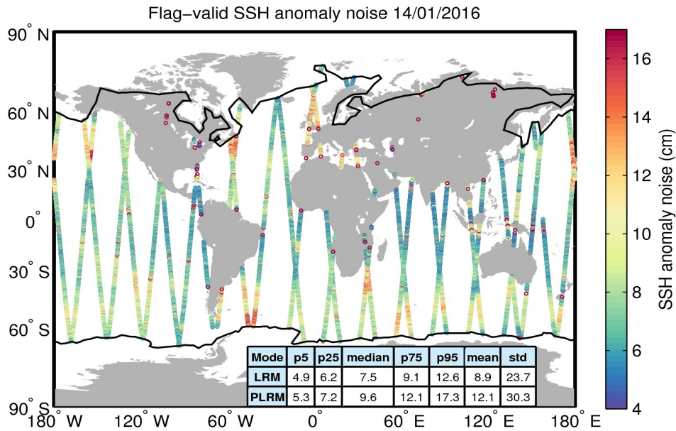
Figure 8. Geographical distribution of flag-valid 20-Hz SSH anomaly measurement noise over oceans and lakes for 14/01/2016. The statistical values shown in the table refer to the SSH anomaly noise and are calculated separately for LRM and PLRM regions. Measurements taken over polar polygons have been excluded from the computation of the statistical values. The black lines mark the outer limit of the Arctic and Antarctic polar polygons.
