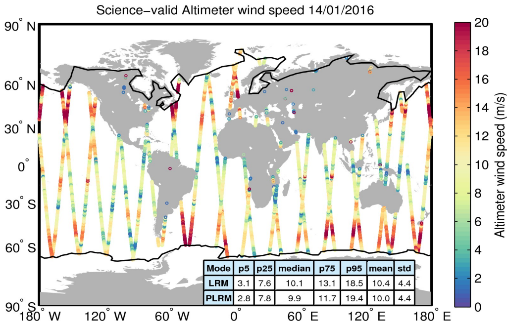
Figure 34. Geographical distribution of science-valid wind data over oceans and lakes for 14/01/2016. The statistical values shown in the table refer to the wind in m/s and are calculated separately for LRM and PLRM regions. The black lines mark the outer limit of the Arctic and Antarctic polar polygons. Gray circles denote records that have been rejected based on the editing criteria described in Table 5.
