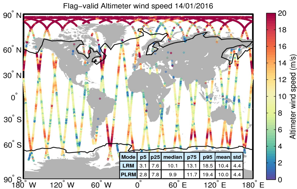
Figure 31. Geographical distribution of flag-valid wind data over oceans and lakes for 14/01/2016. The statistical values shown in the table refer to the wind in m/s and are calculated separately for LRM and PLRM regions. Measurements taken over polar polygons have been excluded from the computation of the statistical values. The black lines mark the outer limit of the Arctic and Antarctic polar polygons.
