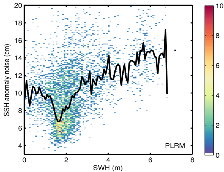
Figure 9. 2D histogram showing flag-valid SSH anomaly noise as a function of SWH for LRM (top) and PLRM (bottom) for 14/01/2016. The black line denotes the median SSH anomaly noise as a function of SWH.
