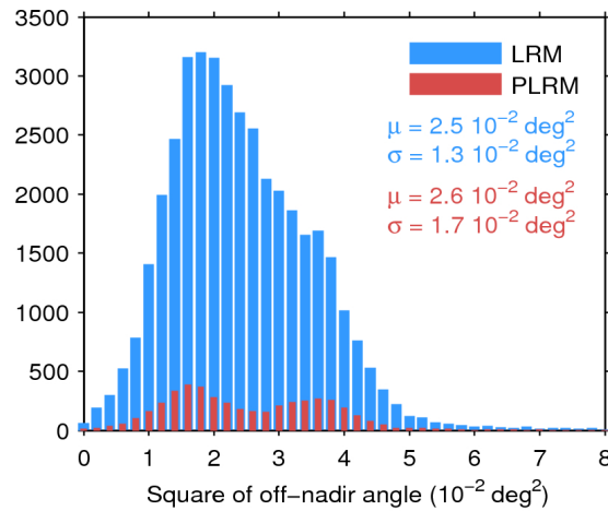
Figure 39. Histogram of flag-valid mispointing over oceans and lakes for LRM (blue) and PLRM (red) for 14/01/2016. Only positive values have been considered. The mean ( \mu ) and standard deviation ( \sigma ) are also shown. Note that values larger than 8 \cdot 10^{-2} \text{ deg}^2 are excluded from the histogram for the sake of readability but not from the computation of \mu and \sigma .
