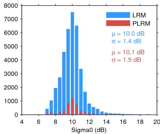
Figure 28. Histogram of science-valid sigma0 over oceans and lakes for LRM (blue) and PLRM (red) for 14/01/2016. The mean ( \mu ) and standard deviation ( \sigma ) are also shown. Note that values outside [4 20] dB are excluded from the histogram for the sake of readability but not from the computation of \mu and \sigma .
