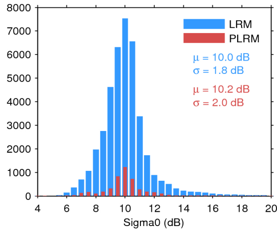
Figure 25. Histogram of flag-valid sigma0 over oceans and lakes for LRM (blue) and PLRM (red) for 14/01/2016. The mean ( \mu ) and standard deviation ( \sigma ) are also shown. Note that values outside [4 20] dB are excluded from the histogram for the sake of readability but not from the computation of \mu and \sigma .
