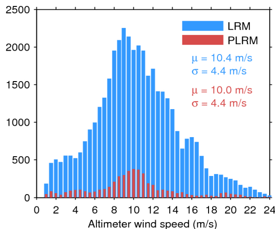
Figure 35. Histogram of science-valid wind over oceans and lakes for LRM (blue) and PLRM (red) for 14/01/2016. The mean ( \mu ) and standard deviation ( \sigma ) are also shown. Note that values larger than 24 m/s are excluded from the histogram for the sake of readability but not from the computation of \mu and \sigma .
