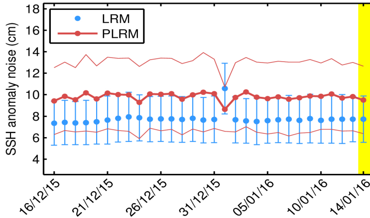
Figure 13. Average science-valid SSH anomaly noise for LRM (blue dot) and PLRM (red dot). The corresponding standard deviation (blue error bar and thin red lines, respectively) for each day in last 30-day window is also shown. The yellow shading highlights the day analyzed in this report.
