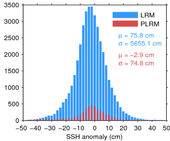
Figure 7. Histogram of flag-valid SSH anomaly over oceans and lakes for LRM (blue) and PLRM (red) for 14/01/2016. The mean ( \mu ) and standard deviation ( \sigma ) are also shown. Note that values outside [-50 50] cm are excluded from the histogram for the sake of readability but not from the computation of \mu and \sigma .
