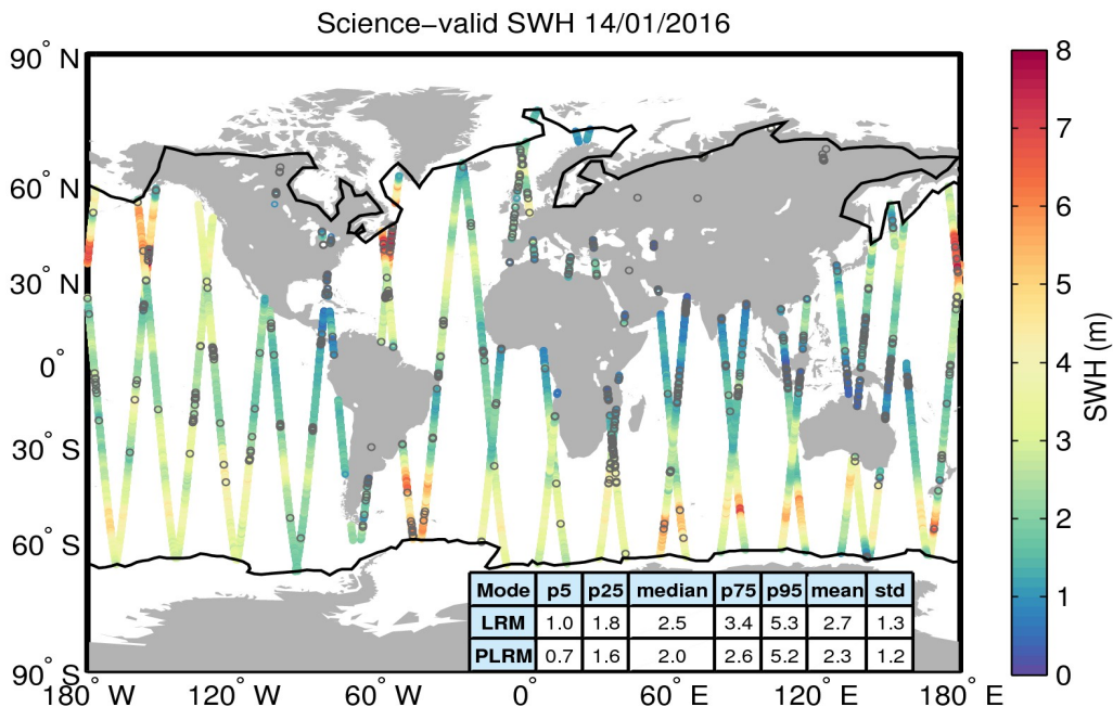
Figure 19. Geographical distribution of science-valid SWH data over oceans and lakes for 14/01/2016. The statistical values shown in the table refer to the SWH in m and are calculated separately for LRM and PLRM regions. The black lines mark the outer limit of the Arctic and Antarctic polar polygons. Gray circles denote records that have been rejected based on the editing criteria described in Table 3.
