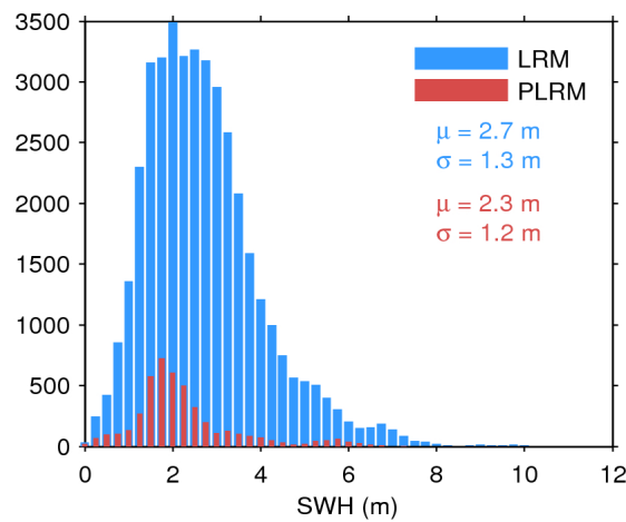
Figure 20. Histogram of science-valid SWH over oceans and lakes for LRM (blue) and PLRM (red) for 14/01/2016. The mean ( \mu ) and standard deviation ( \sigma ) are also shown. Note that values larger than 12 m are excluded from the histogram for the sake of readability but not from the computation of \mu and \sigma .
