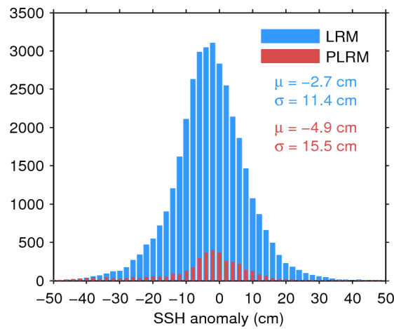
Figure 11. Histogram of science-valid SSH anomaly over oceans and lakes for LRM (blue) and PLRM (red) for 14/01/2016. The mean ( \mu ) and standard deviation ( \sigma ) are also shown. Note that values outside [-50\ 50] cm are excluded from the histogram for the sake of readability but not from the computation of \mu and \sigma .
