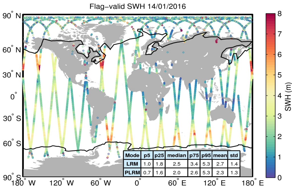
Figure 15. Geographical distribution of flag-valid SWH data over oceans and lakes for 14/01/2016. The statistical values shown in the table refer to the SWH in m and are calculated separately for LRM and PLRM regions. Measurements taken over polar polygons have been excluded from the computation of the statistical values. The black lines mark the outer limit of the Arctic and Antarctic polar polygons.
