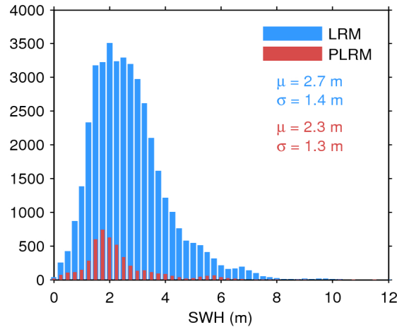
Figure 17. Histogram of flag-valid SWH over oceans and lakes for LRM (blue) and PLRM (red) for 14/01/2016. The mean ( \mu ) and standard deviation ( \sigma ) are also shown. Note that values larger than 12 m are excluded from the histogram for the sake of readability but not from the computation of \mu and \sigma .
