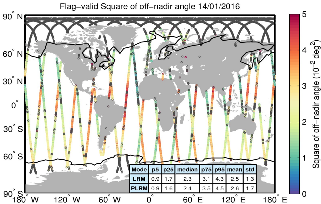
Figure 37. Geographical distribution of flag-valid mispointing data over oceans and lakes for 14/01/2016. The statistical values shown in the table refer to the mispointing in 10^{-2} deg 2 and are calculated separately for LRM and PLRM regions. Measurements taken over polar polygons have been excluded from the computation of the statistical values. The black lines mark the outer limit of the Arctic and Antarctic polar polygons. Gray circles denote negative values.
