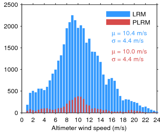
Figure 33. Histogram of flag-valid wind over oceans and lakes for LRM (blue) and PLRM (red) for 14/01/2016. The mean ( \mu ) and standard deviation ( \sigma ) are also shown. Note that values larger than 24 m/s are excluded from the histogram for the sake of readability but not from the computation of \mu and \sigma .
