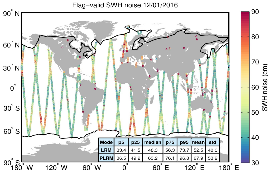
Figure 18. Geographical distribution of flag-valid 20-Hz SWH measurement noise over oceans and lakes for 12/01/2016. The statistical values shown in the table refer to the SWH noise and are calculated separately for LRM and PLRM regions. Measurements taken over polar polygons have been excluded from the computation of the statistical values. The black lines mark the outer limit of the Arctic and Antarctic polar polygons.
