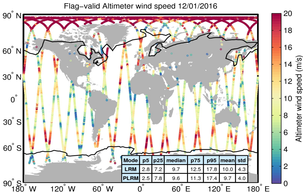
Figure 31. Geographical distribution of flag-valid wind data over oceans and lakes for 12/01/2016. The statistical values shown in the table refer to the wind in m/s and are calculated separately for LRM and PLRM regions. Measurements taken over polar polygons have been excluded from the computation of the statistical values. The black lines mark the outer limit of the Arctic and Antarctic polar polygons.
