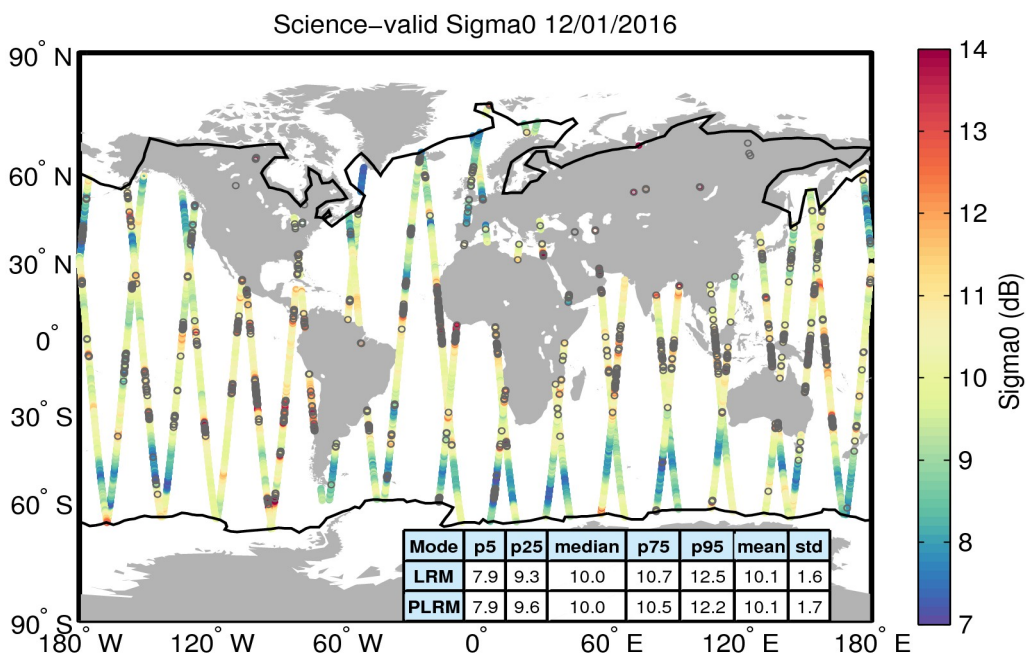
Figure 27. Geographical distribution of science-valid sigma0 data over oceans and lakes for 12/01/2016. The statistical values shown in the table refer to the sigma0 in dB and are calculated separately for LRM and PLRM regions. The black lines mark the outer limit of the Arctic and Antarctic polar polygons. Gray circles denote records that have been rejected based on the editing criteria described in Table 4.
