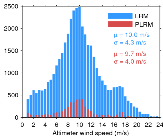
Figure 35. Histogram of science-valid wind over oceans and lakes for LRM (blue) and PLRM (red) for 12/01/2016. The mean ( \mu ) and standard deviation ( \sigma ) are also shown. Note that values larger than 24 m/s are excluded from the histogram for the sake of readability but not from the computation of \mu and \sigma .
