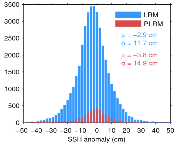
Figure 11. Histogram of science-valid SSH anomaly over oceans and lakes for LRM (blue) and PLRM (red) for 12/01/2016. The mean ( \mu ) and standard deviation ( \sigma ) are also shown. Note that values outside [-50 50] cm are excluded from the histogram for the sake of readability but not from the computation of \mu and \sigma .
