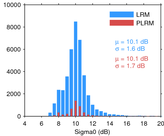
Figure 28. Histogram of science-valid sigma0 over oceans and lakes for LRM (blue) and PLRM (red) for 12/01/2016. The mean ( \mu ) and standard deviation ( \sigma ) are also shown. Note that values outside [4 20] dB are excluded from the histogram for the sake of readability but not from the computation of \mu and \sigma .
