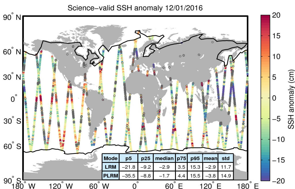
Figure 10. Geographical distribution of science-valid SSH anomaly data over oceans and lakes for 12/01/2016. The statistical values shown in the table refer to the SSH anomaly in cm and are calculated separately for LRM and PLRM regions. The black lines mark the outer limit of the Arctic and Antarctic polar polygons. Gray circles denote records that have been rejected based on the editing criteria described in Table 2.
