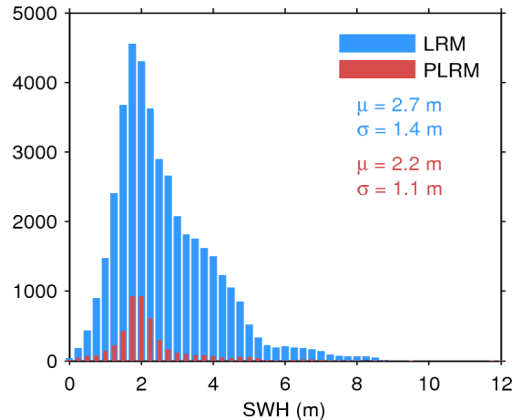
Figure 17. Histogram of flag-valid SWH over oceans and lakes for LRM (blue) and PLRM (red) for 12/01/2016. The mean ( \mu ) and standard deviation ( \sigma ) are also shown. Note that values larger than 12 m are excluded from the histogram for the sake of readability but not from the computation of \mu and \sigma .
