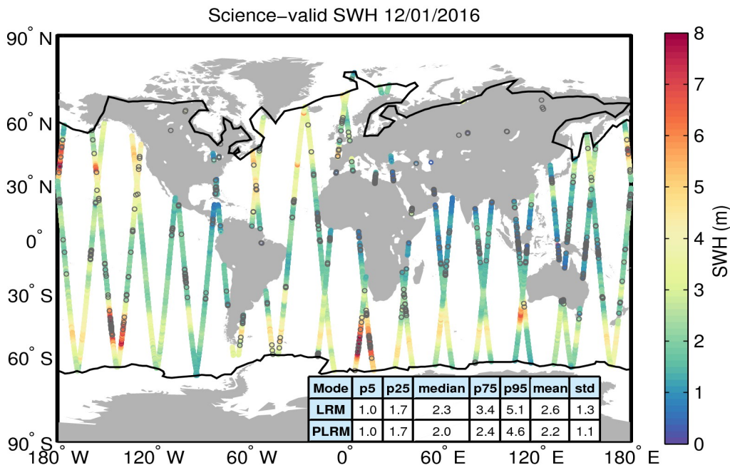
Figure 19. Geographical distribution of science-valid SWH data over oceans and lakes for 12/01/2016. The statistical values shown in the table refer to the SWH in m and are calculated separately for LRM and PLRM regions. The black lines mark the outer limit of the Arctic and Antarctic polar polygons. Gray circles denote records that have been rejected based on the editing criteria described in Table 3.
