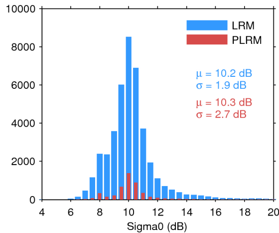
Figure 25. Histogram of flag-valid sigma0 over oceans and lakes for LRM (blue) and PLRM (red) for 12/01/2016. The mean ( \mu ) and standard deviation ( \sigma ) are also shown. Note that values outside [4 20] dB are excluded from the histogram for the sake of readability but not from the computation of \mu and \sigma .
