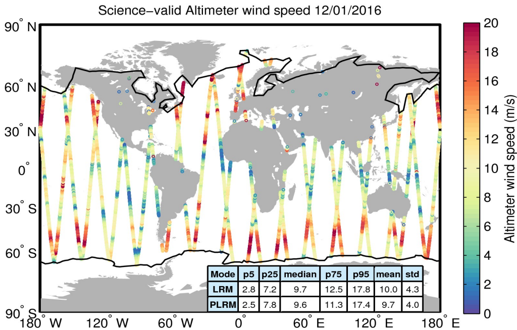
Figure 34. Geographical distribution of science-valid wind data over oceans and lakes for 12/01/2016. The statistical values shown in the table refer to the wind in m/s and are calculated separately for LRM and PLRM regions. The black lines mark the outer limit of the Arctic and Antarctic polar polygons. Gray circles denote records that have been rejected based on the editing criteria described in Table 5.
