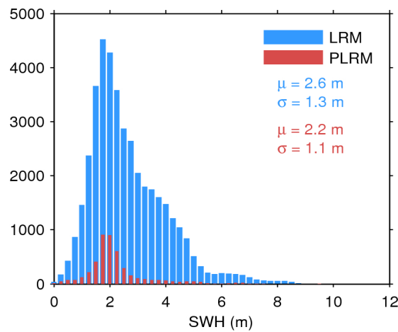
Figure 20. Histogram of science-valid SWH over oceans and lakes for LRM (blue) and PLRM (red) for 12/01/2016. The mean ( \mu ) and standard deviation ( \sigma ) are also shown. Note that values larger than 12 m are excluded from the histogram for the sake of readability but not from the computation of \mu and \sigma .
