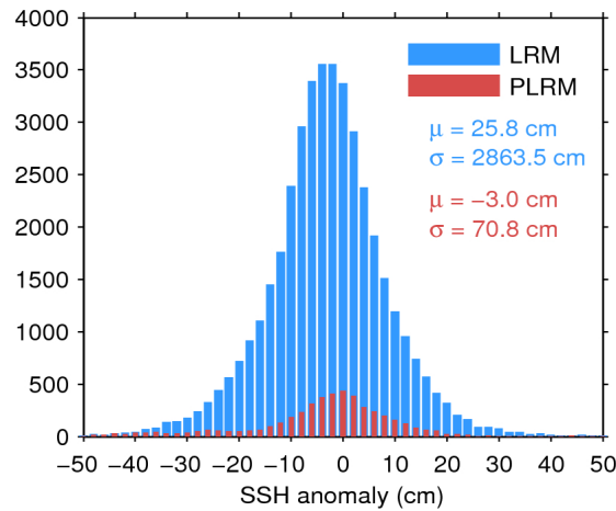
Figure 7. Histogram of flag-valid SSH anomaly over oceans and lakes for LRM (blue) and PLRM (red) for 12/01/2016. The mean ( \mu ) and standard deviation ( \sigma ) are also shown. Note that values outside [-50 \ 50] cm are excluded from the histogram for the sake of readability but not from the computation of \mu and \sigma .
