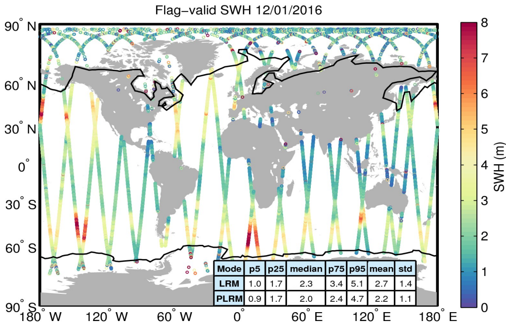
Figure 15. Geographical distribution of flag-valid SWH data over oceans and lakes for 12/01/2016. The statistical values shown in the table refer to the SWH in m and are calculated separately for LRM and PLRM regions. Measurements taken over polar polygons have been excluded from the computation of the statistical values. The black lines mark the outer limit of the Arctic and Antarctic polar polygons.
