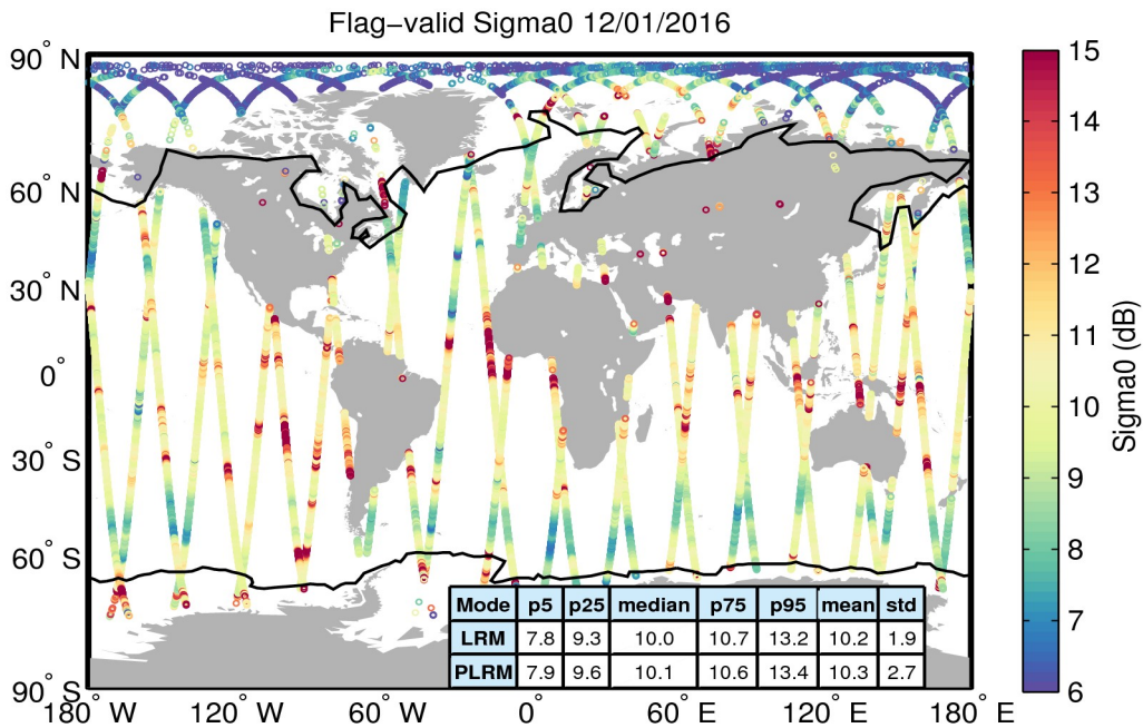
Figure 23. Geographical distribution of flag-valid sigma0 data over oceans and lakes for 12/01/2016. The statistical values shown in the table refer to the sigma0 in dB and are calculated separately for LRM and PLRM regions. Measurements taken over polar polygons have been excluded from the computation of the statistical values. The black lines mark the outer limit of the Arctic and Antarctic polar polygons.
