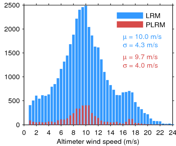
Figure 33. Histogram of flag-valid wind over oceans and lakes for LRM (blue) and PLRM (red) for 12/01/2016. The mean ( \mu ) and standard deviation ( \sigma ) are also shown. Note that values larger than 24 m/s are excluded from the histogram for the sake of readability but not from the computation of \mu and \sigma .
