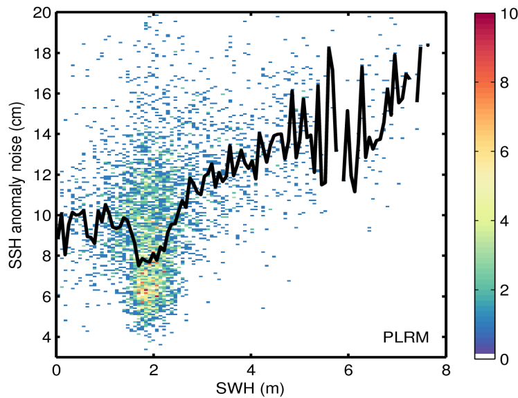
Figure 9. 2D histogram showing flag-valid SSH anomaly noise as a function of SWH for LRM (top) and PLRM (bottom) for 12/01/2016. The black line denotes the median SSH anomaly noise as a function of SWH.
