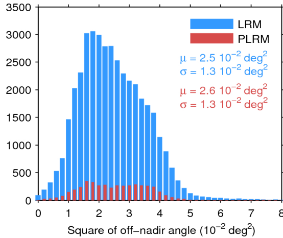
Figure 39. Histogram of flag-valid mispointing over oceans and lakes for LRM (blue) and PLRM (red) for 12/01/2016. Only positive values have been considered. The mean ( \mu ) and standard deviation ( \sigma ) are also shown. Note that values larger than 8 \cdot 10^{-2} \text{ deg}^2 are excluded from the histogram for the sake of readability but not from the computation of \mu and \sigma .
