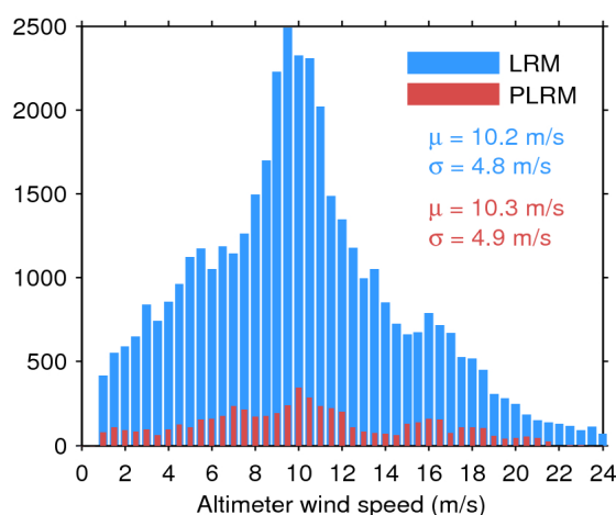
Figure 33. Histogram of flag-valid wind over oceans and lakes for LRM (blue) and PLRM (red) for 11/01/2016. The mean ( \mu ) and standard deviation ( \sigma ) are also shown. Note that values larger than 24 m/s are excluded from the histogram for the sake of readability but not from the computation of \mu and \sigma .
