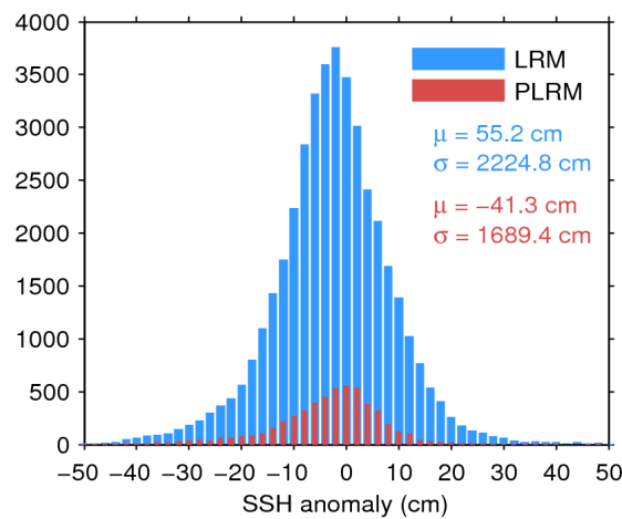
Figure 7. Histogram of flag-valid SSH anomaly over oceans and lakes for LRM (blue) and PLRM (red) for 11/01/2016. The mean ( \mu ) and standard deviation ( \sigma ) are also shown. Note that values outside [-50 50] cm are excluded from the histogram for the sake of readability but not from the computation of \mu and \sigma .
