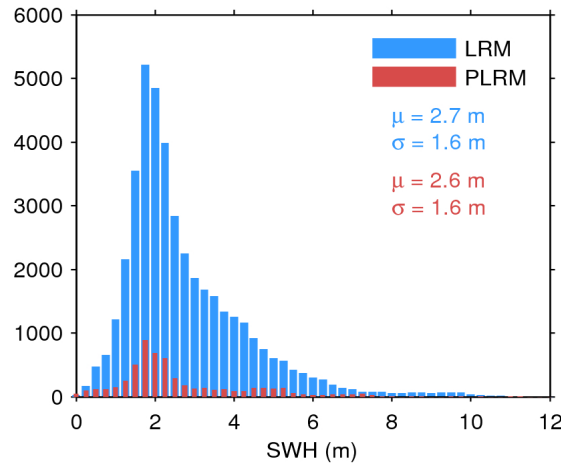
Figure 17. Histogram of flag-valid SWH over oceans and lakes for LRM (blue) and PLRM (red) for 11/01/2016. The mean ( \mu ) and standard deviation ( \sigma ) are also shown. Note that values larger than 12 m are excluded from the histogram for the sake of readability but not from the computation of \mu and \sigma .
