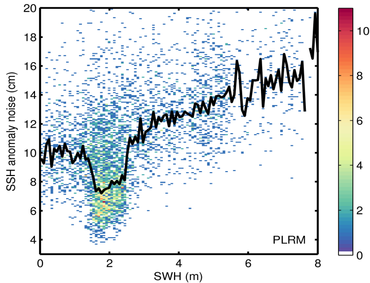
Figure 9. 2D histogram showing flag-valid SSH anomaly noise as a function of SWH for LRM (top) and PLRM (bottom) for 11/01/2016. The black line denotes the median SSH anomaly noise as a function of SWH.
