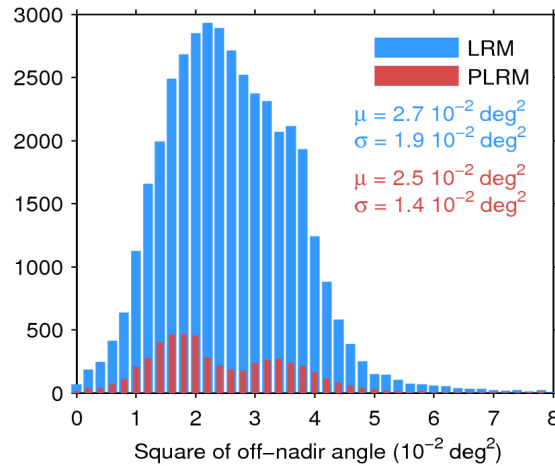
Figure 39. Histogram of flag-valid mispointing over oceans and lakes for LRM (blue) and PLRM (red) for 11/01/2016. Only positive values have been considered. The mean ( \mu ) and standard deviation ( \sigma ) are also shown. Note that values larger than 8 \cdot 10^{-2} \text{ deg}^2 are excluded from the histogram for the sake of readability but not from the computation of \mu and \sigma .
