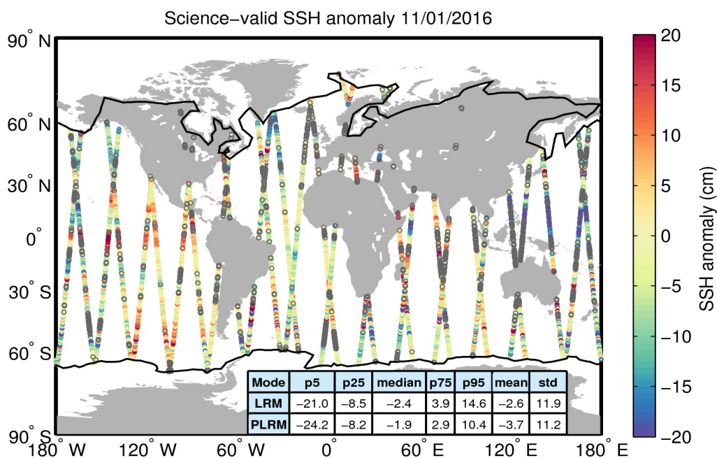
Figure 10. Geographical distribution of science-valid SSH anomaly data over oceans and lakes for 11/01/2016. The statistical values shown in the table refer to the SSH anomaly in cm and are calculated separately for LRM and PLRM regions. The black lines mark the outer limit of the Arctic and Antarctic polar polygons. Gray circles denote records that have been rejected based on the editing criteria described in Table 2.
