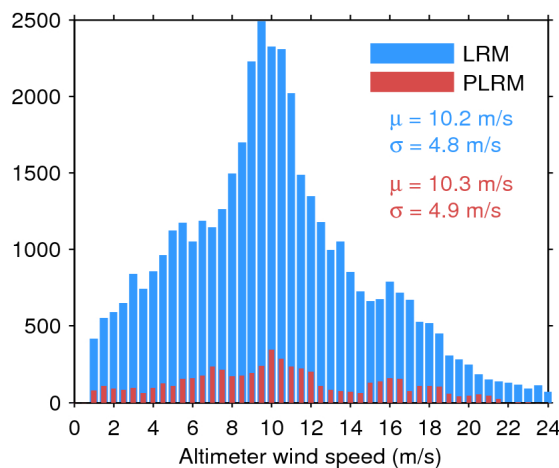
Figure 35. Histogram of science-valid wind over oceans and lakes for LRM (blue) and PLRM (red) for 11/01/2016. The mean ( \mu ) and standard deviation ( \sigma ) are also shown. Note that values larger than 24 m/s are excluded from the histogram for the sake of readability but not from the computation of \mu and \sigma .
