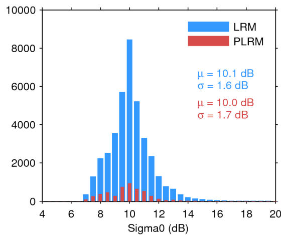
Figure 28. Histogram of science-valid sigma0 over oceans and lakes for LRM (blue) and PLRM (red) for 11/01/2016. The mean ( \mu ) and standard deviation ( \sigma ) are also shown. Note that values outside [4 20] dB are excluded from the histogram for the sake of readability but not from the computation of \mu and \sigma .
