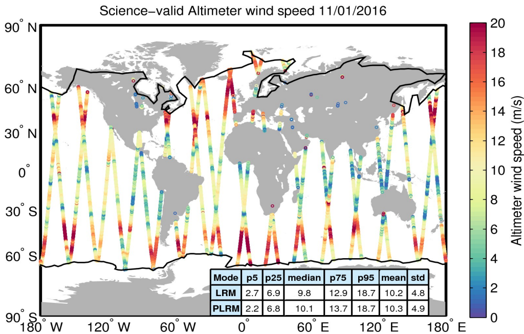
Figure 34. Geographical distribution of science-valid wind data over oceans and lakes for 11/01/2016. The statistical values shown in the table refer to the wind in m/s and are calculated separately for LRM and PLRM regions. The black lines mark the outer limit of the Arctic and Antarctic polar polygons. Gray circles denote records that have been rejected based on the editing criteria described in Table 5.
