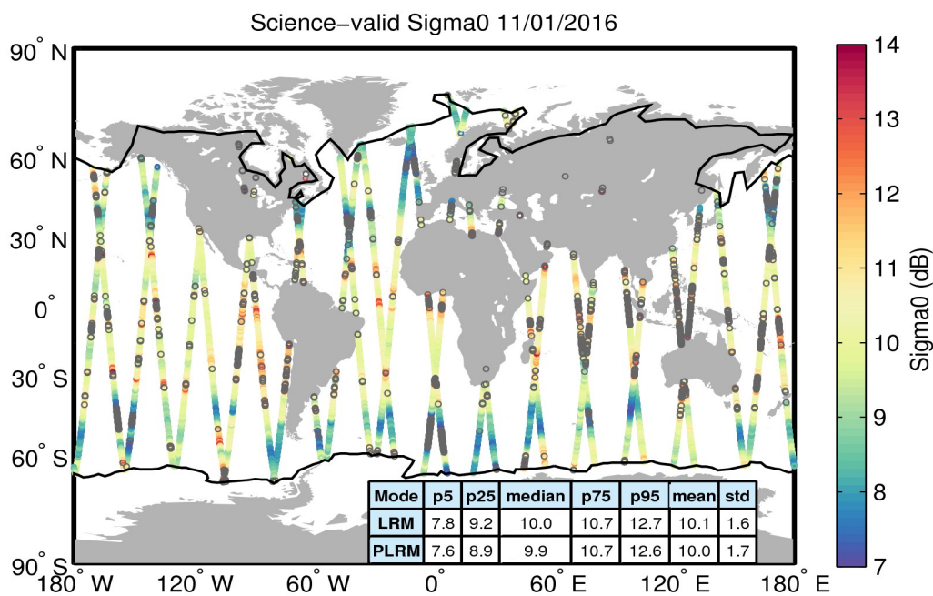
Figure 27. Geographical distribution of science-valid sigma0 data over oceans and lakes for 11/01/2016. The statistical values shown in the table refer to the sigma0 in dB and are calculated separately for LRM and PLRM regions. The black lines mark the outer limit of the Arctic and Antarctic polar polygons. Gray circles denote records that have been rejected based on the editing criteria described in Table 4.
