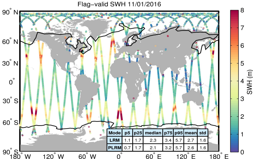
Figure 15. Geographical distribution of flag-valid SWH data over oceans and lakes for 11/01/2016. The statistical values shown in the table refer to the SWH in m and are calculated separately for LRM and PLRM regions. Measurements taken over polar polygons have been excluded from the computation of the statistical values. The black lines mark the outer limit of the Arctic and Antarctic polar polygons.
