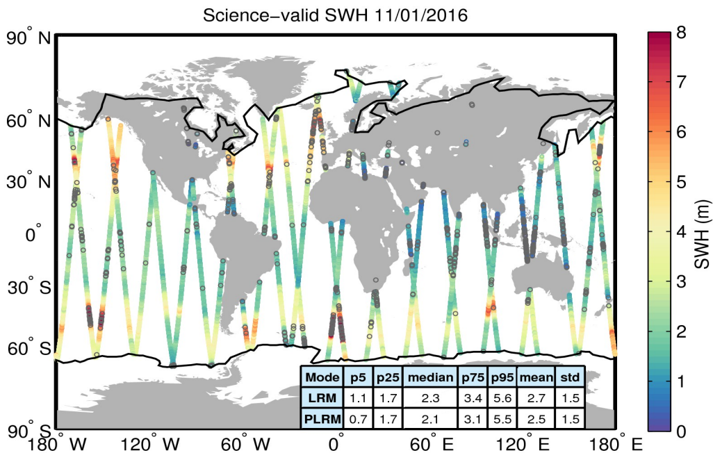
Figure 19. Geographical distribution of science-valid SWH data over oceans and lakes for 11/01/2016. The statistical values shown in the table refer to the SWH in m and are calculated separately for LRM and PLRM regions. The black lines mark the outer limit of the Arctic and Antarctic polar polygons. Gray circles denote records that have been rejected based on the editing criteria described in Table 3.
