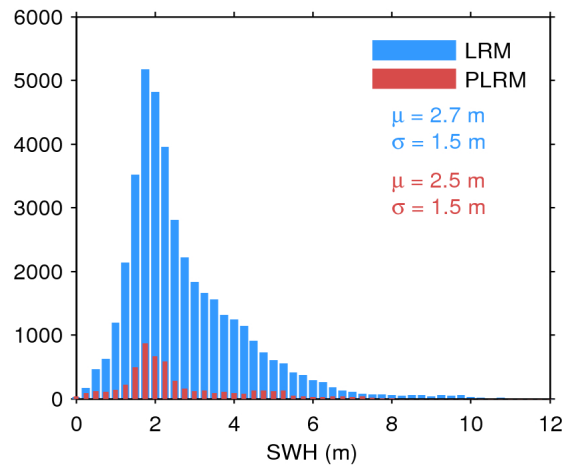
Figure 20. Histogram of science-valid SWH over oceans and lakes for LRM (blue) and PLRM (red) for 11/01/2016. The mean ( \mu ) and standard deviation ( \sigma ) are also shown. Note that values larger than 12 m are excluded from the histogram for the sake of readability but not from the computation of \mu and \sigma .
