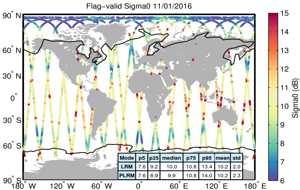
Figure 23. Geographical distribution of flag-valid sigma0 data over oceans and lakes for 11/01/2016. The statistical values shown in the table refer to the sigma0 in dB and are calculated separately for LRM and PLRM regions. Measurements taken over polar polygons have been excluded from the computation of the statistical values. The black lines mark the outer limit of the Arctic and Antarctic polar polygons.
