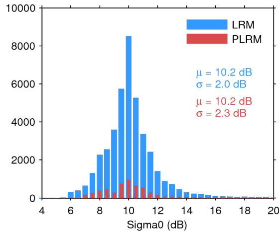
Figure 25. Histogram of flag-valid sigma0 over oceans and lakes for LRM (blue) and PLRM (red) for 11/01/2016. The mean ( \mu ) and standard deviation ( \sigma ) are also shown. Note that values outside [4 20] dB are excluded from the histogram for the sake of readability but not from the computation of \mu and \sigma .
