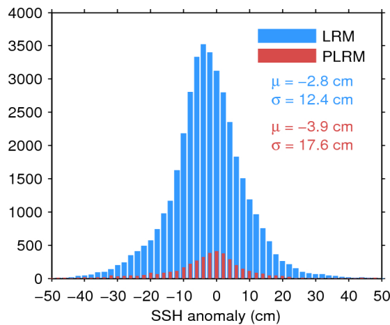
Figure 11. Histogram of science-valid SSH anomaly over oceans and lakes for LRM (blue) and PLRM (red) for 06/01/2016. The mean ( \mu ) and standard deviation ( \sigma ) are also shown. Note that values outside [-50 50] cm are excluded from the histogram for the sake of readability but not from the computation of \mu and \sigma .
