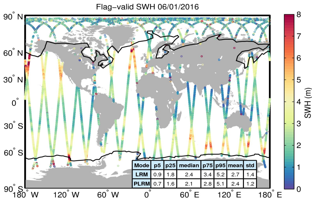
Figure 15. Geographical distribution of flag-valid SWH data over oceans and lakes for 06/01/2016. The statistical values shown in the table refer to the SWH in m and are calculated separately for LRM and PLRM regions. Measurements taken over polar polygons have been excluded from the computation of the statistical values. The black lines mark the outer limit of the Arctic and Antarctic polar polygons.
