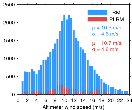
Figure 35. Histogram of science-valid wind over oceans and lakes for LRM (blue) and PLRM (red) for 06/01/2016. The mean ( \mu ) and standard deviation ( \sigma ) are also shown. Note that values larger than 24 m/s are excluded from the histogram for the sake of readability but not from the computation of \mu and \sigma .
