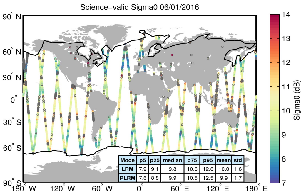
Figure 27. Geographical distribution of science-valid sigma0 data over oceans and lakes for 06/01/2016. The statistical values shown in the table refer to the sigma0 in dB and are calculated separately for LRM and PLRM regions. The black lines mark the outer limit of the Arctic and Antarctic polar polygons. Gray circles denote records that have been rejected based on the editing criteria described in Table 4.
