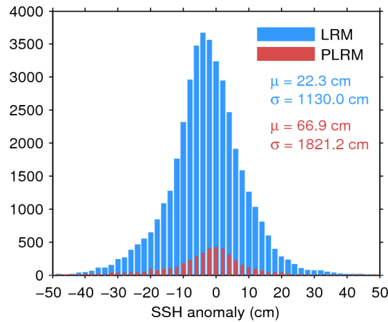
Figure 7. Histogram of flag-valid SSH anomaly over oceans and lakes for LRM (blue) and PLRM (red) for 06/01/2016. The mean ( \mu ) and standard deviation ( \sigma ) are also shown. Note that values outside [-50\ 50] cm are excluded from the histogram for the sake of readability but not from the computation of \mu and \sigma .
