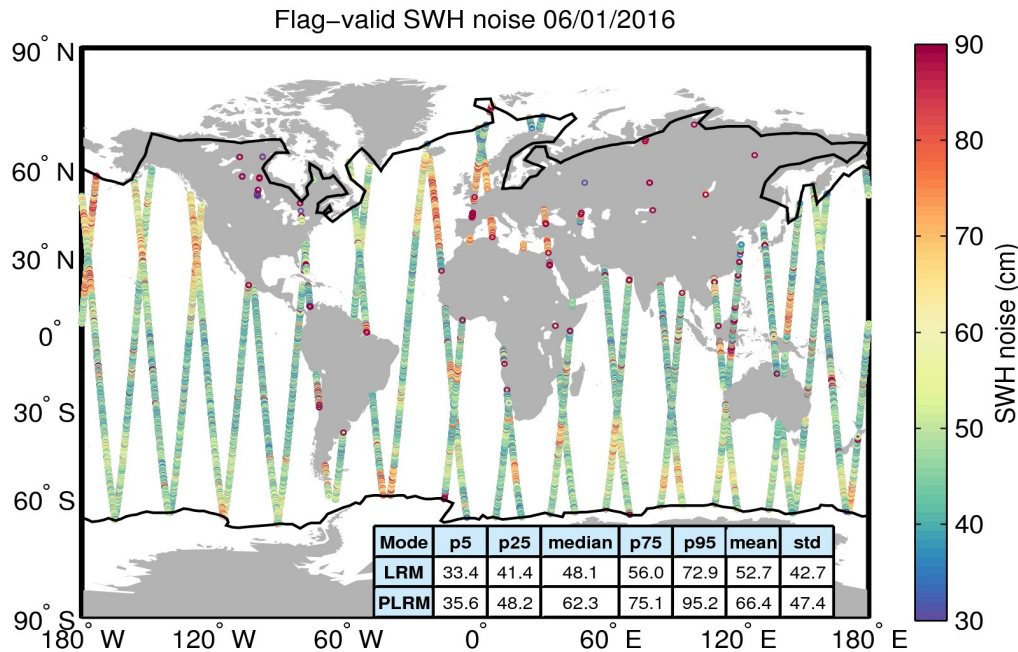
Figure 18. Geographical distribution of flag-valid 20-Hz SWH measurement noise over oceans and lakes for 06/01/2016. The statistical values shown in the table refer to the SWH noise and are calculated separately for LRM and PLRM regions. Measurements taken over polar polygons have been excluded from the computation of the statistical values. The black lines mark the outer limit of the Arctic and Antarctic polar polygons.
