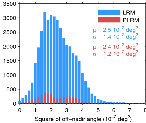
Figure 39. Histogram of flag-valid mispointing over oceans and lakes for LRM (blue) and PLRM (red) for 06/01/2016. Only positive values have been considered. The mean ( \mu ) and standard deviation ( \sigma ) are also shown. Note that values larger than 8 \cdot 10^{-2} \text{ deg}^2 are excluded from the histogram for the sake of readability but not from the computation of \mu and \sigma .
