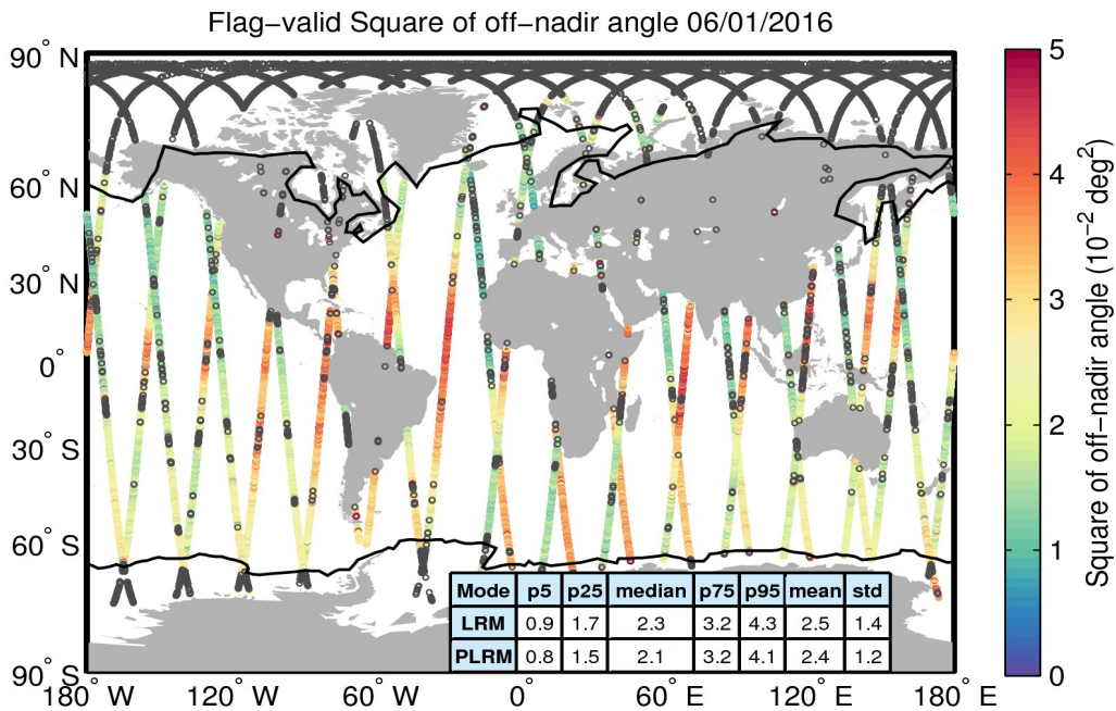
Figure 37. Geographical distribution of flag-valid mispointing data over oceans and lakes for 06/01/2016. The statistical values shown in the table refer to the mispointing in 10^{-2} deg 2 and are calculated separately for LRM and PLRM regions. Measurements taken over polar polygons have been excluded from the computation of the statistical values. The black lines mark the outer limit of the Arctic and Antarctic polar polygons. Gray circles denote negative values.
