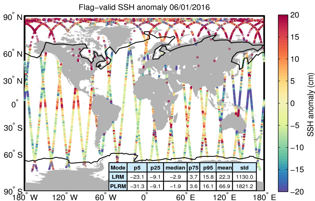
Figure 5. Geographical distribution of flag-valid 1-Hz SSH anomaly data over oceans and lakes for 06/01/2016. The statistical values shown in the table refer to the SSH anomaly in cm and are calculated separately for LRM and PLRM regions. Measurements taken over polar polygons have been excluded from the computation of the statistical values. The black lines mark the outer limit of the Arctic and Antarctic polar polygons.
