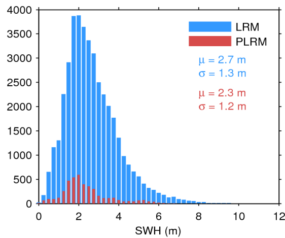
Figure 20. Histogram of science-valid SWH over oceans and lakes for LRM (blue) and PLRM (red) for 06/01/2016. The mean ( \mu ) and standard deviation ( \sigma ) are also shown. Note that values larger than 12 m are excluded from the histogram for the sake of readability but not from the computation of \mu and \sigma .
