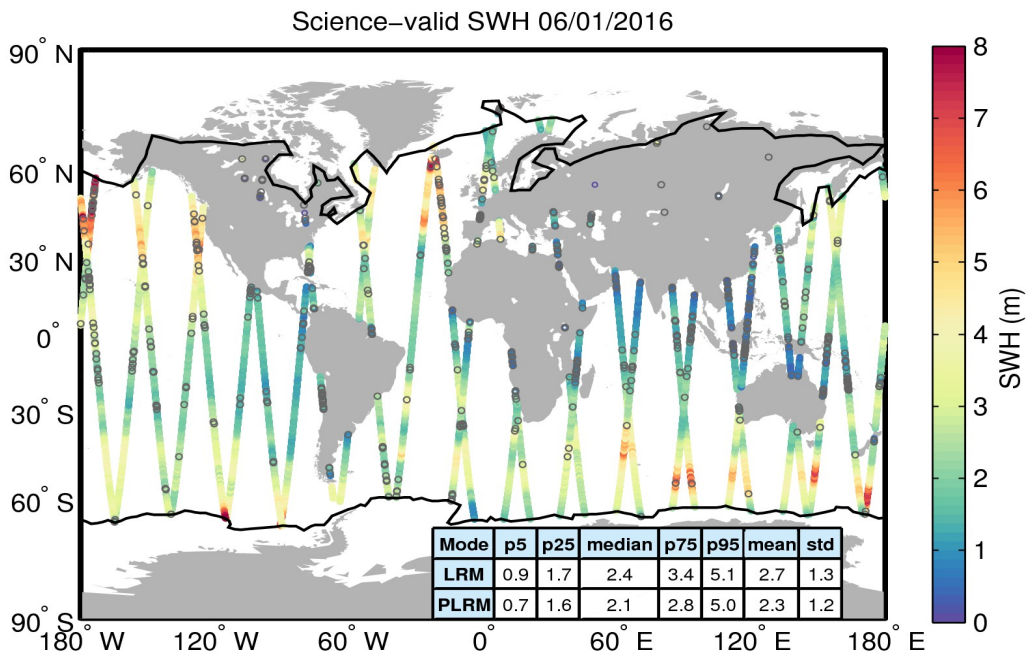
Figure 19. Geographical distribution of science-valid SWH data over oceans and lakes for 06/01/2016. The statistical values shown in the table refer to the SWH in m and are calculated separately for LRM and PLRM regions. The black lines mark the outer limit of the Arctic and Antarctic polar polygons. Gray circles denote records that have been rejected based on the editing criteria described in Table 3.
