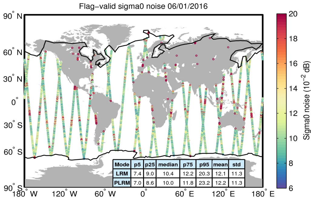
Figure 26. Geographical distribution of flag-valid 20-Hz sigma0 measurement noise over oceans and lakes for 06/01/2016. The statistical values shown in the table refer to the sigma0 noise and are calculated separately for LRM and PLRM regions. Measurements taken over polar polygons have been excluded from the computation of the statistical values. The black lines mark the outer limit of the Arctic and Antarctic polar polygons.
