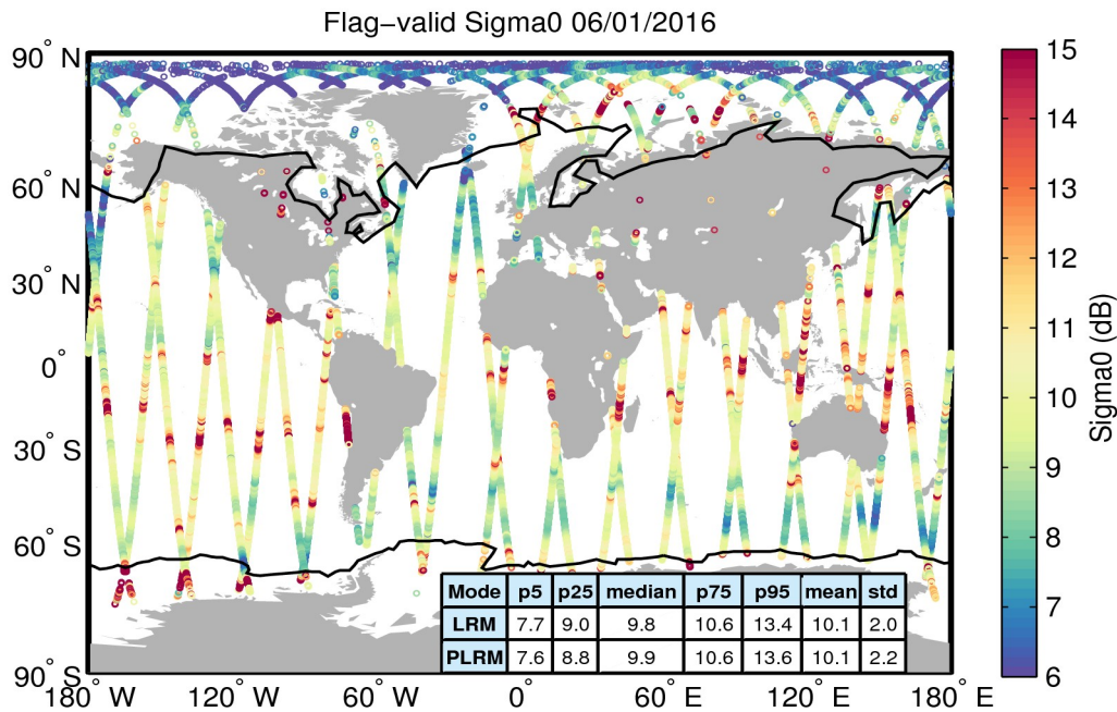
Figure 23. Geographical distribution of flag-valid sigma0 data over oceans and lakes for 06/01/2016. The statistical values shown in the table refer to the sigma0 in dB and are calculated separately for LRM and PLRM regions. Measurements taken over polar polygons have been excluded from the computation of the statistical values. The black lines mark the outer limit of the Arctic and Antarctic polar polygons.
