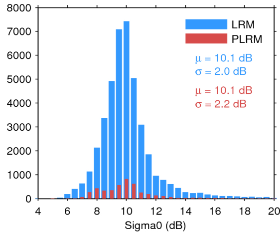
Figure 25. Histogram of flag-valid sigma0 over oceans and lakes for LRM (blue) and PLRM (red) for 06/01/2016. The mean ( \mu ) and standard deviation ( \sigma ) are also shown. Note that values outside [4 20] dB are excluded from the histogram for the sake of readability but not from the computation of \mu and \sigma .
