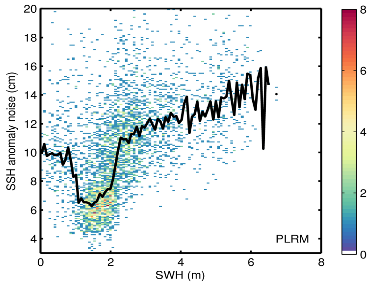
Figure 9. 2D histogram showing flag-valid SSH anomaly noise as a function of SWH for LRM (top) and PLRM (bottom) for 06/01/2016. The black line denotes the median SSH anomaly noise as a function of SWH.
