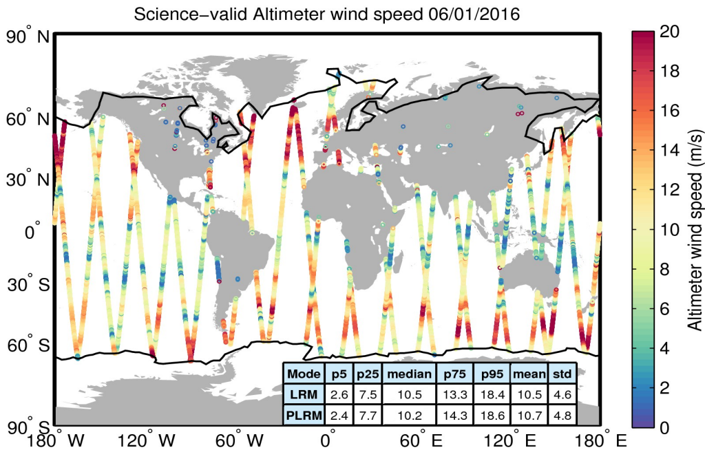
Figure 34. Geographical distribution of science-valid wind data over oceans and lakes for 06/01/2016. The statistical values shown in the table refer to the wind in m/s and are calculated separately for LRM and PLRM regions. The black lines mark the outer limit of the Arctic and Antarctic polar polygons. Gray circles denote records that have been rejected based on the editing criteria described in Table 5.
