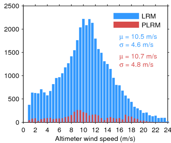
Figure 33. Histogram of flag-valid wind over oceans and lakes for LRM (blue) and PLRM (red) for 06/01/2016. The mean ( \mu ) and standard deviation ( \sigma ) are also shown. Note that values larger than 24 m/s are excluded from the histogram for the sake of readability but not from the computation of \mu and \sigma .
