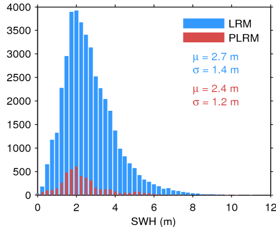
Figure 17. Histogram of flag-valid SWH over oceans and lakes for LRM (blue) and PLRM (red) for 06/01/2016. The mean ( \mu ) and standard deviation ( \sigma ) are also shown. Note that values larger than 12 m are excluded from the histogram for the sake of readability but not from the computation of \mu and \sigma .
