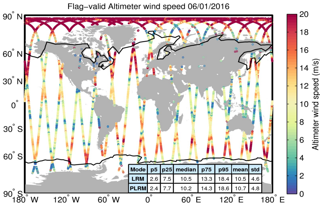
Figure 31. Geographical distribution of flag-valid wind data over oceans and lakes for 06/01/2016. The statistical values shown in the table refer to the wind in m/s and are calculated separately for LRM and PLRM regions. Measurements taken over polar polygons have been excluded from the computation of the statistical values. The black lines mark the outer limit of the Arctic and Antarctic polar polygons.
