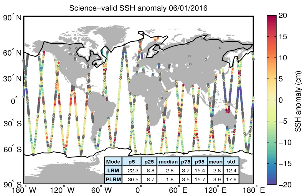
Figure 10. Geographical distribution of science-valid SSH anomaly data over oceans and lakes for 06/01/2016. The statistical values shown in the table refer to the SSH anomaly in cm and are calculated separately for LRM and PLRM regions. The black lines mark the outer limit of the Arctic and Antarctic polar polygons. Gray circles denote records that have been rejected based on the editing criteria described in Table 2.
