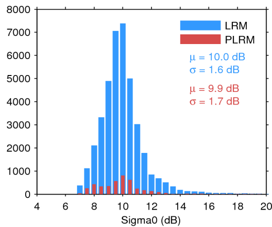
Figure 28. Histogram of science-valid sigma0 over oceans and lakes for LRM (blue) and PLRM (red) for 06/01/2016. The mean ( \mu ) and standard deviation ( \sigma ) are also shown. Note that values outside [4 20] dB are excluded from the histogram for the sake of readability but not from the computation of \mu and \sigma .
