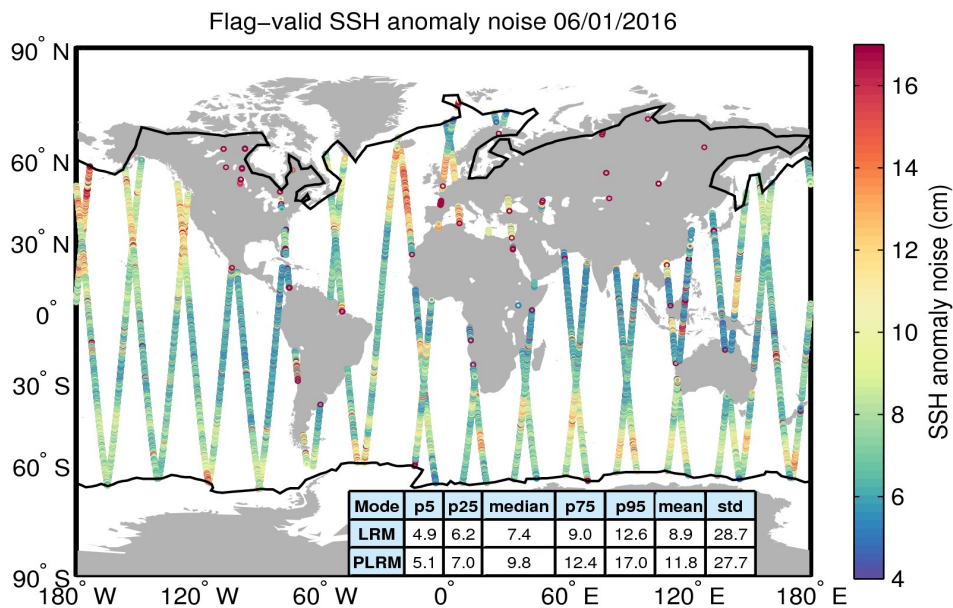
Figure 8. Geographical distribution of flag-valid 20-Hz SSH anomaly measurement noise over oceans and lakes for 06/01/2016. The statistical values shown in the table refer to the SSH anomaly noise and are calculated separately for LRM and PLRM regions. Measurements taken over polar polygons have been excluded from the computation of the statistical values. The black lines mark the outer limit of the Arctic and Antarctic polar polygons.
