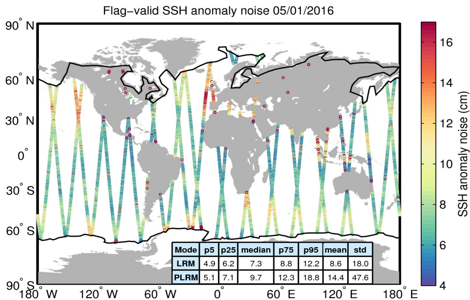
Figure 8. Geographical distribution of flag-valid 20-Hz SSH anomaly measurement noise over oceans and lakes for 05/01/2016. The statistical values shown in the table refer to the SSH anomaly noise and are calculated separately for LRM and PLRM regions. Measurements taken over polar polygons have been excluded from the computation of the statistical values. The black lines mark the outer limit of the Arctic and Antarctic polar polygons.
