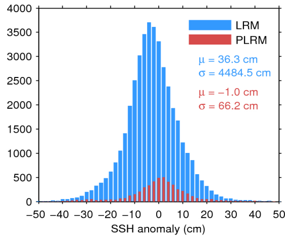
Figure 7. Histogram of flag-valid SSH anomaly over oceans and lakes for LRM (blue) and PLRM (red) for 05/01/2016. The mean ( \mu ) and standard deviation ( \sigma ) are also shown. Note that values outside [-50\ 50] cm are excluded from the histogram for the sake of readability but not from the computation of \mu and \sigma .
