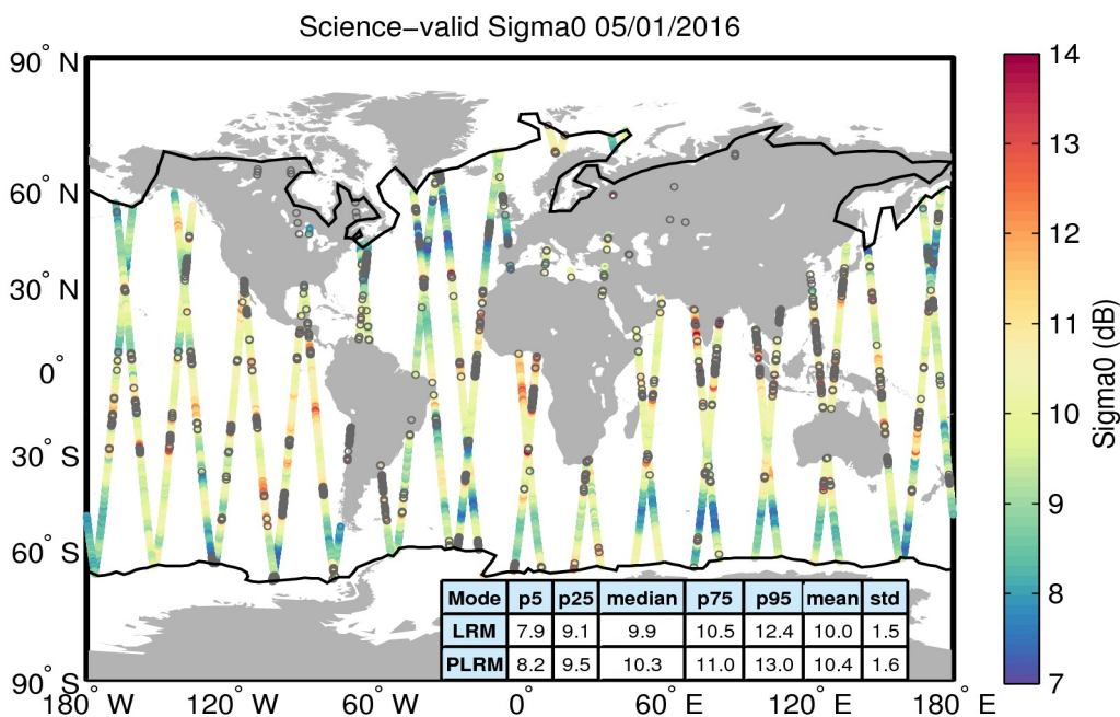
Figure 27. Geographical distribution of science-valid sigma0 data over oceans and lakes for 05/01/2016. The statistical values shown in the table refer to the sigma0 in dB and are calculated separately for LRM and PLRM regions. The black lines mark the outer limit of the Arctic and Antarctic polar polygons. Gray circles denote records that have been rejected based on the editing criteria described in Table 4.
