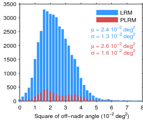
Figure 39. Histogram of flag-valid mispointing over oceans and lakes for LRM (blue) and PLRM (red) for 05/01/2016. Only positive values have been considered. The mean ( \mu ) and standard deviation ( \sigma ) are also shown. Note that values larger than 8 \cdot 10^{-2} \text{ deg}^2 are excluded from the histogram for the sake of readability but not from the computation of \mu and \sigma .
