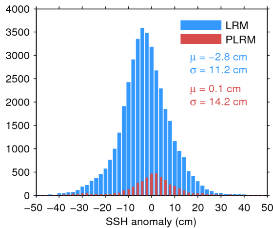
Figure 11. Histogram of science-valid SSH anomaly over oceans and lakes for LRM (blue) and PLRM (red) for 05/01/2016. The mean ( \mu ) and standard deviation ( \sigma ) are also shown. Note that values outside [-50 50] cm are excluded from the histogram for the sake of readability but not from the computation of \mu and \sigma .
