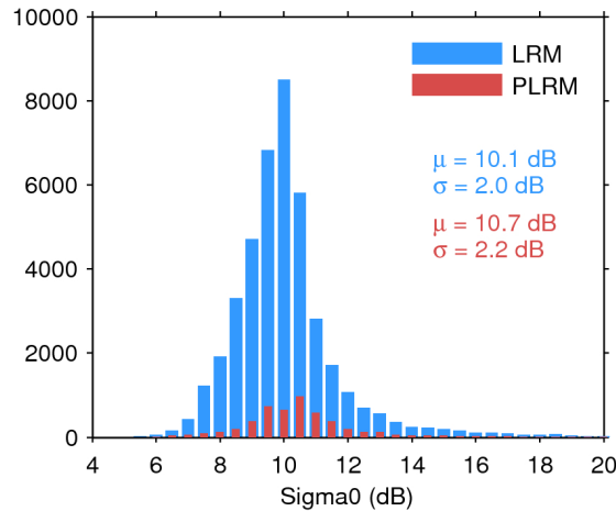
Figure 25. Histogram of flag-valid sigma0 over oceans and lakes for LRM (blue) and PLRM (red) for 05/01/2016. The mean ( \mu ) and standard deviation ( \sigma ) are also shown. Note that values outside [4 20] dB are excluded from the histogram for the sake of readability but not from the computation of \mu and \sigma .
