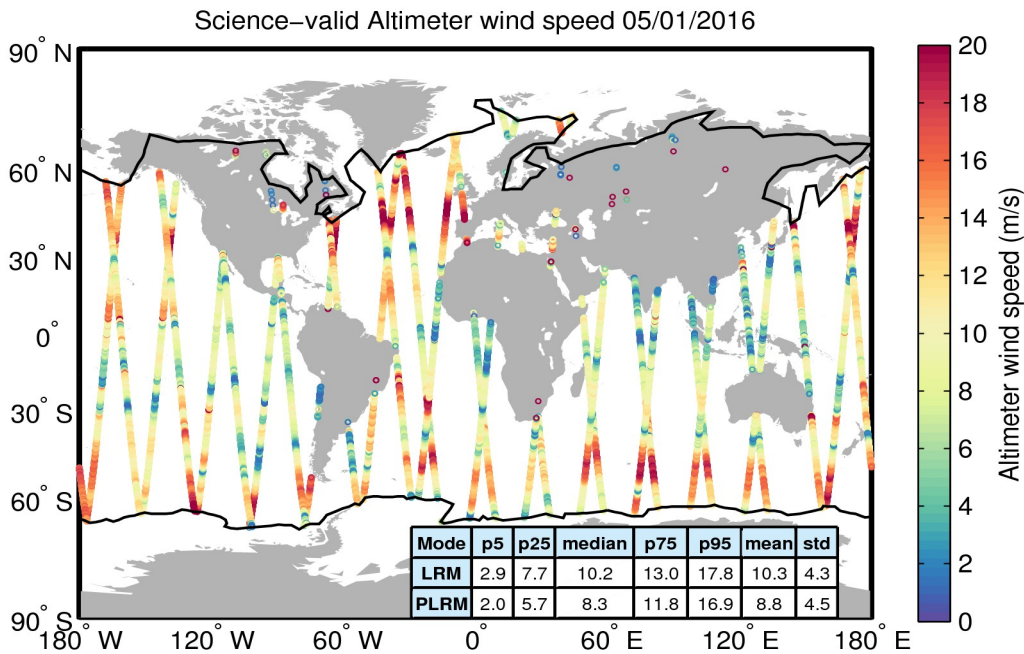
Figure 34. Geographical distribution of science-valid wind data over oceans and lakes for 05/01/2016. The statistical values shown in the table refer to the wind in m/s and are calculated separately for LRM and PLRM regions. The black lines mark the outer limit of the Arctic and Antarctic polar polygons. Gray circles denote records that have been rejected based on the editing criteria described in Table 5.
