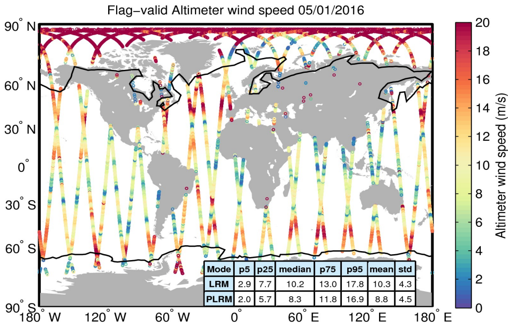
Figure 31. Geographical distribution of flag-valid wind data over oceans and lakes for 05/01/2016. The statistical values shown in the table refer to the wind in m/s and are calculated separately for LRM and PLRM regions. Measurements taken over polar polygons have been excluded from the computation of the statistical values. The black lines mark the outer limit of the Arctic and Antarctic polar polygons.
