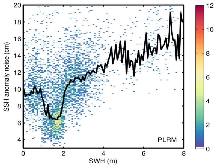
Figure 9. 2D histogram showing flag-valid SSH anomaly noise as a function of SWH for LRM (top) and PLRM (bottom) for 05/01/2016. The black line denotes the median SSH anomaly noise as a function of SWH.
