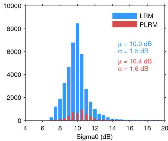
Figure 28. Histogram of science-valid sigma0 over oceans and lakes for LRM (blue) and PLRM (red) for 05/01/2016. The mean ( \mu ) and standard deviation ( \sigma ) are also shown. Note that values outside [4 20] dB are excluded from the histogram for the sake of readability but not from the computation of \mu and \sigma .
