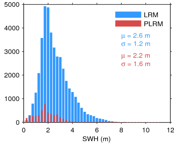
Figure 17. Histogram of flag-valid SWH over oceans and lakes for LRM (blue) and PLRM (red) for 05/01/2016. The mean ( \mu ) and standard deviation ( \sigma ) are also shown. Note that values larger than 12 m are excluded from the histogram for the sake of readability but not from the computation of \mu and \sigma .
