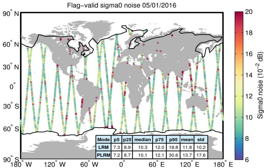
Figure 26. Geographical distribution of flag-valid 20-Hz sigma0 measurement noise over oceans and lakes for 05/01/2016. The statistical values shown in the table refer to the sigma0 noise and are calculated separately for LRM and PLRM regions. Measurements taken over polar polygons have been excluded from the computation of the statistical values. The black lines mark the outer limit of the Arctic and Antarctic polar polygons.
