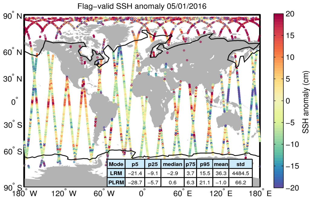
Figure 5. Geographical distribution of flag-valid 1-Hz SSH anomaly data over oceans and lakes for 05/01/2016. The statistical values shown in the table refer to the SSH anomaly in cm and are calculated separately for LRM and PLRM regions. Measurements taken over polar polygons have been excluded from the computation of the statistical values. The black lines mark the outer limit of the Arctic and Antarctic polar polygons.
