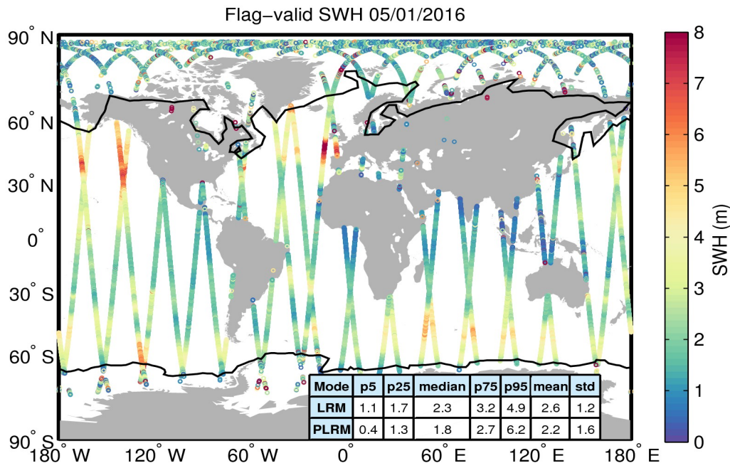
Figure 15. Geographical distribution of flag-valid SWH data over oceans and lakes for 05/01/2016. The statistical values shown in the table refer to the SWH in m and are calculated separately for LRM and PLRM regions. Measurements taken over polar polygons have been excluded from the computation of the statistical values. The black lines mark the outer limit of the Arctic and Antarctic polar polygons.
