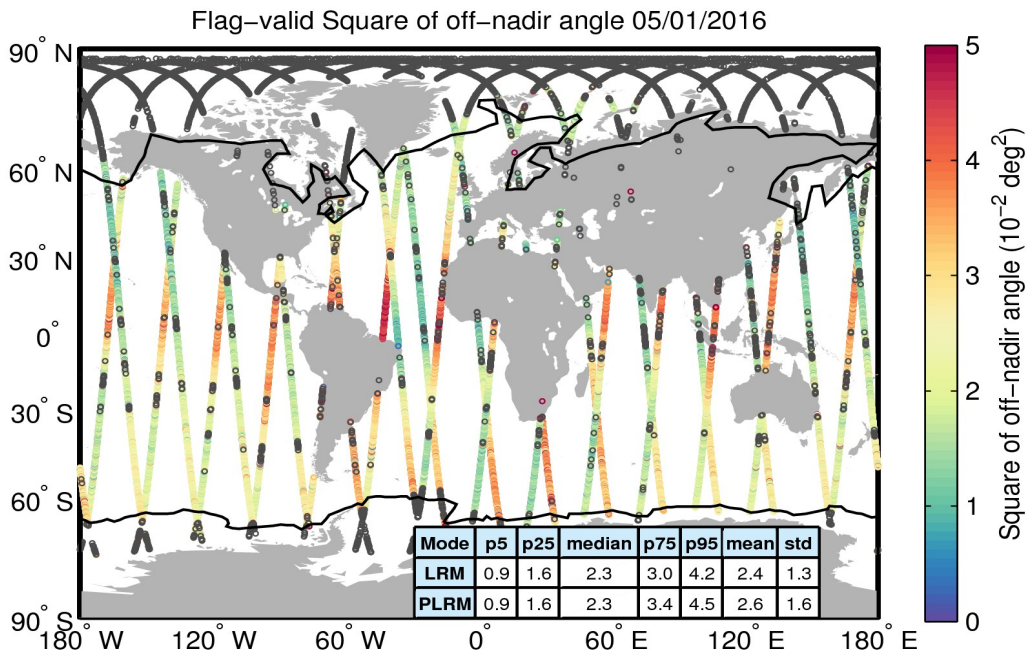
Figure 37. Geographical distribution of flag-valid mispointing data over oceans and lakes for 05/01/2016. The statistical values shown in the table refer to the mispointing in 10^{-2} deg 2 and are calculated separately for LRM and PLRM regions. Measurements taken over polar polygons have been excluded from the computation of the statistical values. The black lines mark the outer limit of the Arctic and Antarctic polar polygons. Gray circles denote negative values.
