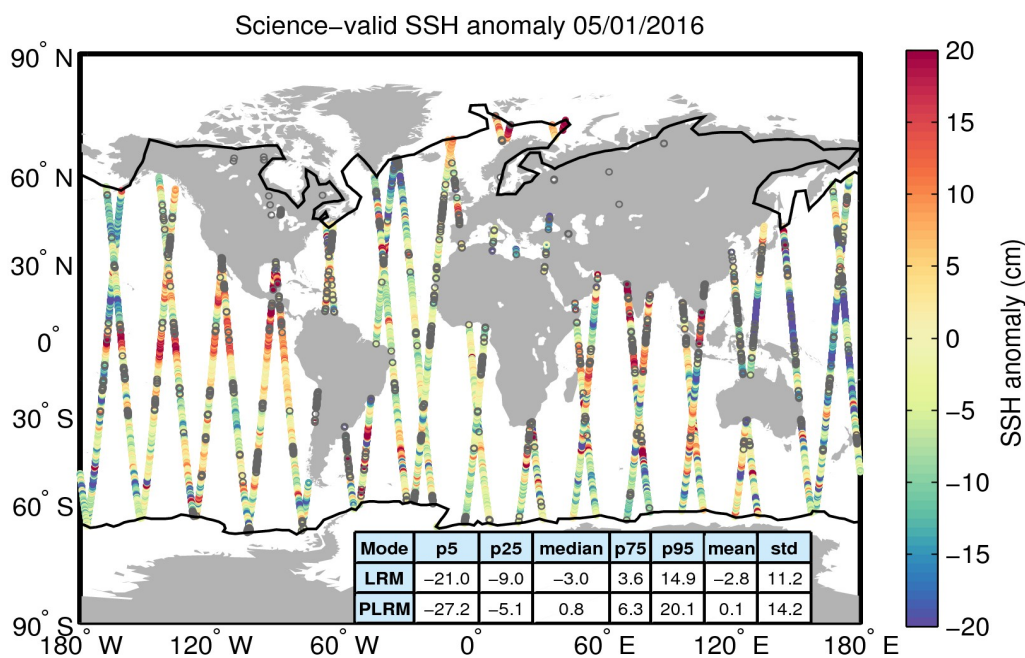
Figure 10. Geographical distribution of science-valid SSH anomaly data over oceans and lakes for 05/01/2016. The statistical values shown in the table refer to the SSH anomaly in cm and are calculated separately for LRM and PLRM regions. The black lines mark the outer limit of the Arctic and Antarctic polar polygons. Gray circles denote records that have been rejected based on the editing criteria described in Table 2.
