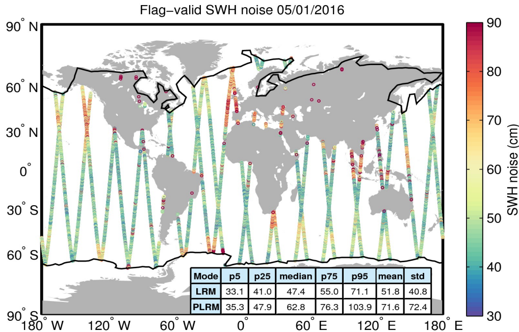
Figure 18. Geographical distribution of flag-valid 20-Hz SWH measurement noise over oceans and lakes for 05/01/2016. The statistical values shown in the table refer to the SWH noise and are calculated separately for LRM and PLRM regions. Measurements taken over polar polygons have been excluded from the computation of the statistical values. The black lines mark the outer limit of the Arctic and Antarctic polar polygons.
