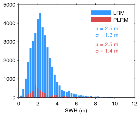
Figure 20. Histogram of science-valid SWH over oceans and lakes for LRM (blue) and PLRM (red) for 04/01/2016. The mean ( \mu ) and standard deviation ( \sigma ) are also shown. Note that values larger than 12 m are excluded from the histogram for the sake of readability but not from the computation of \mu and \sigma .
