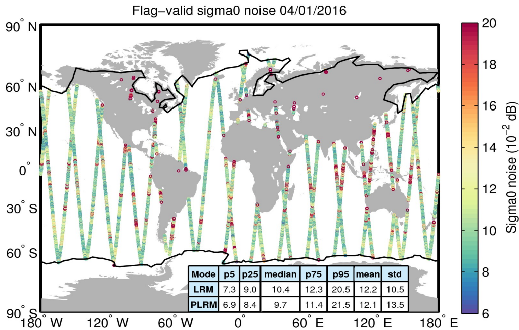
Figure 26. Geographical distribution of flag-valid 20-Hz sigma0 measurement noise over oceans and lakes for 04/01/2016. The statistical values shown in the table refer to the sigma0 noise and are calculated separately for LRM and PLRM regions. Measurements taken over polar polygons have been excluded from the computation of the statistical values. The black lines mark the outer limit of the Arctic and Antarctic polar polygons.
