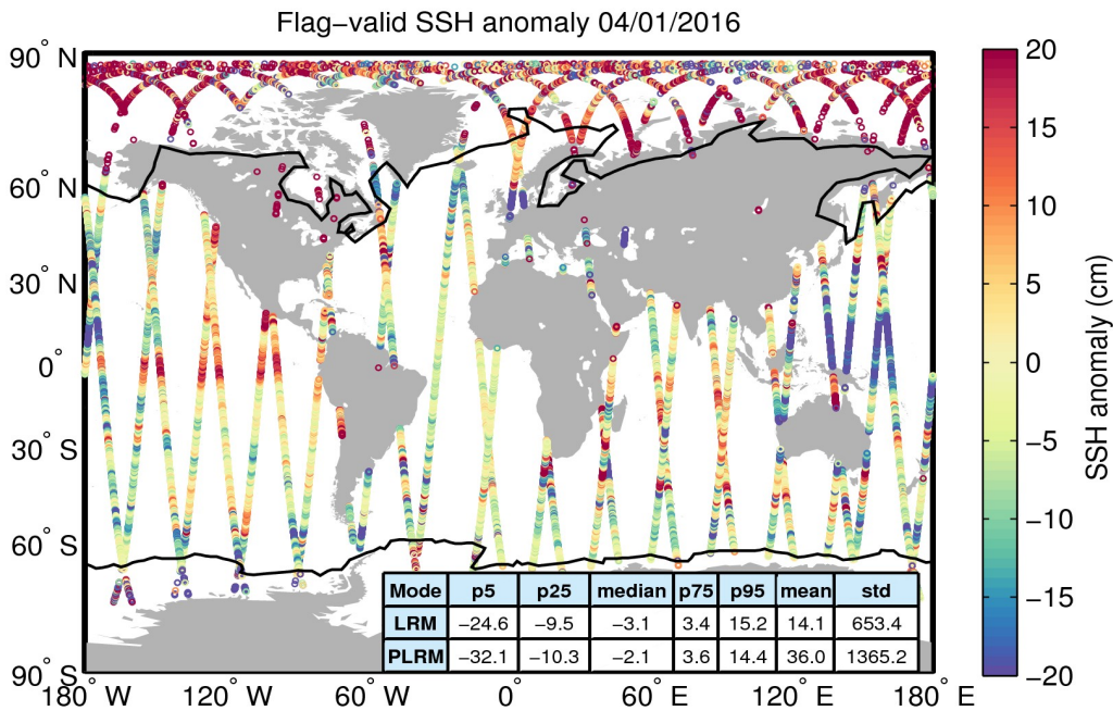
Figure 5. Geographical distribution of flag-valid 1-Hz SSH anomaly data over oceans and lakes for 04/01/2016. The statistical values shown in the table refer to the SSH anomaly in cm and are calculated separately for LRM and PLRM regions. Measurements taken over polar polygons have been excluded from the computation of the statistical values. The black lines mark the outer limit of the Arctic and Antarctic polar polygons.
