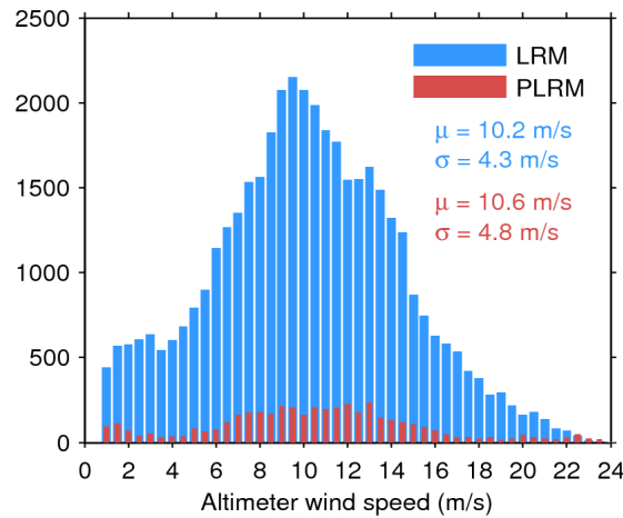
Figure 33. Histogram of flag-valid wind over oceans and lakes for LRM (blue) and PLRM (red) for 04/01/2016. The mean ( \mu ) and standard deviation ( \sigma ) are also shown. Note that values larger than 24 m/s are excluded from the histogram for the sake of readability but not from the computation of \mu and \sigma .
