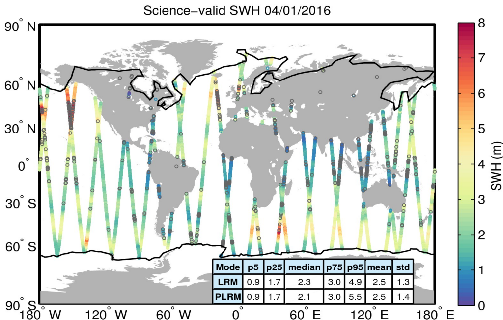
Figure 19. Geographical distribution of science-valid SWH data over oceans and lakes for 04/01/2016. The statistical values shown in the table refer to the SWH in m and are calculated separately for LRM and PLRM regions. The black lines mark the outer limit of the Arctic and Antarctic polar polygons. Gray circles denote records that have been rejected based on the editing criteria described in Table 3.
