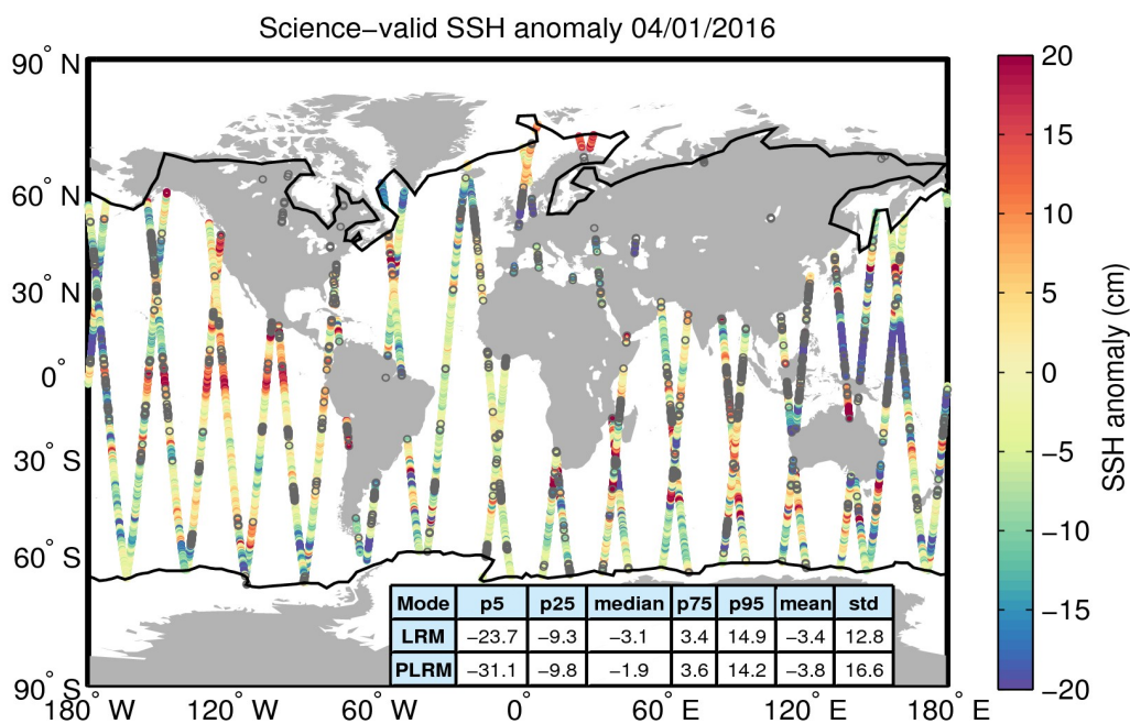
Figure 10. Geographical distribution of science-valid SSH anomaly data over oceans and lakes for 04/01/2016. The statistical values shown in the table refer to the SSH anomaly in cm and are calculated separately for LRM and PLRM regions. The black lines mark the outer limit of the Arctic and Antarctic polar polygons. Gray circles denote records that have been rejected based on the editing criteria described in Table 2.
