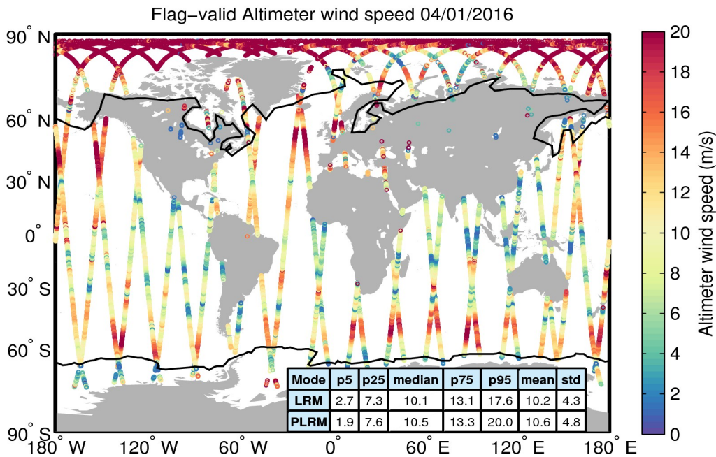
Figure 31. Geographical distribution of flag-valid wind data over oceans and lakes for 04/01/2016. The statistical values shown in the table refer to the wind in m/s and are calculated separately for LRM and PLRM regions. Measurements taken over polar polygons have been excluded from the computation of the statistical values. The black lines mark the outer limit of the Arctic and Antarctic polar polygons.
