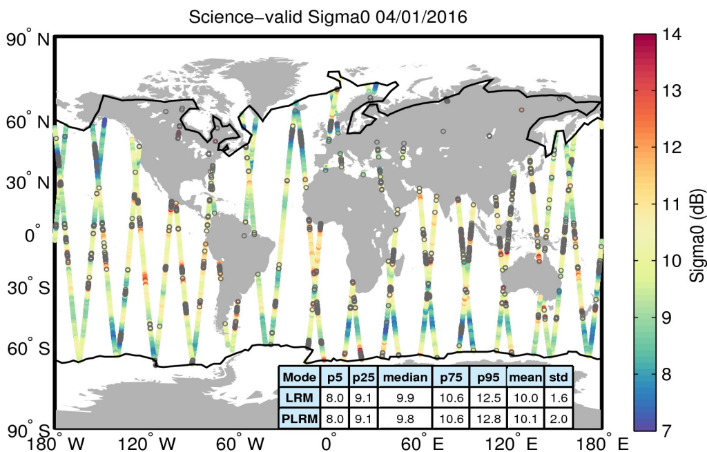
Figure 27. Geographical distribution of science-valid sigma0 data over oceans and lakes for 04/01/2016. The statistical values shown in the table refer to the sigma0 in dB and are calculated separately for LRM and PLRM regions. The black lines mark the outer limit of the Arctic and Antarctic polar polygons. Gray circles denote records that have been rejected based on the editing criteria described in Table 4.
