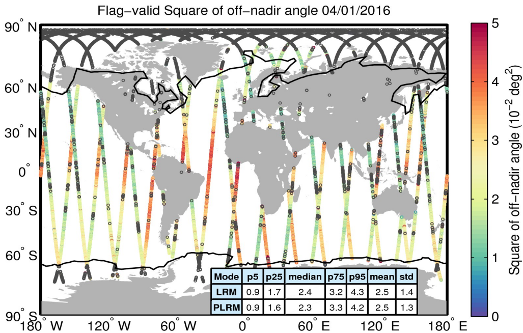
Figure 37. Geographical distribution of flag-valid mispointing data over oceans and lakes for 04/01/2016. The statistical values shown in the table refer to the mispointing in 10^{-2} deg 2 and are calculated separately for LRM and PLRM regions. Measurements taken over polar polygons have been excluded from the computation of the statistical values. The black lines mark the outer limit of the Arctic and Antarctic polar polygons. Gray circles denote negative values.
