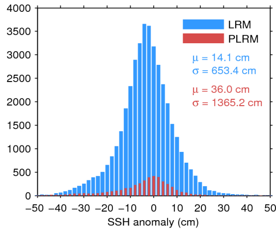
Figure 7. Histogram of flag-valid SSH anomaly over oceans and lakes for LRM (blue) and PLRM (red) for 04/01/2016. The mean ( \mu ) and standard deviation ( \sigma ) are also shown. Note that values outside [-50\ 50] cm are excluded from the histogram for the sake of readability but not from the computation of \mu and \sigma .
