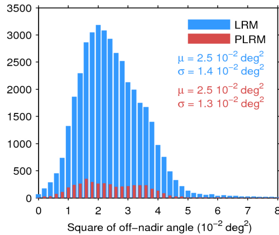
Figure 39. Histogram of flag-valid mispointing over oceans and lakes for LRM (blue) and PLRM (red) for 04/01/2016. Only positive values have been considered. The mean ( \mu ) and standard deviation ( \sigma ) are also shown. Note that values larger than 8 \cdot 10^{-2} \text{ deg}^2 are excluded from the histogram for the sake of readability but not from the computation of \mu and \sigma .
