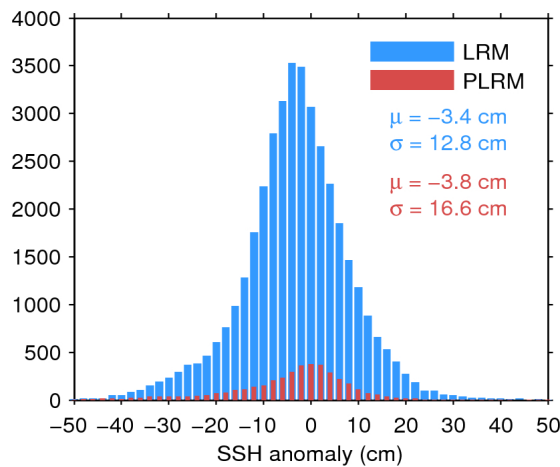
Figure 11. Histogram of science-valid SSH anomaly over oceans and lakes for LRM (blue) and PLRM (red) for 04/01/2016. The mean ( \mu ) and standard deviation ( \sigma ) are also shown. Note that values outside [-50\ 50] cm are excluded from the histogram for the sake of readability but not from the computation of \mu and \sigma .
