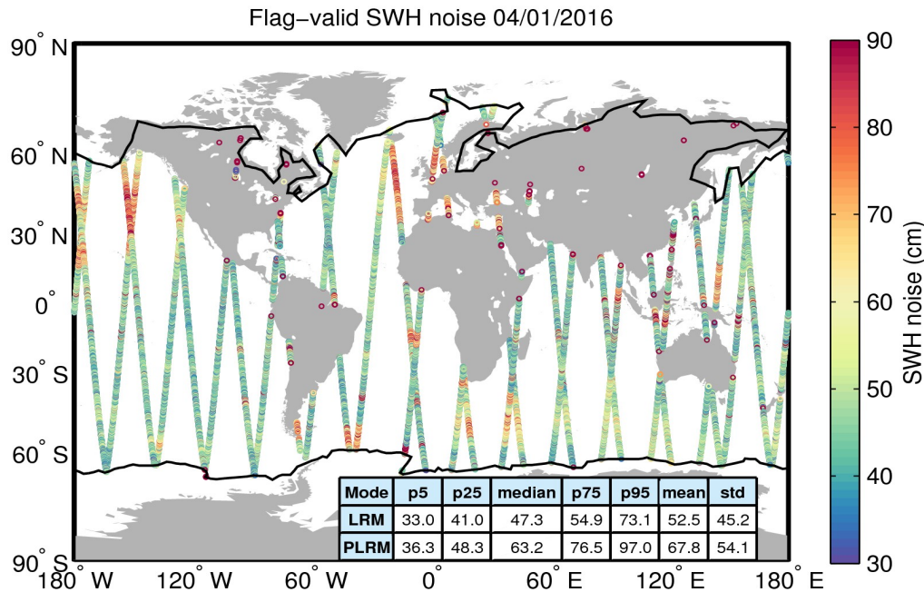
Figure 18. Geographical distribution of flag-valid 20-Hz SWH measurement noise over oceans and lakes for 04/01/2016. The statistical values shown in the table refer to the SWH noise and are calculated separately for LRM and PLRM regions. Measurements taken over polar polygons have been excluded from the computation of the statistical values. The black lines mark the outer limit of the Arctic and Antarctic polar polygons.
