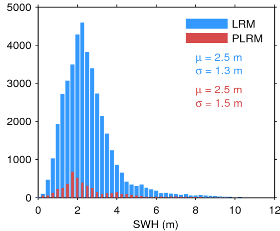
Figure 17. Histogram of flag-valid SWH over oceans and lakes for LRM (blue) and PLRM (red) for 04/01/2016. The mean ( \mu ) and standard deviation ( \sigma ) are also shown. Note that values larger than 12 m are excluded from the histogram for the sake of readability but not from the computation of \mu and \sigma .
