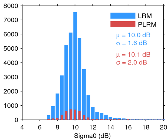
Figure 28. Histogram of science-valid sigma0 over oceans and lakes for LRM (blue) and PLRM (red) for 04/01/2016. The mean ( \mu ) and standard deviation ( \sigma ) are also shown. Note that values outside [4 20] dB are excluded from the histogram for the sake of readability but not from the computation of \mu and \sigma .
