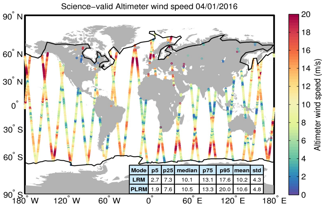
Figure 34. Geographical distribution of science-valid wind data over oceans and lakes for 04/01/2016. The statistical values shown in the table refer to the wind in m/s and are calculated separately for LRM and PLRM regions. The black lines mark the outer limit of the Arctic and Antarctic polar polygons. Gray circles denote records that have been rejected based on the editing criteria described in Table 5.
