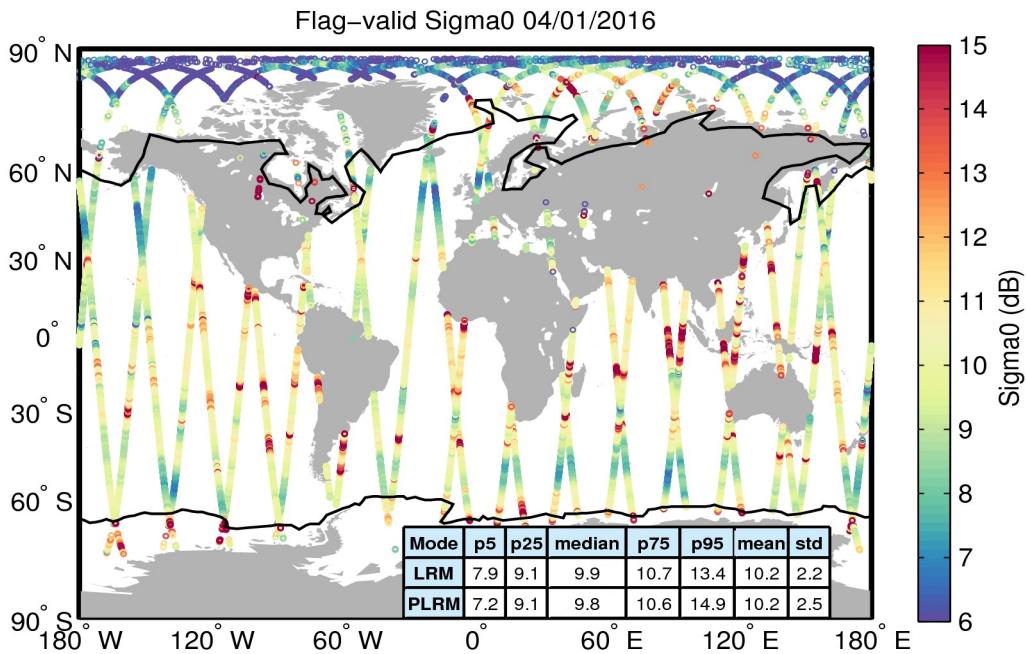
Figure 23. Geographical distribution of flag-valid sigma0 data over oceans and lakes for 04/01/2016. The statistical values shown in the table refer to the sigma0 in dB and are calculated separately for LRM and PLRM regions. Measurements taken over polar polygons have been excluded from the computation of the statistical values. The black lines mark the outer limit of the Arctic and Antarctic polar polygons.
