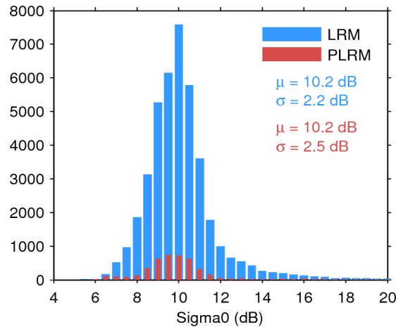
Figure 25. Histogram of flag-valid sigma0 over oceans and lakes for LRM (blue) and PLRM (red) for 04/01/2016. The mean ( \mu ) and standard deviation ( \sigma ) are also shown. Note that values outside [4 20] dB are excluded from the histogram for the sake of readability but not from the computation of \mu and \sigma .
