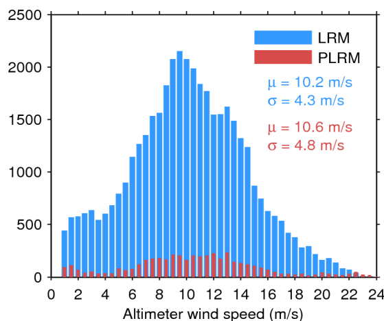
Figure 35. Histogram of science-valid wind over oceans and lakes for LRM (blue) and PLRM (red) for 04/01/2016. The mean ( \mu ) and standard deviation ( \sigma ) are also shown. Note that values larger than 24 m/s are excluded from the histogram for the sake of readability but not from the computation of \mu and \sigma .
