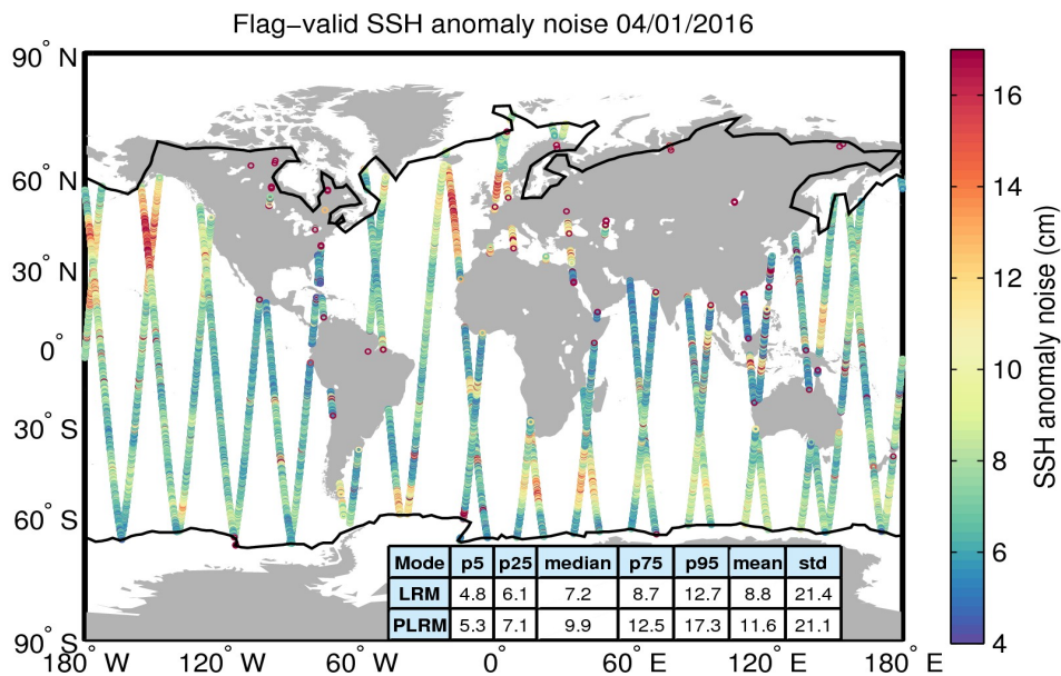
Figure 8. Geographical distribution of flag-valid 20-Hz SSH anomaly measurement noise over oceans and lakes for 04/01/2016. The statistical values shown in the table refer to the SSH anomaly noise and are calculated separately for LRM and PLRM regions. Measurements taken over polar polygons have been excluded from the computation of the statistical values. The black lines mark the outer limit of the Arctic and Antarctic polar polygons.
