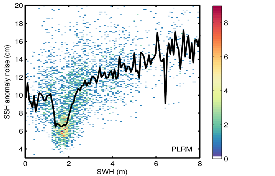
Figure 9. 2D histogram showing flag-valid SSH anomaly noise as a function of SWH for LRM (top) and PLRM (bottom) for 04/01/2016. The black line denotes the median SSH anomaly noise as a function of SWH.
