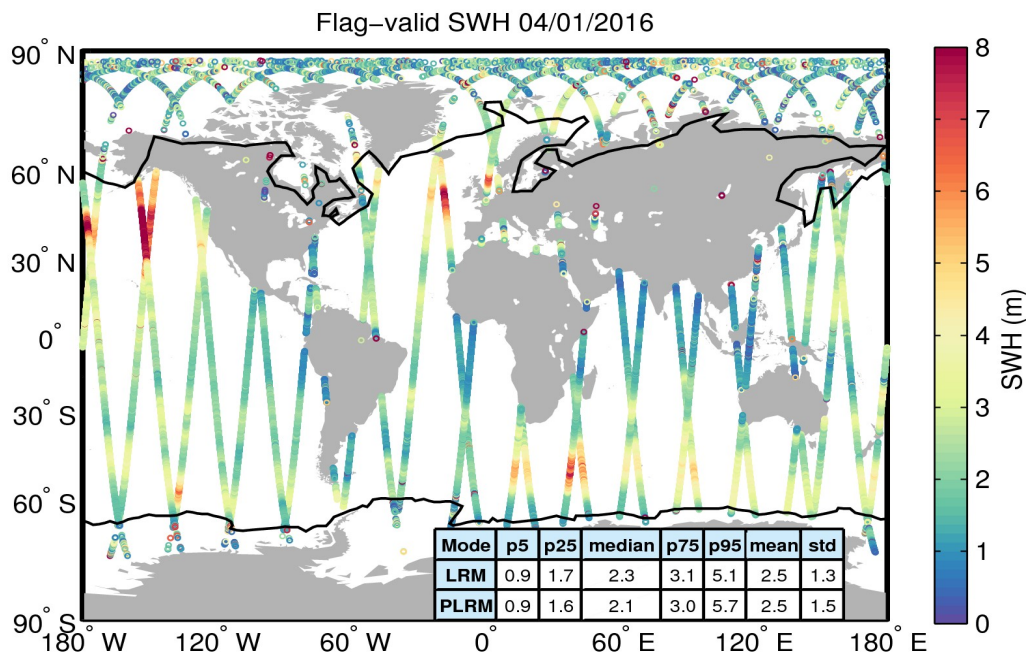
Figure 15. Geographical distribution of flag-valid SWH data over oceans and lakes for 04/01/2016. The statistical values shown in the table refer to the SWH in m and are calculated separately for LRM and PLRM regions. Measurements taken over polar polygons have been excluded from the computation of the statistical values. The black lines mark the outer limit of the Arctic and Antarctic polar polygons.
