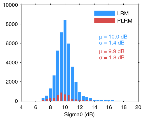
Figure 28. Histogram of science-valid sigma0 over oceans and lakes for LRM (blue) and PLRM (red) for 03/01/2016. The mean ( \mu ) and standard deviation ( \sigma ) are also shown. Note that values outside [4 20] dB are excluded from the histogram for the sake of readability but not from the computation of \mu and \sigma .
