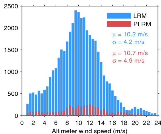
Figure 35. Histogram of science-valid wind over oceans and lakes for LRM (blue) and PLRM (red) for 03/01/2016. The mean ( \mu ) and standard deviation ( \sigma ) are also shown. Note that values larger than 24 m/s are excluded from the histogram for the sake of readability but not from the computation of \mu and \sigma .
