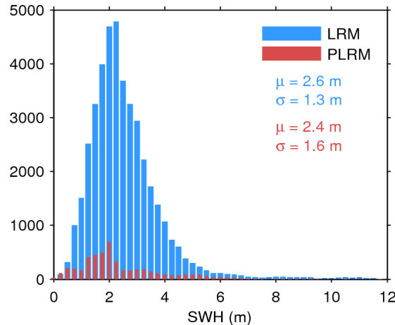
Figure 17. Histogram of flag-valid SWH over oceans and lakes for LRM (blue) and PLRM (red) for 03/01/2016. The mean ( \mu ) and standard deviation ( \sigma ) are also shown. Note that values larger than 12 m are excluded from the histogram for the sake of readability but not from the computation of \mu and \sigma .
