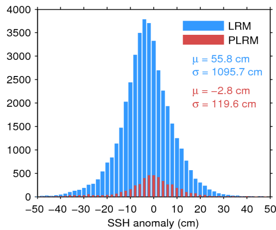
Figure 7. Histogram of flag-valid SSH anomaly over oceans and lakes for LRM (blue) and PLRM (red) for 03/01/2016. The mean ( \mu ) and standard deviation ( \sigma ) are also shown. Note that values outside [-50 \ 50] cm are excluded from the histogram for the sake of readability but not from the computation of \mu and \sigma .
