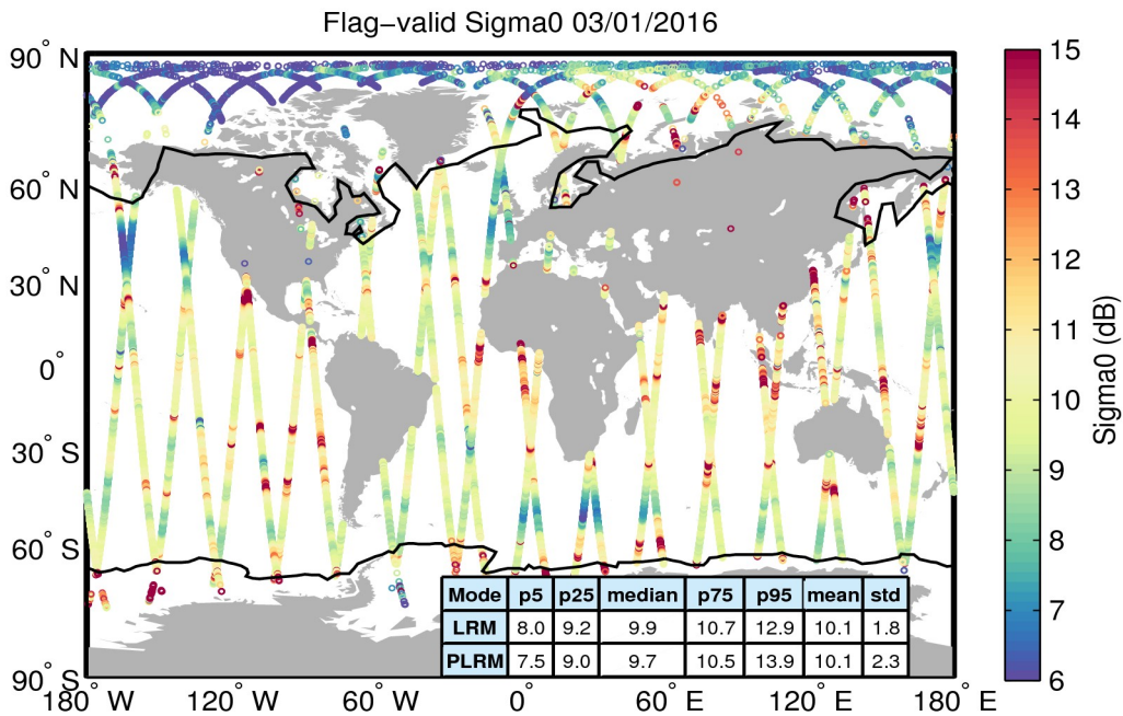
Figure 23. Geographical distribution of flag-valid sigma0 data over oceans and lakes for 03/01/2016. The statistical values shown in the table refer to the sigma0 in dB and are calculated separately for LRM and PLRM regions. Measurements taken over polar polygons have been excluded from the computation of the statistical values. The black lines mark the outer limit of the Arctic and Antarctic polar polygons.
