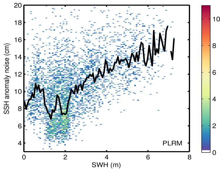
Figure 9. 2D histogram showing flag-valid SSH anomaly noise as a function of SWH for LRM (top) and PLRM (bottom) for 03/01/2016. The black line denotes the median SSH anomaly noise as a function of SWH.
