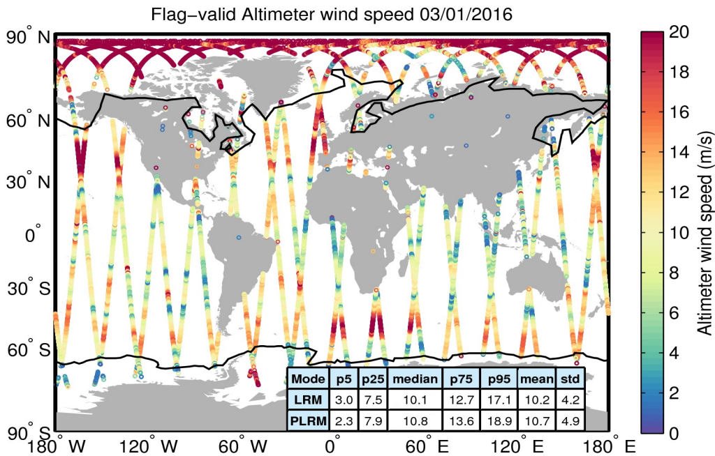
Figure 31. Geographical distribution of flag-valid wind data over oceans and lakes for 03/01/2016. The statistical values shown in the table refer to the wind in m/s and are calculated separately for LRM and PLRM regions. Measurements taken over polar polygons have been excluded from the computation of the statistical values. The black lines mark the outer limit of the Arctic and Antarctic polar polygons.
