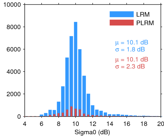
Figure 25. Histogram of flag-valid sigma0 over oceans and lakes for LRM (blue) and PLRM (red) for 03/01/2016. The mean ( \mu ) and standard deviation ( \sigma ) are also shown. Note that values outside [4 20] dB are excluded from the histogram for the sake of readability but not from the computation of \mu and \sigma .
