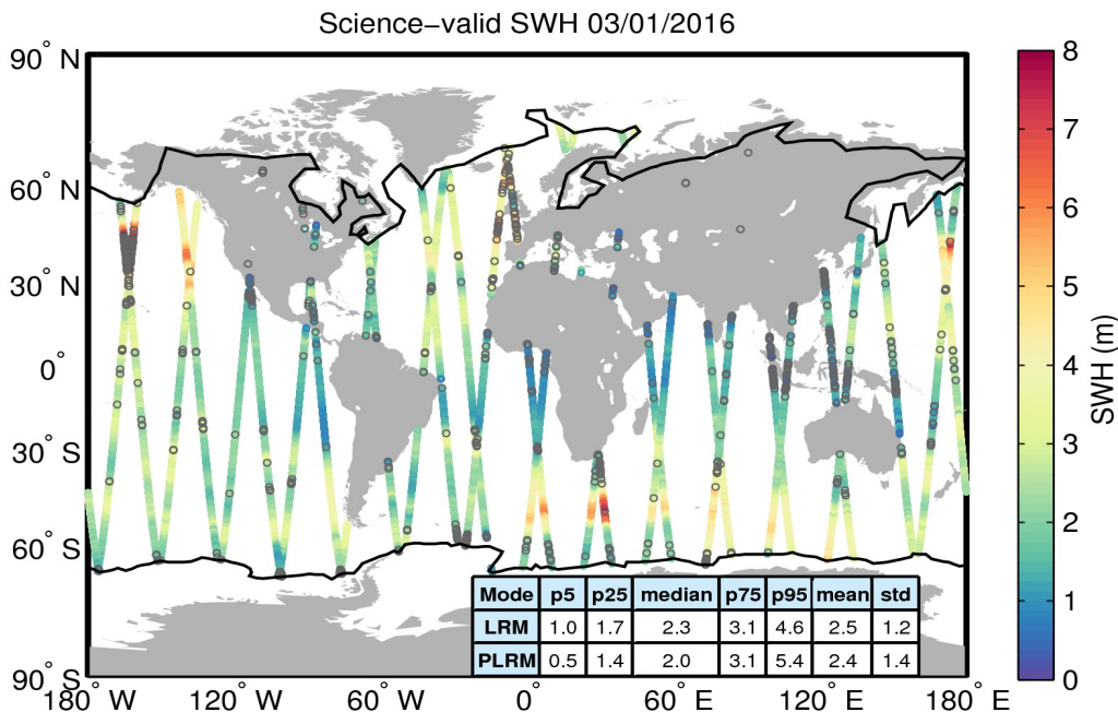
Figure 19. Geographical distribution of science-valid SWH data over oceans and lakes for 03/01/2016. The statistical values shown in the table refer to the SWH in m and are calculated separately for LRM and PLRM regions. The black lines mark the outer limit of the Arctic and Antarctic polar polygons. Gray circles denote records that have been rejected based on the editing criteria described in Table 3.
