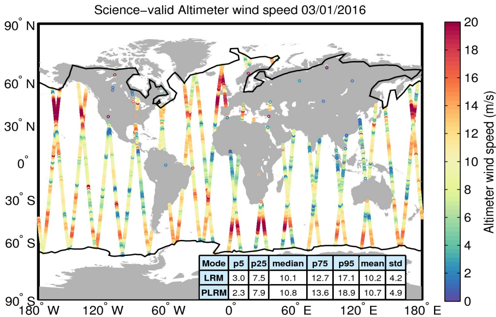
Figure 34. Geographical distribution of science-valid wind data over oceans and lakes for 03/01/2016. The statistical values shown in the table refer to the wind in m/s and are calculated separately for LRM and PLRM regions. The black lines mark the outer limit of the Arctic and Antarctic polar polygons. Gray circles denote records that have been rejected based on the editing criteria described in Table 5.
