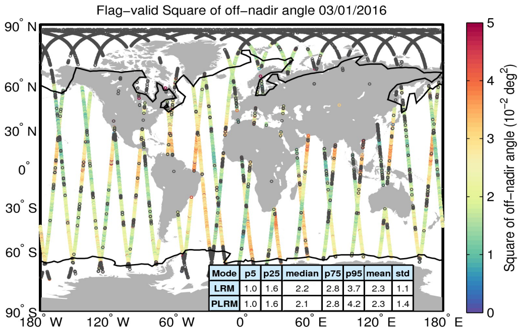
Figure 37. Geographical distribution of flag-valid mispointing data over oceans and lakes for 03/01/2016. The statistical values shown in the table refer to the mispointing in 10^{-2} deg 2 and are calculated separately for LRM and PLRM regions. Measurements taken over polar polygons have been excluded from the computation of the statistical values. The black lines mark the outer limit of the Arctic and Antarctic polar polygons. Gray circles denote negative values.
