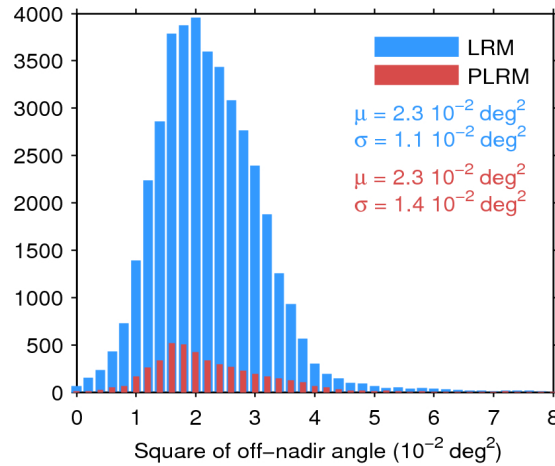
Figure 39. Histogram of flag-valid mispointing over oceans and lakes for LRM (blue) and PLRM (red) for 03/01/2016. Only positive values have been considered. The mean ( \mu ) and standard deviation ( \sigma ) are also shown. Note that values larger than 8 \cdot 10^{-2} \text{ deg}^2 are excluded from the histogram for the sake of readability but not from the computation of \mu and \sigma .
