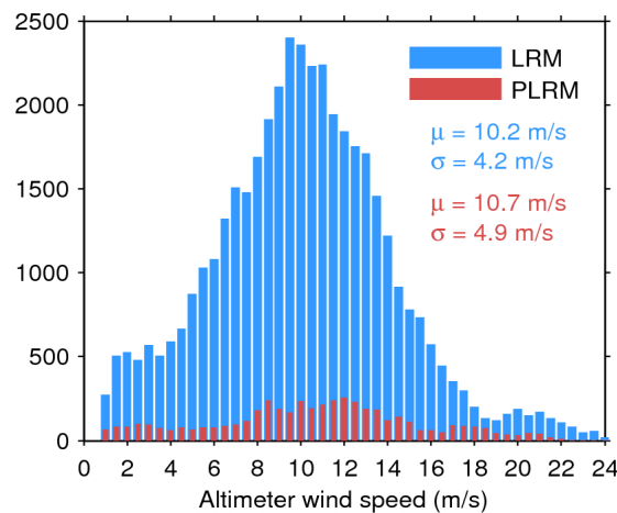
Figure 33. Histogram of flag-valid wind over oceans and lakes for LRM (blue) and PLRM (red) for 03/01/2016. The mean ( \mu ) and standard deviation ( \sigma ) are also shown. Note that values larger than 24 m/s are excluded from the histogram for the sake of readability but not from the computation of \mu and \sigma .
