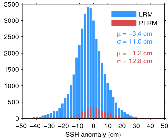
Figure 11. Histogram of science-valid SSH anomaly over oceans and lakes for LRM (blue) and PLRM (red) for 03/01/2016. The mean ( \mu ) and standard deviation ( \sigma ) are also shown. Note that values outside [-50\ 50] cm are excluded from the histogram for the sake of readability but not from the computation of \mu and \sigma .
