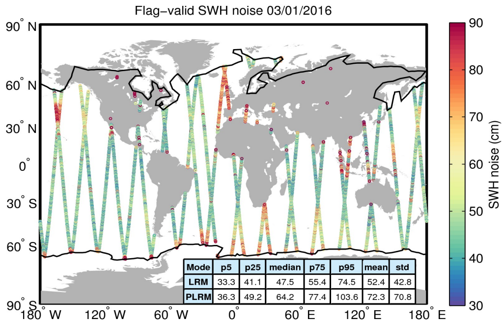
Figure 18. Geographical distribution of flag-valid 20-Hz SWH measurement noise over oceans and lakes for 03/01/2016. The statistical values shown in the table refer to the SWH noise and are calculated separately for LRM and PLRM regions. Measurements taken over polar polygons have been excluded from the computation of the statistical values. The black lines mark the outer limit of the Arctic and Antarctic polar polygons.
