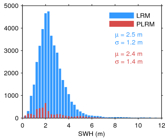
Figure 20. Histogram of science-valid SWH over oceans and lakes for LRM (blue) and PLRM (red) for 03/01/2016. The mean ( \mu ) and standard deviation ( \sigma ) are also shown. Note that values larger than 12 m are excluded from the histogram for the sake of readability but not from the computation of \mu and \sigma .
