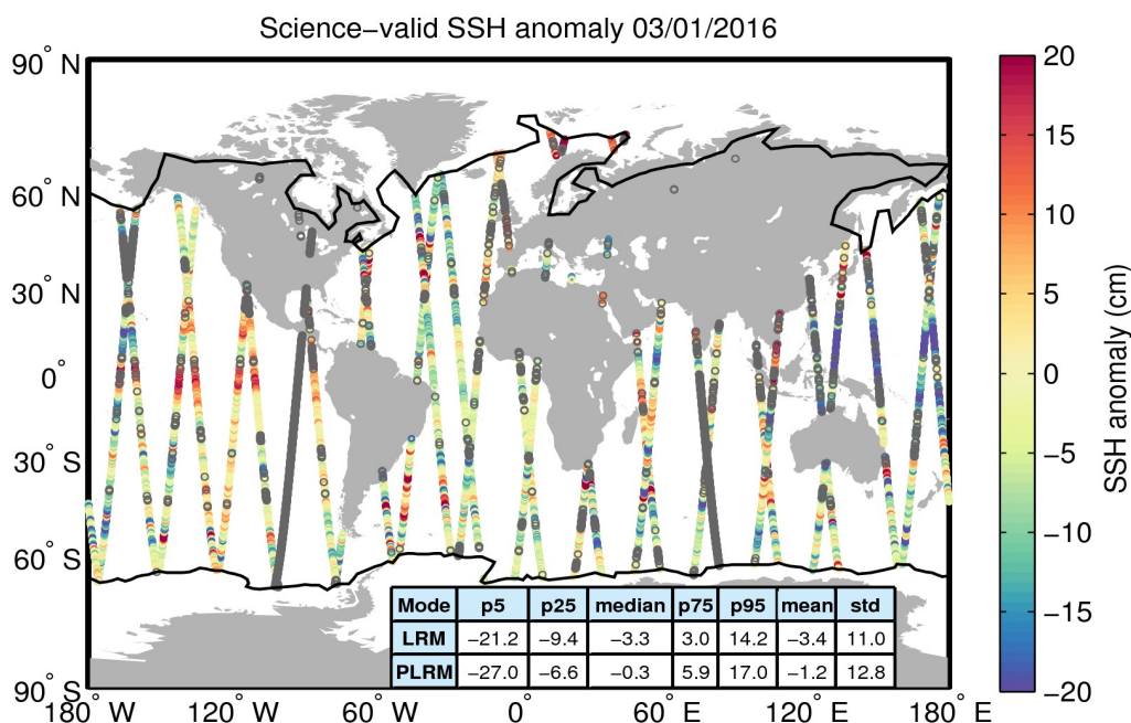
Figure 10. Geographical distribution of science-valid SSH anomaly data over oceans and lakes for 03/01/2016. The statistical values shown in the table refer to the SSH anomaly in cm and are calculated separately for LRM and PLRM regions. The black lines mark the outer limit of the Arctic and Antarctic polar polygons. Gray circles denote records that have been rejected based on the editing criteria described in Table 2.
