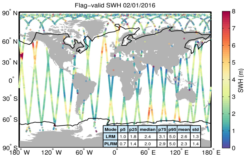
Figure 15. Geographical distribution of flag-valid SWH data over oceans and lakes for 02/01/2016. The statistical values shown in the table refer to the SWH in m and are calculated separately for LRM and PLRM regions. Measurements taken over polar polygons have been excluded from the computation of the statistical values. The black lines mark the outer limit of the Arctic and Antarctic polar polygons.
