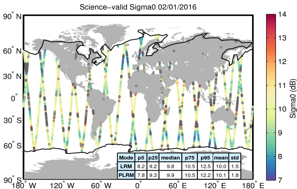
Figure 27. Geographical distribution of science-valid sigma0 data over oceans and lakes for 02/01/2016. The statistical values shown in the table refer to the sigma0 in dB and are calculated separately for LRM and PLRM regions. The black lines mark the outer limit of the Arctic and Antarctic polar polygons. Gray circles denote records that have been rejected based on the editing criteria described in Table 4.
