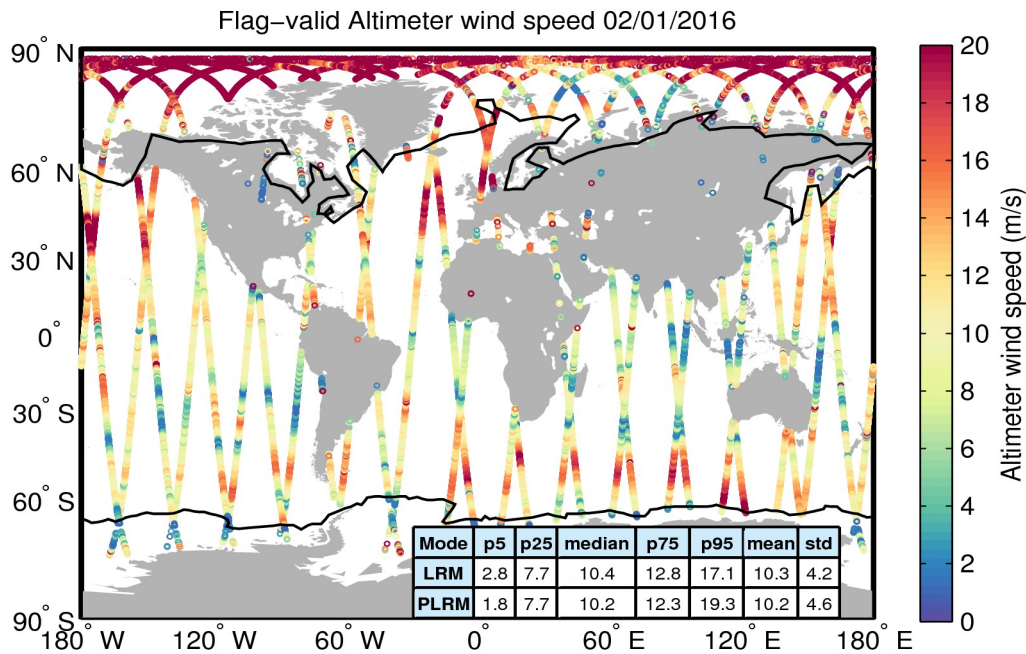
Figure 31. Geographical distribution of flag-valid wind data over oceans and lakes for 02/01/2016. The statistical values shown in the table refer to the wind in m/s and are calculated separately for LRM and PLRM regions. Measurements taken over polar polygons have been excluded from the computation of the statistical values. The black lines mark the outer limit of the Arctic and Antarctic polar polygons.
