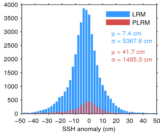
Figure 7. Histogram of flag-valid SSH anomaly over oceans and lakes for LRM (blue) and PLRM (red) for 02/01/2016. The mean ( \mu ) and standard deviation ( \sigma ) are also shown. Note that values outside [-50\ 50] cm are excluded from the histogram for the sake of readability but not from the computation of \mu and \sigma .
