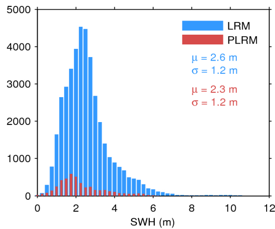
Figure 20. Histogram of science-valid SWH over oceans and lakes for LRM (blue) and PLRM (red) for 02/01/2016. The mean ( \mu ) and standard deviation ( \sigma ) are also shown. Note that values larger than 12 m are excluded from the histogram for the sake of readability but not from the computation of \mu and \sigma .
