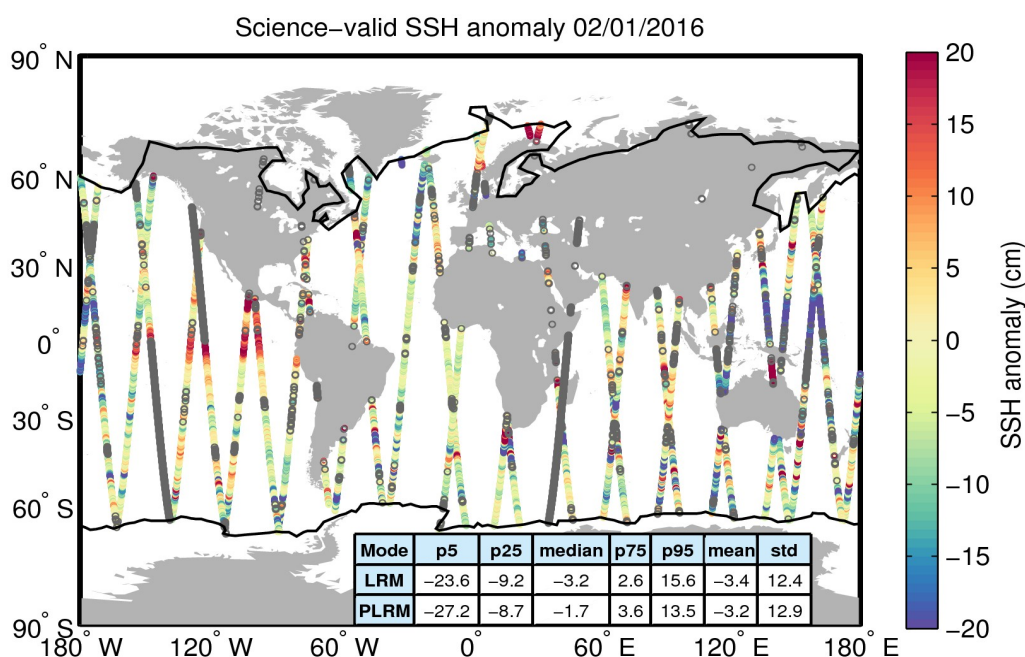
Figure 10. Geographical distribution of science-valid SSH anomaly data over oceans and lakes for 02/01/2016. The statistical values shown in the table refer to the SSH anomaly in cm and are calculated separately for LRM and PLRM regions. The black lines mark the outer limit of the Arctic and Antarctic polar polygons. Gray circles denote records that have been rejected based on the editing criteria described in Table 2.
