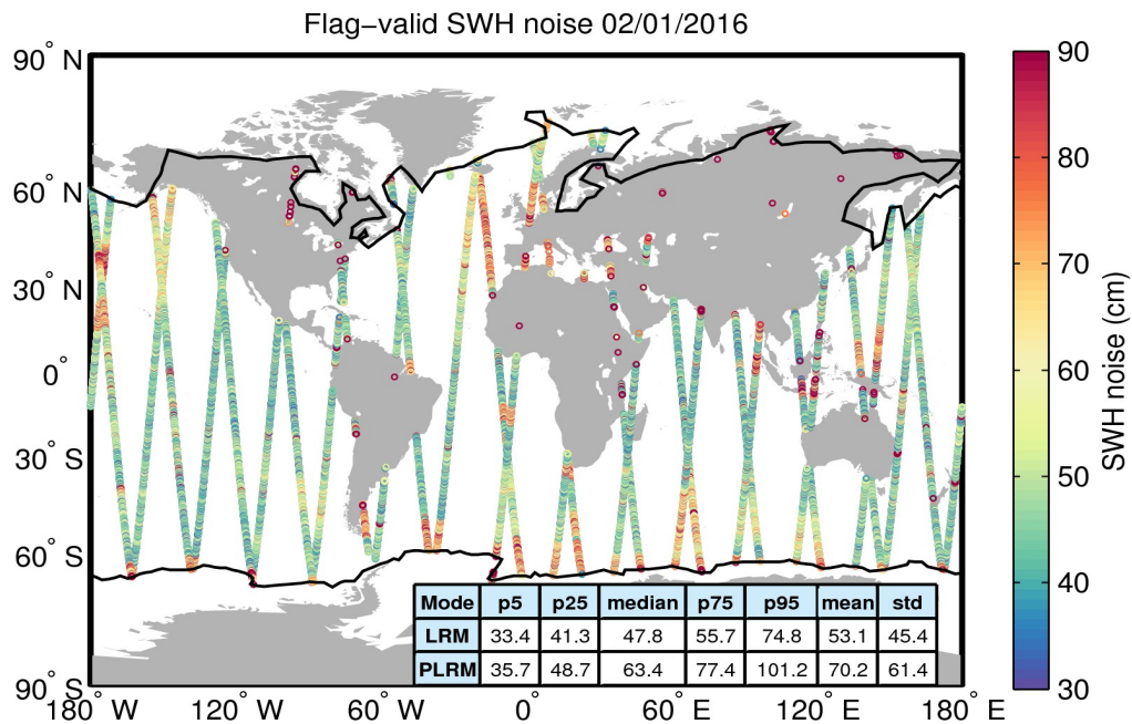
Figure 18. Geographical distribution of flag-valid 20-Hz SWH measurement noise over oceans and lakes for 02/01/2016. The statistical values shown in the table refer to the SWH noise and are calculated separately for LRM and PLRM regions. Measurements taken over polar polygons have been excluded from the computation of the statistical values. The black lines mark the outer limit of the Arctic and Antarctic polar polygons.
