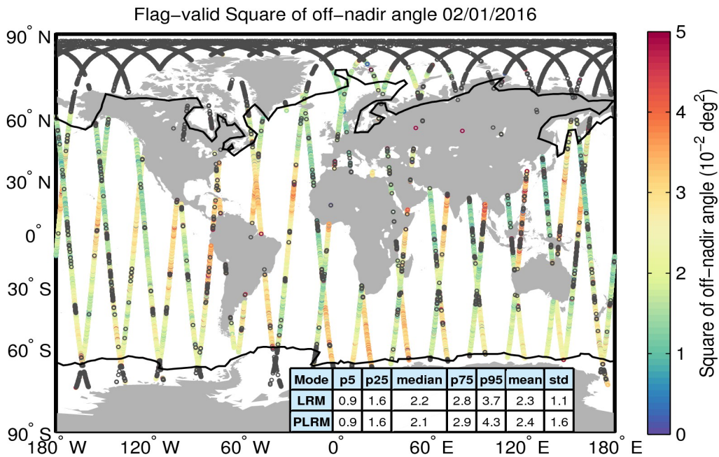
Figure 37. Geographical distribution of flag-valid mispointing data over oceans and lakes for 02/01/2016. The statistical values shown in the table refer to the mispointing in 10^{-2} deg 2 and are calculated separately for LRM and PLRM regions. Measurements taken over polar polygons have been excluded from the computation of the statistical values. The black lines mark the outer limit of the Arctic and Antarctic polar polygons. Gray circles denote negative values.
