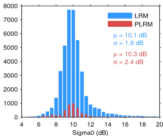
Figure 25. Histogram of flag-valid sigma0 over oceans and lakes for LRM (blue) and PLRM (red) for 02/01/2016. The mean ( \mu ) and standard deviation ( \sigma ) are also shown. Note that values outside [4 20] dB are excluded from the histogram for the sake of readability but not from the computation of \mu and \sigma .
