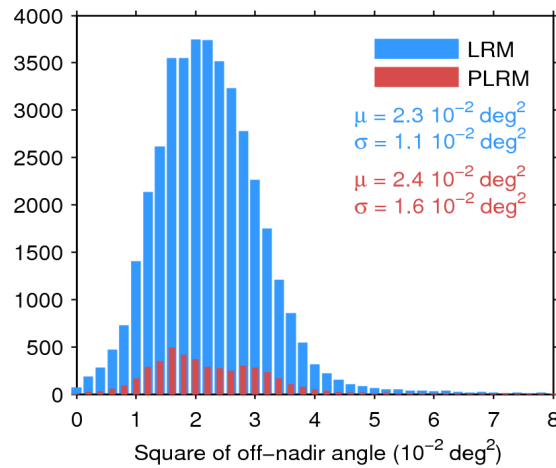
Figure 39. Histogram of flag-valid mispointing over oceans and lakes for LRM (blue) and PLRM (red) for 02/01/2016. Only positive values have been considered. The mean ( \mu ) and standard deviation ( \sigma ) are also shown. Note that values larger than 8 \cdot 10^{-2} \text{ deg}^2 are excluded from the histogram for the sake of readability but not from the computation of \mu and \sigma .
