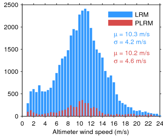
Figure 33. Histogram of flag-valid wind over oceans and lakes for LRM (blue) and PLRM (red) for 02/01/2016. The mean ( \mu ) and standard deviation ( \sigma ) are also shown. Note that values larger than 24 m/s are excluded from the histogram for the sake of readability but not from the computation of \mu and \sigma .
