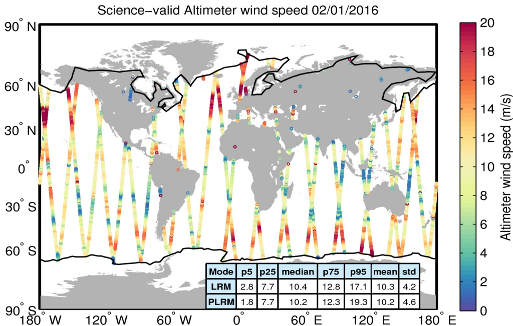
Figure 34. Geographical distribution of science-valid wind data over oceans and lakes for 02/01/2016. The statistical values shown in the table refer to the wind in m/s and are calculated separately for LRM and PLRM regions. The black lines mark the outer limit of the Arctic and Antarctic polar polygons. Gray circles denote records that have been rejected based on the editing criteria described in Table 5.
