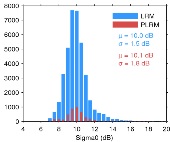
Figure 28. Histogram of science-valid sigma0 over oceans and lakes for LRM (blue) and PLRM (red) for 02/01/2016. The mean ( \mu ) and standard deviation ( \sigma ) are also shown. Note that values outside [4 20] dB are excluded from the histogram for the sake of readability but not from the computation of \mu and \sigma .
