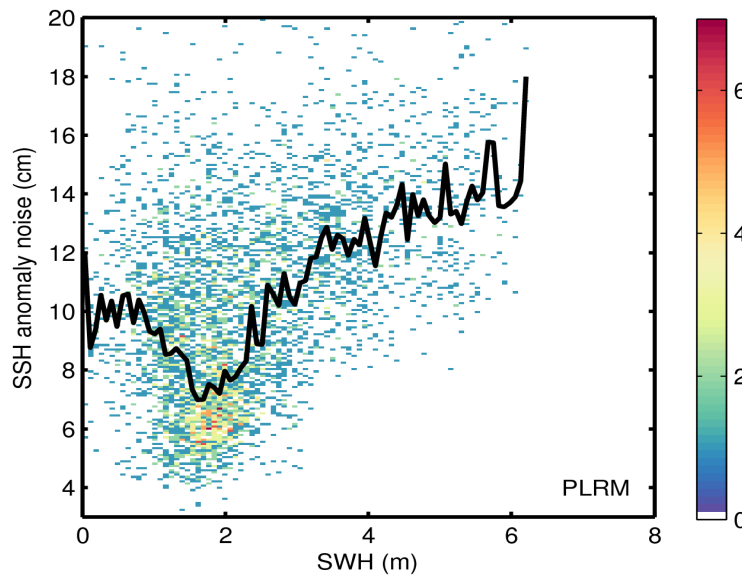
Figure 9. 2D histogram showing flag-valid SSH anomaly noise as a function of SWH for LRM (top) and PLRM (bottom) for 02/01/2016. The black line denotes the median SSH anomaly noise as a function of SWH.
