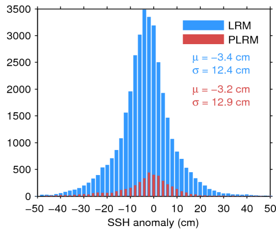
Figure 11. Histogram of science-valid SSH anomaly over oceans and lakes for LRM (blue) and PLRM (red) for 02/01/2016. The mean ( \mu ) and standard deviation ( \sigma ) are also shown. Note that values outside [-50\ 50] cm are excluded from the histogram for the sake of readability but not from the computation of \mu and \sigma .
