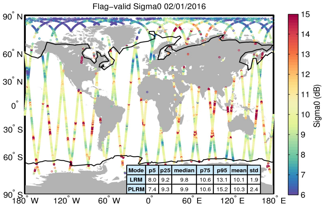
Figure 23. Geographical distribution of flag-valid sigma0 data over oceans and lakes for 02/01/2016. The statistical values shown in the table refer to the sigma0 in dB and are calculated separately for LRM and PLRM regions. Measurements taken over polar polygons have been excluded from the computation of the statistical values. The black lines mark the outer limit of the Arctic and Antarctic polar polygons.
