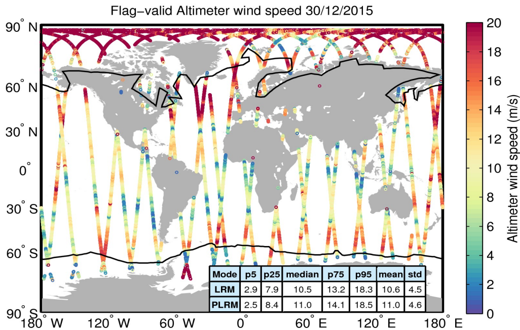
Figure 31. Geographical distribution of flag-valid wind data over oceans and lakes for 30/12/2015. The statistical values shown in the table refer to the wind in m/s and are calculated separately for LRM and PLRM regions. Measurements taken over polar polygons have been excluded from the computation of the statistical values. The black lines mark the outer limit of the Arctic and Antarctic polar polygons.
