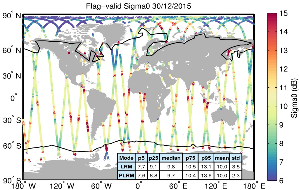
Figure 23. Geographical distribution of flag-valid sigma0 data over oceans and lakes for 30/12/2015. The statistical values shown in the table refer to the sigma0 in dB and are calculated separately for LRM and PLRM regions. Measurements taken over polar polygons have been excluded from the computation of the statistical values. The black lines mark the outer limit of the Arctic and Antarctic polar polygons.
