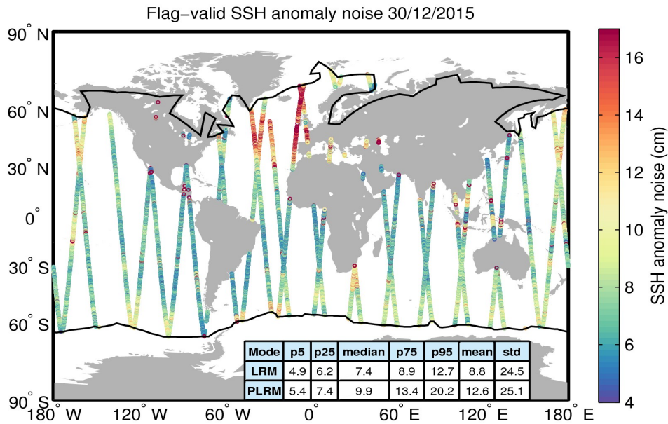
Figure 8. Geographical distribution of flag-valid 20-Hz SSH anomaly measurement noise over oceans and lakes for 30/12/2015. The statistical values shown in the table refer to the SSH anomaly noise and are calculated separately for LRM and PLRM regions. Measurements taken over polar polygons have been excluded from the computation of the statistical values. The black lines mark the outer limit of the Arctic and Antarctic polar polygons.
