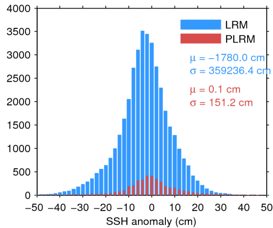
Figure 7. Histogram of flag-valid SSH anomaly over oceans and lakes for LRM (blue) and PLRM (red) for 30/12/2015. The mean ( \mu ) and standard deviation ( \sigma ) are also shown. Note that values outside [-50\ 50] cm are excluded from the histogram for the sake of readability but not from the computation of \mu and \sigma .
