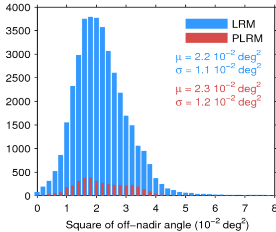
Figure 39. Histogram of flag-valid mispointing over oceans and lakes for LRM (blue) and PLRM (red) for 30/12/2015. Only positive values have been considered. The mean ( \mu ) and standard deviation ( \sigma ) are also shown. Note that values larger than 8 \cdot 10^{-2} \text{ deg}^2 are excluded from the histogram for the sake of readability but not from the computation of \mu and \sigma .
