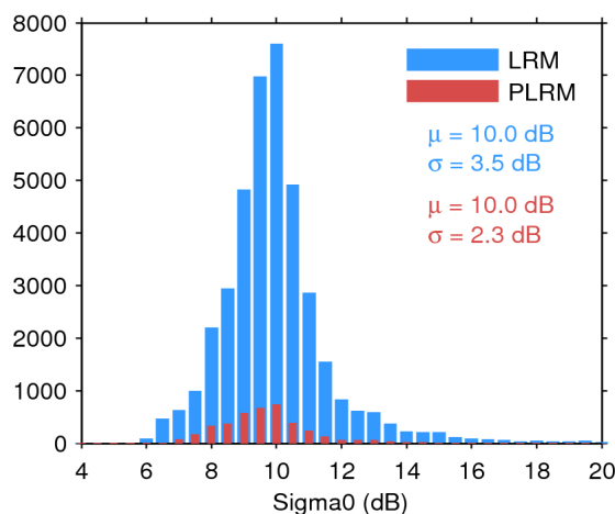
Figure 25. Histogram of flag-valid sigma0 over oceans and lakes for LRM (blue) and PLRM (red) for 30/12/2015. The mean ( \mu ) and standard deviation ( \sigma ) are also shown. Note that values outside [4 20] dB are excluded from the histogram for the sake of readability but not from the computation of \mu and \sigma .
