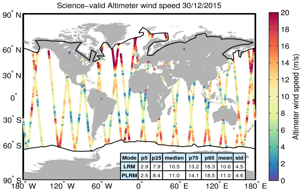
Figure 34. Geographical distribution of science-valid wind data over oceans and lakes for 30/12/2015. The statistical values shown in the table refer to the wind in m/s and are calculated separately for LRM and PLRM regions. The black lines mark the outer limit of the Arctic and Antarctic polar polygons. Gray circles denote records that have been rejected based on the editing criteria described in Table 5.
