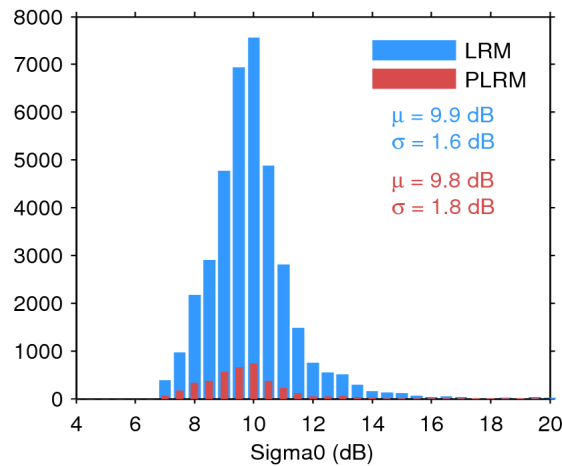
Figure 28. Histogram of science-valid sigma0 over oceans and lakes for LRM (blue) and PLRM (red) for 30/12/2015. The mean ( \mu ) and standard deviation ( \sigma ) are also shown. Note that values outside [4 20] dB are excluded from the histogram for the sake of readability but not from the computation of \mu and \sigma .
