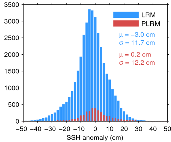
Figure 11. Histogram of science-valid SSH anomaly over oceans and lakes for LRM (blue) and PLRM (red) for 30/12/2015. The mean ( \mu ) and standard deviation ( \sigma ) are also shown. Note that values outside [-50\ 50] cm are excluded from the histogram for the sake of readability but not from the computation of \mu and \sigma .
