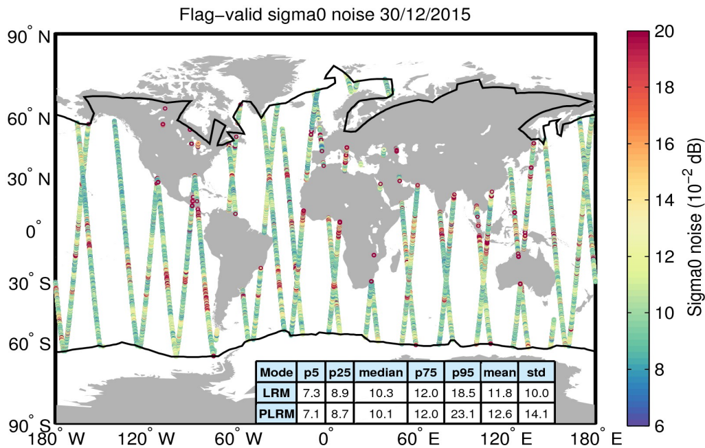
Figure 26. Geographical distribution of flag-valid 20-Hz sigma0 measurement noise over oceans and lakes for 30/12/2015. The statistical values shown in the table refer to the sigma0 noise and are calculated separately for LRM and PLRM regions. Measurements taken over polar polygons have been excluded from the computation of the statistical values. The black lines mark the outer limit of the Arctic and Antarctic polar polygons.
