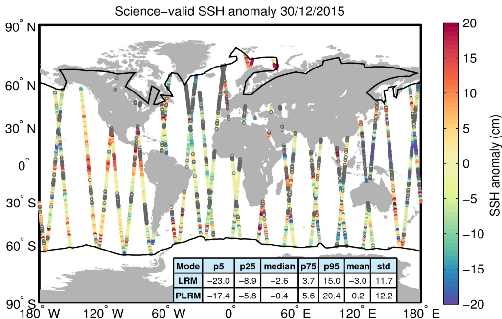
Figure 10. Geographical distribution of science-valid SSH anomaly data over oceans and lakes for 30/12/2015. The statistical values shown in the table refer to the SSH anomaly in cm and are calculated separately for LRM and PLRM regions. The black lines mark the outer limit of the Arctic and Antarctic polar polygons. Gray circles denote records that have been rejected based on the editing criteria described in Table 2.
