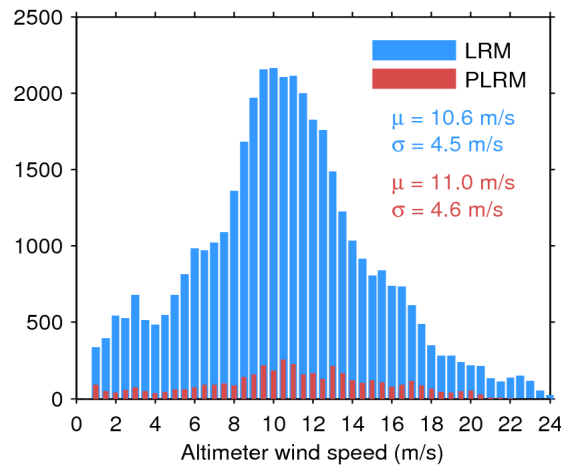
Figure 33. Histogram of flag-valid wind over oceans and lakes for LRM (blue) and PLRM (red) for 30/12/2015. The mean ( \mu ) and standard deviation ( \sigma ) are also shown. Note that values larger than 24 m/s are excluded from the histogram for the sake of readability but not from the computation of \mu and \sigma .
