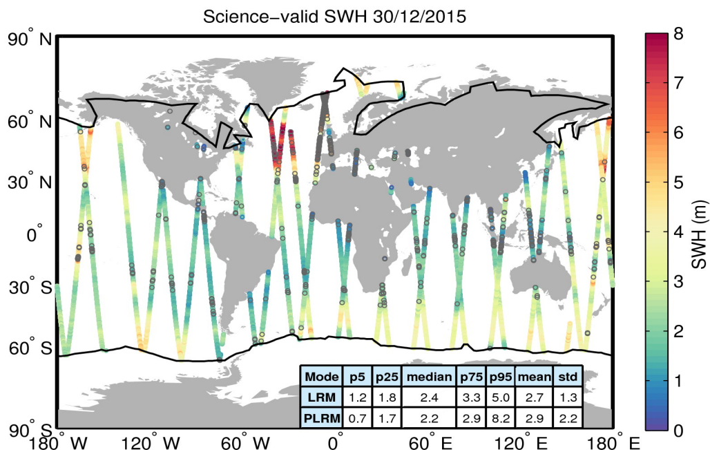
Figure 19. Geographical distribution of science-valid SWH data over oceans and lakes for 30/12/2015. The statistical values shown in the table refer to the SWH in m and are calculated separately for LRM and PLRM regions. The black lines mark the outer limit of the Arctic and Antarctic polar polygons. Gray circles denote records that have been rejected based on the editing criteria described in Table 3.
