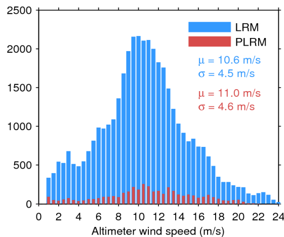
Figure 35. Histogram of science-valid wind over oceans and lakes for LRM (blue) and PLRM (red) for 30/12/2015. The mean ( \mu ) and standard deviation ( \sigma ) are also shown. Note that values larger than 24 m/s are excluded from the histogram for the sake of readability but not from the computation of \mu and \sigma .
