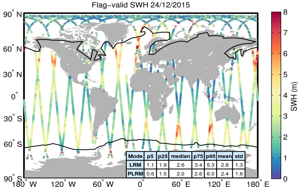
Figure 15. Geographical distribution of flag-valid SWH data over oceans and lakes for 24/12/2015. The statistical values shown in the table refer to the SWH in m and are calculated separately for LRM and PLRM regions. Measurements taken over polar polygons have been excluded from the computation of the statistical values. The black lines mark the outer limit of the Arctic and Antarctic polar polygons.
