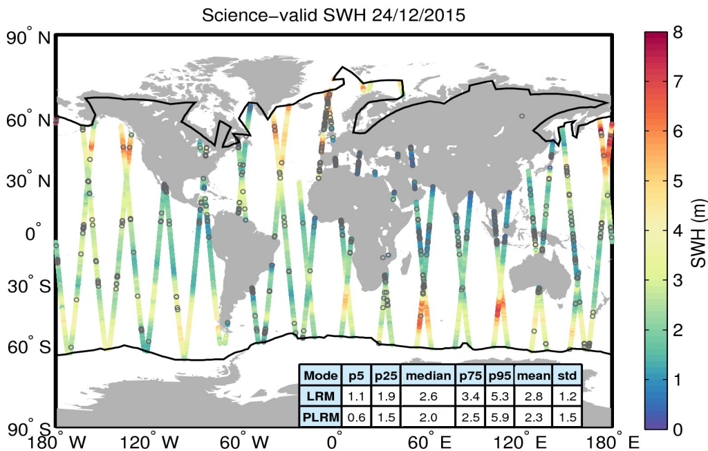
Figure 19. Geographical distribution of science-valid SWH data over oceans and lakes for 24/12/2015. The statistical values shown in the table refer to the SWH in m and are calculated separately for LRM and PLRM regions. The black lines mark the outer limit of the Arctic and Antarctic polar polygons. Gray circles denote records that have been rejected based on the editing criteria described in Table 3.
