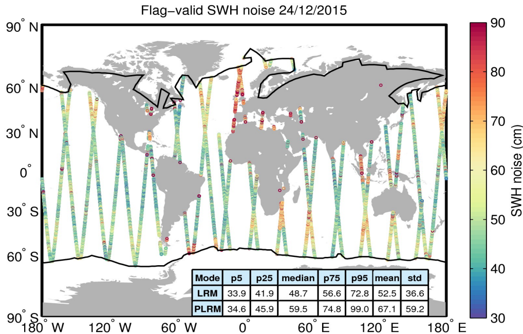
Figure 18. Geographical distribution of flag-valid 20-Hz SWH measurement noise over oceans and lakes for 24/12/2015. The statistical values shown in the table refer to the SWH noise and are calculated separately for LRM and PLRM regions. Measurements taken over polar polygons have been excluded from the computation of the statistical values. The black lines mark the outer limit of the Arctic and Antarctic polar polygons.
