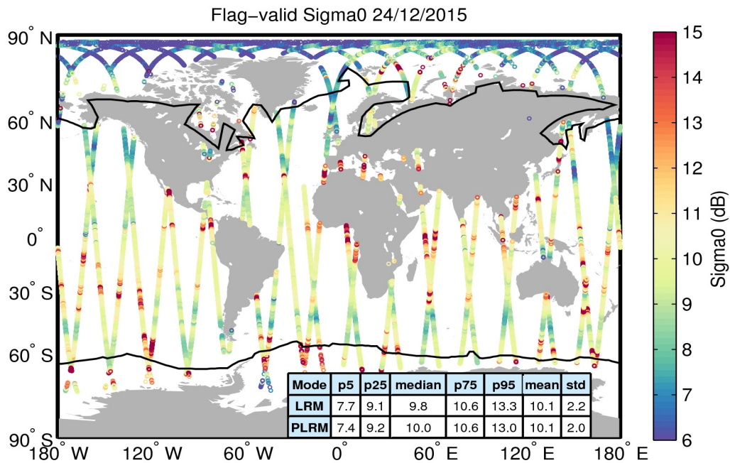
Figure 23. Geographical distribution of flag-valid sigma0 data over oceans and lakes for 24/12/2015. The statistical values shown in the table refer to the sigma0 in dB and are calculated separately for LRM and PLRM regions. Measurements taken over polar polygons have been excluded from the computation of the statistical values. The black lines mark the outer limit of the Arctic and Antarctic polar polygons.
