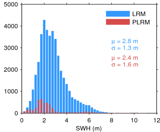
Figure 17. Histogram of flag-valid SWH over oceans and lakes for LRM (blue) and PLRM (red) for 24/12/2015. The mean ( \mu ) and standard deviation ( \sigma ) are also shown. Note that values larger than 12 m are excluded from the histogram for the sake of readability but not from the computation of \mu and \sigma .
