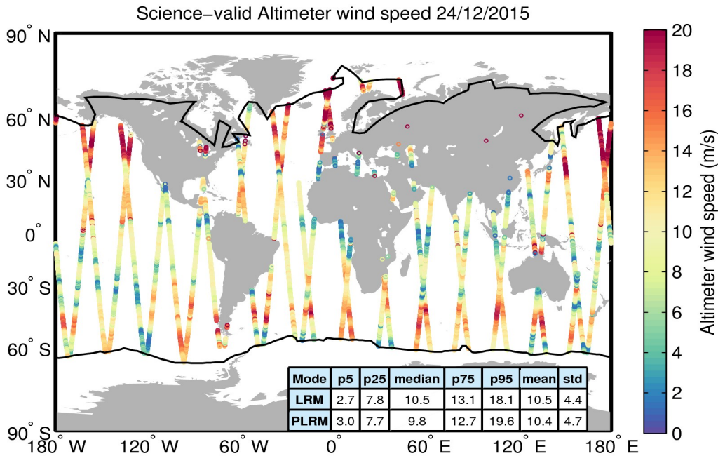
Figure 34. Geographical distribution of science-valid wind data over oceans and lakes for 24/12/2015. The statistical values shown in the table refer to the wind in m/s and are calculated separately for LRM and PLRM regions. The black lines mark the outer limit of the Arctic and Antarctic polar polygons. Gray circles denote records that have been rejected based on the editing criteria described in Table 5.
