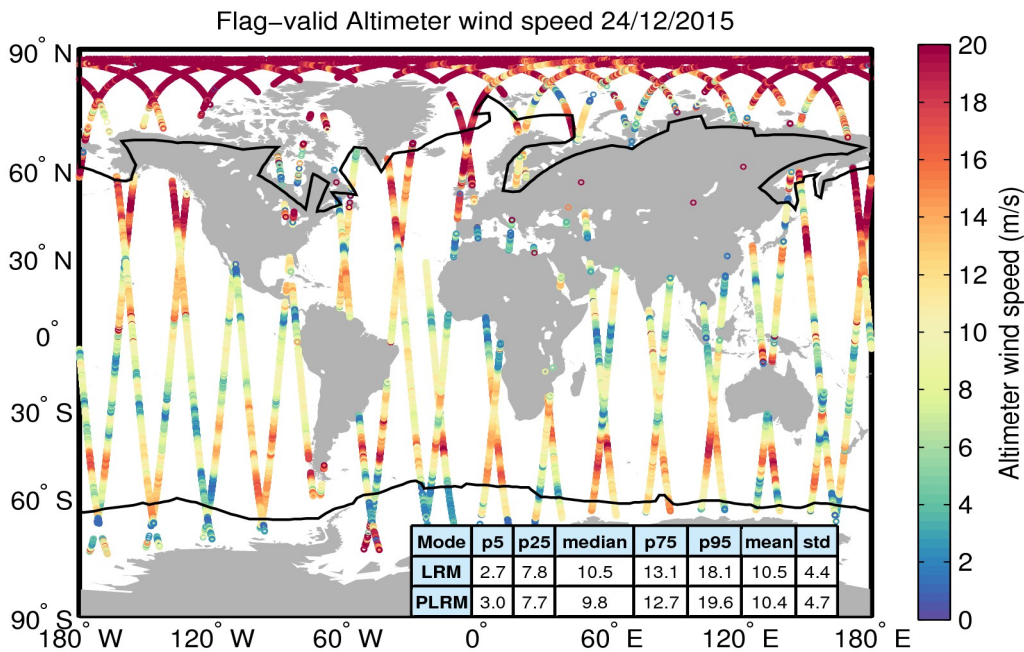
Figure 31. Geographical distribution of flag-valid wind data over oceans and lakes for 24/12/2015. The statistical values shown in the table refer to the wind in m/s and are calculated separately for LRM and PLRM regions. Measurements taken over polar polygons have been excluded from the computation of the statistical values. The black lines mark the outer limit of the Arctic and Antarctic polar polygons.
