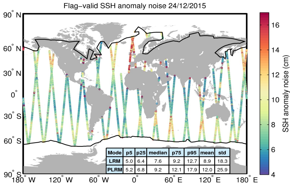
Figure 8. Geographical distribution of flag-valid 20-Hz SSH anomaly measurement noise over oceans and lakes for 24/12/2015. The statistical values shown in the table refer to the SSH anomaly noise and are calculated separately for LRM and PLRM regions. Measurements taken over polar polygons have been excluded from the computation of the statistical values. The black lines mark the outer limit of the Arctic and Antarctic polar polygons.
