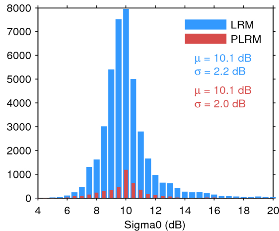
Figure 25. Histogram of flag-valid sigma0 over oceans and lakes for LRM (blue) and PLRM (red) for 24/12/2015. The mean ( \mu ) and standard deviation ( \sigma ) are also shown. Note that values outside [4 20] dB are excluded from the histogram for the sake of readability but not from the computation of \mu and \sigma .
