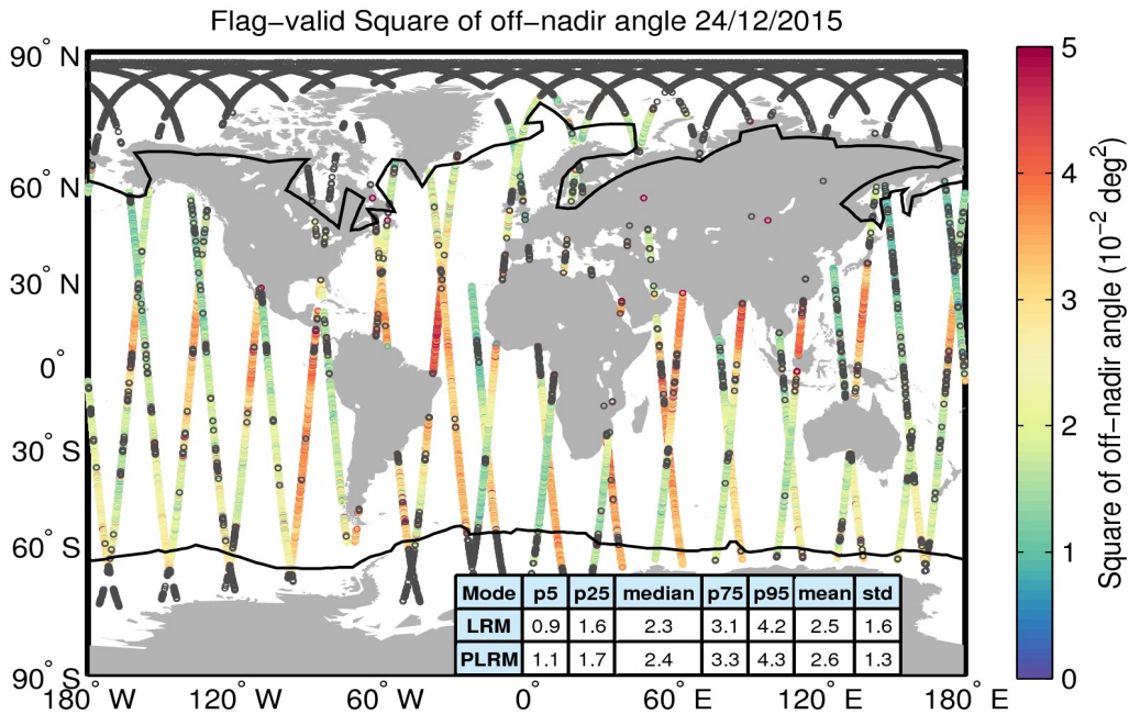
Figure 37. Geographical distribution of flag-valid mispointing data over oceans and lakes for 24/12/2015. The statistical values shown in the table refer to the mispointing in 10^{-2} deg 2 and are calculated separately for LRM and PLRM regions. Measurements taken over polar polygons have been excluded from the computation of the statistical values. The black lines mark the outer limit of the Arctic and Antarctic polar polygons. Gray circles denote negative values.
