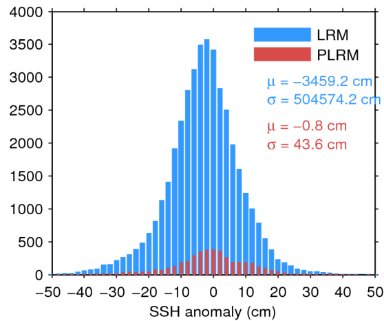
Figure 7. Histogram of flag-valid SSH anomaly over oceans and lakes for LRM (blue) and PLRM (red) for 24/12/2015. The mean ( \mu ) and standard deviation ( \sigma ) are also shown. Note that values outside [-50 50] cm are excluded from the histogram for the sake of readability but not from the computation of \mu and \sigma .
