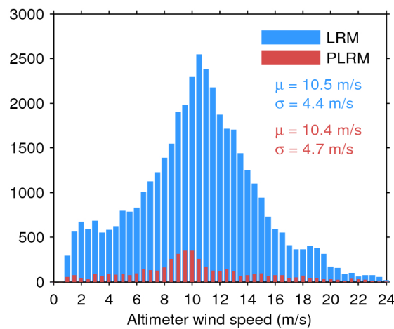
Figure 33. Histogram of flag-valid wind over oceans and lakes for LRM (blue) and PLRM (red) for 24/12/2015. The mean ( \mu ) and standard deviation ( \sigma ) are also shown. Note that values larger than 24 m/s are excluded from the histogram for the sake of readability but not from the computation of \mu and \sigma .
