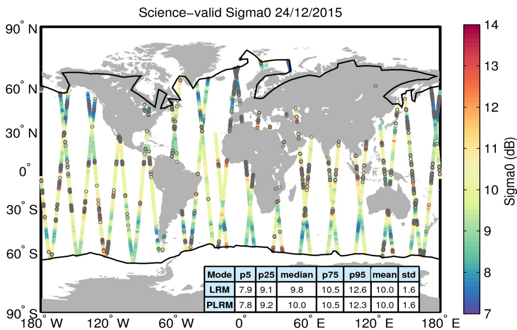
Figure 27. Geographical distribution of science-valid sigma0 data over oceans and lakes for 24/12/2015. The statistical values shown in the table refer to the sigma0 in dB and are calculated separately for LRM and PLRM regions. The black lines mark the outer limit of the Arctic and Antarctic polar polygons. Gray circles denote records that have been rejected based on the editing criteria described in Table 4.
