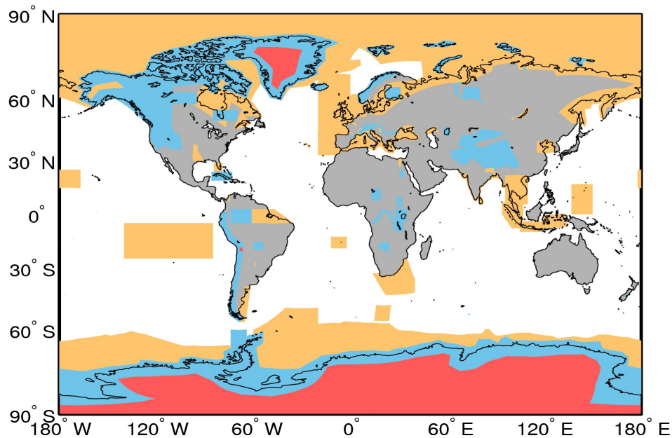
Figure A1. Extent of the regions defining the geographical mode mask for 24/12/2015. The regions where SAR, and SARIn are operated are denoted by the orange and blue polygons, respectively. LRM is operated over areas of the continental ice sheets (red polygons) and over oceans and land not covered by other modes.
