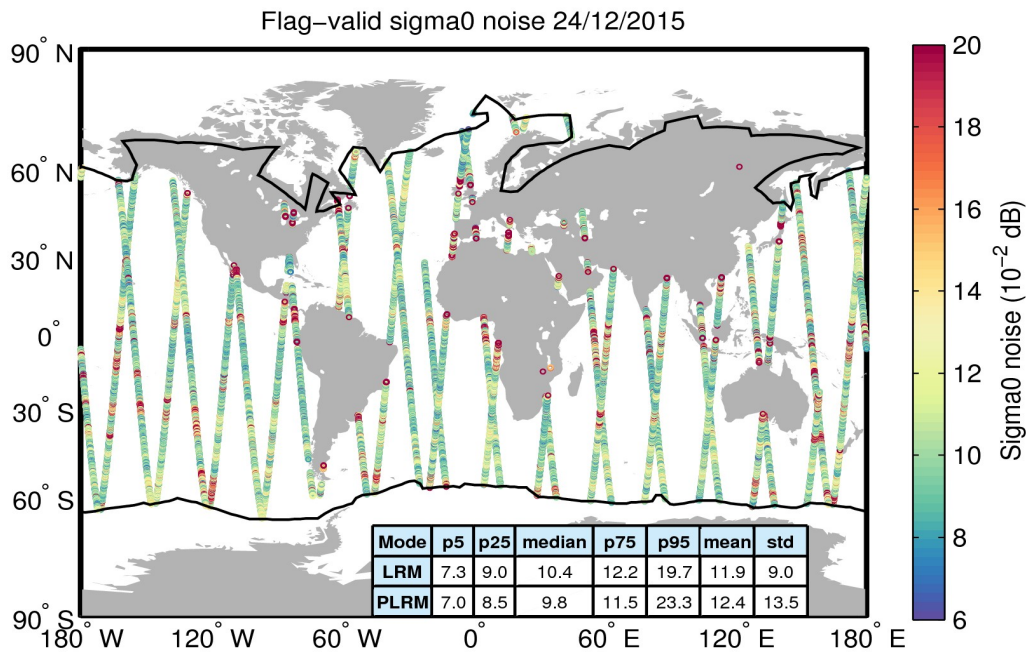
Figure 26. Geographical distribution of flag-valid 20-Hz sigma0 measurement noise over oceans and lakes for 24/12/2015. The statistical values shown in the table refer to the sigma0 noise and are calculated separately for LRM and PLRM regions. Measurements taken over polar polygons have been excluded from the computation of the statistical values. The black lines mark the outer limit of the Arctic and Antarctic polar polygons.
