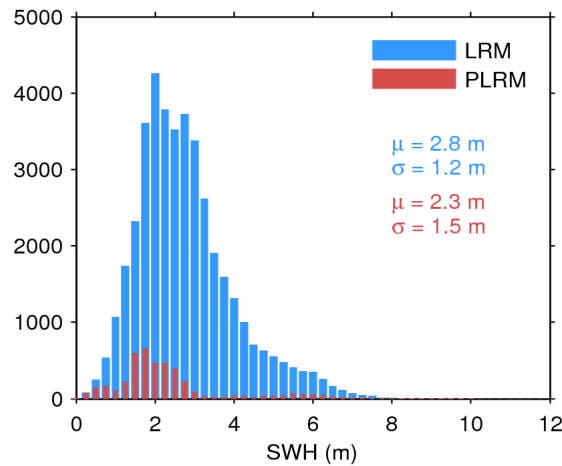
Figure 20. Histogram of science-valid SWH over oceans and lakes for LRM (blue) and PLRM (red) for 24/12/2015. The mean ( \mu ) and standard deviation ( \sigma ) are also shown. Note that values larger than 12 m are excluded from the histogram for the sake of readability but not from the computation of \mu and \sigma .
