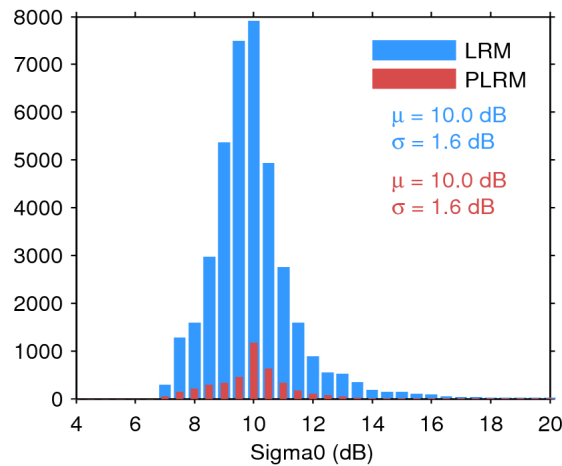
Figure 28. Histogram of science-valid sigma0 over oceans and lakes for LRM (blue) and PLRM (red) for 24/12/2015. The mean ( \mu ) and standard deviation ( \sigma ) are also shown. Note that values outside [4 20] dB are excluded from the histogram for the sake of readability but not from the computation of \mu and \sigma .
