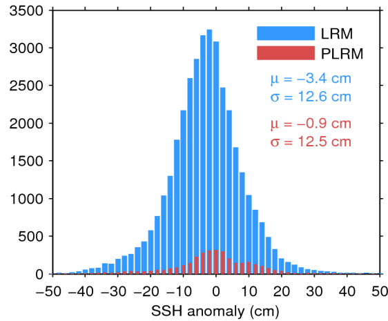
Figure 11. Histogram of science-valid SSH anomaly over oceans and lakes for LRM (blue) and PLRM (red) for 24/12/2015. The mean ( \mu ) and standard deviation ( \sigma ) are also shown. Note that values outside [-50 50] cm are excluded from the histogram for the sake of readability but not from the computation of \mu and \sigma .
