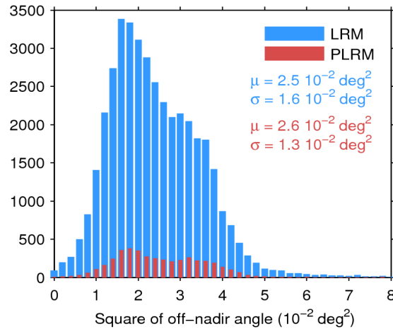
Figure 39. Histogram of flag-valid mispointing over oceans and lakes for LRM (blue) and PLRM (red) for 24/12/2015. Only positive values have been considered. The mean ( \mu ) and standard deviation ( \sigma ) are also shown. Note that values larger than 8 \cdot 10^{-2} \text{ deg}^2 are excluded from the histogram for the sake of readability but not from the computation of \mu and \sigma .
