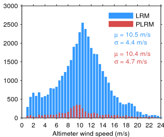
Figure 35. Histogram of science-valid wind over oceans and lakes for LRM (blue) and PLRM (red) for 24/12/2015. The mean ( \mu ) and standard deviation ( \sigma ) are also shown. Note that values larger than 24 m/s are excluded from the histogram for the sake of readability but not from the computation of \mu and \sigma .
