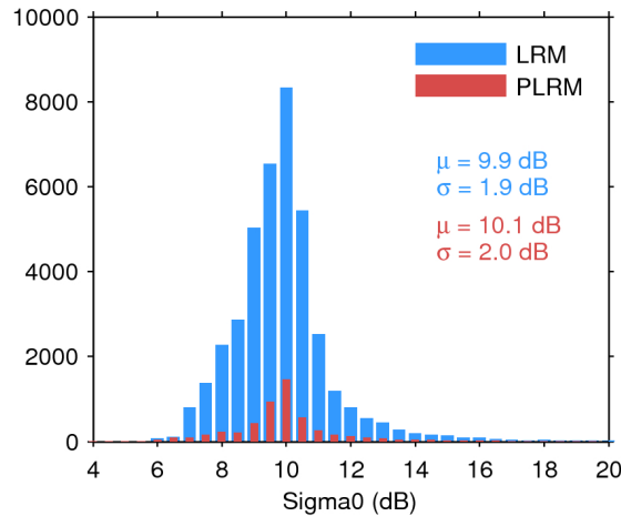
Figure 25. Histogram of flag-valid sigma0 over oceans and lakes for LRM (blue) and PLRM (red) for 23/12/2015. The mean ( \mu ) and standard deviation ( \sigma ) are also shown. Note that values outside [4 20] dB are excluded from the histogram for the sake of readability but not from the computation of \mu and \sigma .
