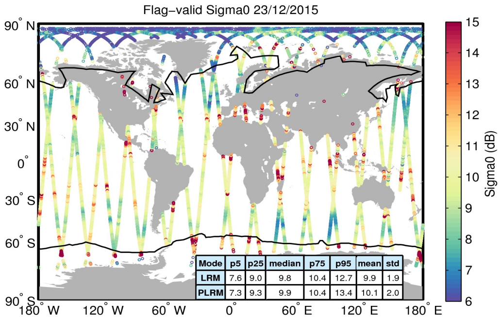
Figure 23. Geographical distribution of flag-valid sigma0 data over oceans and lakes for 23/12/2015. The statistical values shown in the table refer to the sigma0 in dB and are calculated separately for LRM and PLRM regions. Measurements taken over polar polygons have been excluded from the computation of the statistical values. The black lines mark the outer limit of the Arctic and Antarctic polar polygons.
