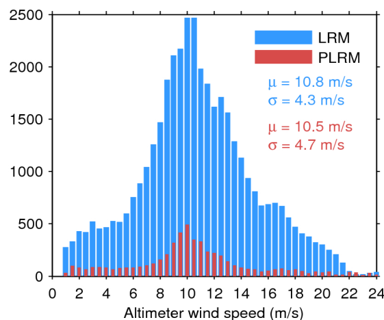
Figure 35. Histogram of science-valid wind over oceans and lakes for LRM (blue) and PLRM (red) for 23/12/2015. The mean ( \mu ) and standard deviation ( \sigma ) are also shown. Note that values larger than 24 m/s are excluded from the histogram for the sake of readability but not from the computation of \mu and \sigma .
