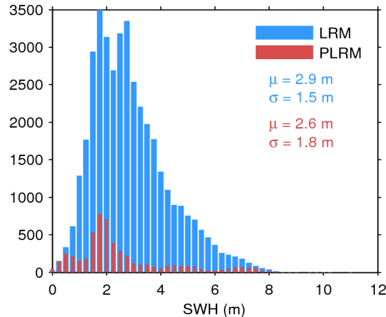
Figure 17. Histogram of flag-valid SWH over oceans and lakes for LRM (blue) and PLRM (red) for 23/12/2015. The mean ( \mu ) and standard deviation ( \sigma ) are also shown. Note that values larger than 12 m are excluded from the histogram for the sake of readability but not from the computation of \mu and \sigma .
