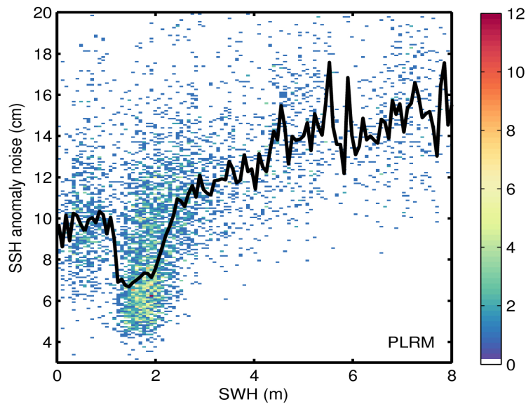
Figure 9. 2D histogram showing flag-valid SSH anomaly noise as a function of SWH for LRM (top) and PLRM (bottom) for 23/12/2015. The black line denotes the median SSH anomaly noise as a function of SWH.
