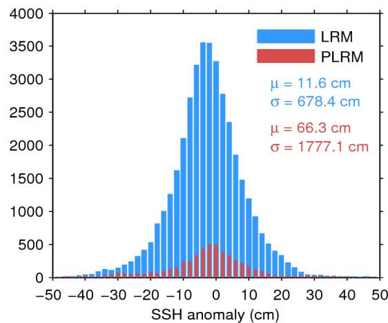
Figure 7. Histogram of flag-valid SSH anomaly over oceans and lakes for LRM (blue) and PLRM (red) for 23/12/2015. The mean ( \mu ) and standard deviation ( \sigma ) are also shown. Note that values outside [-50 50] cm are excluded from the histogram for the sake of readability but not from the computation of \mu and \sigma .
