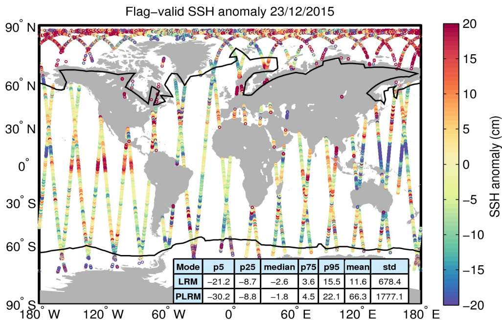
Figure 5. Geographical distribution of flag-valid 1-Hz SSH anomaly data over oceans and lakes for 23/12/2015. The statistical values shown in the table refer to the SSH anomaly in cm and are calculated separately for LRM and PLRM regions. Measurements taken over polar polygons have been excluded from the computation of the statistical values. The black lines mark the outer limit of the Arctic and Antarctic polar polygons.
