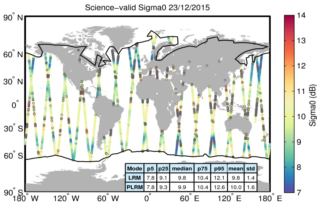
Figure 27. Geographical distribution of science-valid sigma0 data over oceans and lakes for 23/12/2015. The statistical values shown in the table refer to the sigma0 in dB and are calculated separately for LRM and PLRM regions. The black lines mark the outer limit of the Arctic and Antarctic polar polygons. Gray circles denote records that have been rejected based on the editing criteria described in Table 4.
