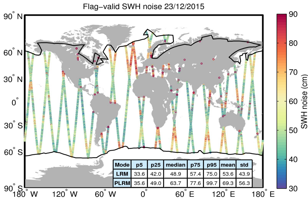
Figure 18. Geographical distribution of flag-valid 20-Hz SWH measurement noise over oceans and lakes for 23/12/2015. The statistical values shown in the table refer to the SWH noise and are calculated separately for LRM and PLRM regions. Measurements taken over polar polygons have been excluded from the computation of the statistical values. The black lines mark the outer limit of the Arctic and Antarctic polar polygons.
