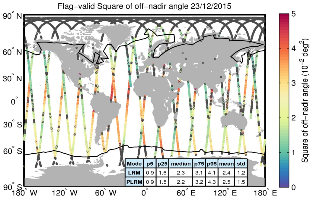
Figure 37. Geographical distribution of flag-valid mispointing data over oceans and lakes for 23/12/2015. The statistical values shown in the table refer to the mispointing in 10^{-2} deg 2 and are calculated separately for LRM and PLRM regions. Measurements taken over polar polygons have been excluded from the computation of the statistical values. The black lines mark the outer limit of the Arctic and Antarctic polar polygons. Gray circles denote negative values.
