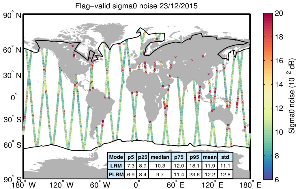
Figure 26. Geographical distribution of flag-valid 20-Hz sigma0 measurement noise over oceans and lakes for 23/12/2015. The statistical values shown in the table refer to the sigma0 noise and are calculated separately for LRM and PLRM regions. Measurements taken over polar polygons have been excluded from the computation of the statistical values. The black lines mark the outer limit of the Arctic and Antarctic polar polygons.
