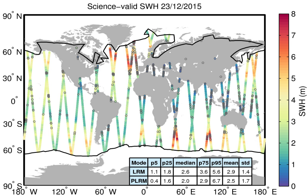
Figure 19. Geographical distribution of science-valid SWH data over oceans and lakes for 23/12/2015. The statistical values shown in the table refer to the SWH in m and are calculated separately for LRM and PLRM regions. The black lines mark the outer limit of the Arctic and Antarctic polar polygons. Gray circles denote records that have been rejected based on the editing criteria described in Table 3.
