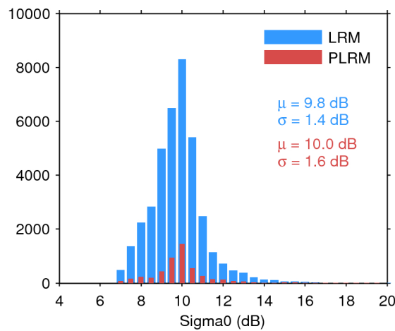
Figure 28. Histogram of science-valid sigma0 over oceans and lakes for LRM (blue) and PLRM (red) for 23/12/2015. The mean ( \mu ) and standard deviation ( \sigma ) are also shown. Note that values outside [4 20] dB are excluded from the histogram for the sake of readability but not from the computation of \mu and \sigma .
