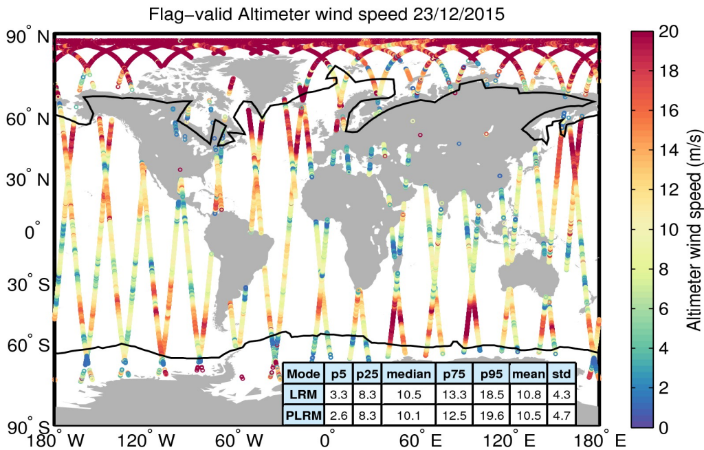
Figure 31. Geographical distribution of flag-valid wind data over oceans and lakes for 23/12/2015. The statistical values shown in the table refer to the wind in m/s and are calculated separately for LRM and PLRM regions. Measurements taken over polar polygons have been excluded from the computation of the statistical values. The black lines mark the outer limit of the Arctic and Antarctic polar polygons.
