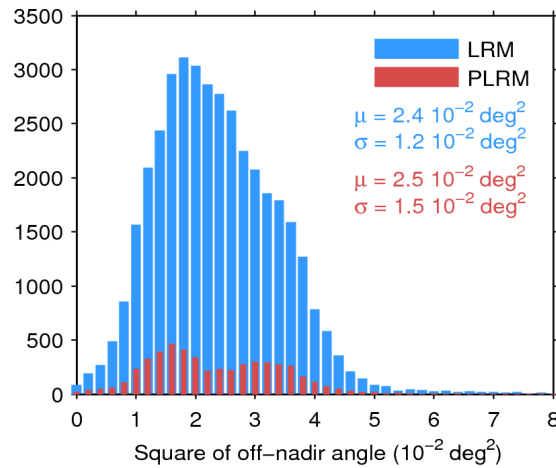
Figure 39. Histogram of flag-valid mispointing over oceans and lakes for LRM (blue) and PLRM (red) for 23/12/2015. Only positive values have been considered. The mean ( \mu ) and standard deviation ( \sigma ) are also shown. Note that values larger than 8 \cdot 10^{-2} \text{ deg}^2 are excluded from the histogram for the sake of readability but not from the computation of \mu and \sigma .
