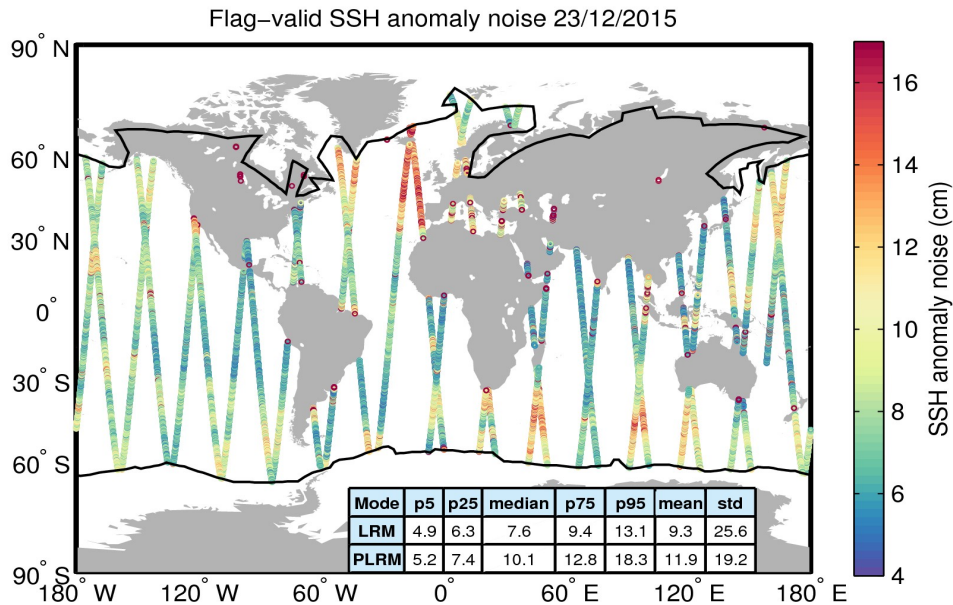
Figure 8. Geographical distribution of flag-valid 20-Hz SSH anomaly measurement noise over oceans and lakes for 23/12/2015. The statistical values shown in the table refer to the SSH anomaly noise and are calculated separately for LRM and PLRM regions. Measurements taken over polar polygons have been excluded from the computation of the statistical values. The black lines mark the outer limit of the Arctic and Antarctic polar polygons.
