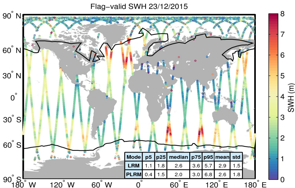
Figure 15. Geographical distribution of flag-valid SWH data over oceans and lakes for 23/12/2015. The statistical values shown in the table refer to the SWH in m and are calculated separately for LRM and PLRM regions. Measurements taken over polar polygons have been excluded from the computation of the statistical values. The black lines mark the outer limit of the Arctic and Antarctic polar polygons.
