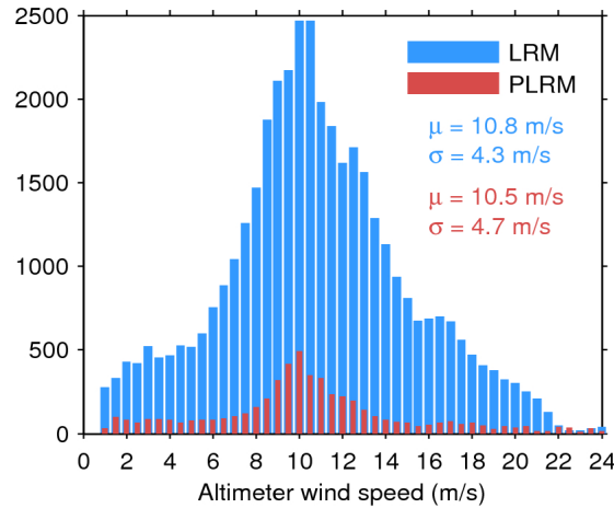
Figure 33. Histogram of flag-valid wind over oceans and lakes for LRM (blue) and PLRM (red) for 23/12/2015. The mean ( \mu ) and standard deviation ( \sigma ) are also shown. Note that values larger than 24 m/s are excluded from the histogram for the sake of readability but not from the computation of \mu and \sigma .
