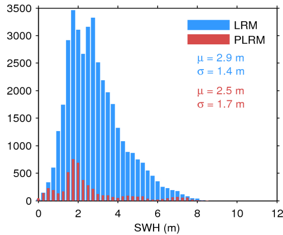
Figure 20. Histogram of science-valid SWH over oceans and lakes for LRM (blue) and PLRM (red) for 23/12/2015. The mean ( \mu ) and standard deviation ( \sigma ) are also shown. Note that values larger than 12 m are excluded from the histogram for the sake of readability but not from the computation of \mu and \sigma .
