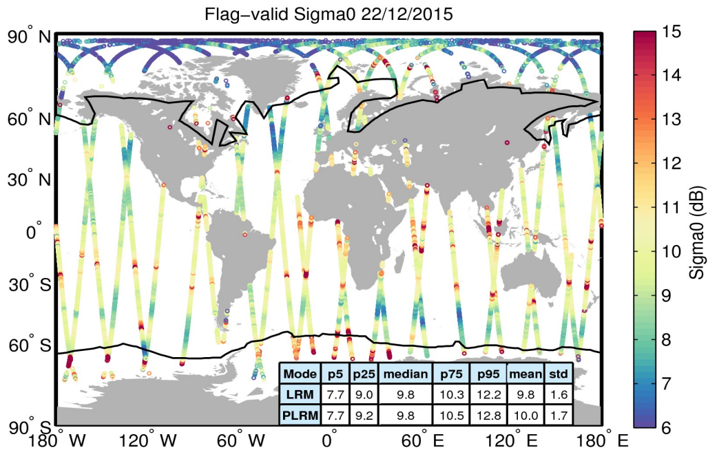
Figure 23. Geographical distribution of flag-valid sigma0 data over oceans and lakes for 22/12/2015. The statistical values shown in the table refer to the sigma0 in dB and are calculated separately for LRM and PLRM regions. Measurements taken over polar polygons have been excluded from the computation of the statistical values. The black lines mark the outer limit of the Arctic and Antarctic polar polygons.
