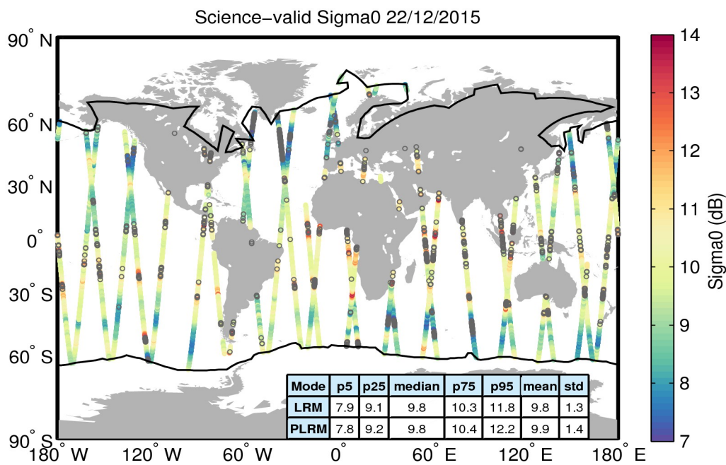
Figure 27. Geographical distribution of science-valid sigma0 data over oceans and lakes for 22/12/2015. The statistical values shown in the table refer to the sigma0 in dB and are calculated separately for LRM and PLRM regions. The black lines mark the outer limit of the Arctic and Antarctic polar polygons. Gray circles denote records that have been rejected based on the editing criteria described in Table 4.
