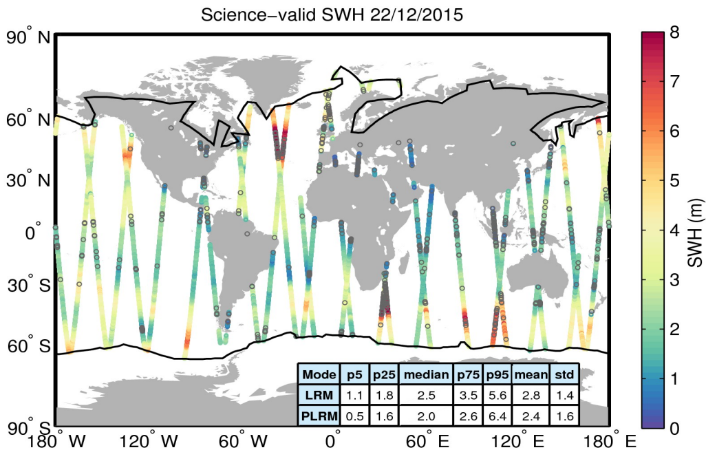
Figure 19. Geographical distribution of science-valid SWH data over oceans and lakes for 22/12/2015. The statistical values shown in the table refer to the SWH in m and are calculated separately for LRM and PLRM regions. The black lines mark the outer limit of the Arctic and Antarctic polar polygons. Gray circles denote records that have been rejected based on the editing criteria described in Table 3.
