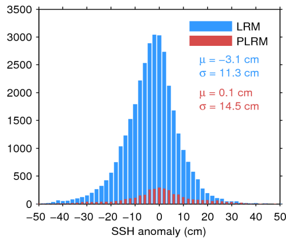
Figure 11. Histogram of science-valid SSH anomaly over oceans and lakes for LRM (blue) and PLRM (red) for 22/12/2015. The mean ( \mu ) and standard deviation ( \sigma ) are also shown. Note that values outside [-50 50] cm are excluded from the histogram for the sake of readability but not from the computation of \mu and \sigma .
