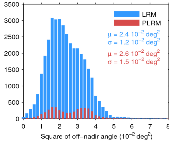
Figure 39. Histogram of flag-valid mispointing over oceans and lakes for LRM (blue) and PLRM (red) for 22/12/2015. Only positive values have been considered. The mean ( \mu ) and standard deviation ( \sigma ) are also shown. Note that values larger than 8 \cdot 10^{-2} \text{ deg}^2 are excluded from the histogram for the sake of readability but not from the computation of \mu and \sigma .
