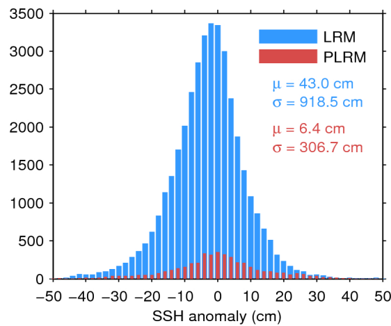
Figure 7. Histogram of flag-valid SSH anomaly over oceans and lakes for LRM (blue) and PLRM (red) for 22/12/2015. The mean ( \mu ) and standard deviation ( \sigma ) are also shown. Note that values outside [-50 50] cm are excluded from the histogram for the sake of readability but not from the computation of \mu and \sigma .
