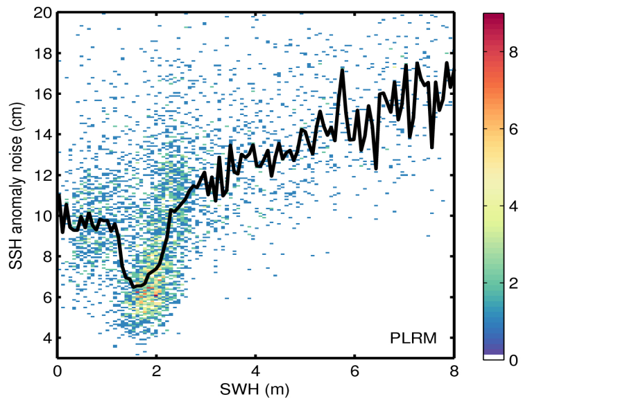
Figure 9. 2D histogram showing flag-valid SSH anomaly noise as a function of SWH for LRM (top) and PLRM (bottom) for 22/12/2015. The black line denotes the median SSH anomaly noise as a function of SWH.
