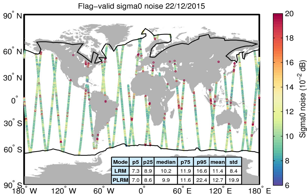
Figure 26. Geographical distribution of flag-valid 20-Hz sigma0 measurement noise over oceans and lakes for 22/12/2015. The statistical values shown in the table refer to the sigma0 noise and are calculated separately for LRM and PLRM regions. Measurements taken over polar polygons have been excluded from the computation of the statistical values. The black lines mark the outer limit of the Arctic and Antarctic polar polygons.
