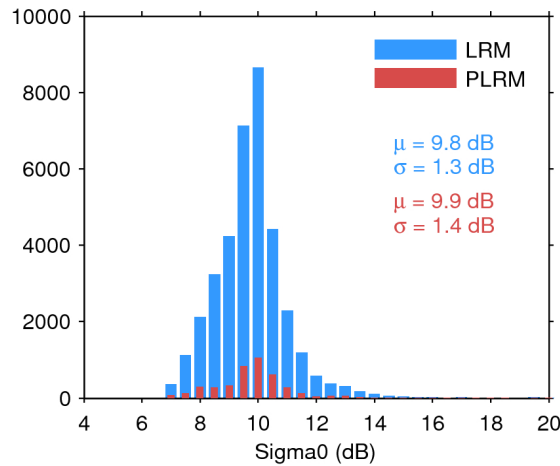
Figure 28. Histogram of science-valid sigma0 over oceans and lakes for LRM (blue) and PLRM (red) for 22/12/2015. The mean ( \mu ) and standard deviation ( \sigma ) are also shown. Note that values outside [4 20] dB are excluded from the histogram for the sake of readability but not from the computation of \mu and \sigma .
