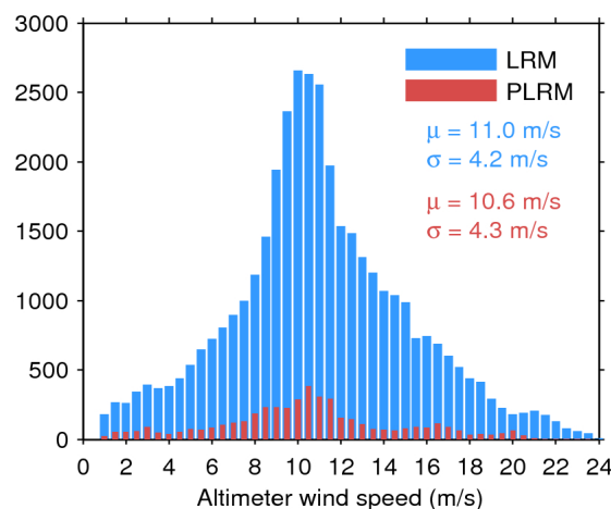
Figure 35. Histogram of science-valid wind over oceans and lakes for LRM (blue) and PLRM (red) for 22/12/2015. The mean ( \mu ) and standard deviation ( \sigma ) are also shown. Note that values larger than 24 m/s are excluded from the histogram for the sake of readability but not from the computation of \mu and \sigma .
