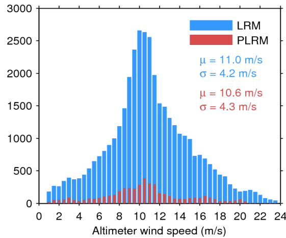
Figure 33. Histogram of flag-valid wind over oceans and lakes for LRM (blue) and PLRM (red) for 22/12/2015. The mean ( \mu ) and standard deviation ( \sigma ) are also shown. Note that values larger than 24 m/s are excluded from the histogram for the sake of readability but not from the computation of \mu and \sigma .
