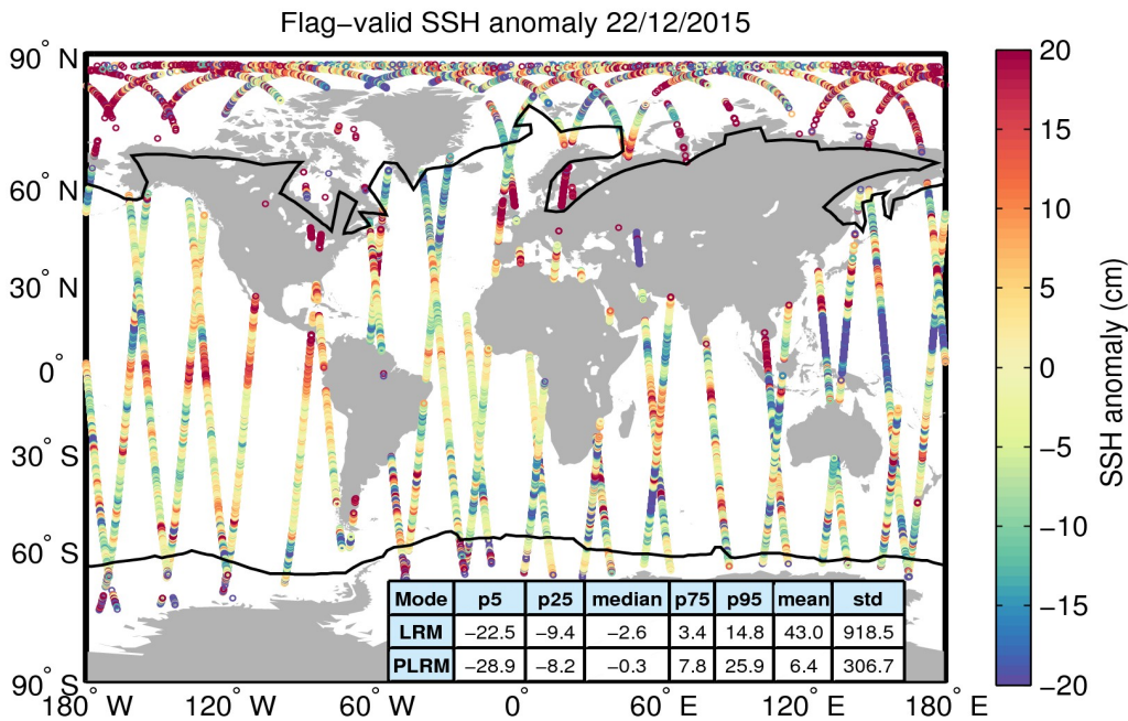
Figure 5. Geographical distribution of flag-valid 1-Hz SSH anomaly data over oceans and lakes for 22/12/2015. The statistical values shown in the table refer to the SSH anomaly in cm and are calculated separately for LRM and PLRM regions. Measurements taken over polar polygons have been excluded from the computation of the statistical values. The black lines mark the outer limit of the Arctic and Antarctic polar polygons.
