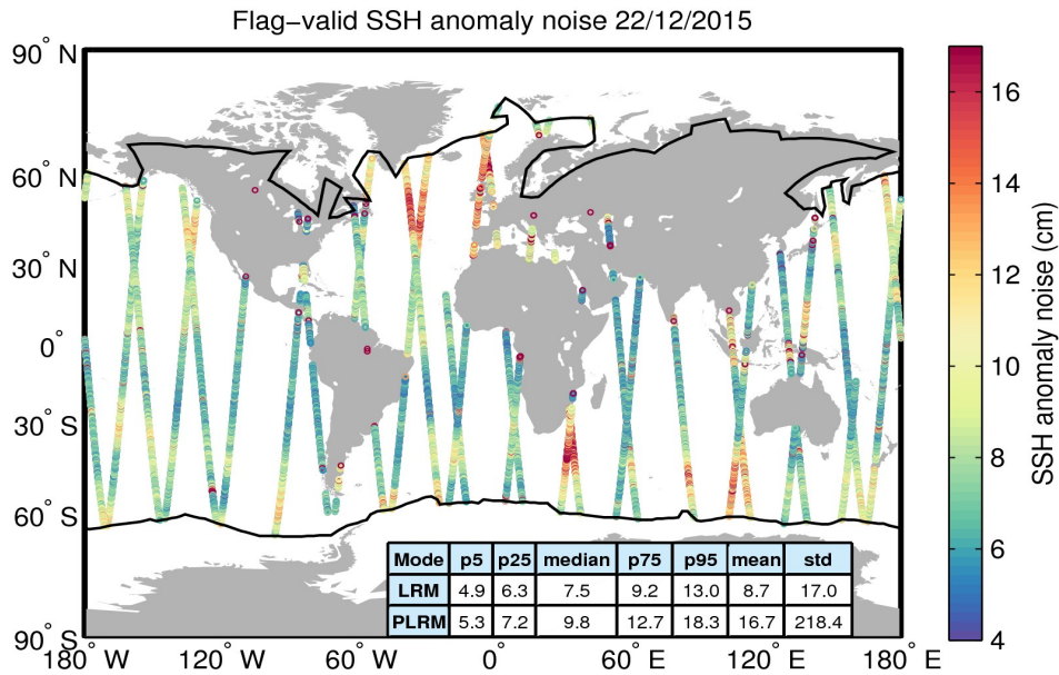
Figure 8. Geographical distribution of flag-valid 20-Hz SSH anomaly measurement noise over oceans and lakes for 22/12/2015. The statistical values shown in the table refer to the SSH anomaly noise and are calculated separately for LRM and PLRM regions. Measurements taken over polar polygons have been excluded from the computation of the statistical values. The black lines mark the outer limit of the Arctic and Antarctic polar polygons.
