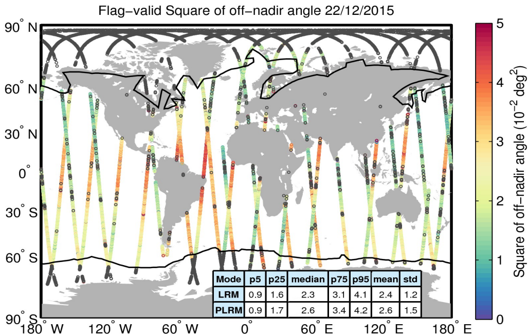
Figure 37. Geographical distribution of flag-valid mispointing data over oceans and lakes for 22/12/2015. The statistical values shown in the table refer to the mispointing in 10^{-2} deg 2 and are calculated separately for LRM and PLRM regions. Measurements taken over polar polygons have been excluded from the computation of the statistical values. The black lines mark the outer limit of the Arctic and Antarctic polar polygons. Gray circles denote negative values.
