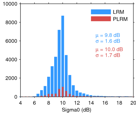
Figure 25. Histogram of flag-valid sigma0 over oceans and lakes for LRM (blue) and PLRM (red) for 22/12/2015. The mean ( \mu ) and standard deviation ( \sigma ) are also shown. Note that values outside [4 20] dB are excluded from the histogram for the sake of readability but not from the computation of \mu and \sigma .
