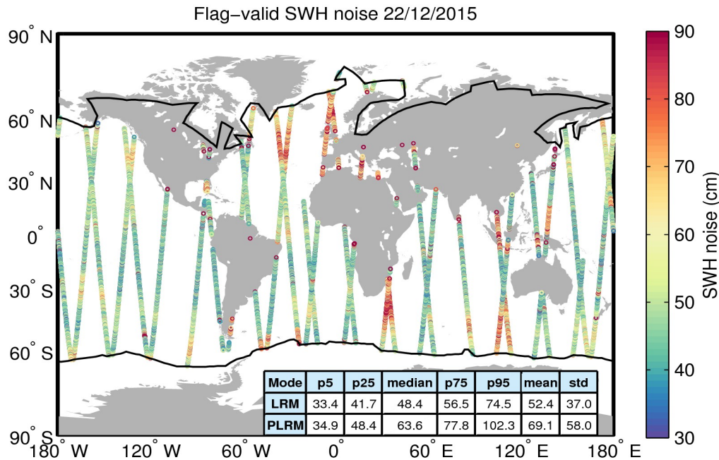
Figure 18. Geographical distribution of flag-valid 20-Hz SWH measurement noise over oceans and lakes for 22/12/2015. The statistical values shown in the table refer to the SWH noise and are calculated separately for LRM and PLRM regions. Measurements taken over polar polygons have been excluded from the computation of the statistical values. The black lines mark the outer limit of the Arctic and Antarctic polar polygons.
