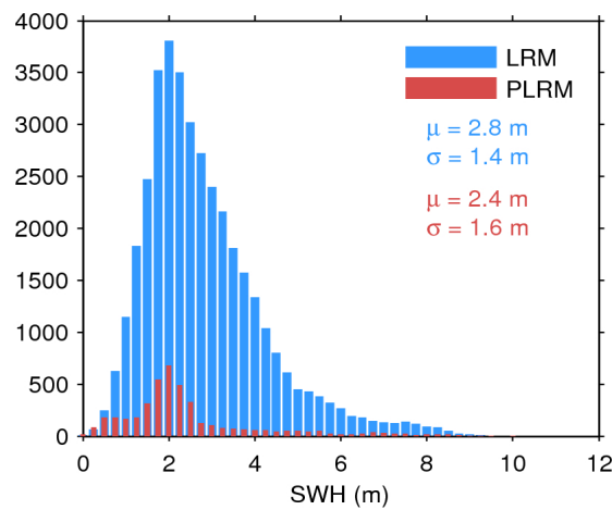
Figure 20. Histogram of science-valid SWH over oceans and lakes for LRM (blue) and PLRM (red) for 22/12/2015. The mean ( \mu ) and standard deviation ( \sigma ) are also shown. Note that values larger than 12 m are excluded from the histogram for the sake of readability but not from the computation of \mu and \sigma .
