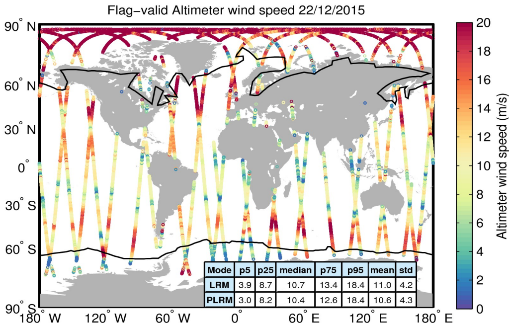
Figure 31. Geographical distribution of flag-valid wind data over oceans and lakes for 22/12/2015. The statistical values shown in the table refer to the wind in m/s and are calculated separately for LRM and PLRM regions. Measurements taken over polar polygons have been excluded from the computation of the statistical values. The black lines mark the outer limit of the Arctic and Antarctic polar polygons.
