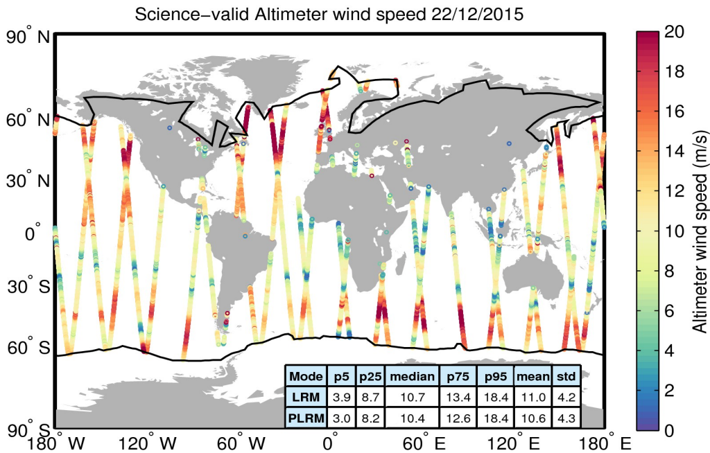
Figure 34. Geographical distribution of science-valid wind data over oceans and lakes for 22/12/2015. The statistical values shown in the table refer to the wind in m/s and are calculated separately for LRM and PLRM regions. The black lines mark the outer limit of the Arctic and Antarctic polar polygons. Gray circles denote records that have been rejected based on the editing criteria described in Table 5.
