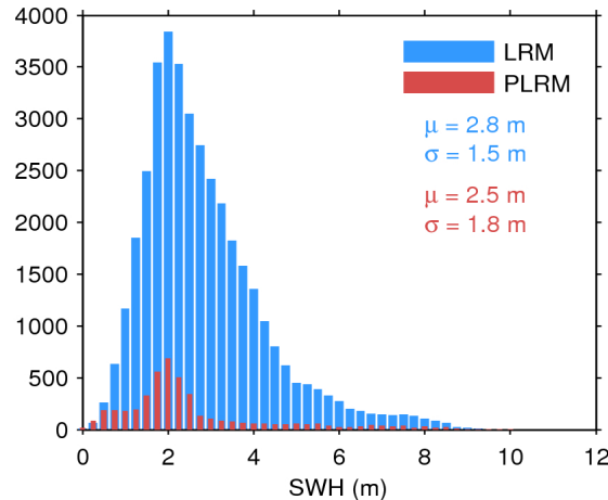
Figure 17. Histogram of flag-valid SWH over oceans and lakes for LRM (blue) and PLRM (red) for 22/12/2015. The mean ( \mu ) and standard deviation ( \sigma ) are also shown. Note that values larger than 12 m are excluded from the histogram for the sake of readability but not from the computation of \mu and \sigma .
