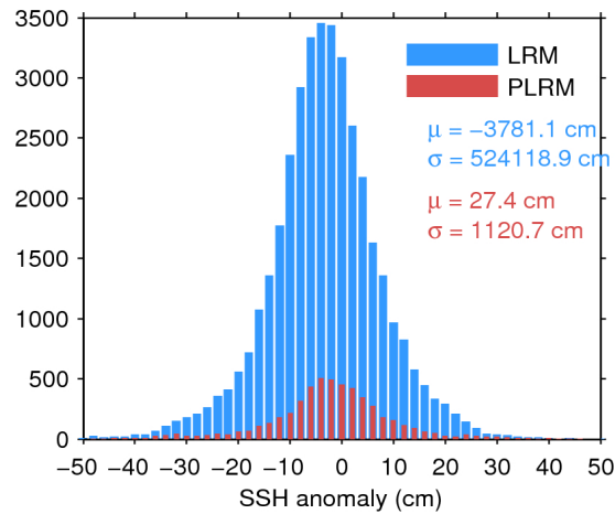
Figure 7. Histogram of flag-valid SSH anomaly over oceans and lakes for LRM (blue) and PLRM (red) for 21/12/2015. The mean ( \mu ) and standard deviation ( \sigma ) are also shown. Note that values outside [-50 50] cm are excluded from the histogram for the sake of readability but not from the computation of \mu and \sigma .
