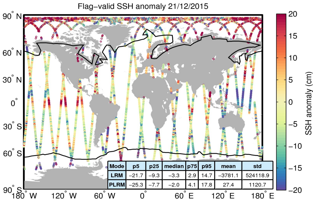
Figure 5. Geographical distribution of flag-valid 1-Hz SSH anomaly data over oceans and lakes for 21/12/2015. The statistical values shown in the table refer to the SSH anomaly in cm and are calculated separately for LRM and PLRM regions. Measurements taken over polar polygons have been excluded from the computation of the statistical values. The black lines mark the outer limit of the Arctic and Antarctic polar polygons.
