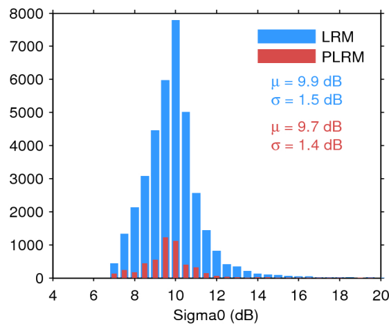
Figure 28. Histogram of science-valid sigma0 over oceans and lakes for LRM (blue) and PLRM (red) for 21/12/2015. The mean ( \mu ) and standard deviation ( \sigma ) are also shown. Note that values outside [4 20] dB are excluded from the histogram for the sake of readability but not from the computation of \mu and \sigma .
