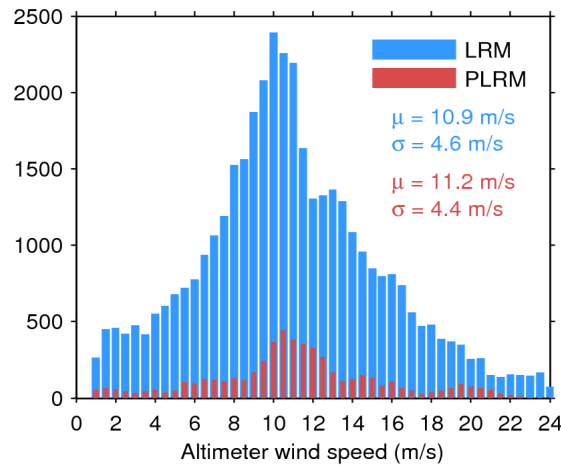
Figure 33. Histogram of flag-valid wind over oceans and lakes for LRM (blue) and PLRM (red) for 21/12/2015. The mean ( \mu ) and standard deviation ( \sigma ) are also shown. Note that values larger than 24 m/s are excluded from the histogram for the sake of readability but not from the computation of \mu and \sigma .
