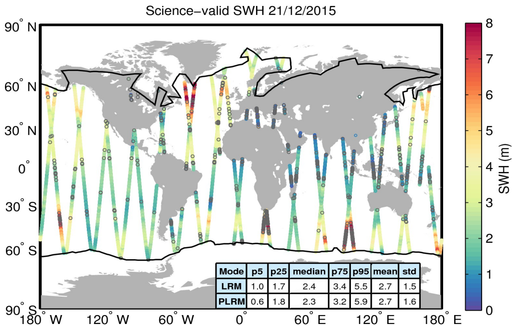
Figure 19. Geographical distribution of science-valid SWH data over oceans and lakes for 21/12/2015. The statistical values shown in the table refer to the SWH in m and are calculated separately for LRM and PLRM regions. The black lines mark the outer limit of the Arctic and Antarctic polar polygons. Gray circles denote records that have been rejected based on the editing criteria described in Table 3.
