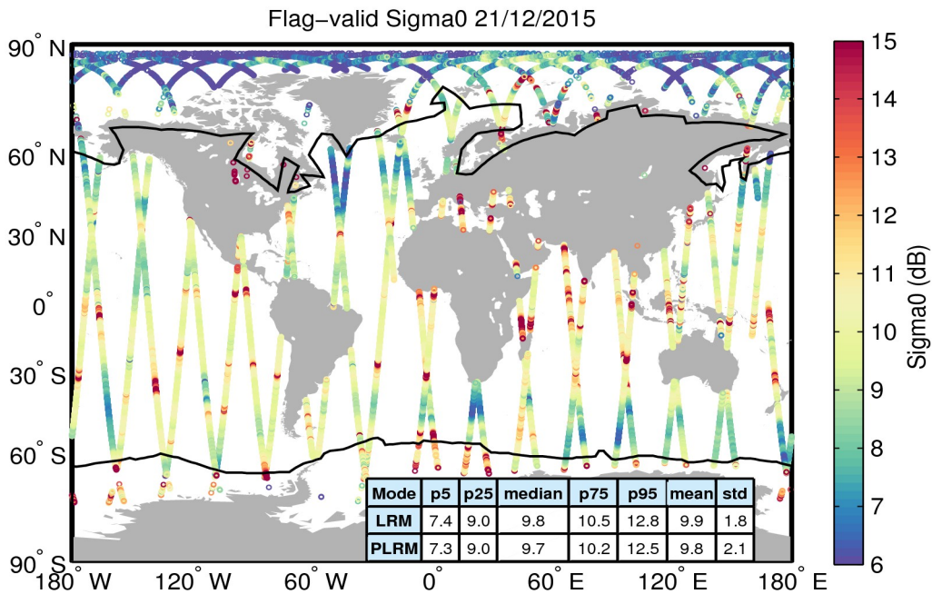
Figure 23. Geographical distribution of flag-valid sigma0 data over oceans and lakes for 21/12/2015. The statistical values shown in the table refer to the sigma0 in dB and are calculated separately for LRM and PLRM regions. Measurements taken over polar polygons have been excluded from the computation of the statistical values. The black lines mark the outer limit of the Arctic and Antarctic polar polygons.
