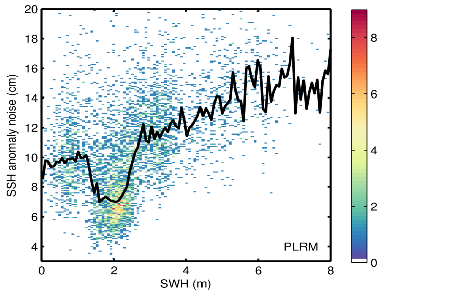
Figure 9. 2D histogram showing flag-valid SSH anomaly noise as a function of SWH for LRM (top) and PLRM (bottom) for 21/12/2015. The black line denotes the median SSH anomaly noise as a function of SWH.
