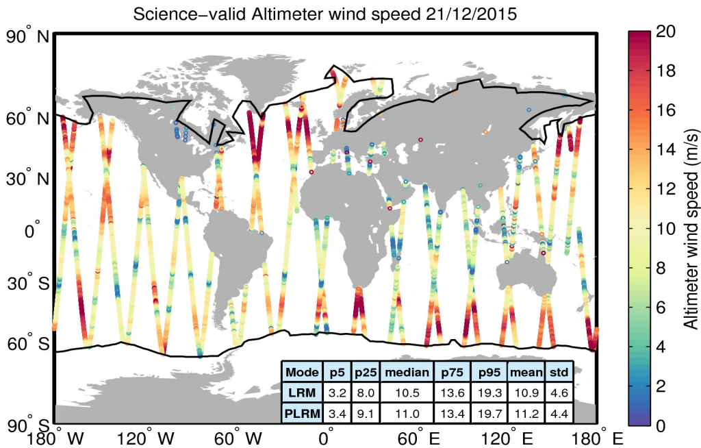
Figure 34. Geographical distribution of science-valid wind data over oceans and lakes for 21/12/2015. The statistical values shown in the table refer to the wind in m/s and are calculated separately for LRM and PLRM regions. The black lines mark the outer limit of the Arctic and Antarctic polar polygons. Gray circles denote records that have been rejected based on the editing criteria described in Table 5.
