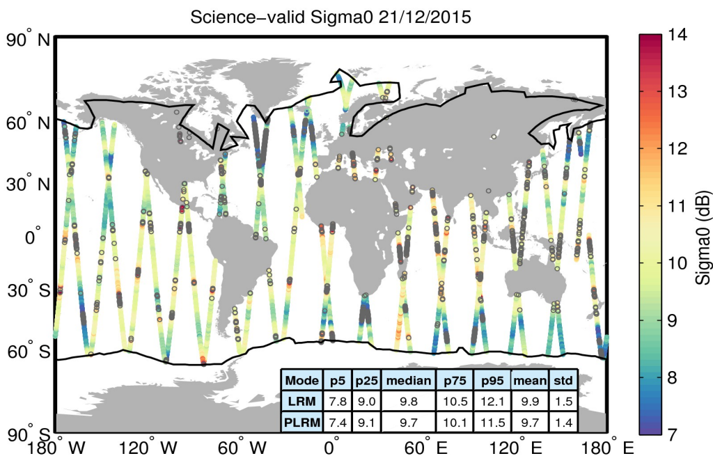
Figure 27. Geographical distribution of science-valid sigma0 data over oceans and lakes for 21/12/2015. The statistical values shown in the table refer to the sigma0 in dB and are calculated separately for LRM and PLRM regions. The black lines mark the outer limit of the Arctic and Antarctic polar polygons. Gray circles denote records that have been rejected based on the editing criteria described in Table 4.
