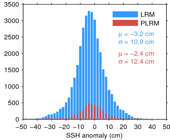
Figure 11. Histogram of science-valid SSH anomaly over oceans and lakes for LRM (blue) and PLRM (red) for 21/12/2015. The mean ( \mu ) and standard deviation ( \sigma ) are also shown. Note that values outside [-50 50] cm are excluded from the histogram for the sake of readability but not from the computation of \mu and \sigma .
