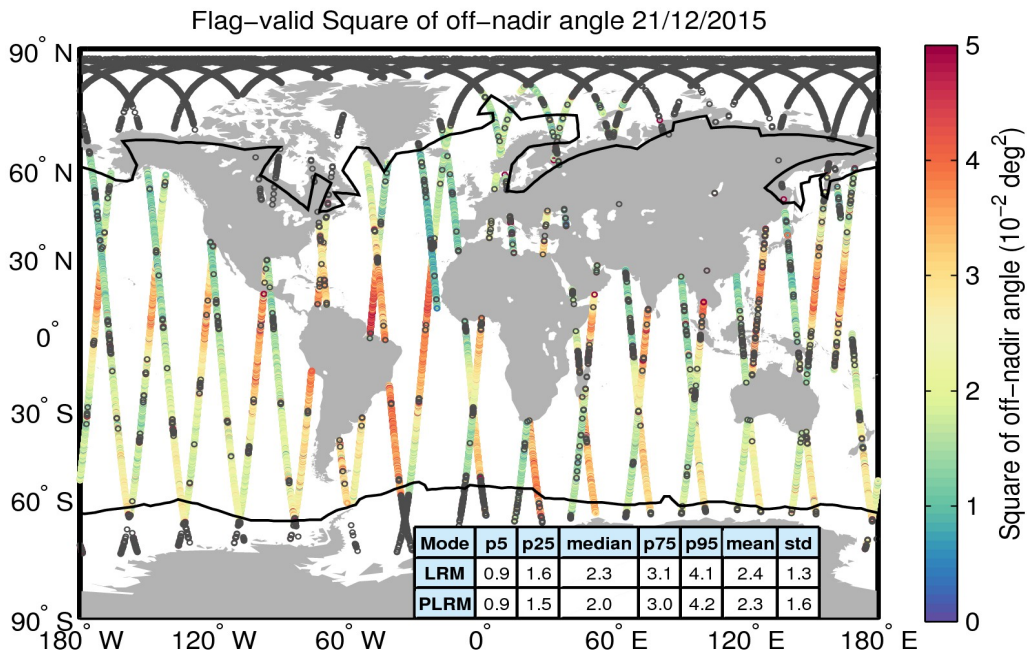
Figure 37. Geographical distribution of flag-valid mispointing data over oceans and lakes for 21/12/2015. The statistical values shown in the table refer to the mispointing in 10^{-2} deg 2 and are calculated separately for LRM and PLRM regions. Measurements taken over polar polygons have been excluded from the computation of the statistical values. The black lines mark the outer limit of the Arctic and Antarctic polar polygons. Gray circles denote negative values.
