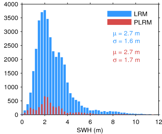
Figure 17. Histogram of flag-valid SWH over oceans and lakes for LRM (blue) and PLRM (red) for 21/12/2015. The mean ( \mu ) and standard deviation ( \sigma ) are also shown. Note that values larger than 12 m are excluded from the histogram for the sake of readability but not from the computation of \mu and \sigma .
