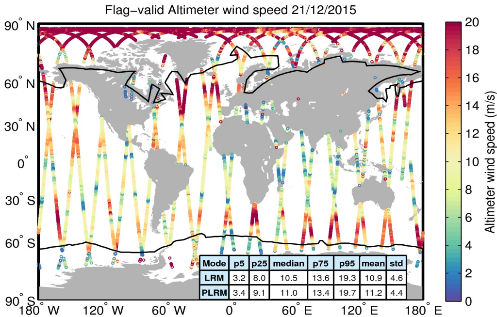
Figure 31. Geographical distribution of flag-valid wind data over oceans and lakes for 21/12/2015. The statistical values shown in the table refer to the wind in m/s and are calculated separately for LRM and PLRM regions. Measurements taken over polar polygons have been excluded from the computation of the statistical values. The black lines mark the outer limit of the Arctic and Antarctic polar polygons.
