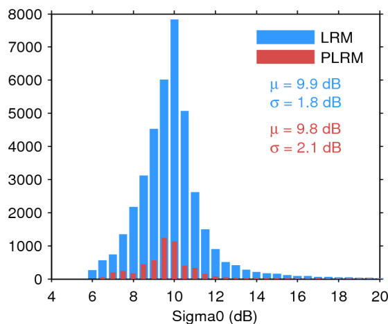
Figure 25. Histogram of flag-valid sigma0 over oceans and lakes for LRM (blue) and PLRM (red) for 21/12/2015. The mean ( \mu ) and standard deviation ( \sigma ) are also shown. Note that values outside [4 20] dB are excluded from the histogram for the sake of readability but not from the computation of \mu and \sigma .
