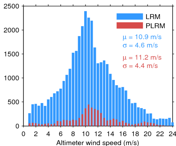
Figure 35. Histogram of science-valid wind over oceans and lakes for LRM (blue) and PLRM (red) for 21/12/2015. The mean ( \mu ) and standard deviation ( \sigma ) are also shown. Note that values larger than 24 m/s are excluded from the histogram for the sake of readability but not from the computation of \mu and \sigma .
