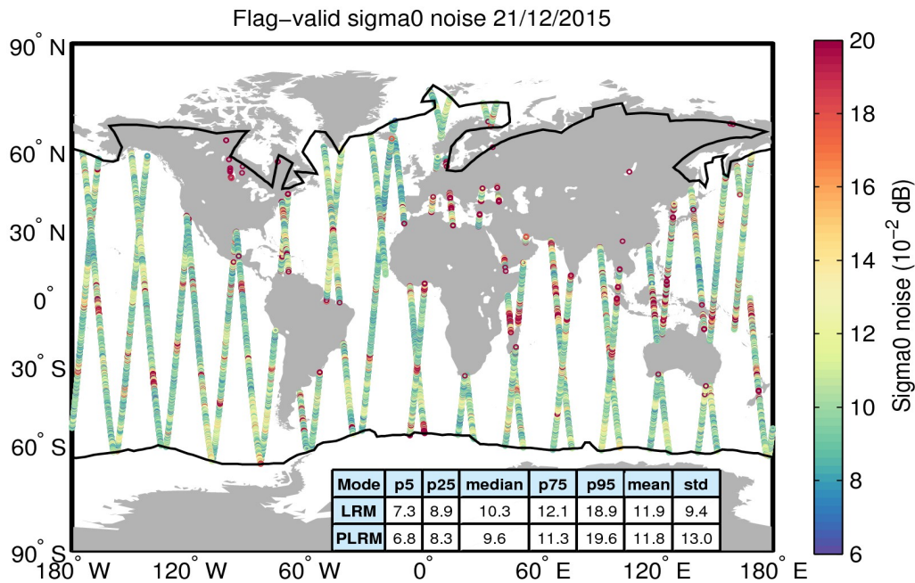
Figure 26. Geographical distribution of flag-valid 20-Hz sigma0 measurement noise over oceans and lakes for 21/12/2015. The statistical values shown in the table refer to the sigma0 noise and are calculated separately for LRM and PLRM regions. Measurements taken over polar polygons have been excluded from the computation of the statistical values. The black lines mark the outer limit of the Arctic and Antarctic polar polygons.
