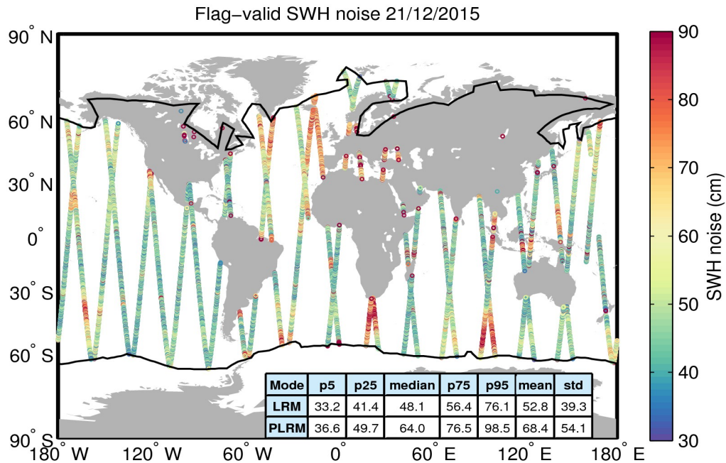
Figure 18. Geographical distribution of flag-valid 20-Hz SWH measurement noise over oceans and lakes for 21/12/2015. The statistical values shown in the table refer to the SWH noise and are calculated separately for LRM and PLRM regions. Measurements taken over polar polygons have been excluded from the computation of the statistical values. The black lines mark the outer limit of the Arctic and Antarctic polar polygons.
