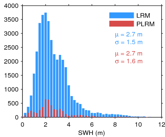
Figure 20. Histogram of science-valid SWH over oceans and lakes for LRM (blue) and PLRM (red) for 21/12/2015. The mean ( \mu ) and standard deviation ( \sigma ) are also shown. Note that values larger than 12 m are excluded from the histogram for the sake of readability but not from the computation of \mu and \sigma .
