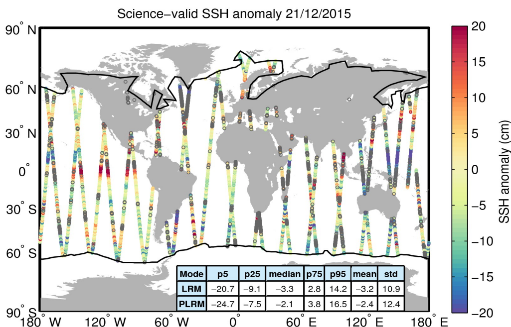
Figure 10. Geographical distribution of science-valid SSH anomaly data over oceans and lakes for 21/12/2015. The statistical values shown in the table refer to the SSH anomaly in cm and are calculated separately for LRM and PLRM regions. The black lines mark the outer limit of the Arctic and Antarctic polar polygons. Gray circles denote records that have been rejected based on the editing criteria described in Table 2.
