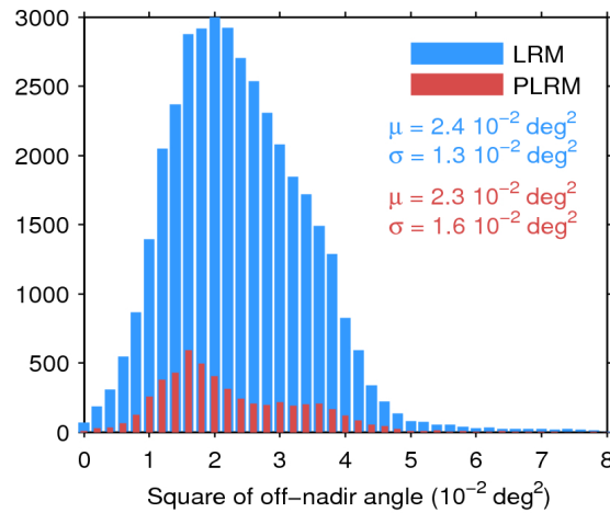
Figure 39. Histogram of flag-valid mispointing over oceans and lakes for LRM (blue) and PLRM (red) for 21/12/2015. Only positive values have been considered. The mean ( \mu ) and standard deviation ( \sigma ) are also shown. Note that values larger than 8 \cdot 10^{-2} \text{ deg}^2 are excluded from the histogram for the sake of readability but not from the computation of \mu and \sigma .
