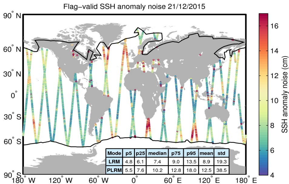
Figure 8. Geographical distribution of flag-valid 20-Hz SSH anomaly measurement noise over oceans and lakes for 21/12/2015. The statistical values shown in the table refer to the SSH anomaly noise and are calculated separately for LRM and PLRM regions. Measurements taken over polar polygons have been excluded from the computation of the statistical values. The black lines mark the outer limit of the Arctic and Antarctic polar polygons.
