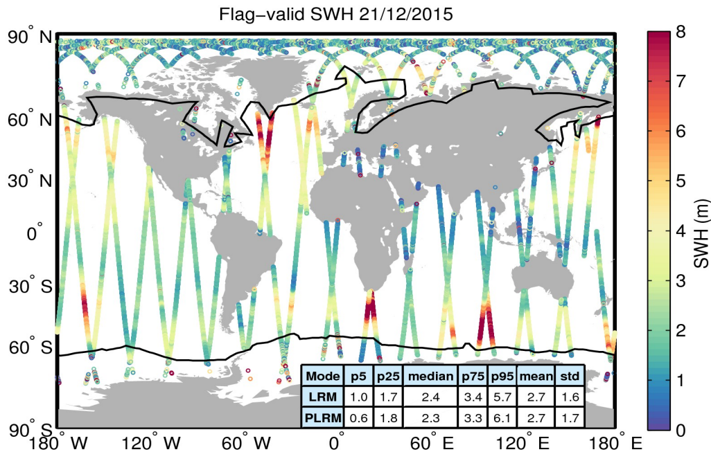
Figure 15. Geographical distribution of flag-valid SWH data over oceans and lakes for 21/12/2015. The statistical values shown in the table refer to the SWH in m and are calculated separately for LRM and PLRM regions. Measurements taken over polar polygons have been excluded from the computation of the statistical values. The black lines mark the outer limit of the Arctic and Antarctic polar polygons.
