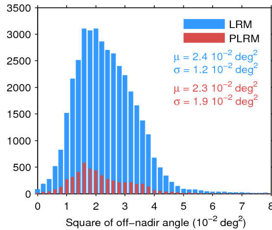
Figure 39. Histogram of flag-valid mispointing over oceans and lakes for LRM (blue) and PLRM (red) for 19/12/2015. Only positive values have been considered. The mean ( \mu ) and standard deviation ( \sigma ) are also shown. Note that values larger than 8 \cdot 10^{-2} \text{ deg}^2 are excluded from the histogram for the sake of readability but not from the computation of \mu and \sigma .
