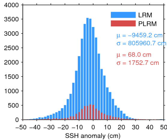
Figure 7. Histogram of flag-valid SSH anomaly over oceans and lakes for LRM (blue) and PLRM (red) for 19/12/2015. The mean ( \mu ) and standard deviation ( \sigma ) are also shown. Note that values outside [-50 \ 50] cm are excluded from the histogram for the sake of readability but not from the computation of \mu and \sigma .
