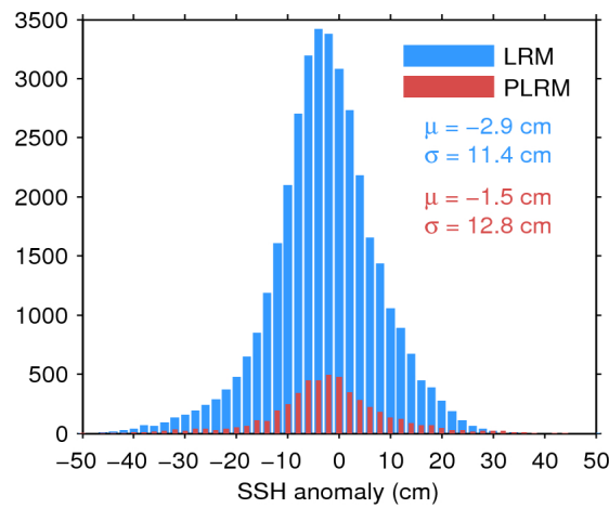
Figure 11. Histogram of science-valid SSH anomaly over oceans and lakes for LRM (blue) and PLRM (red) for 19/12/2015. The mean ( \mu ) and standard deviation ( \sigma ) are also shown. Note that values outside [-50 50] cm are excluded from the histogram for the sake of readability but not from the computation of \mu and \sigma .
