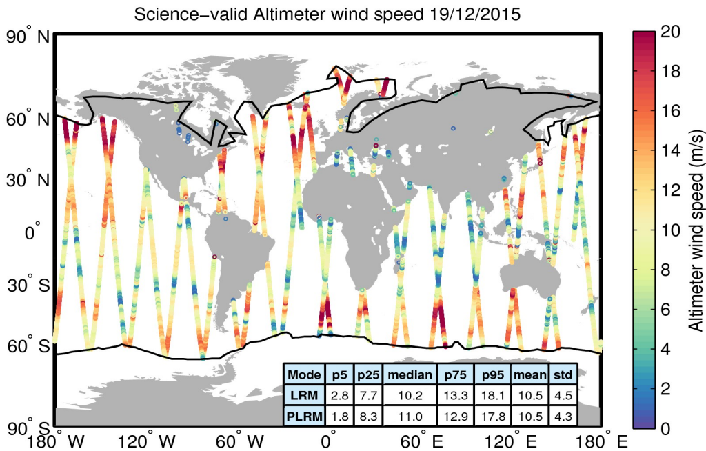
Figure 34. Geographical distribution of science-valid wind data over oceans and lakes for 19/12/2015. The statistical values shown in the table refer to the wind in m/s and are calculated separately for LRM and PLRM regions. The black lines mark the outer limit of the Arctic and Antarctic polar polygons. Gray circles denote records that have been rejected based on the editing criteria described in Table 5.
