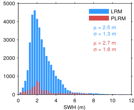
Figure 17. Histogram of flag-valid SWH over oceans and lakes for LRM (blue) and PLRM (red) for 19/12/2015. The mean ( \mu ) and standard deviation ( \sigma ) are also shown. Note that values larger than 12 m are excluded from the histogram for the sake of readability but not from the computation of \mu and \sigma .
