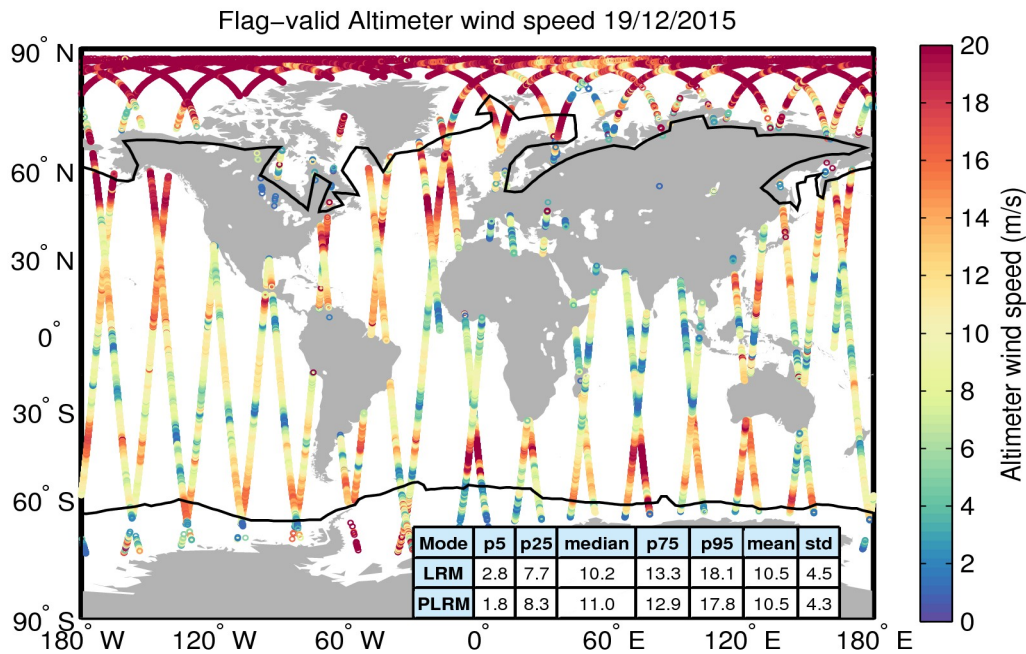
Figure 31. Geographical distribution of flag-valid wind data over oceans and lakes for 19/12/2015. The statistical values shown in the table refer to the wind in m/s and are calculated separately for LRM and PLRM regions. Measurements taken over polar polygons have been excluded from the computation of the statistical values. The black lines mark the outer limit of the Arctic and Antarctic polar polygons.
