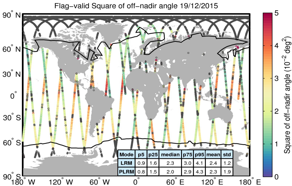
Figure 37. Geographical distribution of flag-valid mispointing data over oceans and lakes for 19/12/2015. The statistical values shown in the table refer to the mispointing in 10^{-2} deg 2 and are calculated separately for LRM and PLRM regions. Measurements taken over polar polygons have been excluded from the computation of the statistical values. The black lines mark the outer limit of the Arctic and Antarctic polar polygons. Gray circles denote negative values.
