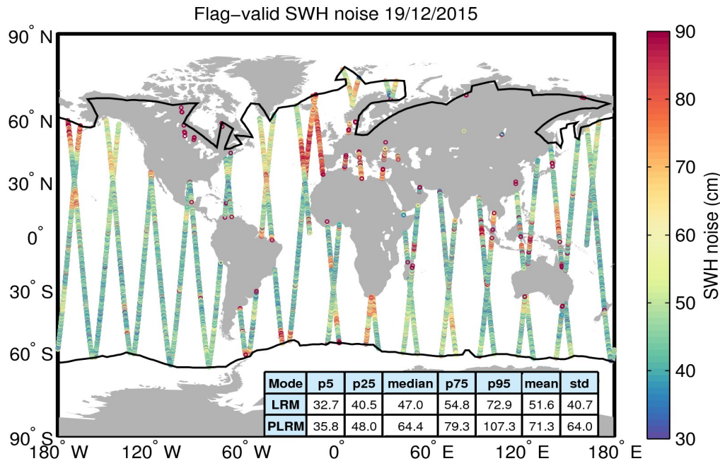
Figure 18. Geographical distribution of flag-valid 20-Hz SWH measurement noise over oceans and lakes for 19/12/2015. The statistical values shown in the table refer to the SWH noise and are calculated separately for LRM and PLRM regions. Measurements taken over polar polygons have been excluded from the computation of the statistical values. The black lines mark the outer limit of the Arctic and Antarctic polar polygons.
