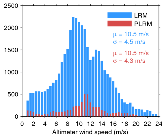
Figure 35. Histogram of science-valid wind over oceans and lakes for LRM (blue) and PLRM (red) for 19/12/2015. The mean ( \mu ) and standard deviation ( \sigma ) are also shown. Note that values larger than 24 m/s are excluded from the histogram for the sake of readability but not from the computation of \mu and \sigma .
