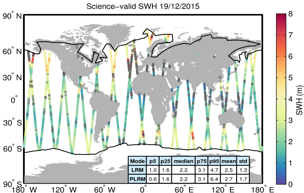
Figure 19. Geographical distribution of science-valid SWH data over oceans and lakes for 19/12/2015. The statistical values shown in the table refer to the SWH in m and are calculated separately for LRM and PLRM regions. The black lines mark the outer limit of the Arctic and Antarctic polar polygons. Gray circles denote records that have been rejected based on the editing criteria described in Table 3.
