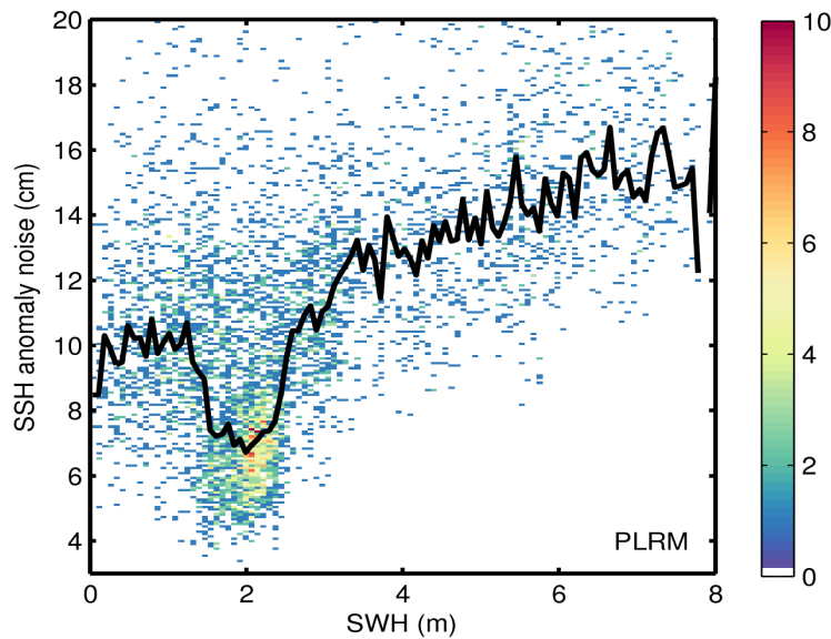
Figure 9. 2D histogram showing flag-valid SSH anomaly noise as a function of SWH for LRM (top) and PLRM (bottom) for 19/12/2015. The black line denotes the median SSH anomaly noise as a function of SWH.
