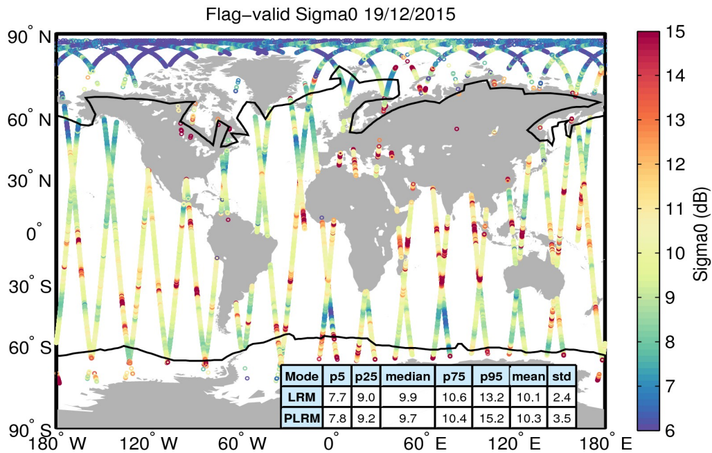
Figure 23. Geographical distribution of flag-valid sigma0 data over oceans and lakes for 19/12/2015. The statistical values shown in the table refer to the sigma0 in dB and are calculated separately for LRM and PLRM regions. Measurements taken over polar polygons have been excluded from the computation of the statistical values. The black lines mark the outer limit of the Arctic and Antarctic polar polygons.
