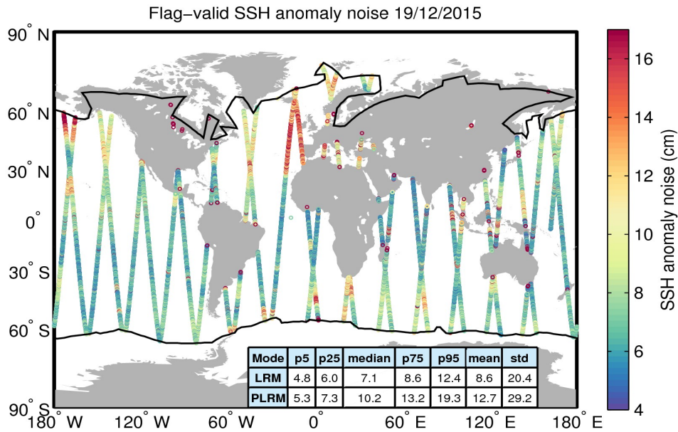
Figure 8. Geographical distribution of flag-valid 20-Hz SSH anomaly measurement noise over oceans and lakes for 19/12/2015. The statistical values shown in the table refer to the SSH anomaly noise and are calculated separately for LRM and PLRM regions. Measurements taken over polar polygons have been excluded from the computation of the statistical values. The black lines mark the outer limit of the Arctic and Antarctic polar polygons.
