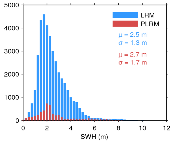
Figure 20. Histogram of science-valid SWH over oceans and lakes for LRM (blue) and PLRM (red) for 19/12/2015. The mean ( \mu ) and standard deviation ( \sigma ) are also shown. Note that values larger than 12 m are excluded from the histogram for the sake of readability but not from the computation of \mu and \sigma .
