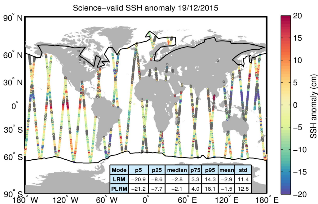
Figure 10. Geographical distribution of science-valid SSH anomaly data over oceans and lakes for 19/12/2015. The statistical values shown in the table refer to the SSH anomaly in cm and are calculated separately for LRM and PLRM regions. The black lines mark the outer limit of the Arctic and Antarctic polar polygons. Gray circles denote records that have been rejected based on the editing criteria described in Table 2.
