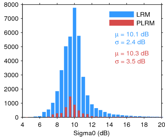
Figure 25. Histogram of flag-valid sigma0 over oceans and lakes for LRM (blue) and PLRM (red) for 19/12/2015. The mean ( \mu ) and standard deviation ( \sigma ) are also shown. Note that values outside [4 20] dB are excluded from the histogram for the sake of readability but not from the computation of \mu and \sigma .
