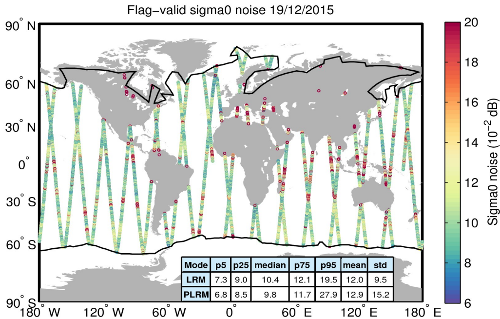
Figure 26. Geographical distribution of flag-valid 20-Hz sigma0 measurement noise over oceans and lakes for 19/12/2015. The statistical values shown in the table refer to the sigma0 noise and are calculated separately for LRM and PLRM regions. Measurements taken over polar polygons have been excluded from the computation of the statistical values. The black lines mark the outer limit of the Arctic and Antarctic polar polygons.
