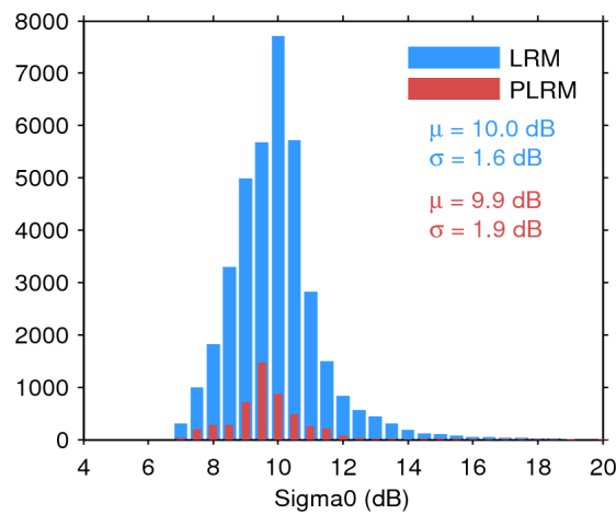
Figure 28. Histogram of science-valid sigma0 over oceans and lakes for LRM (blue) and PLRM (red) for 19/12/2015. The mean ( \mu ) and standard deviation ( \sigma ) are also shown. Note that values outside [4 20] dB are excluded from the histogram for the sake of readability but not from the computation of \mu and \sigma .
