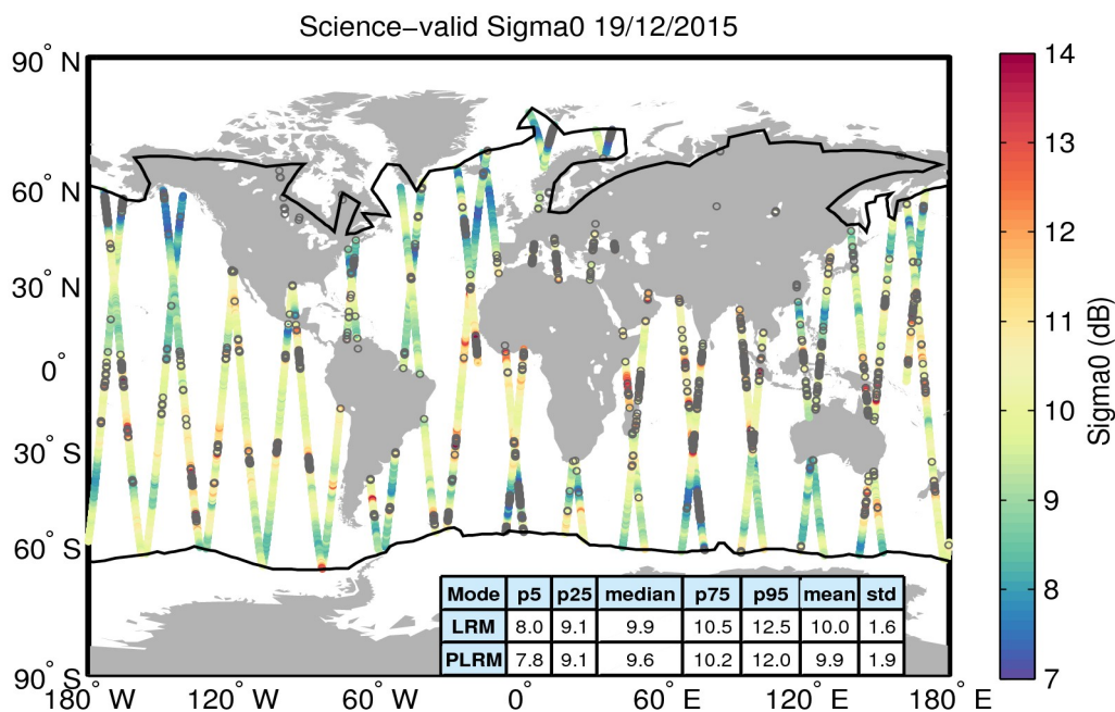
Figure 27. Geographical distribution of science-valid sigma0 data over oceans and lakes for 19/12/2015. The statistical values shown in the table refer to the sigma0 in dB and are calculated separately for LRM and PLRM regions. The black lines mark the outer limit of the Arctic and Antarctic polar polygons. Gray circles denote records that have been rejected based on the editing criteria described in Table 4.
