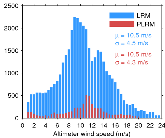
Figure 33. Histogram of flag-valid wind over oceans and lakes for LRM (blue) and PLRM (red) for 19/12/2015. The mean ( \mu ) and standard deviation ( \sigma ) are also shown. Note that values larger than 24 m/s are excluded from the histogram for the sake of readability but not from the computation of \mu and \sigma .
