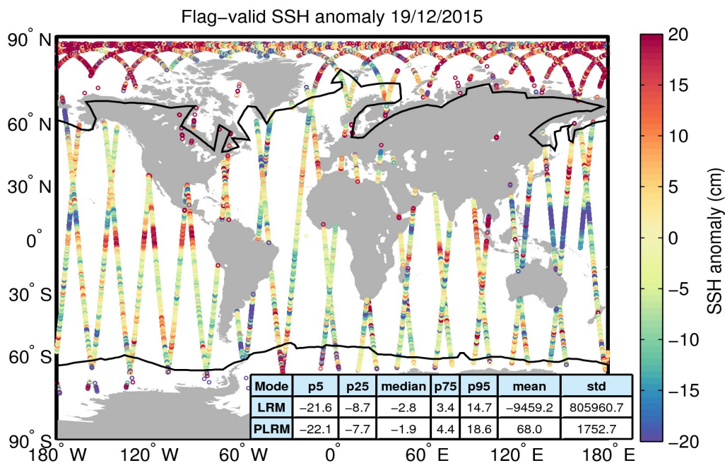
Figure 5. Geographical distribution of flag-valid 1-Hz SSH anomaly data over oceans and lakes for 19/12/2015. The statistical values shown in the table refer to the SSH anomaly in cm and are calculated separately for LRM and PLRM regions. Measurements taken over polar polygons have been excluded from the computation of the statistical values. The black lines mark the outer limit of the Arctic and Antarctic polar polygons.
