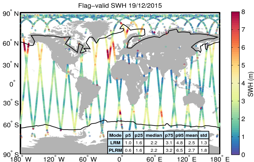
Figure 15. Geographical distribution of flag-valid SWH data over oceans and lakes for 19/12/2015. The statistical values shown in the table refer to the SWH in m and are calculated separately for LRM and PLRM regions. Measurements taken over polar polygons have been excluded from the computation of the statistical values. The black lines mark the outer limit of the Arctic and Antarctic polar polygons.
