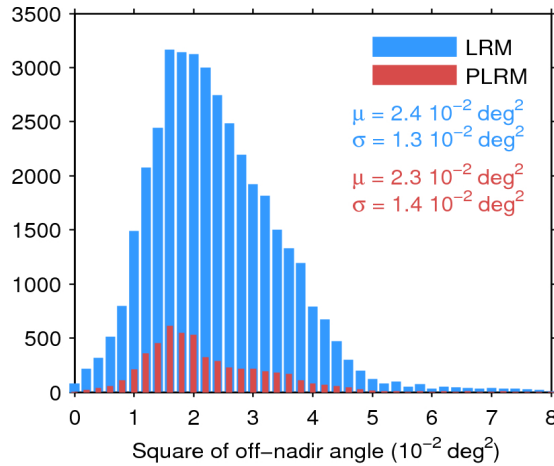
Figure 39. Histogram of flag-valid mispointing over oceans and lakes for LRM (blue) and PLRM (red) for 17/12/2015. Only positive values have been considered. The mean ( \mu ) and standard deviation ( \sigma ) are also shown. Note that values larger than 8 \cdot 10^{-2} \text{ deg}^2 are excluded from the histogram for the sake of readability but not from the computation of \mu and \sigma .
