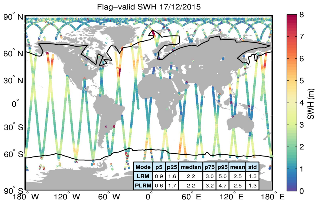
Figure 15. Geographical distribution of flag-valid SWH data over oceans and lakes for 17/12/2015. The statistical values shown in the table refer to the SWH in m and are calculated separately for LRM and PLRM regions. Measurements taken over polar polygons have been excluded from the computation of the statistical values. The black lines mark the outer limit of the Arctic and Antarctic polar polygons.
