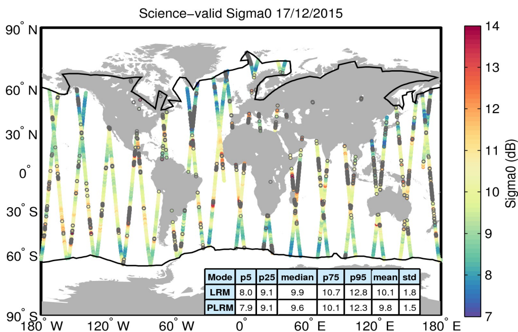
Figure 27. Geographical distribution of science-valid sigma0 data over oceans and lakes for 17/12/2015. The statistical values shown in the table refer to the sigma0 in dB and are calculated separately for LRM and PLRM regions. The black lines mark the outer limit of the Arctic and Antarctic polar polygons. Gray circles denote records that have been rejected based on the editing criteria described in Table 4.
