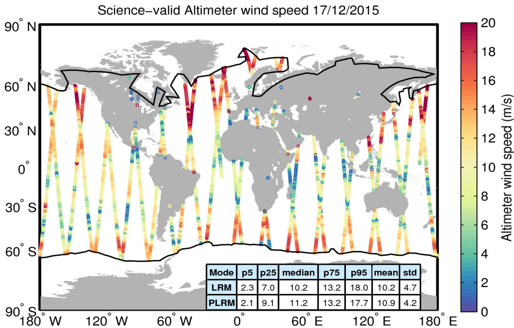
Figure 34. Geographical distribution of science-valid wind data over oceans and lakes for 17/12/2015. The statistical values shown in the table refer to the wind in m/s and are calculated separately for LRM and PLRM regions. The black lines mark the outer limit of the Arctic and Antarctic polar polygons. Gray circles denote records that have been rejected based on the editing criteria described in Table 5.
