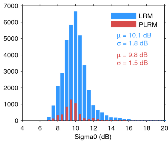
Figure 28. Histogram of science-valid sigma0 over oceans and lakes for LRM (blue) and PLRM (red) for 17/12/2015. The mean ( \mu ) and standard deviation ( \sigma ) are also shown. Note that values outside [4 20] dB are excluded from the histogram for the sake of readability but not from the computation of \mu and \sigma .
