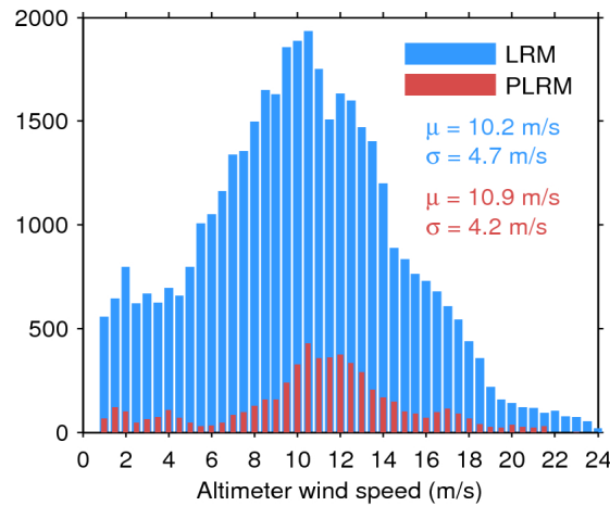
Figure 33. Histogram of flag-valid wind over oceans and lakes for LRM (blue) and PLRM (red) for 17/12/2015. The mean ( \mu ) and standard deviation ( \sigma ) are also shown. Note that values larger than 24 m/s are excluded from the histogram for the sake of readability but not from the computation of \mu and \sigma .
