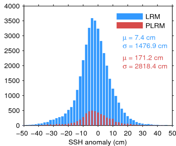
Figure 7. Histogram of flag-valid SSH anomaly over oceans and lakes for LRM (blue) and PLRM (red) for 17/12/2015. The mean ( \mu ) and standard deviation ( \sigma ) are also shown. Note that values outside [-50 50] cm are excluded from the histogram for the sake of readability but not from the computation of \mu and \sigma .
