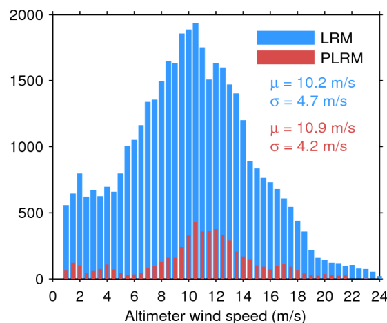
Figure 35. Histogram of science-valid wind over oceans and lakes for LRM (blue) and PLRM (red) for 17/12/2015. The mean ( \mu ) and standard deviation ( \sigma ) are also shown. Note that values larger than 24 m/s are excluded from the histogram for the sake of readability but not from the computation of \mu and \sigma .
