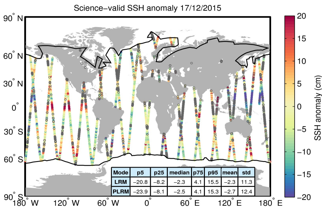
Figure 10. Geographical distribution of science-valid SSH anomaly data over oceans and lakes for 17/12/2015. The statistical values shown in the table refer to the SSH anomaly in cm and are calculated separately for LRM and PLRM regions. The black lines mark the outer limit of the Arctic and Antarctic polar polygons. Gray circles denote records that have been rejected based on the editing criteria described in Table 2.
