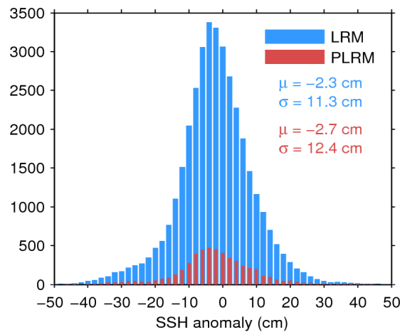
Figure 11. Histogram of science-valid SSH anomaly over oceans and lakes for LRM (blue) and PLRM (red) for 17/12/2015. The mean ( \mu ) and standard deviation ( \sigma ) are also shown. Note that values outside [-50 50] cm are excluded from the histogram for the sake of readability but not from the computation of \mu and \sigma .
