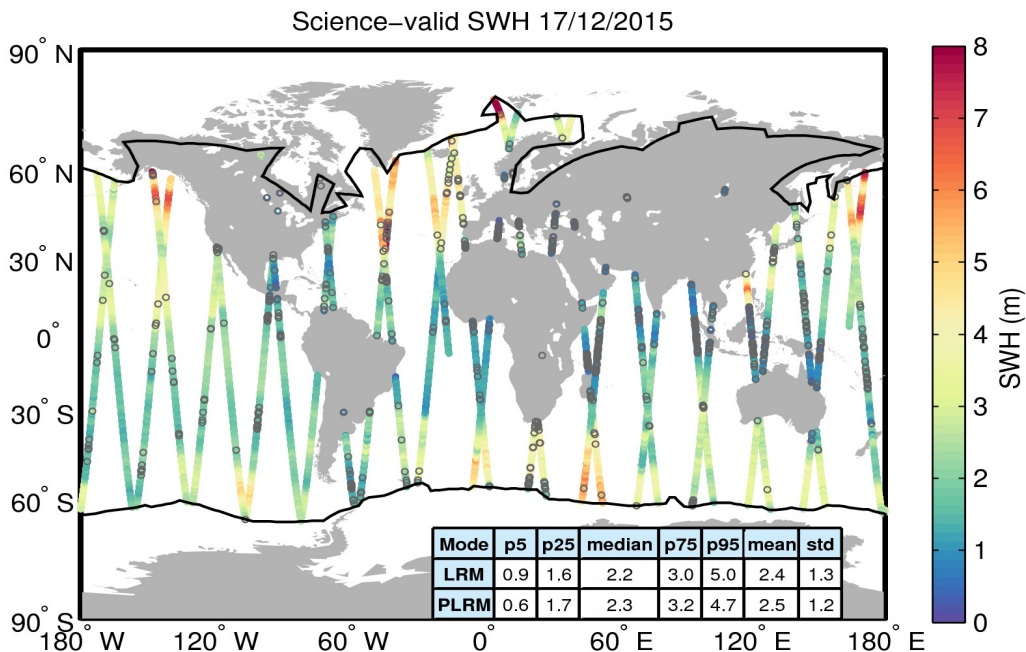
Figure 19. Geographical distribution of science-valid SWH data over oceans and lakes for 17/12/2015. The statistical values shown in the table refer to the SWH in m and are calculated separately for LRM and PLRM regions. The black lines mark the outer limit of the Arctic and Antarctic polar polygons. Gray circles denote records that have been rejected based on the editing criteria described in Table 3.
