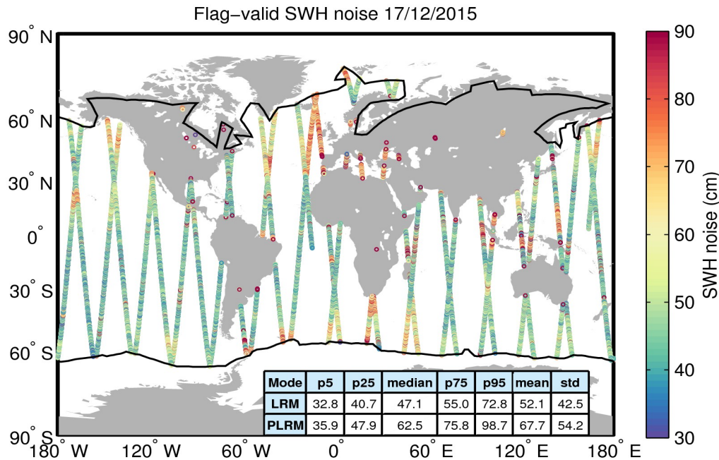
Figure 18. Geographical distribution of flag-valid 20-Hz SWH measurement noise over oceans and lakes for 17/12/2015. The statistical values shown in the table refer to the SWH noise and are calculated separately for LRM and PLRM regions. Measurements taken over polar polygons have been excluded from the computation of the statistical values. The black lines mark the outer limit of the Arctic and Antarctic polar polygons.
