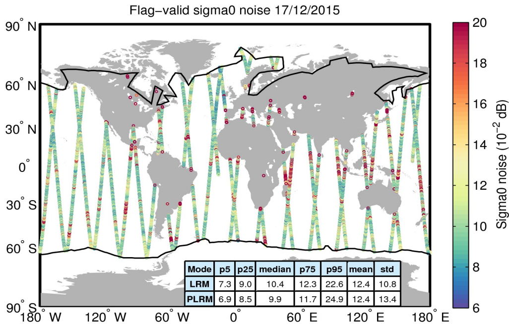
Figure 26. Geographical distribution of flag-valid 20-Hz sigma0 measurement noise over oceans and lakes for 17/12/2015. The statistical values shown in the table refer to the sigma0 noise and are calculated separately for LRM and PLRM regions. Measurements taken over polar polygons have been excluded from the computation of the statistical values. The black lines mark the outer limit of the Arctic and Antarctic polar polygons.
