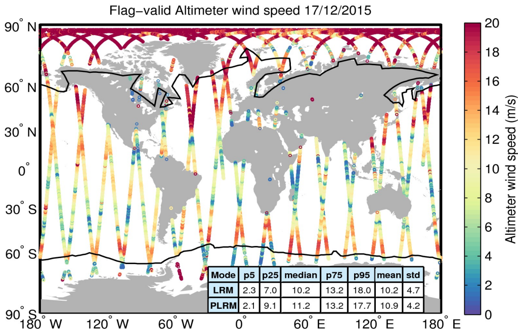
Figure 31. Geographical distribution of flag-valid wind data over oceans and lakes for 17/12/2015. The statistical values shown in the table refer to the wind in m/s and are calculated separately for LRM and PLRM regions. Measurements taken over polar polygons have been excluded from the computation of the statistical values. The black lines mark the outer limit of the Arctic and Antarctic polar polygons.
