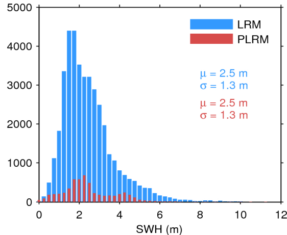
Figure 17. Histogram of flag-valid SWH over oceans and lakes for LRM (blue) and PLRM (red) for 17/12/2015. The mean ( \mu ) and standard deviation ( \sigma ) are also shown. Note that values larger than 12 m are excluded from the histogram for the sake of readability but not from the computation of \mu and \sigma .
