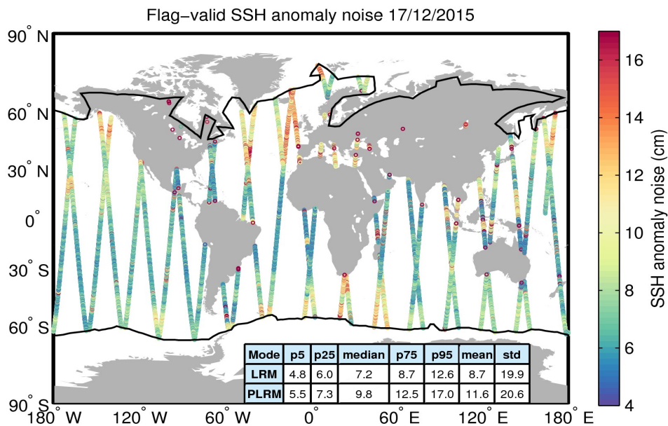
Figure 8. Geographical distribution of flag-valid 20-Hz SSH anomaly measurement noise over oceans and lakes for 17/12/2015. The statistical values shown in the table refer to the SSH anomaly noise and are calculated separately for LRM and PLRM regions. Measurements taken over polar polygons have been excluded from the computation of the statistical values. The black lines mark the outer limit of the Arctic and Antarctic polar polygons.
