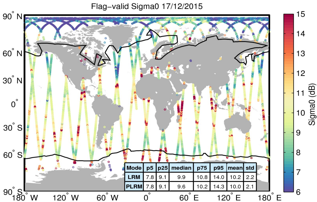
Figure 23. Geographical distribution of flag-valid sigma0 data over oceans and lakes for 17/12/2015. The statistical values shown in the table refer to the sigma0 in dB and are calculated separately for LRM and PLRM regions. Measurements taken over polar polygons have been excluded from the computation of the statistical values. The black lines mark the outer limit of the Arctic and Antarctic polar polygons.
