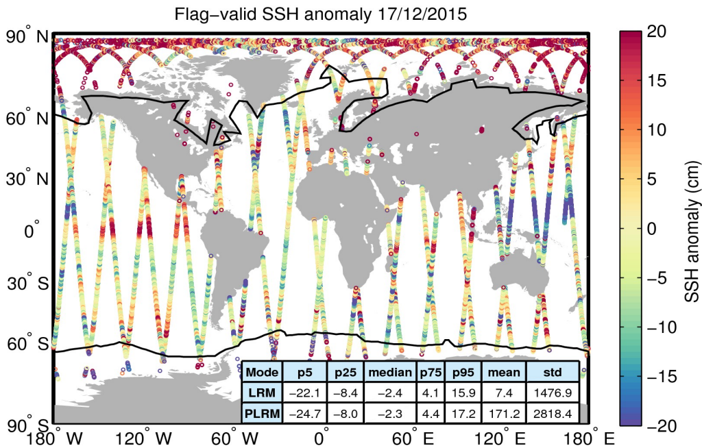
Figure 5. Geographical distribution of flag-valid 1-Hz SSH anomaly data over oceans and lakes for 17/12/2015. The statistical values shown in the table refer to the SSH anomaly in cm and are calculated separately for LRM and PLRM regions. Measurements taken over polar polygons have been excluded from the computation of the statistical values. The black lines mark the outer limit of the Arctic and Antarctic polar polygons.
