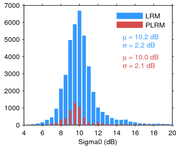
Figure 25. Histogram of flag-valid sigma0 over oceans and lakes for LRM (blue) and PLRM (red) for 17/12/2015. The mean ( \mu ) and standard deviation ( \sigma ) are also shown. Note that values outside [4 20] dB are excluded from the histogram for the sake of readability but not from the computation of \mu and \sigma .
