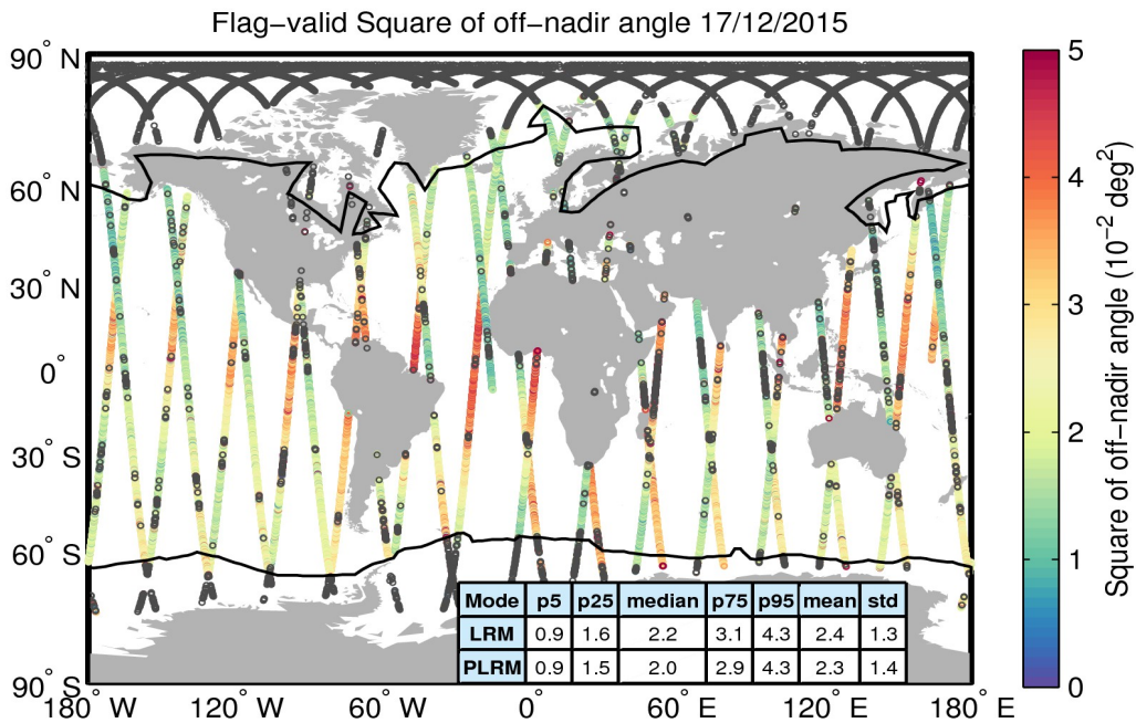
Figure 37. Geographical distribution of flag-valid mispointing data over oceans and lakes for 17/12/2015. The statistical values shown in the table refer to the mispointing in 10^{-2} deg 2 and are calculated separately for LRM and PLRM regions. Measurements taken over polar polygons have been excluded from the computation of the statistical values. The black lines mark the outer limit of the Arctic and Antarctic polar polygons. Gray circles denote negative values.
