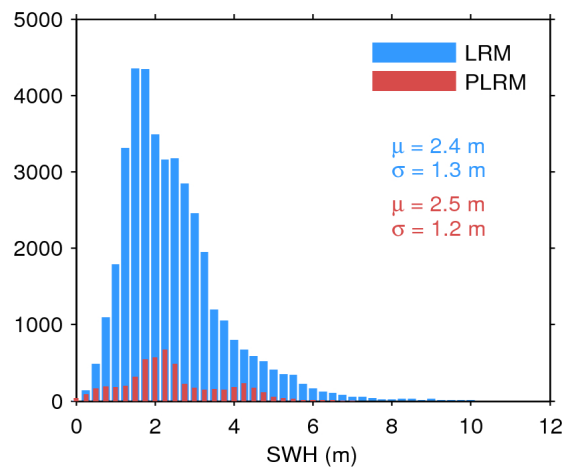
Figure 20. Histogram of science-valid SWH over oceans and lakes for LRM (blue) and PLRM (red) for 17/12/2015. The mean ( \mu ) and standard deviation ( \sigma ) are also shown. Note that values larger than 12 m are excluded from the histogram for the sake of readability but not from the computation of \mu and \sigma .
