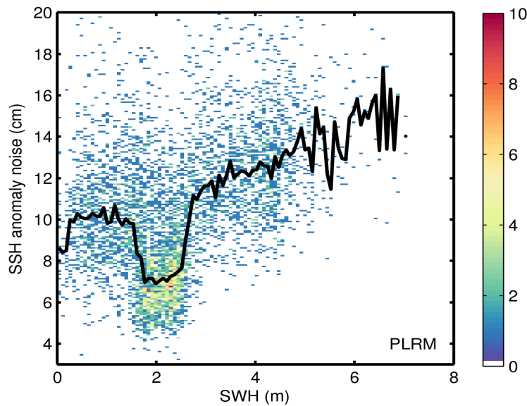
Figure 9. 2D histogram showing flag-valid SSH anomaly noise as a function of SWH for LRM (top) and PLRM (bottom) for 17/12/2015. The black line denotes the median SSH anomaly noise as a function of SWH.
