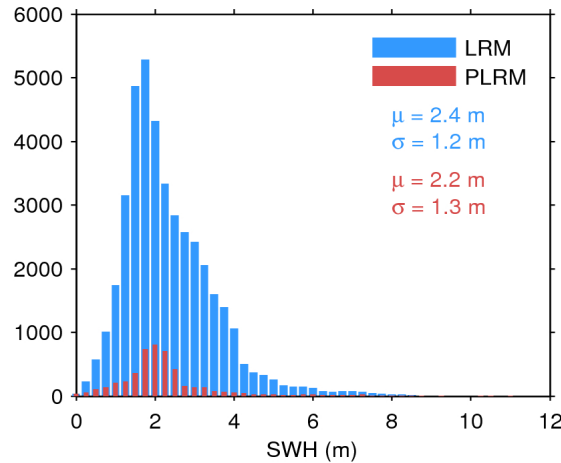
Figure 17. Histogram of flag-valid SWH over oceans and lakes for LRM (blue) and PLRM (red) for 16/12/2015. The mean ( \mu ) and standard deviation ( \sigma ) are also shown. Note that values larger than 12 m are excluded from the histogram for the sake of readability but not from the computation of \mu and \sigma .
