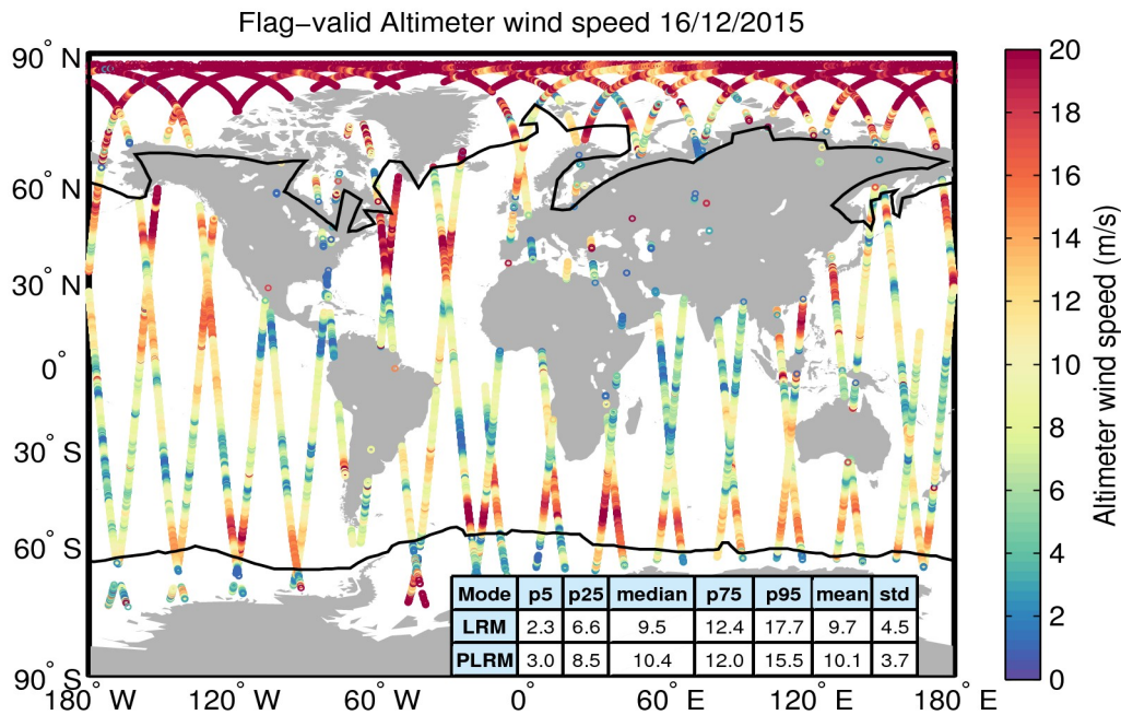
Figure 31. Geographical distribution of flag-valid wind data over oceans and lakes for 16/12/2015. The statistical values shown in the table refer to the wind in m/s and are calculated separately for LRM and PLRM regions. Measurements taken over polar polygons have been excluded from the computation of the statistical values. The black lines mark the outer limit of the Arctic and Antarctic polar polygons.
