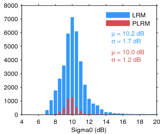
Figure 28. Histogram of science-valid sigma0 over oceans and lakes for LRM (blue) and PLRM (red) for 16/12/2015. The mean ( \mu ) and standard deviation ( \sigma ) are also shown. Note that values outside [4 20] dB are excluded from the histogram for the sake of readability but not from the computation of \mu and \sigma .
