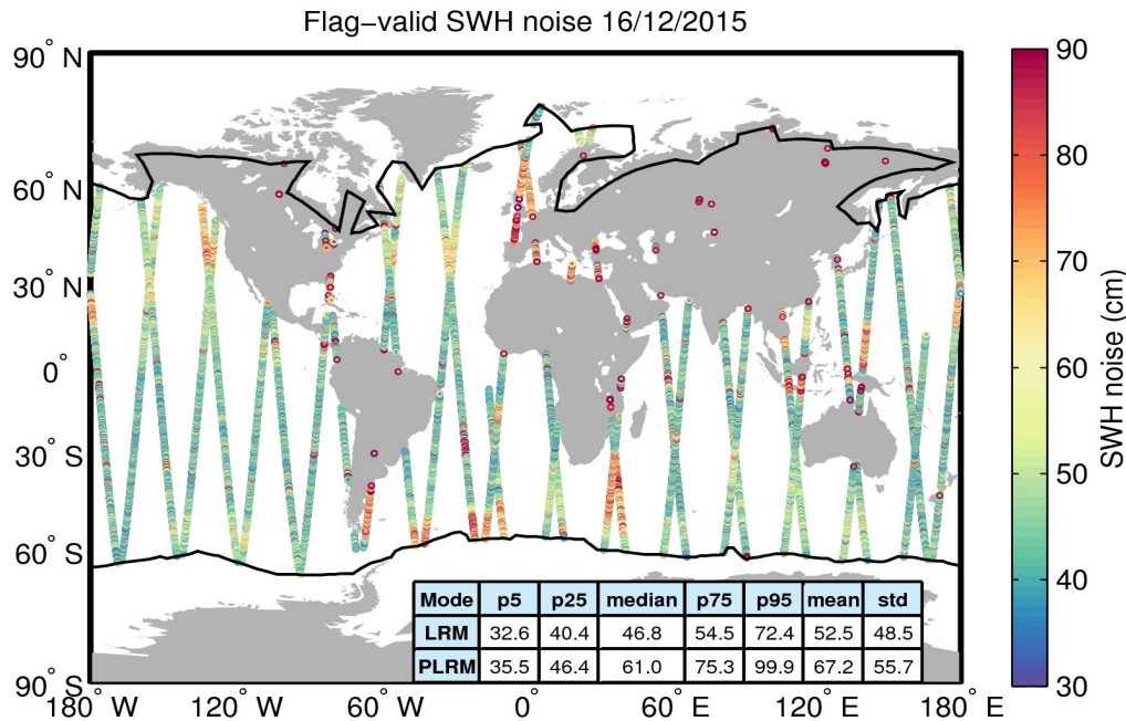
Figure 18. Geographical distribution of flag-valid 20-Hz SWH measurement noise over oceans and lakes for 16/12/2015. The statistical values shown in the table refer to the SWH noise and are calculated separately for LRM and PLRM regions. Measurements taken over polar polygons have been excluded from the computation of the statistical values. The black lines mark the outer limit of the Arctic and Antarctic polar polygons.
