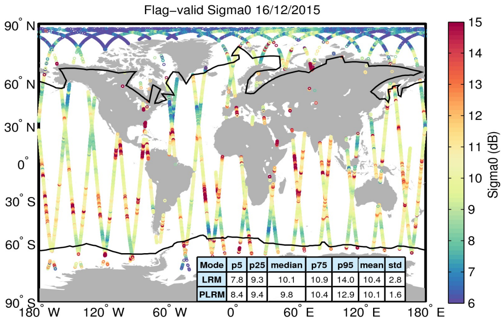
Figure 23. Geographical distribution of flag-valid sigma0 data over oceans and lakes for 16/12/2015. The statistical values shown in the table refer to the sigma0 in dB and are calculated separately for LRM and PLRM regions. Measurements taken over polar polygons have been excluded from the computation of the statistical values. The black lines mark the outer limit of the Arctic and Antarctic polar polygons.
