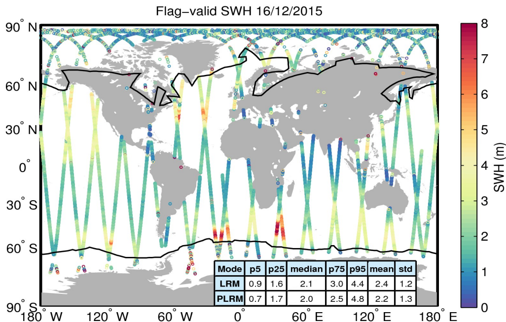
Figure 15. Geographical distribution of flag-valid SWH data over oceans and lakes for 16/12/2015. The statistical values shown in the table refer to the SWH in m and are calculated separately for LRM and PLRM regions. Measurements taken over polar polygons have been excluded from the computation of the statistical values. The black lines mark the outer limit of the Arctic and Antarctic polar polygons.
