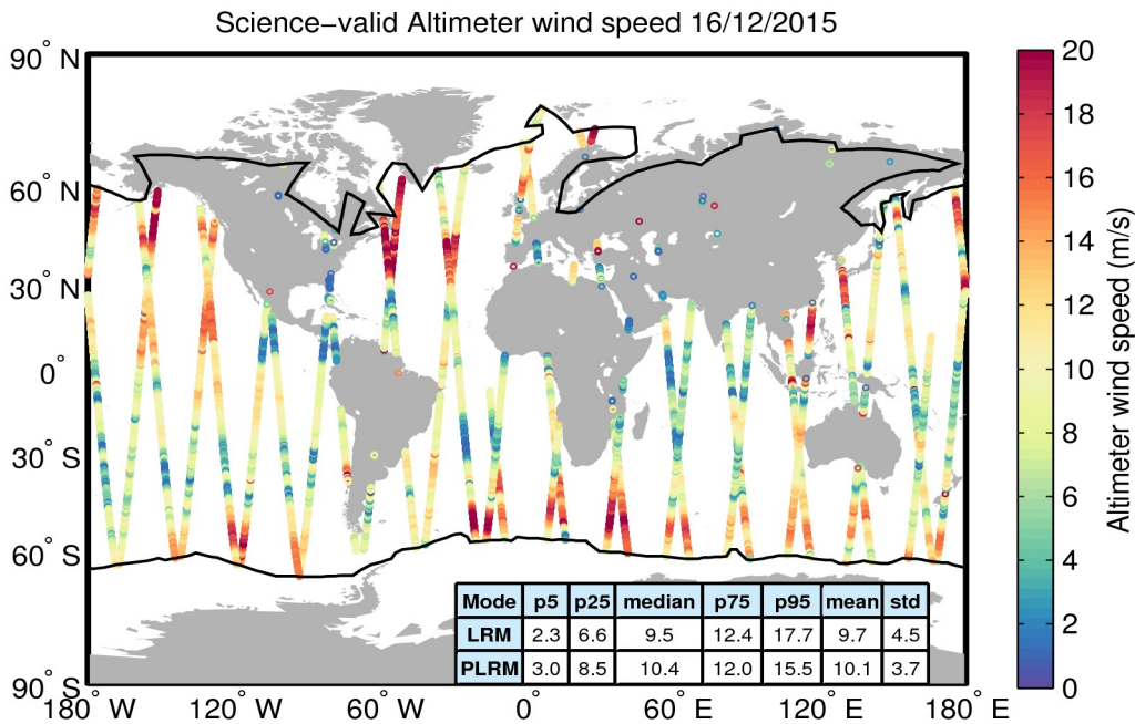
Figure 34. Geographical distribution of science-valid wind data over oceans and lakes for 16/12/2015. The statistical values shown in the table refer to the wind in m/s and are calculated separately for LRM and PLRM regions. The black lines mark the outer limit of the Arctic and Antarctic polar polygons. Gray circles denote records that have been rejected based on the editing criteria described in Table 5.
