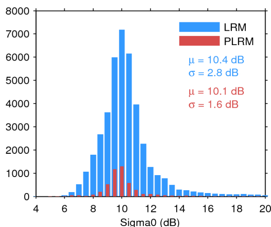
Figure 25. Histogram of flag-valid sigma0 over oceans and lakes for LRM (blue) and PLRM (red) for 16/12/2015. The mean ( \mu ) and standard deviation ( \sigma ) are also shown. Note that values outside [4 20] dB are excluded from the histogram for the sake of readability but not from the computation of \mu and \sigma .
