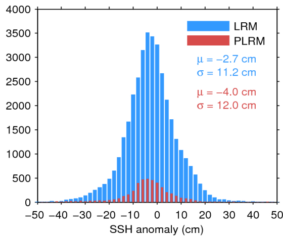
Figure 11. Histogram of science-valid SSH anomaly over oceans and lakes for LRM (blue) and PLRM (red) for 16/12/2015. The mean ( \mu ) and standard deviation ( \sigma ) are also shown. Note that values outside [-50 50] cm are excluded from the histogram for the sake of readability but not from the computation of \mu and \sigma .
