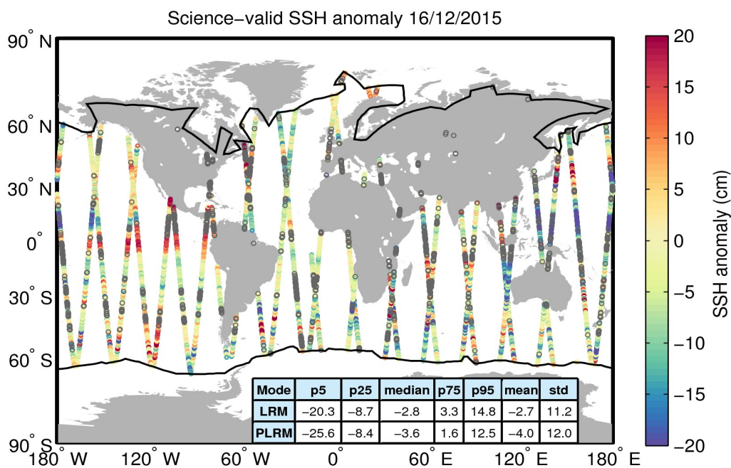
Figure 10. Geographical distribution of science-valid SSH anomaly data over oceans and lakes for 16/12/2015. The statistical values shown in the table refer to the SSH anomaly in cm and are calculated separately for LRM and PLRM regions. The black lines mark the outer limit of the Arctic and Antarctic polar polygons. Gray circles denote records that have been rejected based on the editing criteria described in Table 2.
