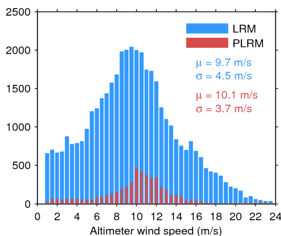
Figure 33. Histogram of flag-valid wind over oceans and lakes for LRM (blue) and PLRM (red) for 16/12/2015. The mean ( \mu ) and standard deviation ( \sigma ) are also shown. Note that values larger than 24 m/s are excluded from the histogram for the sake of readability but not from the computation of \mu and \sigma .
