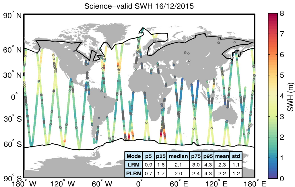
Figure 19. Geographical distribution of science-valid SWH data over oceans and lakes for 16/12/2015. The statistical values shown in the table refer to the SWH in m and are calculated separately for LRM and PLRM regions. The black lines mark the outer limit of the Arctic and Antarctic polar polygons. Gray circles denote records that have been rejected based on the editing criteria described in Table 3.
