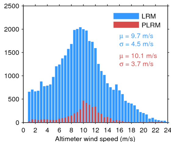
Figure 35. Histogram of science-valid wind over oceans and lakes for LRM (blue) and PLRM (red) for 16/12/2015. The mean ( \mu ) and standard deviation ( \sigma ) are also shown. Note that values larger than 24 m/s are excluded from the histogram for the sake of readability but not from the computation of \mu and \sigma .
