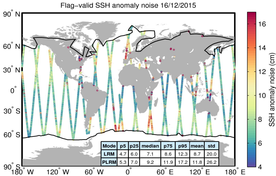
Figure 8. Geographical distribution of flag-valid 20-Hz SSH anomaly measurement noise over oceans and lakes for 16/12/2015. The statistical values shown in the table refer to the SSH anomaly noise and are calculated separately for LRM and PLRM regions. Measurements taken over polar polygons have been excluded from the computation of the statistical values. The black lines mark the outer limit of the Arctic and Antarctic polar polygons.
