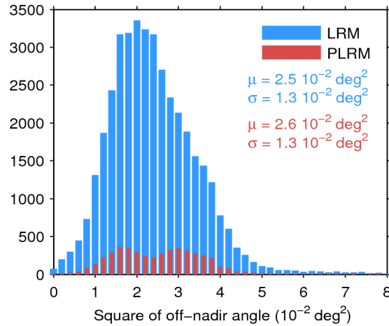
Figure 39. Histogram of flag-valid mispointing over oceans and lakes for LRM (blue) and PLRM (red) for 16/12/2015. Only positive values have been considered. The mean ( \mu ) and standard deviation ( \sigma ) are also shown. Note that values larger than 8 \cdot 10^{-2} \text{ deg}^2 are excluded from the histogram for the sake of readability but not from the computation of \mu and \sigma .
