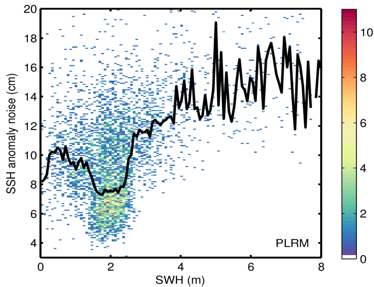
Figure 9. 2D histogram showing flag-valid SSH anomaly noise as a function of SWH for LRM (top) and PLRM (bottom) for 16/12/2015. The black line denotes the median SSH anomaly noise as a function of SWH.
