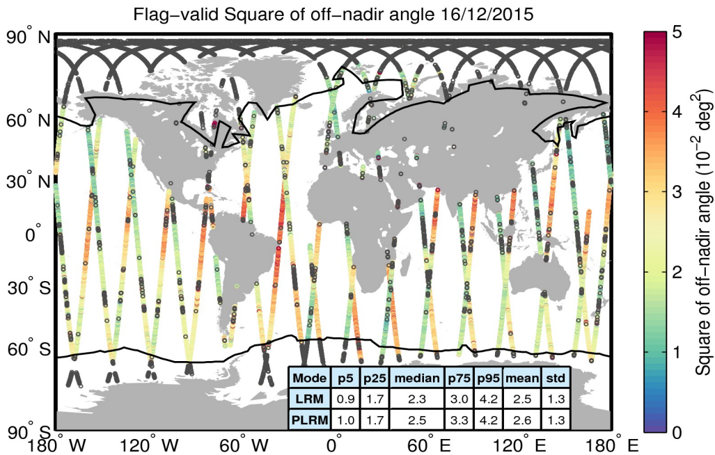
Figure 37. Geographical distribution of flag-valid mispointing data over oceans and lakes for 16/12/2015. The statistical values shown in the table refer to the mispointing in 10^{-2} deg 2 and are calculated separately for LRM and PLRM regions. Measurements taken over polar polygons have been excluded from the computation of the statistical values. The black lines mark the outer limit of the Arctic and Antarctic polar polygons. Gray circles denote negative values.
