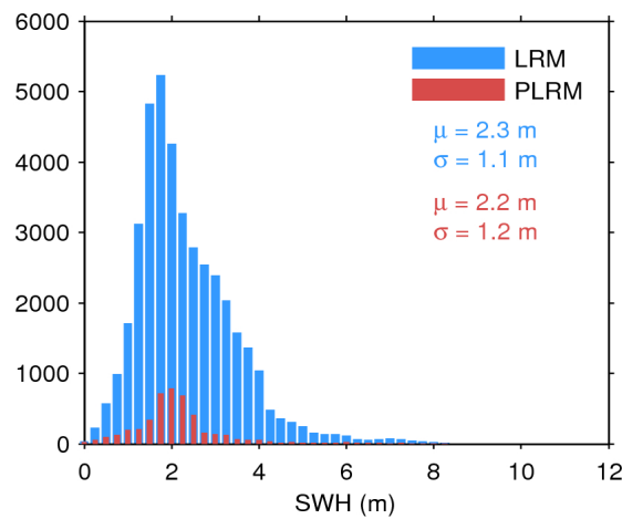
Figure 20. Histogram of science-valid SWH over oceans and lakes for LRM (blue) and PLRM (red) for 16/12/2015. The mean ( \mu ) and standard deviation ( \sigma ) are also shown. Note that values larger than 12 m are excluded from the histogram for the sake of readability but not from the computation of \mu and \sigma .
