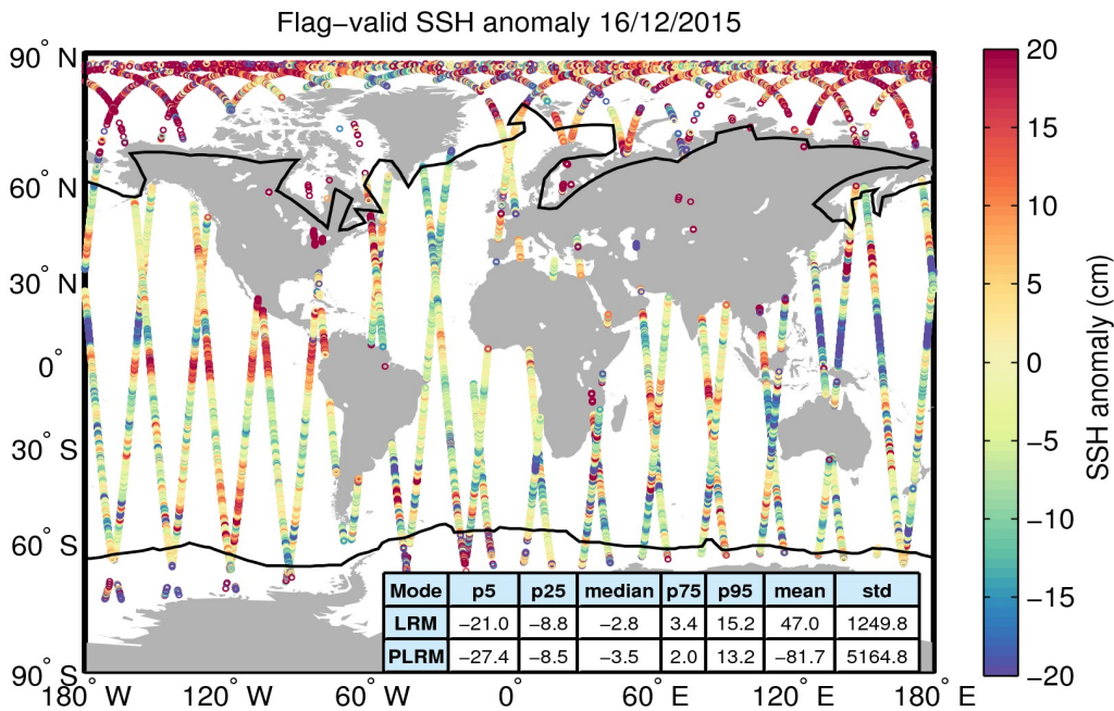
Figure 5. Geographical distribution of flag-valid 1-Hz SSH anomaly data over oceans and lakes for 16/12/2015. The statistical values shown in the table refer to the SSH anomaly in cm and are calculated separately for LRM and PLRM regions. Measurements taken over polar polygons have been excluded from the computation of the statistical values. The black lines mark the outer limit of the Arctic and Antarctic polar polygons.
