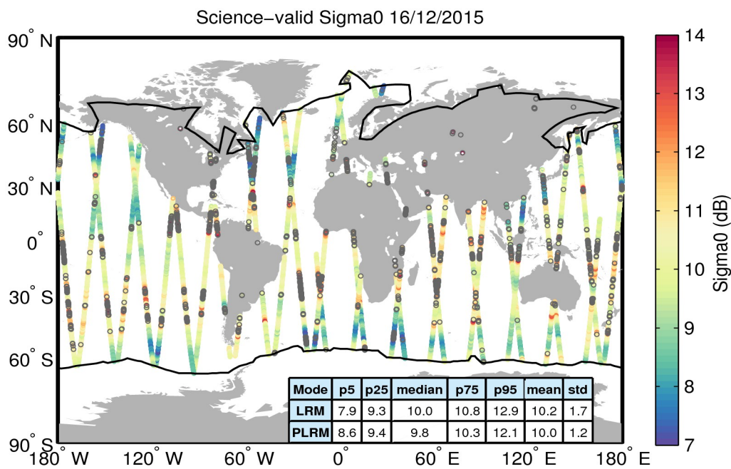
Figure 27. Geographical distribution of science-valid sigma0 data over oceans and lakes for 16/12/2015. The statistical values shown in the table refer to the sigma0 in dB and are calculated separately for LRM and PLRM regions. The black lines mark the outer limit of the Arctic and Antarctic polar polygons. Gray circles denote records that have been rejected based on the editing criteria described in Table 4.
