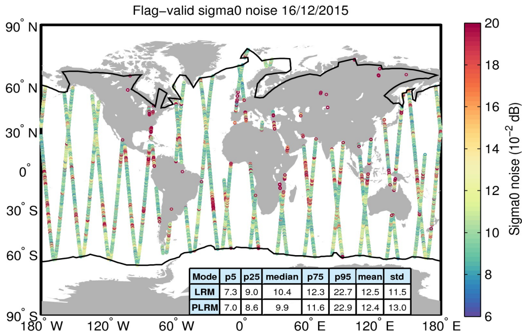
Figure 26. Geographical distribution of flag-valid 20-Hz sigma0 measurement noise over oceans and lakes for 16/12/2015. The statistical values shown in the table refer to the sigma0 noise and are calculated separately for LRM and PLRM regions. Measurements taken over polar polygons have been excluded from the computation of the statistical values. The black lines mark the outer limit of the Arctic and Antarctic polar polygons.
